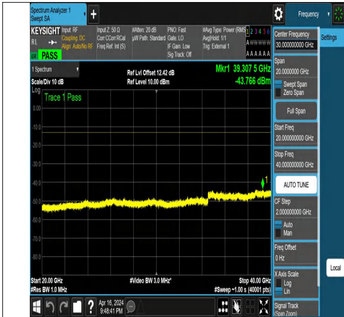
NTNV_N78-3450-3550_PC2_30_80_H_TID5_NS_01_20000_400
