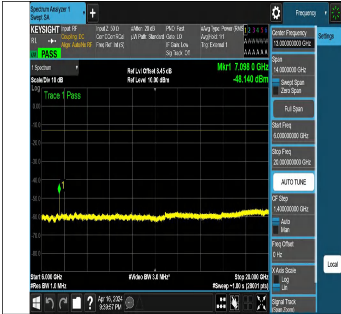
NTNV_N78-3450-3550_PC2_30_80_H_TID3_NS_01_6000_2000
