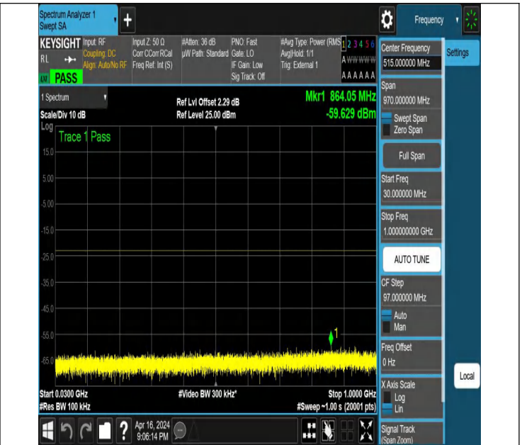
NTNV_N78-3450-3550_PC2_30_80_M_TID3_NS_01_30_1000_#1
