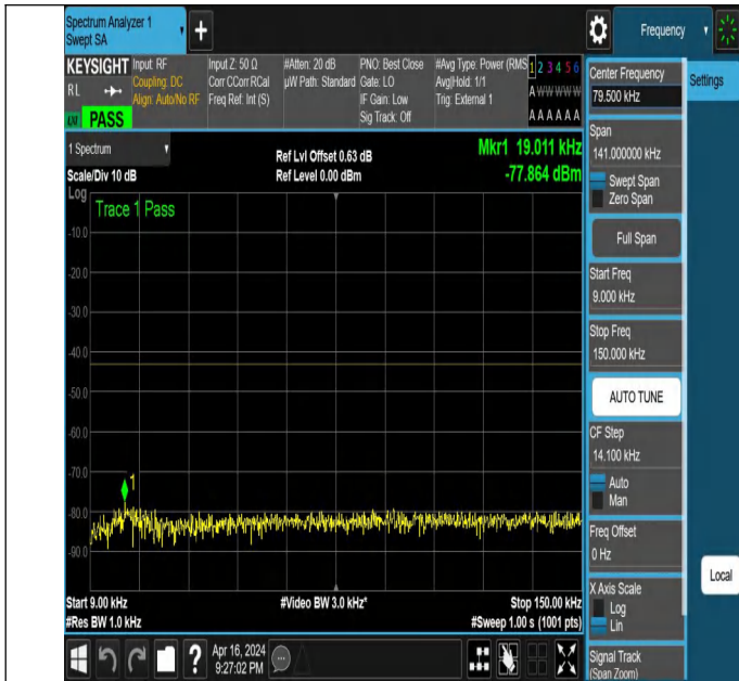
NTNV_N78-3450-3550_PC2_30_80_H_TID2_NS_01_0.009_0.15
