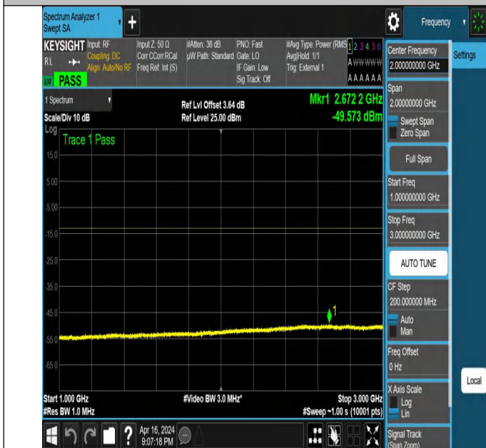
NTNV_N78-3450-3550_PC2_30_80_M_TID3_NS_01_1000_300_0_#1
