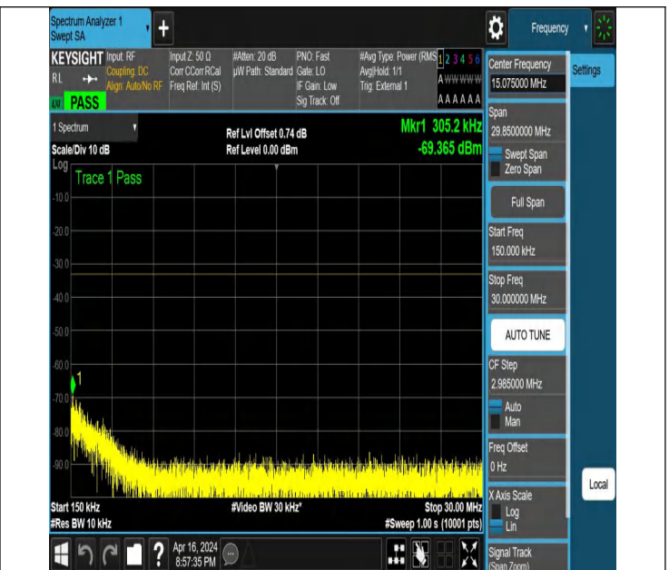
NTNV_N78-3450-3550_PC2_30_80_M_TID2_NS_01_0.15_30_#
