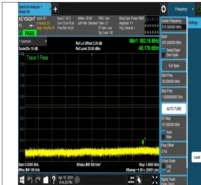
NTNV_N78-3450-3550_PC2_30_80_H_TID5 NS_01_30_1000_#
