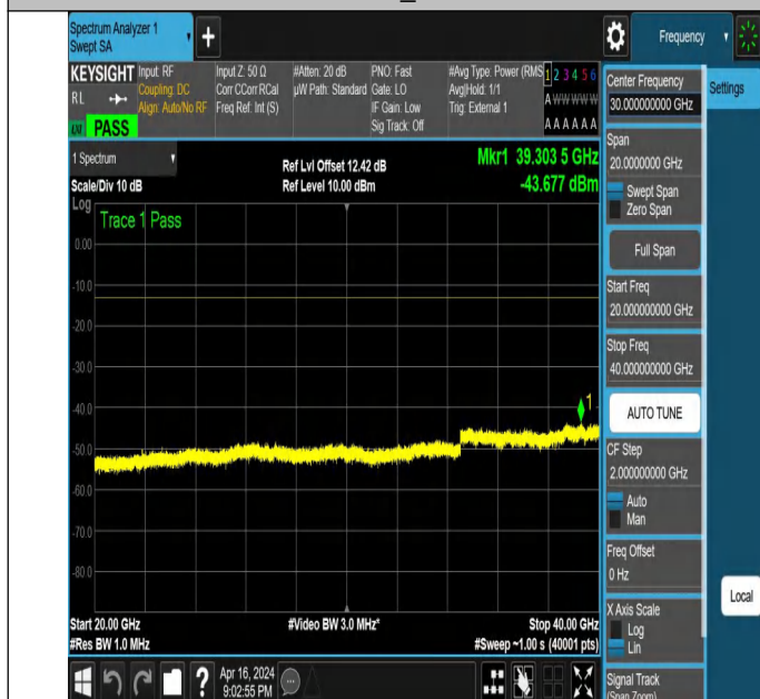
NTNV_N78-3450-3550_PC2_30_80_M_TID2_NS_01_20000_40000 #1
