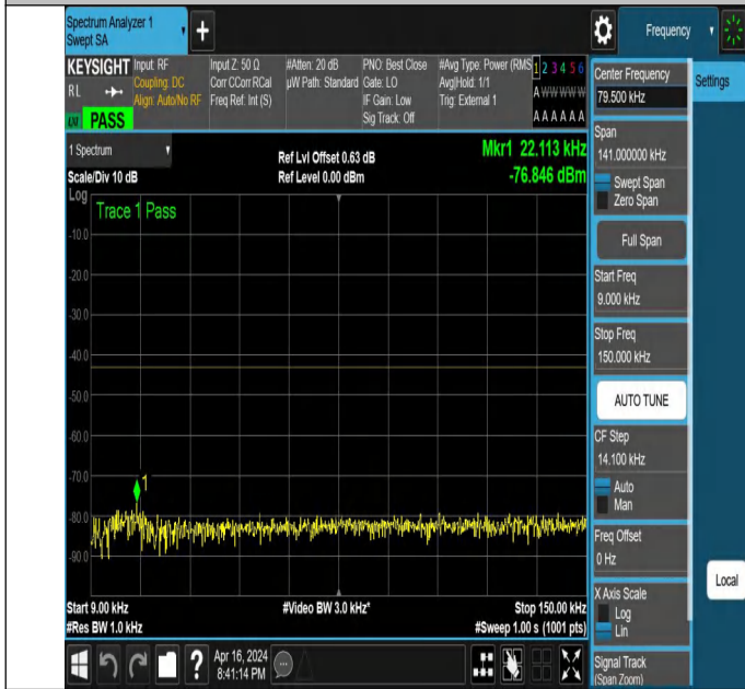
NTNV_N78-3450-3550_PC2_30_80_L_TID5_NS_01_0.009_0.15
