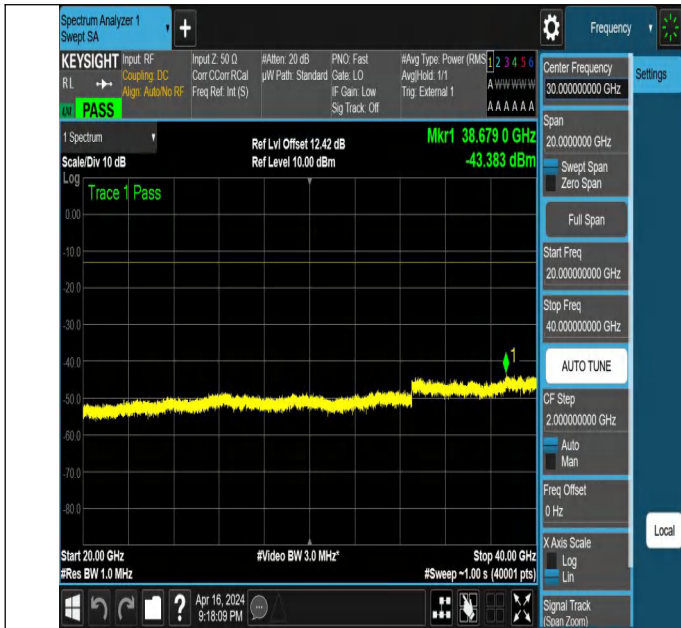
NTNV_N78-3450-3550_PC2_30_80_M_TID5_NS_01_20000_40
