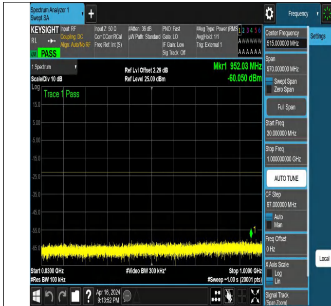
NTNV_N78-3450-3550_PC2_30_80_M_TID5_NS_01_30_1000_
