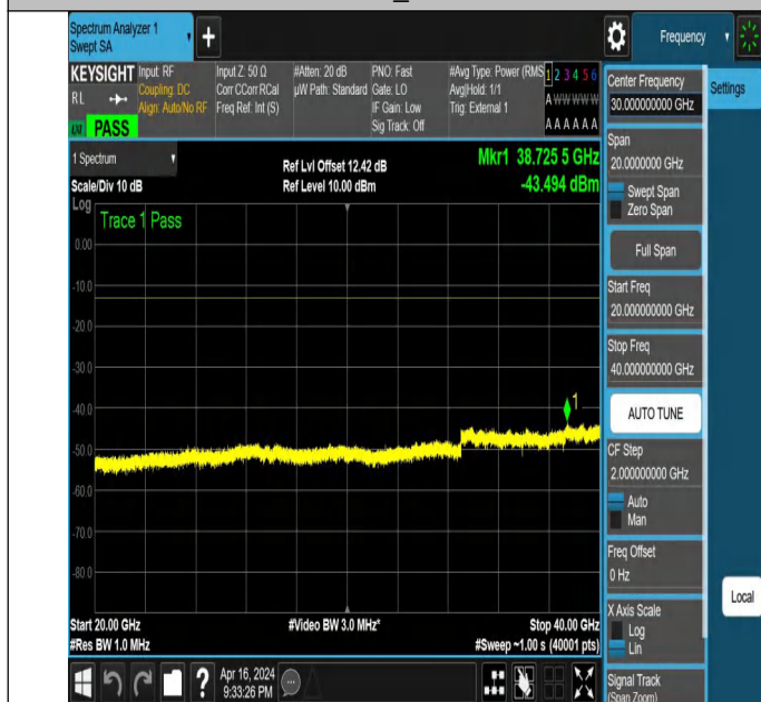
NTNV_N78-3450-3550_PC2_30_80_H_TID2_NS_01_20000_400
