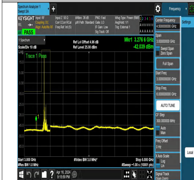
NTNV_N78-3450-3550_PC2_30_80_M_TID5_NS_01_3000_600
