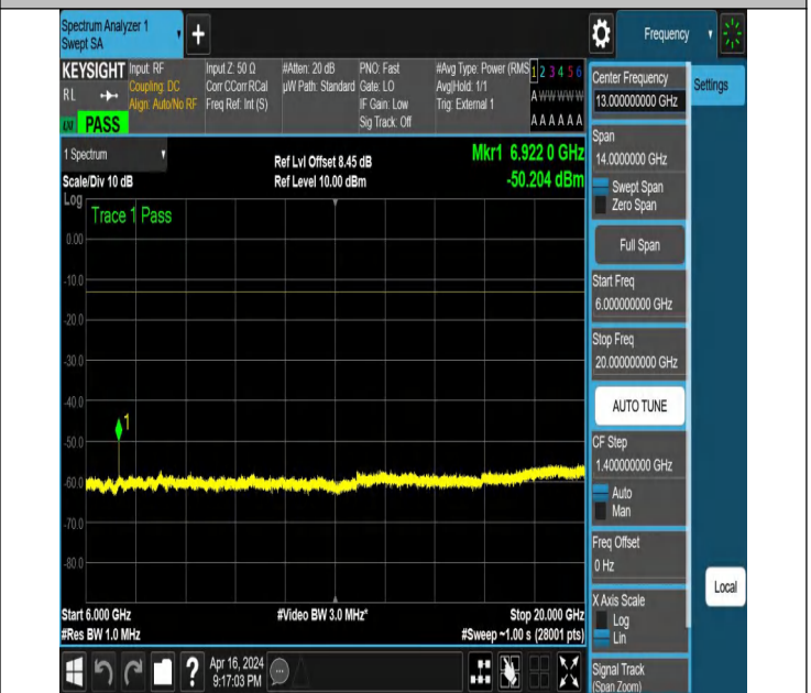
NTNV_N78-3450-3550_PC2_30_80_M_TID5_NS_01_6000_200
