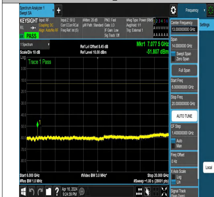
NTNV_N78-3450-3550_PC2_30_80_M_TID6_NS_01_6000_200 00 #1
