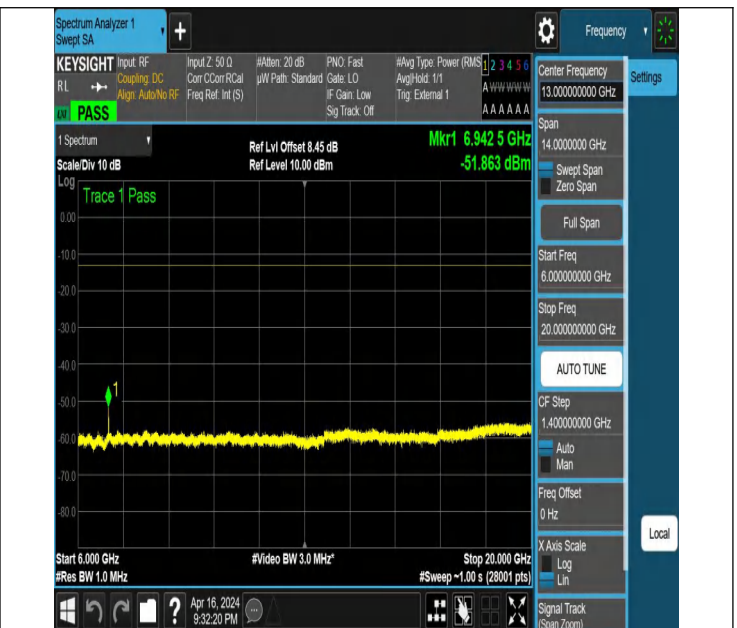
NTNV_N78-3450-3550_PC2_30_80_H_TID2_NS_01_6000_2000
