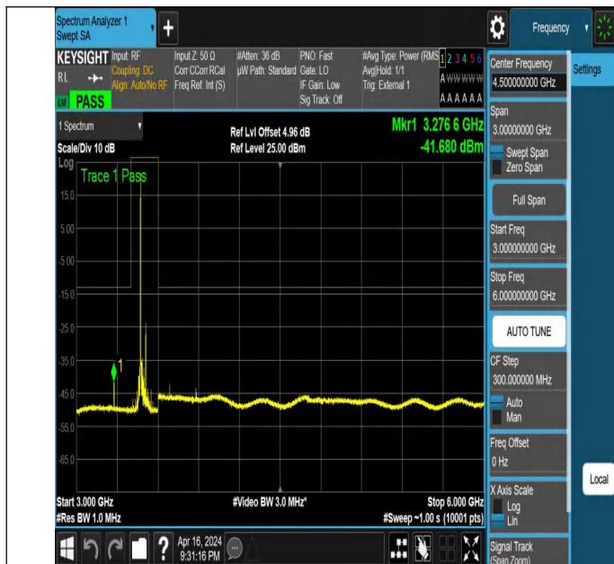
NTNV_N78-3450-3550_PC2_30_80_H_TID2_NS_01_3000_6000
