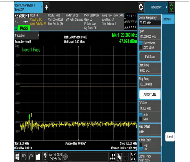
NTNV_N78-3450-3550_PC2_30_80_H_TID6_NS_01_0.009_0.15
