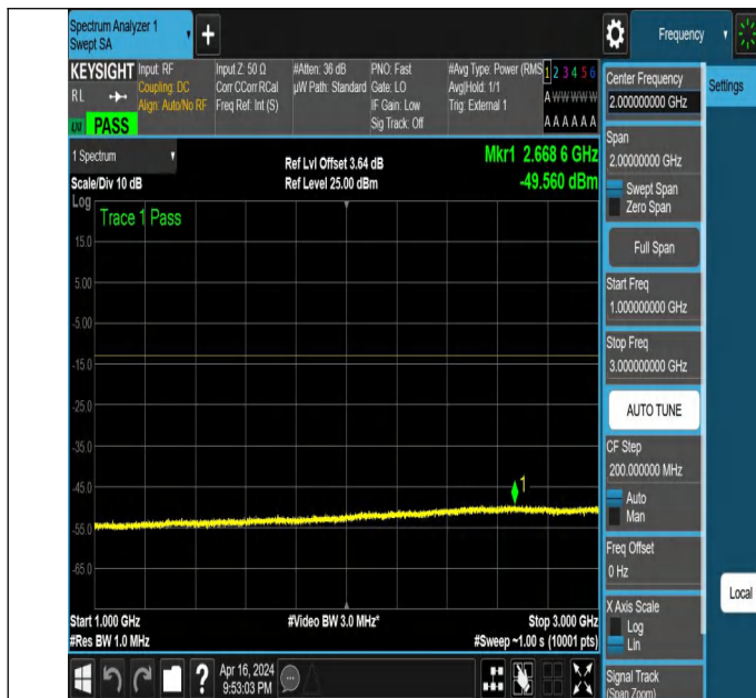
NTNV_N78-3450-3550_PC2_30_80_H_TID6 NS_01_1000_3000
