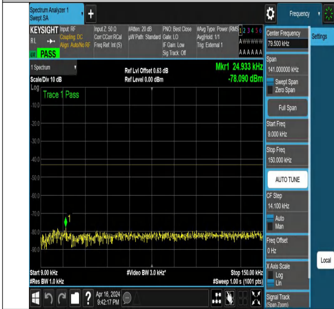
NTNV_N78-3450-3550_PC2_30_80_H_TID5_NS_01_0.009_0.15
