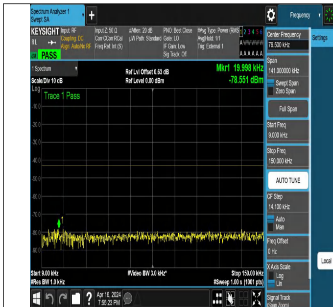
NTNV_N78-3450-3550_PC2_30_70_H_TID2_NS_01_0.009_0.15
