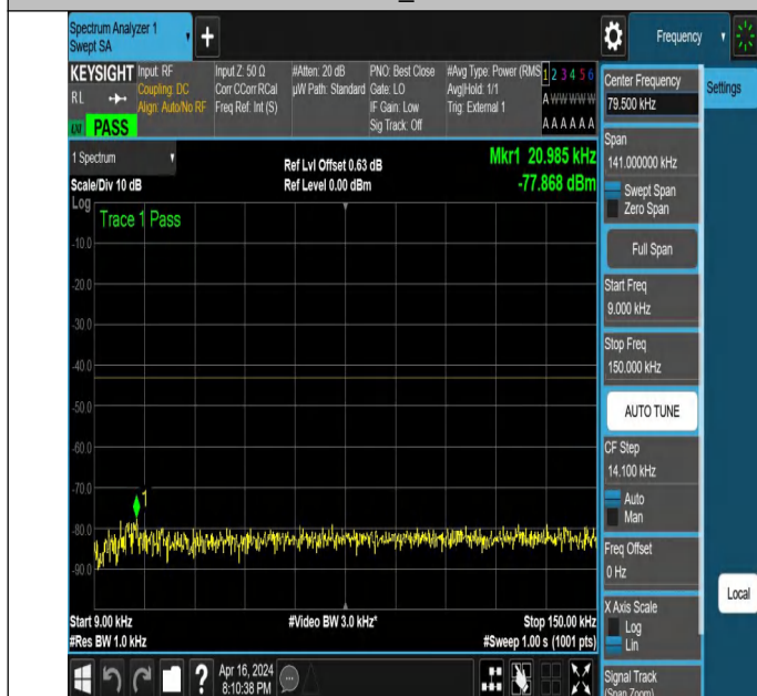
NTNV_N78-3450-3550_PC2_30_70_H_TID5_NS_01_0.009_0.15
