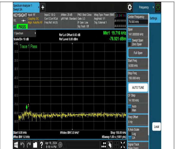
NTNV_N78-3450-3550_PC2_30_70_H_TID6_NS_01_0.009_0.15 #1
