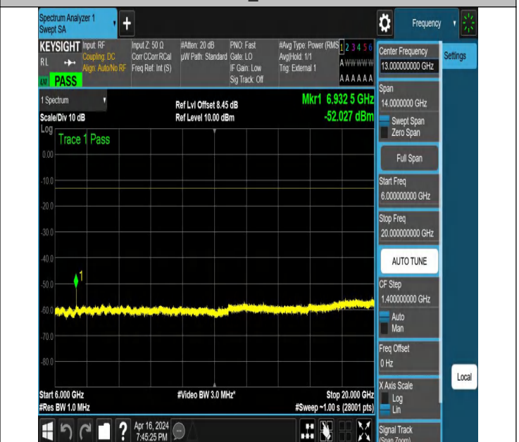
NTNV_N78-3450-3550_PC2_30_70_M_TID5_NS_01_6000_200 00 #1
