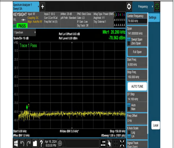
NTNV_N78-3450-3550_PC2_30_70_H_TID3_NS_01_0.009_0.15
