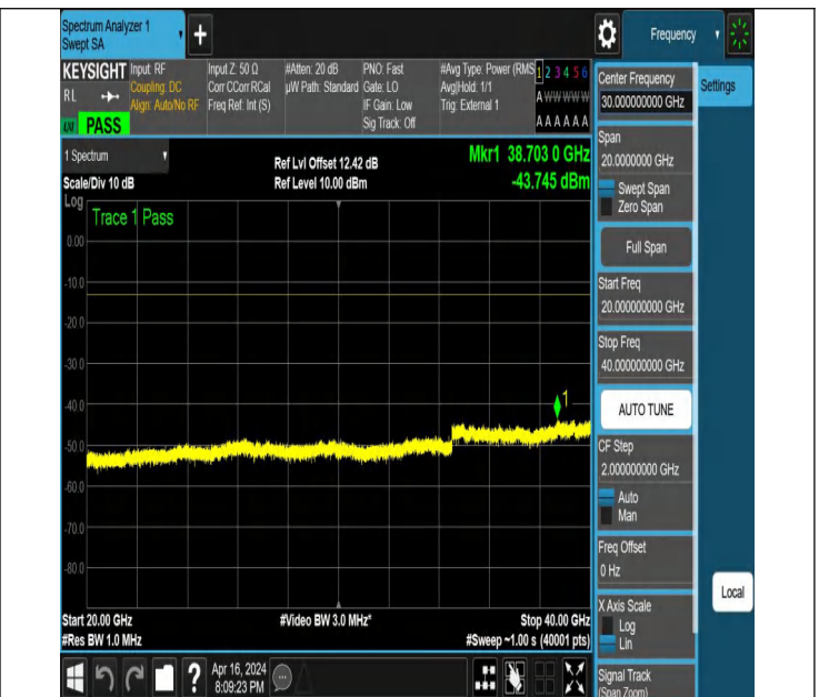
NTNV_N78-3450-3550_PC2_30_70_H_TID3_NS_01_20000_400 00 #1
