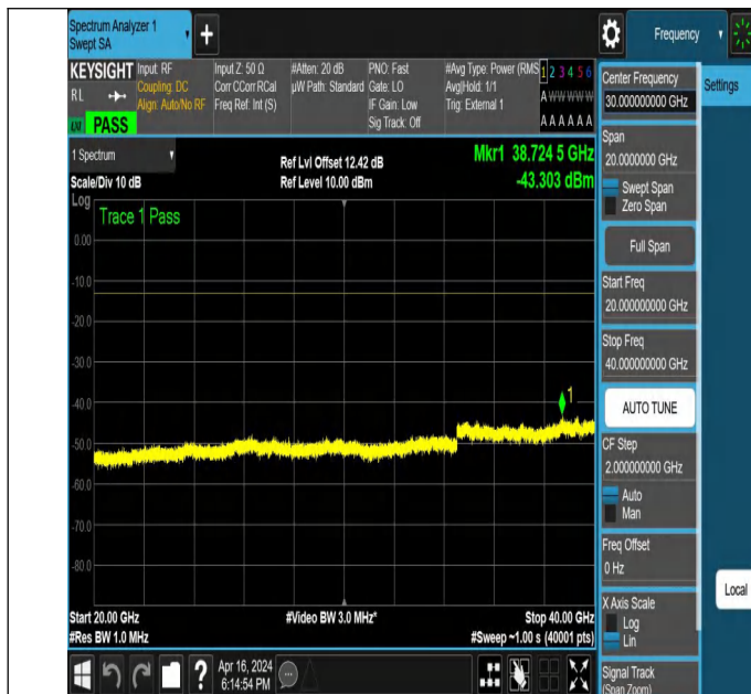
NTNV_N78-3450-3550_PC2_30_60_M_TID5_NS_01_20000_40 000 #1
