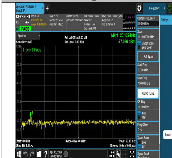
NTNV_N78-3450-3550_PC2_30_60_M_TID5_NS_01_0.009_0.1 5 #1
