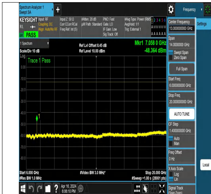
NTNV_N78-3450-3550_PC2_30_60_M_TID3_NS_01_6000_200 00 #1
