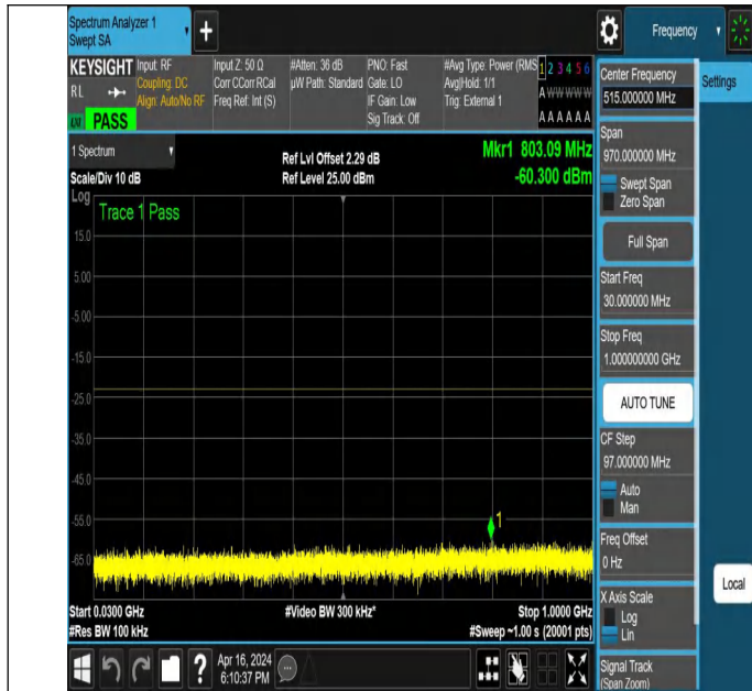
NTNV_N78-3450-3550_PC2_30_60_M_TID5_NS_01_30_1000_
