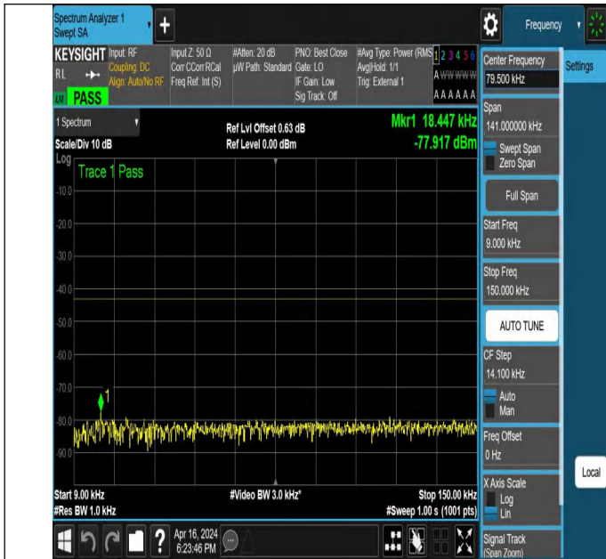
NTNV_N78-3450-3550_PC2_30_60_H_TID2_NS_01_0.009_0.15
