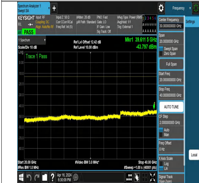
NTNV_N78-3450-3550_PC2_30_60_H_TID2_NS_01_20000_400
