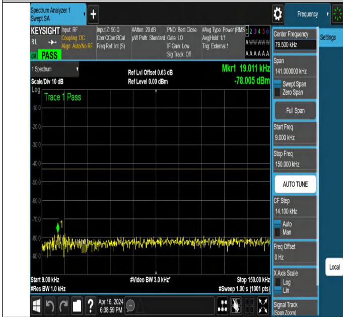
NTNV_N78-3450-3550_PC2_30_60_H_TID5_NS_01_0.009_0.15
