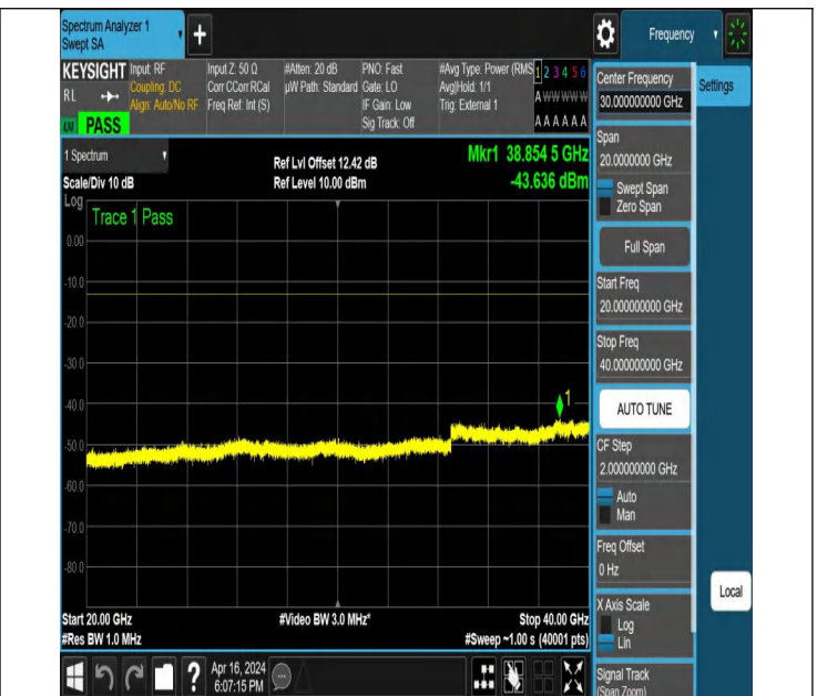
NTNV_N78-3450-3550_PC2_30_60_M_TID3_NS_01_20000_40 000 #1
