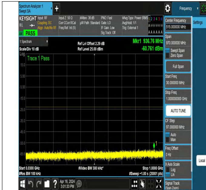
NTNV_N78-3450-3550_PC2_30_40_M_TID5_NS_01_30_1000_
