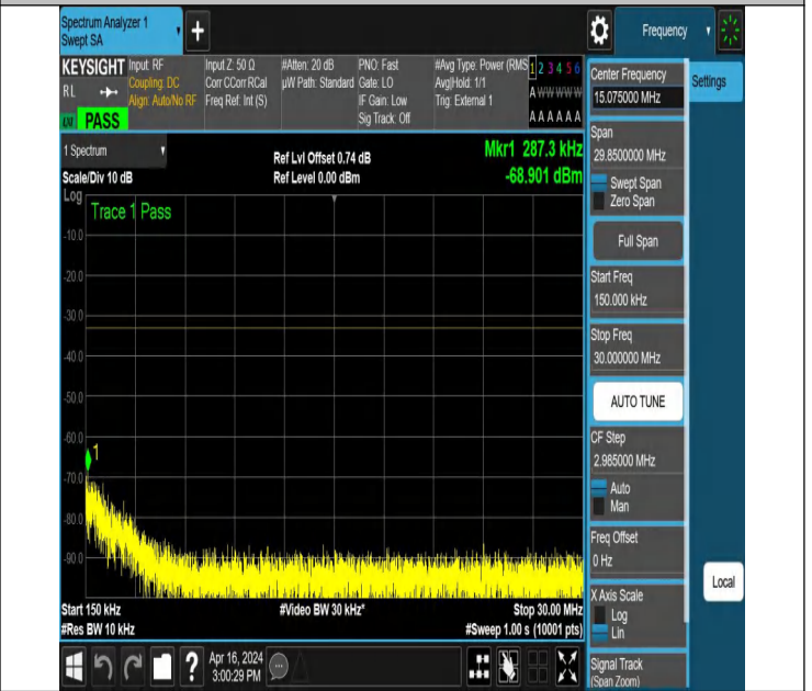
NTNV_N78-3450-3550_PC2_30_40_M_TID5_NS_01_0.15_30_#1
