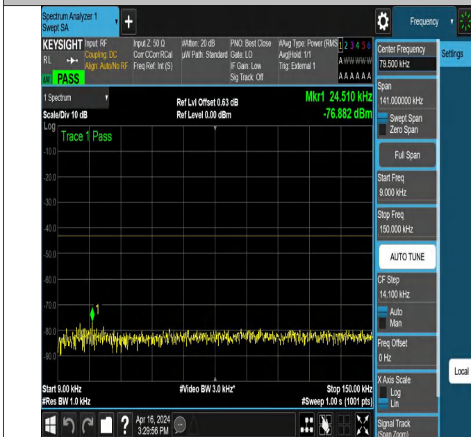
NTNV_N78-3450-3550_PC2_30_40_H_TID5_NS_01_0.009_0.15
