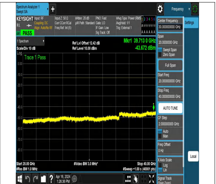
NTNV_N78-3450-3550_PC2_30_30_M_TID3_NS_01_20000_40 000 #1
