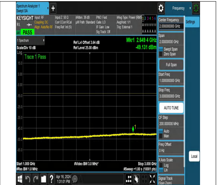
NTNV_N78-3450-3550_PC2_30_30_M_TID5_NS_01_1000_300
