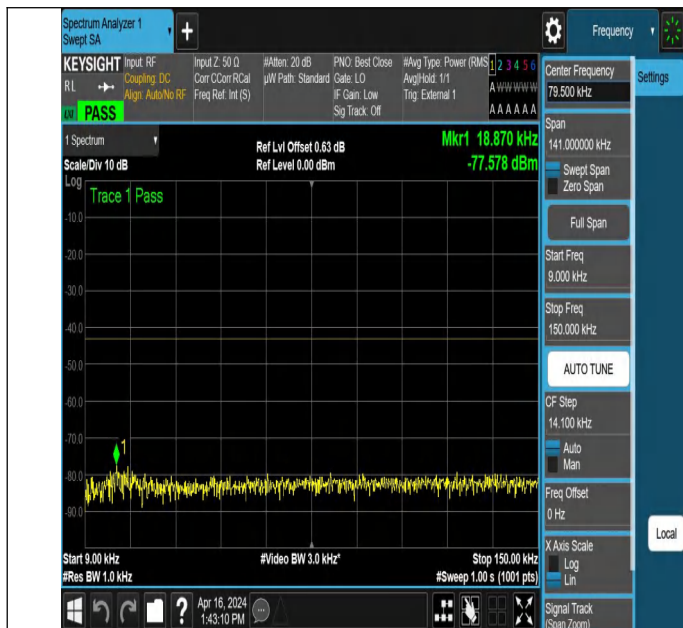
NTNV_N78-3450-3550_PC2_30_30_H_TID2_NS_01_0.009_0.15
