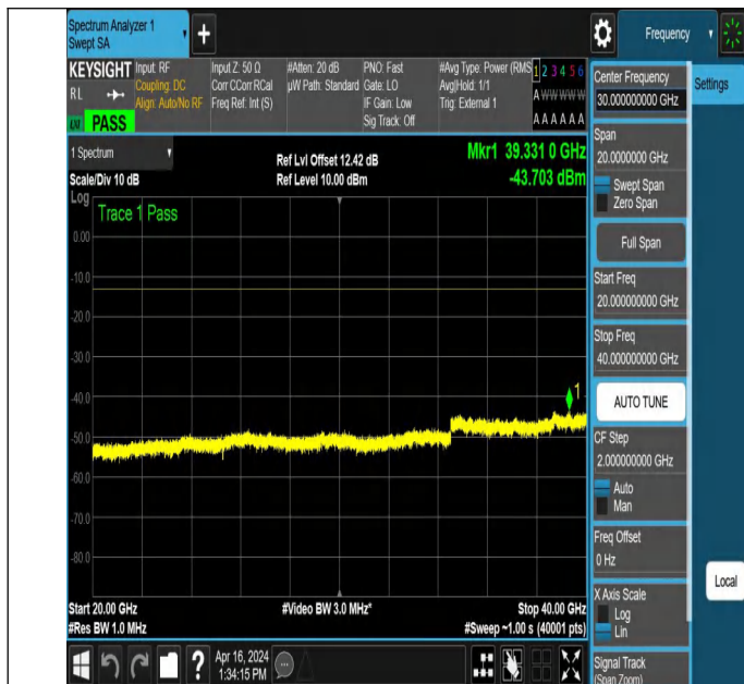
NTNV_N78-3450-3550_PC2_30_30_M_TID5_NS_01_20000_40 000 #1
