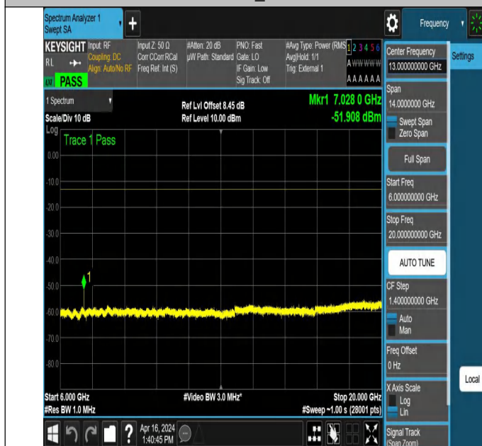
NTNV_N78-3450-3550_PC2_30_30_M_TID6_NS_01_6000_200 00 #1
