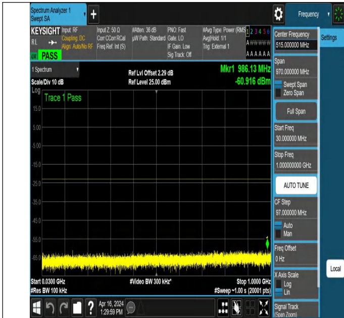
NTNV_N78-3450-3550_PC2_30_30_M_TID5_NS_01_30_1000_
