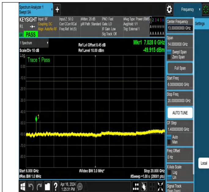
NTNV_N78-3450-3550_PC2_30_30_M_TID3_NS_01_6000_200 00 #1
