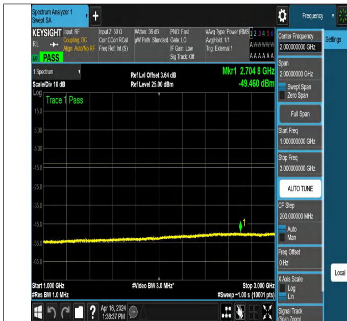
NTNV_N78-3450-3550_PC2_30_30_M_TID6_NS_01_1000_300 0 #1
