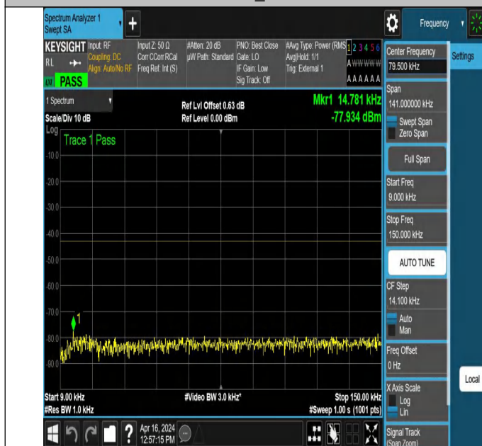
NTNV_N78-3450-3550_PC2_30_30_L_TID5_NS_01_0.009_0.15 #1
