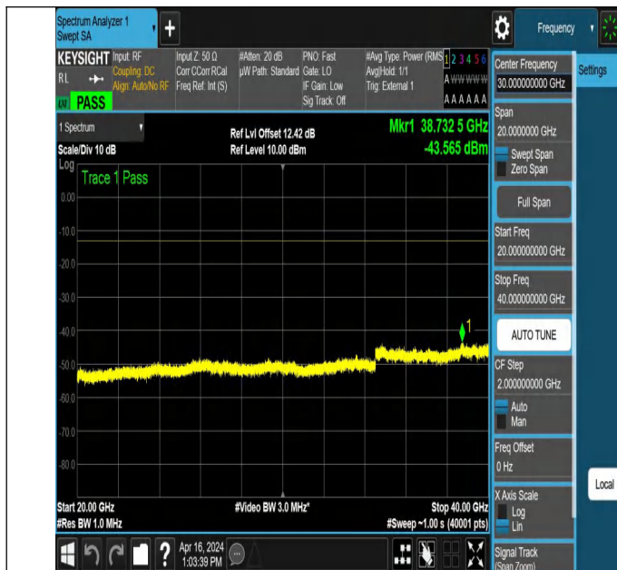
NTNV_N78-3450-3550_PC2_30_30_L_TID5_NS_01_20000_400 00 #1
