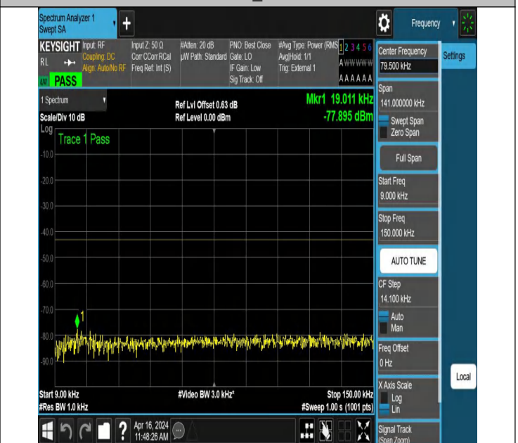
NTNV_N78-3450-3550_PC2_30_20_M_TID3_NS_01_0.009_0.1 5_#1
