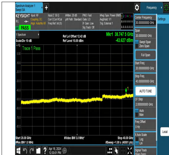
NTNV_N78-3450-3550_PC2_30_20_H_TID5_NS_01_20000_400 00 #1
