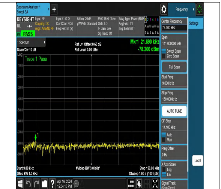
NTNV_N78-3450-3550_PC2_30_20_H_TID6_NS_01_0.009_0.15 #1
