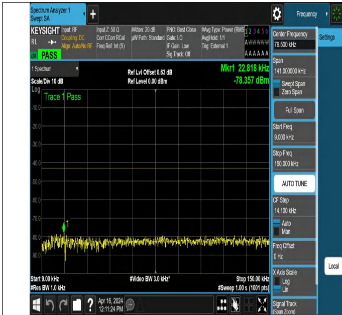
NTNV_N78-3450-3550_PC2_30_20_H_TID2_NS_01_0.009_0.15
