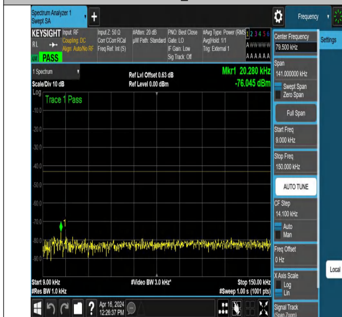
NTNV_N78-3450-3550_PC2_30_20_H_TID5_NS_01_0.009_0.15
