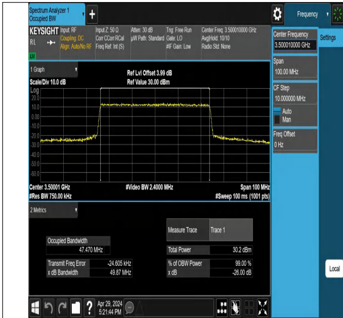
NTNV-N78-3450-3550-PC2-30-50-M-CP-QPSK-Outter_Full-Ant1- PASS
