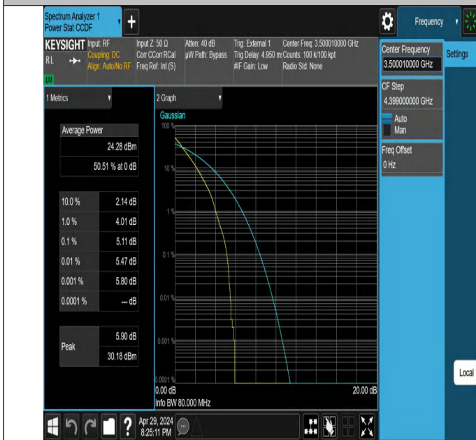
NTNV-N78-3450-3550-PC2-30-80-M-DFT-PI2BPSK-Outer_Full-P
