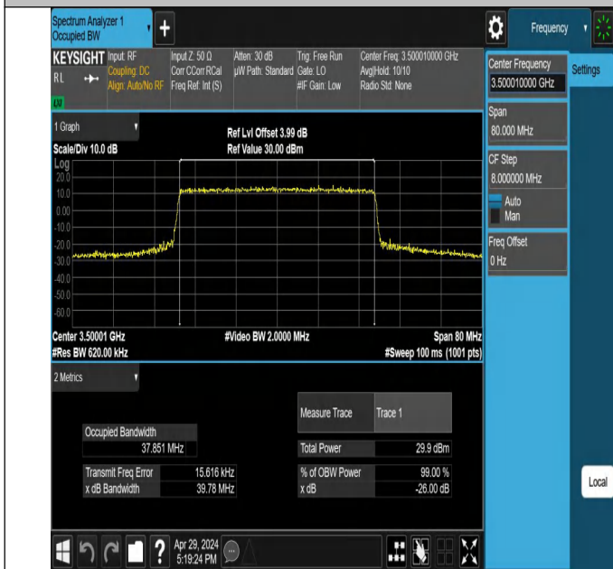
NTNV-N78-3450-3550-PC2-30-40-M-CP-64QAM-Outer_Full-Ant 1-PASS
