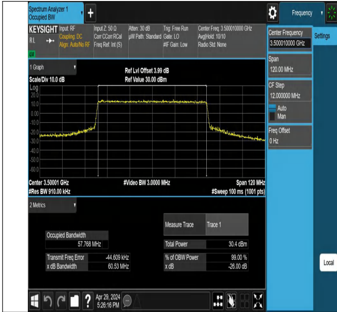
NTNV-N78-3450-3550-PC2-30-60-M-CP-QPSK-Outter_Full-Ant1-
