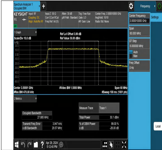
NTNV-N78-3450-3550-PC2-30-30-M-CP-QPSK-Outer_Full-Ant1- PASS
