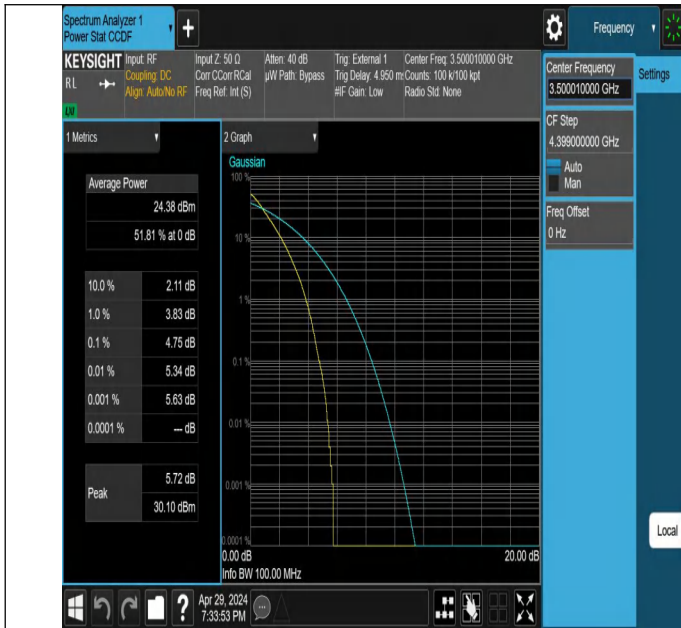
NTNV-N78-3450-3550-PC2-30-100-M-DFT-PI2BPSK-Outter_Full-P
