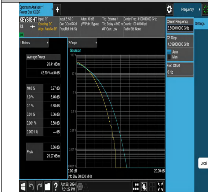
NTNV-N78-3450-3550-PC2-30-80-M-DFT-256QAM-Outer_Full-PA
