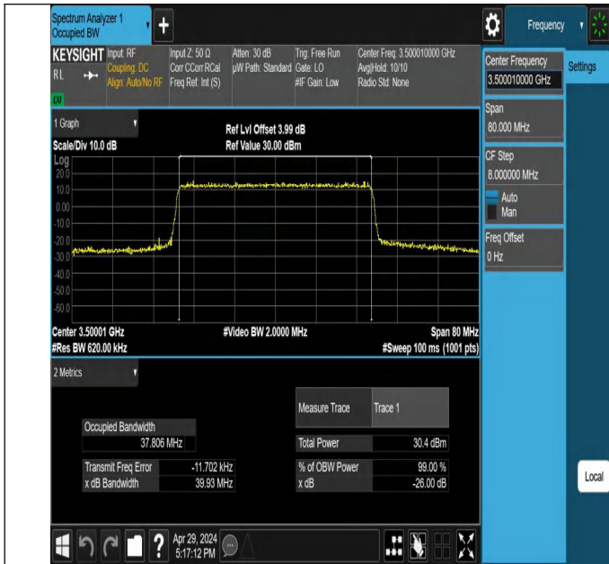
NTNV-N78-3450-3550-PC2-30-40-M-CP-QPSK-Outer_Full-Ant1- PASS
