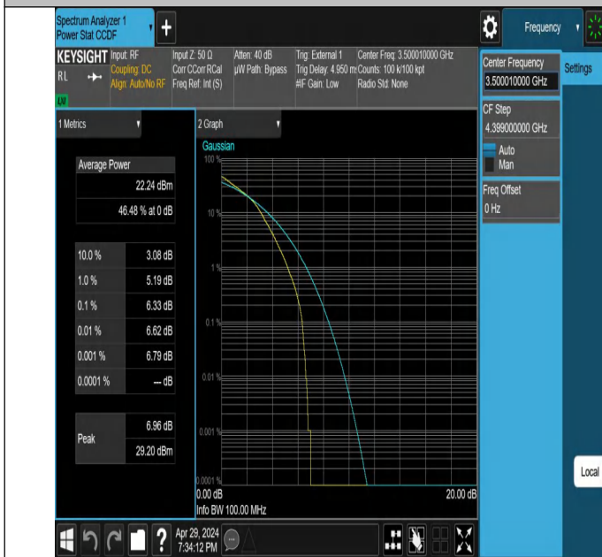
NTNV-N78-3450-3550-PC2-30-100-M-DFT-16QAM-Outter_Full-PA
