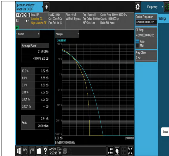
NTNV-N78-3450-3550-PC2-30-70-M-DFT-64QAM-Outer_Full-PAS
