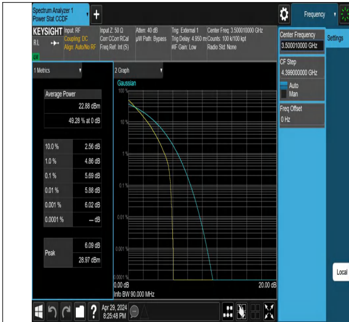
NTNV-N78-3450-3550-PC2-30-90-M-DFT-QPSK-Outter_Full-PASS
