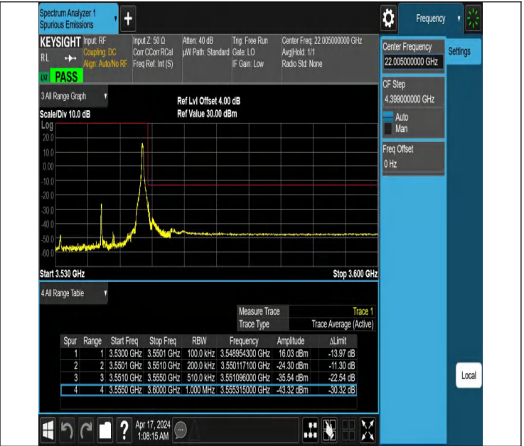
NTNV_N78-3450-3550_PC2_30_20_H_TID3_#1
