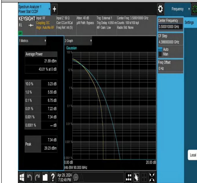
NTNV-N78-3450-3550-PC2-30-90-M-DFT-64QAM-Outter_Full-PAS S
