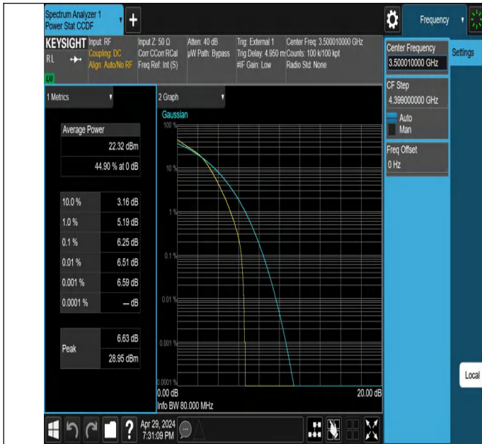
NTNV-N78-3450-3550-PC2-30-80-M-DFT-16QAM-Outer_Full-PAS
