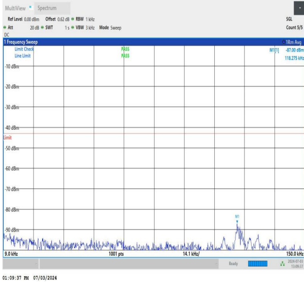
NTNV_DC_26A_n77A-3700-3980_PC2_30_5+90_M+M_TID1_N S_01_0.009_0.15_#1
