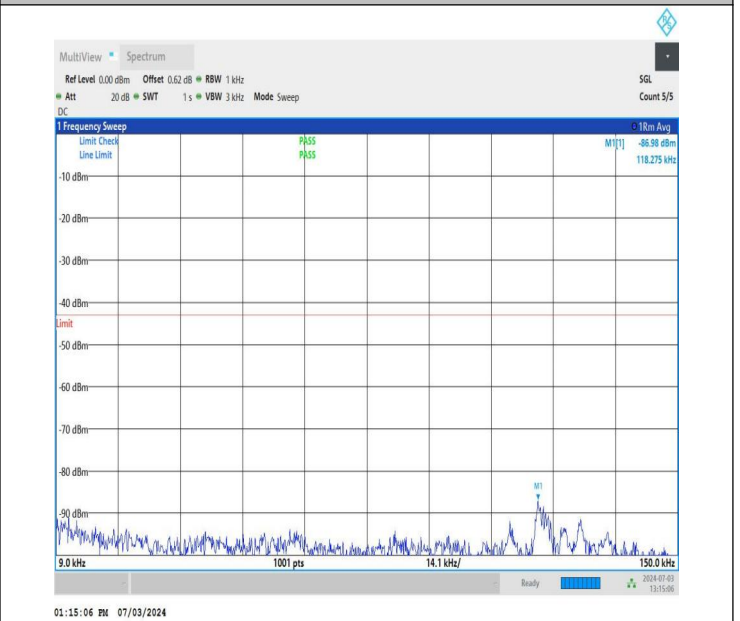
NTNV_DC_26A_n77A-3700-3980_PC2_30_5+90_M+H_TID2_N S_01_0.009_0.15_#1
