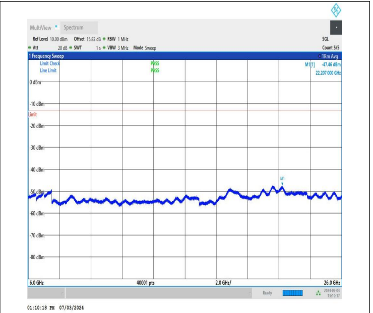
NTNV_DC_26A_n77A-3700-3980_PC2_30_5+90_M+M_TID1_N S_01_6000_26000_#1
