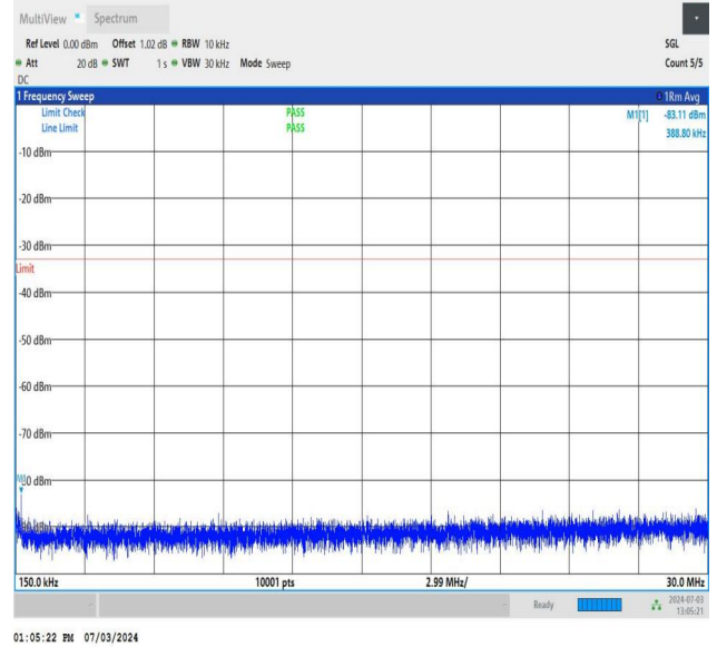
NTNV_DC_26A_n77A-3700-3980_PC2_30_5+90_M+L_TID1_NS_01_0.15_30_#1
