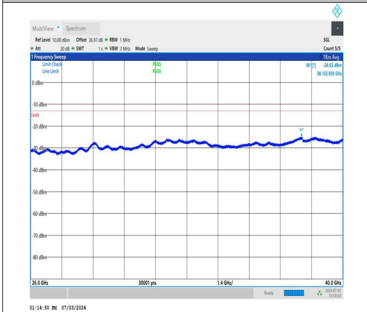
NTNV_DC_26A_n77A-3700-3980_PC2_30_5+90_M+H_TID1_N S_01_26000_40000_#1
