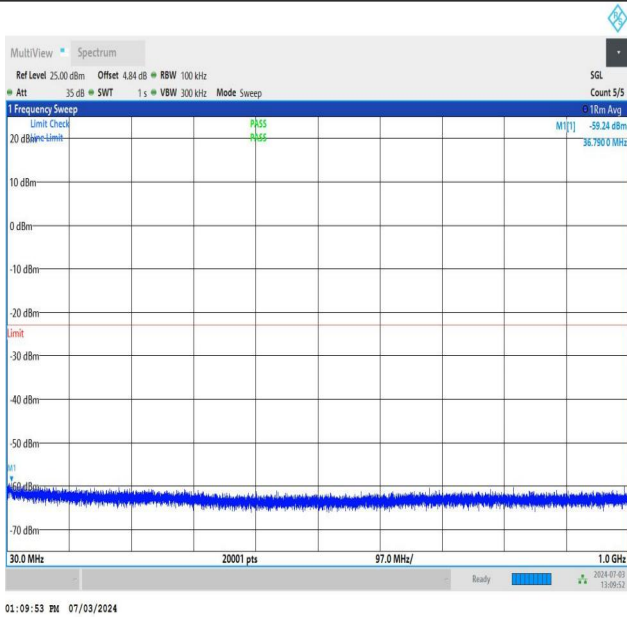
NTNV_DC_26A_n77A-3700-3980_PC2_30_5+90_M+M_TID1_N S_01_30_1000_#1
