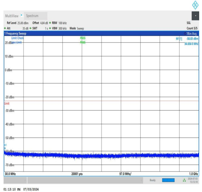
NTNV_DC_26A_n77A-3700-3980_PC2_30_5+90_M+M_TID5_N S_01_30_1000_#1
