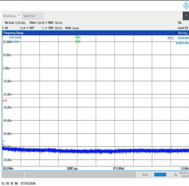
NTNV_DC_26A_n77A-3700-3980_PC2_30_5+90_M+L_TID1_NS_01_30_1000_#1
