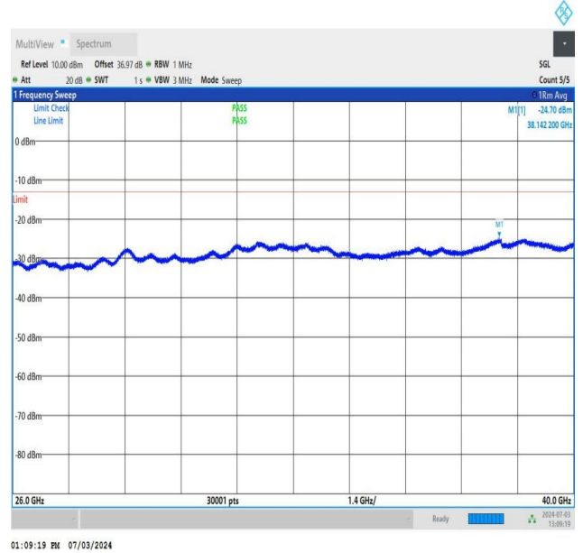
NTNV_DC_26A_n77A-3700-3980_PC2_30_5+90_M+L_TID5_NS_01_26000_40000_#1
