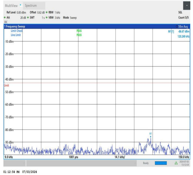
NTNV_DC_26A_n77A-3700-3980_PC2_30_5+90_M+M_TID5_N S_01_0.009_0.15_#1
