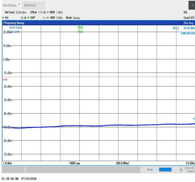
NTNV_DC_26A_n77A-3700-3980_PC2_30_5+90_M+L_TID5_NS_01_1000_3000_#1
