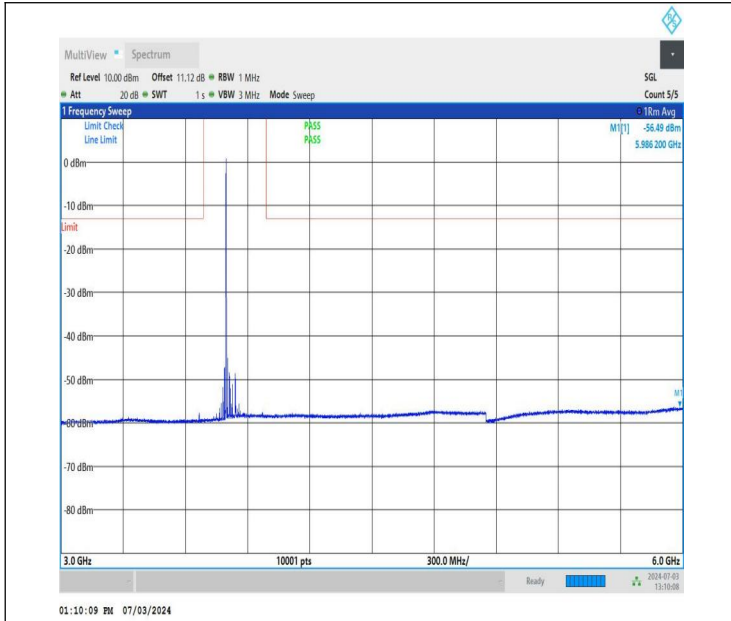
NTNV_DC_26A_n77A-3700-3980_PC2_30_5+90_M+M_TID1_N S_01_3000_6000_#1
