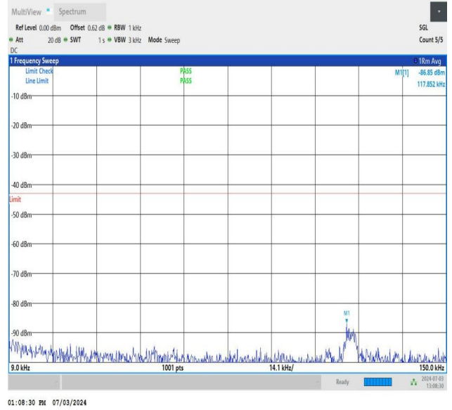
NTNV_DC_26A_n77A-3700-3980_PC2_30_5+90_M+L_TID5_NS_01_0.009_0.15_#1
