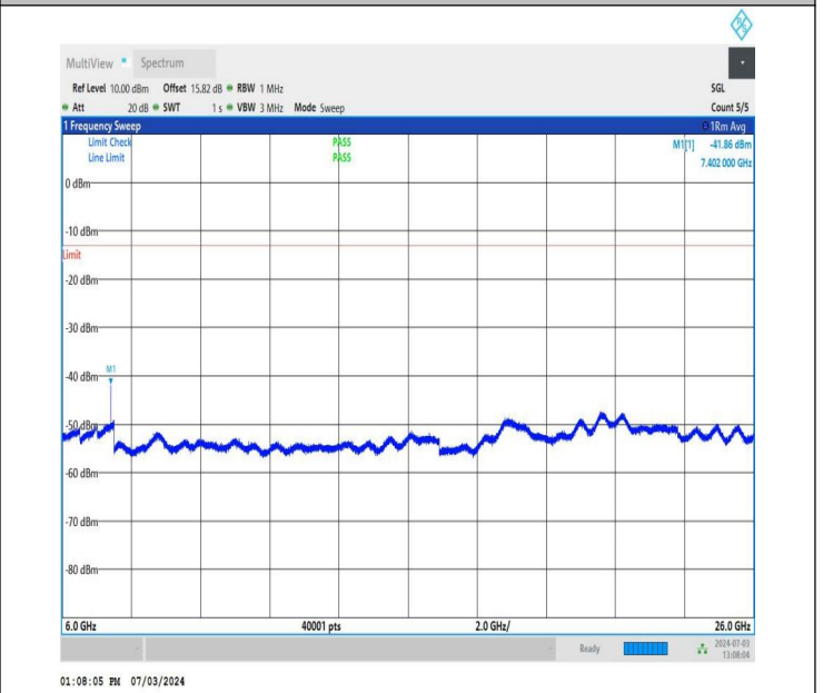
NTNV_DC_26A_n77A-3700-3980_PC2_30_5+90_M+L_TID4_NS_01_6000_26000_#1
