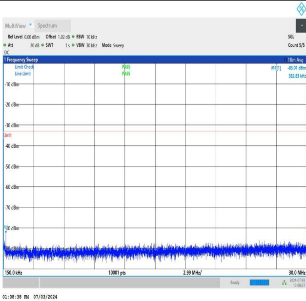
NTNV_DC_26A_n77A-3700-3980_PC2_30_5+90_M+L_TID5_NS_01_0.15_30_#1
