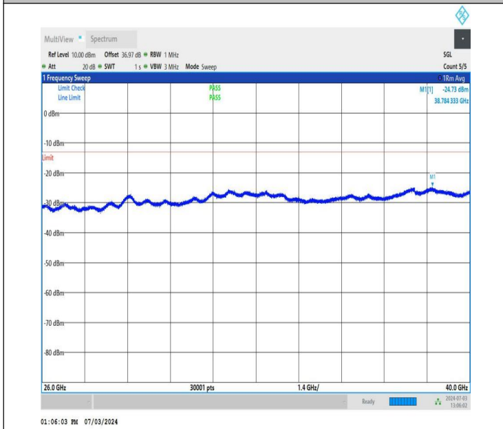
NTNV_DC_26A_n77A-3700-3980_PC2_30_5+90_M+L_TID1_NS_01_26000_40000_#1
