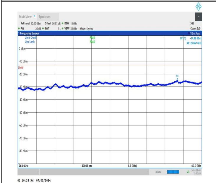
NTNV_DC_26A_n77A-3700-3980_PC2_30_5+90_M+M_TID1_N S_01_26000_40000_#1
