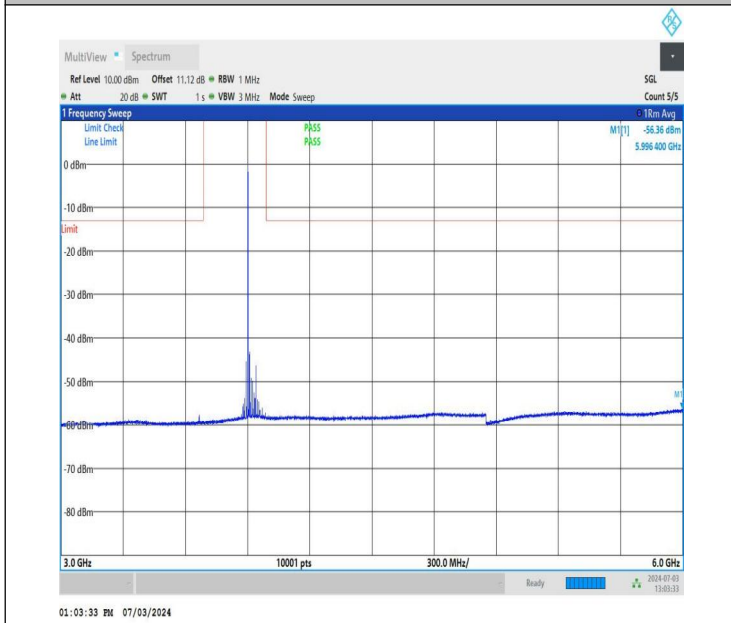
NTNV_DC_26A_n77A-3700-3980_PC2_30_5+80_M+H_TID4_N S_01_3000_6000_#1
