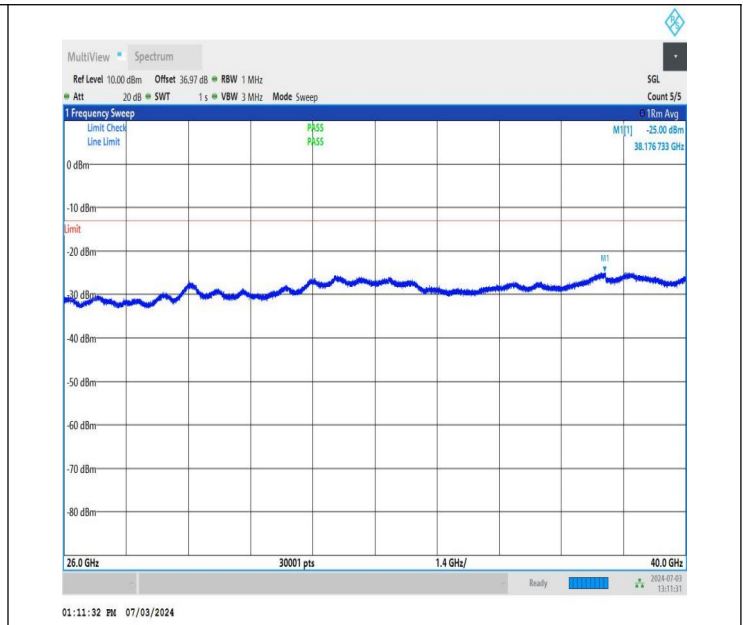
NTNV_DC_26A_n77A-3700-3980_PC2_30_5+90_M+M_TID2_N S_01_26000_40000_#1
