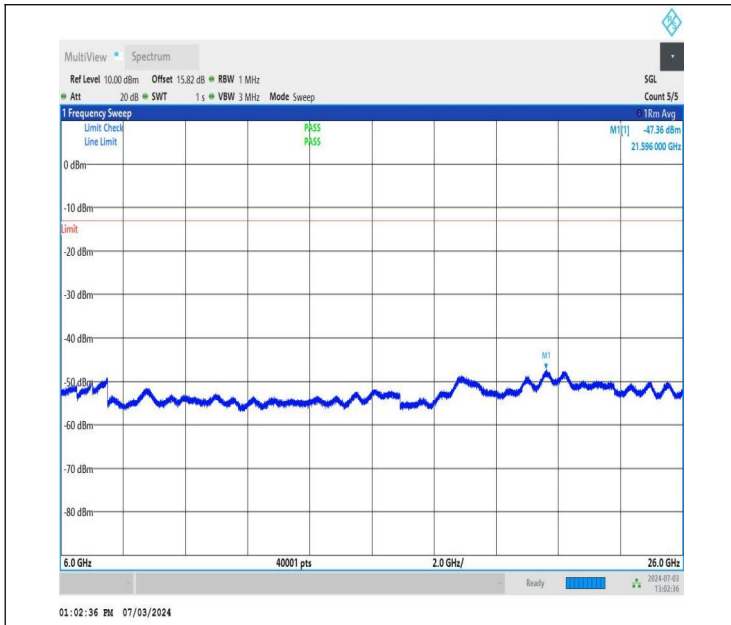
NTNV_DC_26A_n77A-3700-3980_PC2_30_5+80_M+H_TID2_N S_01_6000_26000_#1
