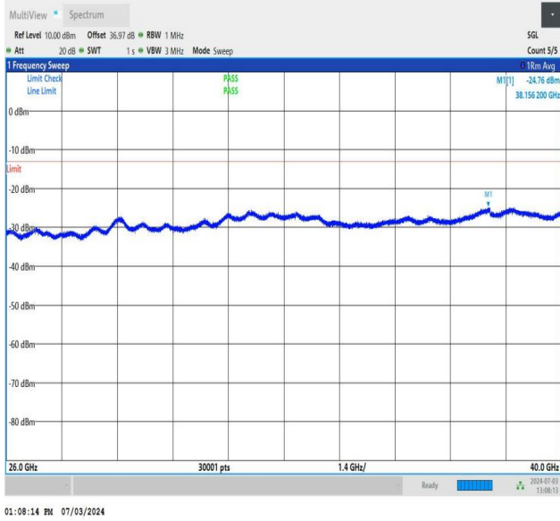
NTNV_DC_26A_n77A-3700-3980_PC2_30_5+90_M+L_TID4_NS_01_26000_40000_#1
