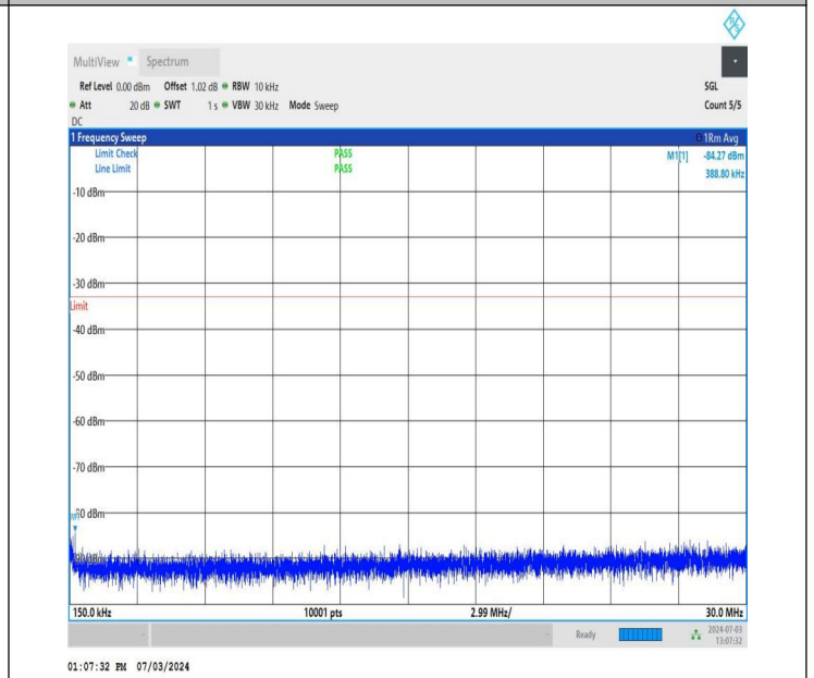
NTNV_DC_26A_n77A-3700-3980_PC2_30_5+90_M+L_TID4_NS_01_0.15_30_#1
