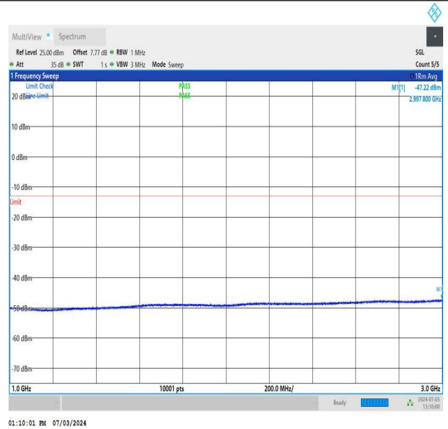
NTNV_DC_26A_n77A-3700-3980_PC2_30_5+90_M+M_TID1_N S_01_1000_3000_#1
