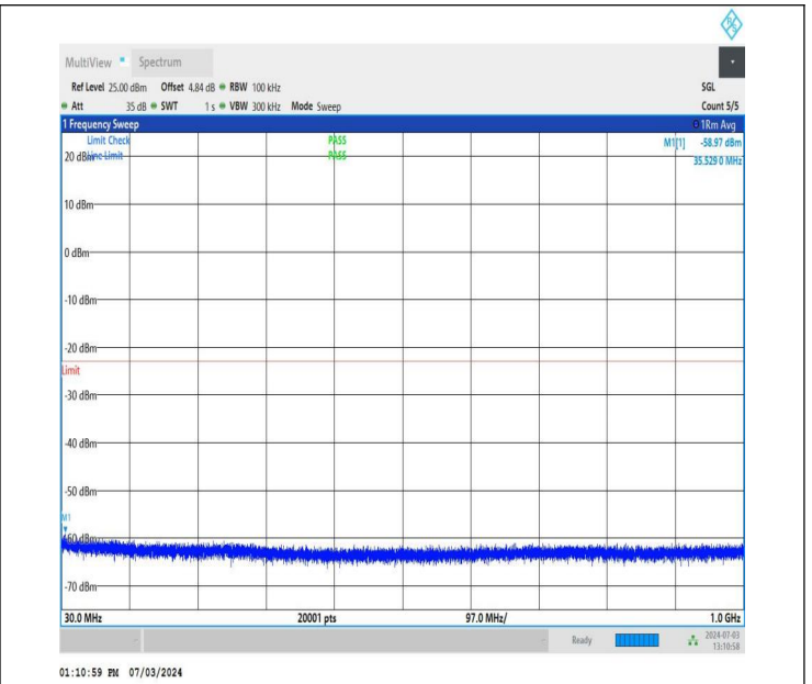
NTNV_DC_26A_n77A-3700-3980_PC2_30_5+90_M+M_TID2_N S_01_30_1000_#1
