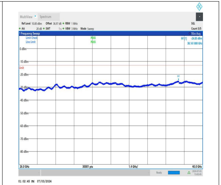
NTNV_DC_26A_n77A-3700-3980_PC2_30_5+80_M+H_TID2_N S_01_26000_40000_#1
