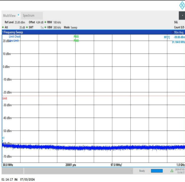
NTNV_DC_26A_n77A-3700-3980_PC2_30_5+90_M+H_TID1_N S_01_30_1000_#1
