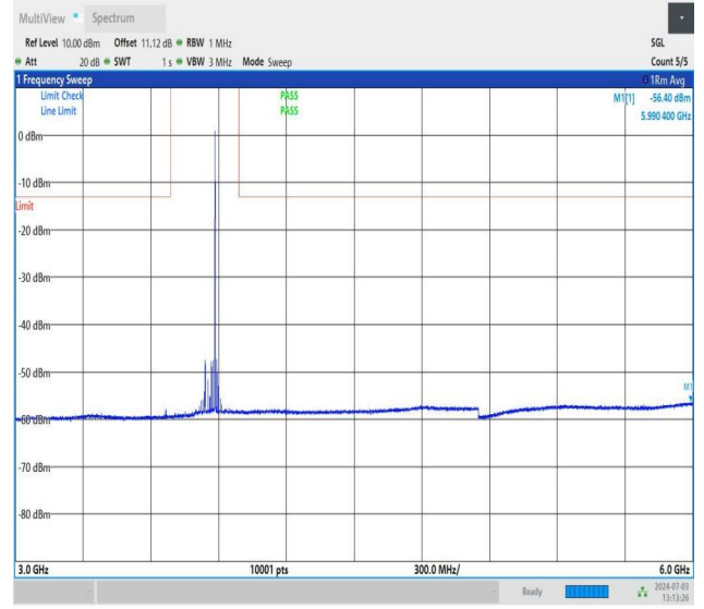
NTNV_DC_26A_n77A-3700-3980_PC2_30_5+90_M+M_TID5_N S_01_3000_6000_#1
