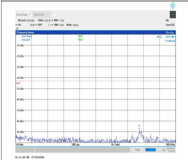
NTNV_DC_26A_n77A-3700-3980_PC2_30_5+90_M+M_TID4_N S_01_0.009_0.15_#1
