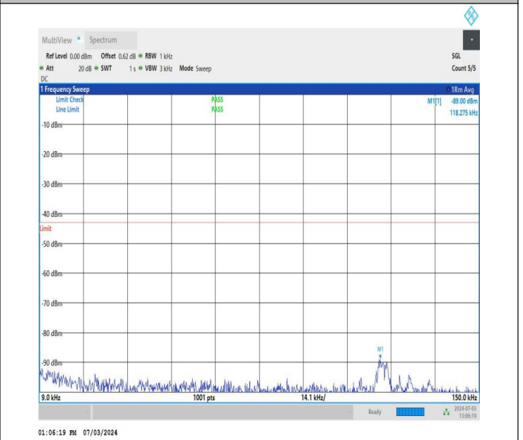
NTNV_DC_26A_n77A-3700-3980_PC2_30_5+90_M+L_TID2_NS_01_0.009_0.15_#1
