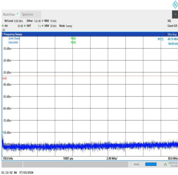
NTNV_DC_26A_n77A-3700-3980_PC2_30_5+90_M+M_TID5_N S_01_0.15_30_#1
