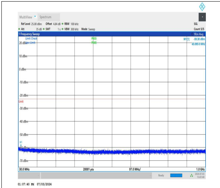
NTNV_DC_26A_n77A-3700-3980_PC2_30_5+90_M+L_TID4_NS_01_30_1000_#1
