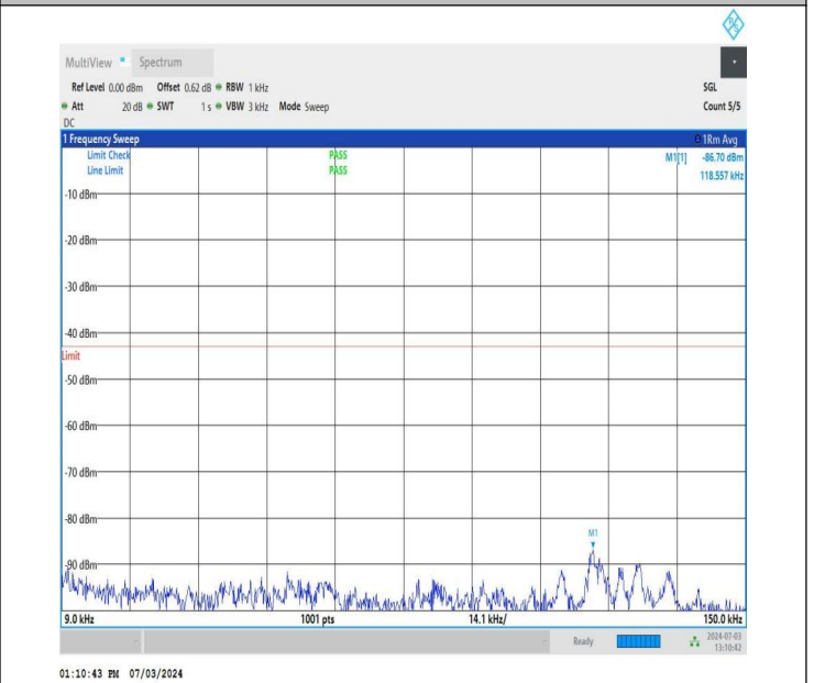
NTNV_DC_26A_n77A-3700-3980_PC2_30_5+90_M+M_TID2_N S_01_0.009_0.15_#1
