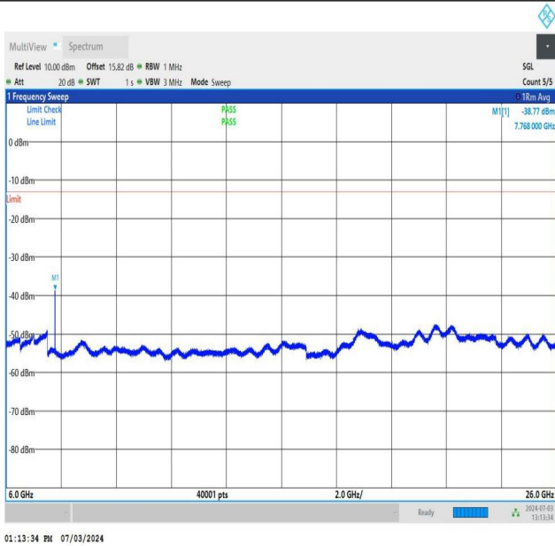
NTNV_DC_26A_n77A-3700-3980_PC2_30_5+90_M+M_TID5_N S_01_6000_26000_#1
