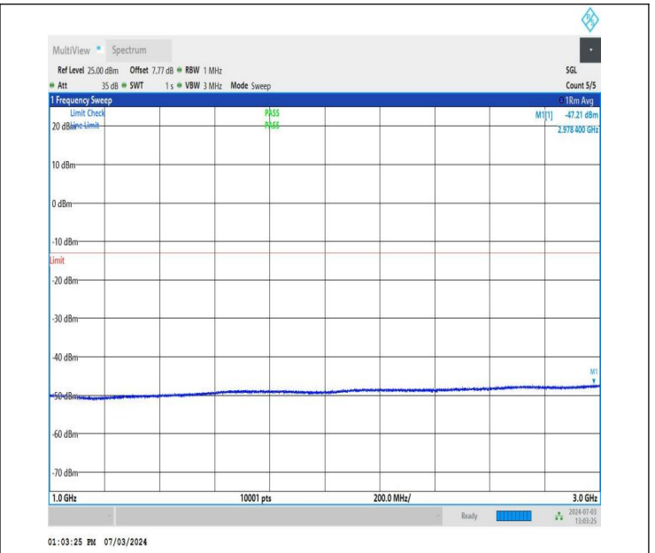
NTNV_DC_26A_n77A-3700-3980_PC2_30_5+80_M+H_TID4_N S_01_1000_3000_#1
