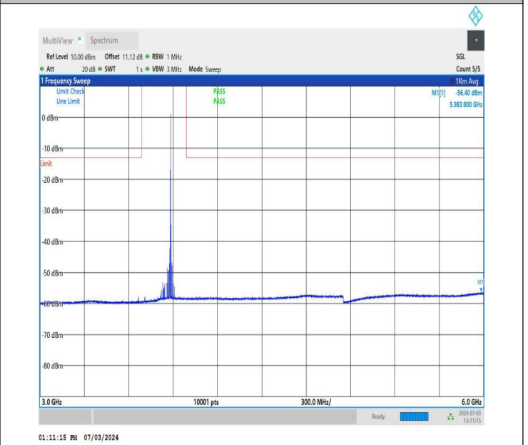
NTNV_DC_26A_n77A-3700-3980_PC2_30_5+90_M+M_TID2_N S_01_3000_6000_#1
