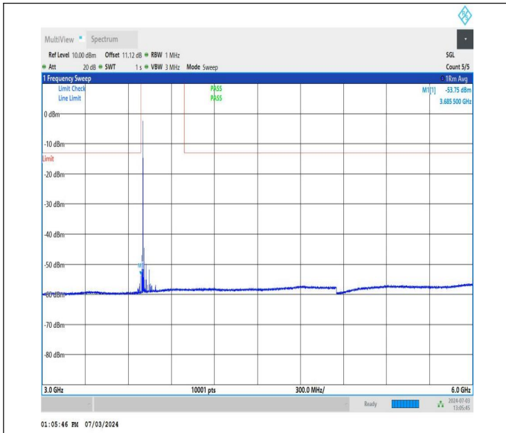
NTNV_DC_26A_n77A-3700-3980_PC2_30_5+90_M+L_TID1_NS_01_3000_6000_#1
