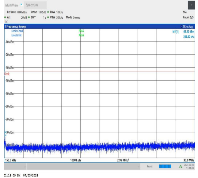
NTNV_DC_26A_n77A-3700-3980_PC2_30_5+90_M+H_TID1_N S_01_0.15_30_#1
