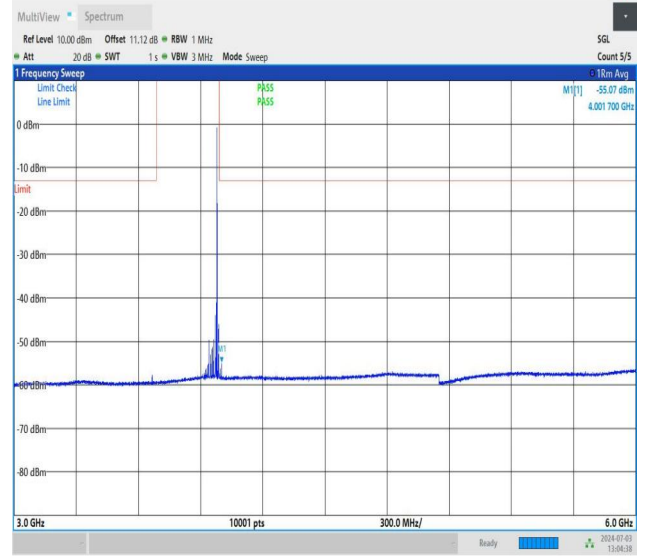
NTNV_DC_26A_n77A-3700-3980_PC2_30_5+80_M+H_TID5_N S_01_3000_6000_#1
