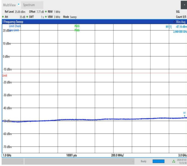
NTNV_DC_26A_n77A-3700-3980_PC2_30_5+90_M+M_TID5_N S_01_1000_3000_#1
