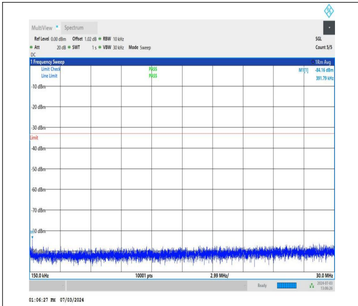
NTNV_DC_26A_n77A-3700-3980_PC2_30_5+90_M+L_TID2_NS_01_0.15_30_#1
