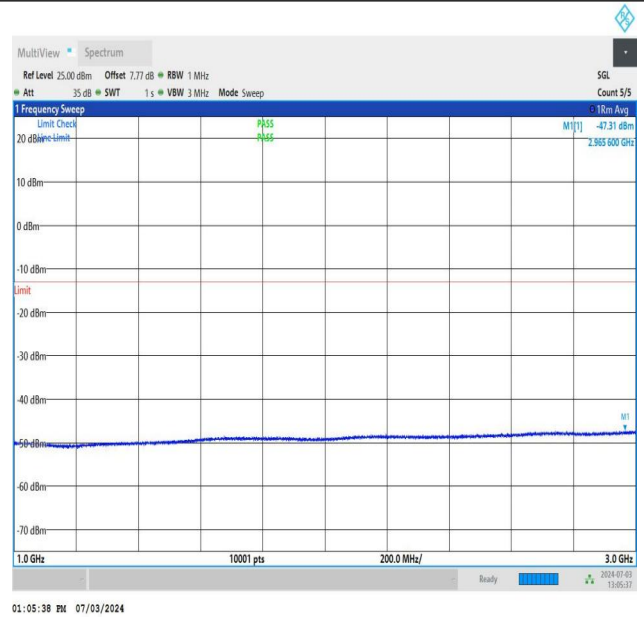
NTNV_DC_26A_n77A-3700-3980_PC2_30_5+90_M+L_TID1_NS_01_1000_3000_#1
