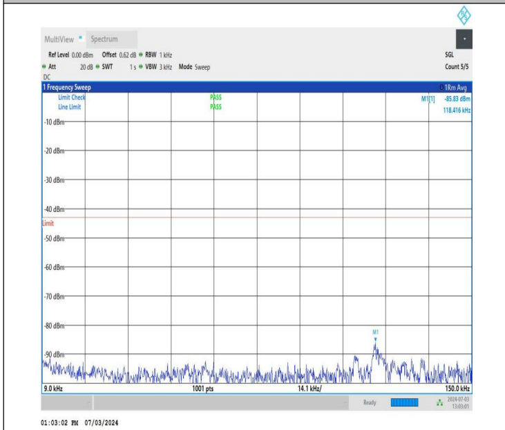
NTNV_DC_26A_n77A-3700-3980_PC2_30_5+80_M+H_TID4_N S_01_0.009_0.15_#1
