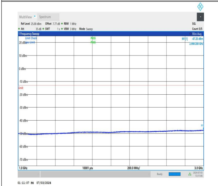
NTNV_DC_26A_n77A-3700-3980_PC2_30_5+90_M+M_TID2_N S_01_1000_3000_#1
