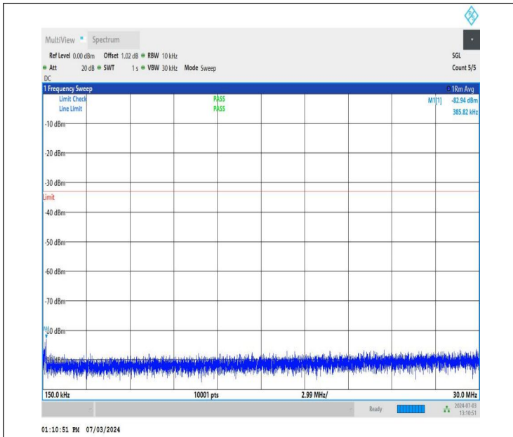
NTNV_DC_26A_n77A-3700-3980_PC2_30_5+90_M+M_TID2_N S_01_0.15_30_#1
