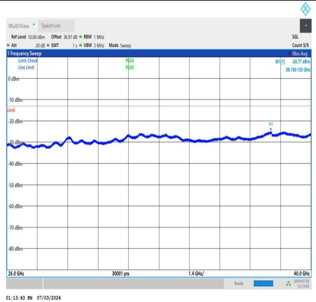
NTNV_DC_26A_n77A-3700-3980_PC2_30_5+90_M+M_TID5_N S_01_26000_40000_#1
