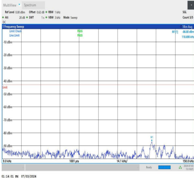
NTNV_DC_26A_n77A-3700-3980_PC2_30_5+90_M+H_TID1_N S_01_0.009_0.15_#1
