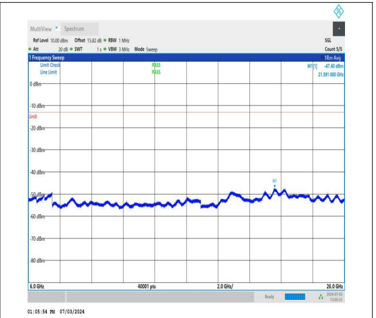
NTNV_DC_26A_n77A-3700-3980_PC2_30_5+90_M+L_TID1_NS_01_6000_26000_#1
