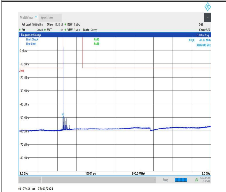
NTNV_DC_26A_n77A-3700-3980_PC2_30_5+90_M+L_TID4_NS_01_3000_6000_#1
