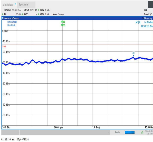
NTNV_DC_26A_n77A-3700-3980_PC2_30_5+90_M+M_TID4_N S_01_26000_40000_#1
