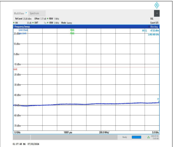
NTNV_DC_26A_n77A-3700-3980_PC2_30_5+90_M+L_TID4_NS_01_1000_3000_#1
