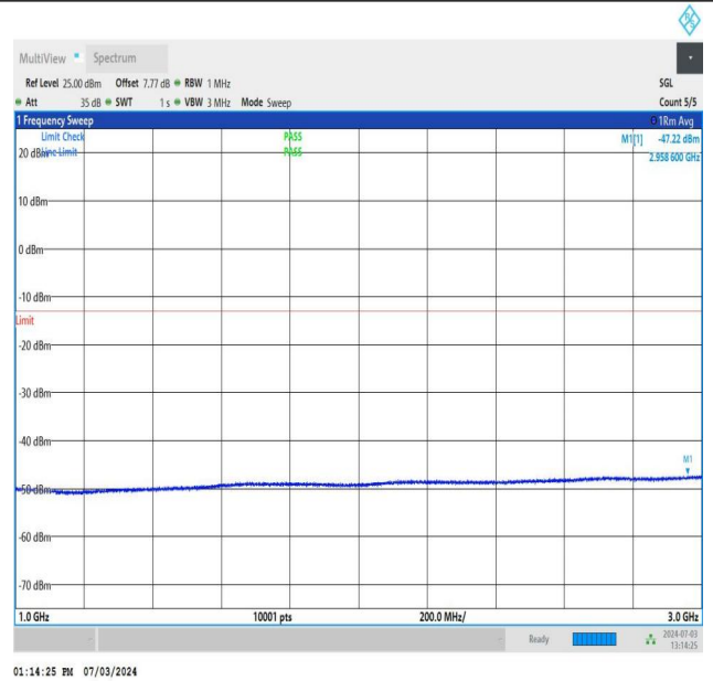
NTNV_DC_26A_n77A-3700-3980_PC2_30_5+90_M+H_TID1_N S_01_1000_3000_#1
