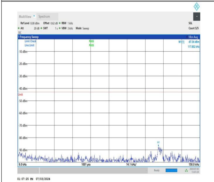
NTNV_DC_26A_n77A-3700-3980_PC2_30_5+90_M+L_TID4_NS_01_0.009_0.15_#1
