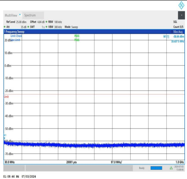
NTNV_DC_26A_n77A-3700-3980_PC2_30_5+90_M+L_TID5_NS_01_30_1000_#1
