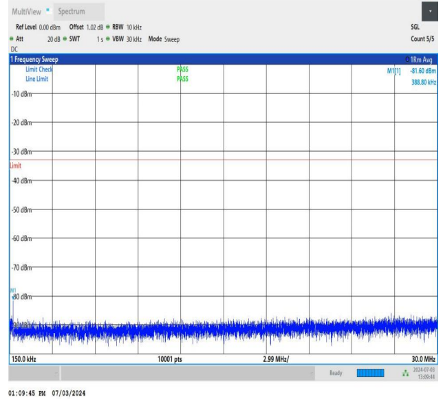
NTNV_DC_26A_n77A-3700-3980_PC2_30_5+90_M+M_TID1_N S_01_0.15_30_#1
