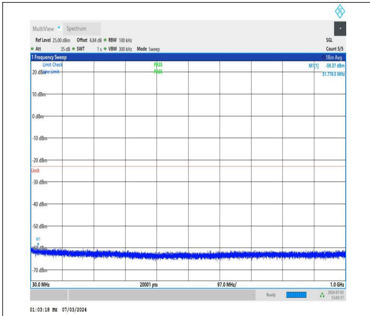
NTNV_DC_26A_n77A-3700-3980_PC2_30_5+80_M+H_TID4_N S_01_30_1000_#1
