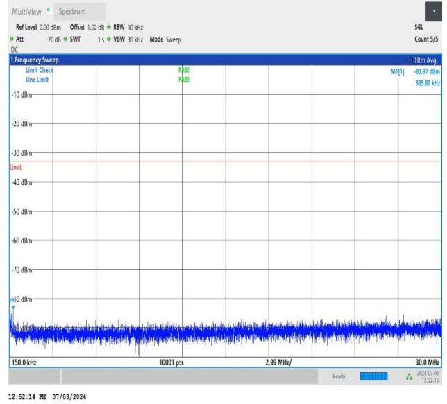
NTNV_DC_26A_n77A-3700-3980_PC2_30_5+80_M+L_TID1_NS_01_0.15_30_#1
