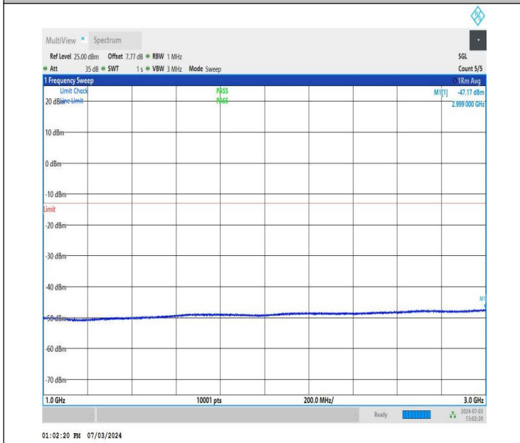
NTNV_DC_26A_n77A-3700-3980_PC2_30_5+80_M+H_TID2_N S_01_1000_3000_#1
