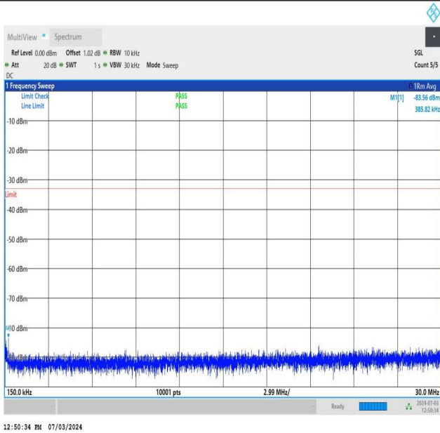
NTNV_DC_26A_n77A-3700-3980_PC2_30_5+60_M+H_TID5_N S_01_0.15_30_#1
