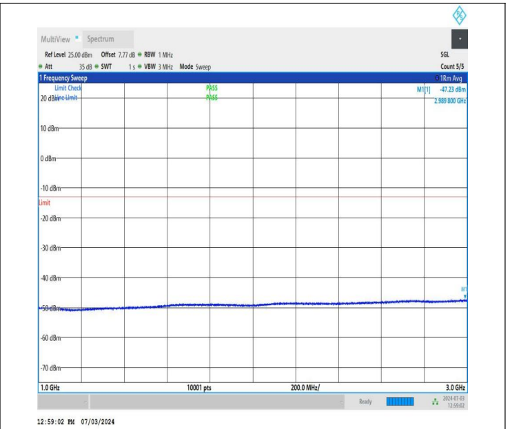
NTNV_DC_26A_n77A-3700-3980_PC2_30_5+80_M+M_TID4_N S_01_1000_3000_#1
