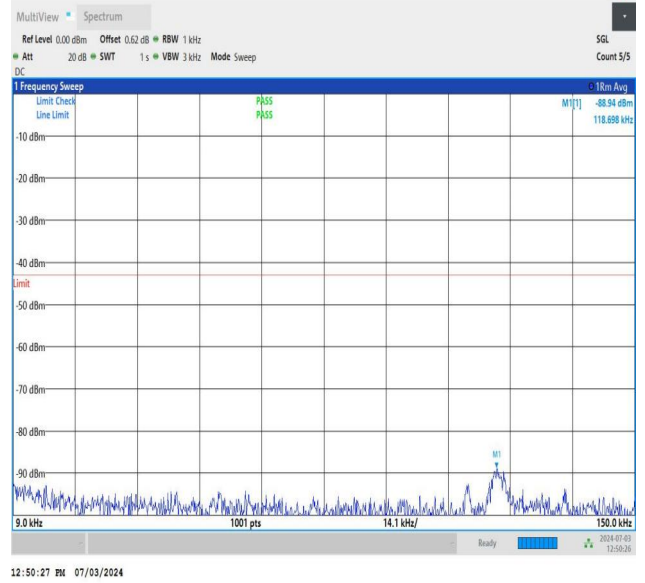
NTNV_DC_26A_n77A-3700-3980_PC2_30_5+60_M+H_TID5_N S_01_0.009_0.15_#1
