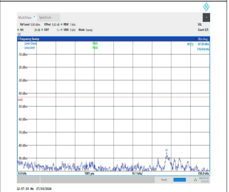
NTNV_DC_26A_n77A-3700-3980_PC2_30_5+80_M+M_TID2_N S_01_0.009_0.15_#1
