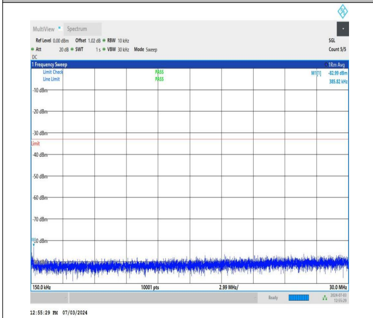
NTNV_DC_26A_n77A-3700-3980_PC2_30_5+80_M+L_TID5_NS_01_0.15_30_#1
