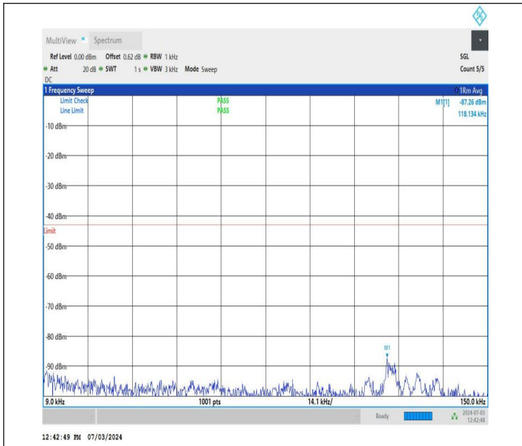
NTNV_DC_26A_n77A-3700-3980_PC2_30_5+60_M+M_TID1_N S_01_0.009_0.15_#1
