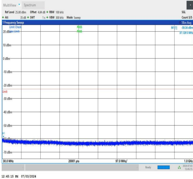
NTNV_DC_26A_n77A-3700-3980_PC2_30_5+60_M+M_TID4_N S_01_30_1000_#1
