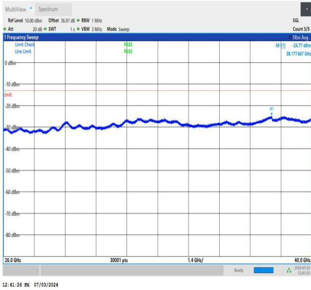
NTNV_DC_26A_n77A-3700-3980_PC2_30_5+60_M+L_TID4_NS_01_26000_40000_#1
