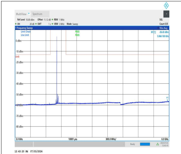
NTNV_DC_26A_n77A-3700-3980_PC2_30_5+60_M+M_TID1_N S_01_3000_6000_#1
