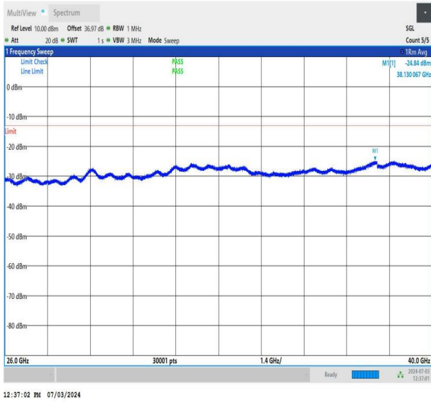
NTNV_DC_26A_n77A-3700-3980_PC2_30_5+50_M+H_TID4_N S_01_26000_40000_#1
