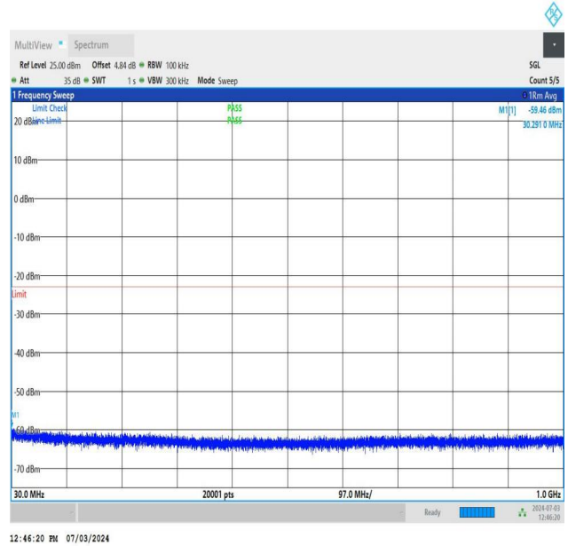
NTNV_DC_26A_n77A-3700-3980_PC2_30_5+60_M+M_TID5_N S_01_30_1000_#1
