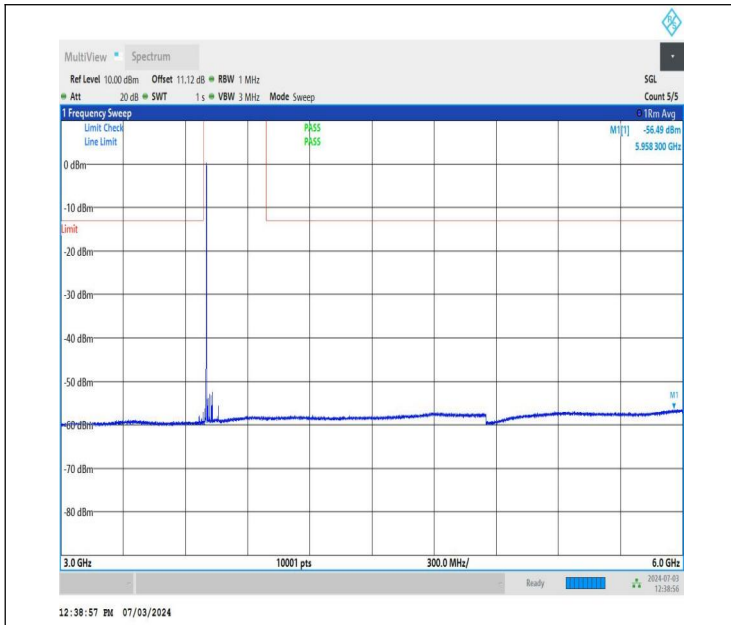
NTNV_DC_26A_n77A-3700-3980_PC2_30_5+60_M+L_TID1_NS_01_3000_6000_#1
