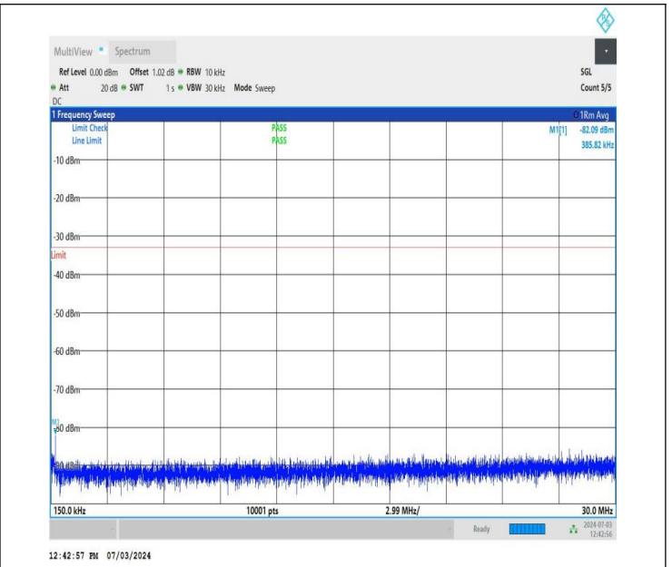
NTNV_DC_26A_n77A-3700-3980_PC2_30_5+60_M+M_TID1_N S_01_0.15_30_#1
