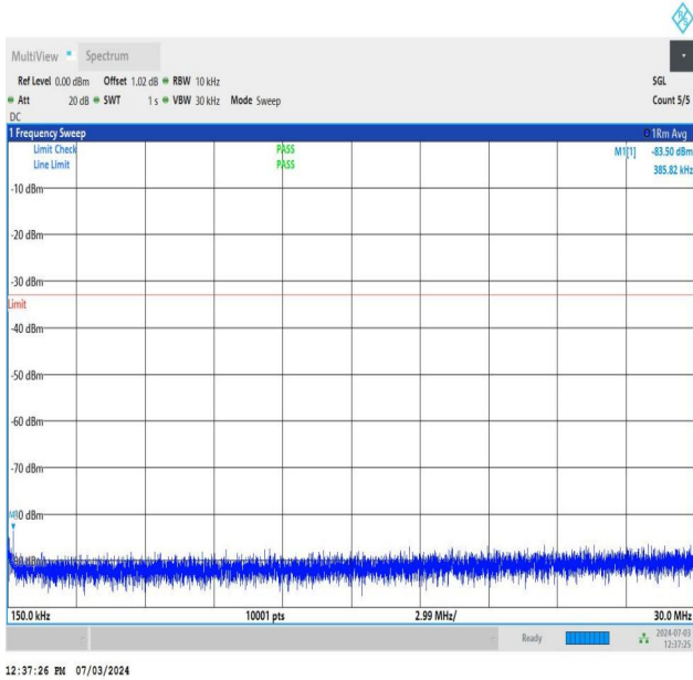
NTNV_DC_26A_n77A-3700-3980_PC2_30_5+50_M+H_TID5_N S_01_0.15_30_#1
