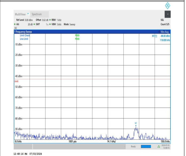
NTNV_DC_26A_n77A-3700-3980_PC2_30_5+60_M+H_TID2_N S_01_0.009_0.15_#1
