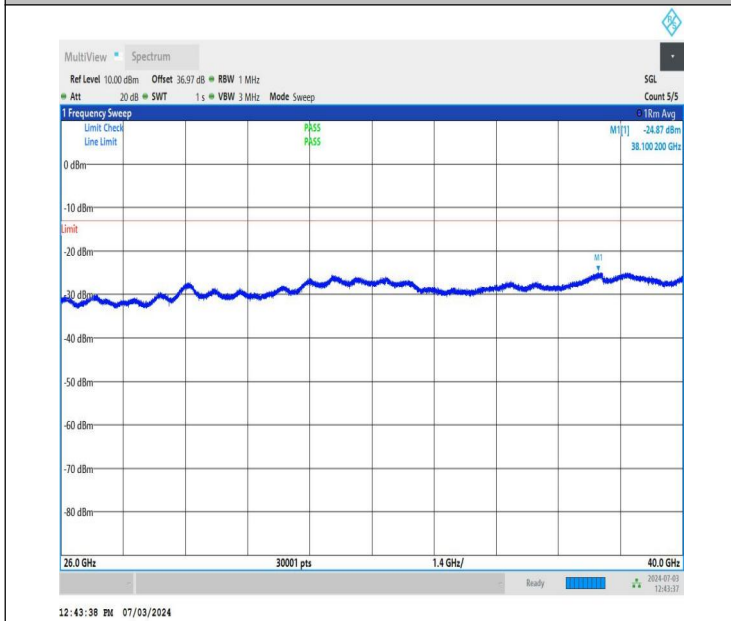
NTNV_DC_26A_n77A-3700-3980_PC2_30_5+60_M+M_TID1_N S_01_26000_40000_#1
