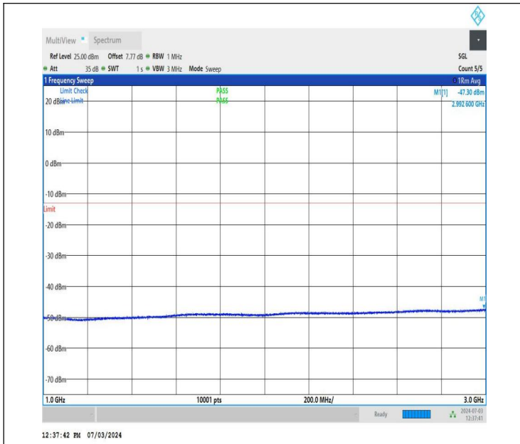
NTNV_DC_26A_n77A-3700-3980_PC2_30_5+50_M+H_TID5_N S_01_1000_3000_#1
