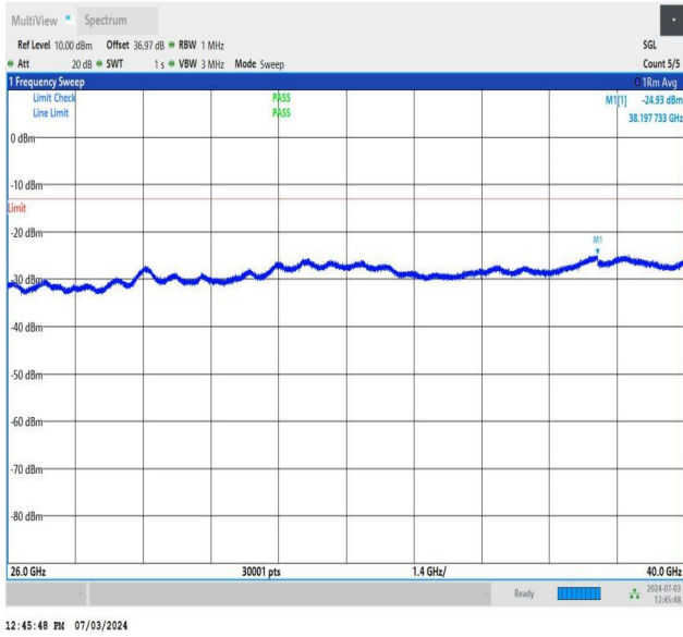
NTNV_DC_26A_n77A-3700-3980_PC2_30_5+60_M+M_TID4_N S_01_26000_40000_#1
