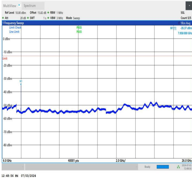
NTNV_DC_26A_n77A-3700-3980_PC2_30_5+60_M+H_TID2_N S_01_6000_26000_#1
