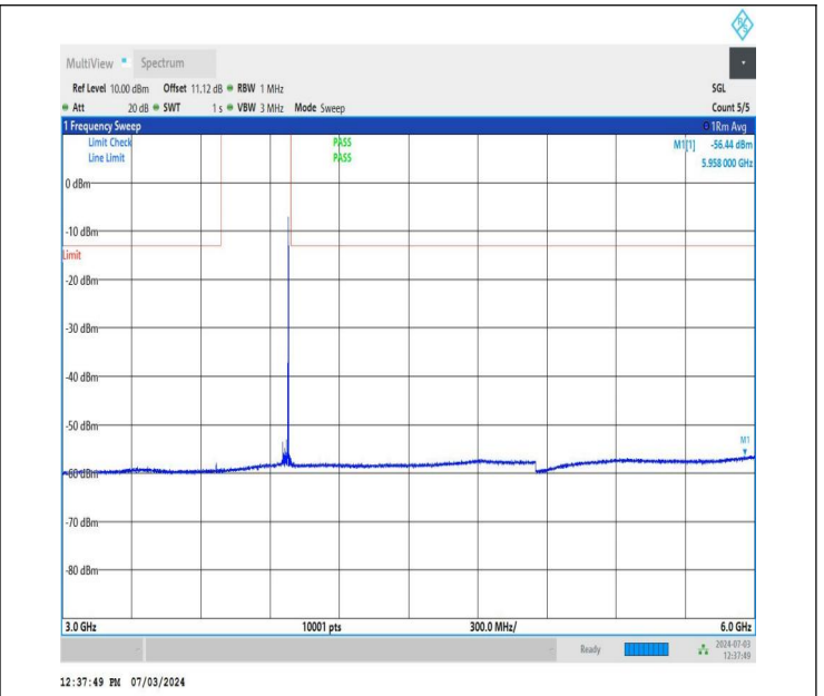
NTNV_DC_26A_n77A-3700-3980_PC2_30_5+50_M+H_TID5_N S_01_3000_6000_#1
