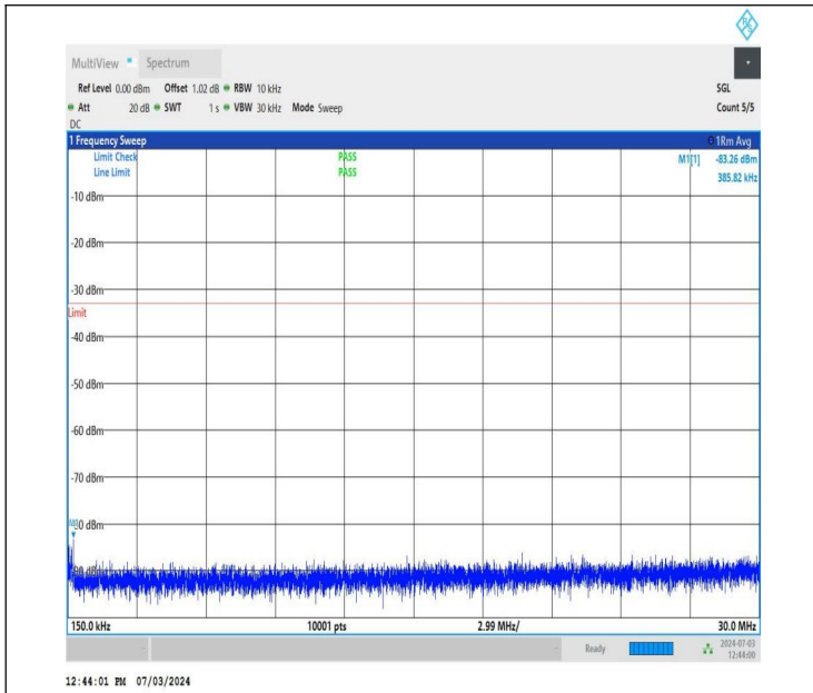
NTNV_DC_26A_n77A-3700-3980_PC2_30_5+60_M+M_TID2_N S_01_0.15_30_#1
