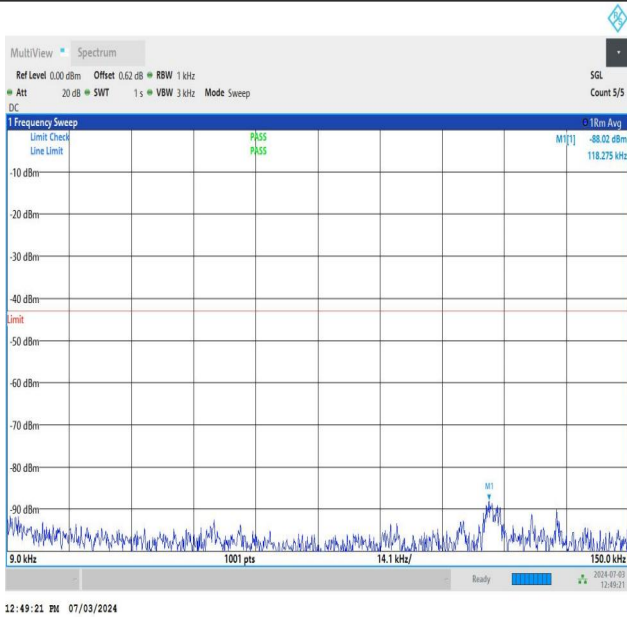
NTNV_DC_26A_n77A-3700-3980_PC2_30_5+60_M+H_TID4_N S_01_0.009_0.15_#1
