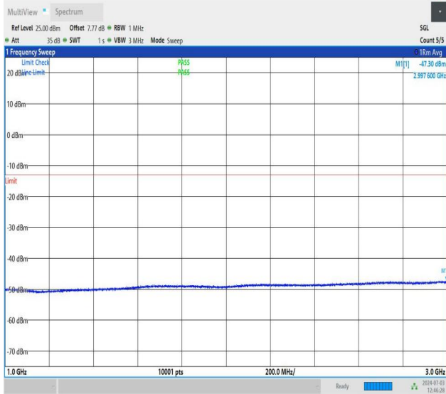
NTNV_DC_26A_n77A-3700-3980_PC2_30_5+60_M+M_TID5_N S_01_1000_3000_#1
