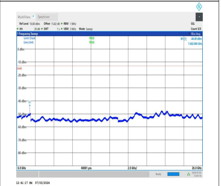
NTNV_DC_26A_n77A-3700-3980_PC2_30_5+60_M+L_TID4_NS_01_6000_26000_#1
