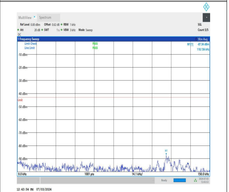
NTNV_DC_26A_n77A-3700-3980_PC2_30_5+60_M+M_TID2_N S_01_0.009_0.15_#1
