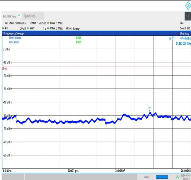
NTNV_DC_26A_n77A-3700-3980_PC2_30_5+60_M+M_TID5_N S_01_1000_3000_#1
