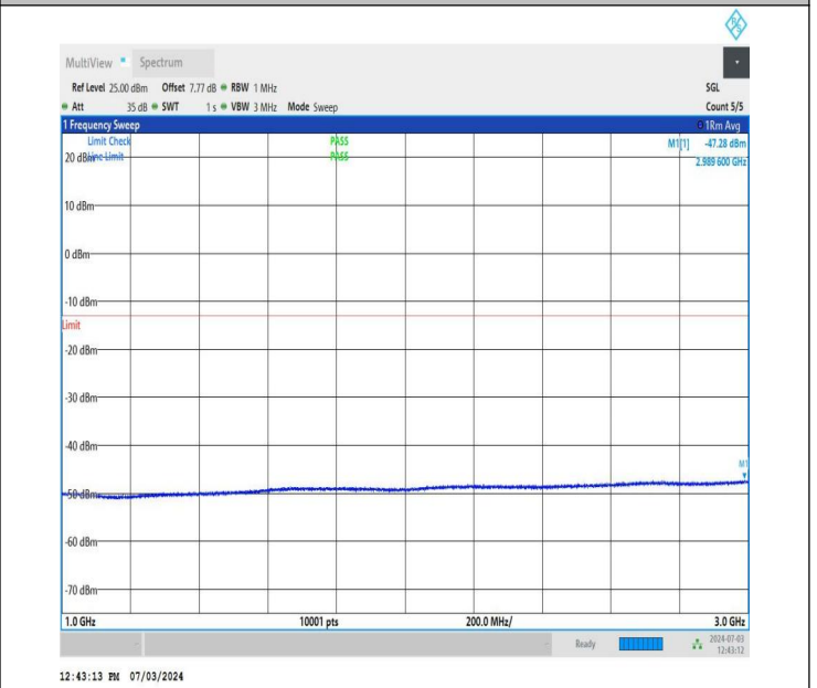
NTNV_DC_26A_n77A-3700-3980_PC2_30_5+60_M+M_TID1_N S_01_1000_3000_#1
