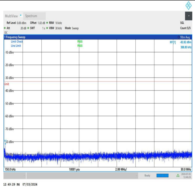
NTNV_DC_26A_n77A-3700-3980_PC2_30_5+60_M+H_TID4_N S_01_0.15_30_#1
