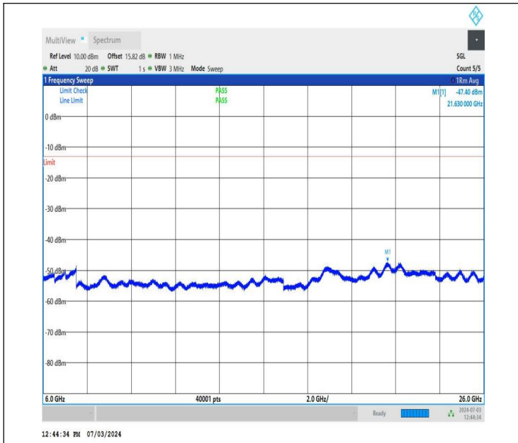
NTNV_DC_26A_n77A-3700-3980_PC2_30_5+60_M+M_TID2_N S_01_6000_26000_#1
