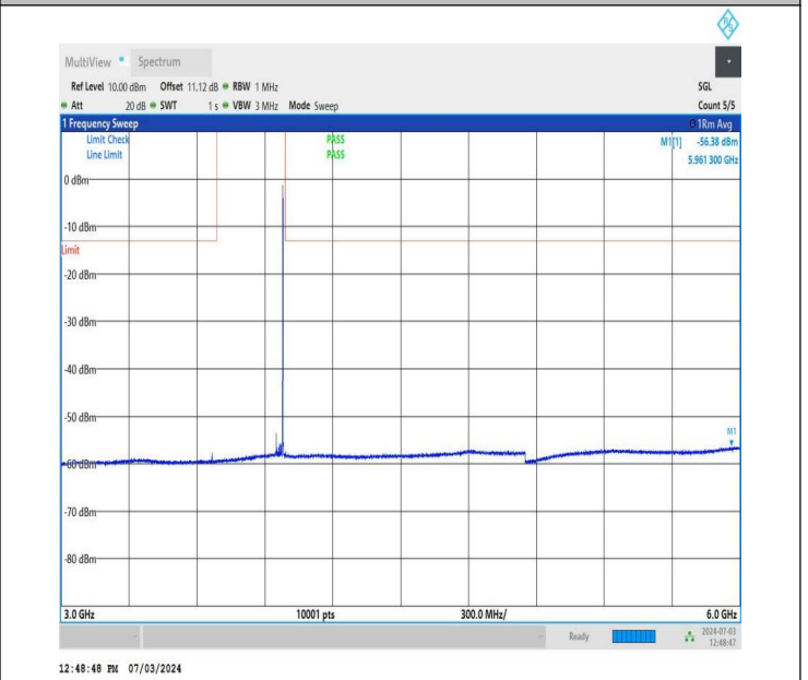
NTNV_DC_26A_n77A-3700-3980_PC2_30_5+60_M+H_TID2_N S_01_3000_6000_#1
