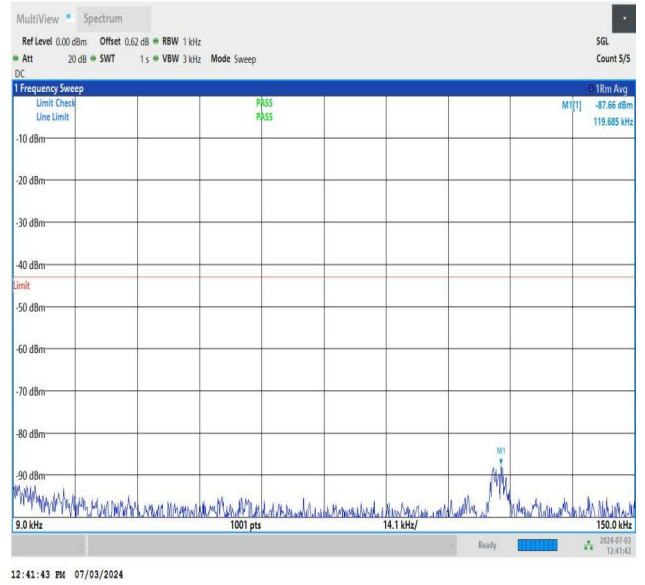
NTNV_DC_26A_n77A-3700-3980_PC2_30_5+60_M+L_TID5_NS_01_0.009_0.15_#1
