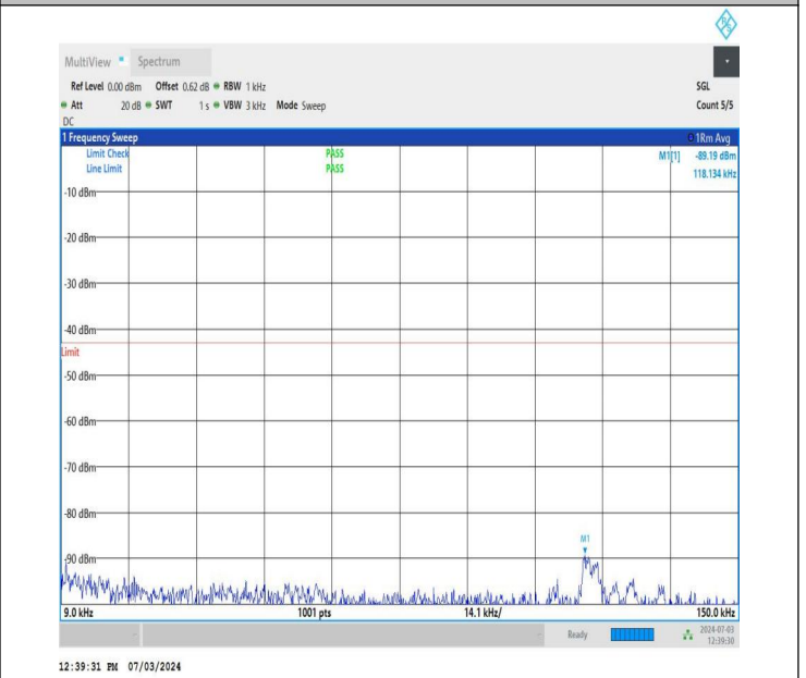
NTNV_DC_26A_n77A-3700-3980_PC2_30_5+60_M+L_TID2_NS_01_0.009_0.15_#1
