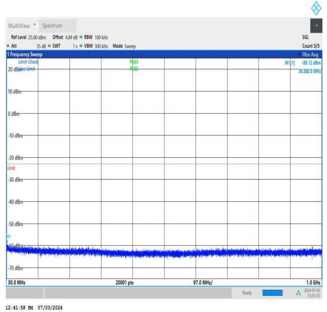
NTNV_DC_26A_n77A-3700-3980_PC2_30_5+60_M+L_TID5_NS_01_30_1000_#1
