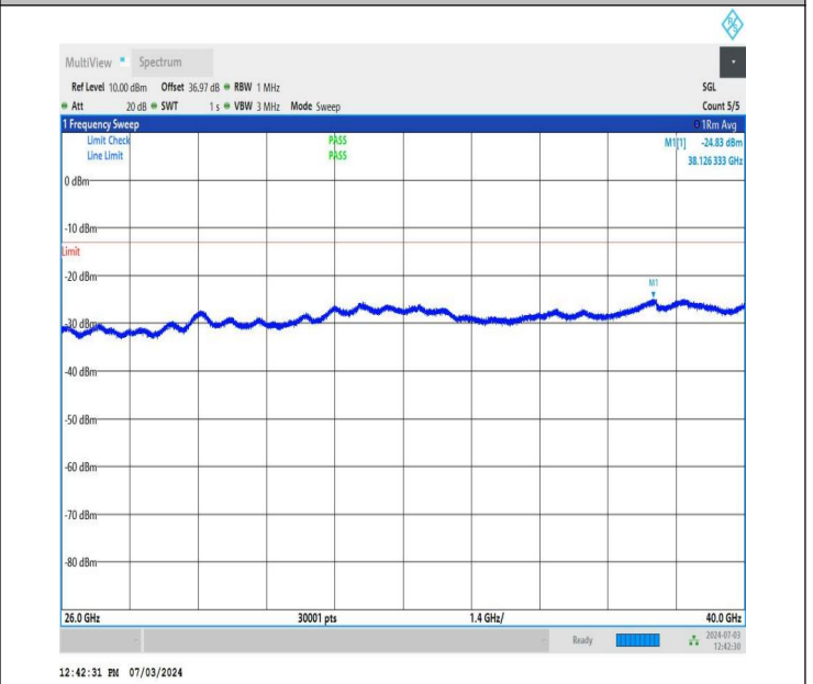
NTNV_DC_26A_n77A-3700-3980_PC2_30_5+60_M+L_TID5_NS_01_26000_40000_#1
