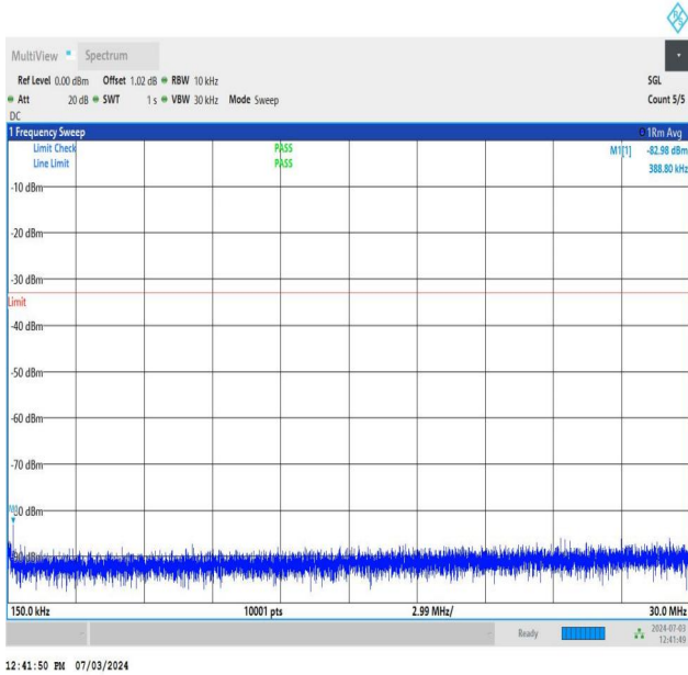
NTNV_DC_26A_n77A-3700-3980_PC2_30_5+60_M+L_TID5_NS_01_0.15_30_#1
