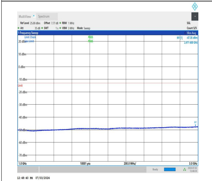
NTNV_DC_26A_n77A-3700-3980_PC2_30_5+60_M+H_TID2_N S_01_1000_3000_#1
