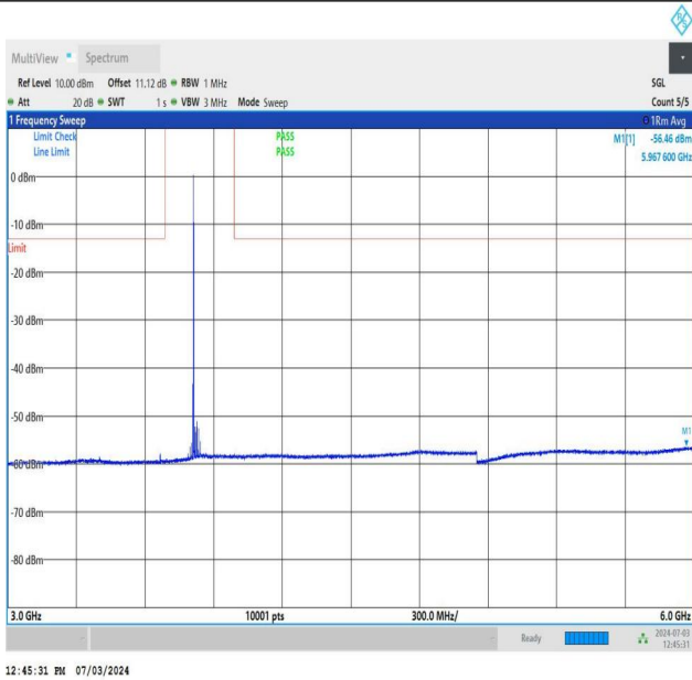
NTNV_DC_26A_n77A-3700-3980_PC2_30_5+60_M+M_TID4_N S_01_3000_6000_#1
