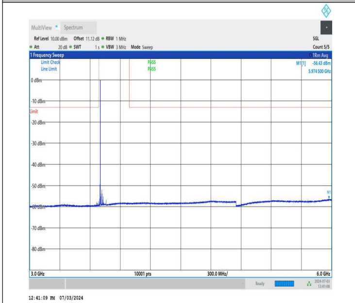
NTNV_DC_26A_n77A-3700-3980_PC2_30_5+60_M+L_TID4_NS_01_3000_6000_#1
