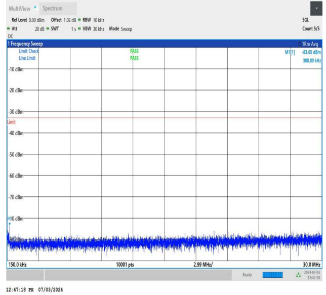
NTNV_DC_26A_n77A-3700-3980_PC2_30_5+60_M+H_TID1_N S_01_0.15_30_#1
