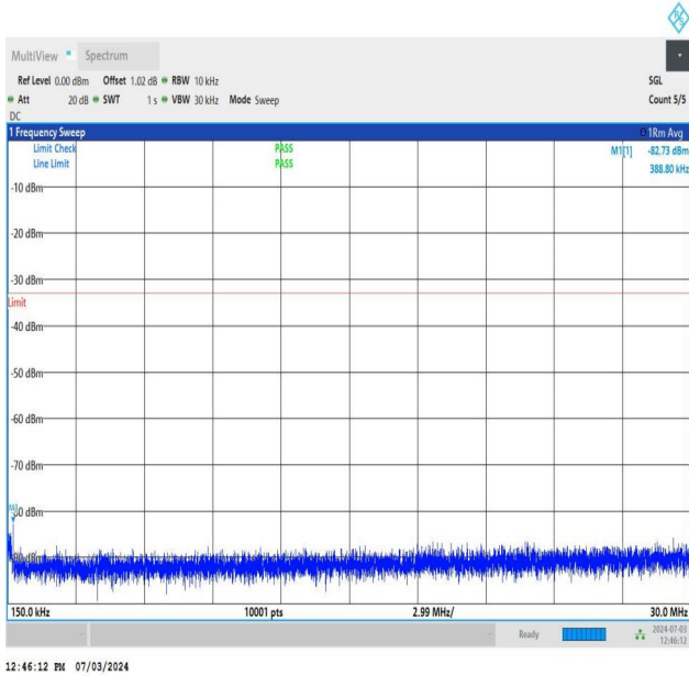
NTNV_DC_26A_n77A-3700-3980_PC2_30_5+60_M+M_TID5_N S_01_0.15_30_#1
