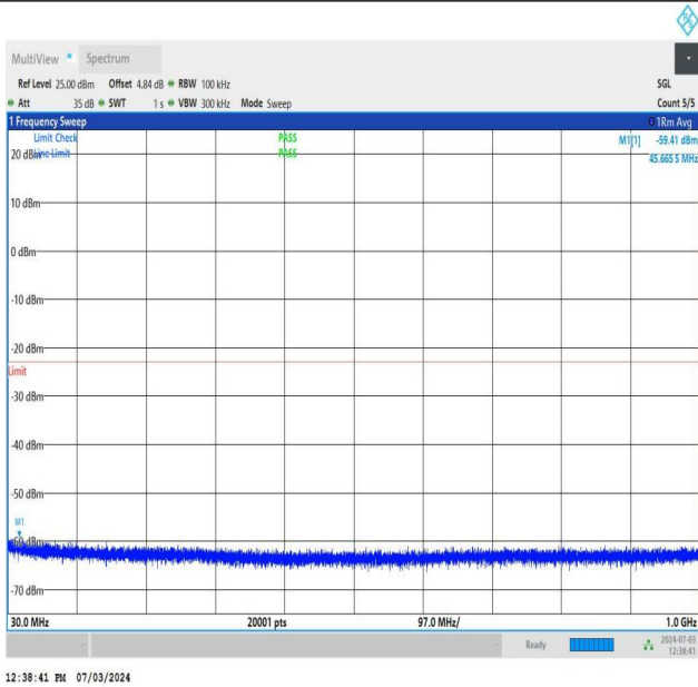
NTNV_DC_26A_n77A-3700-3980_PC2_30_5+60_M+L_TID1_NS_01_30_1000_#1
