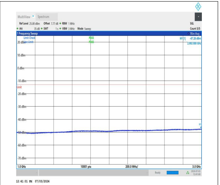
NTNV_DC_26A_n77A-3700-3980_PC2_30_5+60_M+L_TID4_NS_01_1000_3000_#1
