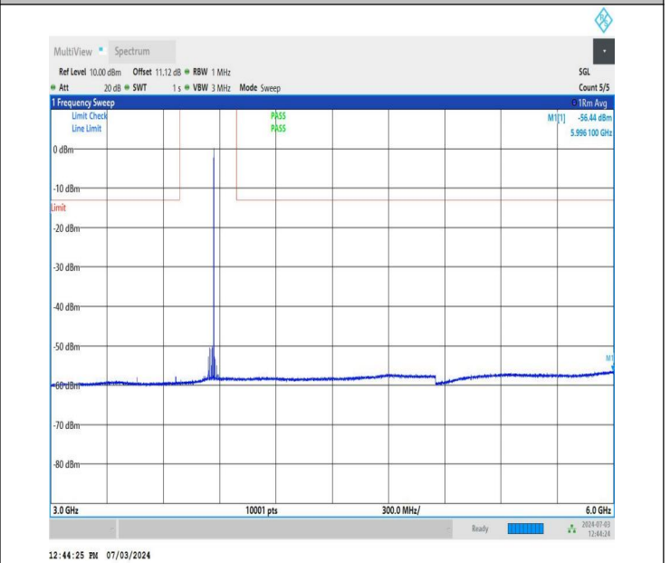
NTNV_DC_26A_n77A-3700-3980_PC2_30_5+60_M+M_TID2_N S_01_3000_6000_#1
