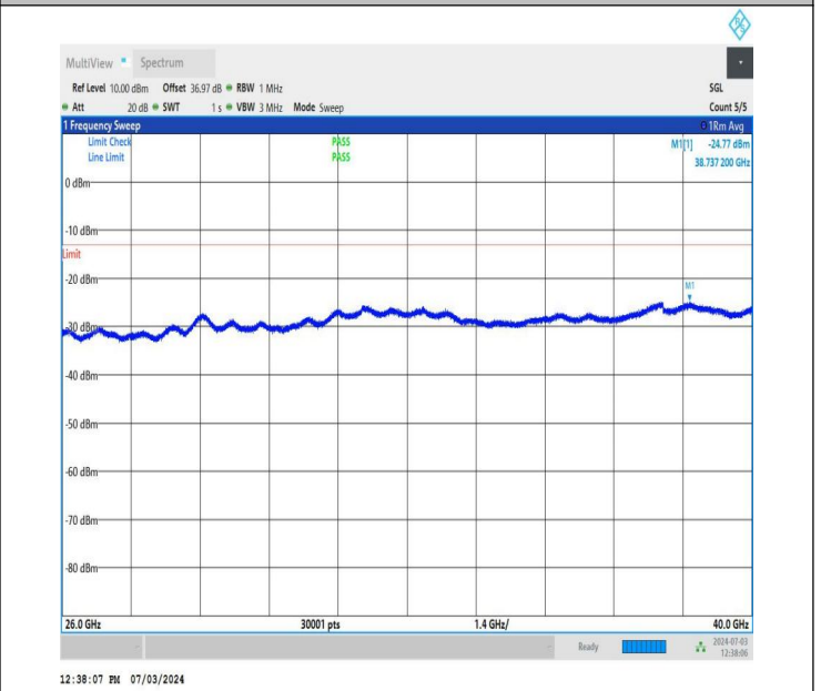
NTNV_DC_26A_n77A-3700-3980_PC2_30_5+50_M+H_TID5_N S_01_26000_40000_#1
