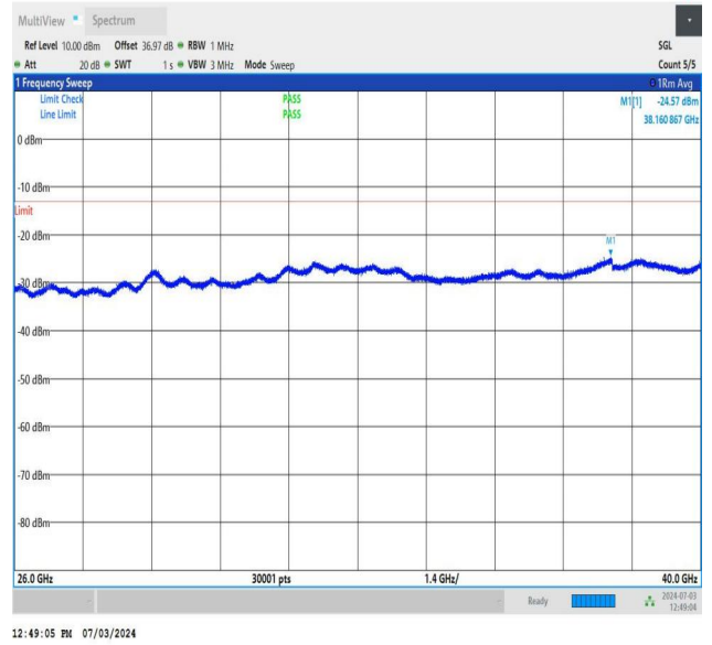
NTNV_DC_26A_n77A-3700-3980_PC2_30_5+60_M+H_TID2_N S_01_26000_40000_#1
