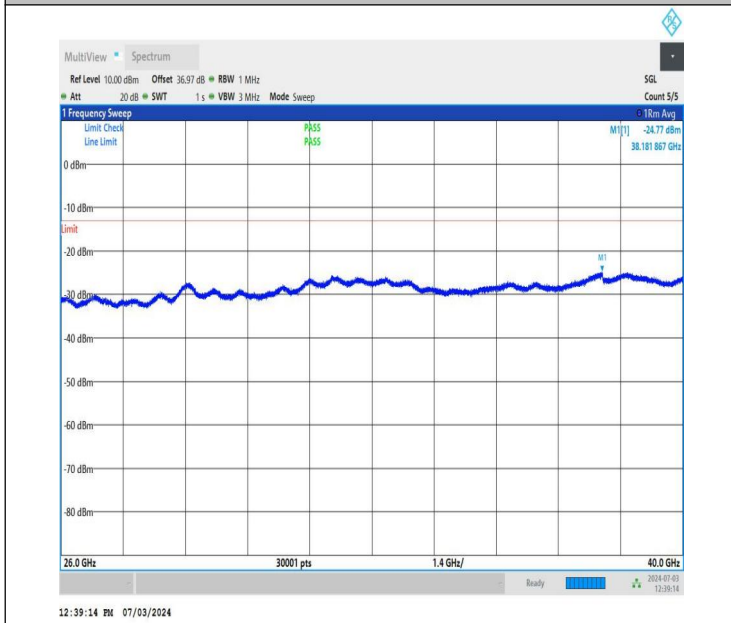
NTNV_DC_26A_n77A-3700-3980_PC2_30_5+60_M+L_TID1_NS_01_26000_40000_#1
