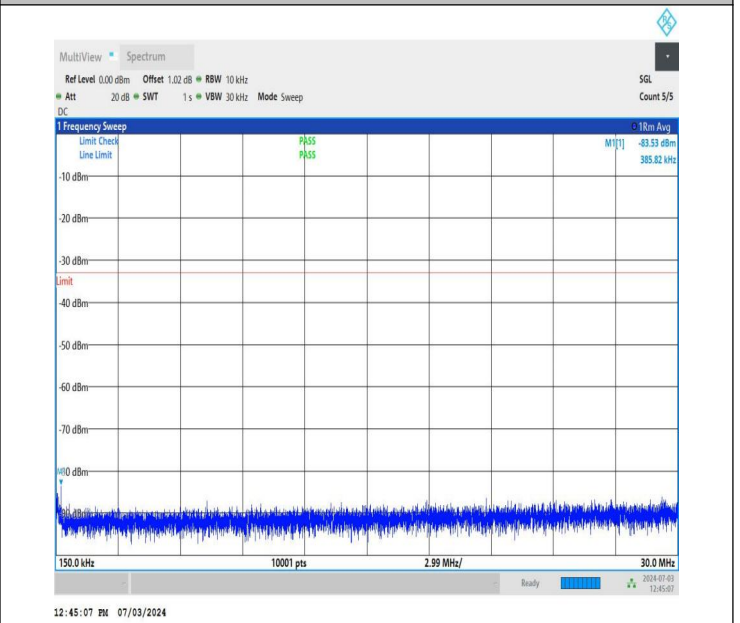
NTNV_DC_26A_n77A-3700-3980_PC2_30_5+60_M+M_TID4_N S_01_0.15_30_#1
