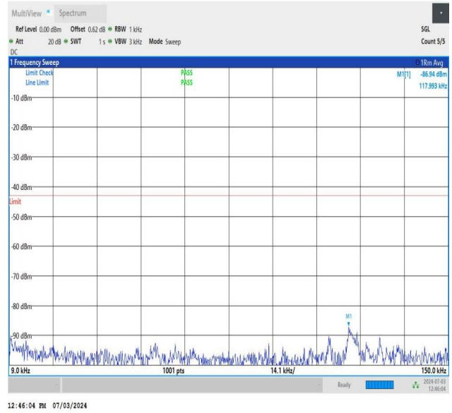
NTNV_DC_26A_n77A-3700-3980_PC2_30_5+60_M+M_TID5_N S_01_0.009_0.15_#1
