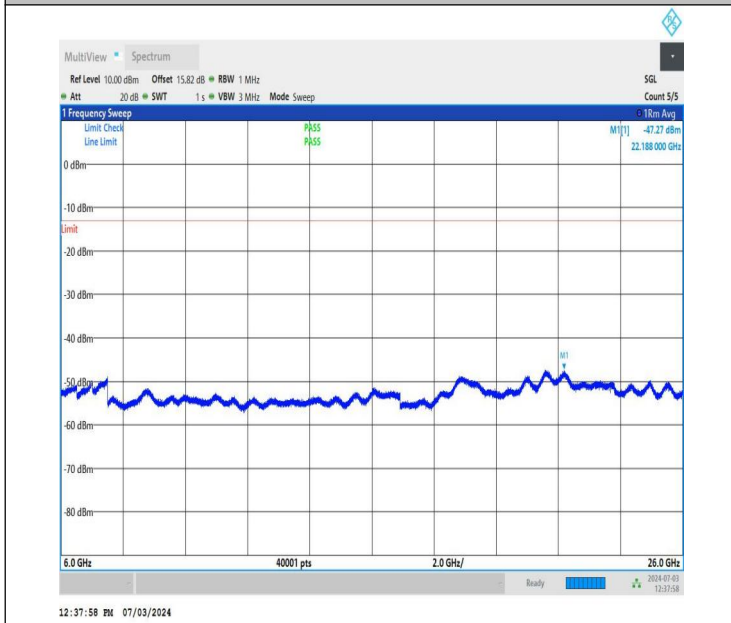
NTNV_DC_26A_n77A-3700-3980_PC2_30_5+50_M+H_TID5_N S_01_6000_26000_#1
