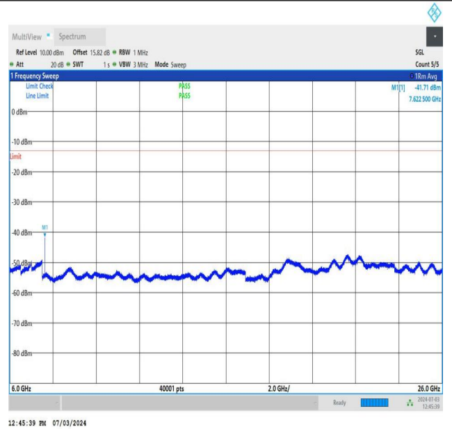
NTNV_DC_26A_n77A-3700-3980_PC2_30_5+60_M+M_TID4_N S_01_6000_26000_#1
