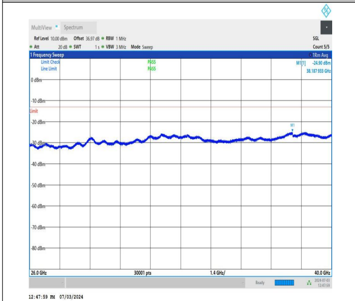
NTNV_DC_26A_n77A-3700-3980_PC2_30_5+60_M+H_TID1_N S_01_26000_40000_#1
