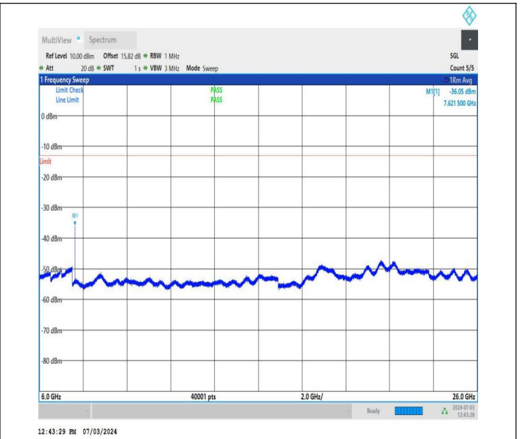
NTNV_DC_26A_n77A-3700-3980_PC2_30_5+60_M+M_TID1_N S_01_6000_26000_#1
