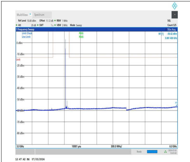
NTNV_DC_26A_n77A-3700-3980_PC2_30_5+60_M+H_TID1_N S_01_3000_6000_#1
