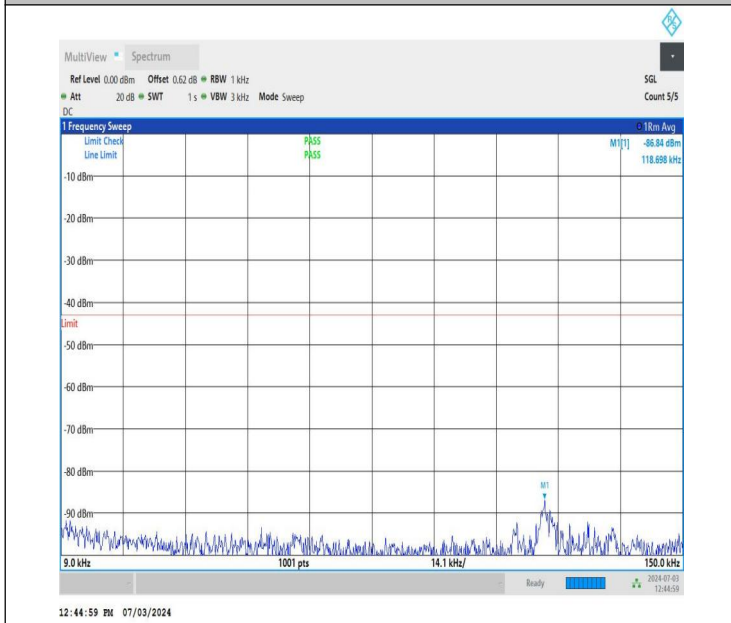
NTNV_DC_26A_n77A-3700-3980_PC2_30_5+60_M+M_TID4_N S_01_0.009_0.15_#1
