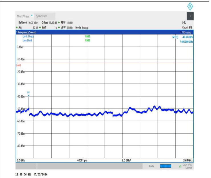
NTNV_DC_26A_n77A-3700-3980_PC2_30_5+60_M+L_TID1_NS_01_6000_26000_#1
