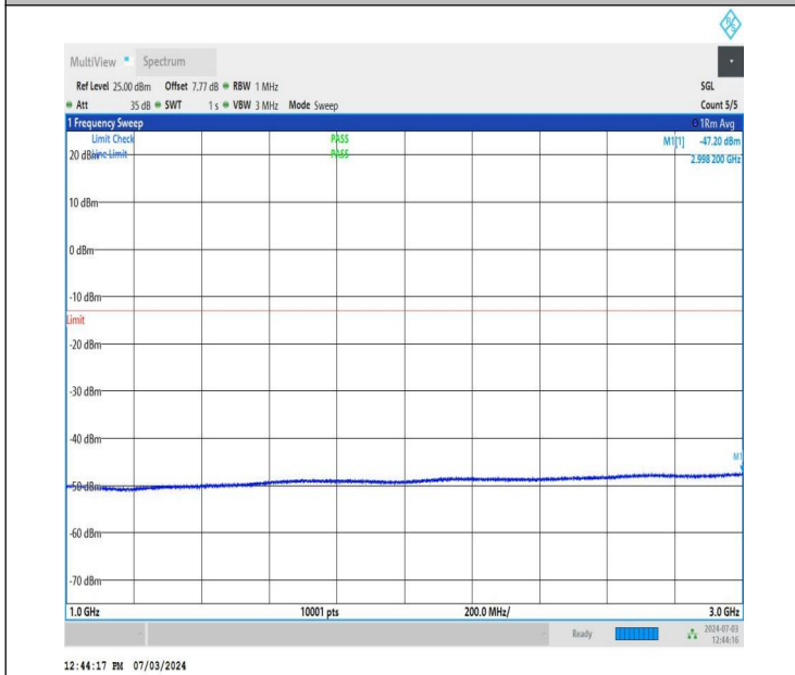
NTNV_DC_26A_n77A-3700-3980_PC2_30_5+60_M+M_TID2_N S_01_1000_3000_#1
