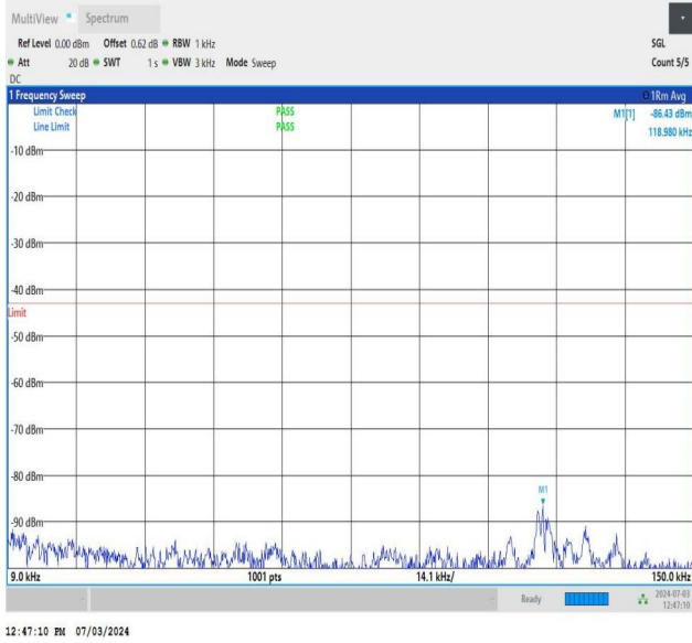
NTNV_DC_26A_n77A-3700-3980_PC2_30_5+60_M+H_TID1_N S_01_0.009_0.15_#1
