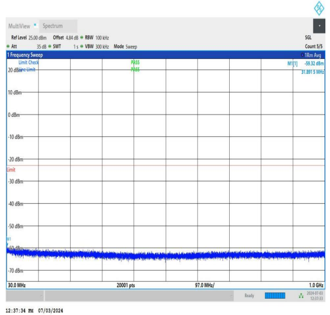
NTNV_DC_26A_n77A-3700-3980_PC2_30_5+50_M+H_TID5_N S_01_30_1000_#1
