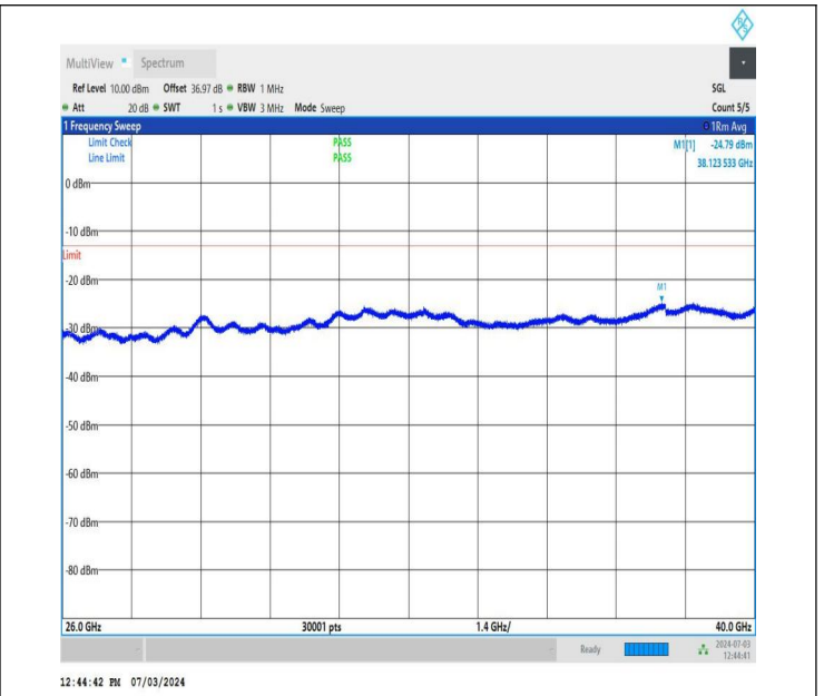
NTNV_DC_26A_n77A-3700-3980_PC2_30_5+60_M+M_TID2_N S_01_26000_40000_#1
