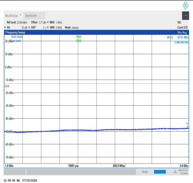
NTNV_DC_26A_n77A-3700-3980_PC2_30_5+60_M+L_TID1_NS_01_1000_3000_#1
