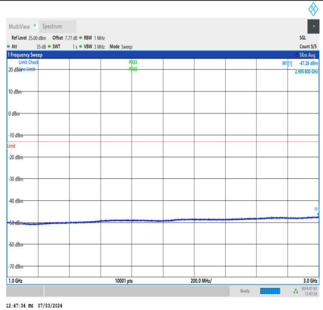
NTNV_DC_26A_n77A-3700-3980_PC2_30_5+60_M+H_TID1_N S_01_1000_3000_#1
