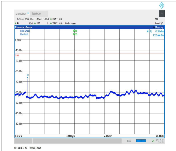
NTNV_DC_26A_n77A-3700-3980_PC2_30_5+50_M+M_TID2_N S_01_6000_26000_#1
