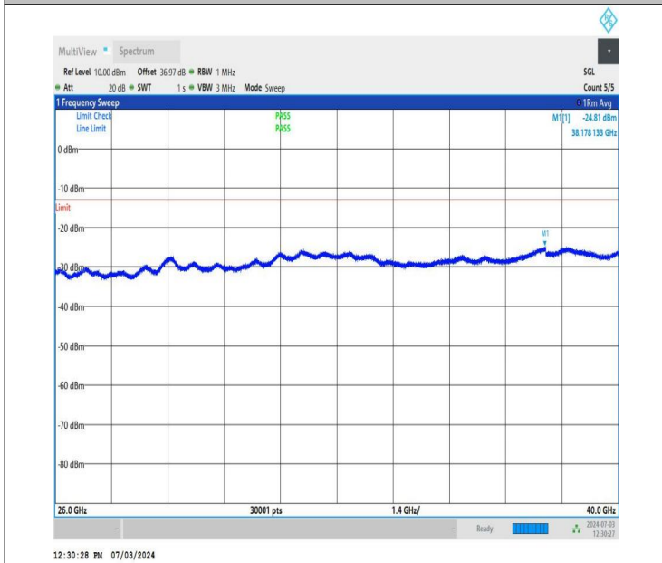
NTNV_DC_26A_n77A-3700-3980_PC2_30_5+50_M+M_TID1_N S_01_26000_40000_#1
