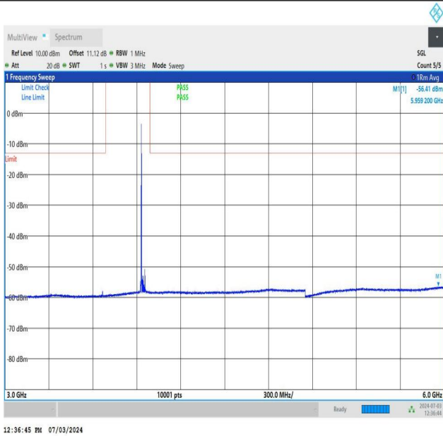
NTNV_DC_26A_n77A-3700-3980_PC2_30_5+50_M+H_TID4_N S_01_3000_6000_#1
