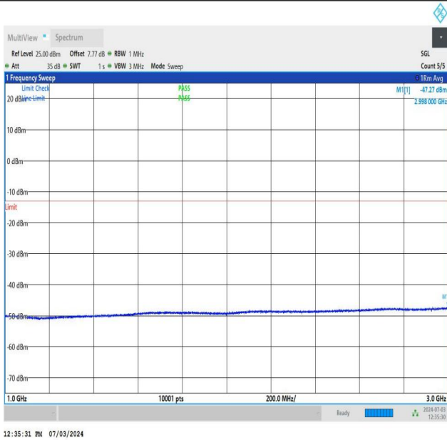
NTNV_DC_26A_n77A-3700-3980_PC2_30_5+50_M+H_TID2_N S_01_1000_3000_#1
