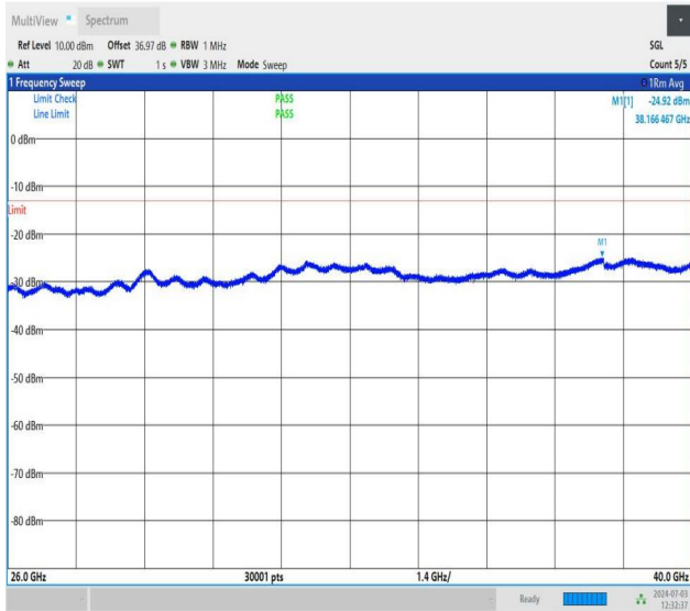
NTNV_DC_26A_n77A-3700-3980_PC2_30_5+50_M+M_TID4_N S_01_26000_40000_#1
