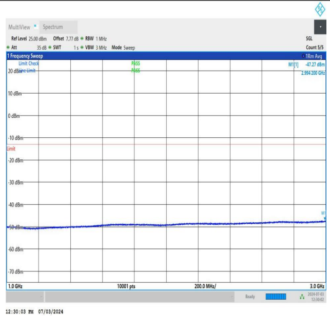
NTNV_DC_26A_n77A-3700-3980_PC2_30_5+50_M+M_TID1_N S_01_1000_3000_#1
