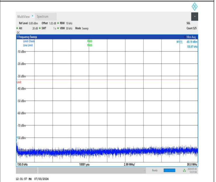
NTNV_DC_26A_n77A-3700-3980_PC2_30_5+50_M+M_TID4_N S_01_0.15_30_#1
