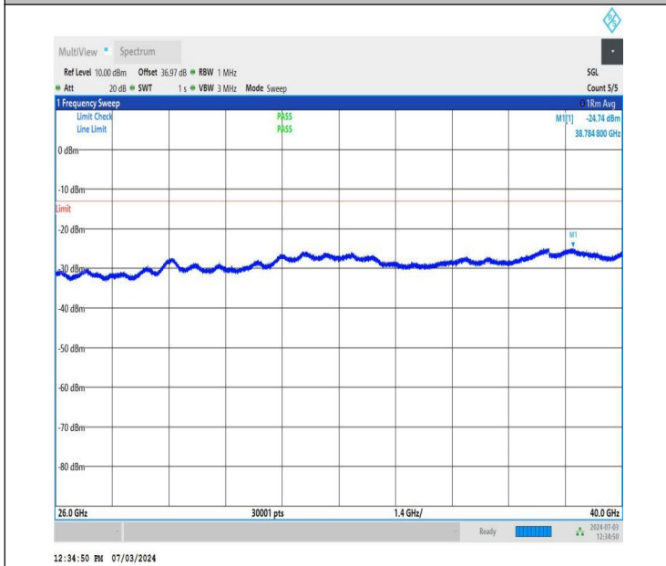
NTNV_DC_26A_n77A-3700-3980_PC2_30_5+50_M+H_TID1_N S_01_26000_40000_#1
