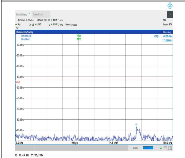
NTNV_DC_26A_n77A-3700-3980_PC2_30_5+50_M+M_TID4_N S_01_0.009_0.15_#1
