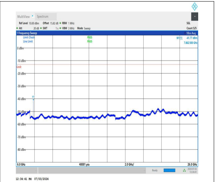
NTNV_DC_26A_n77A-3700-3980_PC2_30_5+50_M+H_TID1_N S_01_6000_26000_#1
