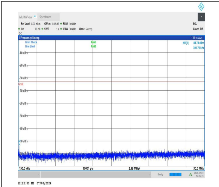
NTNV_DC_26A_n77A-3700-3980_PC2_30_5+50_M+L_TID2_NS_01_0.15_30_#1
