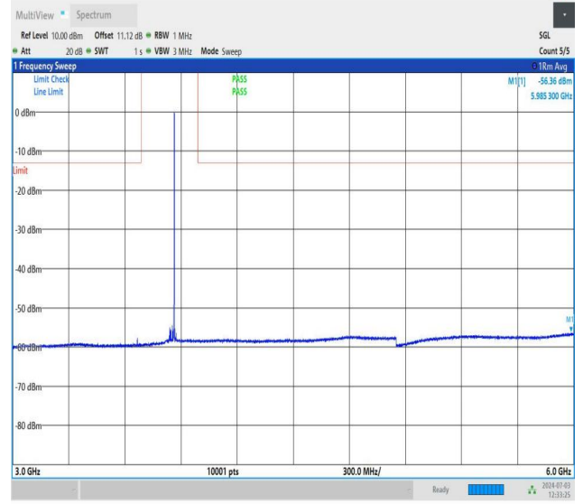
NTNV_DC_26A_n77A-3700-3980_PC2_30_5+50_M+M_TID5_N S_01_3000_6000_#1
