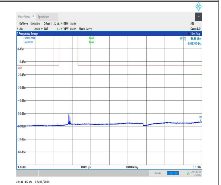
NTNV_DC_26A_n77A-3700-3980_PC2_30_5+50_M+M_TID2_N S_01_3000_6000_#1
