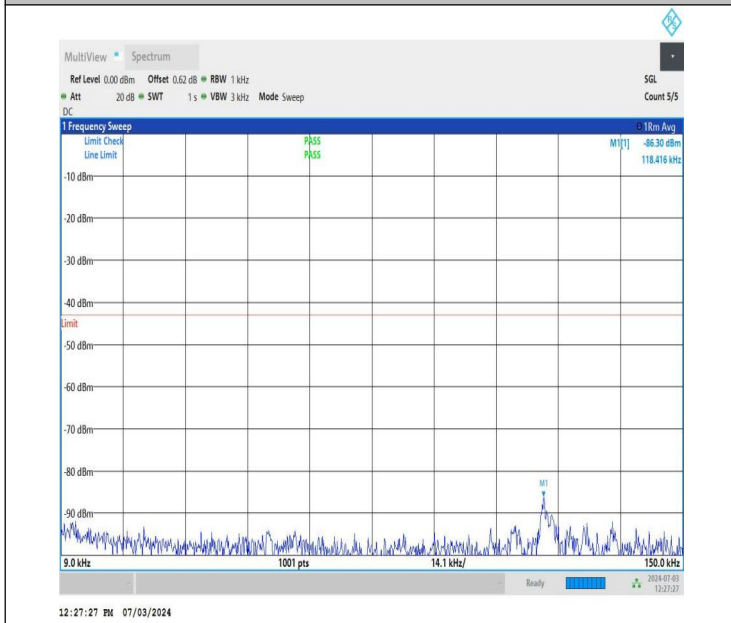
NTNV_DC_26A_n77A-3700-3980_PC2_30_5+50_M+L_TID4_NS_01_0.009_0.15_#1
