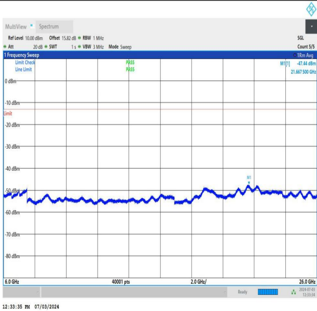
NTNV_DC_26A_n77A-3700-3980_PC2_30_5+50_M+M_TID5_N S_01_6000_26000_#1
