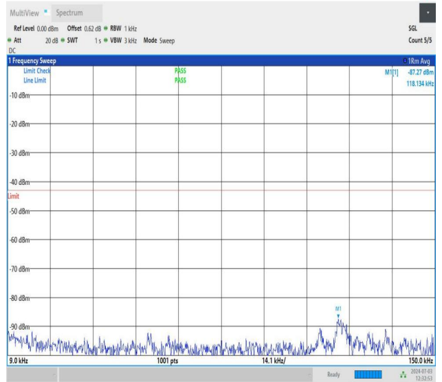
NTNV_DC_26A_n77A-3700-3980_PC2_30_5+50_M+M_TID5_N S_01_0.009_0.15_#1
