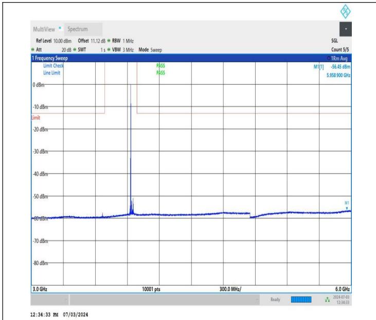
NTNV_DC_26A_n77A-3700-3980_PC2_30_5+50_M+H_TID1_N S_01_3000_6000_#1
