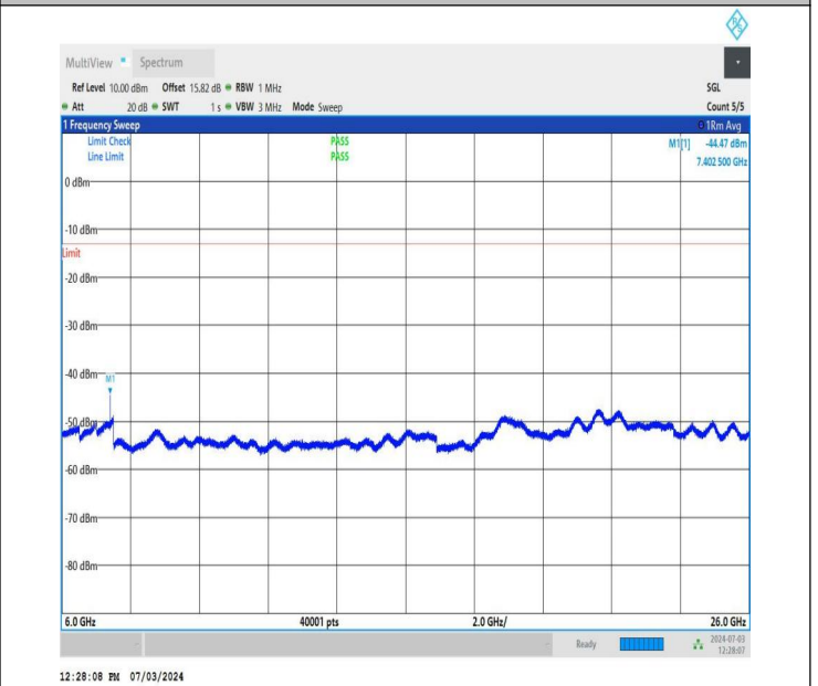
NTNV_DC_26A_n77A-3700-3980_PC2_30_5+50_M+L_TID4_NS_01_6000_26000_#1
