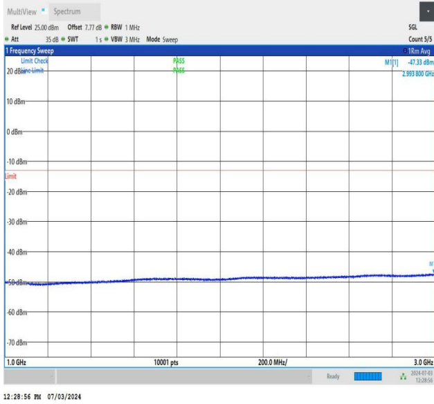
NTNV_DC_26A_n77A-3700-3980_PC2_30_5+50_M+L_TID5_NS_01_1000_3000_#1
