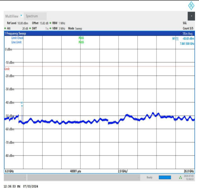
NTNV_DC_26A_n77A-3700-3980_PC2_30_5+50_M+H_TID4_N S_01_6000_26000_#1
