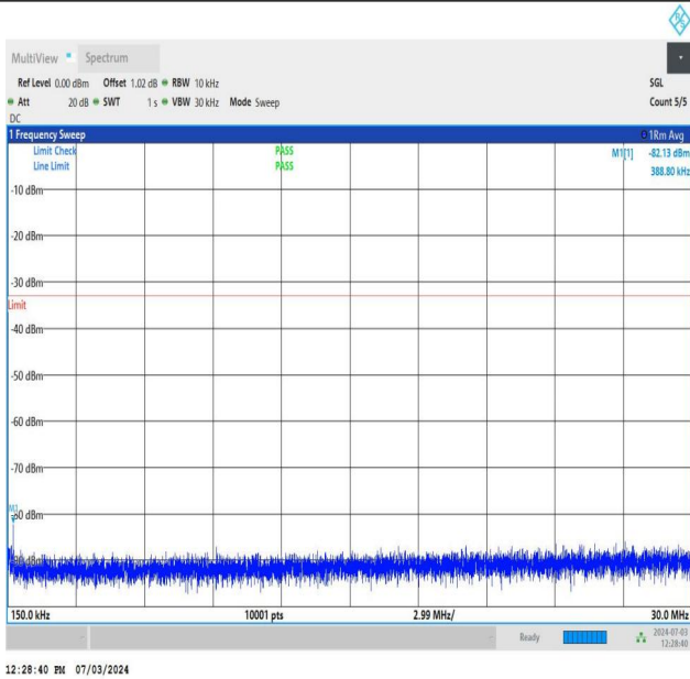
NTNV_DC_26A_n77A-3700-3980_PC2_30_5+50_M+L_TID5_NS_01_0.15_30_#1
