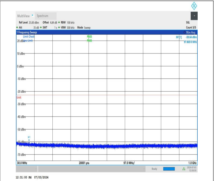
NTNV_DC_26A_n77A-3700-3980_PC2_30_5+50_M+M_TID2_N S_01_30_1000_#1
