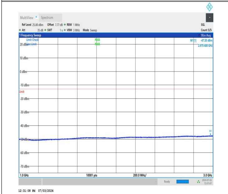
NTNV_DC_26A_n77A-3700-3980_PC2_30_5+50_M+M_TID2_N S_01_1000_3000_#1
