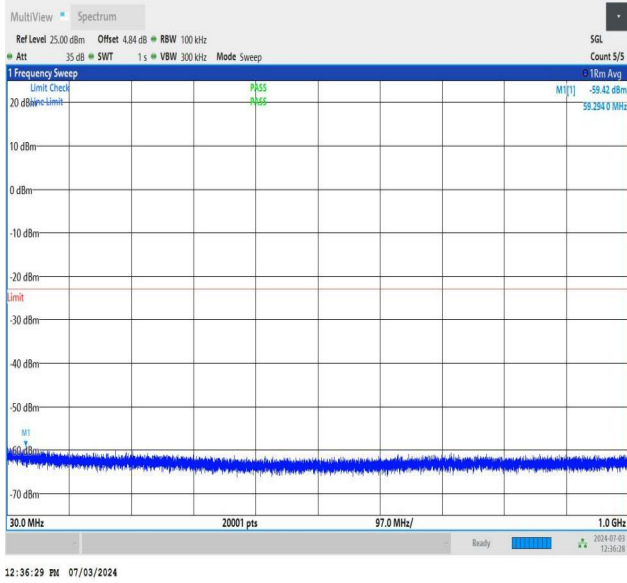
NTNV_DC_26A_n77A-3700-3980_PC2_30_5+50_M+H_TID4_N S_01_30_1000_#1
