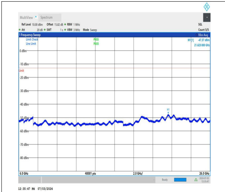
NTNV_DC_26A_n77A-3700-3980_PC2_30_5+50_M+H_TID2_N S_01_6000_26000_#1
