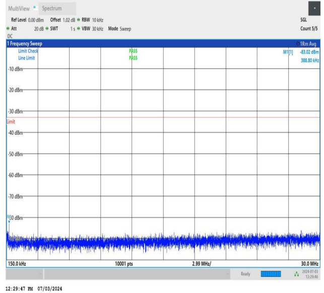
NTNV_DC_26A_n77A-3700-3980_PC2_30_5+50_M+M_TID1_N S_01_0.15_30_#1
