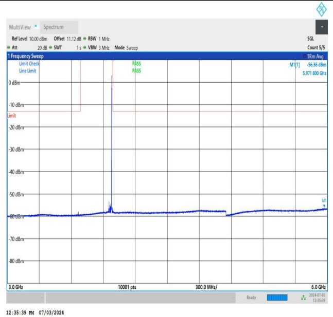
NTNV_DC_26A_n77A-3700-3980_PC2_30_5+50_M+H_TID2_N S_01_3000_6000_#1
