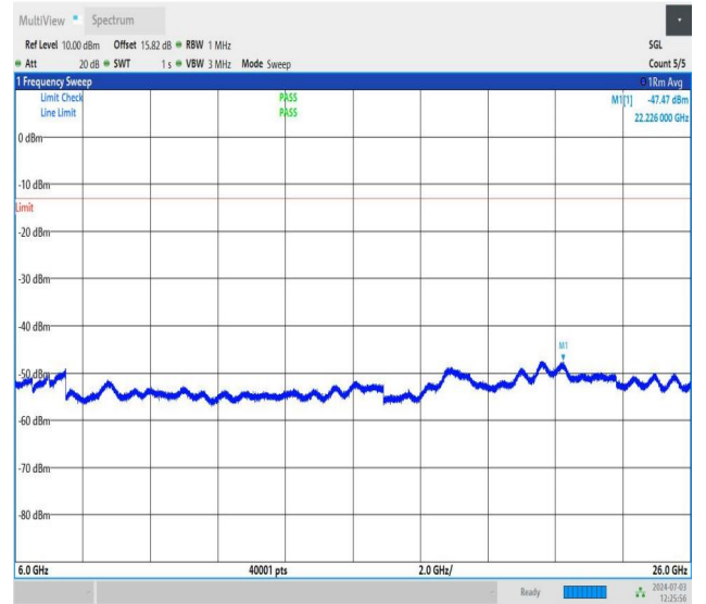
NTNV_DC_26A_n77A-3700-3980_PC2_30_5+50_M+L_TID1_NS_01_6000_26000_#1
