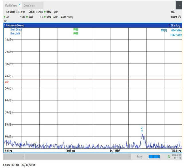
NTNV_DC_26A_n77A-3700-3980_PC2_30_5+50_M+L_TID5_NS_01_0.009_0.15_#1
