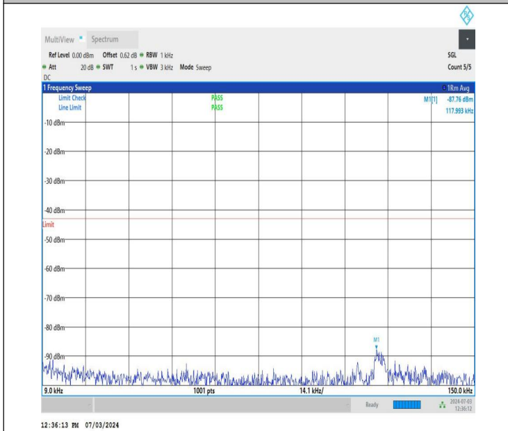
NTNV_DC_26A_n77A-3700-3980_PC2_30_5+50_M+H_TID4_N S_01_0.009_0.15_#1
