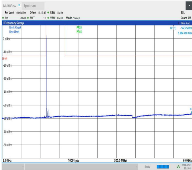
NTNV_DC_26A_n77A-3700-3980_PC2_30_5+50_M+L_TID1_NS_01_3000_6000_#1
