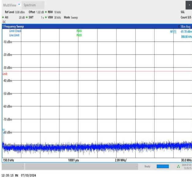
NTNV_DC_26A_n77A-3700-3980_PC2_30_5+50_M+H_TID2_N S_01_0.15_30_#1
