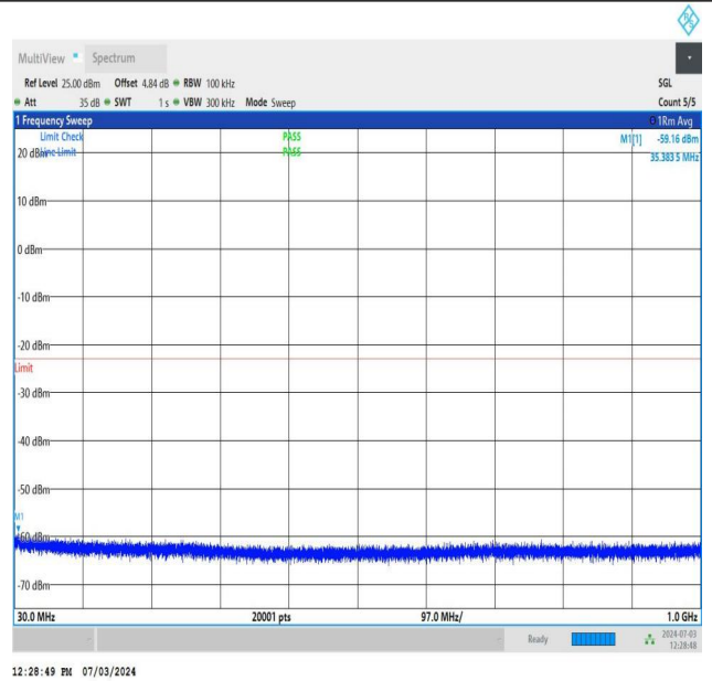
NTNV_DC_26A_n77A-3700-3980_PC2_30_5+50_M+L_TID5_NS_01_30_1000_#1
