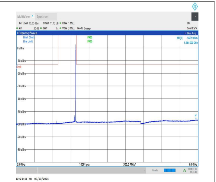
NTNV_DC_26A_n77A-3700-3980_PC2_30_5+40_M+H_TID5_N S_01_3000_6000_#1
