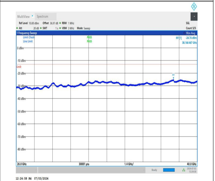
NTNV_DC_26A_n77A-3700-3980_PC2_30_5+40_M+H_TID5_N S_01_26000_40000_#1
