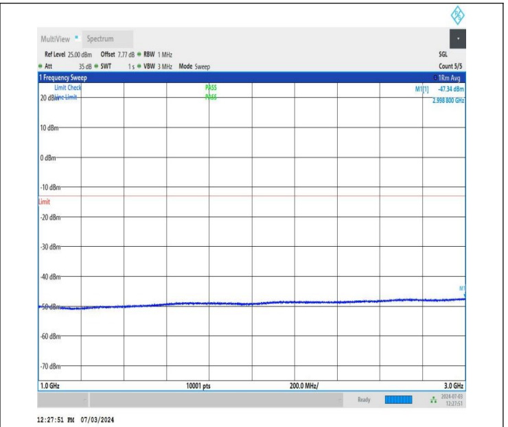
NTNV_DC_26A_n77A-3700-3980_PC2_30_5+50_M+L_TID4_NS_01_1000_3000_#1
