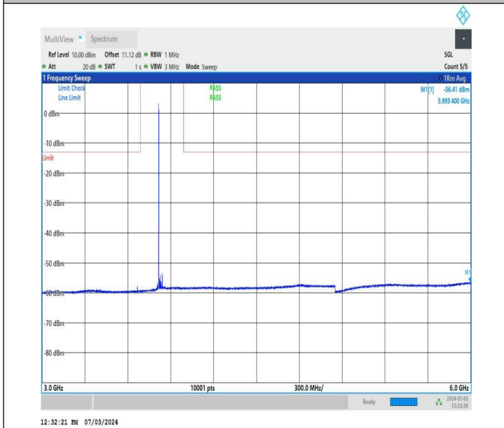
NTNV_DC_26A_n77A-3700-3980_PC2_30_5+50_M+M_TID4_N S_01_3000_6000_#1
