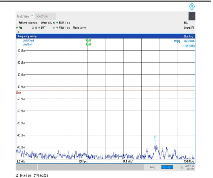
NTNV_DC_26A_n77A-3700-3980_PC2_30_5+50_M+M_TID2_N S_01_0.009_0.15_#1
