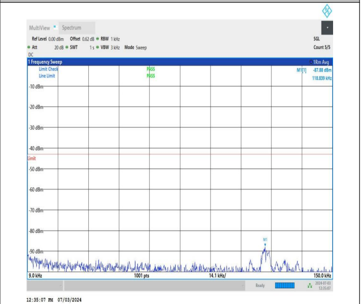
NTNV_DC_26A_n77A-3700-3980_PC2_30_5+50_M+H_TID2_N S_01_0.009_0.15_#1
