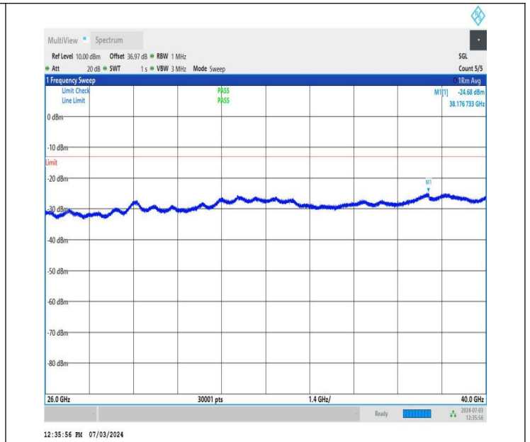
NTNV_DC_26A_n77A-3700-3980_PC2_30_5+50_M+H_TID2_N S_01_26000_40000_#1
