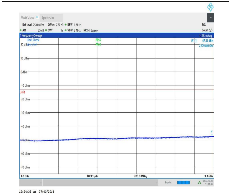
NTNV_DC_26A_n77A-3700-3980_PC2_30_5+40_M+H_TID5_N S_01_1000_3000_#1
