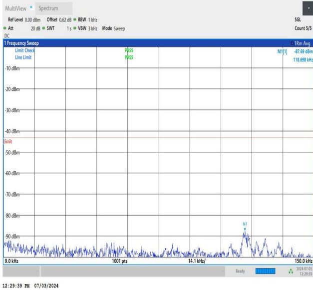
NTNV_DC_26A_n77A-3700-3980_PC2_30_5+50_M+M_TID1_N S_01_0.009_0.15_#1
