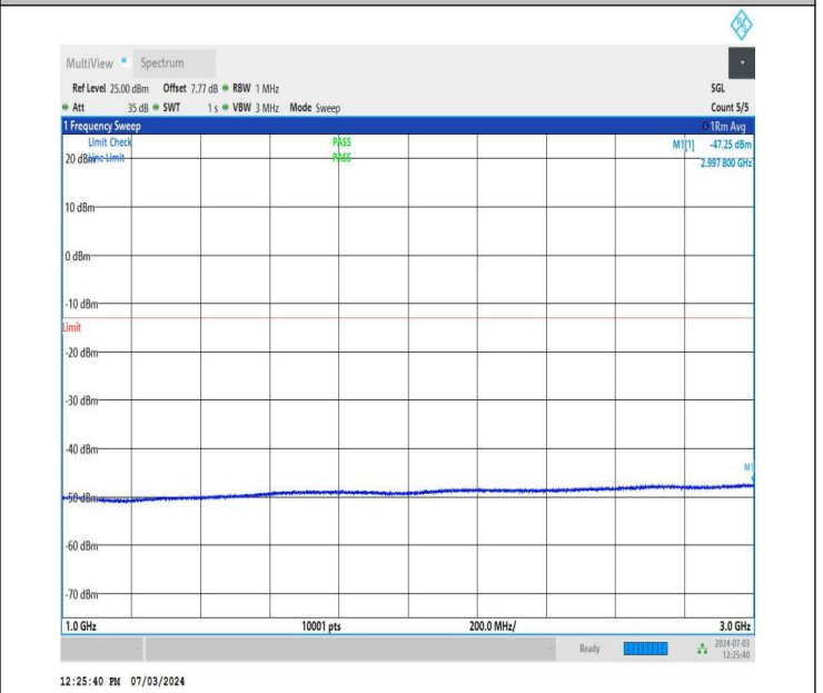
NTNV_DC_26A_n77A-3700-3980_PC2_30_5+50_M+L_TID1_NS_01_1000_3000_#1
