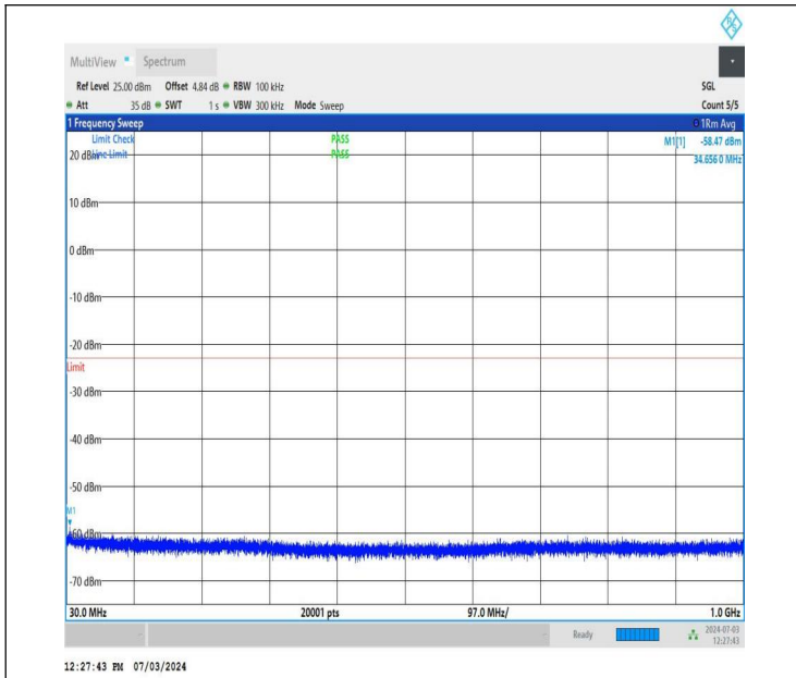
NTNV_DC_26A_n77A-3700-3980_PC2_30_5+50_M+L_TID4_NS_01_30_1000_#1
