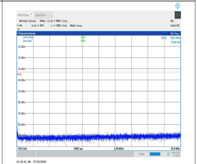
NTNV_DC_26A_n77A-3700-3980_PC2_30_5+50_M+H_TID4_N S_01_0.15_30_#1
