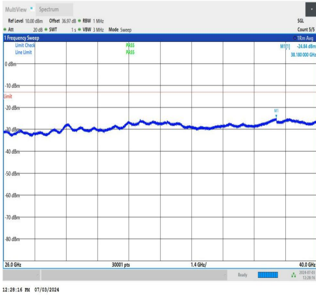
NTNV_DC_26A_n77A-3700-3980_PC2_30_5+50_M+L_TID4_NS_01_26000_40000_#1
