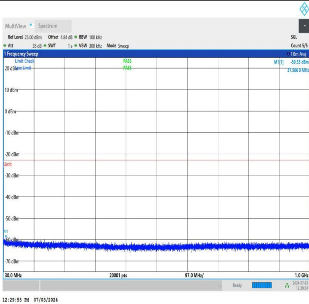
NTNV_DC_26A_n77A-3700-3980_PC2_30_5+50_M+M_TID1_N S_01_30_1000_#1
