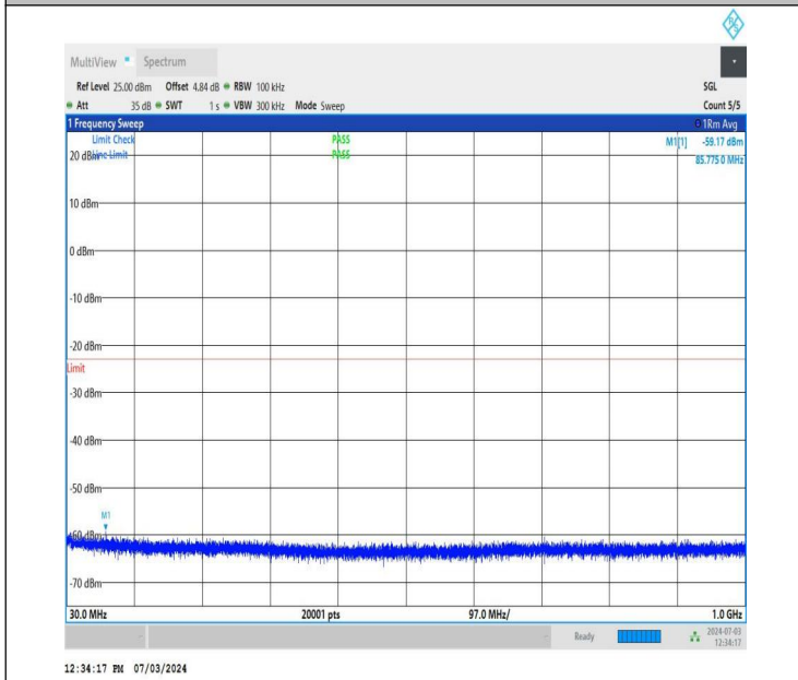
NTNV_DC_26A_n77A-3700-3980_PC2_30_5+50_M+H_TID1_N S_01_30_1000_#1
