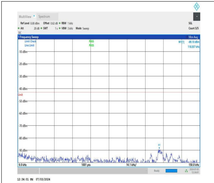
NTNV_DC_26A_n77A-3700-3980_PC2_30_5+50_M+H_TID1_N S_01_0.009_0.15_#1
