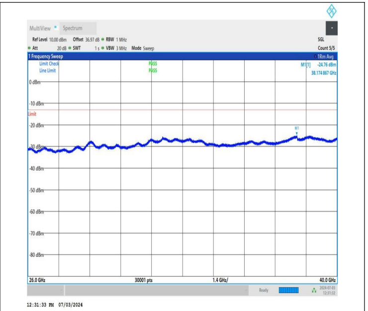
NTNV_DC_26A_n77A-3700-3980_PC2_30_5+50_M+M_TID2_N S_01_26000_40000_#1
