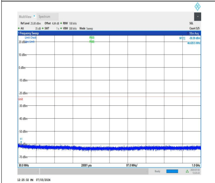
NTNV_DC_26A_n77A-3700-3980_PC2_30_5+50_M+L_TID1_NS_01_30_1000_#1
