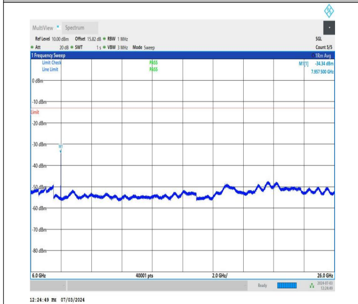
NTNV_DC_26A_n77A-3700-3980_PC2_30_5+40_M+H_TID5_N S_01_6000_26000_#1
