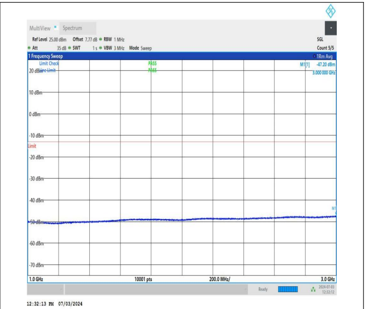
NTNV_DC_26A_n77A-3700-3980_PC2_30_5+50_M+M_TID4_N S_01_1000_3000_#1
