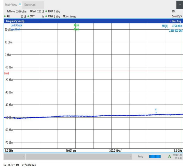
NTNV_DC_26A_n77A-3700-3980_PC2_30_5+50_M+H_TID4_N S_01_1000_3000_#1
