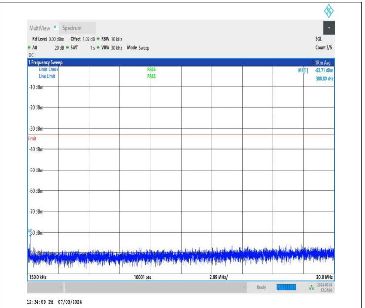
NTNV_DC_26A_n77A-3700-3980_PC2_30_5+50_M+H_TID1_N S_01_0.15_30_#1
