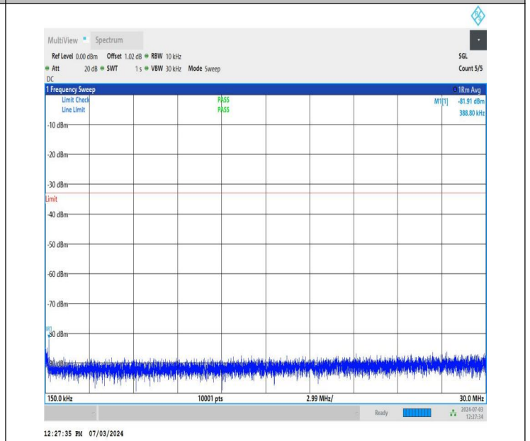
NTNV_DC_26A_n77A-3700-3980_PC2_30_5+50_M+L_TID4_NS_01_0.15_30_#1
