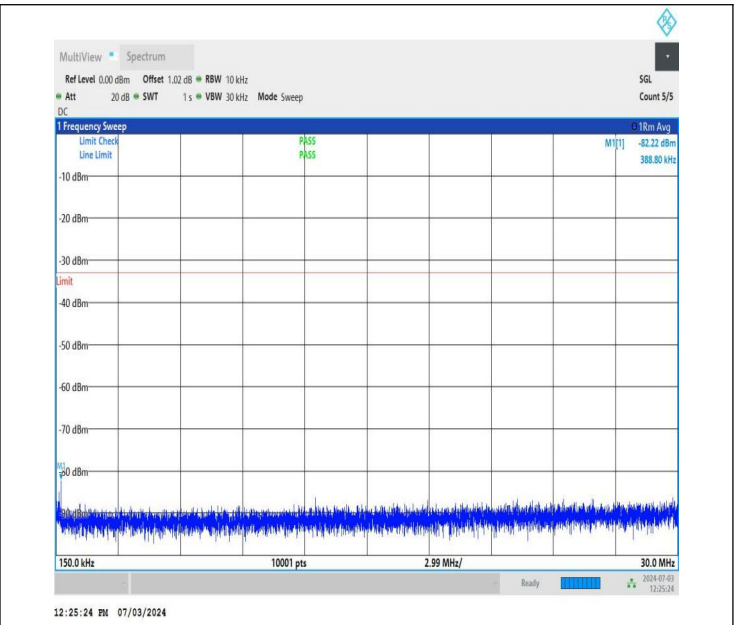
NTNV_DC_26A_n77A-3700-3980_PC2_30_5+50_M+L_TID1_NS_01_0.15_30_#1
