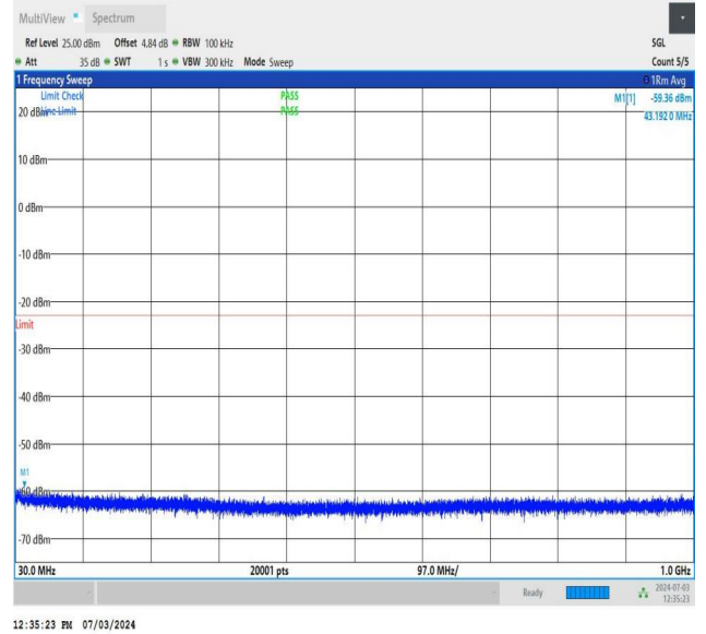
NTNV_DC_26A_n77A-3700-3980_PC2_30_5+50_M+H_TID2_N S_01_30_1000_#1
