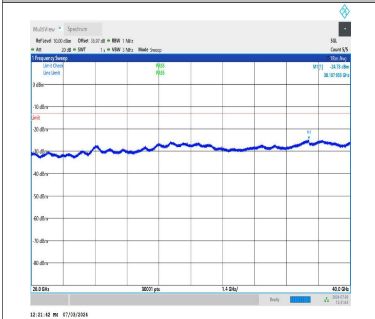
NTNV_DC_26A_n77A-3700-3980_PC2_30_5+40_M+H_TID1_N S_01_26000_40000_#1
