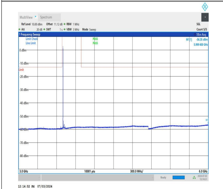
NTNV_DC_26A_n77A-3700-3980_PC2_30_5+40_M+L_TID4_NS_01_3000_6000_#1
