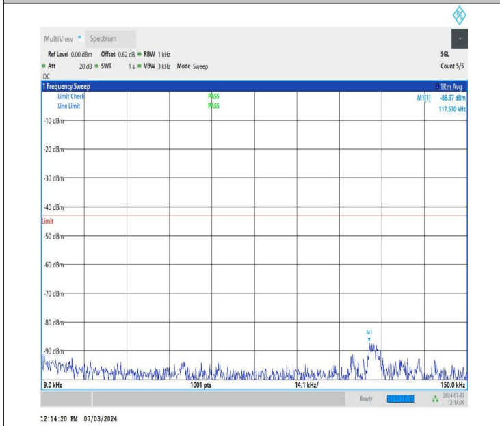
NTNV_DC_26A_n77A-3700-3980_PC2_30_5+40_M+L_TID4_NS_01_0.009_0.15_#1
