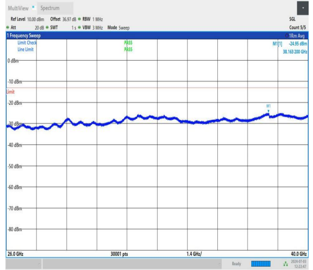
NTNV_DC_26A_n77A-3700-3980_PC2_30_5+40_M+H_TID2_N S_01_26000_40000_#1
