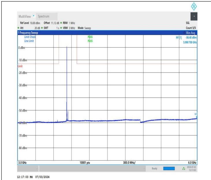
NTNV_DC_26A_n77A-3700-3980_PC2_30_5+40_M+M_TID1_N S_01_3000_6000_#1
