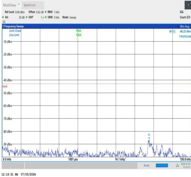
NTNV_DC_26A_n77A-3700-3980_PC2_30_5+40_M+M_TID1_N S_01_0.009_0.15_#1
