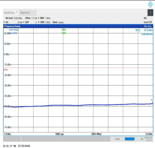
NTNV_DC_26A_n77A-3700-3980_PC2_30_5+40_M+H_TID1_N S_01_1000_3000_#1
