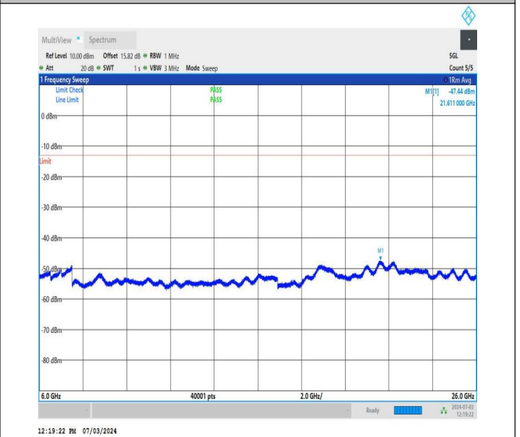
NTNV_DC_26A_n77A-3700-3980_PC2_30_5+40_M+M_TID4_N S_01_6000_26000_#1
