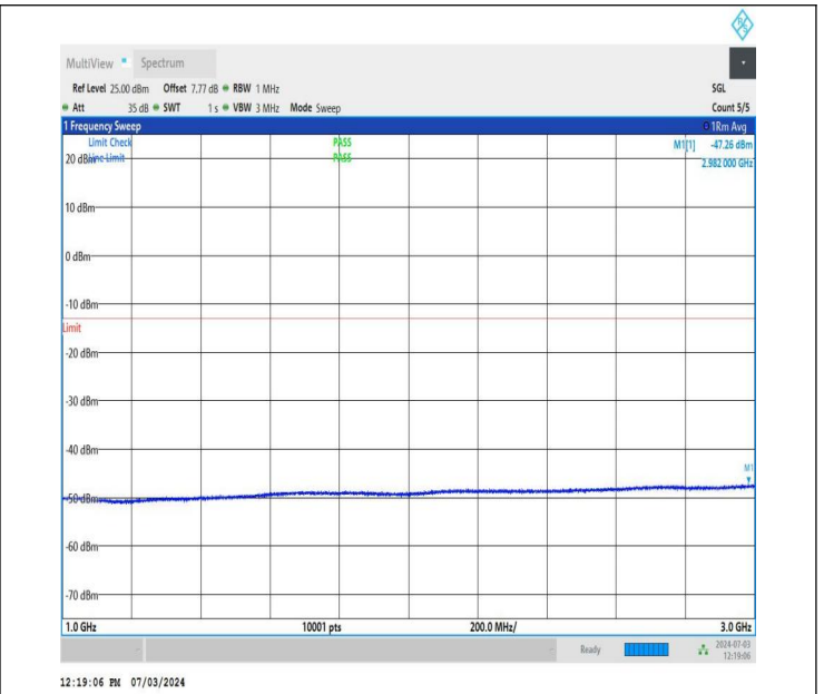
NTNV_DC_26A_n77A-3700-3980_PC2_30_5+40_M+M_TID4_N S_01_1000_3000_#1
