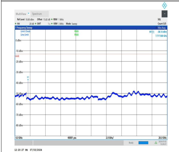
NTNV_DC_26A_n77A-3700-3980_PC2_30_5+40_M+M_TID5_N S_01_6000_26000_#1
