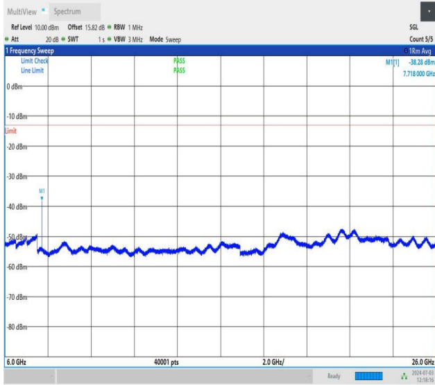
NTNV_DC_26A_n77A-3700-3980_PC2_30_5+40_M+M_TID2_N S_01_6000_26000_#1
