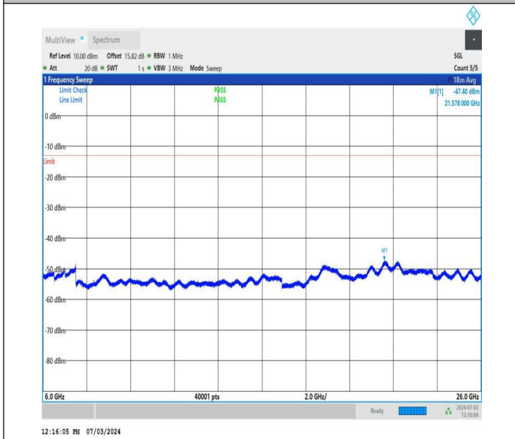
NTNV_DC_26A_n77A-3700-3980_PC2_30_5+40_M+L_TID5_NS_01_6000_26000_#1
