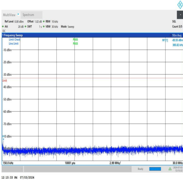
NTNV_DC_26A_n77A-3700-3980_PC2_30_5+40_M+L_TID5_NS_01_0.15_30_#1
