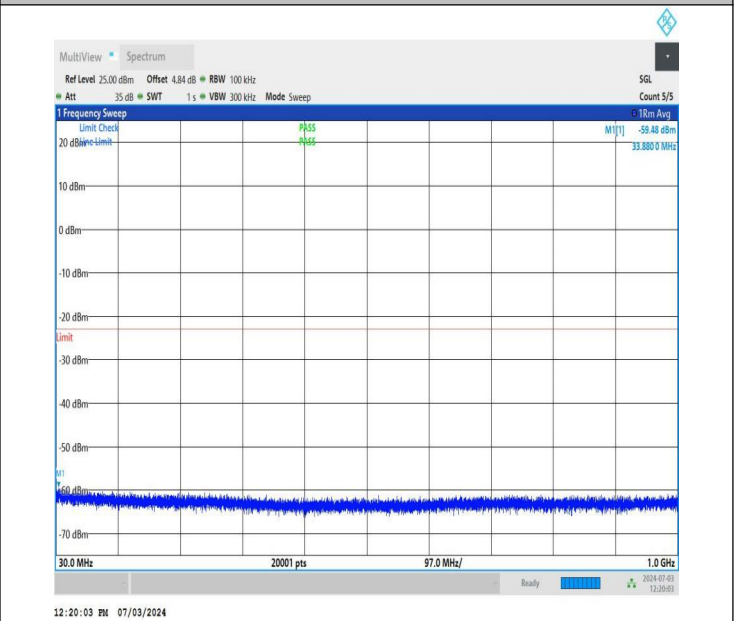
NTNV_DC_26A_n77A-3700-3980_PC2_30_5+40_M+M_TID5_N S_01_30_1000_#1
