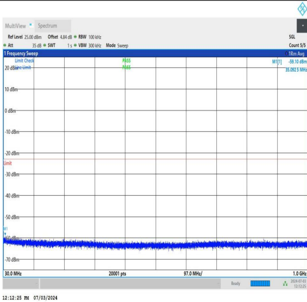
NTNV_DC_26A_n77A-3700-3980_PC2_30_5+40_M+L_TID1_NS_01_30_1000_#1
