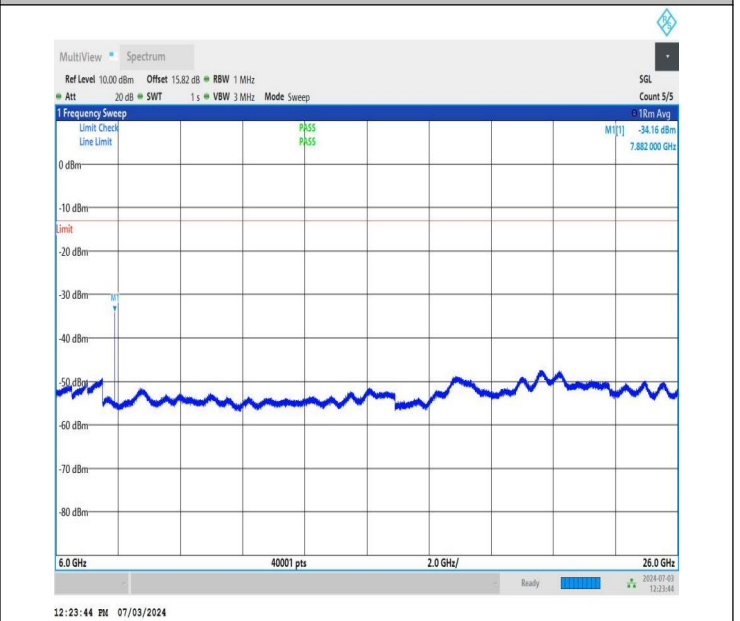
NTNV_DC_26A_n77A-3700-3980_PC2_30_5+40_M+H_TID4_N S_01_6000_26000_#1
