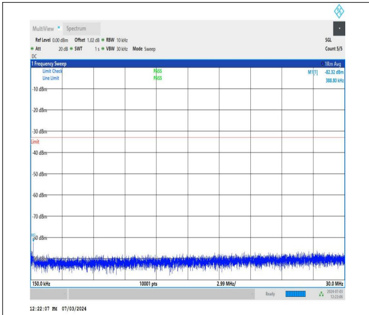
NTNV_DC_26A_n77A-3700-3980_PC2_30_5+40_M+H_TID2_N S_01_0.15_30_#1
