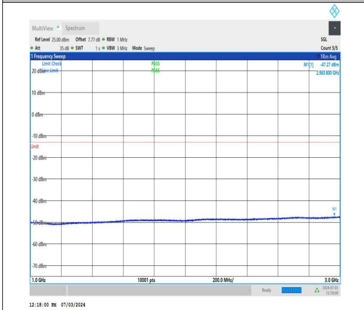
NTNV_DC_26A_n77A-3700-3980_PC2_30_5+40_M+M_TID2_N S_01_1000_3000_#1
