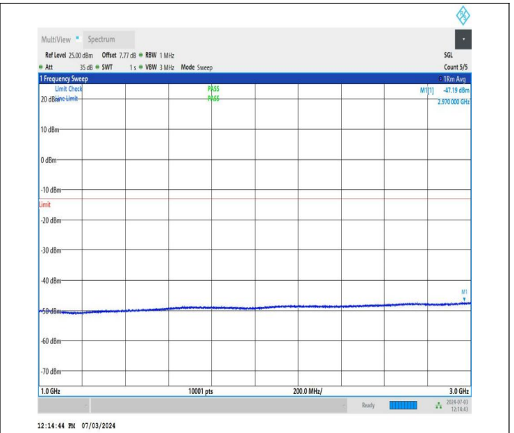
NTNV_DC_26A_n77A-3700-3980_PC2_30_5+40_M+L_TID4_NS_01_1000_3000_#1
