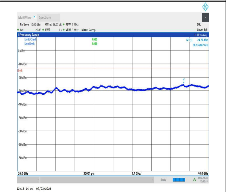
NTNV_DC_26A_n77A-3700-3980_PC2_30_5+40_M+L_TID5_NS_01_26000_40000_#1
