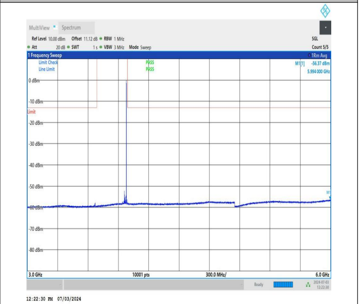
NTNV_DC_26A_n77A-3700-3980_PC2_30_5+40_M+H_TID2_N S_01_3000_6000_#1
