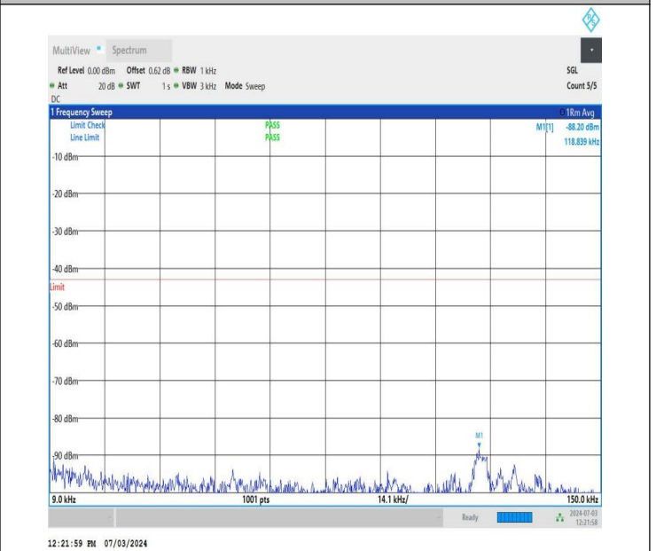
NTNV_DC_26A_n77A-3700-3980_PC2_30_5+40_M+H_TID2_N S_01_0.009_0.15_#1
