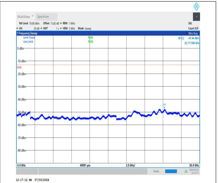
NTNV_DC_26A_n77A-3700-3980_PC2_30_5+40_M+M_TID1_N S_01_6000_26000_#1
