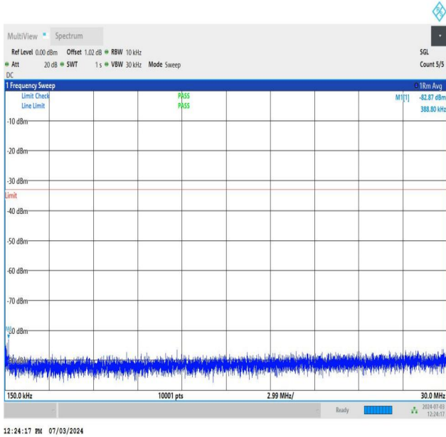
NTNV_DC_26A_n77A-3700-3980_PC2_30_5+40_M+H_TID5_N S_01_0.15_30_#1
