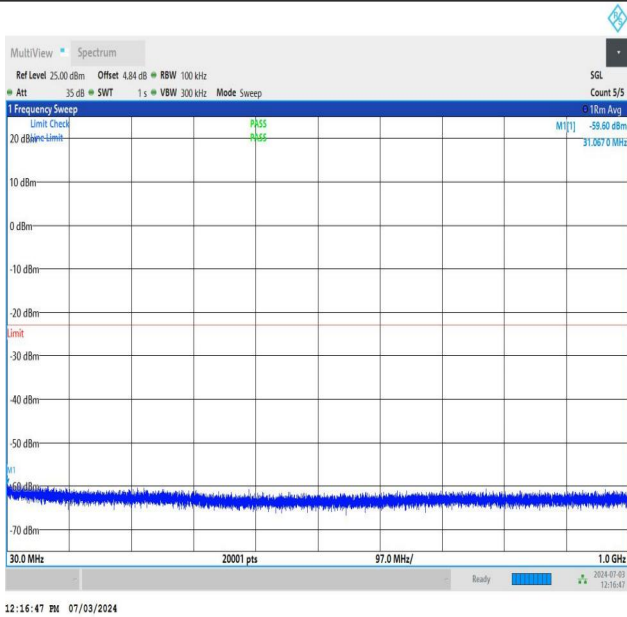
NTNV_DC_26A_n77A-3700-3980_PC2_30_5+40_M+M_TID1_N S_01_30_1000_#1
