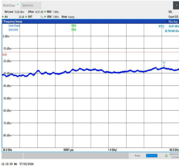
NTNV_DC_26A_n77A-3700-3980_PC2_30_5+40_M+L_TID4_NS_01_26000_40000_#1
