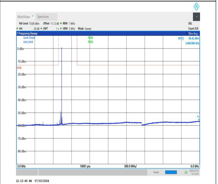
NTNV_DC_26A_n77A-3700-3980_PC2_30_5+40_M+L_TID2_NS_01_3000_6000_#1
