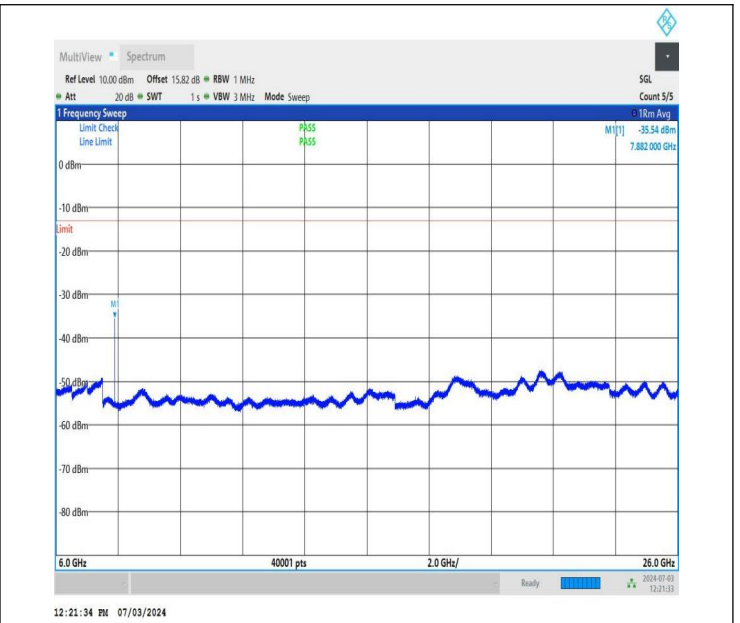
NTNV_DC_26A_n77A-3700-3980_PC2_30_5+40_M+H_TID1_N S_01_6000_26000_#1
