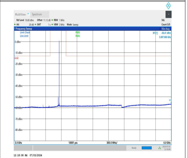
NTNV_DC_26A_n77A-3700-3980_PC2_30_5+40_M+M_TID2_N S_01_3000_6000_#1
