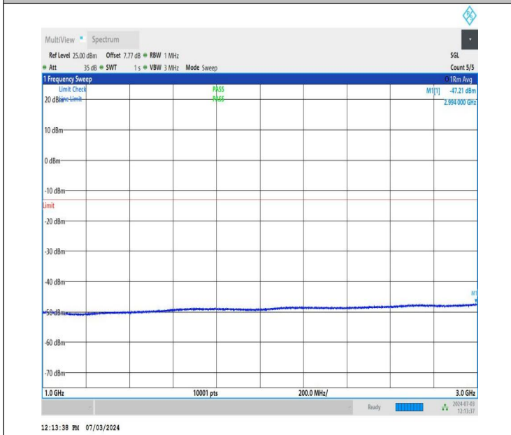
NTNV_DC_26A_n77A-3700-3980_PC2_30_5+40_M+L_TID2_NS_01_1000_3000_#1
