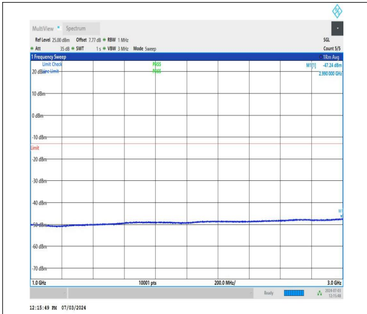
NTNV_DC_26A_n77A-3700-3980_PC2_30_5+40_M+L_TID5_NS_01_1000_3000_#1
