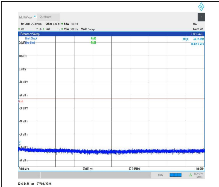
NTNV_DC_26A_n77A-3700-3980_PC2_30_5+40_M+L_TID4_NS_01_30_1000_#1
