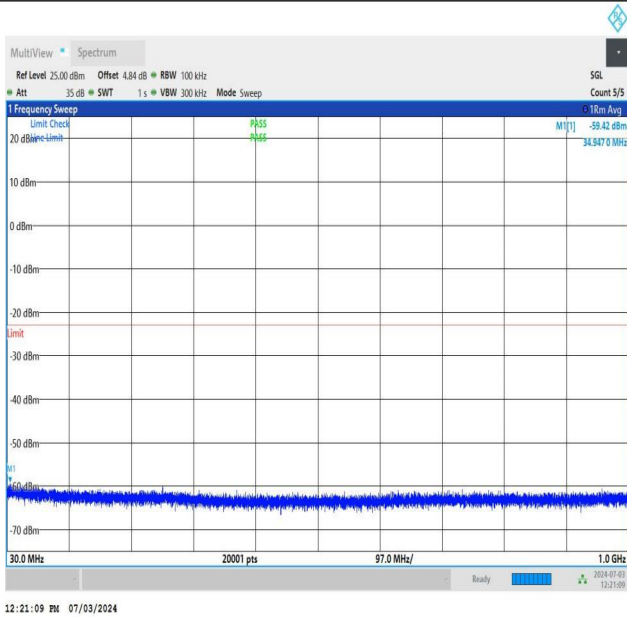
NTNV_DC_26A_n77A-3700-3980_PC2_30_5+40_M+H_TID1_N S_01_30_1000_#1
