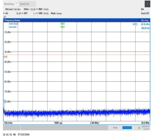
NTNV_DC_26A_n77A-3700-3980_PC2_30_5+40_M+H_TID1_N S_01_0.15_30_#1
