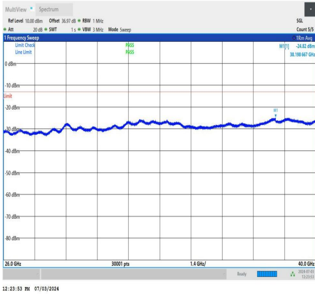
NTNV_DC_26A_n77A-3700-3980_PC2_30_5+40_M+H_TID4_N S_01_26000_40000_#1
