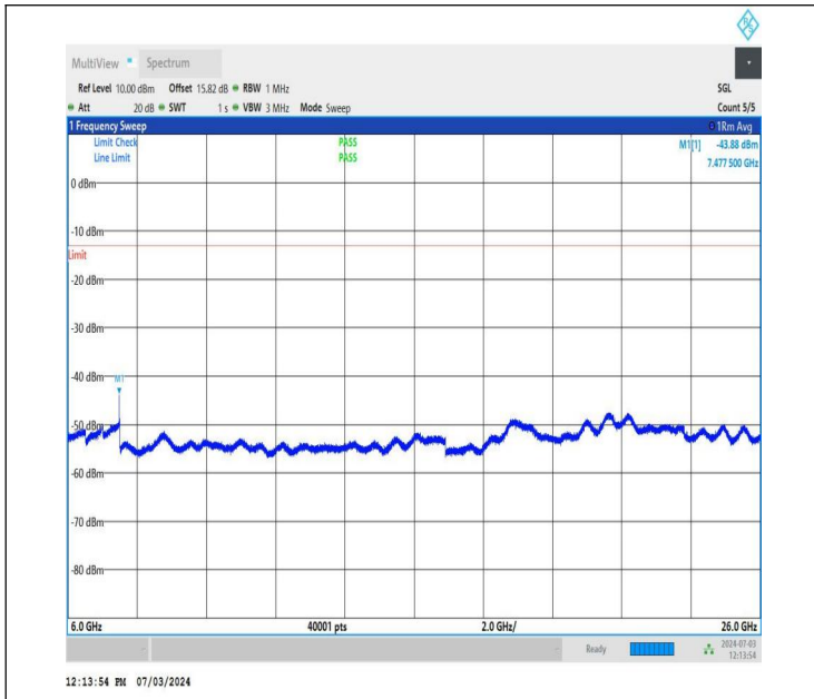
NTNV_DC_26A_n77A-3700-3980_PC2_30_5+40_M+L_TID2_NS_01_6000_26000_#1
