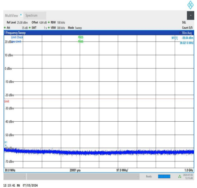
NTNV_DC_26A_n77A-3700-3980_PC2_30_5+40_M+L_TID5_NS_01_30_1000_#1
