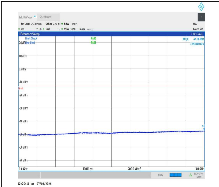
NTNV_DC_26A_n77A-3700-3980_PC2_30_5+40_M+M_TID5_N S_01_1000_3000_#1
