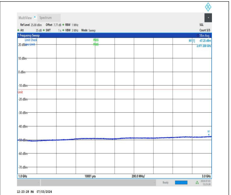
NTNV_DC_26A_n77A-3700-3980_PC2_30_5+40_M+H_TID4_N S_01_1000_3000_#1
