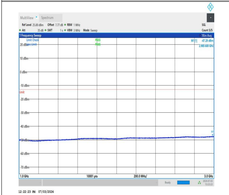
NTNV_DC_26A_n77A-3700-3980_PC2_30_5+40_M+H_TID2_N S_01_1000_3000_#1
