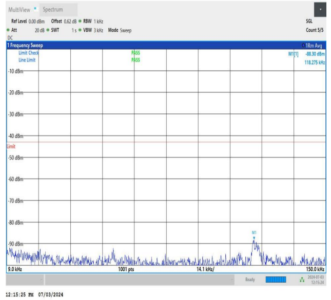
NTNV_DC_26A_n77A-3700-3980_PC2_30_5+40_M+L_TID5_NS_01_0.009_0.15_#1
