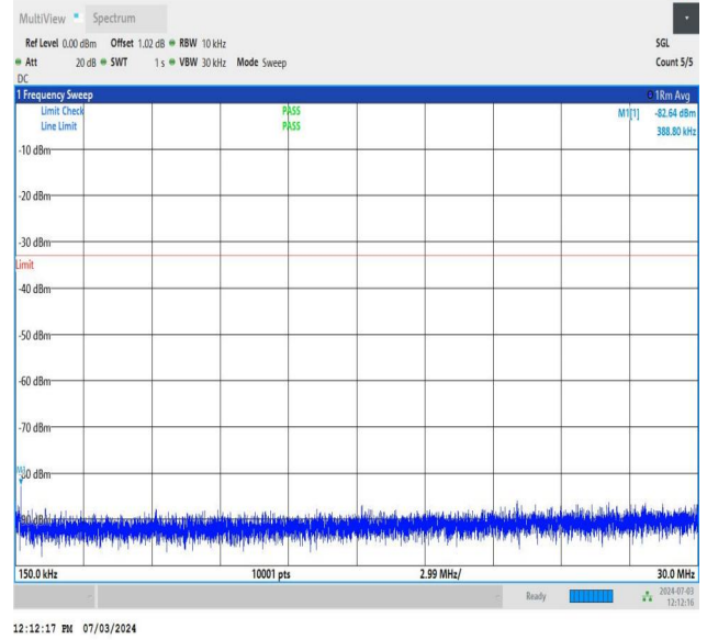
NTNV_DC_26A_n77A-3700-3980_PC2_30_5+40_M+L_TID1_NS_01_0.15_30_#1
