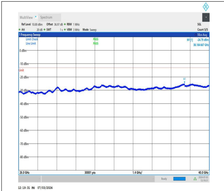
NTNV_DC_26A_n77A-3700-3980_PC2_30_5+40_M+M_TID4_N S_01_26000_40000_#1
