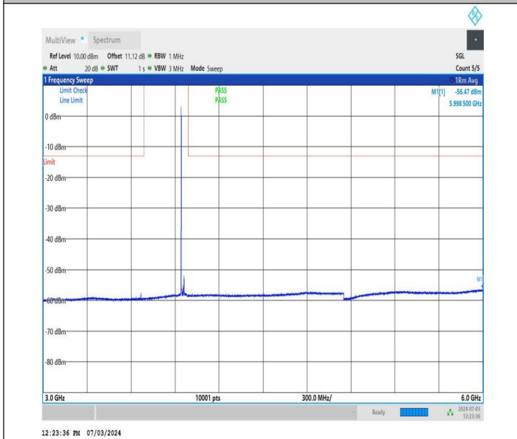
NTNV_DC_26A_n77A-3700-3980_PC2_30_5+40_M+H_TID4_N S_01_3000_6000_#1
