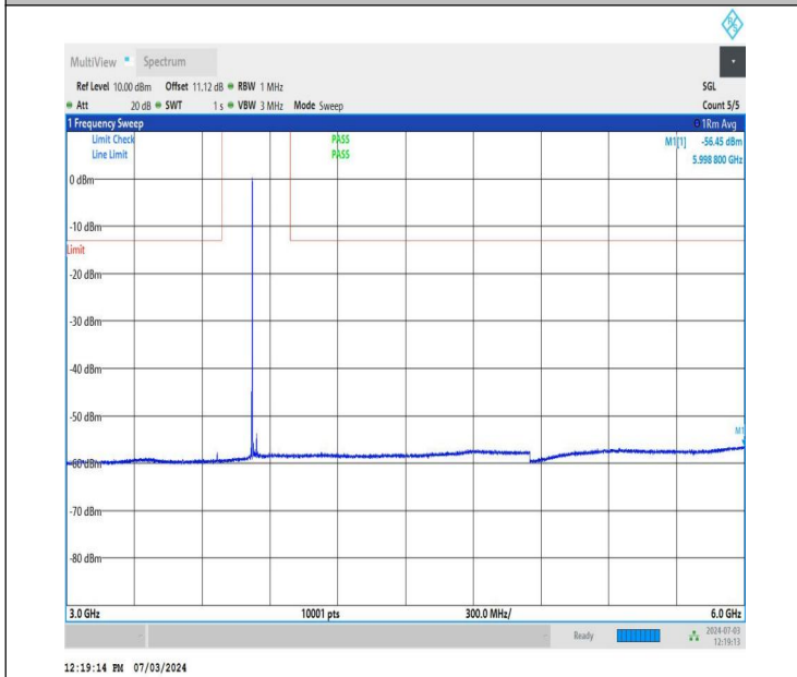
NTNV_DC_26A_n77A-3700-3980_PC2_30_5+40_M+M_TID4_N S_01_3000_6000_#1
