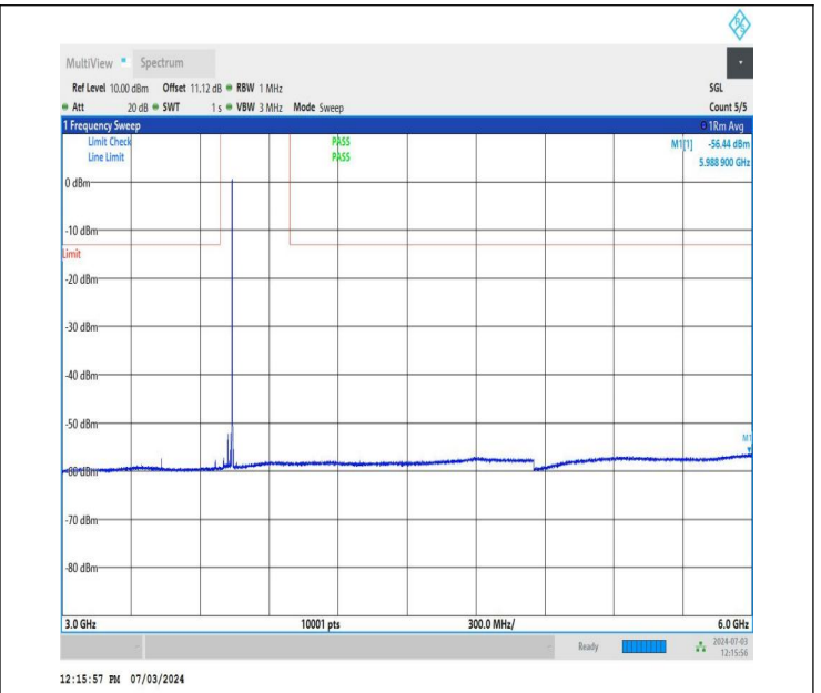
NTNV_DC_26A_n77A-3700-3980_PC2_30_5+40_M+L_TID5_NS_01_3000_6000_#1
