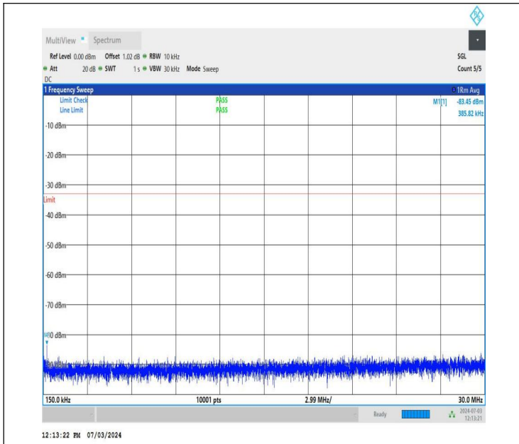
NTNV_DC_26A_n77A-3700-3980_PC2_30_5+40_M+L_TID2_NS_01_0.15_30_#1
