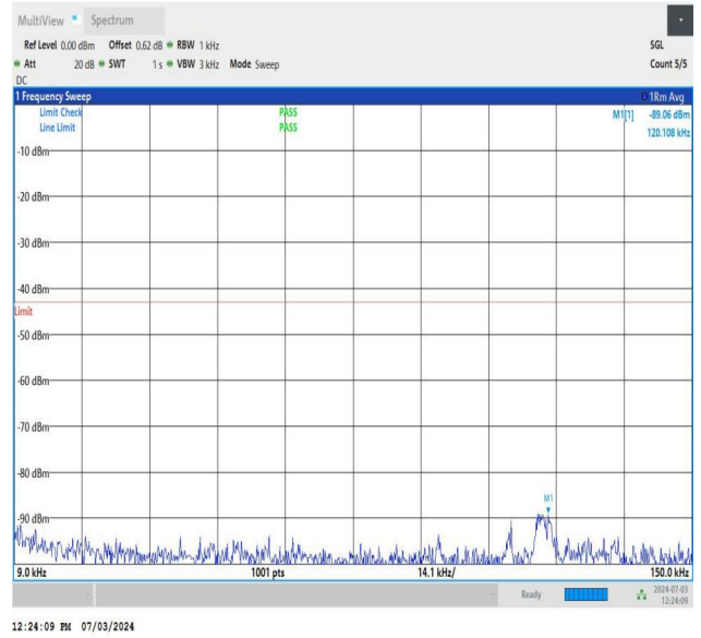
NTNV_DC_26A_n77A-3700-3980_PC2_30_5+40_M+H_TID5_N S_01_0.009_0.15_#1
