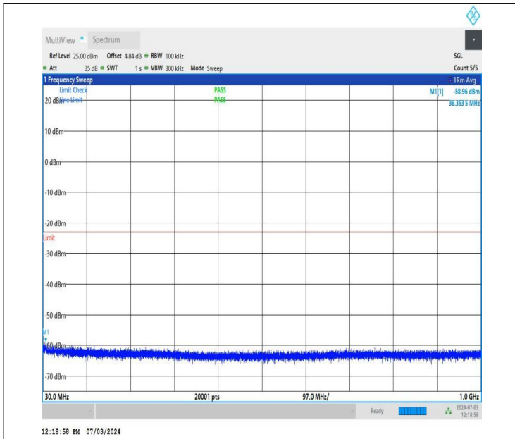
NTNV_DC_26A_n77A-3700-3980_PC2_30_5+40_M+M_TID4_N S_01_30_1000_#1
