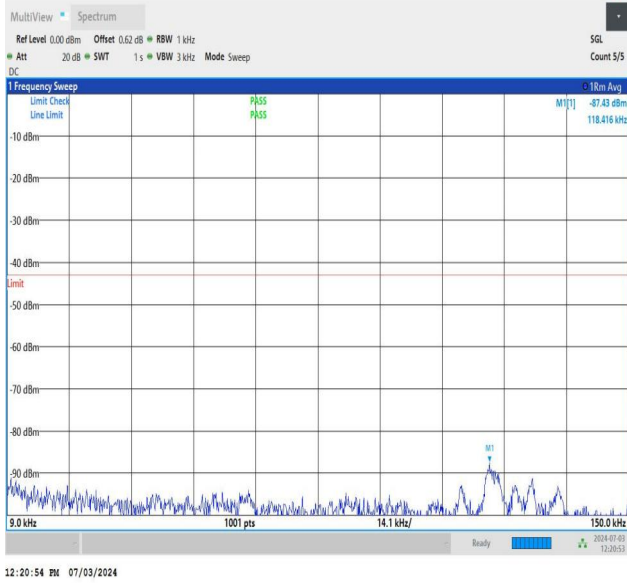
NTNV_DC_26A_n77A-3700-3980_PC2_30_5+40_M+H_TID1_N S_01_0.009_0.15_#1
