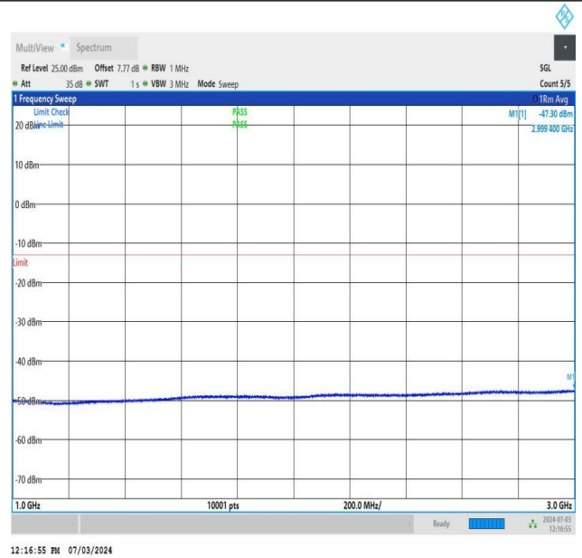
NTNV_DC_26A_n77A-3700-3980_PC2_30_5+40_M+M_TID1_N S_01_1000_3000_#1
