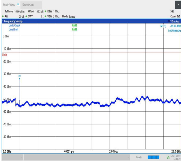
NTNV_DC_26A_n77A-3700-3980_PC2_30_5+40_M+H_TID2_N S_01_6000_26000_#1
