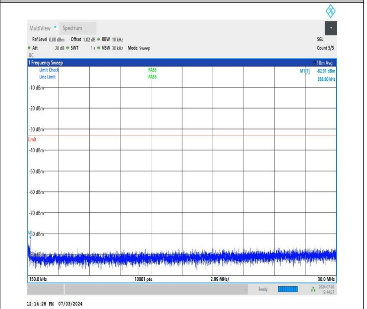
NTNV_DC_26A_n77A-3700-3980_PC2_30_5+40_M+L_TID4_NS_01_0.15_30_#1
