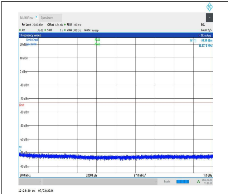
NTNV_DC_26A_n77A-3700-3980_PC2_30_5+40_M+H_TID4_N S_01_30_1000_#1
