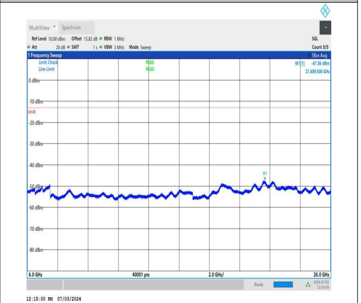
NTNV_DC_26A_n77A-3700-3980_PC2_30_5+40_M+L_TID4_NS_01_6000_26000_#1
