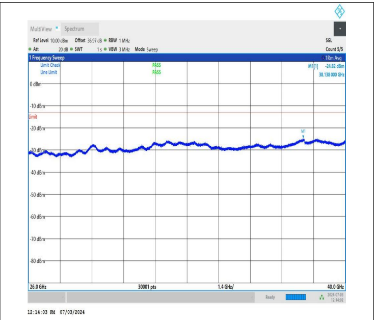
NTNV_DC_26A_n77A-3700-3980_PC2_30_5+40_M+L_TID2_NS_01_26000_40000_#1
