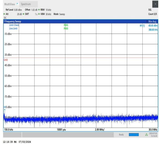
NTNV_DC_26A_n77A-3700-3980_PC2_30_5+40_M+M_TID1_N S_01_0.15_30_#1
