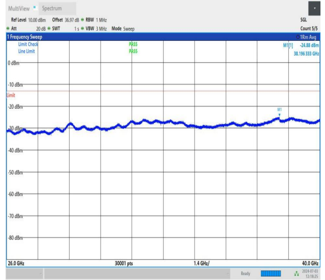
NTNV_DC_26A_n77A-3700-3980_PC2_30_5+40_M+M_TID2_N S_01_26000_40000_#1
