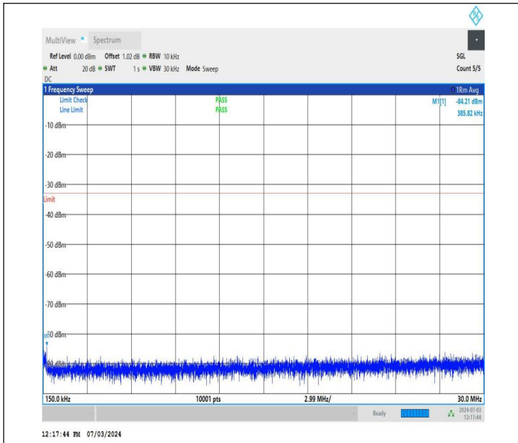
NTNV_DC_26A_n77A-3700-3980_PC2_30_5+40_M+M_TID2_N S_01_0.15_30_#1
