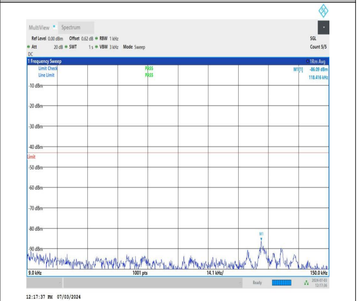
NTNV_DC_26A_n77A-3700-3980_PC2_30_5+40_M+M_TID2_N S_01_0.009_0.15_#1
