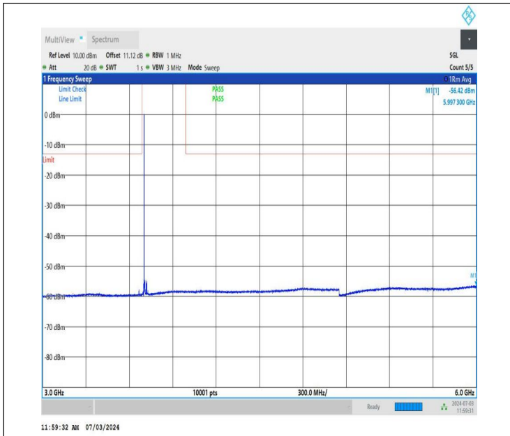
NTNV_DC_26A_n77A-3700-3980_PC2_30_5+30_M+L_TID1_NS_01_3000_6000_#1
