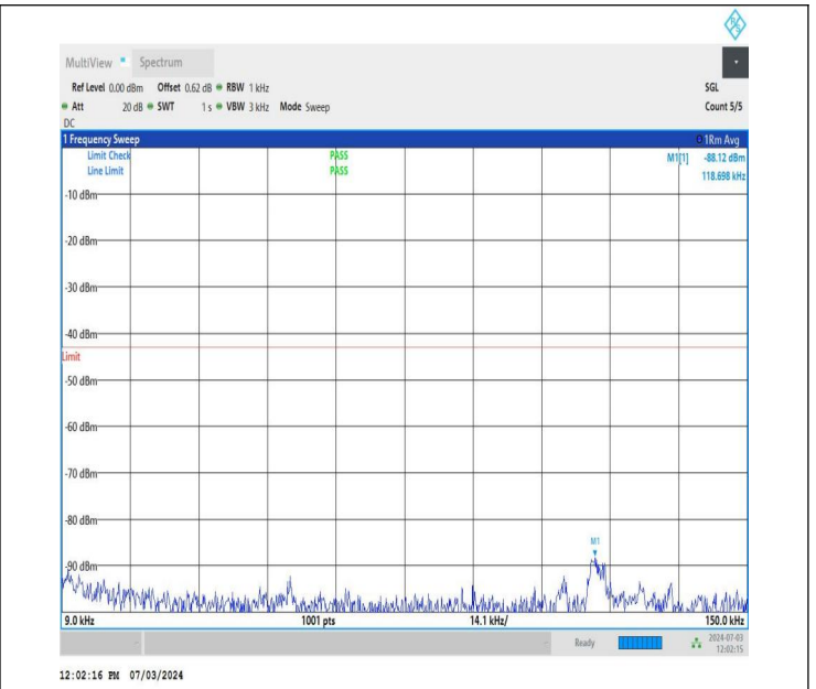
NTNV_DC_26A_n77A-3700-3980_PC2_30_5+30_M+L_TID5_NS_01_0.009_0.15_#1
