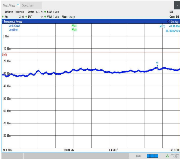
NTNV_DC_26A_n77A-3700-3980_PC2_30_5+30_M+M_TID4_N S_01_26000_40000_#1
