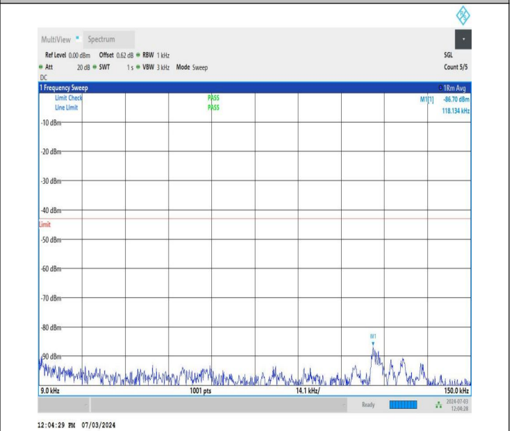
NTNV_DC_26A_n77A-3700-3980_PC2_30_5+30_M+M_TID2_N S_01_0.009_0.15_#1
