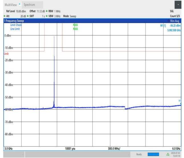
NTNV_DC_26A_n77A-3700-3980_PC2_30_5+30_M+M_TID5_N S_01_3000_6000_#1
