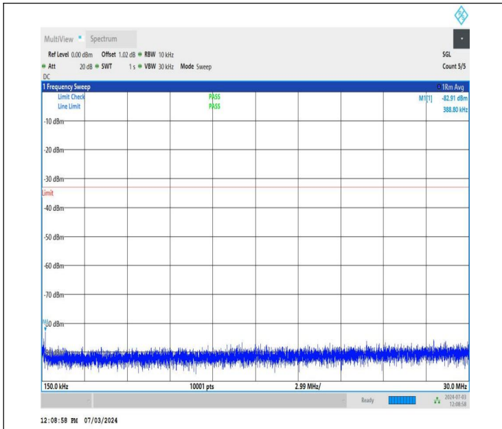
NTNV_DC_26A_n77A-3700-3980_PC2_30_5+30_M+H_TID2_N S_01_0.15_30_#1
