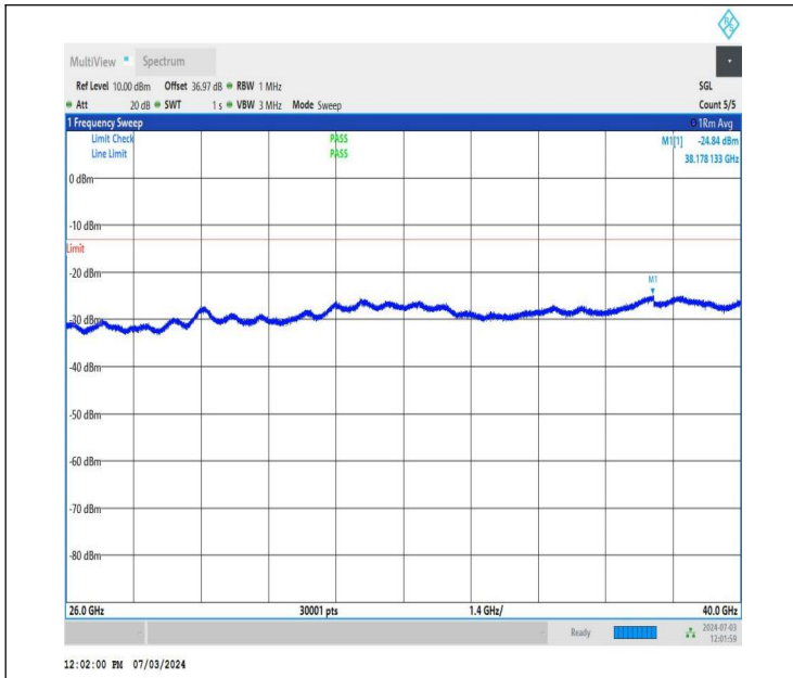
NTNV_DC_26A_n77A-3700-3980_PC2_30_5+30_M+L_TID4_NS_01_26000_40000_#1
