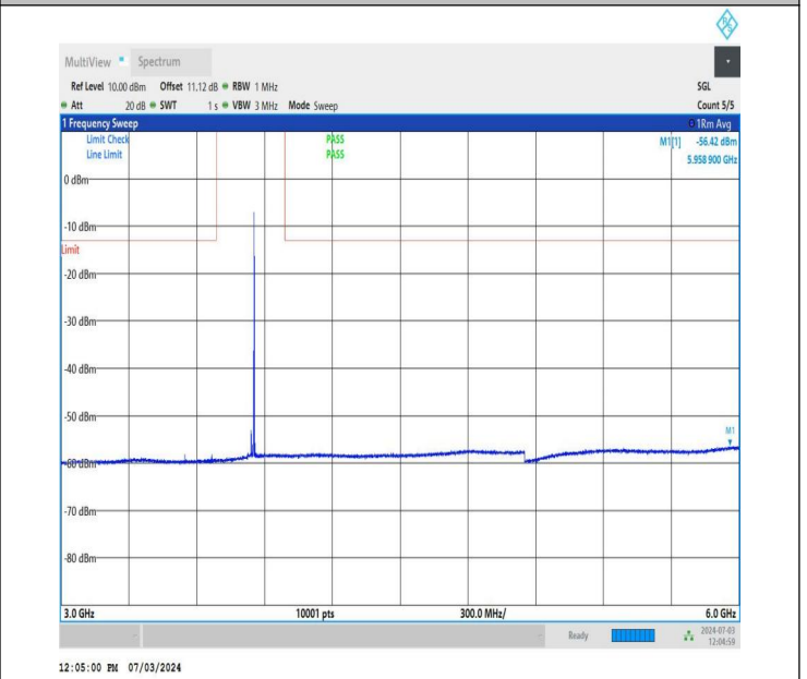
NTNV_DC_26A_n77A-3700-3980_PC2_30_5+30_M+M_TID2_N S_01_3000_6000_#1
