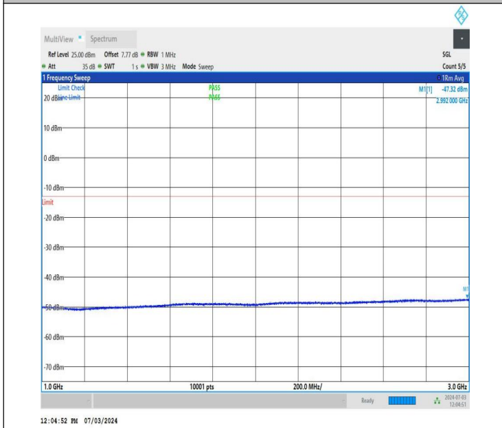
NTNV_DC_26A_n77A-3700-3980_PC2_30_5+30_M+M_TID2_N S_01_1000_3000_#1
