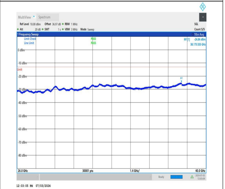
NTNV_DC_26A_n77A-3700-3980_PC2_30_5+30_M+L_TID5_NS_01_26000_40000_#1
