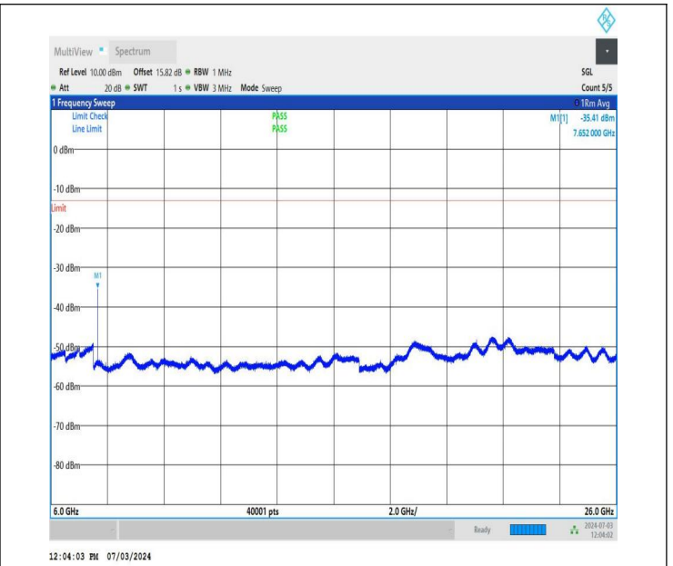
NTNV_DC_26A_n77A-3700-3980_PC2_30_5+30_M+M_TID1_N S_01_6000_26000_#1
