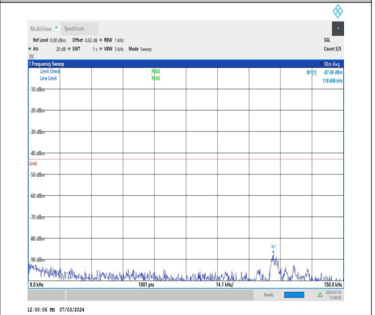
NTNV_DC_26A_n77A-3700-3980_PC2_30_5+30_M+L_TID2_NS_01_0.009_0.15_#1
