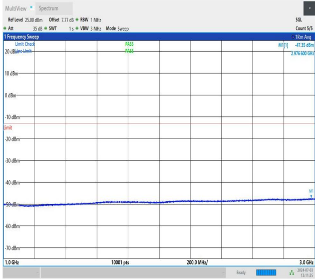
NTNV_DC_26A_n77A-3700-3980_PC2_30_5+30_M+H_TID5_N S_01_1000_3000_#1
