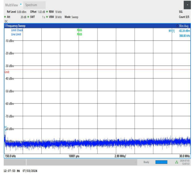
NTNV_DC_26A_n77A-3700-3980_PC2_30_5+30_M+H_TID1_N S_01_0.15_30_#1
