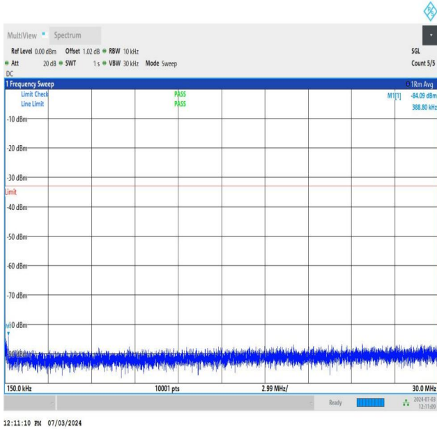
NTNV_DC_26A_n77A-3700-3980_PC2_30_5+30_M+H_TID5_N S_01_0.15_30_#1
