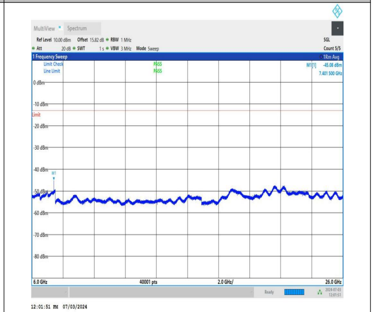
NTNV_DC_26A_n77A-3700-3980_PC2_30_5+30_M+L_TID4_NS_01_6000_26000_#1
