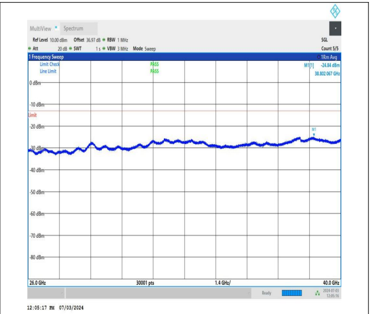
NTNV_DC_26A_n77A-3700-3980_PC2_30_5+30_M+M_TID2_N S_01_26000_40000_#1
