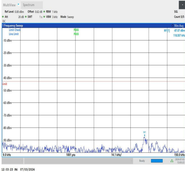
NTNV_DC_26A_n77A-3700-3980_PC2_30_5+30_M+M_TID1_N S_01_0.009_0.15_#1
