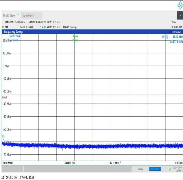
NTNV_DC_26A_n77A-3700-3980_PC2_30_5+30_M+H_TID1_N S_01_30_1000_#1
