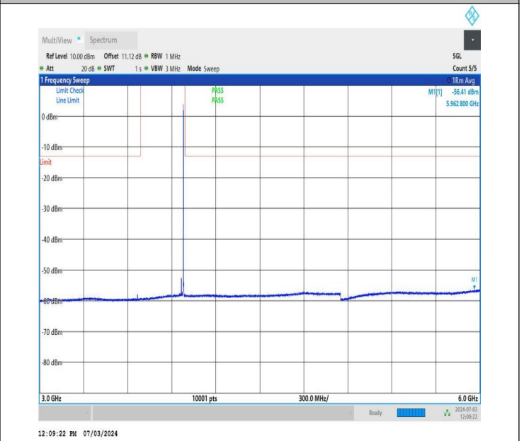
NTNV_DC_26A_n77A-3700-3980_PC2_30_5+30_M+H_TID2_N S_01_3000_6000_#1
