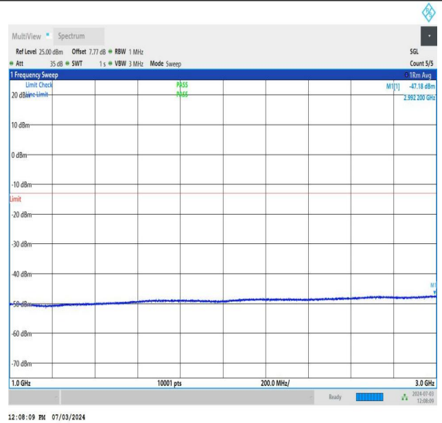
NTNV_DC_26A_n77A-3700-3980_PC2_30_5+30_M+H_TID1_N S_01_1000_3000_#1
