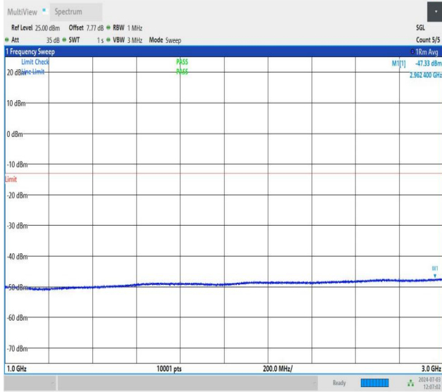
NTNV_DC_26A_n77A-3700-3980_PC2_30_5+30_M+M_TID5_N S_01_1000_3000_#1
