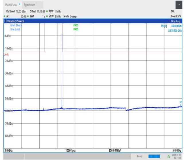
NTNV_DC_26A_n77A-3700-3980_PC2_30_5+30_M+H_TID5_N S_01_3000_6000_#1
