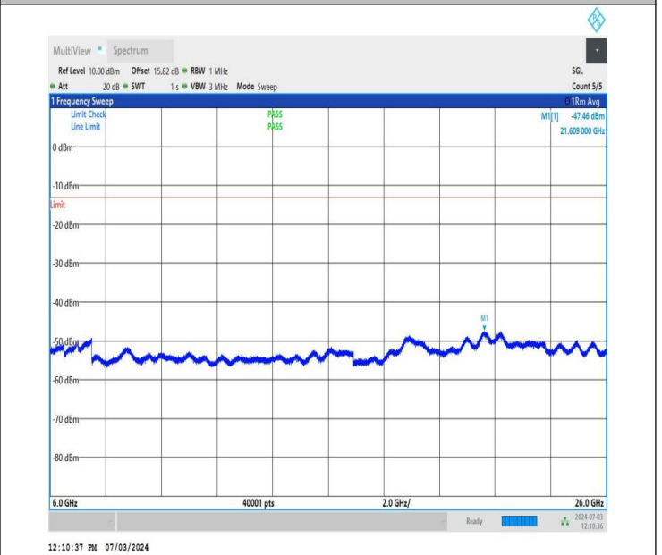
NTNV_DC_26A_n77A-3700-3980_PC2_30_5+30_M+H_TID4_N S_01_6000_26000_#1
