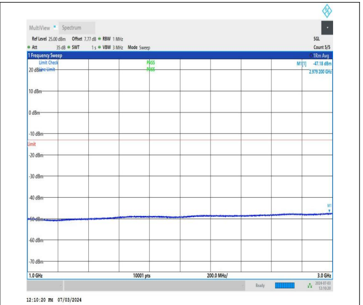
NTNV_DC_26A_n77A-3700-3980_PC2_30_5+30_M+H_TID4_N S_01_1000_3000_#1
