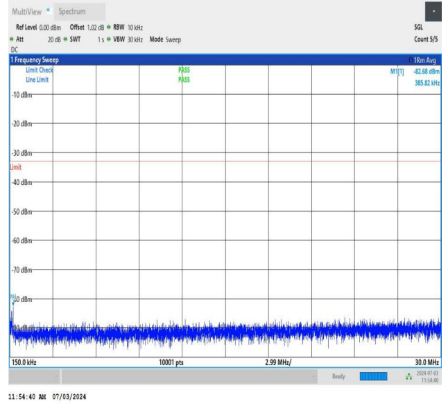
NTNV_DC_26A_n77A-3700-3980_PC2_30_5+20_M+H_TID1_N S_01_0.15_30_#1
