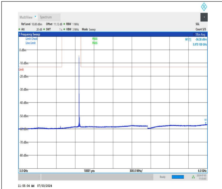
NTNV_DC_26A_n77A-3700-3980_PC2_30_5+20_M+H_TID1_N S_01_3000_6000_#1
