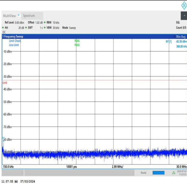
NTNV_DC_26A_n77A-3700-3980_PC2_30_5+20_M+H_TID5_N S_01_0.15_30_#1
