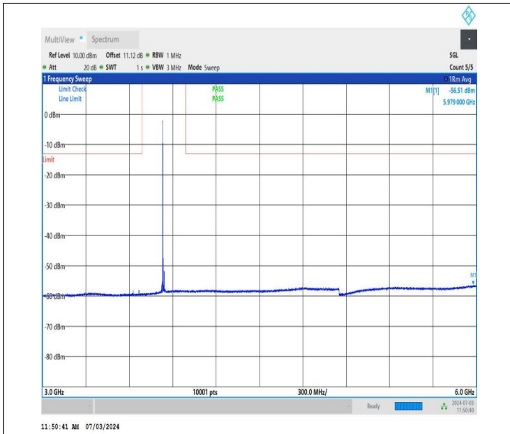
NTNV_DC_26A_n77A-3700-3980_PC2_30_5+20_M+M_TID1_N S_01_3000_6000_#1
