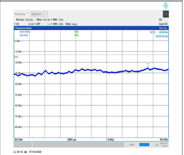
NTNV_DC_26A_n77A-3700-3980_PC2_30_5+20_M+L_TID5_NS_01_26000_40000_#1
