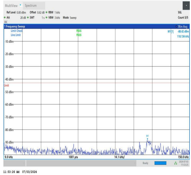
NTNV_DC_26A_n77A-3700-3980_PC2_30_5+20_M+M_TID5_N S_01_0.009_0.15_#1
