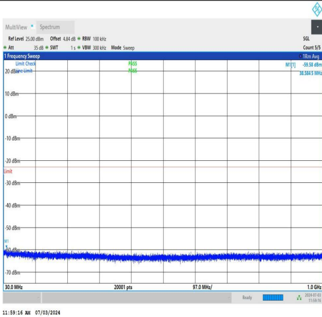
NTNV_DC_26A_n77A-3700-3980_PC2_30_5+30_M+L_TID1_NS_01_30_1000_#1
