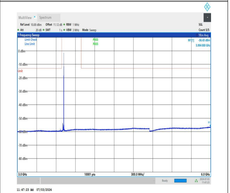
NTNV_DC_26A_n77A-3700-3980_PC2_30_5+20_M+L_TID2_NS_01_3000_6000_#1
