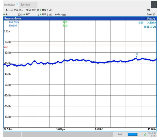
NTNV_DC_26A_n77A-3700-3980_PC2_30_5+20_M+H_TID2_N S_01_26000_40000_#1
