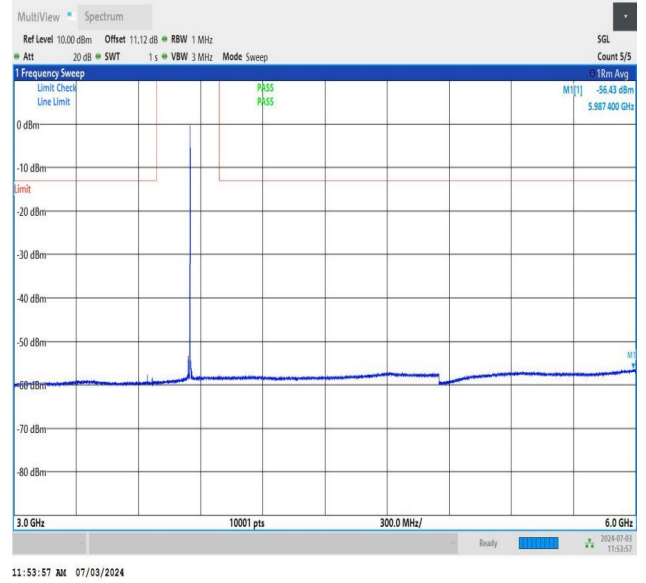
NTNV_DC_26A_n77A-3700-3980_PC2_30_5+20_M+M_TID5_N S_01_3000_6000_#1
