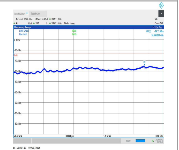
NTNV_DC_26A_n77A-3700-3980_PC2_30_5+20_M+H_TID5_N S_01_26000_40000_#1
