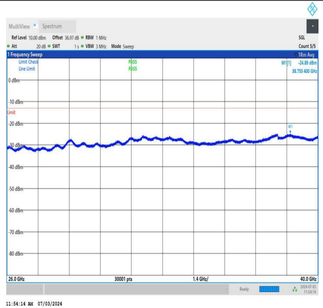
NTNV_DC_26A_n77A-3700-3980_PC2_30_5+20_M+M_TID5_N S_01_26000_40000_#1
