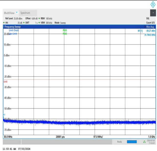
NTNV_DC_26A_n77A-3700-3980_PC2_30_5+20_M+M_TID5_N S_01_30_1000_#1
