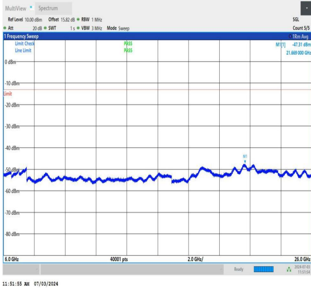
NTNV_DC_26A_n77A-3700-3980_PC2_30_5+20_M+M_TID2_N S_01_6000_26000_#1
