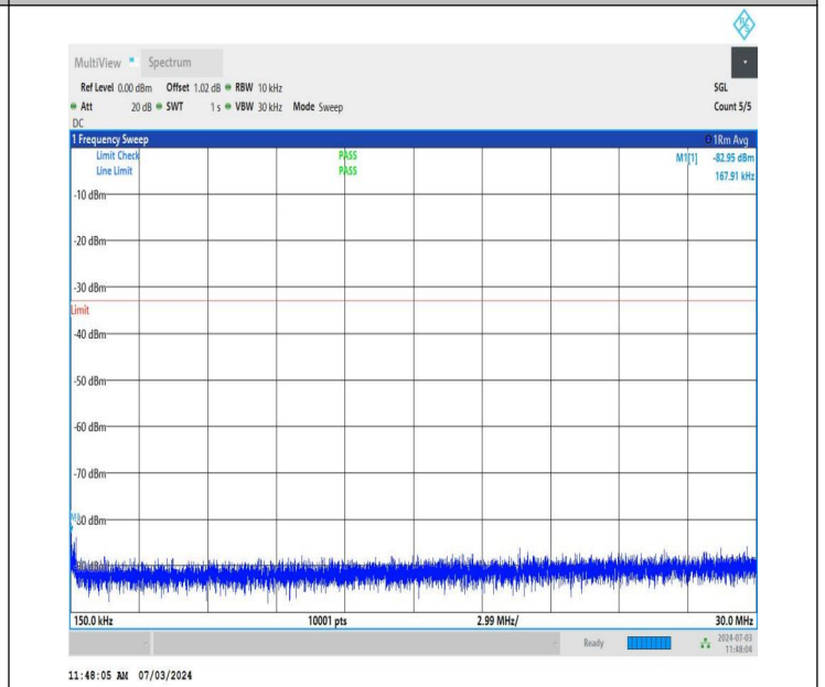
NTNV_DC_26A_n77A-3700-3980_PC2_30_5+20_M+L_TID4_NS_01_0.15_30_#1
