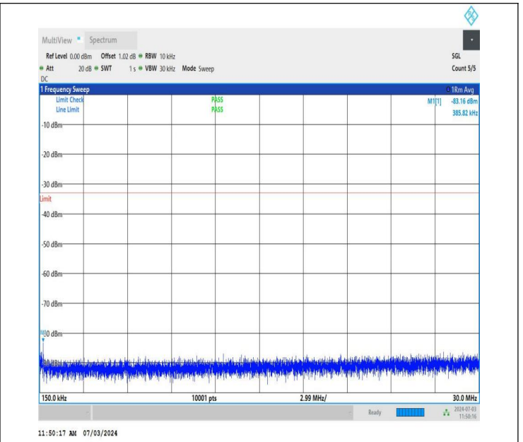
NTNV_DC_26A_n77A-3700-3980_PC2_30_5+20_M+M_TID1_N S_01_0.15_30_#1
