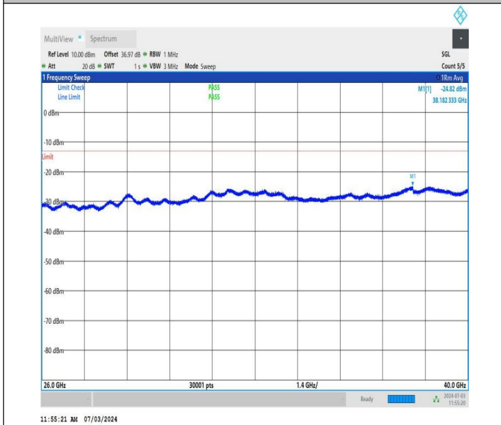
NTNV_DC_26A_n77A-3700-3980_PC2_30_5+20_M+H_TID1_N S_01_26000_40000_#1
