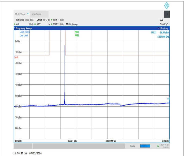
NTNV_DC_26A_n77A-3700-3980_PC2_30_5+20_M+H_TID5_N S_01_3000_6000_#1
