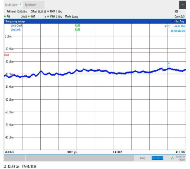
NTNV_DC_26A_n77A-3700-3980_PC2_30_5+20_M+M_TID2_N S_01_26000_40000_#1
