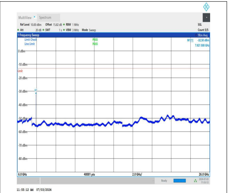
NTNV_DC_26A_n77A-3700-3980_PC2_30_5+20_M+H_TID1_N S_01_6000_26000_#1
