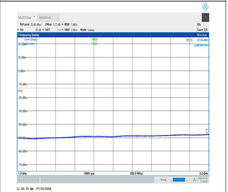
NTNV_DC_26A_n77A-3700-3980_PC2_30_5+20_M+M_TID1_N S_01_1000_3000_#1
