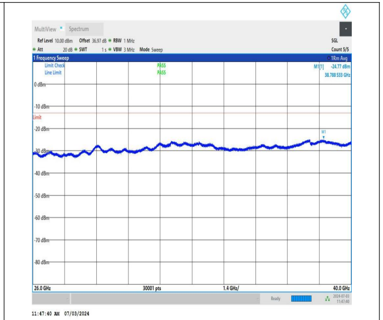
NTNV_DC_26A_n77A-3700-3980_PC2_30_5+20_M+L_TID2_NS_01_26000_40000_#1
