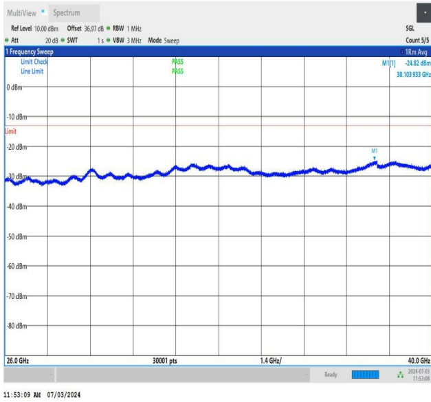
NTNV_DC_26A_n77A-3700-3980_PC2_30_5+20_M+M_TID4_N S_01_26000_40000_#1
