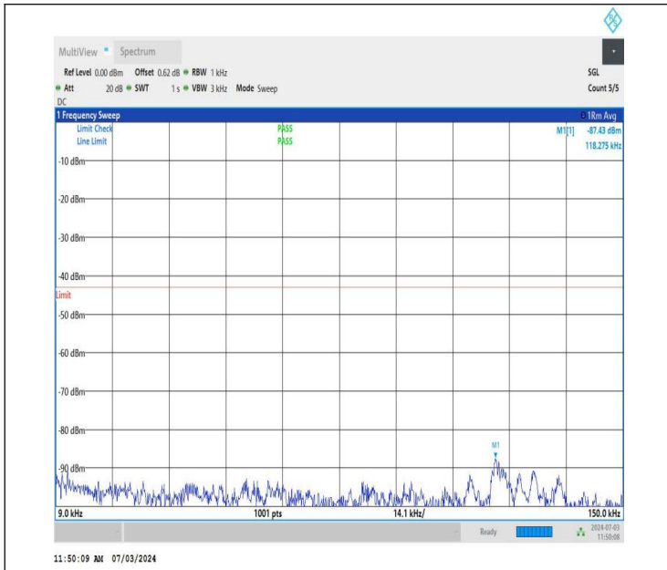
NTNV_DC_26A_n77A-3700-3980_PC2_30_5+20_M+M_TID1_N S_01_0.009_0.15_#1
