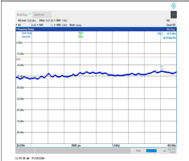
NTNV_DC_26A_n77A-3700-3980_PC2_30_5+20_M+M_TID1_N S_01_26000_40000_#1
