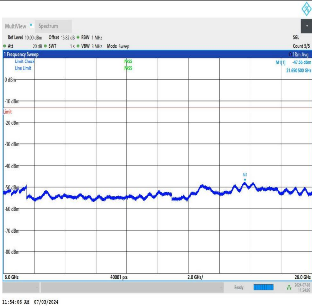
NTNV_DC_26A_n77A-3700-3980_PC2_30_5+20_M+M_TID5_N S_01_6000_26000_#1
