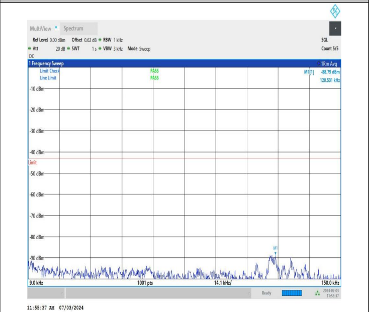
NTNV_DC_26A_n77A-3700-3980_PC2_30_5+20_M+H_TID2_N S_01_0.009_0.15_#1
