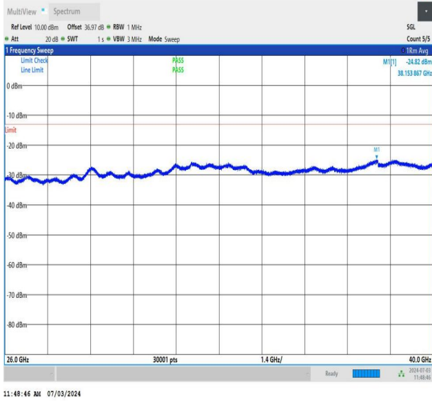
NTNV_DC_26A_n77A-3700-3980_PC2_30_5+20_M+L_TID4_NS_01_26000_40000_#1
