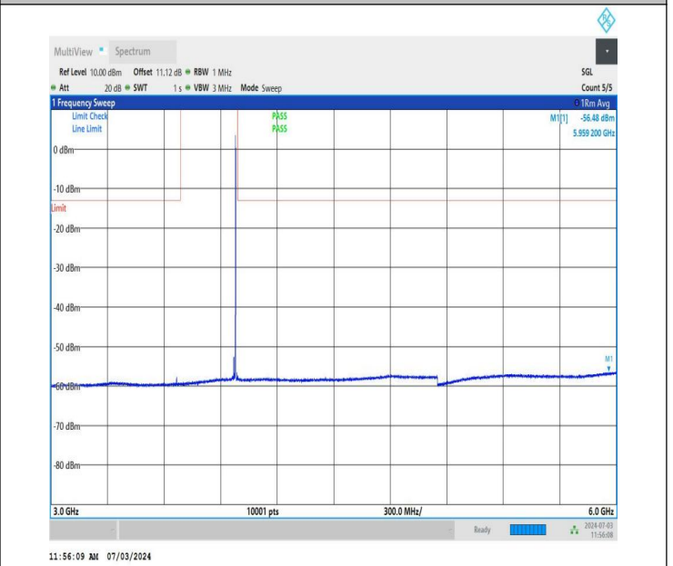
NTNV_DC_26A_n77A-3700-3980_PC2_30_5+20_M+H_TID2_N S_01_3000_6000_#1
