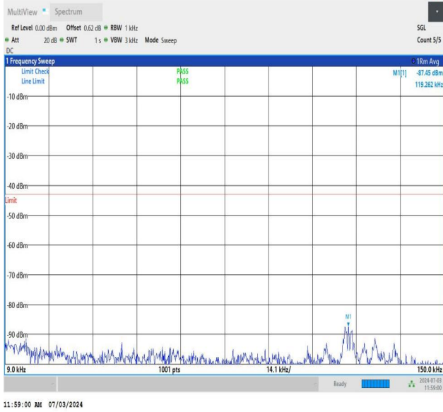
NTNV_DC_26A_n77A-3700-3980_PC2_30_5+30_M+L_TID1_NS_01_0.009_0.15_#1
