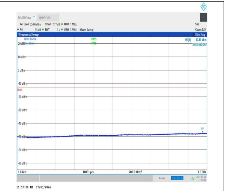
NTNV_DC_26A_n77A-3700-3980_PC2_30_5+20_M+H_TID4_N S_01_1000_3000_#1
