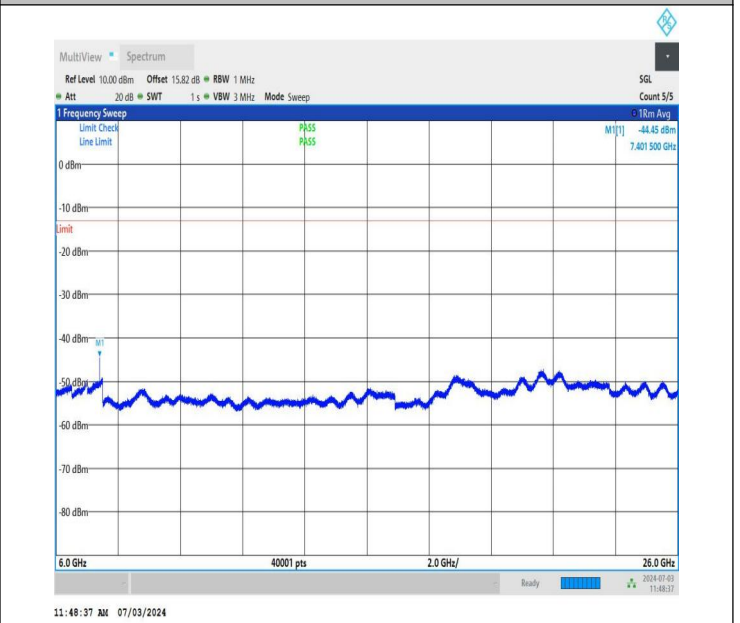
NTNV_DC_26A_n77A-3700-3980_PC2_30_5+20_M+L_TID4_NS_01_6000_26000_#1
