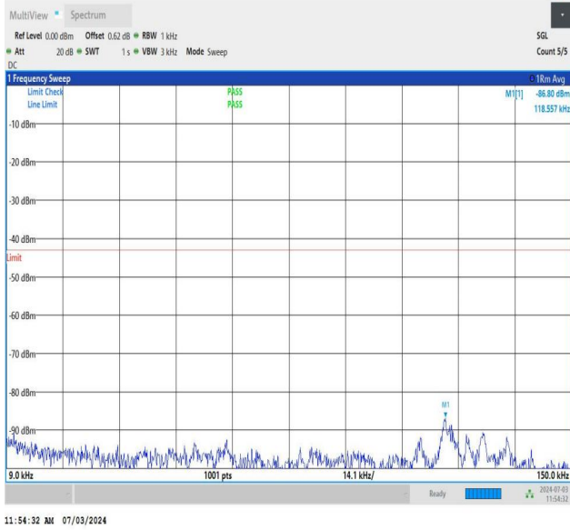
NTNV_DC_26A_n77A-3700-3980_PC2_30_5+20_M+H_TID1_N S_01_0.009_0.15_#1
