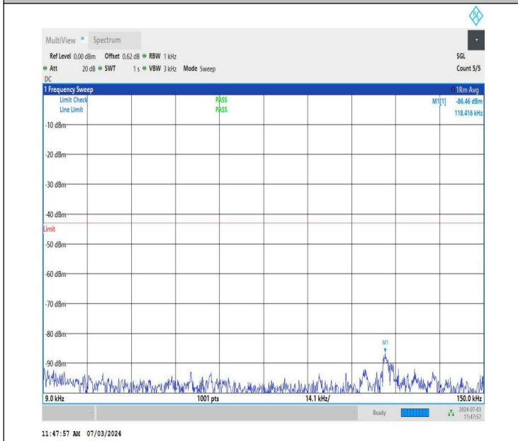
NTNV_DC_26A_n77A-3700-3980_PC2_30_5+20_M+L_TID4_NS_01_0.009_0.15_#1
