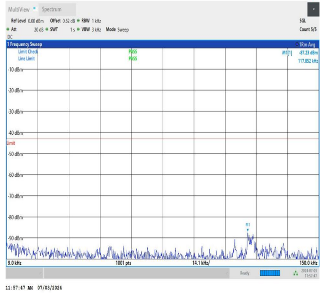
NTNV_DC_26A_n77A-3700-3980_PC2_30_5+20_M+H_TID5_N S_01_0.009_0.15_#1
