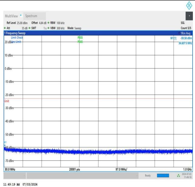
NTNV_DC_26A_n77A-3700-3980_PC2_30_5+20_M+L_TID5_NS_01_30_1000_#1
