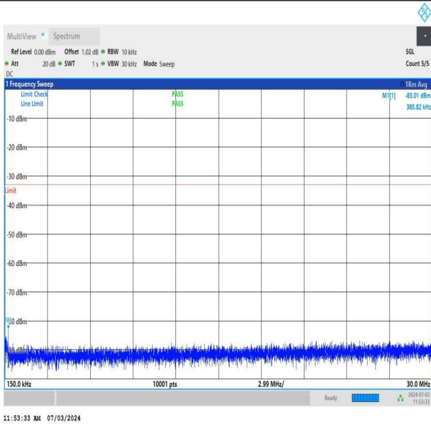
NTNV_DC_26A_n77A-3700-3980_PC2_30_5+20_M+M_TID5_N S_01_0.15_30_#1
