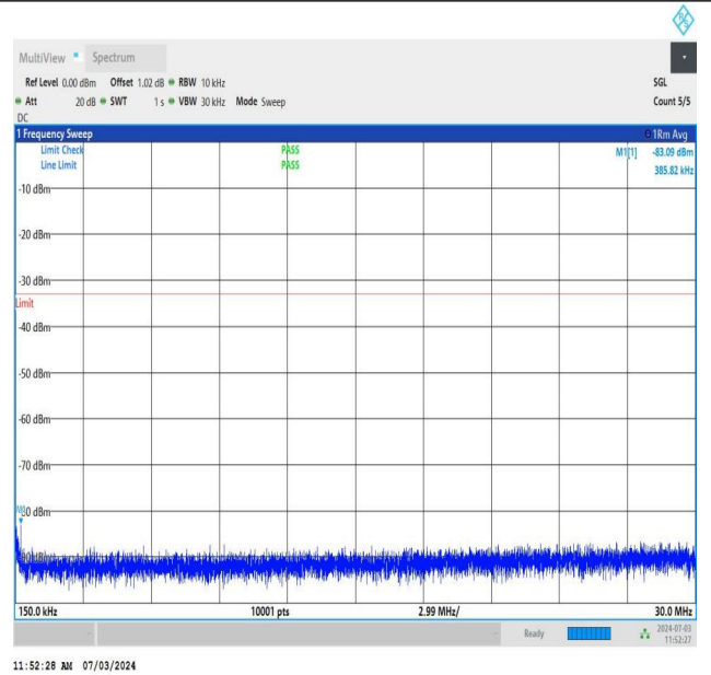
NTNV_DC_26A_n77A-3700-3980_PC2_30_5+20_M+M_TID4_N S_01_0.15_30_#1
