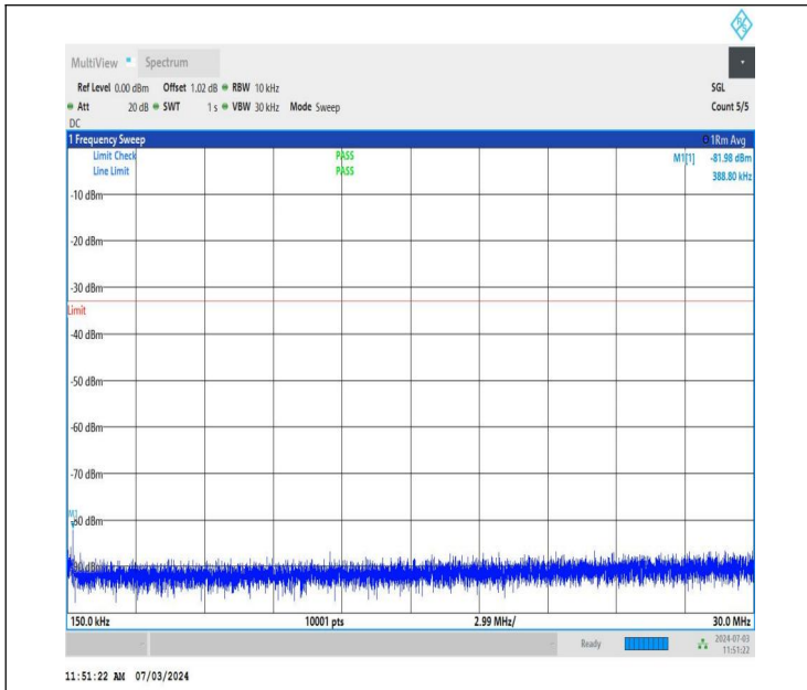
NTNV_DC_26A_n77A-3700-3980_PC2_30_5+20_M+M_TID2_N S_01_0.15_30_#1
