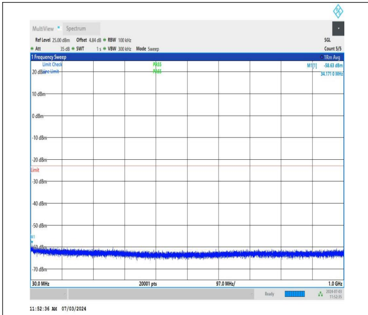
NTNV_DC_26A_n77A-3700-3980_PC2_30_5+20_M+M_TID4_N S_01_30_1000_#1
