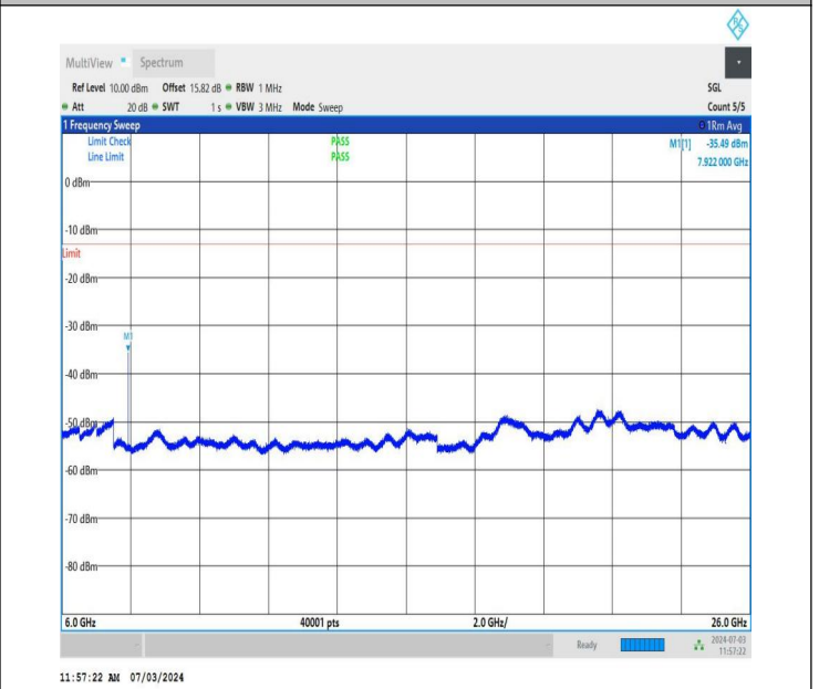
NTNV_DC_26A_n77A-3700-3980_PC2_30_5+20_M+H_TID4_N S_01_6000_26000_#1
