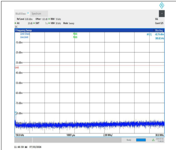
NTNV_DC_26A_n77A-3700-3980_PC2_30_5+20_M+L_TID2_NS_01_0.15_30_#1
