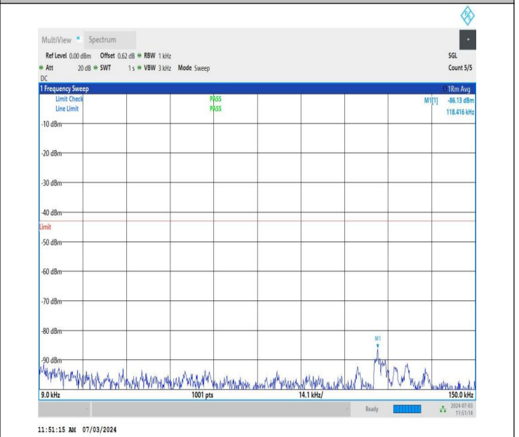
NTNV_DC_26A_n77A-3700-3980_PC2_30_5+20_M+M_TID2_N S_01_0.009_0.15_#1
