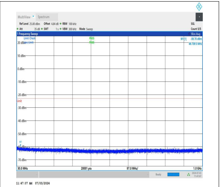
NTNV_DC_26A_n77A-3700-3980_PC2_30_5+20_M+L_TID2_NS_01_30_1000_#1
