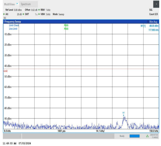
NTNV_DC_26A_n77A-3700-3980_PC2_30_5+20_M+L_TID5_NS_01_0.009_0.15_#1
