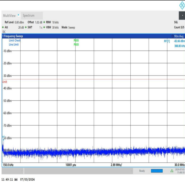
NTNV_DC_26A_n77A-3700-3980_PC2_30_5+20_M+L_TID5_NS_01_0.15_30_#1
