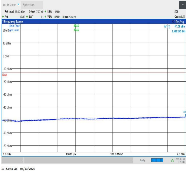
NTNV_DC_26A_n77A-3700-3980_PC2_30_5+20_M+M_TID5_N S_01_1000_3000_#1
