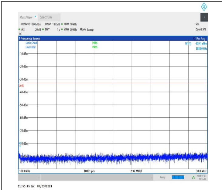
NTNV_DC_26A_n77A-3700-3980_PC2_30_5+20_M+H_TID2_N S_01_0.15_30_#1
