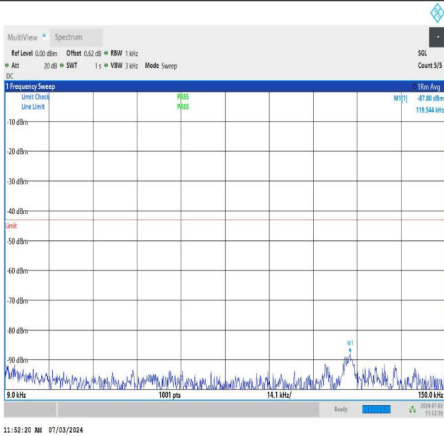
NTNV_DC_26A_n77A-3700-3980_PC2_30_5+20_M+M_TID4_N S_01_0.009_0.15_#1
