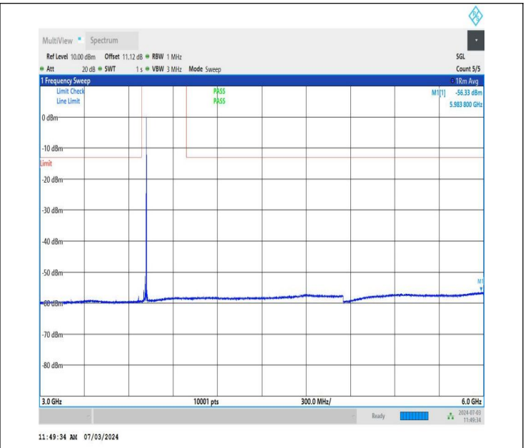
NTNV_DC_26A_n77A-3700-3980_PC2_30_5+20_M+L_TID5_NS_01_3000_6000_#1
