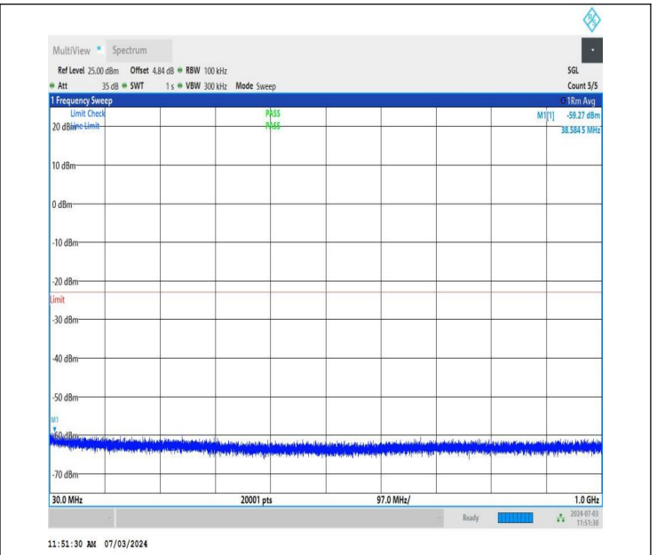
NTNV_DC_26A_n77A-3700-3980_PC2_30_5+20_M+M_TID2_N S_01_30_1000_#1
