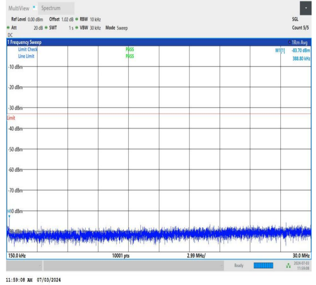
NTNV_DC_26A_n77A-3700-3980_PC2_30_5+30_M+L_TID1_NS_01_0.15_30_#1
