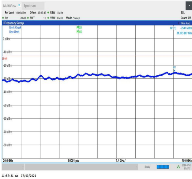
NTNV_DC_26A_n77A-3700-3980_PC2_30_5+20_M+H_TID4_N S_01_26000_40000_#1
