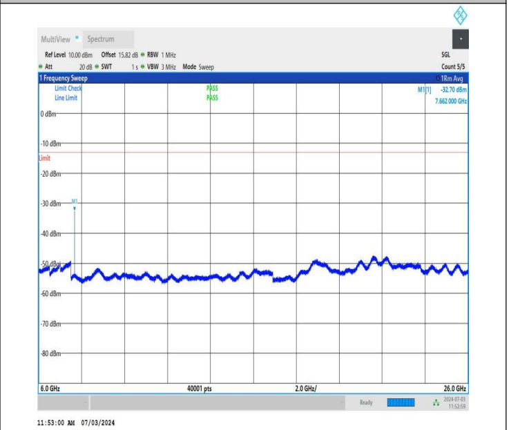
NTNV_DC_26A_n77A-3700-3980_PC2_30_5+20_M+M_TID4_N S_01_6000_26000_#1
