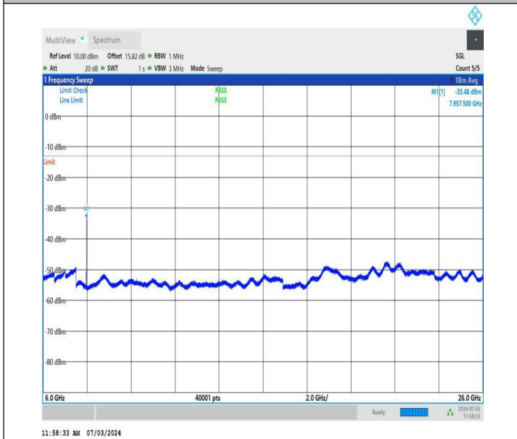
NTNV_DC_26A_n77A-3700-3980_PC2_30_5+20_M+H_TID5_N S_01_6000_26000_#1
