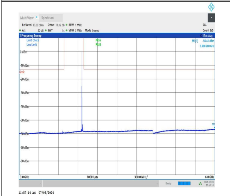
NTNV_DC_26A_n77A-3700-3980_PC2_30_5+20_M+H_TID4_N S_01_3000_6000_#1
