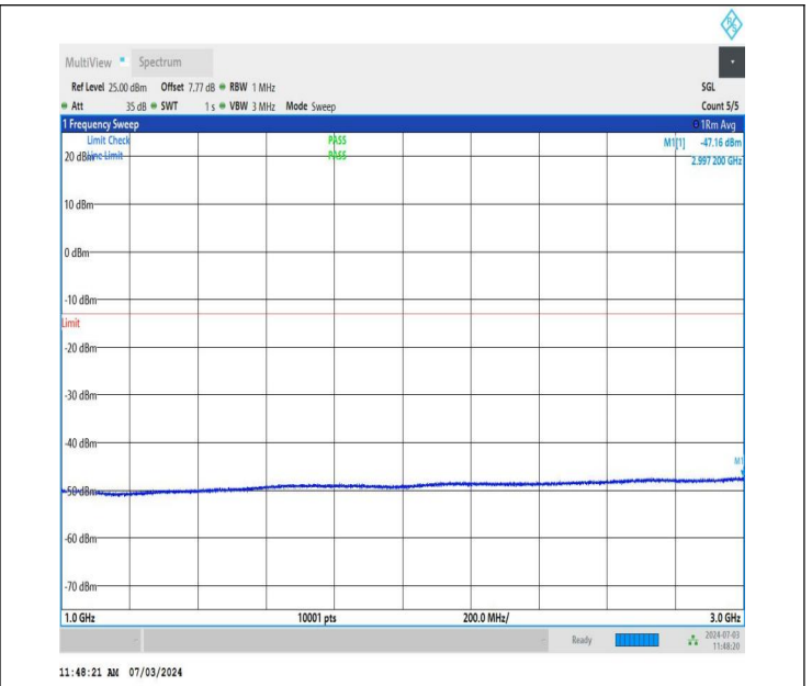
NTNV_DC_26A_n77A-3700-3980_PC2_30_5+20_M+L_TID4_NS_01_1000_3000_#1
