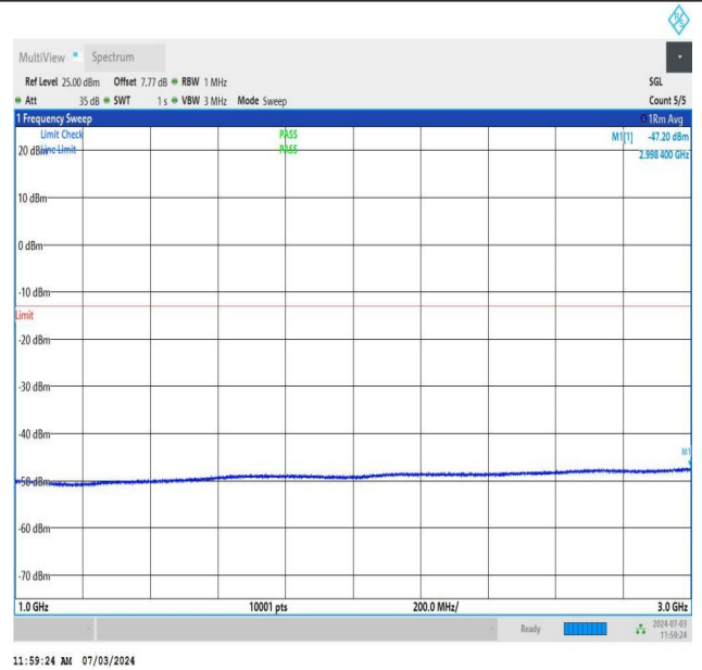
NTNV_DC_26A_n77A-3700-3980_PC2_30_5+30_M+L_TID1_NS_01_1000_3000_#1
