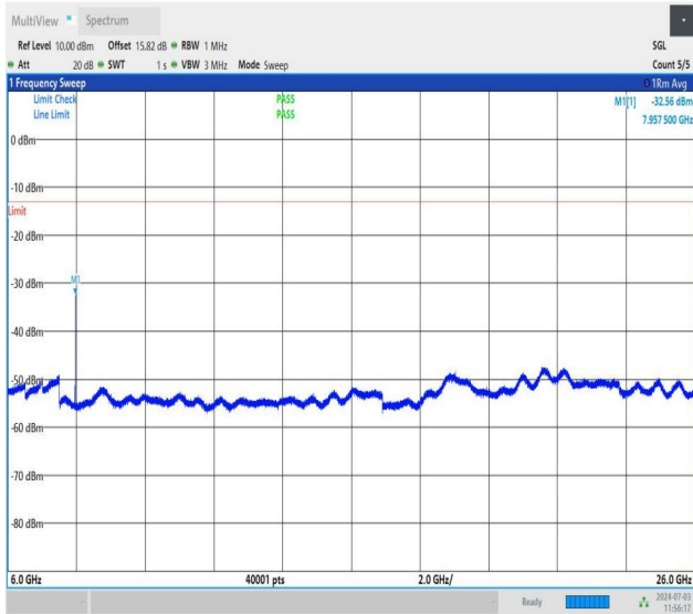
NTNV_DC_26A_n77A-3700-3980_PC2_30_5+20_M+H_TID2_N S_01_6000_26000_#1
