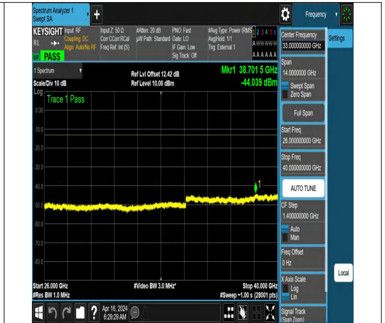
NTNV_N77-3700-3980_PC2_30_90_H_TID3_NS_01_26000_400
