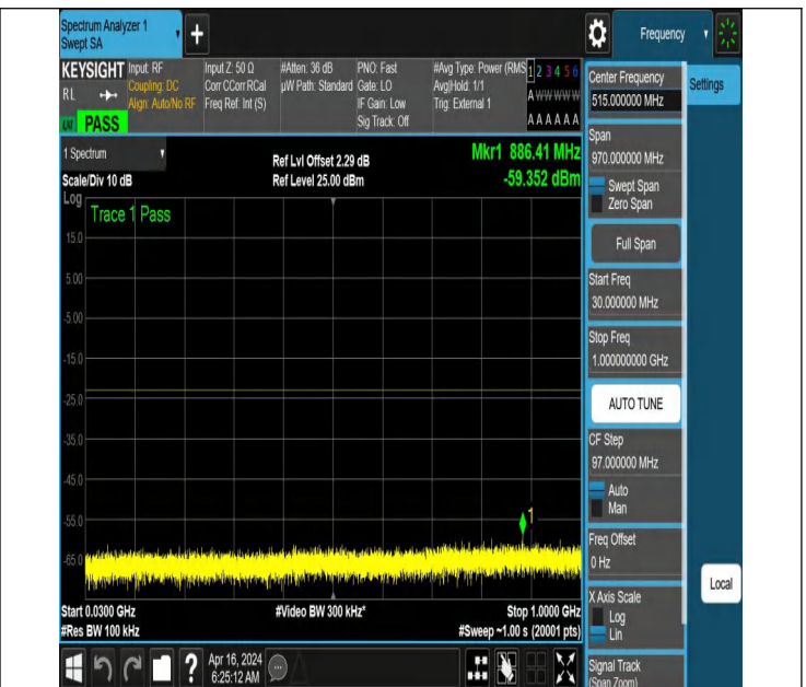
NTNV_N77-3700-3980_PC2_30_90_H_TID3_NS_01_30_1000_#
