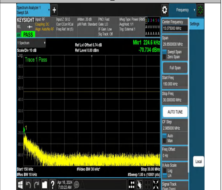
NTNV_N77-3700-3980_PC2_30_100_L_TID5_NS_01_0.15_30_#1
