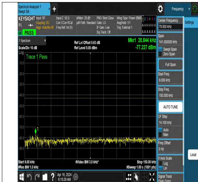
NTNV_N77-3700-3980_PC2_30_90_H_TID2_NS_01_0.009_0.15 #1
