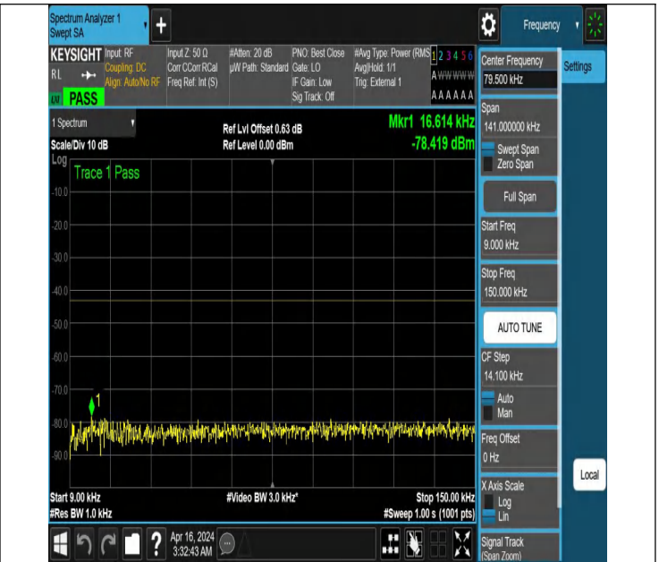
NTNV_N77-3700-3980_PC2_30_60_H_TID6_NS_01_0.009_0.15
