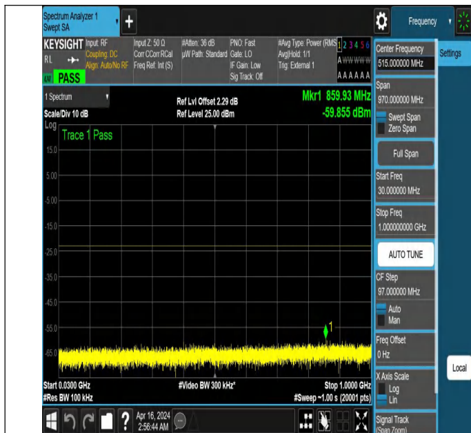
NTNV_N77-3700-3980_PC2_30_60_M_TID5_NS_01_30_1000_#1
