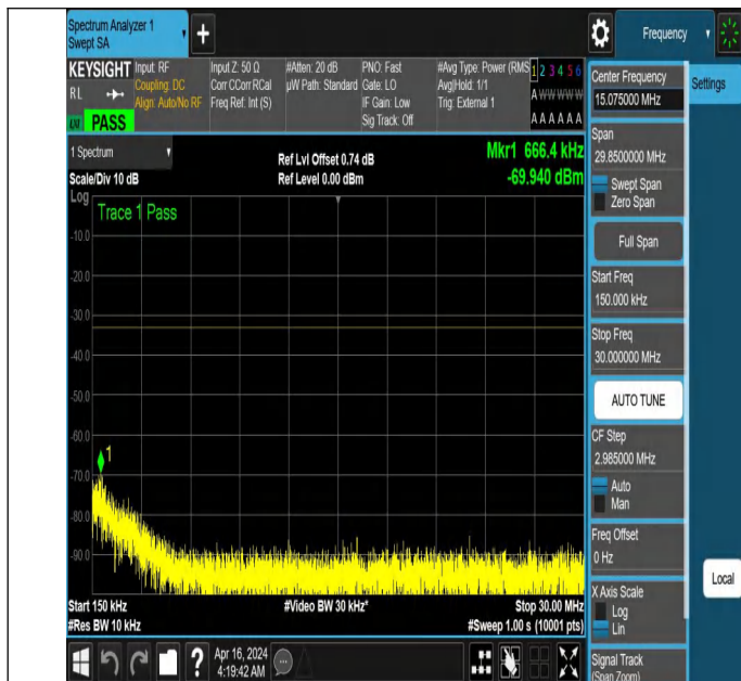
NTNV_N77-3700-3980_PC2_30_80_M_TID3_NS_01_0.15_30_#
