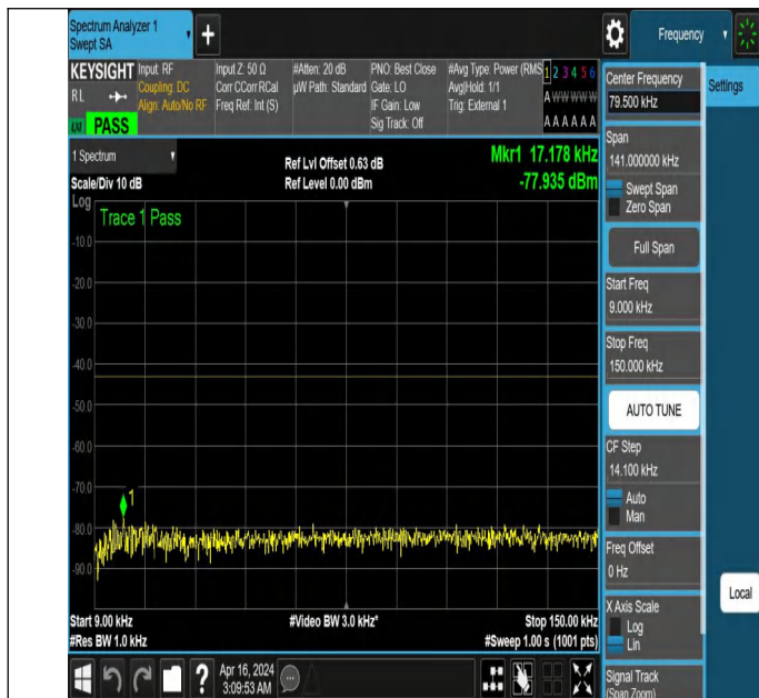
NTNV_N77-3700-3980_PC2_30_60_H_TID2_NS_01_0.009_0.15 #1
