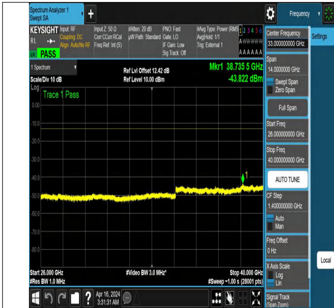
NTNV_N77-3700-3980_PC2_30_60_H_TID5_NS_01_26000_400
