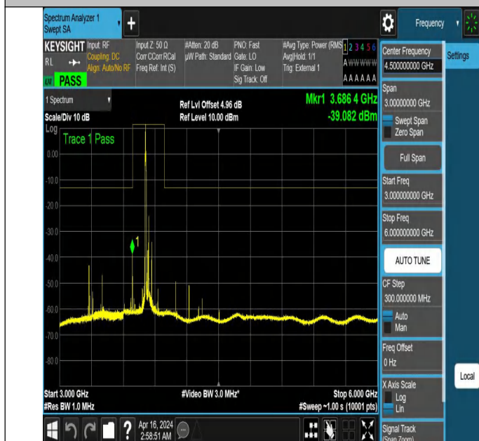
NTNV_N77-3700-3980_PC2_30_60_M_TID5_NS_01_3000_600 0 #1
