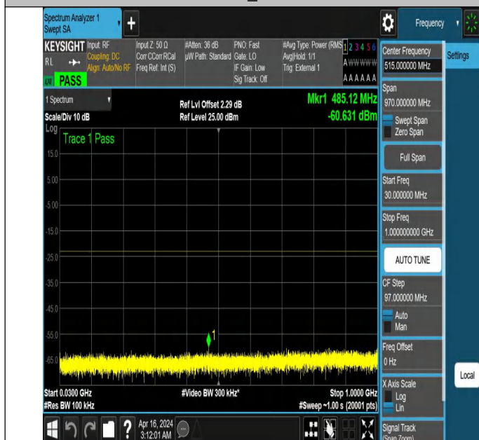
NTNV_N77-3700-3980_PC2_30_60_H_TID2_NS_01_30_1000_#
