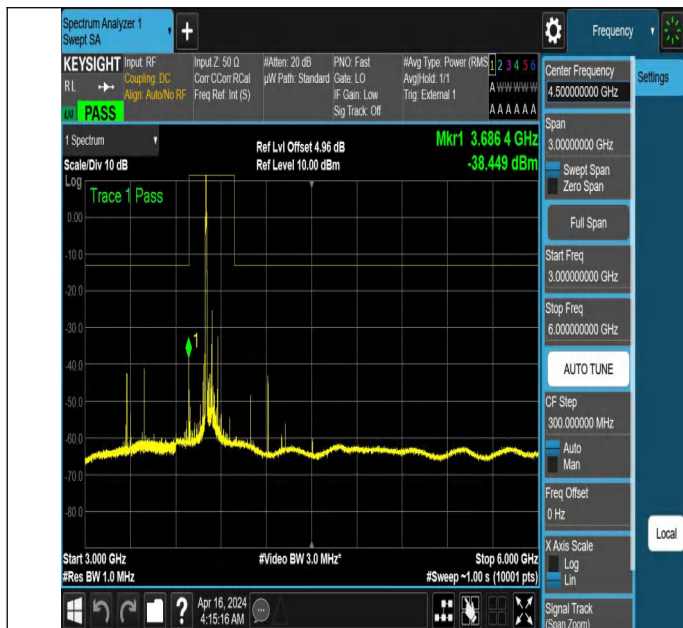
NTNV_N77-3700-3980_PC2_30_80_M_TID2_NS_01_3000_600
