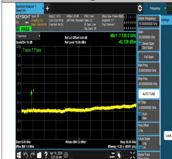
NTNV_N77-3700-3980_PC2_30_60_M_TID6_NS_01_6000_260 00 #1
