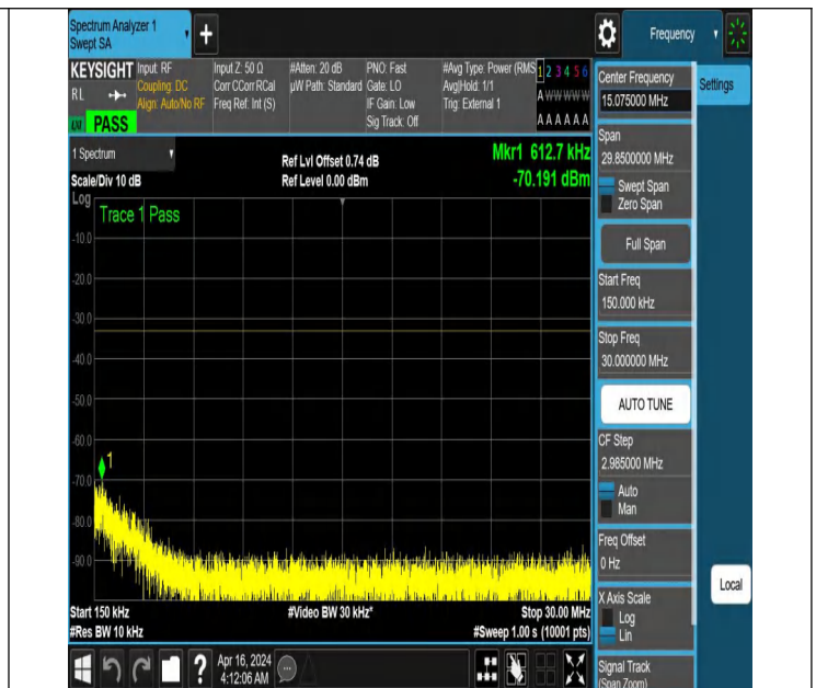
NTNV_N77-3700-3980_PC2_30_80_M_TID2_NS_01_0.15_30_#
