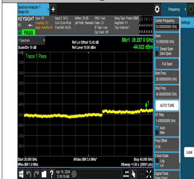
NTNV_N77-3700-3980_PC2_30_60_H_TID2_NS_01_26000_400
