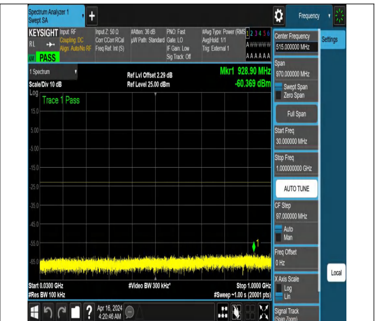
NTNV_N77-3700-3980_PC2_30_80_M_TID3_NS_01_30_1000_
