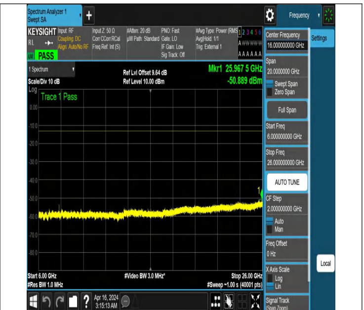
NTNV_N77-3700-3980_PC2_30_60_H_TID2_NS_01_6000_2600
