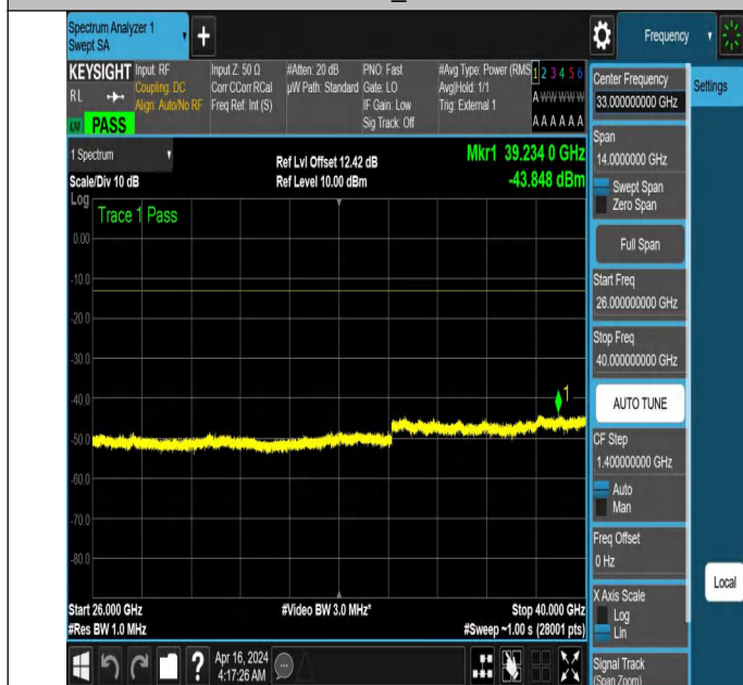
NTNV_N77-3700-3980_PC2_30_80_M_TID2_NS_01_26000_40000_#1
