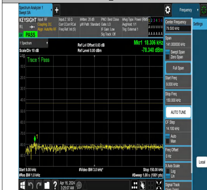
NTNV_N77-3700-3980_PC2_30_60_H_TID5_NS_01_0.009_0.15
