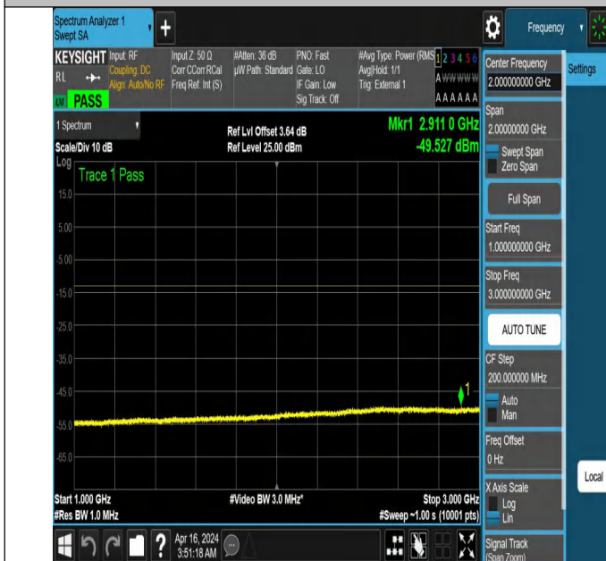
NTNV_N77-3700-3980_PC2_30_80_L_TID3_NS_01_1000_3000
