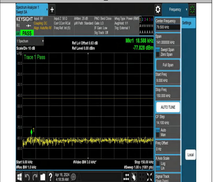
NTNV_N77-3700-3980_PC2_30_80_M_TID3_NS_01_0.009_0.1 5_#1
