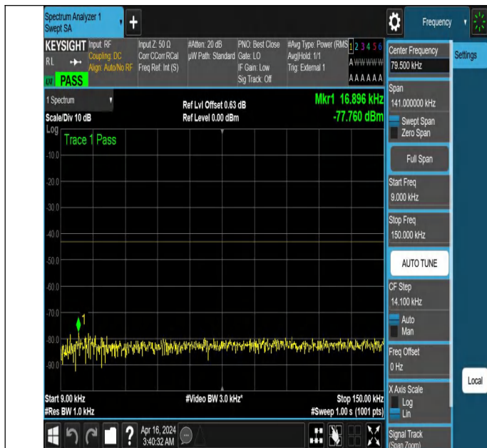
NTNV_N77-3700-3980_PC2_30_80_L_TID2_NS_01_0.009_0.15
