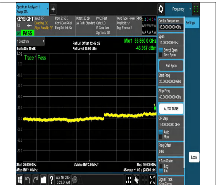
NTNV_N77-3700-3980_PC2_30_60_H_TID3_NS_01_26000_400 00 #1
