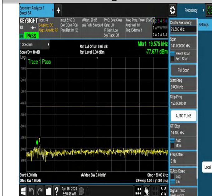
NTNV_N77-3700-3980_PC2_30_80_L_TID5_NS_01_0.009_0.15 #1
