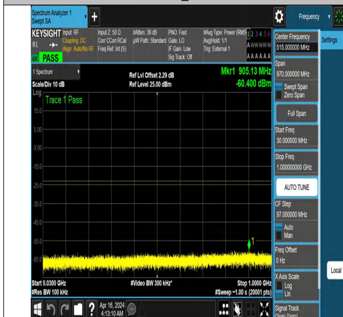
NTNV_N77-3700-3980_PC2_30_80_M_TID2_NS_01_30_1000_#1
