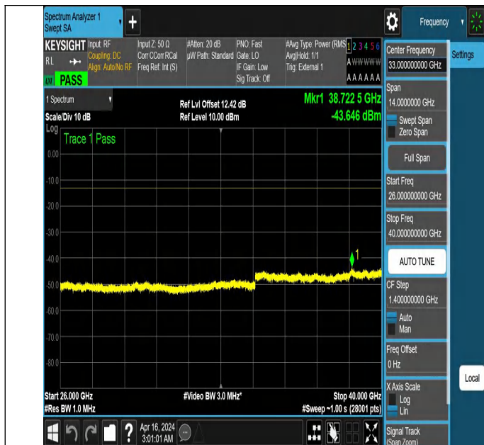
NTNV_N77-3700-3980_PC2_30_60_M_TID5_NS_01_26000_40 000 #1
