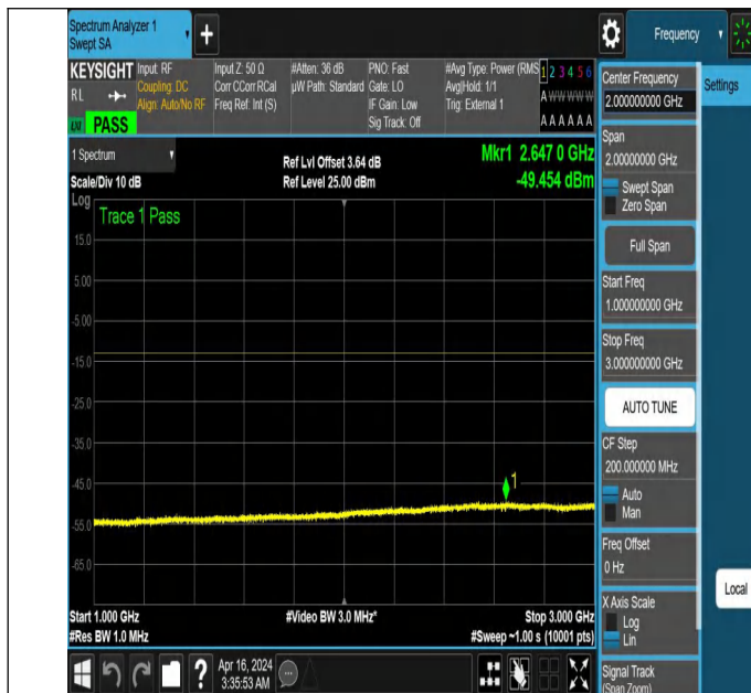
NTNV_N77-3700-3980_PC2_30_60_H_TID6 NS_01_1000_3000
