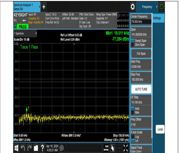
NTNV_N77-3700-3980_PC2_30_80_L_TID6_NS_01_0.009_0.15
