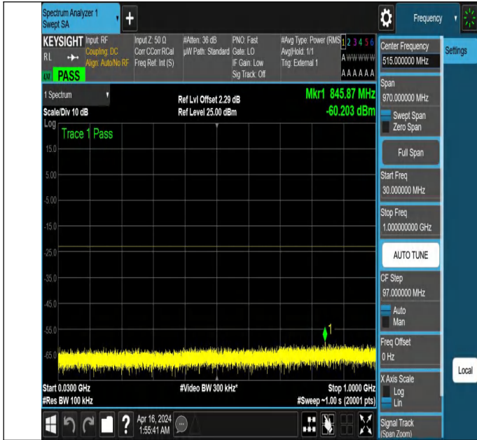
NTNV_N77-3700-3980_PC2_30_50_H_TID5_NS_01_30_1000_#
