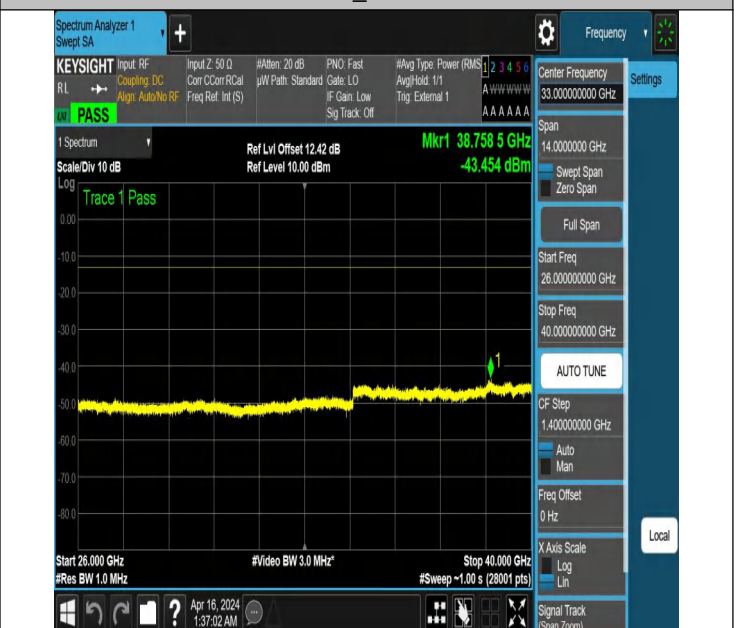
NTNV_N77-3700-3980_PC2_30_50_M_TID6_NS_01_26000_40 000 #1
