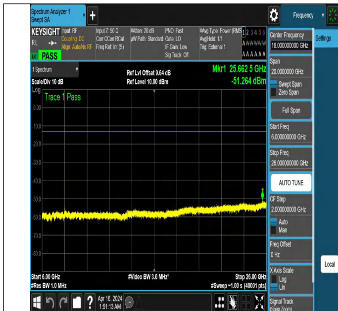
NTNV_N77-3700-3980_PC2_30_50_H_TID3_NS_01_6000_2600
