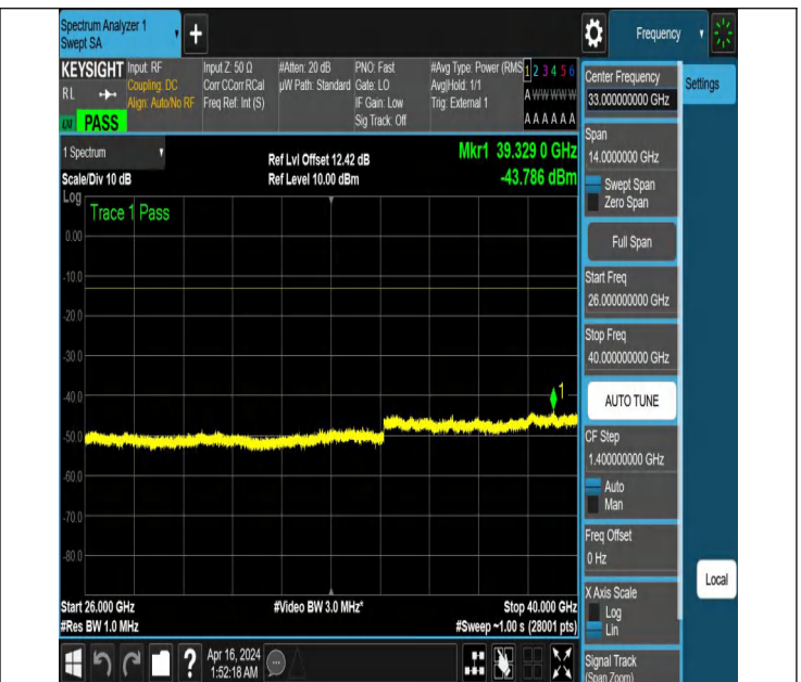
NTNV_N77-3700-3980_PC2_30_50_H_TID3_NS_01_26000_400 00 #1
