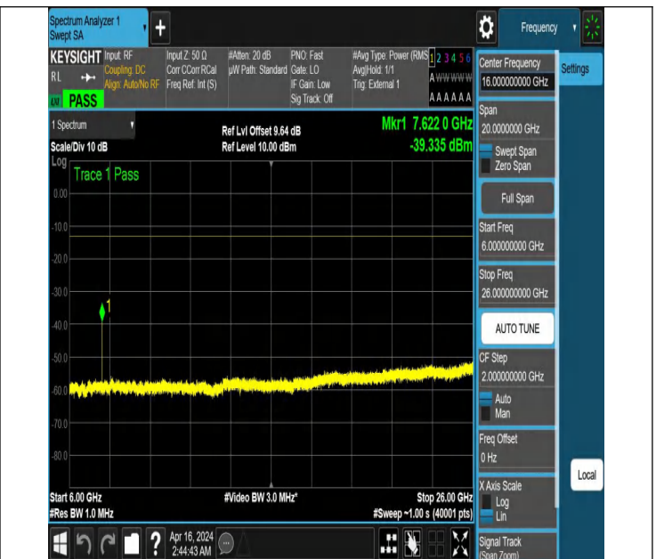
NTNV_N77-3700-3980_PC2_30_60_M_TID2_NS_01_6000_260 00 #1
