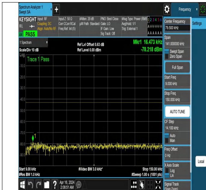
NTNV_N77-3700-3980_PC2_30_60_L_TID2_NS_01_0.009_0.15
