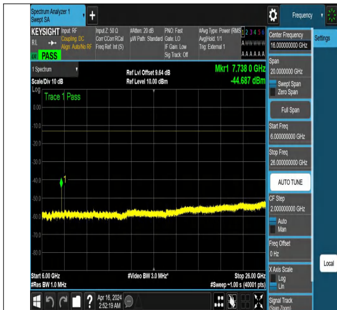
NTNV_N77-3700-3980_PC2_30_60_M_TID3_NS_01_6000_260 00 #1
