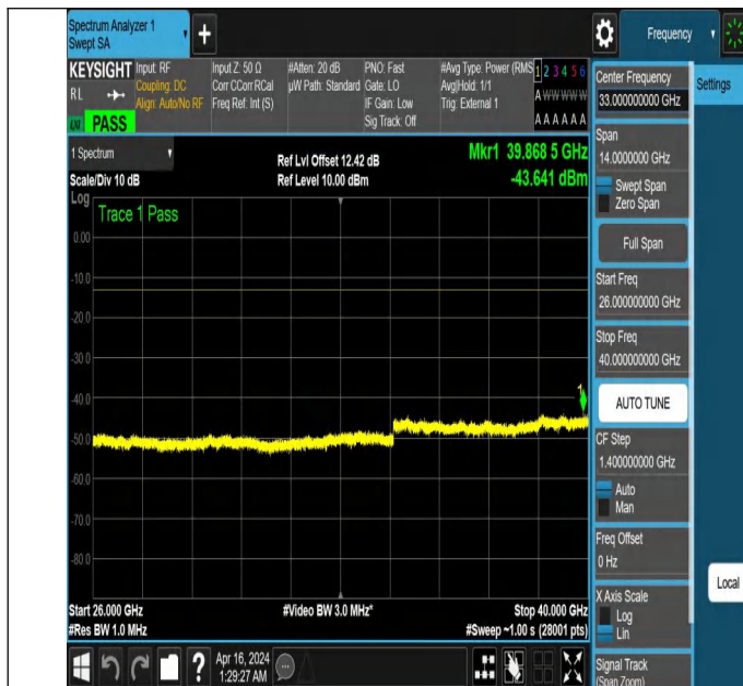
NTNV_N77-3700-3980_PC2_30_50_M_TID5_NS_01_26000_40 000 #1
