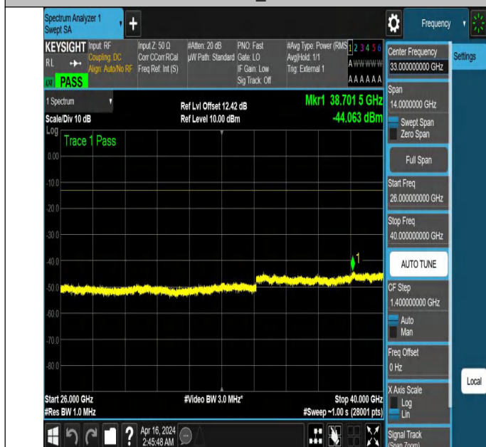
NTNV_N77-3700-3980_PC2_30_60_M_TID2_NS_01_26000_40 000 #1
