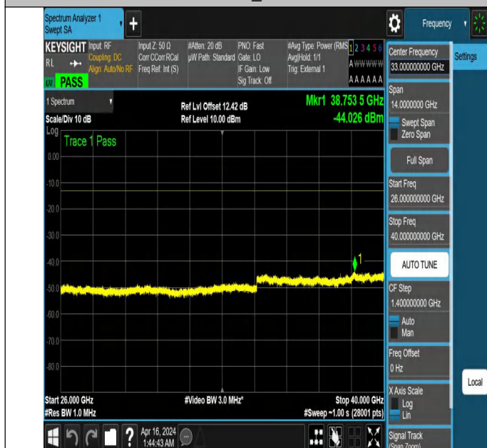
NTNV_N77-3700-3980_PC2_30_50_H_TID2_NS_01_26000_400
