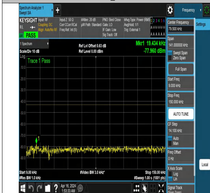
NTNV_N77-3700-3980_PC2_30_50_H_TID5_NS_01_0.009_0.15 #1
