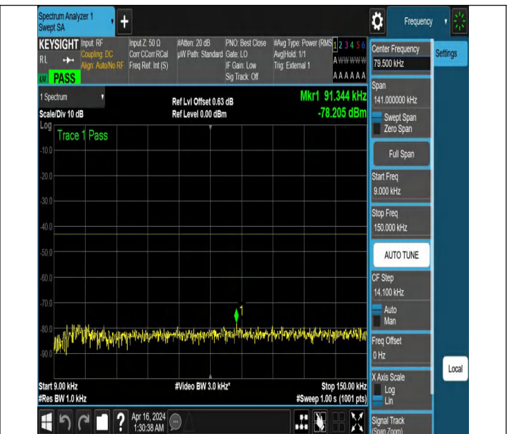
NTNV_N77-3700-3980_PC2_30_50_M_TID6_NS_01_0.009_0.1
