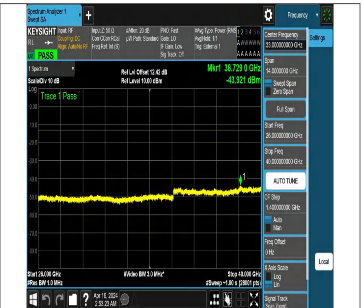
NTNV_N77-3700-3980_PC2_30_60_M_TID3_NS_01_26000_40 000 #1
