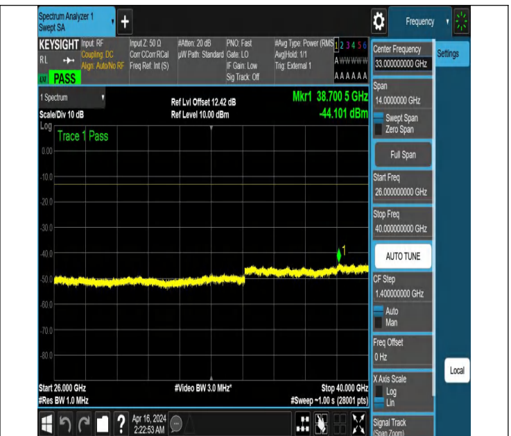
NTNV_N77-3700-3980_PC2_30_60_L_TID3_NS_01_26000_400 00 #1
