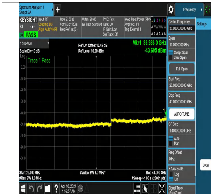
NTNV_N77-3700-3980_PC2_30_50_H_TID5_NS_01_26000_400
