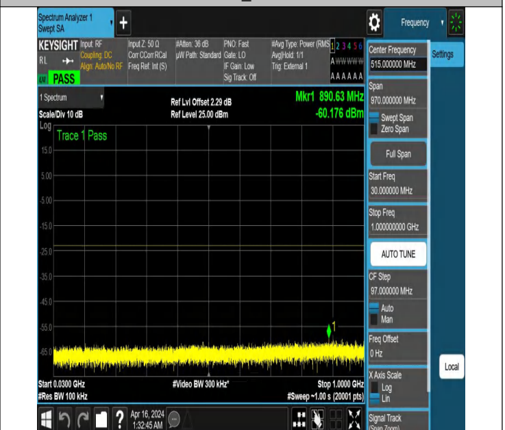
NTNV_N77-3700-3980_PC2_30_50_M_TID6_NS_01_30_1000_#1
