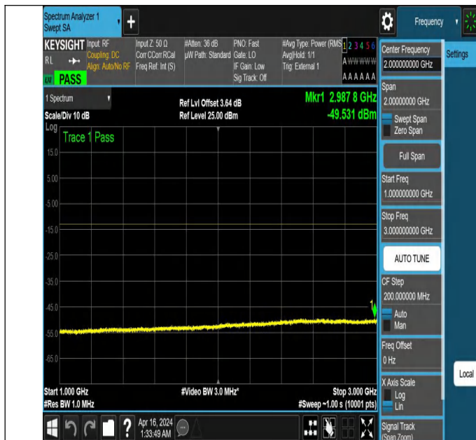
NTNV_N77-3700-3980_PC2_30_50_M_TID6_NS_01_1000_300
