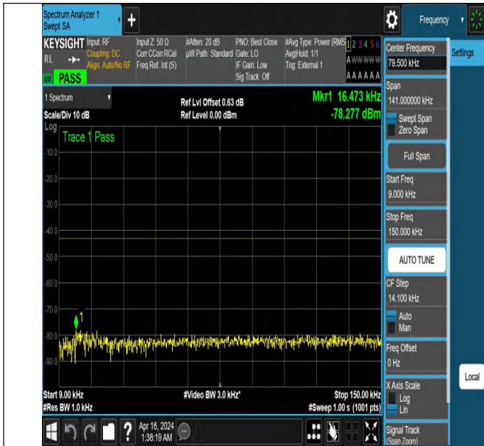
NTNV_N77-3700-3980_PC2_30_50_H_TID2_NS_01_0.009_0.15
