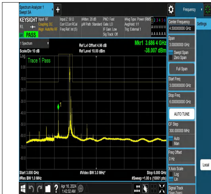
NTNV_N77-3700-3980_PC2_30_50_H_TID2_NS_01_3000_6000
