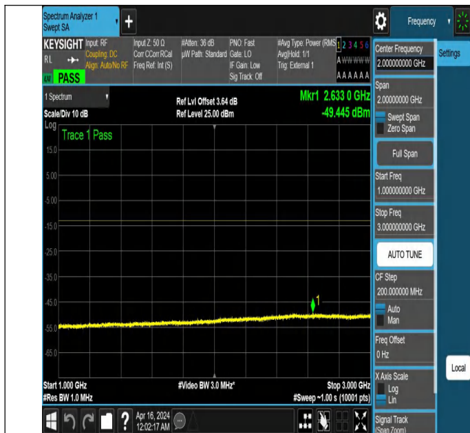
NTNV_N77-3700-3980_PC2_30_40_M_TID6_NS_01_1000_300 0 #1
