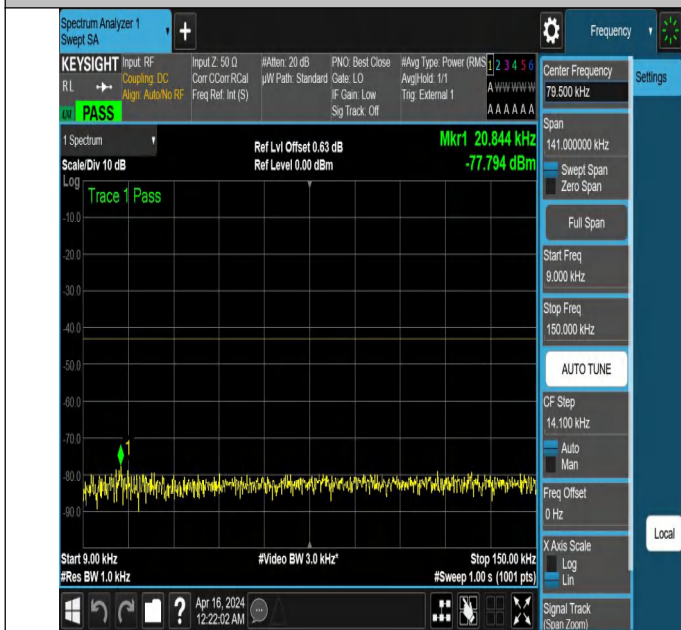
NTNV_N77-3700-3980_PC2_30_40_H_TID5_NS_01_0.009_0.15
