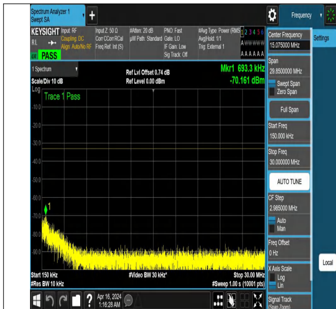
NTNV_N77-3700-3980_PC2_30_50_M_TID3_NS_01_0.15_30_#
