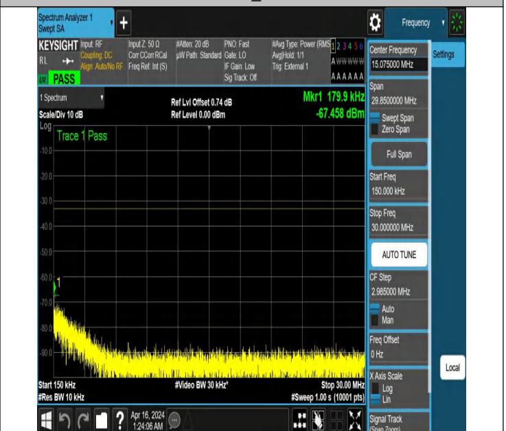
NTNV_N77-3700-3980_PC2_30_50_M_TID5_NS_01_0.15_30_#
