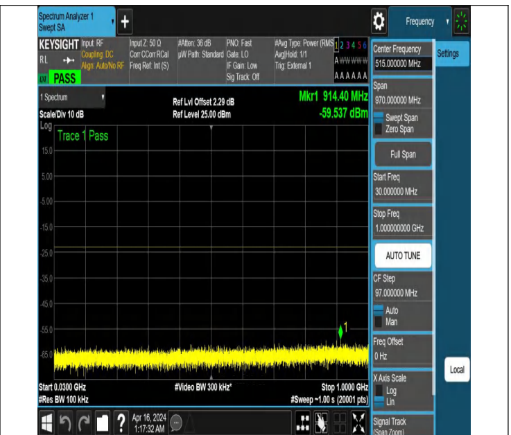
NTNV_N77-3700-3980_PC2_30_50_M_TID3_NS_01_30_1000_
