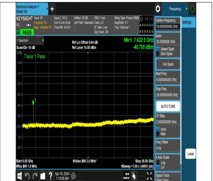
NTNV_N77-3700-3980_PC2_30_50_M_TID2_NS_01_6000_260 00 #1
