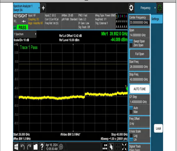
NTNV_N77-3700-3980_PC2_30_40_M_TID6_NS_01_26000_40 000 #1
