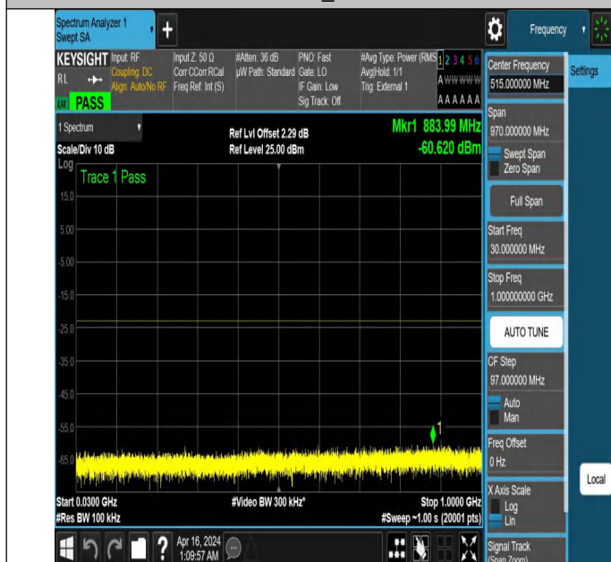
NTNV_N77-3700-3980_PC2_30_50_M_TID2_NS_01_30_1000_#1
