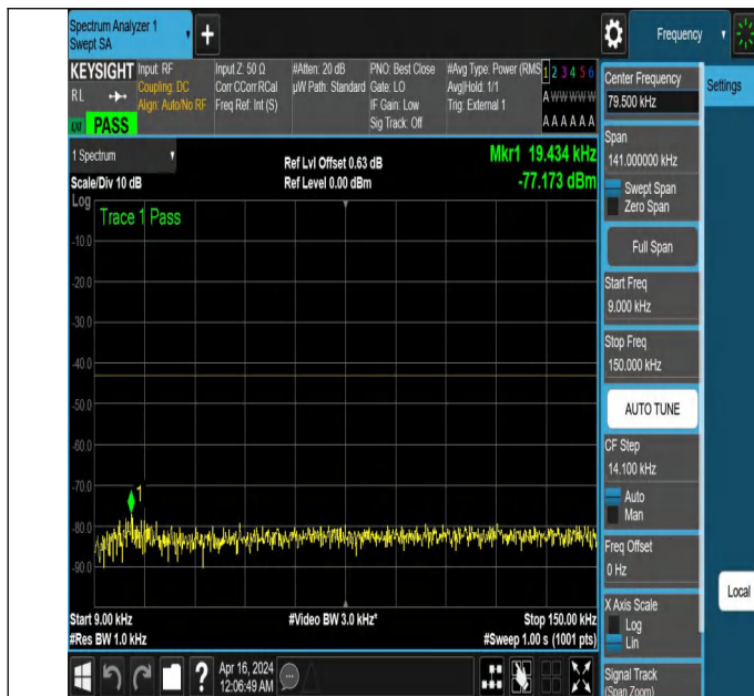
NTNV_N77-3700-3980_PC2_30_40_H_TID2_NS_01_0.009_0.15
