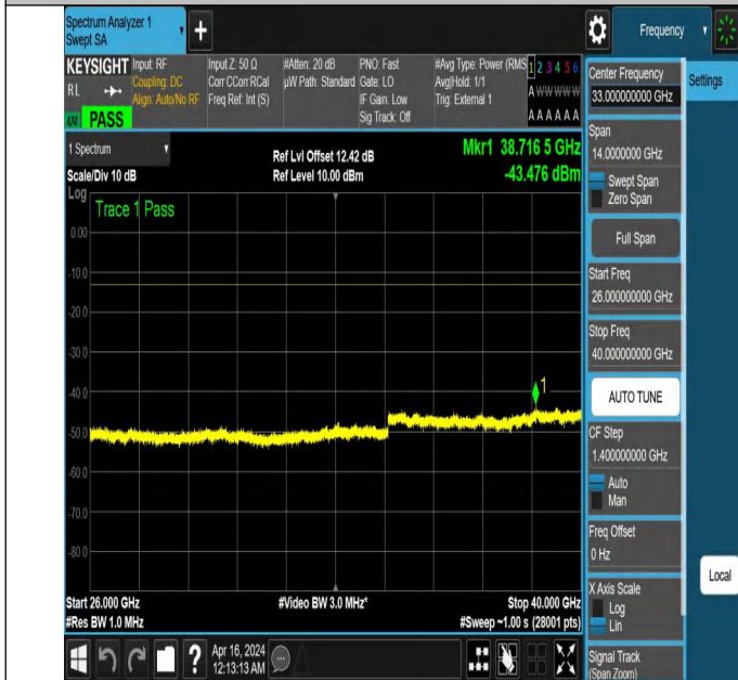
NTNV_N77-3700-3980_PC2_30_40_H_TID2_NS_01_26000_400
