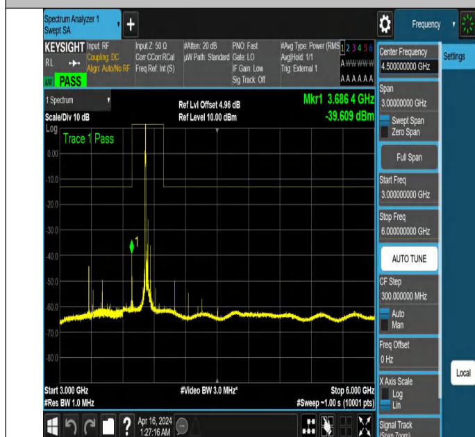
NTNV_N77-3700-3980_PC2_30_50_M_TID5_NS_01_3000_600 0 #1
