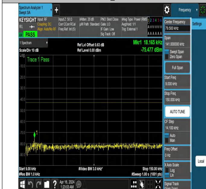
NTNV_N77-3700-3980_PC2_30_50_M_TID5_NS_01_0.009_0.1
