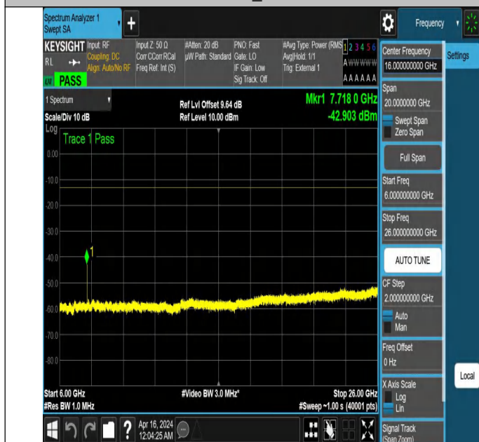
NTNV_N77-3700-3980_PC2_30_40_M_TID6_NS_01_6000_260 00 #1
