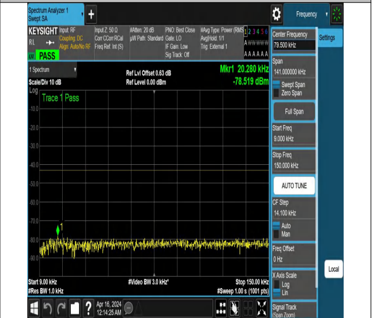
NTNV_N77-3700-3980_PC2_30_40_H_TID3_NS_01_0.009_0.15
