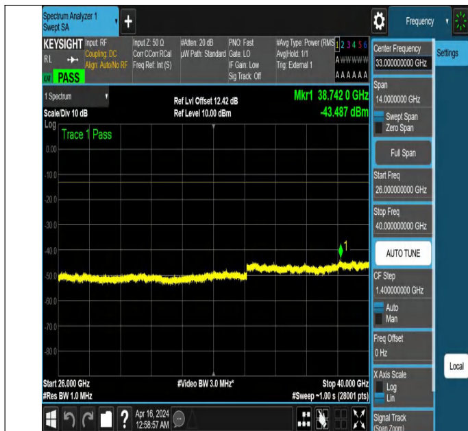
NTNV_N77-3700-3980_PC2_30_50_L_TID5_NS_01_26000_400 00 #1
