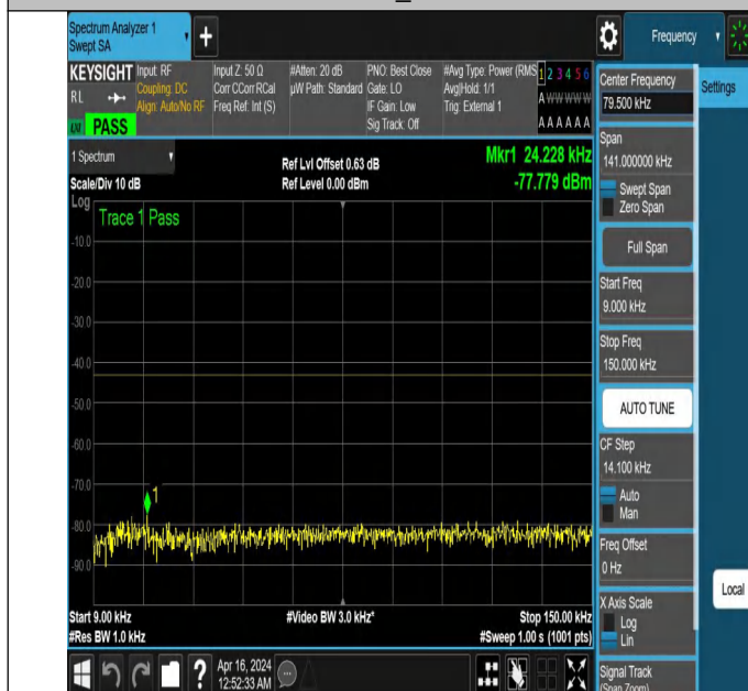
NTNV_N77-3700-3980_PC2_30_50_L_TID5_NS_01_0.009_0.15
