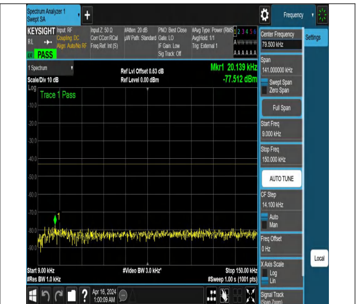
NTNV_N77-3700-3980_PC2_30_50_L_TID6_NS_01_0.009_0.15 _#1
