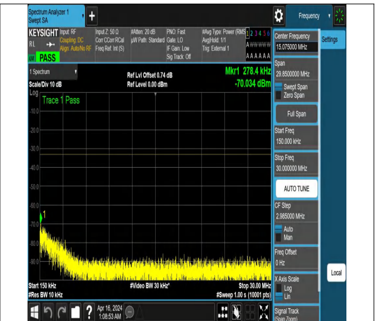
NTNV_N77-3700-3980_PC2_30_50_M_TID2_NS_01_0.15_30_#
