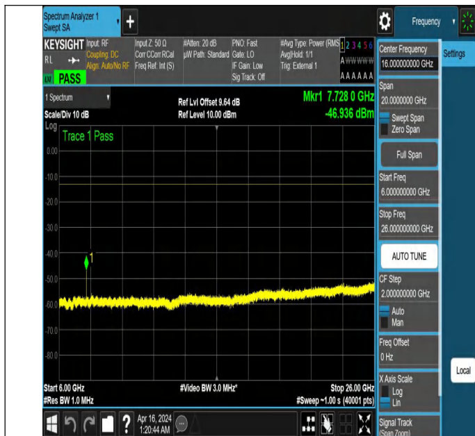
NTNV_N77-3700-3980_PC2_30_50_M_TID3_NS_01_6000_260
