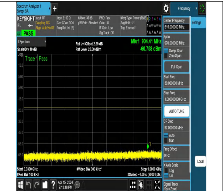
NTNV_N77-3700-3980_PC2_30_20_H_TID3_NS_01_30_1000_#
