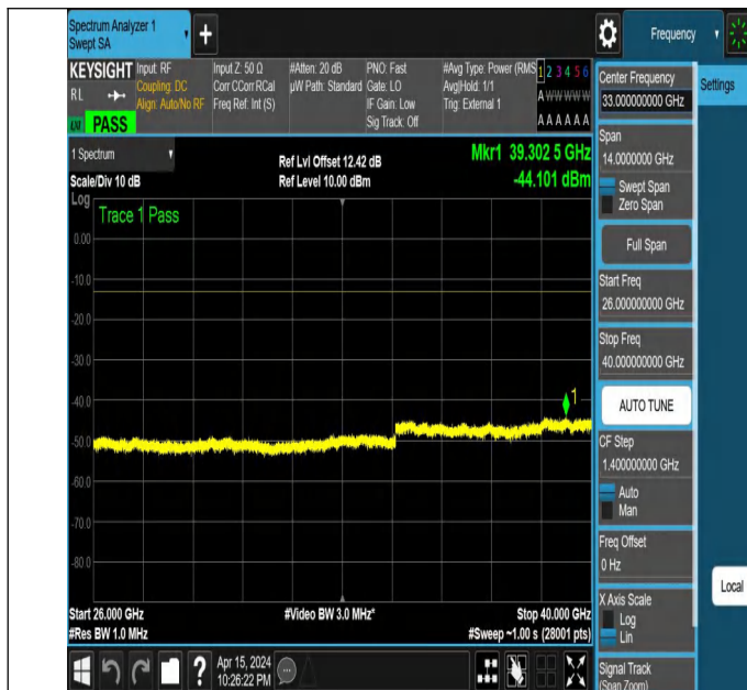
NTNV_N77-3700-3980_PC2_30_30_M_TID5_NS_01_26000_40 000 #1
