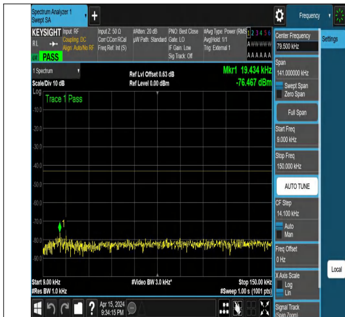
NTNV_N77-3700-3980_PC2_30_30_L_TID2_NS_01_0.009_0.15
