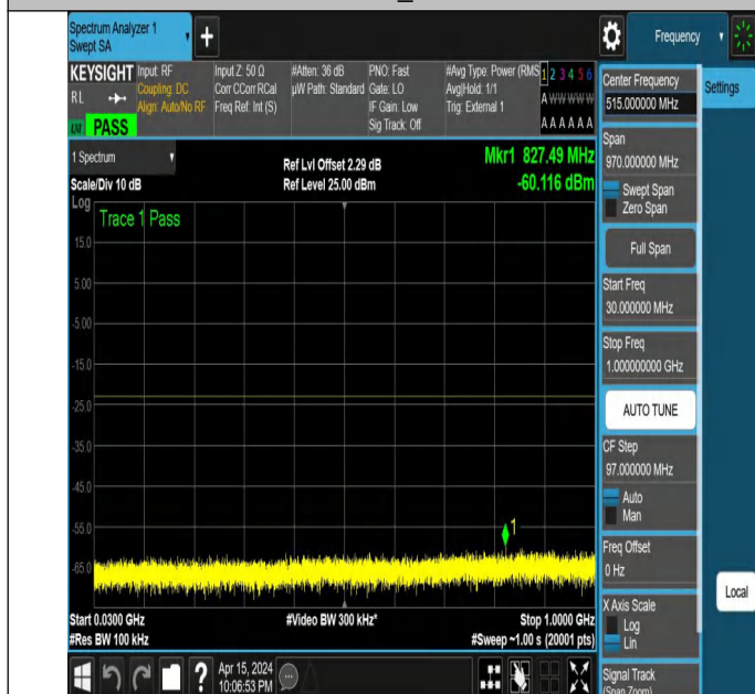
NTNV_N77-3700-3980_PC2_30_30_M_TID2_NS_01_30_1000_#1
