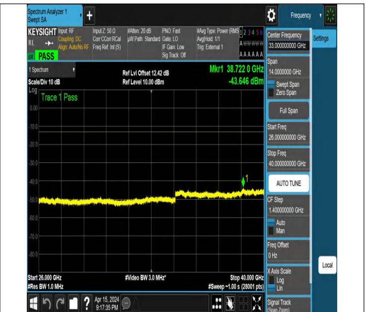
NTNV_N77-3700-3980_PC2_30_20_H_TID3_NS_01_26000_400 00 #1
