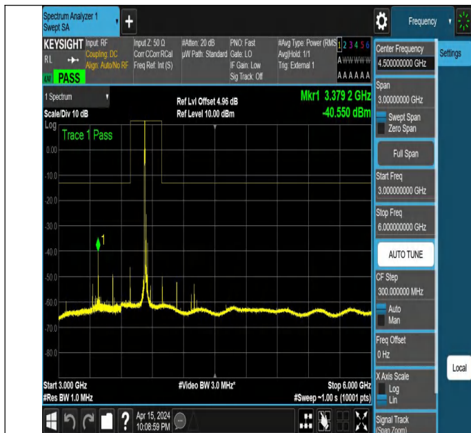
NTNV_N77-3700-3980_PC2_30_30_M_TID2_NS_01_3000_600
