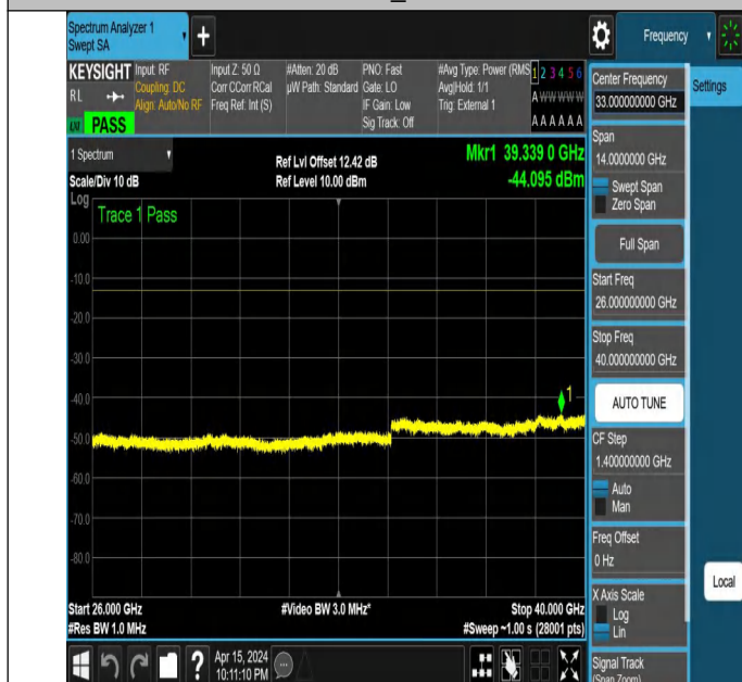
NTNV_N77-3700-3980_PC2_30_30_M_TID2_NS_01_26000_40 000 #1
