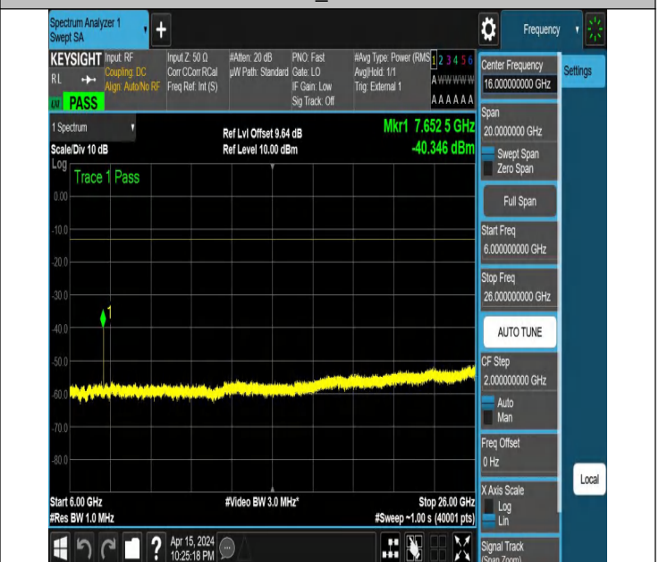
NTNV_N77-3700-3980_PC2_30_30_M_TID5_NS_01_6000_260 00 #1
