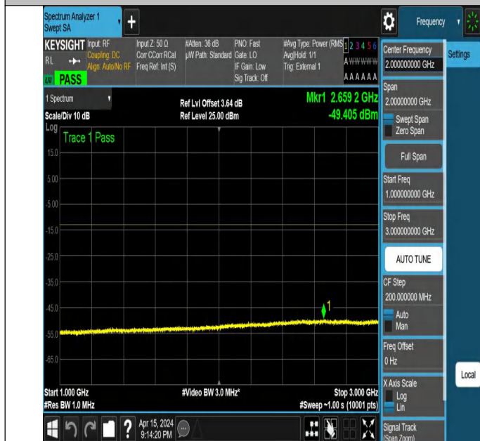
NTNV_N77-3700-3980_PC2_30_20_H_TID3_NS_01_1000_3000
