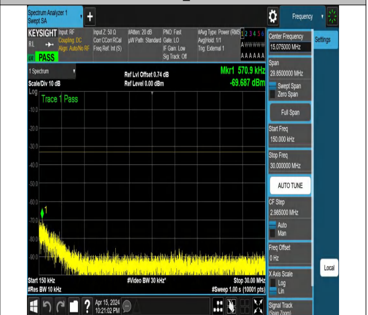
NTNV_N77-3700-3980_PC2_30_30_M_TID5_NS_01_0.15_30_#
