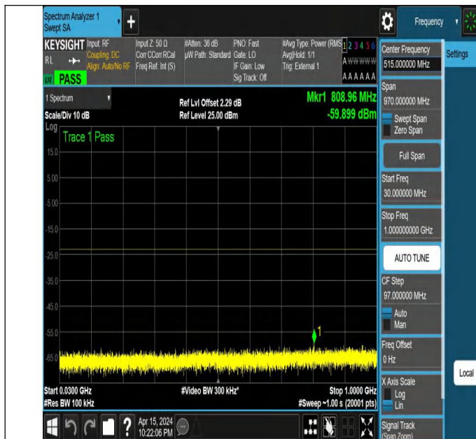
NTNV_N77-3700-3980_PC2_30_30_M_TID5_NS_01_30_1000_#1
