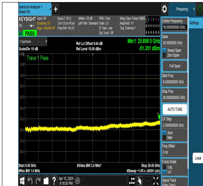
NTNV_N77-3700-3980_PC2_30_20_H_TID3_NS_01_6000_2600
