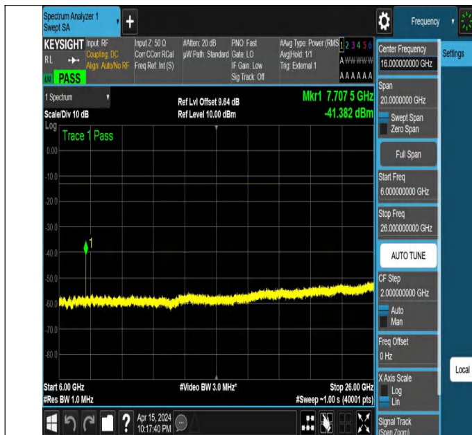
NTNV_N77-3700-3980_PC2_30_30_M_TID3_NS_01_6000_260
