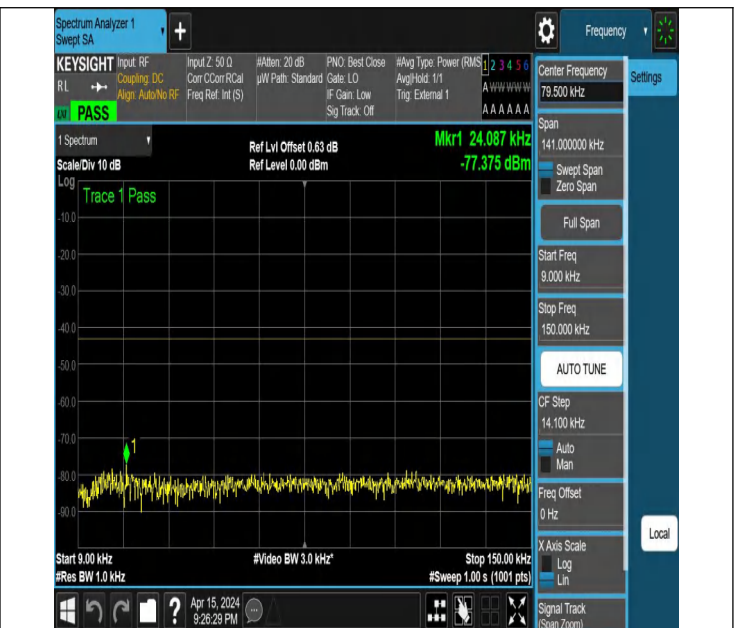
NTNV_N77-3700-3980_PC2_30_20_H_TID6_NS_01_0.009_0.15 #1
