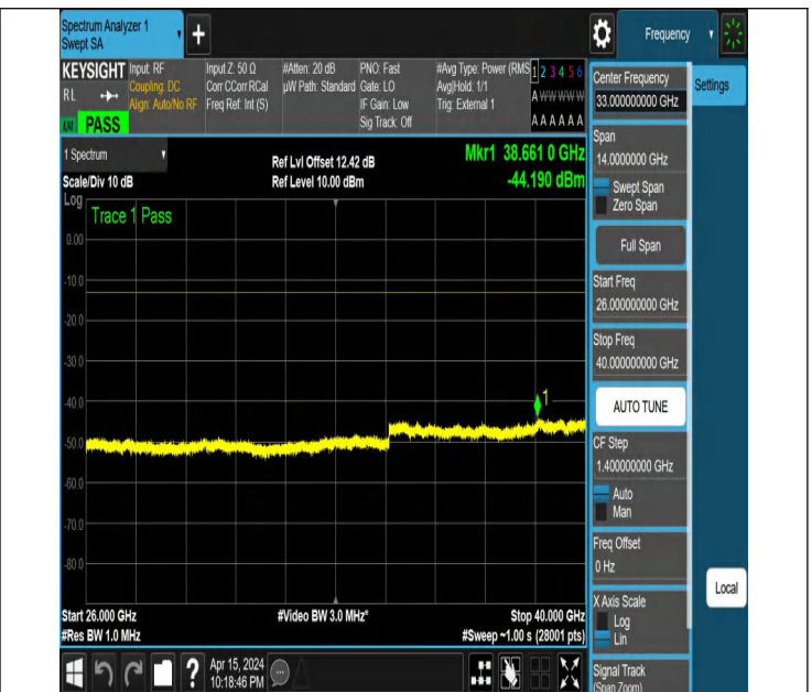
NTNV_N77-3700-3980_PC2_30_30_M_TID3_NS_01_26000_40 000 #1
