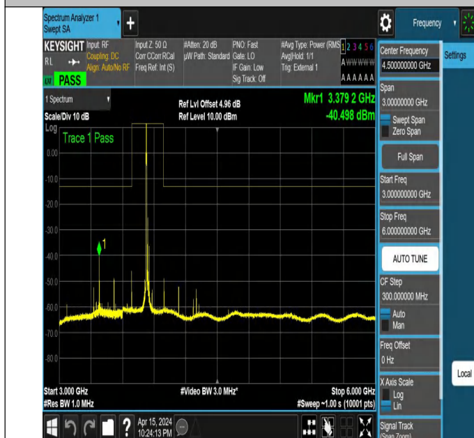
NTNV_N77-3700-3980_PC2_30_30_M_TID5_NS_01_3000_600
