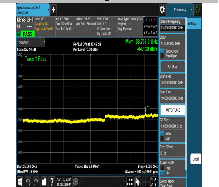
NTNV_N77-3700-3980_PC2_30_30_M_TID6_NS_01_26000_40 000 #1
