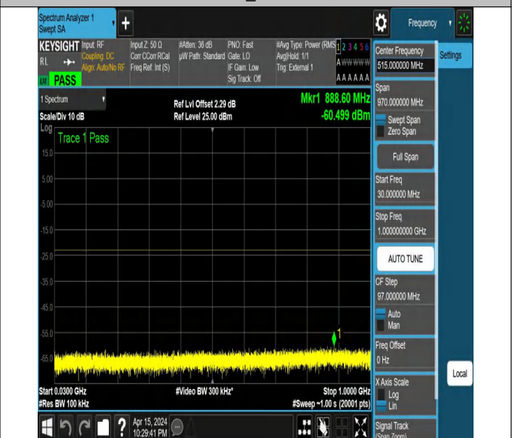
NTNV_N77-3700-3980_PC2_30_30_M_TID6_NS_01_30_1000_ #1
