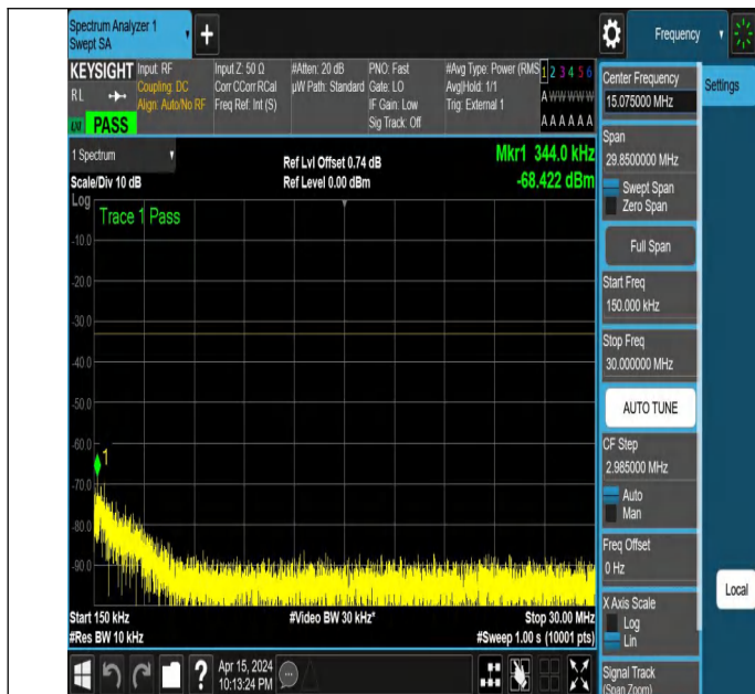
NTNV_N77-3700-3980_PC2_30_30_M_TID3_NS_01_0.15_30_#
