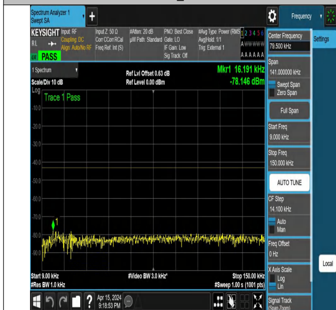
NTNV_N77-3700-3980_PC2_30_20_H_TID5_NS_01_0.009_0.15
