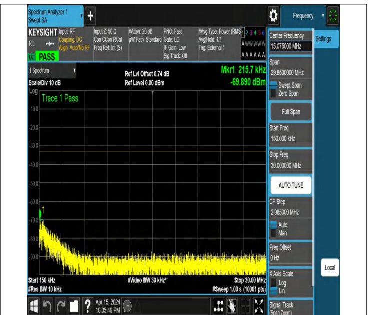
NTNV_N77-3700-3980_PC2_30_30_M_TID2_NS_01_0.15_30_#
