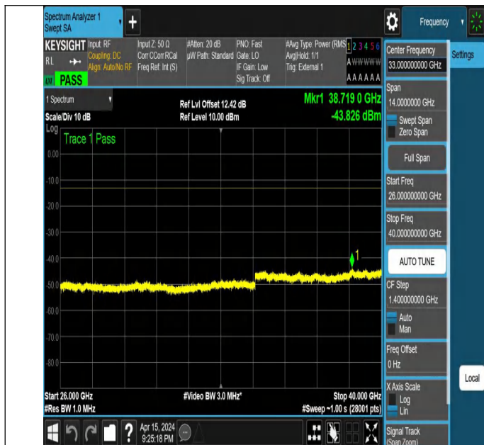
NTNV_N77-3700-3980_PC2_30_20_H_TID5_NS_01_26000_400
