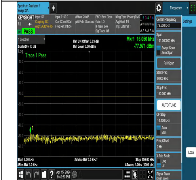
NTNV_N77-3700-3980_PC2_30_30_L_TID5_NS_01_0.009_0.15
