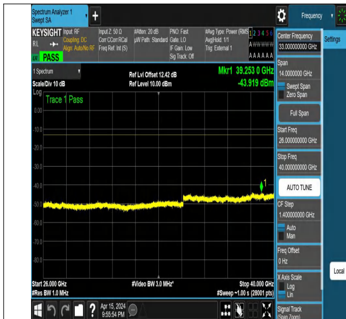
NTNV_N77-3700-3980_PC2_30_30_L_TID5_NS_01_26000_400 00 #1
