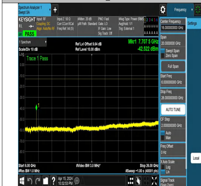
NTNV_N77-3700-3980_PC2_30_30_M_TID6_NS_01_6000_260 00 #1
