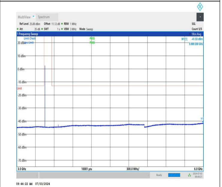
NTNV_DC_26A_n77A-3450-3550_PC2_30_5+80_M+L_TID4_NS_01_3000_6000_#1
