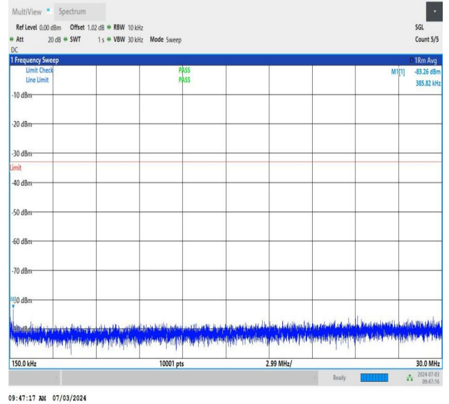
NTNV_DC_26A_n77A-3450-3550_PC2_30_5+80_M+M_TID2_N S_01_0.15_30_#1
