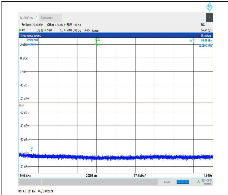
NTNV_DC_26A_n77A-3450-3550_PC2_30_5+80_M+L_TID5_NS_01_30_1000_#1
