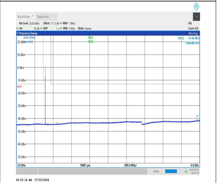
NTNV_DC_26A_n77A-3450-3550_PC2_30_5+80_M+H_TID4_N S_01_3000_6000_#1
