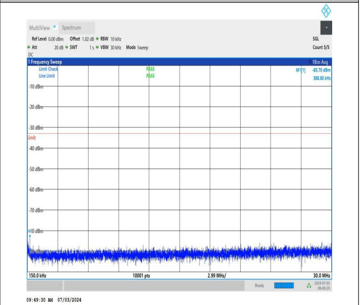
NTNV_DC_26A_n77A-3450-3550_PC2_30_5+80_M+M_TID5_N S_01_0.15_30_#1
