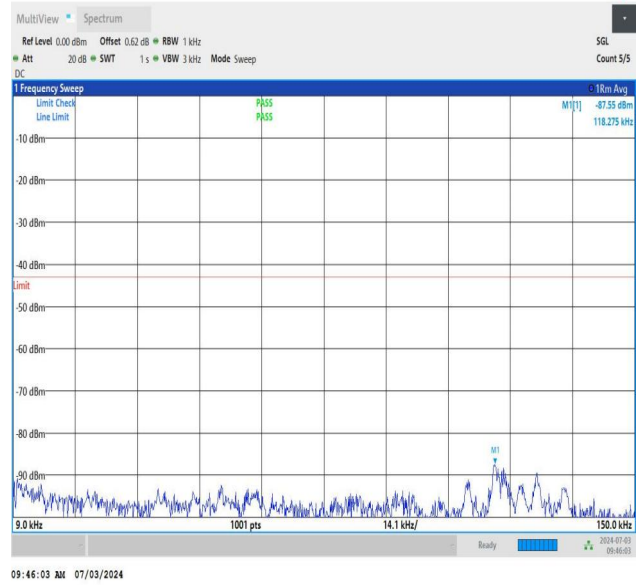
NTNV_DC_26A_n77A-3450-3550_PC2_30_5+80_M+M_TID1_N_S_01_0.009_0.15_#1
