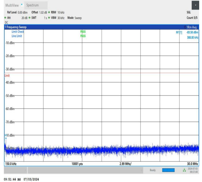
NTNV_DC_26A_n77A-3450-3550_PC2_30_5+80_M+H_TID2_N S_01_0.15_30_#1
