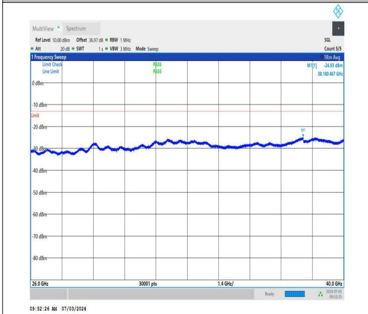
NTNV_DC_26A_n77A-3450-3550_PC2_30_5+80_M+H_TID2_N S_01_26000_40000_#1
