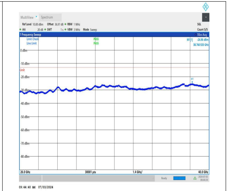
NTNV_DC_26A_n77A-3450-3550_PC2_30_5+80_M+L_TID4_NS _01_26000_40000_#1
