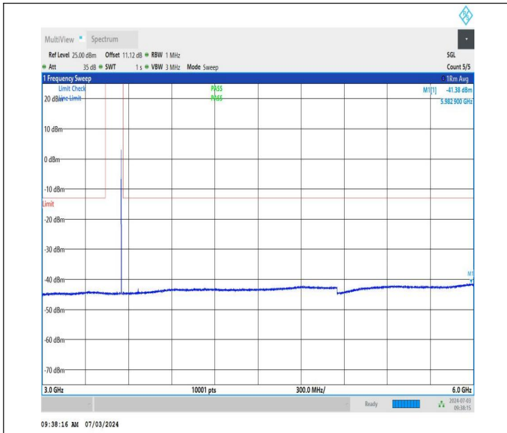
NTNV_DC_26A_n77A-3450-3550_PC2_30_5+60_M+H_TID2_N S_01_3000_6000_#1
