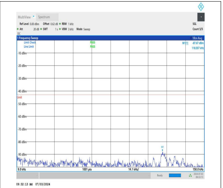
NTNV_DC_26A_n77A-3450-3550_PC2_30_5+60_M+M_TID1_N_S_01_0.009_0.15_#1
