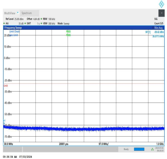
NTNV_DC_26A_n77A-3450-3550_PC2_30_5+60_M+H_TID1_N S_01_30_1000_#1
