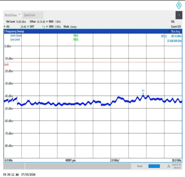
NTNV_DC_26A_n77A-3450-3550_PC2_30_5+60_M+M_TID5_N S_01_6000_26000_#1
