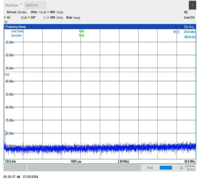
NTNV_DC_26A_n77A-3450-3550_PC2_30_5+60_M+M_TID2_N S_01_0.15_30_#1
