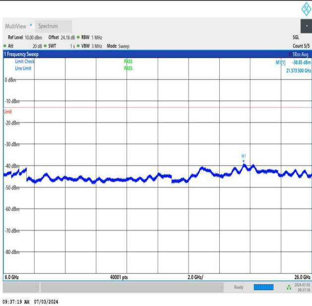
NTNV_DC_26A_n77A-3450-3550_PC2_30_5+60_M+H_TID1_N S_01_6000_26000_#1
