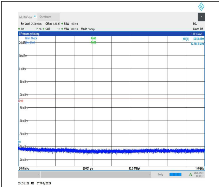
NTNV_DC_26A_n77A-3450-3550_PC2_30_5+60_M+L_TID5_NS_01_30_1000_#1
