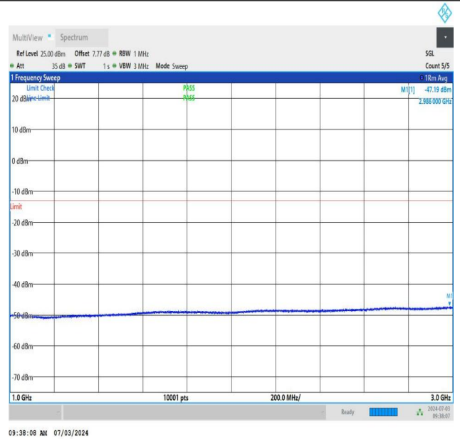
NTNV_DC_26A_n77A-3450-3550_PC2_30_5+60_M+H_TID2_N S_01_1000_3000_#1
