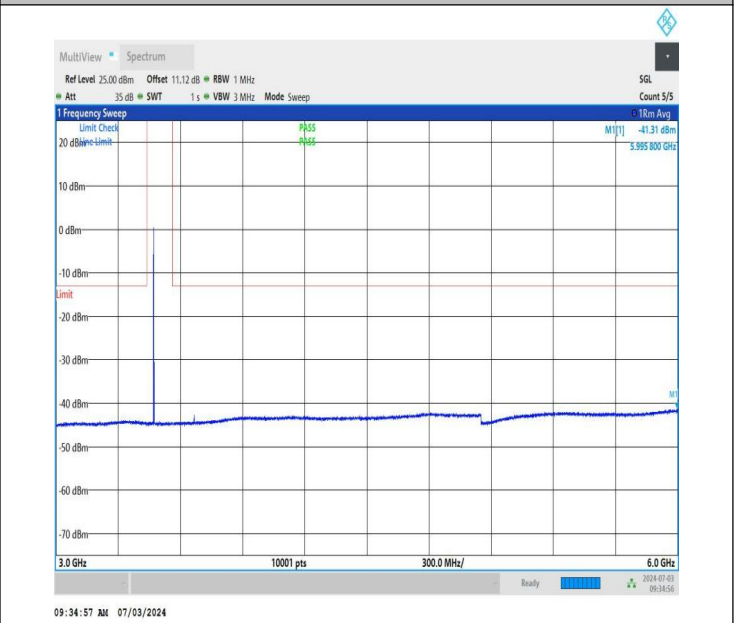
NTNV_DC_26A_n77A-3450-3550_PC2_30_5+60_M+M_TID4_N S_01_3000_6000_#1
