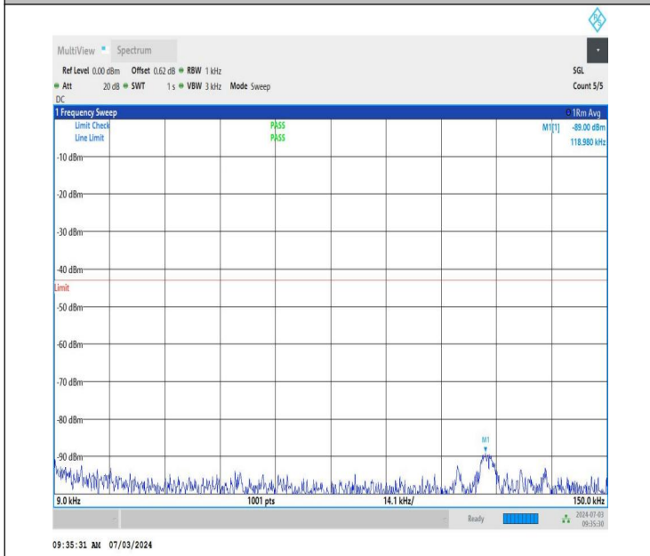
NTNV_DC_26A_n77A-3450-3550_PC2_30_5+60_M+M_TID5_N S_01_0.009_0.15_#1
