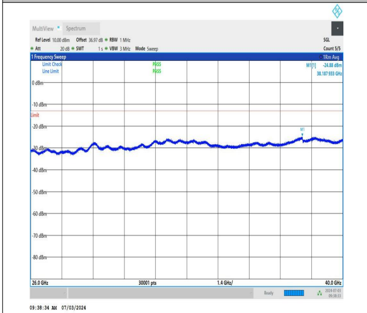
NTNV_DC_26A_n77A-3450-3550_PC2_30_5+60_M+H_TID2_N S_01_26000_40000_#1
