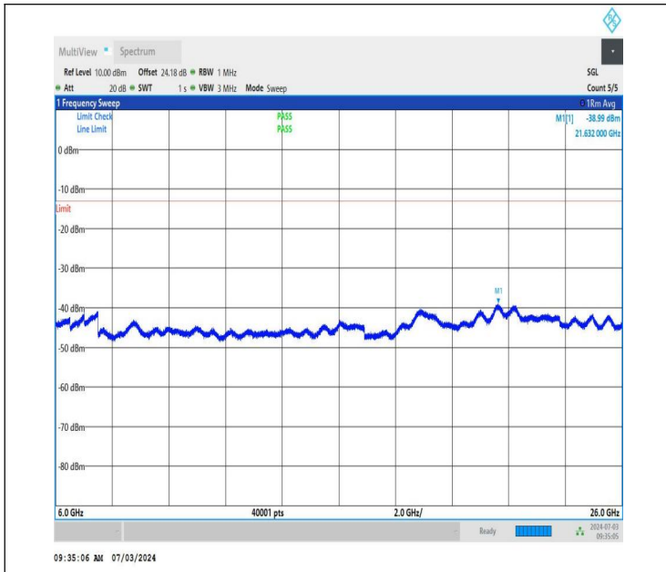
NTNV_DC_26A_n77A-3450-3550_PC2_30_5+60_M+M_TID4_N S_01_6000_26000_#1
