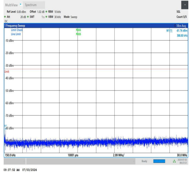
NTNV_DC_26A_n77A-3450-3550_PC2_30_5+60_M+H_TID2_N S_01_0.15_30_#1
