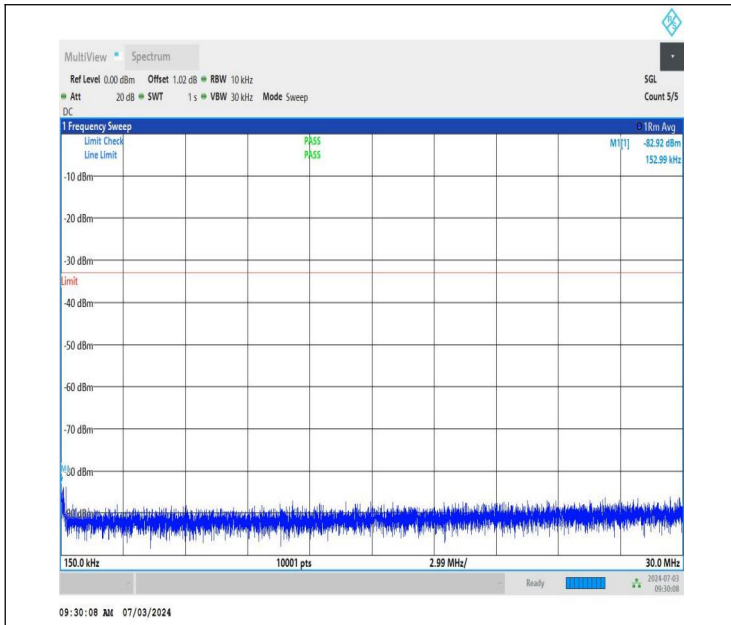
NTNV_DC_26A_n77A-3450-3550_PC2_30_5+60_M+L_TID4_NS_01_0.15_30_#1
