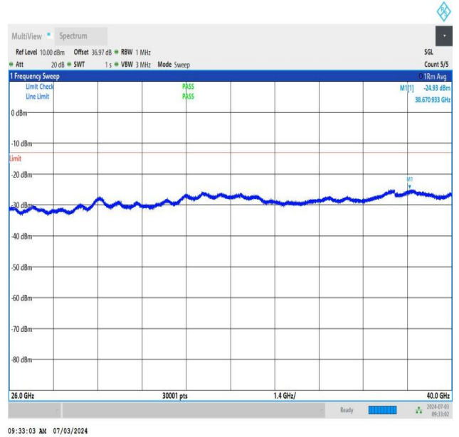
NTNV_DC_26A_n77A-3450-3550_PC2_30_5+60_M+M_TID1_N S_01_26000_40000_#1
