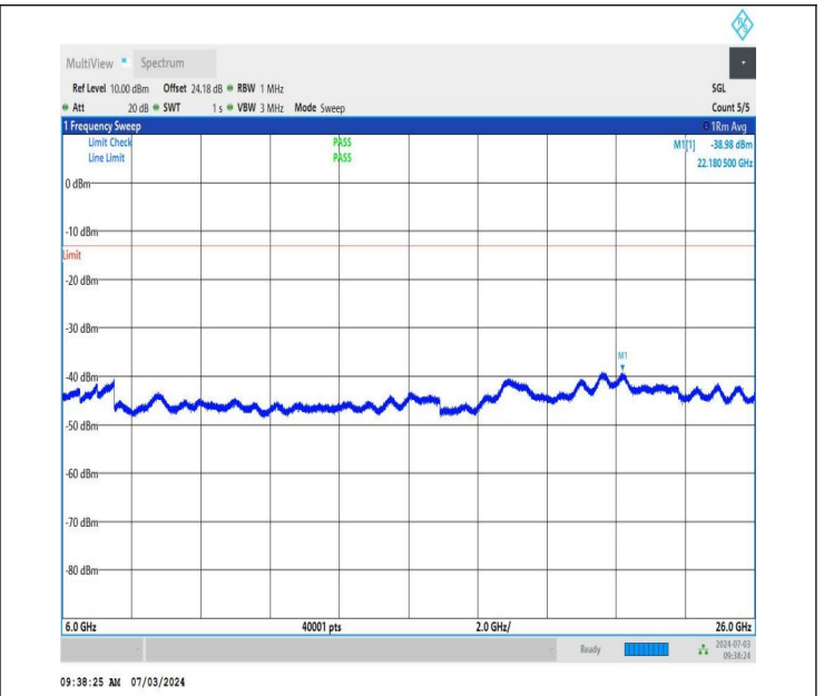
NTNV_DC_26A_n77A-3450-3550_PC2_30_5+60_M+H_TID2_N S_01_6000_26000_#1
