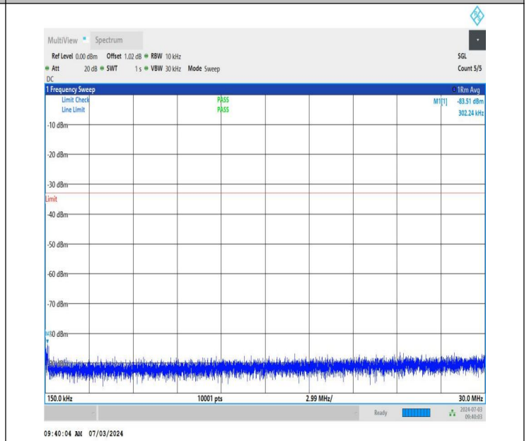
NTNV_DC_26A_n77A-3450-3550_PC2_30_5+60_M+H_TID5_N S_01_0.15_30_#1
