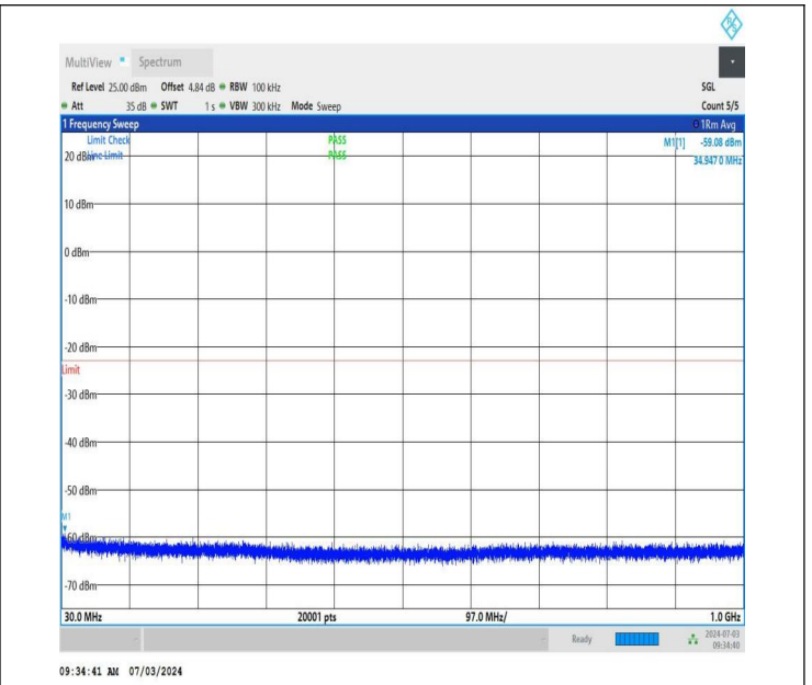
NTNV_DC_26A_n77A-3450-3550_PC2_30_5+60_M+M_TID4_N S_01_30_1000_#1
