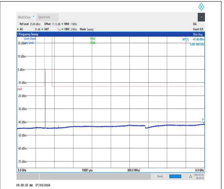
NTNV_DC_26A_n77A-3450-3550_PC2_30_5+60_M+L_TID1_NS_01_3000_6000_#1
