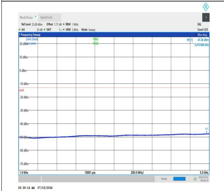
NTNV_DC_26A_n77A-3450-3550_PC2_30_5+60_M+H_TID4_N S_01_1000_3000_#1
