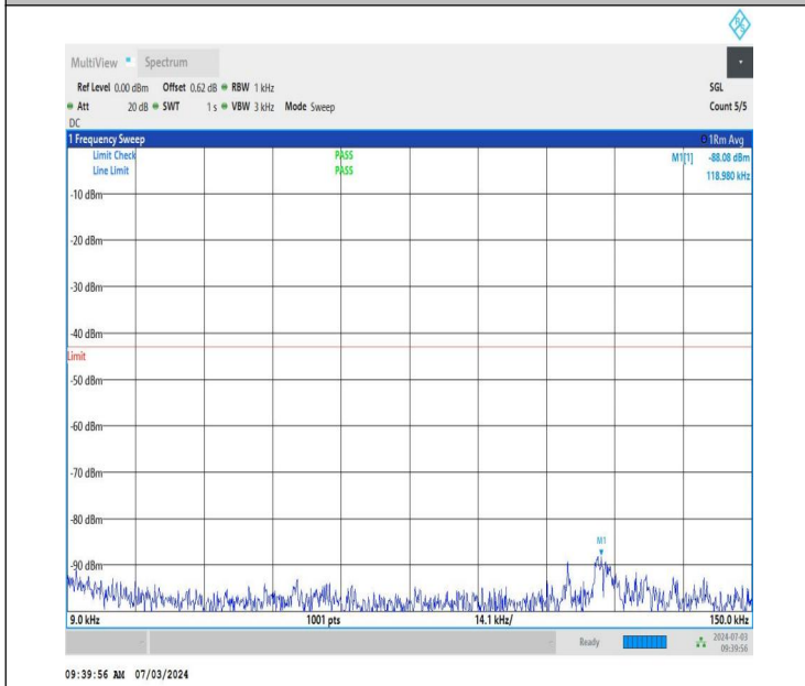
NTNV_DC_26A_n77A-3450-3550_PC2_30_5+60_M+H_TID5_N S_01_0.009_0.15_#1
