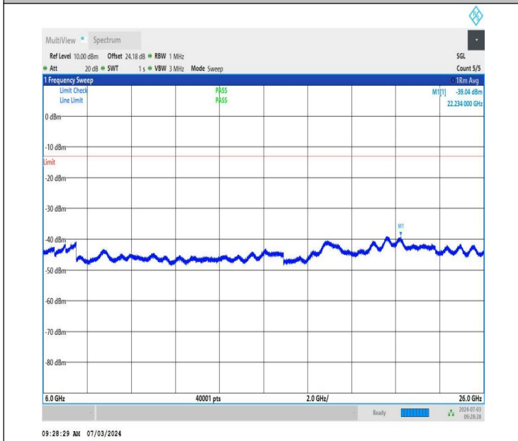
NTNV_DC_26A_n77A-3450-3550_PC2_30_5+60_M+L_TID1_NS_01_6000_26000_#1
