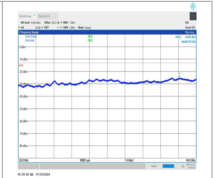
NTNV_DC_26A_n77A-3450-3550_PC2_30_5+60_M+H_TID4_N S_01_26000_40000_#1
