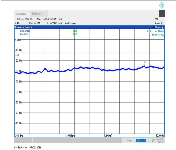
NTNV_DC_26A_n77A-3450-3550_PC2_30_5+60_M+M_TID2_N S_01_26000_40000_#1
