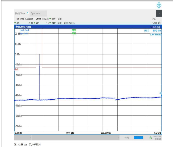
NTNV_DC_26A_n77A-3450-3550_PC2_30_5+60_M+L_TID5_NS_01_3000_6000_#1
