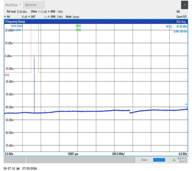
NTNV_DC_26A_n77A-3450-3550_PC2_30_5+60_M+H_TID1_N S_01_3000_6000_#1
