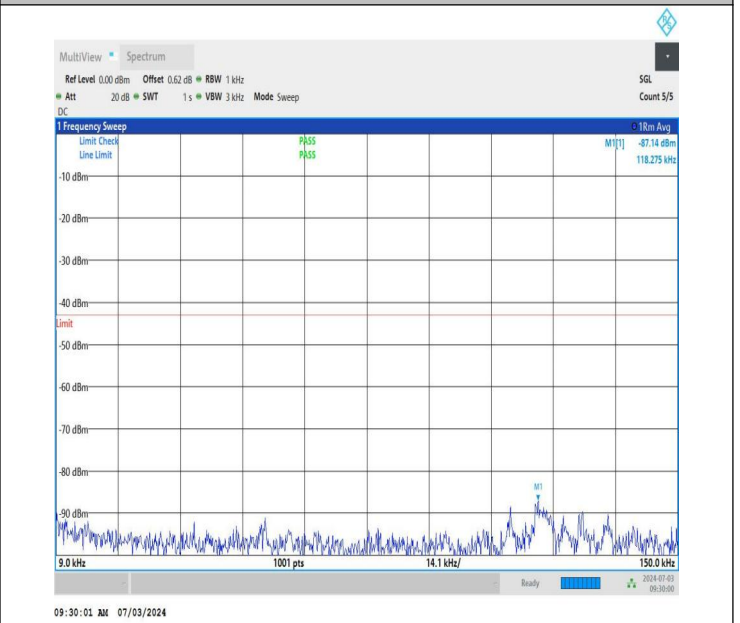
NTNV_DC_26A_n77A-3450-3550_PC2_30_5+60_M+L_TID4_NS_01_0.009_0.15_#1
