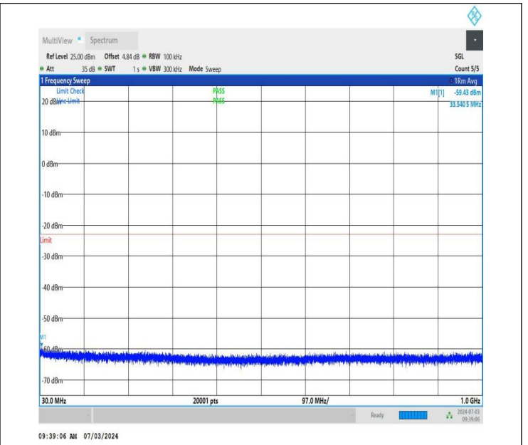
NTNV_DC_26A_n77A-3450-3550_PC2_30_5+60_M+H_TID4_N S_01_30_1000_#1
