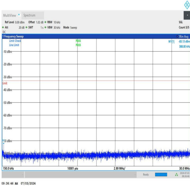
NTNV_DC_26A_n77A-3450-3550_PC2_30_5+60_M+H_TID1_N S_01_0.15_30_#1
