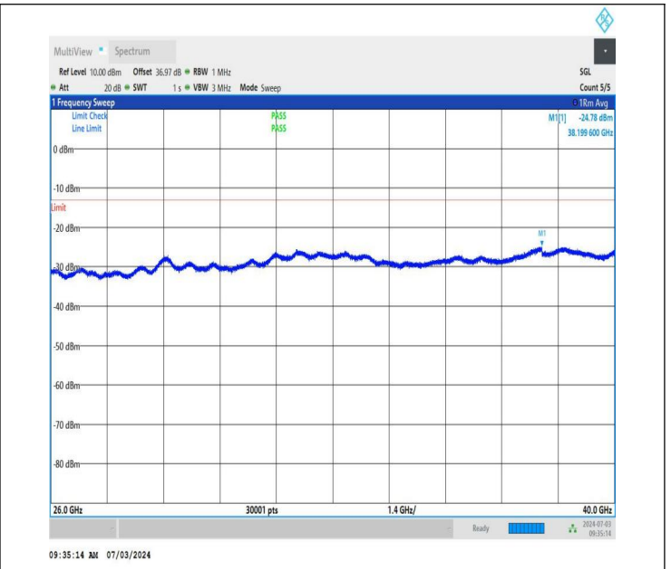
NTNV_DC_26A_n77A-3450-3550_PC2_30_5+60_M+M_TID4_N S_01_26000_40000_#1
