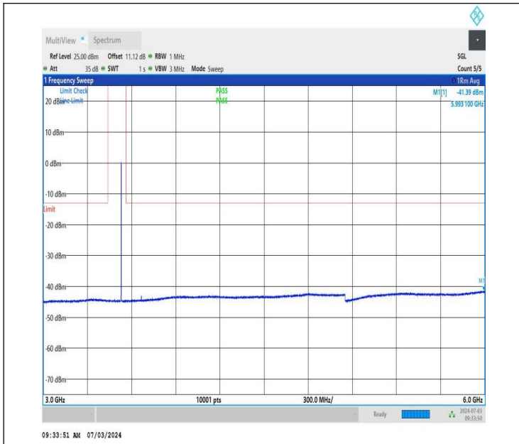
NTNV_DC_26A_n77A-3450-3550_PC2_30_5+60_M+M_TID2_N S_01_3000_6000_#1
