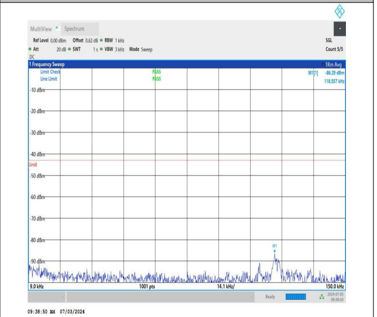
NTNV_DC_26A_n77A-3450-3550_PC2_30_5+60_M+H_TID4_N S_01_0.009_0.15_#1
