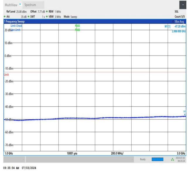
NTNV_DC_26A_n77A-3450-3550_PC2_30_5+60_M+M_TID5_N S_01_1000_3000_#1
