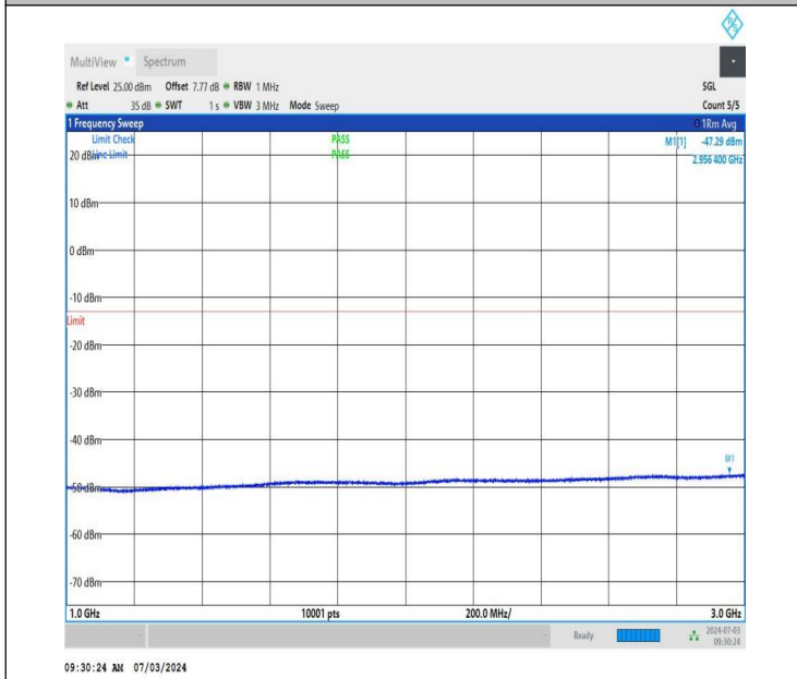
NTNV_DC_26A_n77A-3450-3550_PC2_30_5+60_M+L_TID4_NS_01_1000_3000_#1
