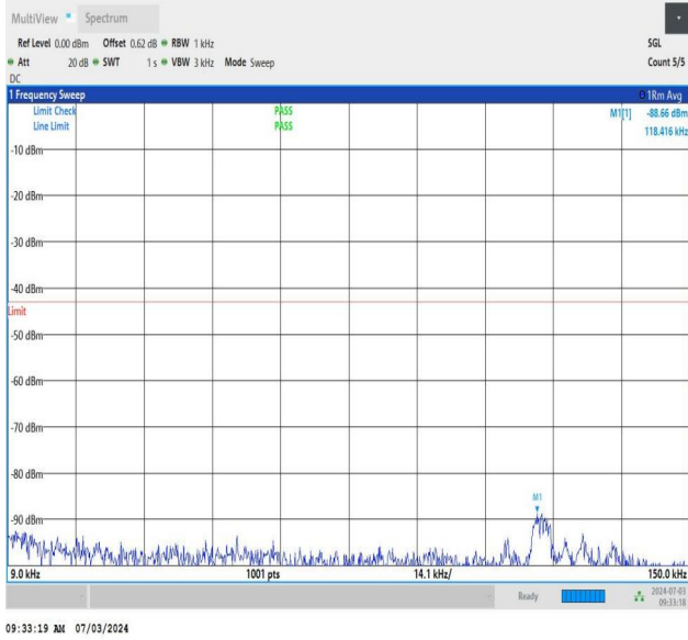
NTNV_DC_26A_n77A-3450-3550_PC2_30_5+60_M+M_TID2_N S_01_0.009_0.15_#1
