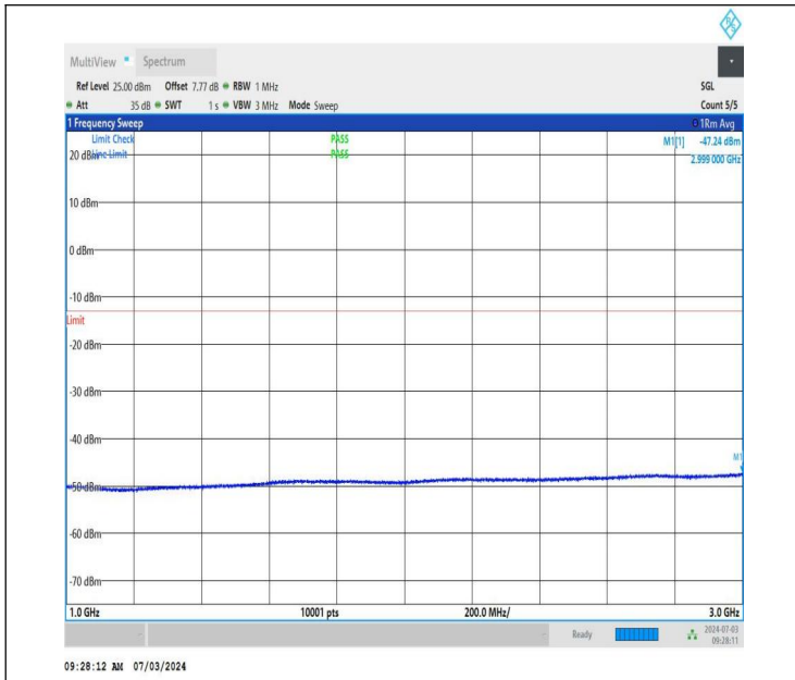
NTNV_DC_26A_n77A-3450-3550_PC2_30_5+60_M+L_TID1_NS_01_1000_3000_#1
