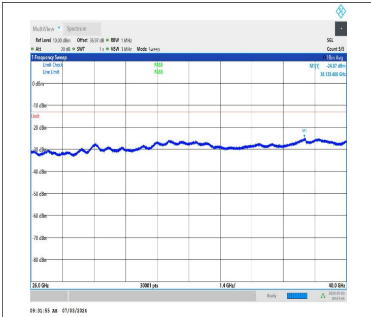
NTNV_DC_26A_n77A-3450-3550_PC2_30_5+60_M+L_TID5_NS_01_26000_40000_#1
