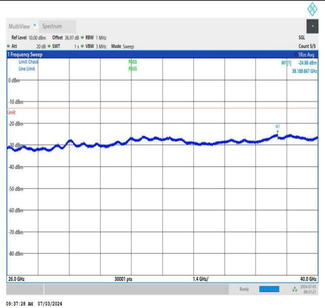
NTNV_DC_26A_n77A-3450-3550_PC2_30_5+60_M+H_TID1_N S_01_26000_40000_#1
