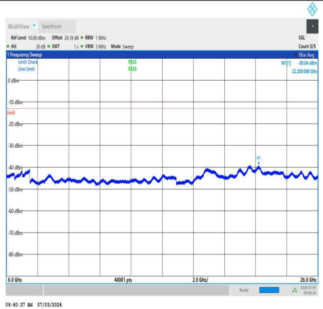
NTNV_DC_26A_n77A-3450-3550_PC2_30_5+60_M+H_TID5_N S_01_6000_26000_#1
