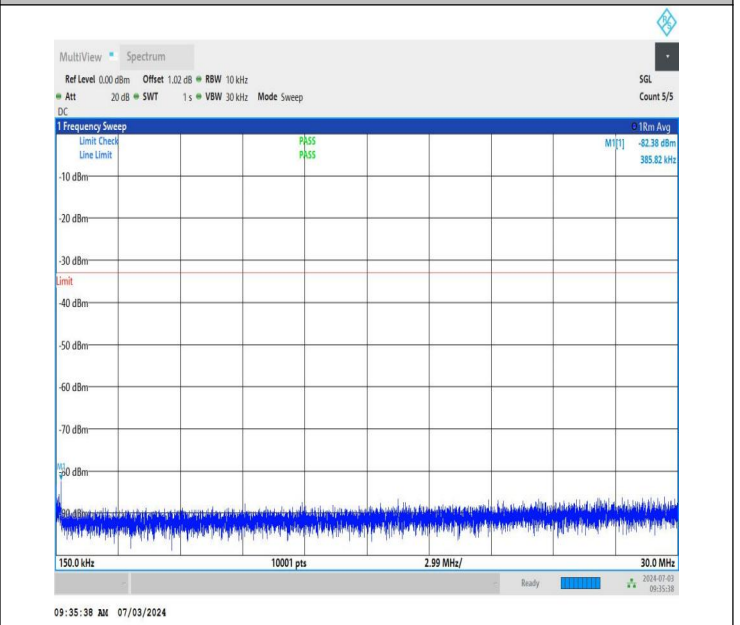
NTNV_DC_26A_n77A-3450-3550_PC2_30_5+60_M+M_TID5_N S_01_0.15_30_#1
