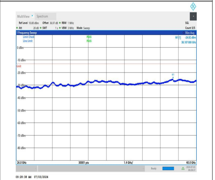
NTNV_DC_26A_n77A-3450-3550_PC2_30_5+60_M+L_TID1_NS_01_26000_40000_#1
