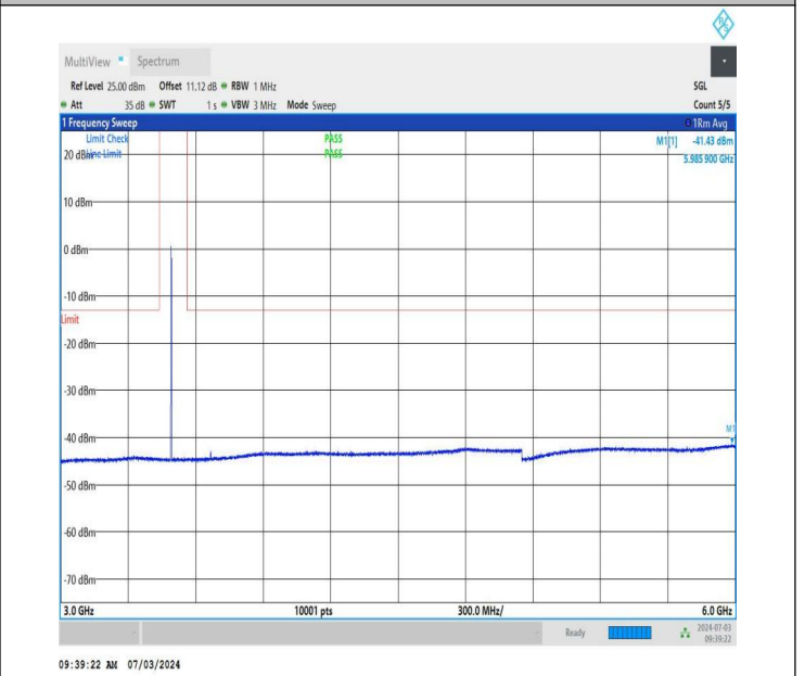
NTNV_DC_26A_n77A-3450-3550_PC2_30_5+60_M+H_TID4_N S_01_3000_6000_#1
