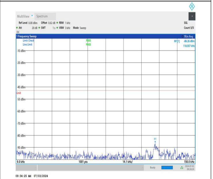
NTNV_DC_26A_n77A-3450-3550_PC2_30_5+60_M+M_TID4_N S_01_0.009_0.15_#1
