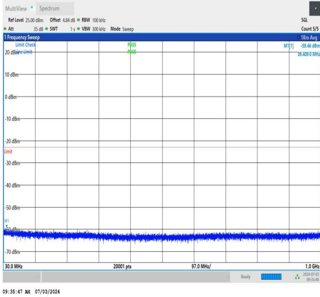
NTNV_DC_26A_n77A-3450-3550_PC2_30_5+60_M+M_TID5_N S_01_30_1000_#1
