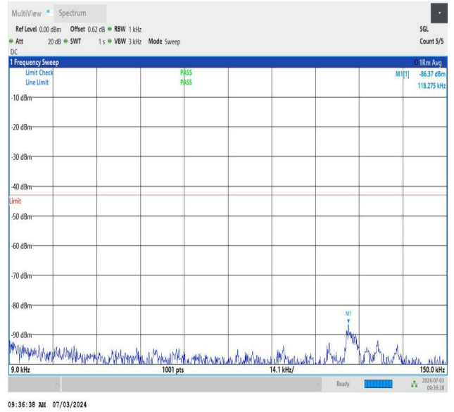
NTNV_DC_26A_n77A-3450-3550_PC2_30_5+60_M+H_TID1_N S_01_0.009_0.15_#1
