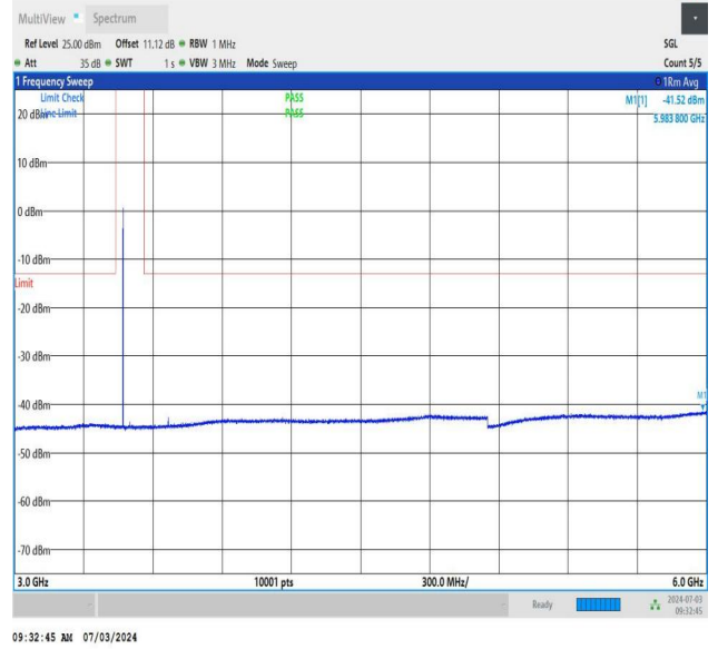
NTNV_DC_26A_n77A-3450-3550_PC2_30_5+60_M+M_TID1_N S_01_3000_6000_#1
