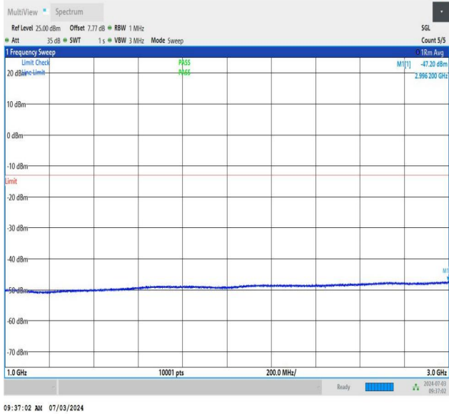
NTNV_DC_26A_n77A-3450-3550_PC2_30_5+60_M+H_TID1_N S_01_1000_3000_#1
