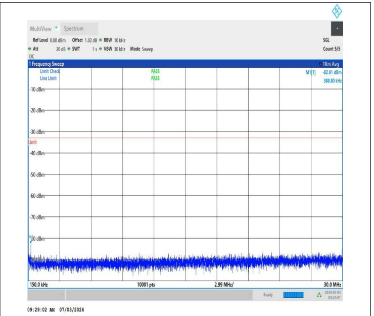
NTNV_DC_26A_n77A-3450-3550_PC2_30_5+60_M+L_TID2_NS_01_0.15_30_#1
