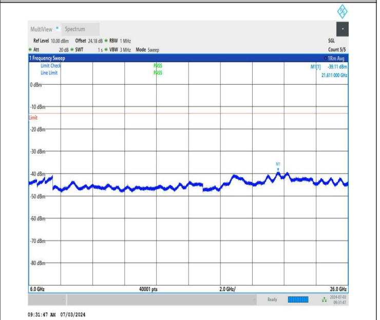
NTNV_DC_26A_n77A-3450-3550_PC2_30_5+60_M+L_TID5_NS_01_6000_26000_#1
