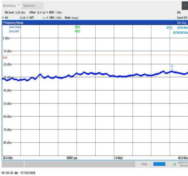
NTNV_DC_26A_n77A-3450-3550_PC2_30_5+60_M+M_TID5_N S_01_26000_40000_#1
