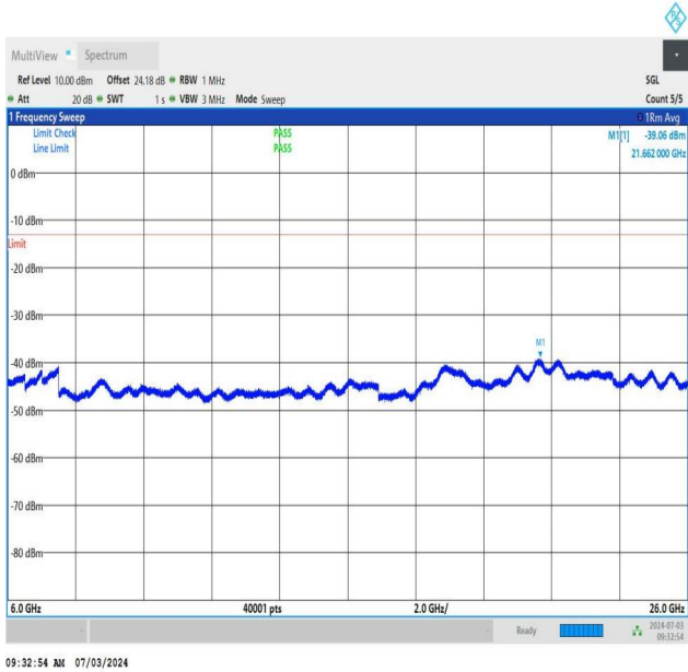
NTNV_DC_26A_n77A-3450-3550_PC2_30_5+60_M+M_TID1_N S_01_6000_26000_#1
