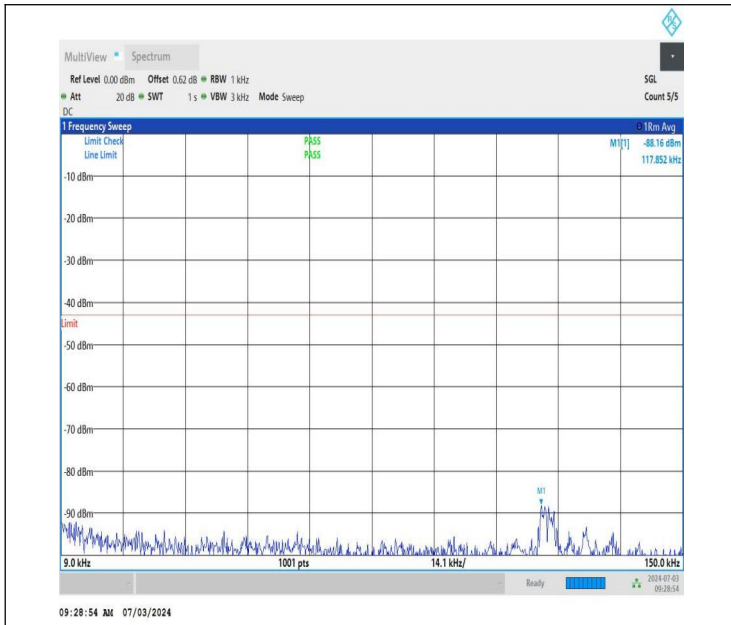
NTNV_DC_26A_n77A-3450-3550_PC2_30_5+60_M+L_TID2_NS_01_0.009_0.15_#1
