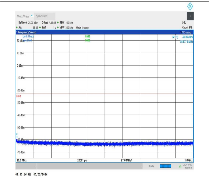
NTNV_DC_26A_n77A-3450-3550_PC2_30_5+60_M+L_TID4_NS_01_30_1000_#1
