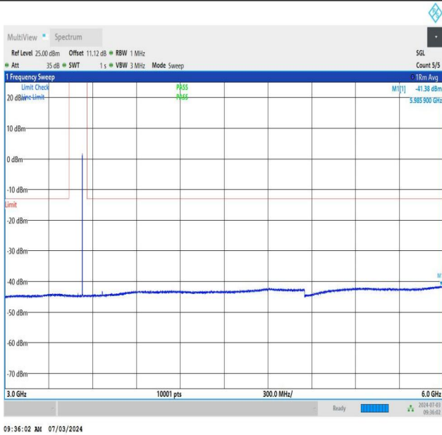
NTNV_DC_26A_n77A-3450-3550_PC2_30_5+60_M+M_TID5_N S_01_3000_6000_#1
