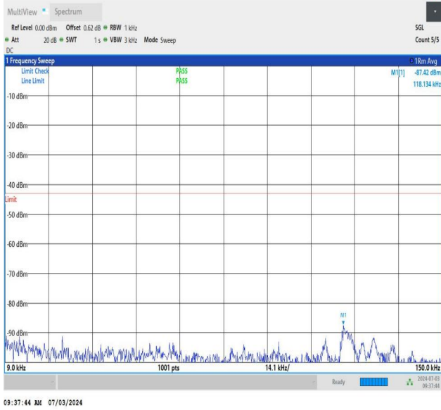
NTNV_DC_26A_n77A-3450-3550_PC2_30_5+60_M+H_TID2_N S_01_0.009_0.15_#1
