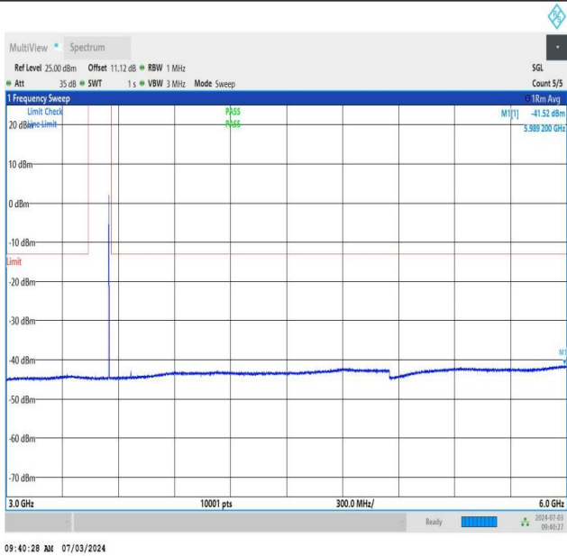
NTNV_DC_26A_n77A-3450-3550_PC2_30_5+60_M+H_TID5_N S_01_3000_6000_#1
