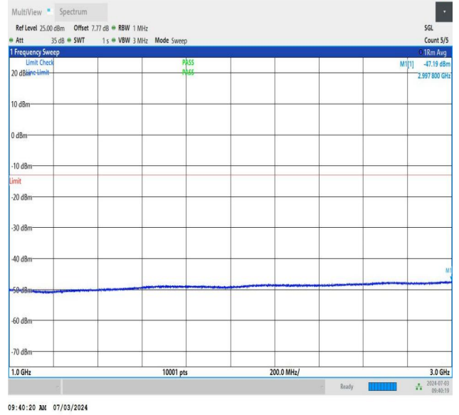
NTNV_DC_26A_n77A-3450-3550_PC2_30_5+60_M+H_TID5_N S_01_1000_3000_#1
