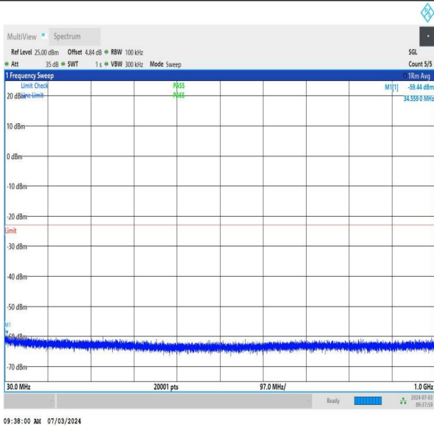
NTNV_DC_26A_n77A-3450-3550_PC2_30_5+60_M+H_TID2_N S_01_30_1000_#1
