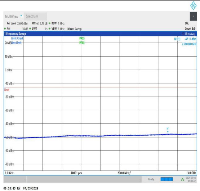
NTNV_DC_26A_n77A-3450-3550_PC2_30_5+60_M+M_TID2_N S_01_1000_3000_#1
