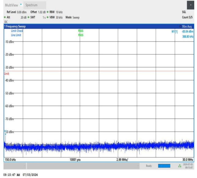
NTNV_DC_26A_n77A-3450-3550_PC2_30_5+50_M+L_TID2_NS_01_0.15_30_#1
