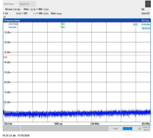
NTNV_DC_26A_n77A-3450-3550_PC2_30_5+50_M+M_TID2_N S_01_0.15_30_#1
