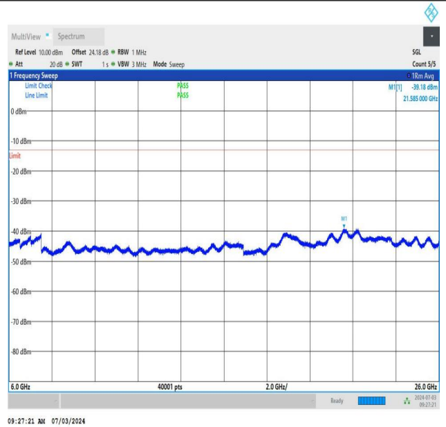
NTNV_DC_26A_n77A-3450-3550_PC2_30_5+50_M+H_TID5_N S_01_6000_26000_#1
