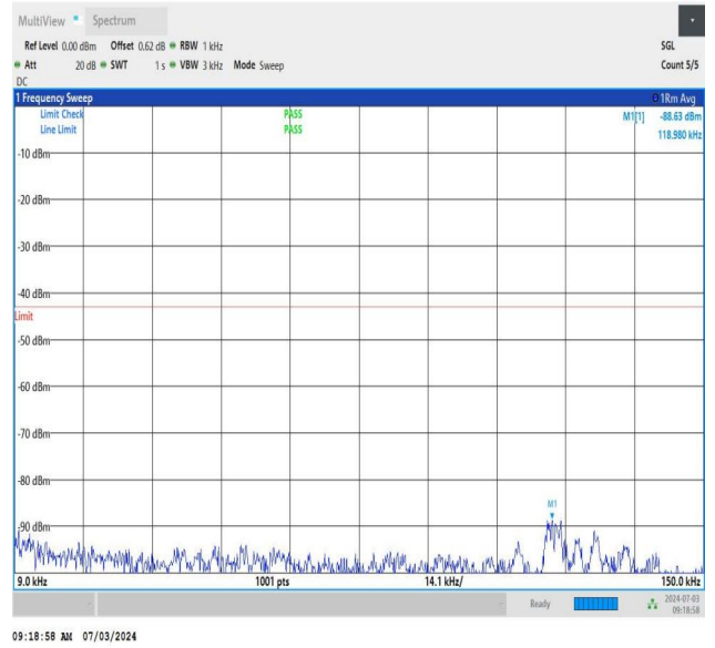
NTNV_DC_26A_n77A-3450-3550_PC2_30_5+50_M+M_TID1_N_S_01_0.009_0.15_#1
