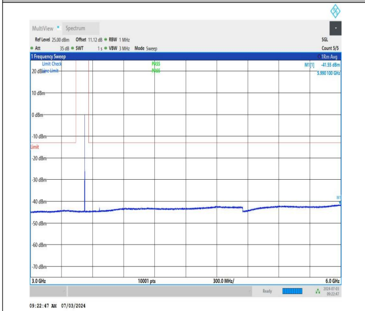
NTNV_DC_26A_n77A-3450-3550_PC2_30_5+50_M+M_TID5_N S_01_3000_6000_#1
