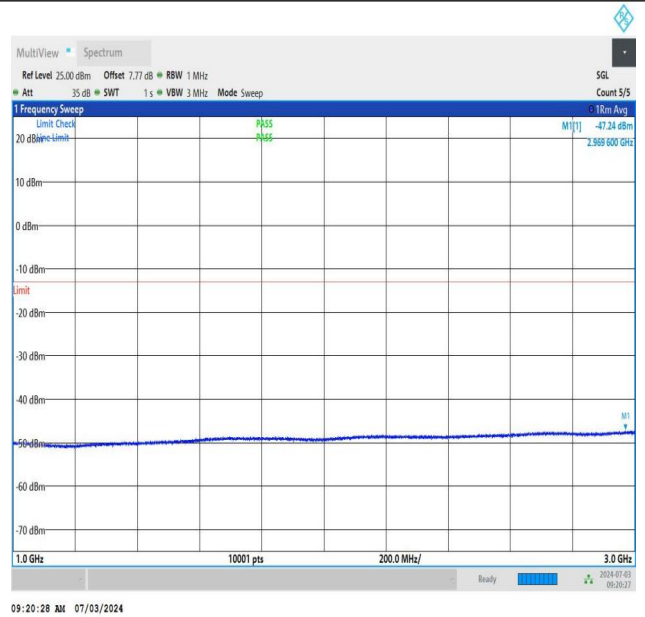
NTNV_DC_26A_n77A-3450-3550_PC2_30_5+50_M+M_TID2_N S_01_1000_3000_#1
