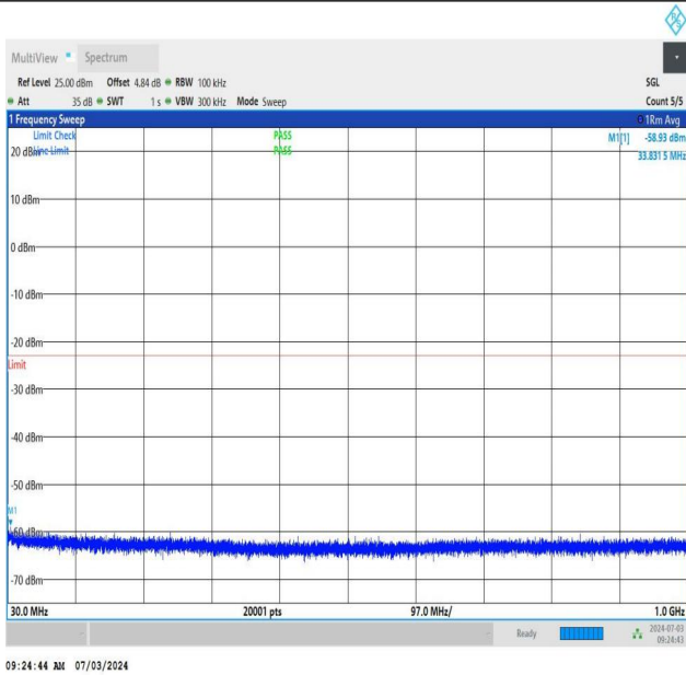
NTNV_DC_26A_n77A-3450-3550_PC2_30_5+50_M+H_TID2_N S_01_30_1000_#1
