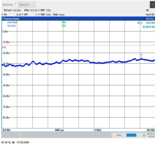
NTNV_DC_26A_n77A-3450-3550_PC2_30_5+50_M+L_TID5_NS_01_26000_40000_#1
