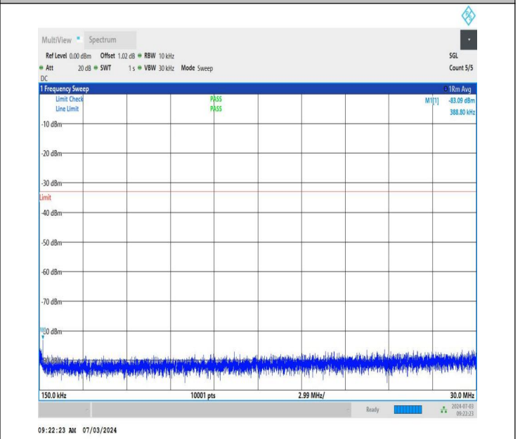
NTNV_DC_26A_n77A-3450-3550_PC2_30_5+50_M+M_TID5_N S_01_0.15_30_#1
