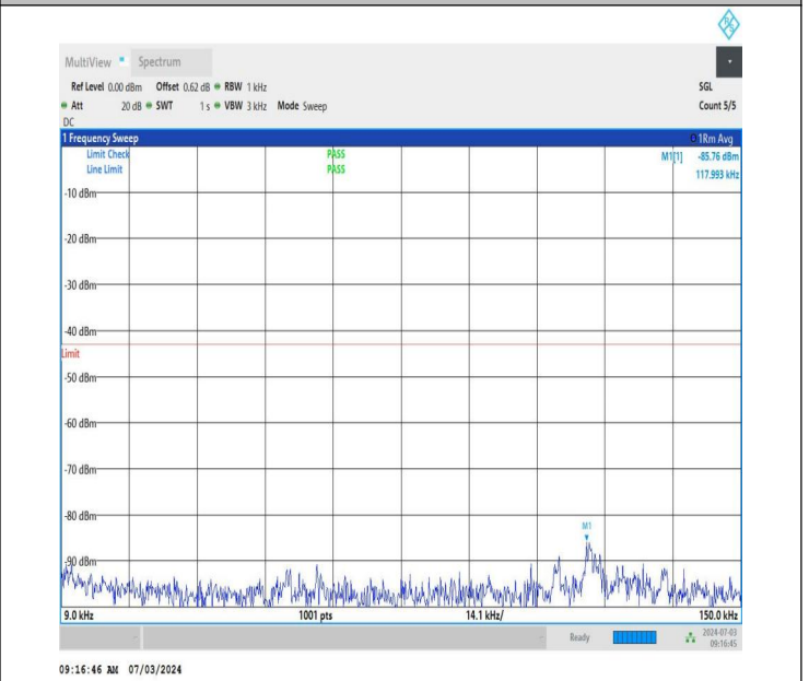
NTNV_DC_26A_n77A-3450-3550_PC2_30_5+50_M+L_TID4_NS_01_0.009_0.15_#1
