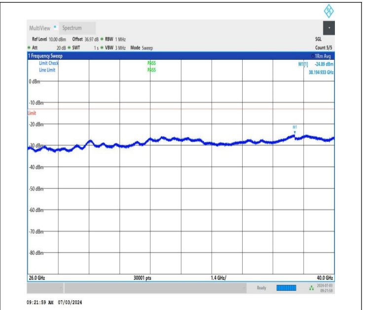
NTNV_DC_26A_n77A-3450-3550_PC2_30_5+50_M+M_TID4_N S_01_26000_40000_#1
