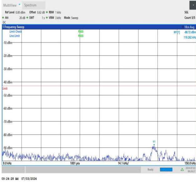
NTNV_DC_26A_n77A-3450-3550_PC2_30_5+50_M+H_TID2_N S_01_0.009_0.15_#1
