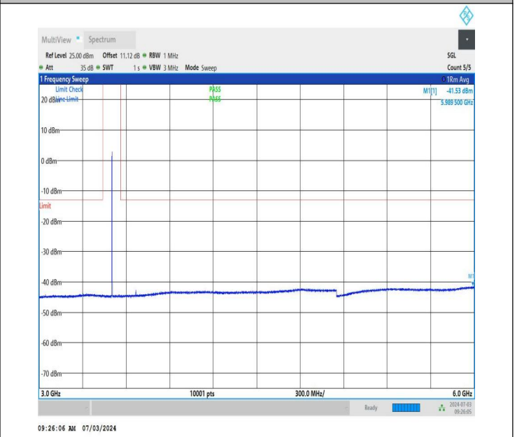
NTNV_DC_26A_n77A-3450-3550_PC2_30_5+50_M+H_TID4_N S_01_3000_6000_#1
