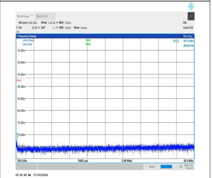
NTNV_DC_26A_n77A-3450-3550_PC2_30_5+50_M+H_TID5_N S_01_0.15_30_#1
