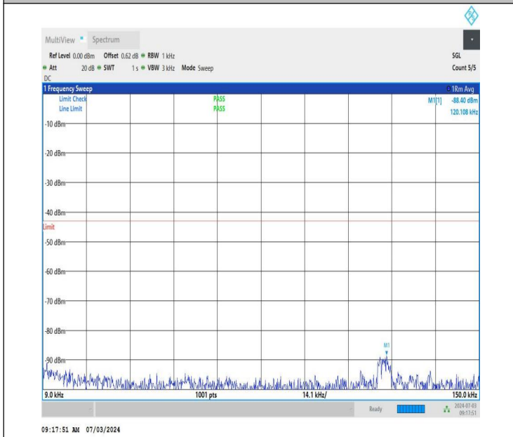
NTNV_DC_26A_n77A-3450-3550_PC2_30_5+50_M+L_TID5_NS_01_0.009_0.15_#1
