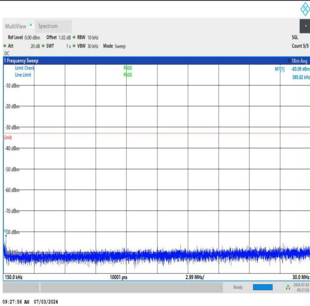
NTNV_DC_26A_n77A-3450-3550_PC2_30_5+60_M+L_TID1_NS _01_0.15_30_#1
