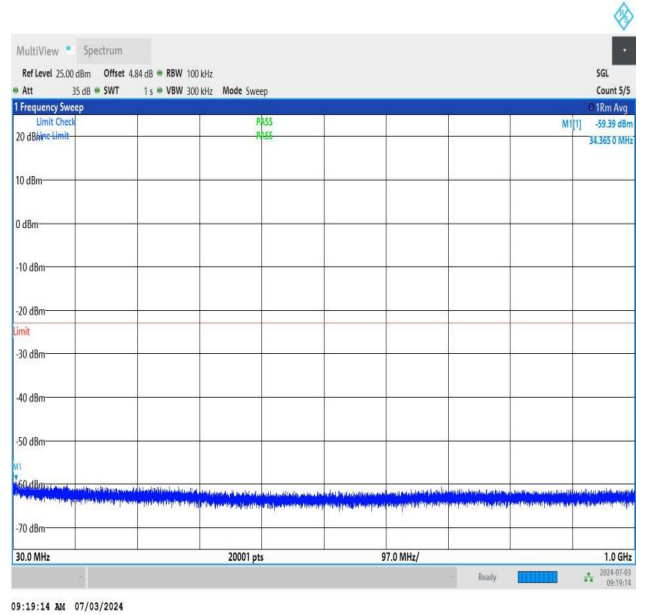
NTNV_DC_26A_n77A-3450-3550_PC2_30_5+50_M+M_TID1_N_S_01_30_1000_#1
