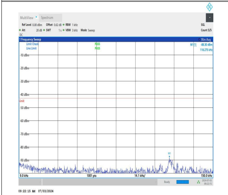
NTNV_DC_26A_n77A-3450-3550_PC2_30_5+50_M+M_TID5_N S_01_0.009_0.15_#1
