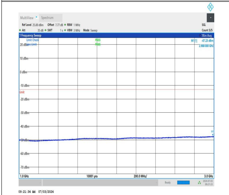
NTNV_DC_26A_n77A-3450-3550_PC2_30_5+50_M+M_TID4_N S_01_1000_3000_#1
