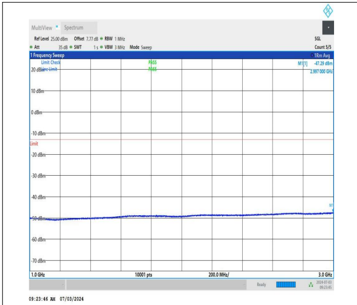
NTNV_DC_26A_n77A-3450-3550_PC2_30_5+50_M+H_TID1_N S_01_1000_3000_#1
