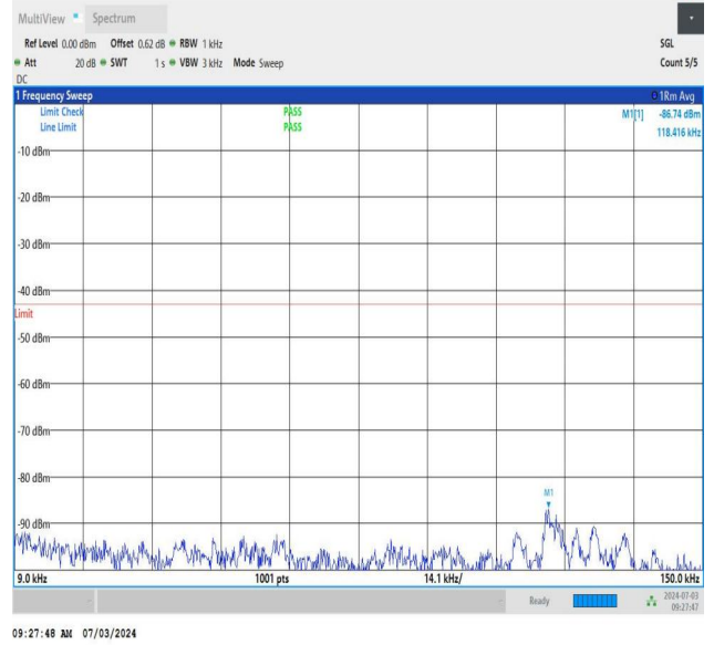
NTNV_DC_26A_n77A-3450-3550_PC2_30_5+60_M+L_TID1_NS _01_0.009_0.15_#1
