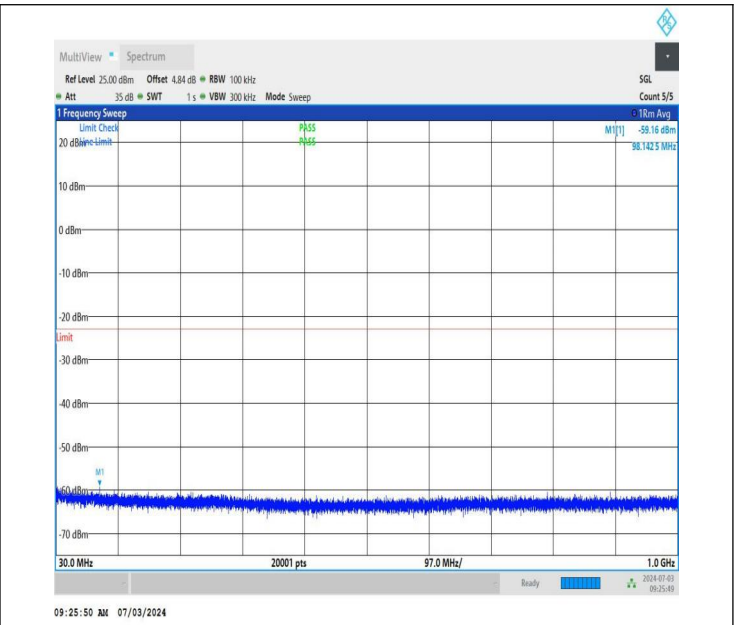
NTNV_DC_26A_n77A-3450-3550_PC2_30_5+50_M+H_TID4_N S_01_30_1000_#1
