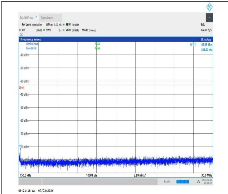
NTNV_DC_26A_n77A-3450-3550_PC2_30_5+50_M+M_TID4_N S_01_0.15_30_#1
