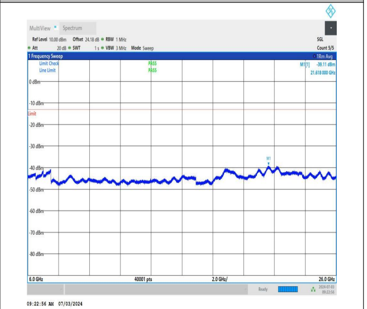
NTNV_DC_26A_n77A-3450-3550_PC2_30_5+50_M+M_TID5_N S_01_6000_26000_#1
