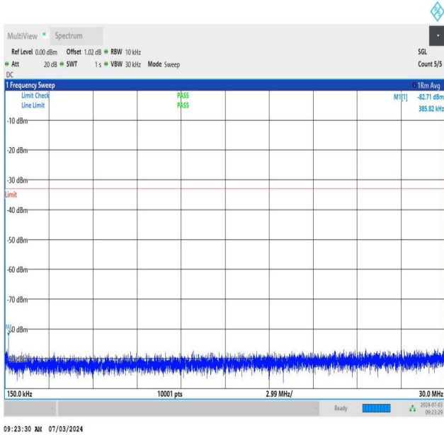
NTNV_DC_26A_n77A-3450-3550_PC2_30_5+50_M+H_TID1_N S_01_0.15_30_#1
