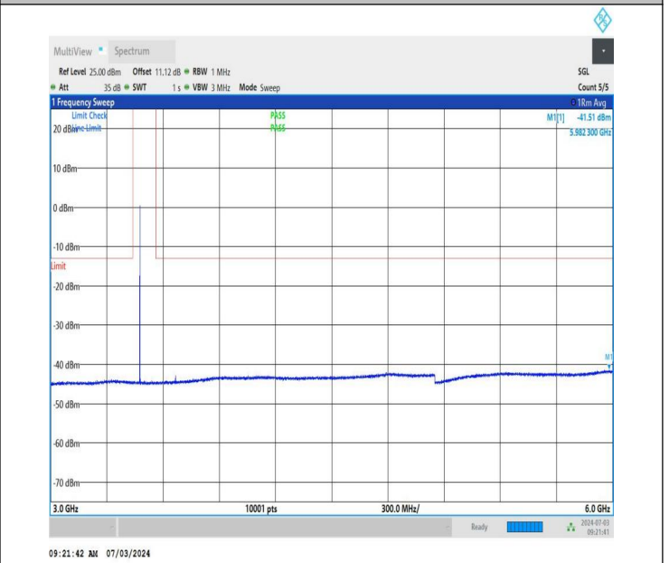
NTNV_DC_26A_n77A-3450-3550_PC2_30_5+50_M+M_TID4_N S_01_3000_6000_#1
