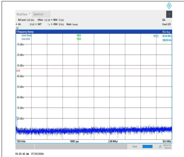
NTNV_DC_26A_n77A-3450-3550_PC2_30_5+50_M+H_TID4_N S_01_0.15_30_#1
