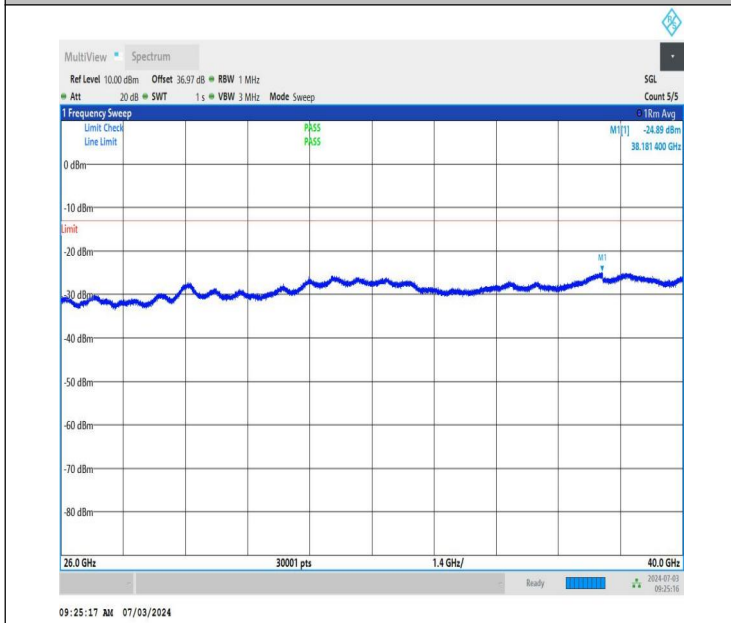
NTNV_DC_26A_n77A-3450-3550_PC2_30_5+50_M+H_TID2_N S_01_26000_40000_#1
