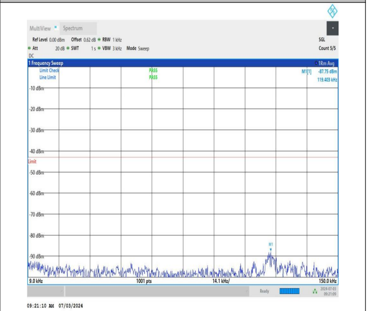
NTNV_DC_26A_n77A-3450-3550_PC2_30_5+50_M+M_TID4_N S_01_0.009_0.15_#1
