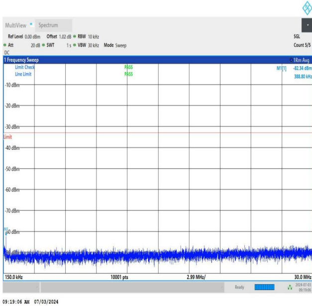
NTNV_DC_26A_n77A-3450-3550_PC2_30_5+50_M+M_TID1_N_S_01_0.15_30_#1
