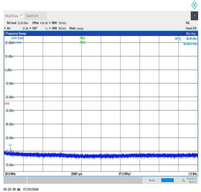
NTNV_DC_26A_n77A-3450-3550_PC2_30_5+50_M+H_TID1_N S_01_30_1000_#1
