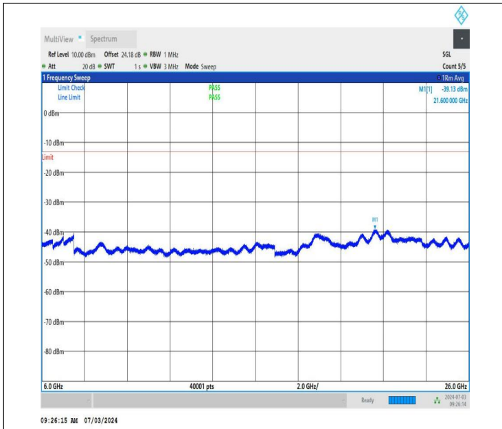
NTNV_DC_26A_n77A-3450-3550_PC2_30_5+50_M+H_TID4_N S_01_6000_26000_#1
