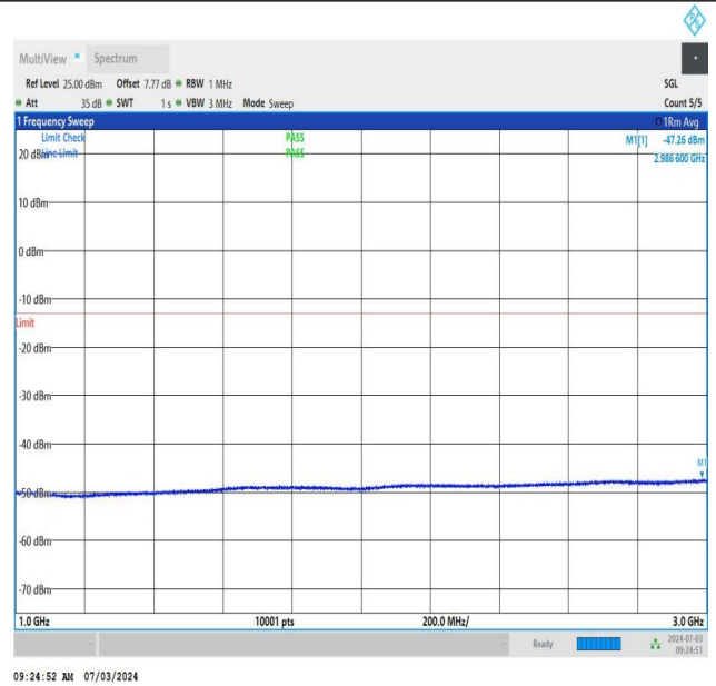
NTNV_DC_26A_n77A-3450-3550_PC2_30_5+50_M+H_TID2_N S_01_1000_3000_#1
