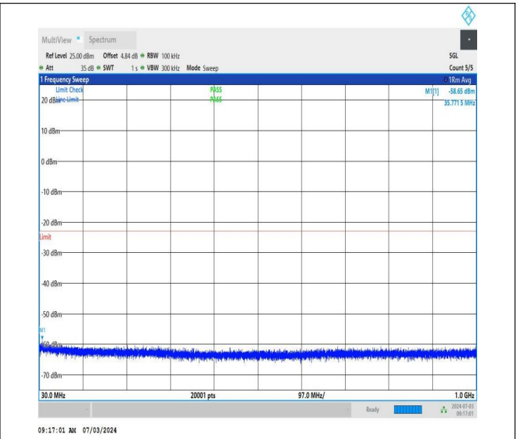
NTNV_DC_26A_n77A-3450-3550_PC2_30_5+50_M+L_TID4_NS_01_30_1000_#1
