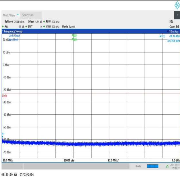
NTNV_DC_26A_n77A-3450-3550_PC2_30_5+50_M+M_TID2_N S_01_30_1000_#1
