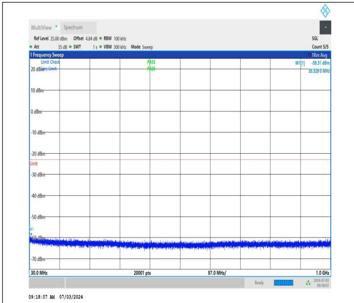
NTNV_DC_26A_n77A-3450-3550_PC2_30_5+50_M+L_TID5_NS_01_30_1000_#1
