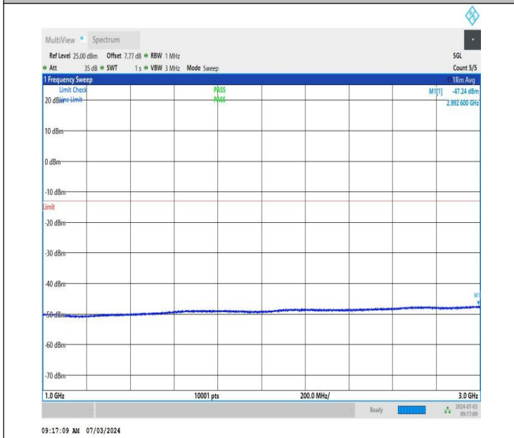
NTNV_DC_26A_n77A-3450-3550_PC2_30_5+50_M+L_TID4_NS_01_1000_3000_#1
