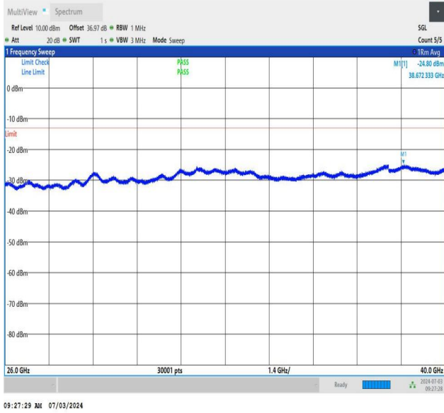
NTNV_DC_26A_n77A-3450-3550_PC2_30_5+50_M+H_TID5_N S_01_26000_40000_#1
