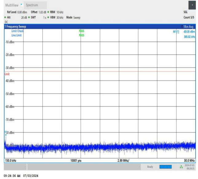
NTNV_DC_26A_n77A-3450-3550_PC2_30_5+50_M+H_TID2_N S_01_0.15_30_#1
