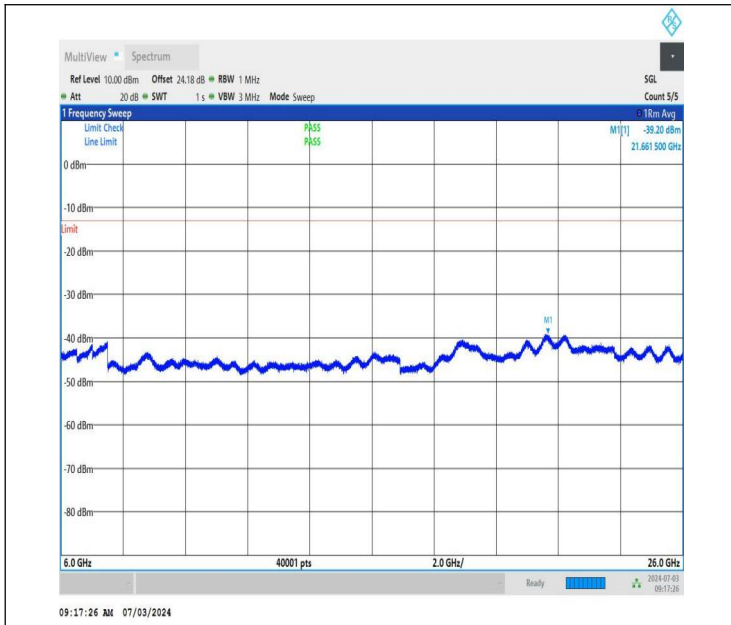
NTNV_DC_26A_n77A-3450-3550_PC2_30_5+50_M+L_TID4_NS_01_6000_26000_#1
