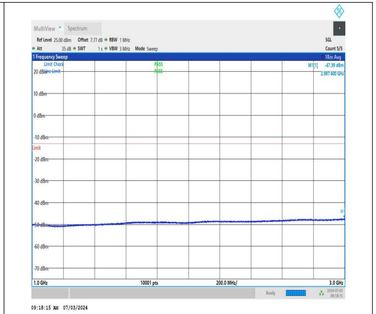
NTNV_DC_26A_n77A-3450-3550_PC2_30_5+50_M+L_TID5_NS_01_1000_3000_#1
