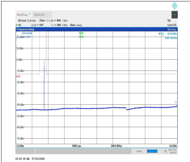
NTNV_DC_26A_n77A-3450-3550_PC2_30_5+50_M+M_TID2_N S_01_3000_6000_#1
