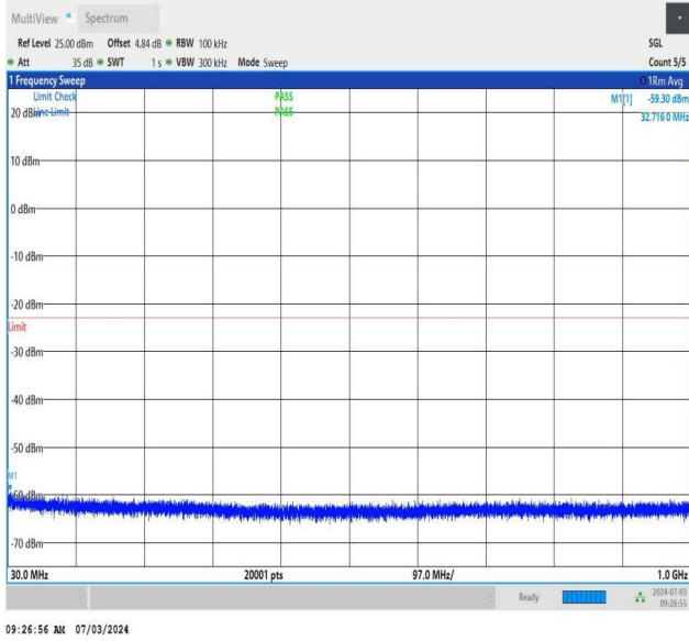
NTNV_DC_26A_n77A-3450-3550_PC2_30_5+50_M+H_TID5_N S_01_30_1000_#1
