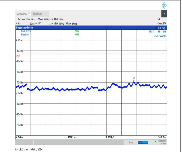
NTNV_DC_26A_n77A-3450-3550_PC2_30_5+50_M+L_TID5_NS_01_6000_26000_#1
