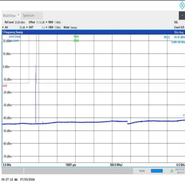
NTNV_DC_26A_n77A-3450-3550_PC2_30_5+50_M+H_TID5_N S_01_3000_6000_#1
