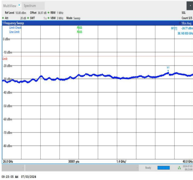
NTNV_DC_26A_n77A-3450-3550_PC2_30_5+50_M+M_TID5_N S_01_26000_40000_#1
