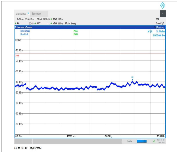
NTNV_DC_26A_n77A-3450-3550_PC2_30_5+50_M+M_TID4_N S_01_6000_26000_#1
