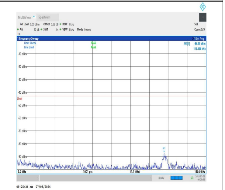
NTNV_DC_26A_n77A-3450-3550_PC2_30_5+50_M+H_TID4_N S_01_0.009_0.15_#1
