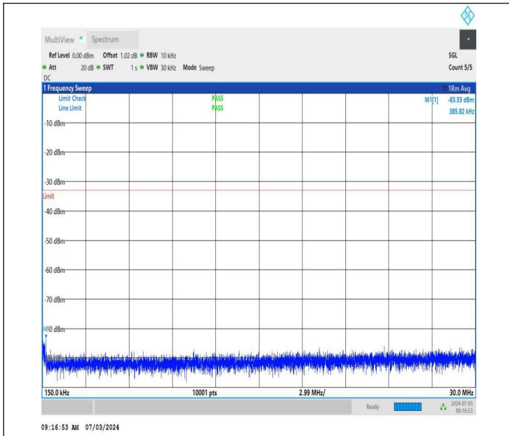
NTNV_DC_26A_n77A-3450-3550_PC2_30_5+50_M+L_TID4_NS_01_0.15_30_#1
