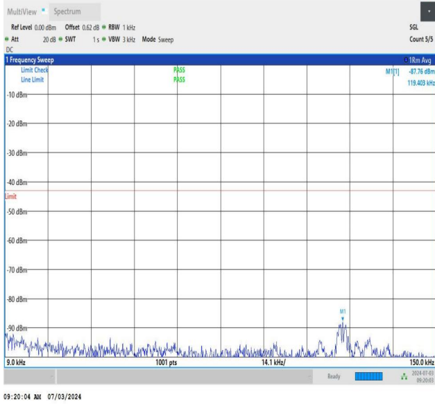
NTNV_DC_26A_n77A-3450-3550_PC2_30_5+50_M+M_TID2_N S_01_0.009_0.15_#1
