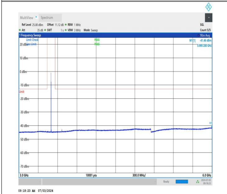
NTNV_DC_26A_n77A-3450-3550_PC2_30_5+50_M+L_TID5_NS_01_3000_6000_#1
