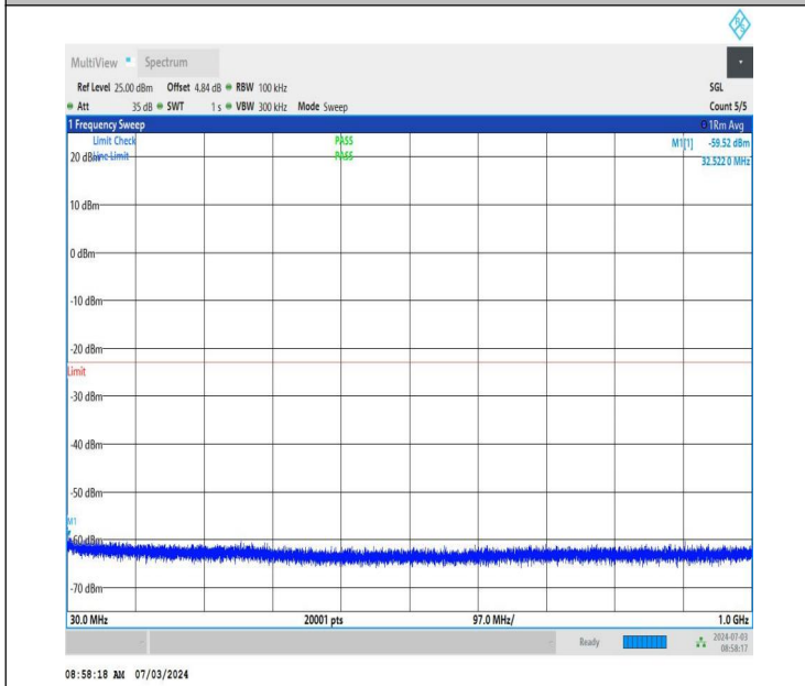
NTNV_DC_26A_n77A-3450-3550_PC2_30_5+30_M+H_TID2_N S_01_30_1000_#1
