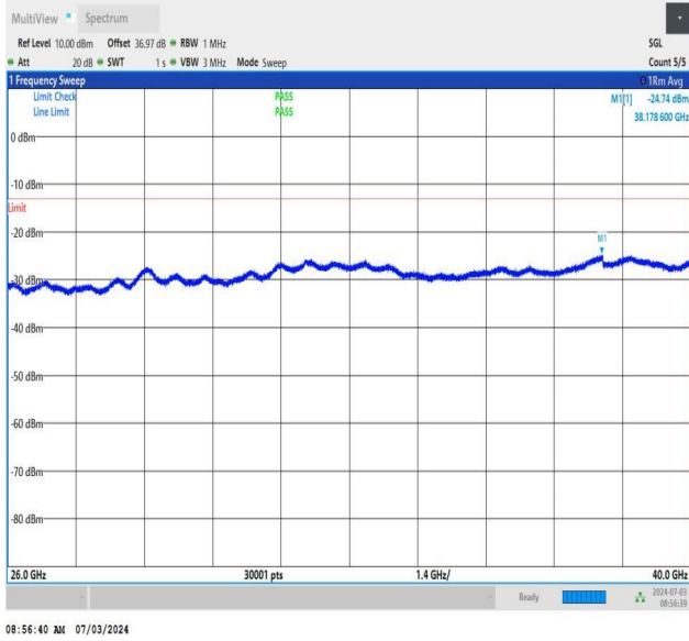
NTNV_DC_26A_n77A-3450-3550_PC2_30_5+30_M+M_TID5_N S_01_26000_40000_#1
