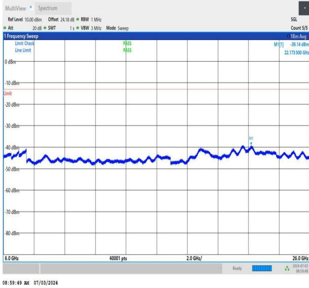
NTNV_DC_26A_n77A-3450-3550_PC2_30_5+30_M+H_TID4_N S_01_6000_26000_#1
