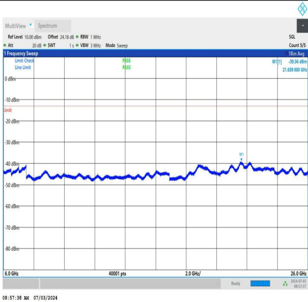
NTNV_DC_26A_n77A-3450-3550_PC2_30_5+30_M+H_TID1_N S_01_6000_26000_#1
