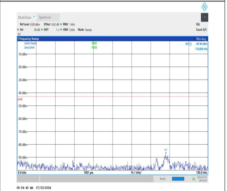
NTNV_DC_26A_n77A-3450-3550_PC2_30_5+30_M+M_TID4_N S_01_0.009_0.15_#1
