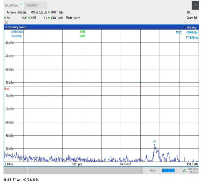
NTNV_DC_26A_n77A-3450-3550_PC2_30_5+30_M+H_TID1_N S_01_0.009_0.15_#1
