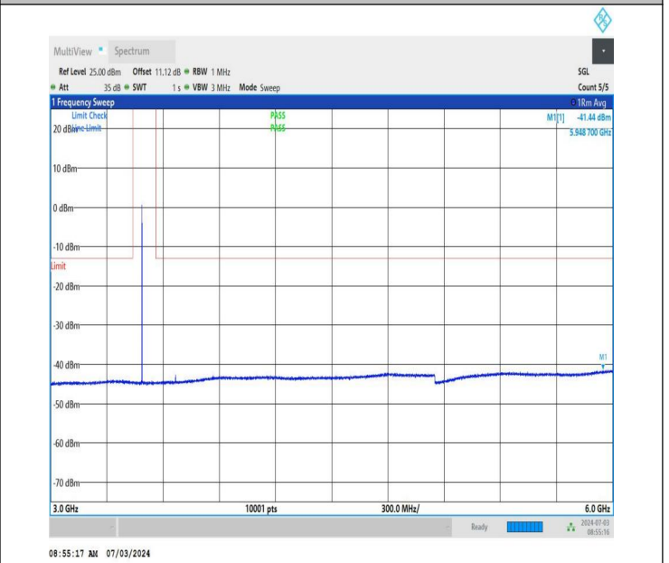
NTNV_DC_26A_n77A-3450-3550_PC2_30_5+30_M+M_TID4_N S_01_3000_6000_#1
