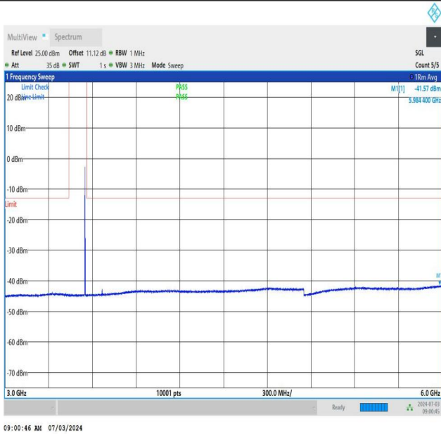
NTNV_DC_26A_n77A-3450-3550_PC2_30_5+30_M+H_TID5_N S_01_3000_6000_#1
