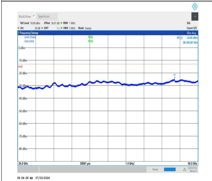
NTNV_DC_26A_n77A-3450-3550_PC2_30_5+30_M+M_TID2_N S_01_26000_40000_#1
