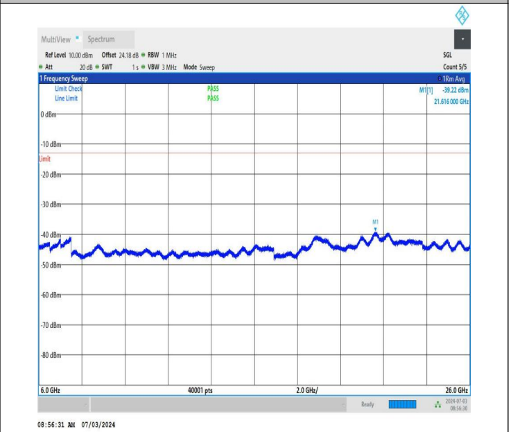
NTNV_DC_26A_n77A-3450-3550_PC2_30_5+30_M+M_TID5_N S_01_6000_26000_#1
