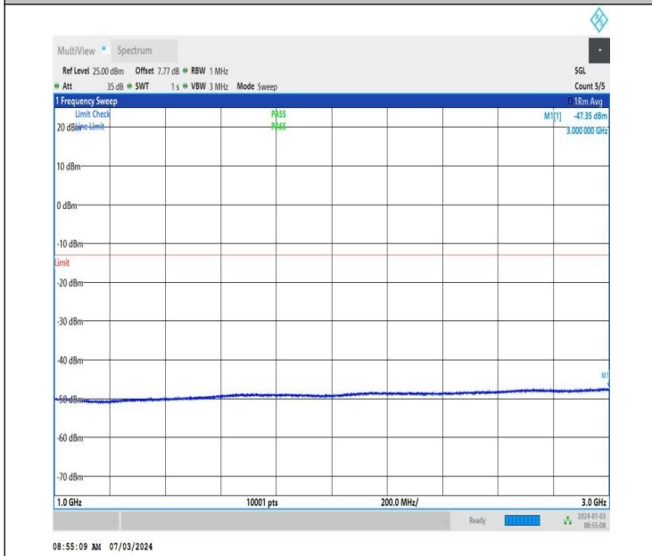
NTNV_DC_26A_n77A-3450-3550_PC2_30_5+30_M+M_TID4_N S_01_1000_3000_#1
