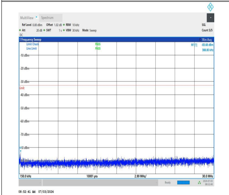
NTNV_DC_26A_n77A-3450-3550_PC2_30_5+30_M+M_TID1_N_S_01_0.15_30_#1
