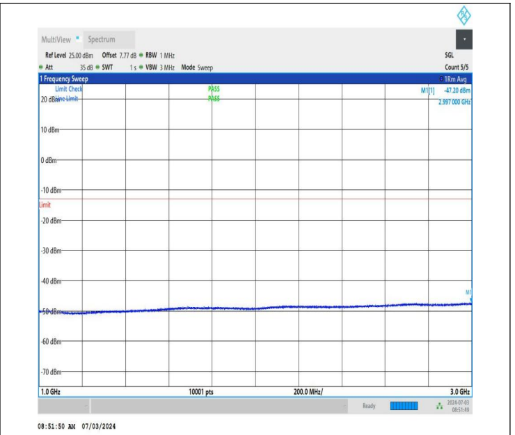
NTNV_DC_26A_n77A-3450-3550_PC2_30_5+30_M+L_TID5_NS_01_1000_3000_#1
