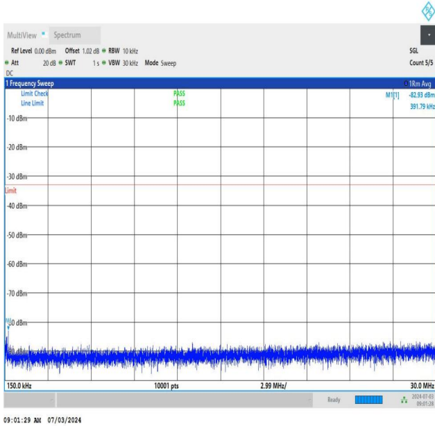
NTNV_DC_26A_n77A-3450-3550_PC2_30_5+40_M+L_TID1_NS _01_0.15_30_#1
