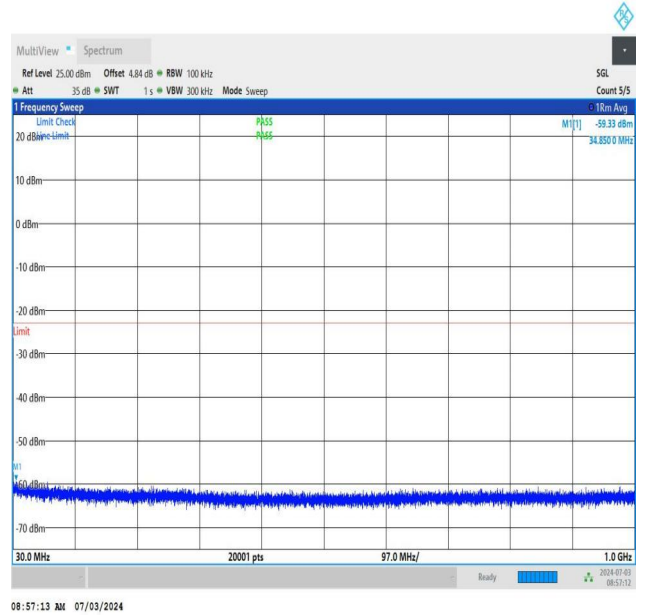
NTNV_DC_26A_n77A-3450-3550_PC2_30_5+30_M+H_TID1_N S_01_30_1000_#1
