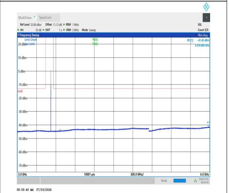
NTNV_DC_26A_n77A-3450-3550_PC2_30_5+30_M+H_TID4_N S_01_3000_6000_#1
