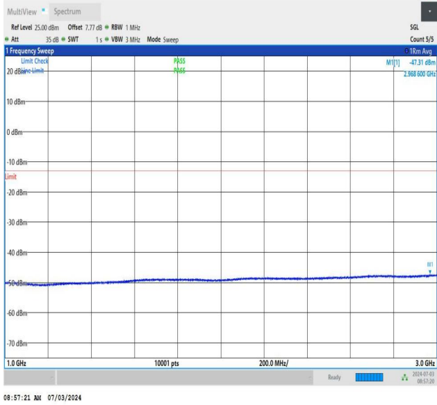
NTNV_DC_26A_n77A-3450-3550_PC2_30_5+30_M+H_TID1_N S_01_1000_3000_#1
