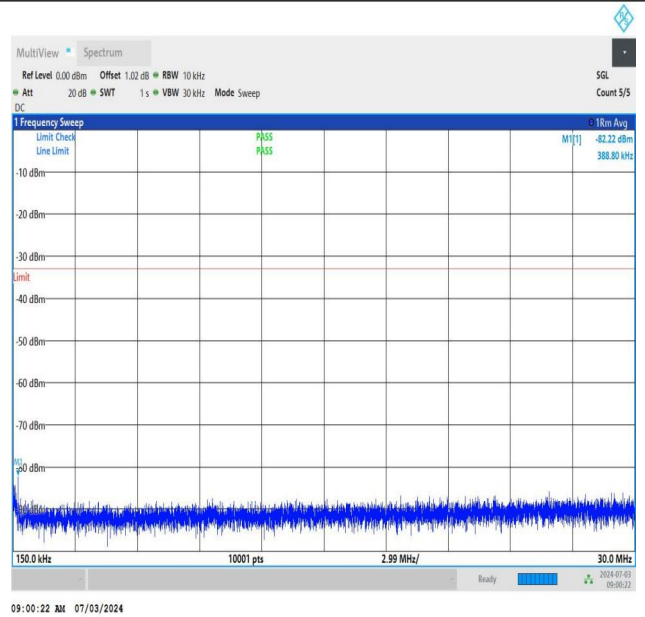
NTNV_DC_26A_n77A-3450-3550_PC2_30_5+30_M+H_TID5_N S_01_0.15_30_#1
