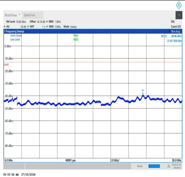
NTNV_DC_26A_n77A-3450-3550_PC2_30_5+30_M+H_TID5_N S_01_6000_26000_#1
