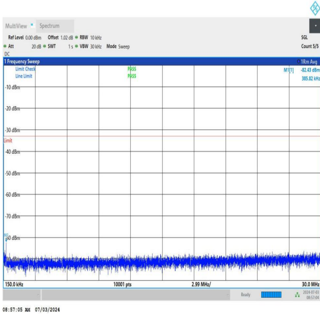
NTNV_DC_26A_n77A-3450-3550_PC2_30_5+30_M+H_TID1_N S_01_0.15_30_#1
