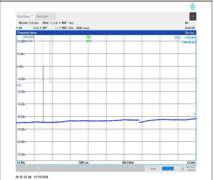
NTNV_DC_26A_n77A-3450-3550_PC2_30_5+30_M+L_TID4_NS_01_3000_6000_#1
