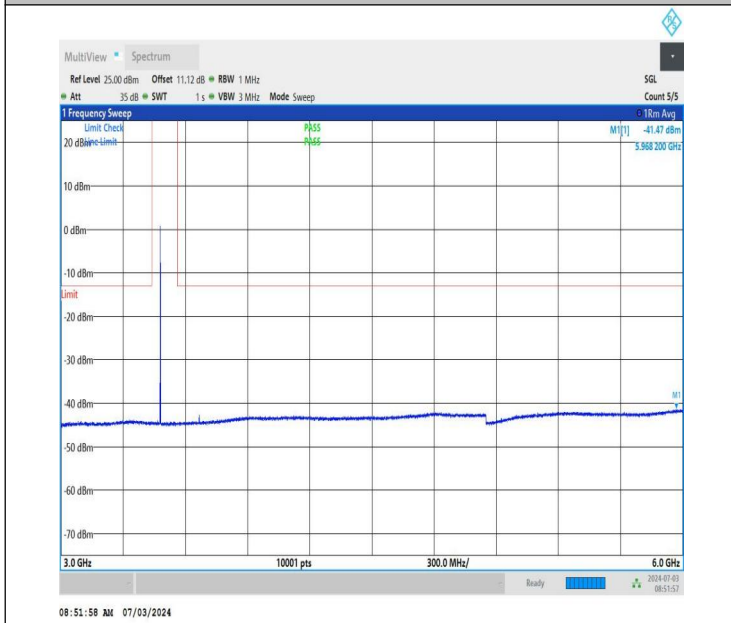
NTNV_DC_26A_n77A-3450-3550_PC2_30_5+30_M+L_TID5_NS_01_3000_6000_#1
