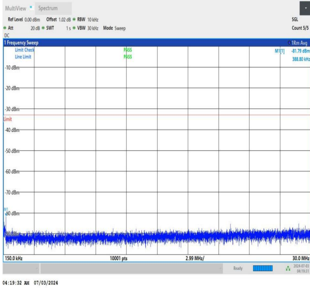
NTNV_DC_26A_n77A-3450-3550_PC2_30_5+20_M+H_TID2_N S_01_0.15_30_#1
