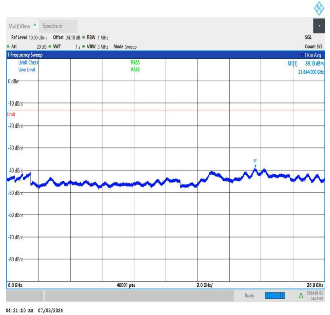
NTNV_DC_26A_n77A-3450-3550_PC2_30_5+20_M+H_TID4_N S_01_6000_26000_#1
