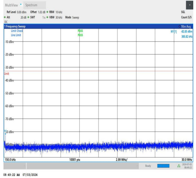
NTNV_DC_26A_n77A-3450-3550_PC2_30_5+30_M+L_TID2_NS_01_0.15_30_#1
