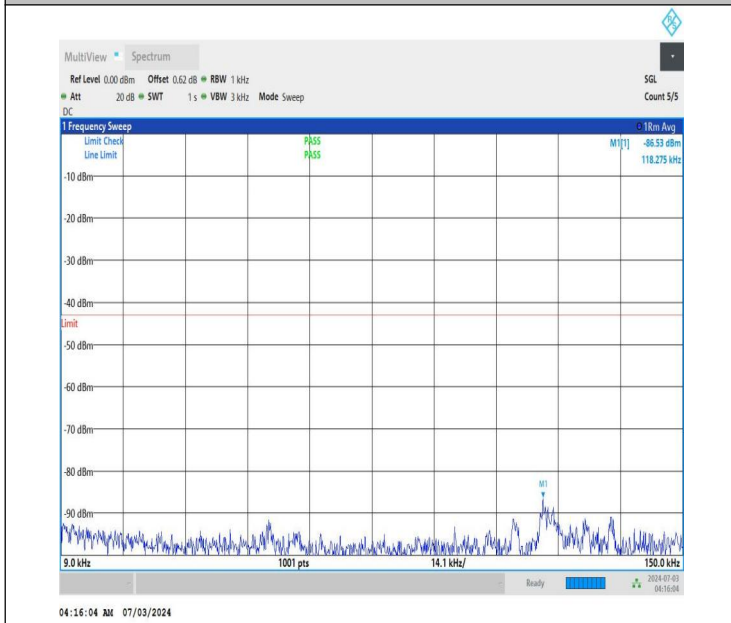
NTNV_DC_26A_n77A-3450-3550_PC2_30_5+20_M+M_TID4_N S_01_0.009_0.15_#1
