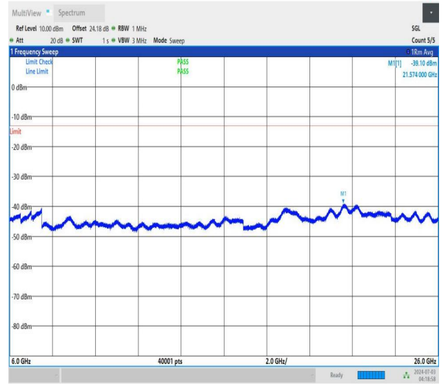
NTNV_DC_26A_n77A-3450-3550_PC2_30_5+20_M+H_TID1_N S_01_6000_26000_#1
