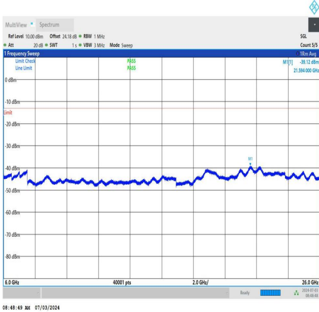
NTNV_DC_26A_n77A-3450-3550_PC2_30_5+30_M+L_TID1_NS_01_6000_26000_#1
