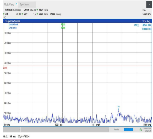
NTNV_DC_26A_n77A-3450-3550_PC2_30_5+20_M+H_TID5_N S_01_0.009_0.15_#1
