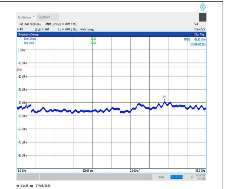
NTNV_DC_26A_n77A-3450-3550_PC2_30_5+20_M+M_TID1_N S_01_6000_26000_#1
