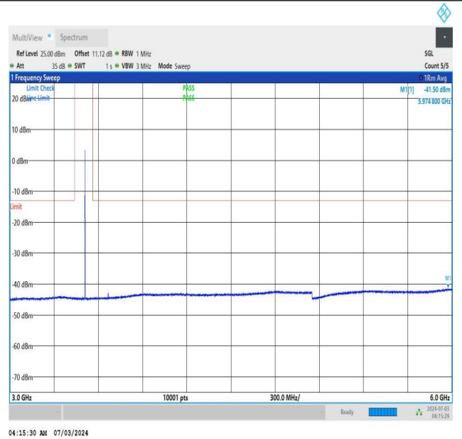
NTNV_DC_26A_n77A-3450-3550_PC2_30_5+20_M+M_TID2_N S_01_3000_6000_#1
