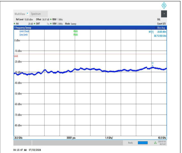
NTNV_DC_26A_n77A-3450-3550_PC2_30_5+20_M+M_TID2_N S_01_26000_40000_#1
