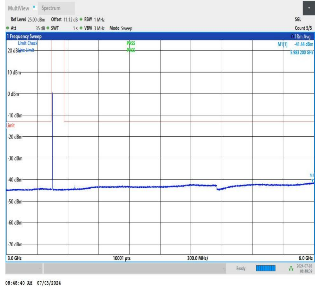
NTNV_DC_26A_n77A-3450-3550_PC2_30_5+30_M+L_TID1_NS_01_3000_6000_#1
