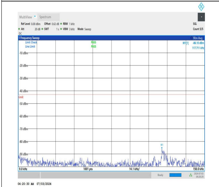
NTNV_DC_26A_n77A-3450-3550_PC2_30_5+20_M+H_TID4_N S_01_0.009_0.15_#1
