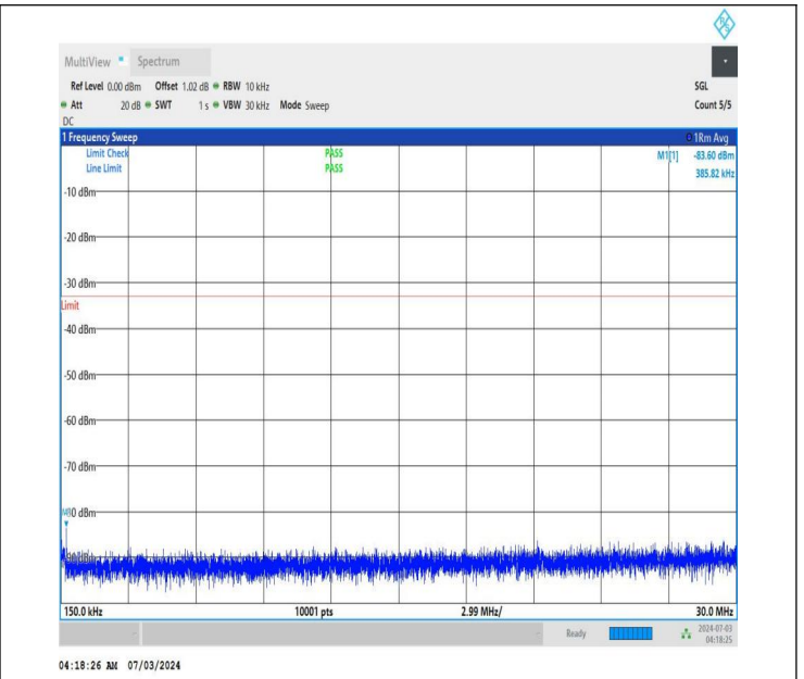
NTNV_DC_26A_n77A-3450-3550_PC2_30_5+20_M+H_TID1_N S_01_0.15_30_#1
