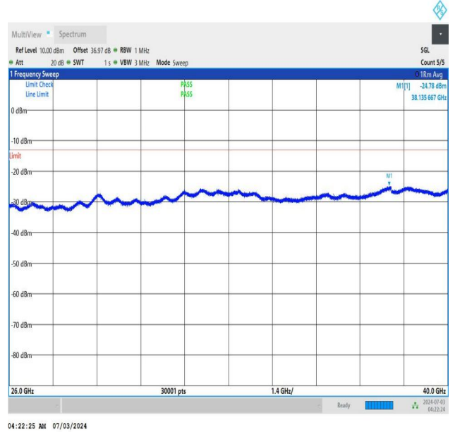
NTNV_DC_26A_n77A-3450-3550_PC2_30_5+20_M+H_TID5_N S_01_26000_40000_#1
