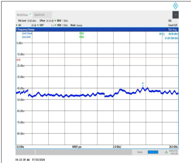
NTNV_DC_26A_n77A-3450-3550_PC2_30_5+20_M+M_TID2_N S_01_6000_26000_#1
