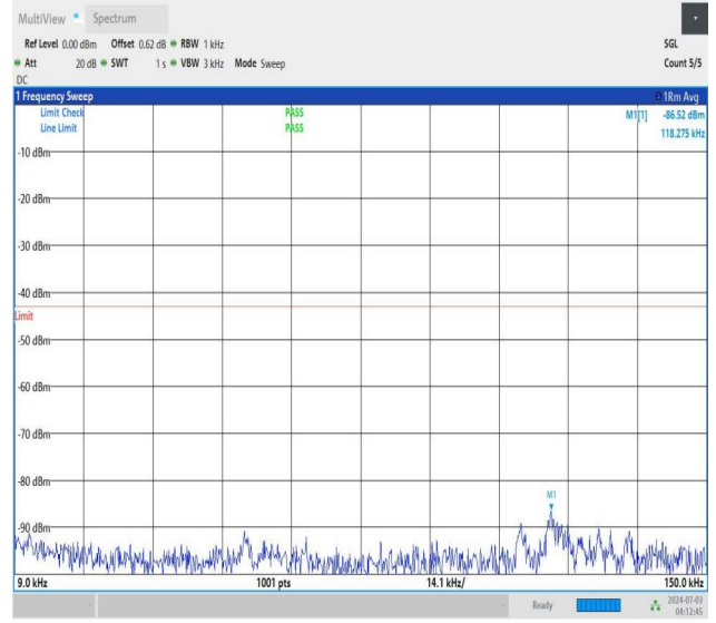
NTNV_DC_26A_n77A-3450-3550_PC2_30_5+20_M+L_TID5_NS_01_0.009_0.15_#1
