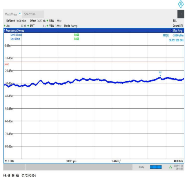
NTNV_DC_26A_n77A-3450-3550_PC2_30_5+30_M+L_TID1_NS_01_26000_40000_#1
