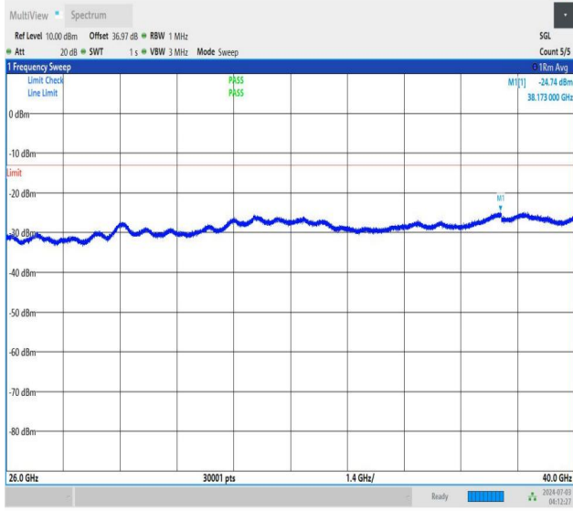
NTNV_DC_26A_n77A-3450-3550_PC2_30_5+20_M+L_TID4_NS_01_26000_40000_#1
