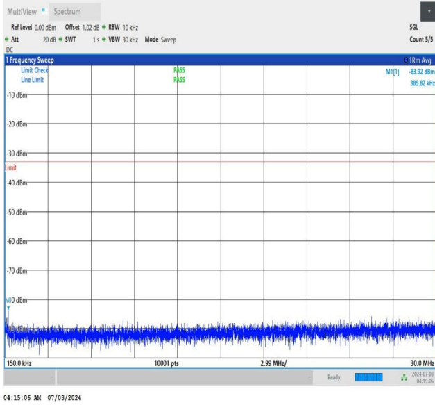
NTNV_DC_26A_n77A-3450-3550_PC2_30_5+20_M+M_TID2_N S_01_0.15_30_#1
