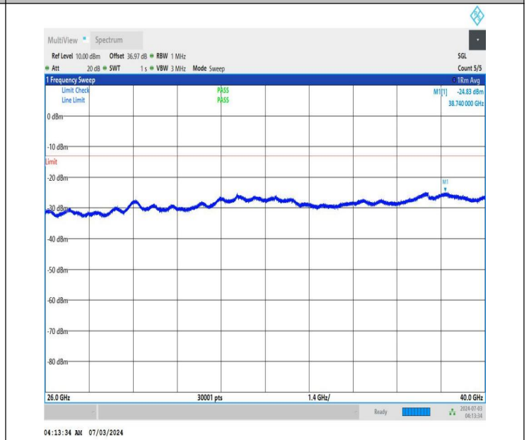
NTNV_DC_26A_n77A-3450-3550_PC2_30_5+20_M+L_TID5_NS_01_26000_40000_#1
