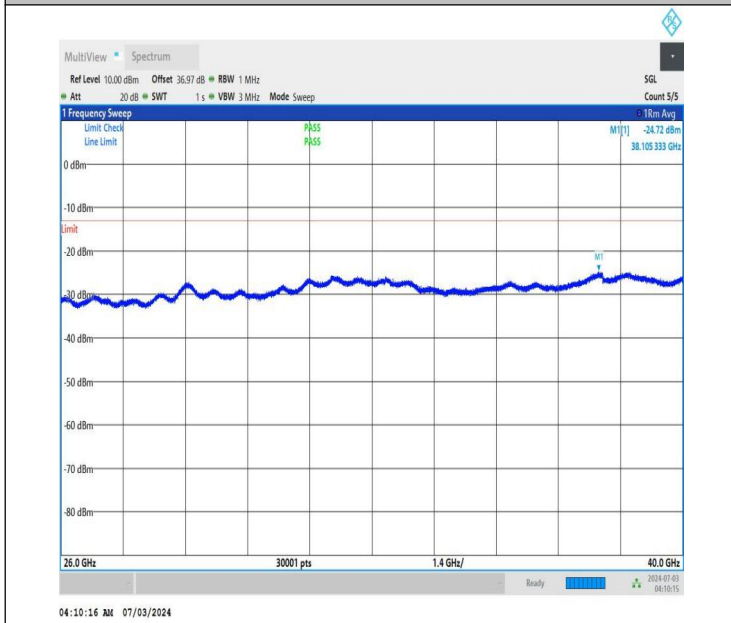
NTNV_DC_26A_n77A-3450-3550_PC2_30_5+20_M+L_TID1_NS_01_26000_40000_#1
