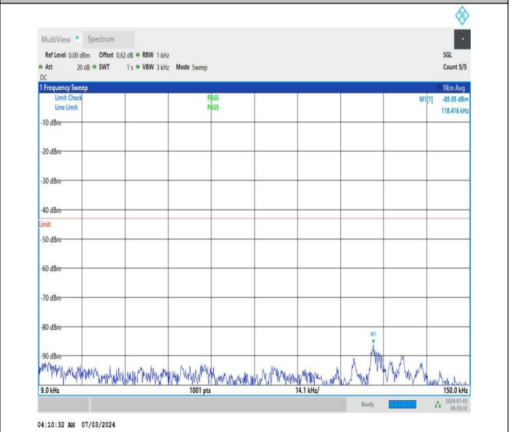
NTNV_DC_26A_n77A-3450-3550_PC2_30_5+20_M+L_TID2_NS_01_0.009_0.15_#1
