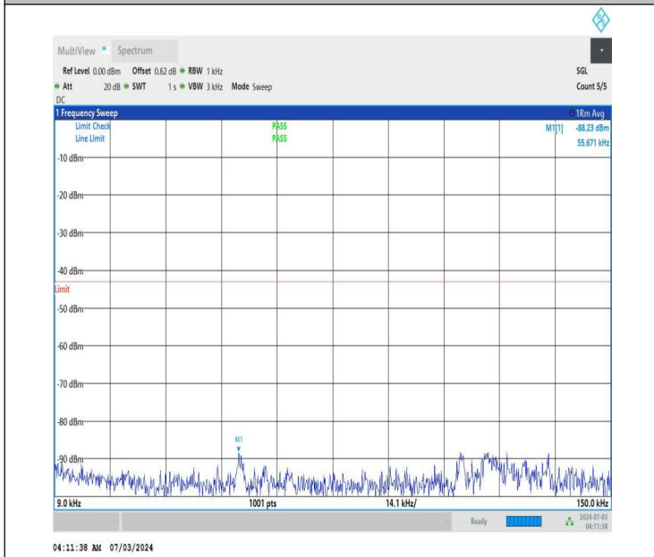
NTNV_DC_26A_n77A-3450-3550_PC2_30_5+20_M+L_TID4_NS_01_0.009_0.15_#1
