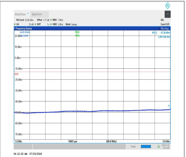
NTNV_DC_26A_n77A-3450-3550_PC2_30_5+20_M+L_TID4_NS_01_1000_3000_#1
