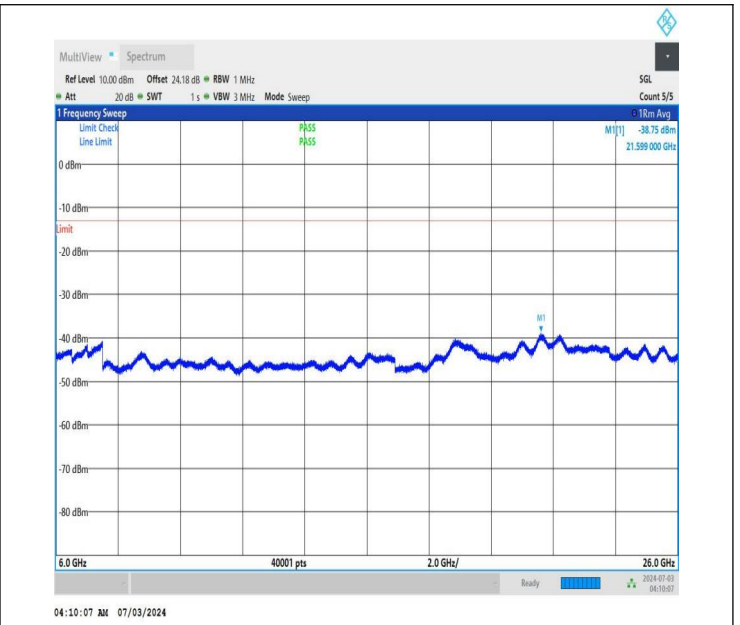
NTNV_DC_26A_n77A-3450-3550_PC2_30_5+20_M+L_TID1_NS_01_6000_26000_#1
