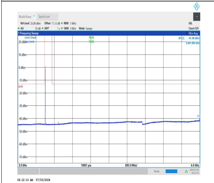
NTNV_DC_26A_n77A-3450-3550_PC2_30_5+20_M+L_TID4_NS_01_3000_6000_#1
