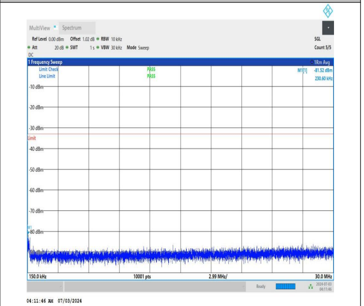
NTNV_DC_26A_n77A-3450-3550_PC2_30_5+20_M+L_TID4_NS_01_0.15_30_#1
