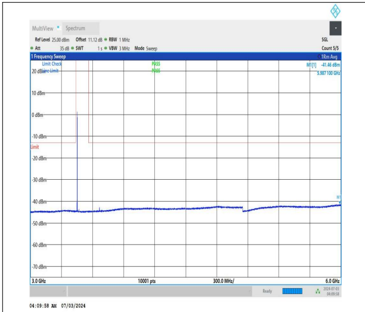
NTNV_DC_26A_n77A-3450-3550_PC2_30_5+20_M+L_TID1_NS_01_3000_6000_#1
