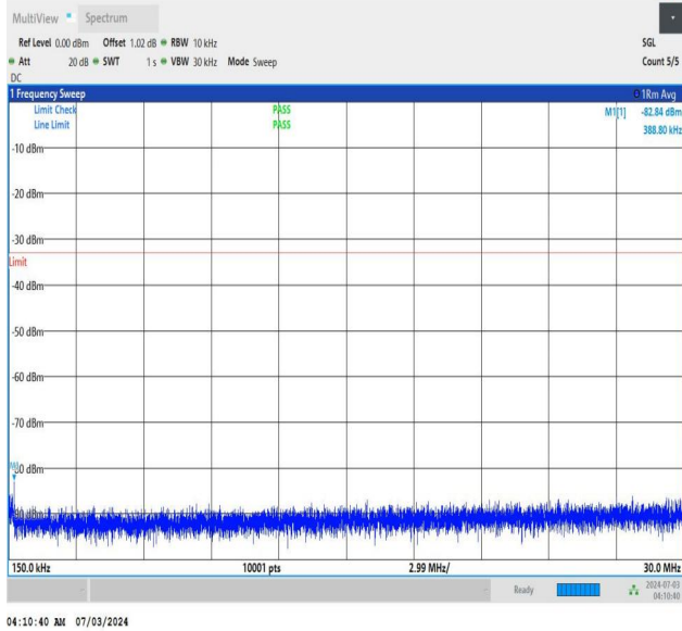
NTNV_DC_26A_n77A-3450-3550_PC2_30_5+20_M+L_TID2_NS _01_0.15_30_#1
