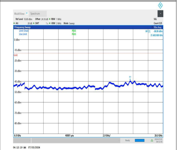
NTNV_DC_26A_n77A-3450-3550_PC2_30_5+20_M+L_TID4_NS_01_6000_26000_#1
