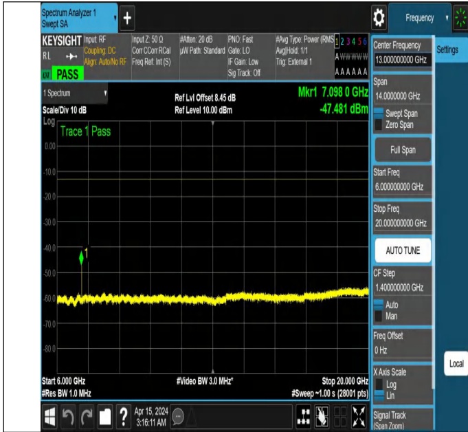
NTNV_N77-3450-3550_PC2_30_60_H_TID3_NS_01_6000_2000
