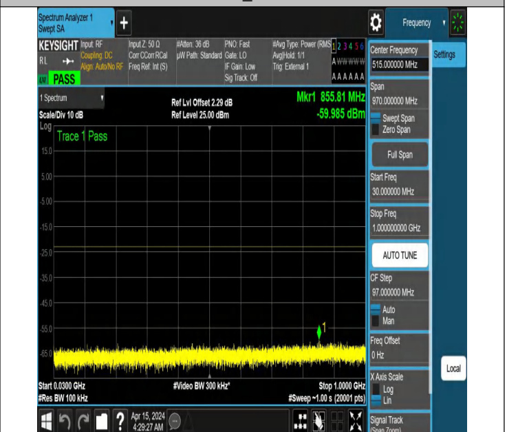
NTNV_N77-3450-3550_PC2_30_80_M_TID6_NS_01_30_1000_ #1
