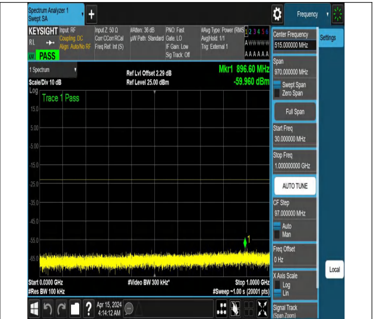
NTNV_N77-3450-3550_PC2_30_80_M_TID3_NS_01_30_1000_#1
