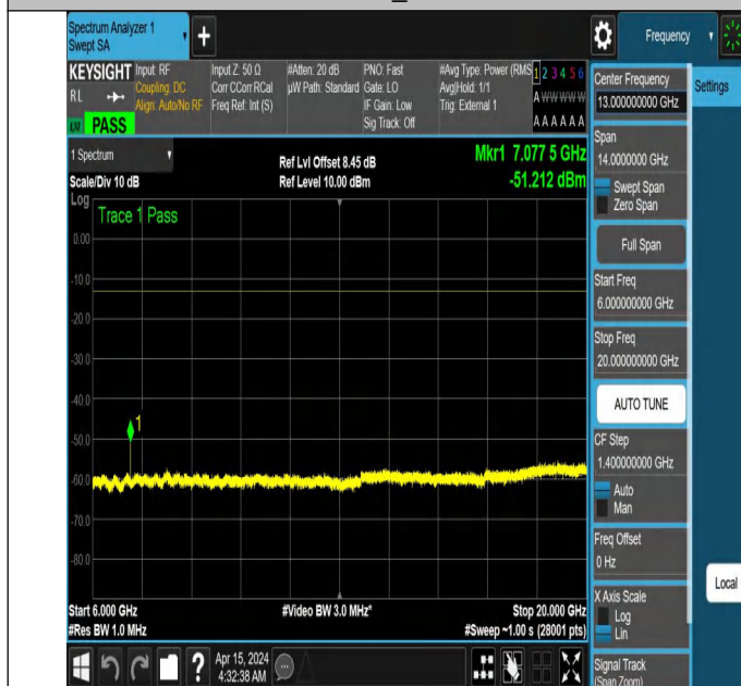
NTNV_N77-3450-3550_PC2_30_80_M_TID6_NS_01_6000_200 00 #1
