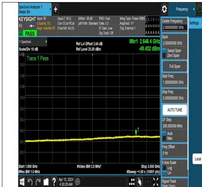
NTNV_N77-3450-3550_PC2_30_80_M_TID6_NS_01_1000_300 0 #1
