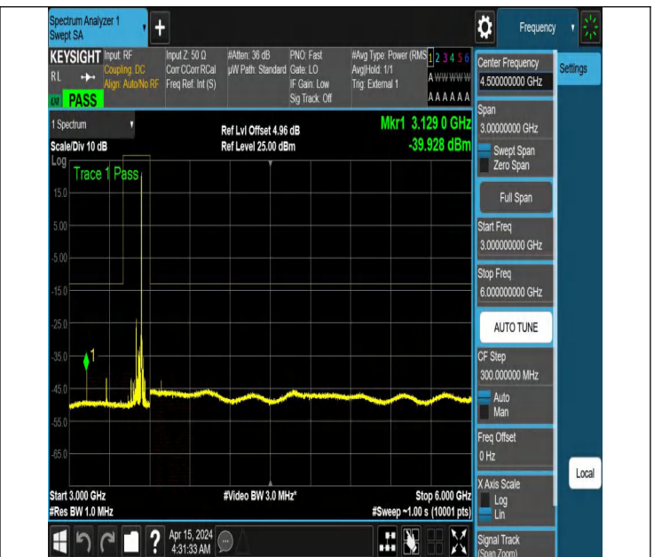
NTNV_N77-3450-3550_PC2_30_80_M_TID6_NS_01_3000_600
