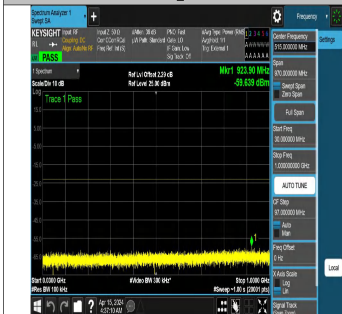
NTNV_N77-3450-3550_PC2_30_80_H_TID2_NS_01_30_1000_#
