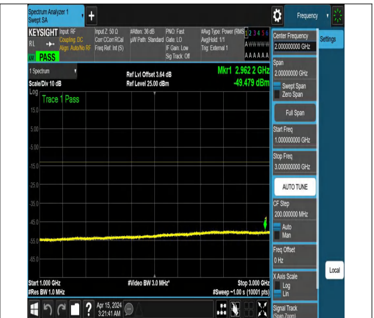
NTNV_N77-3450-3550_PC2_30_60_H_TID5_NS_01_1000_3000
