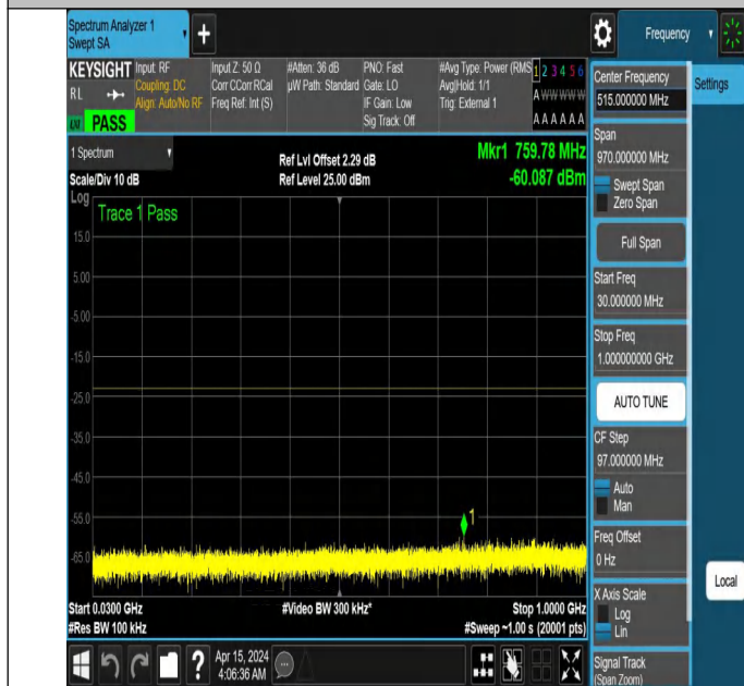
NTNV_N77-3450-3550_PC2_30_80_M_TID2_NS_01_30_1000_
