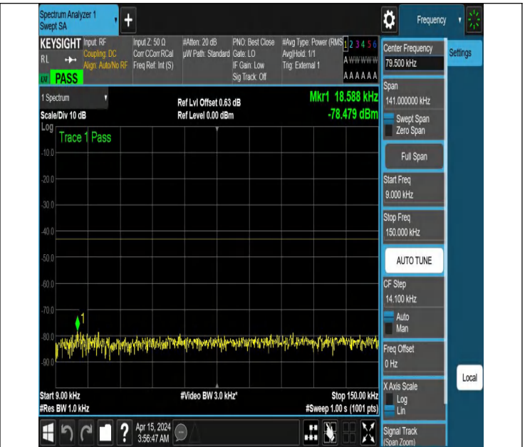
NTNV_N77-3450-3550_PC2_30_80_L_TID6_NS_01_0.009_0.15
