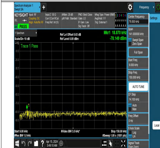
NTNV_N77-3450-3550_PC2_30_80_L_TID5_NS_01_0.009_0.15
