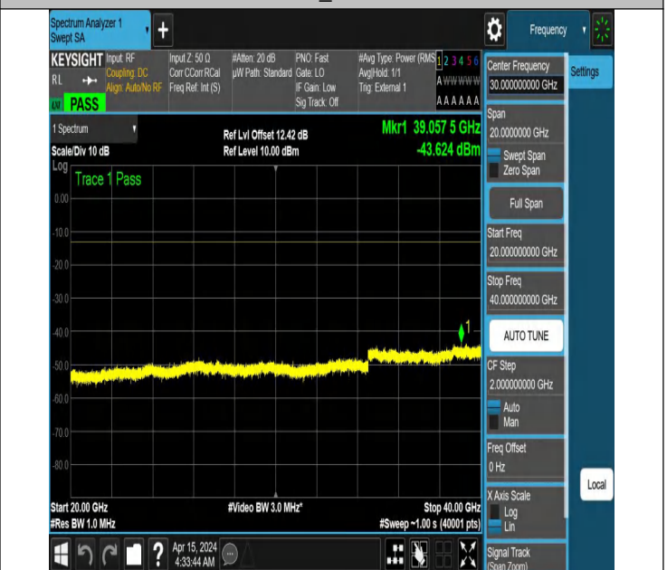
NTNV_N77-3450-3550_PC2_30_80_M_TID6_NS_01_20000_40 000 #1
