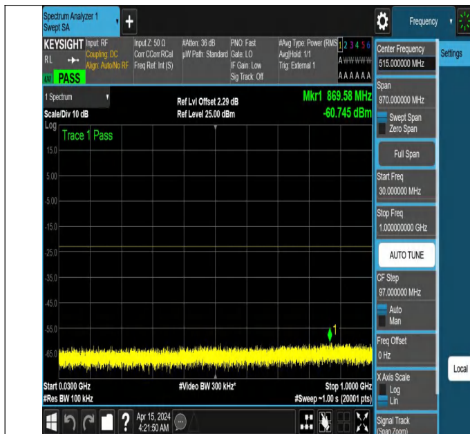
NTNV_N77-3450-3550_PC2_30_80_M_TID5_NS_01_30_1000_#1
