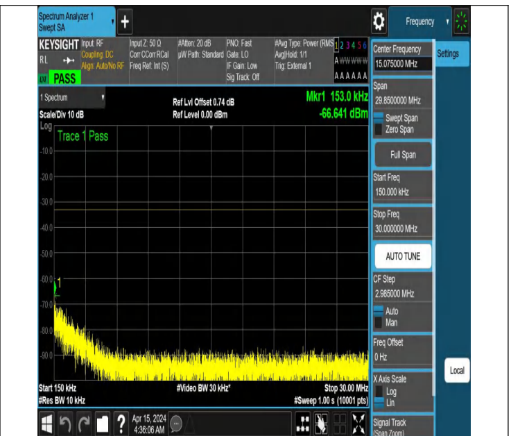
NTNV_N77-3450-3550_PC2_30_80_H_TID2_NS_01_0.15_30_#
