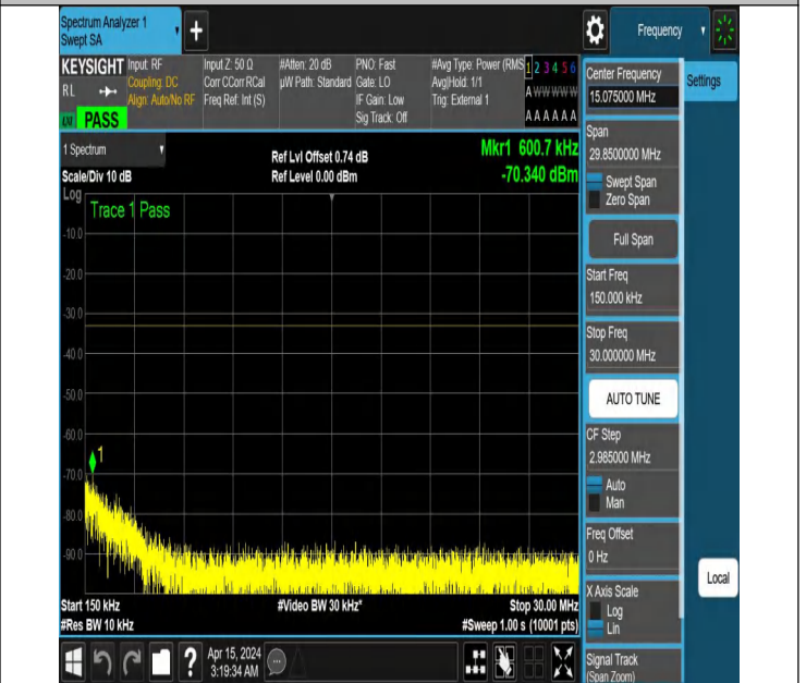
NTNV_N77-3450-3550_PC2_30_60_H_TID5_NS_01_0.15_30_#
