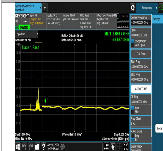
NTNV_N77-3450-3550_PC2_30_80_M_TID5_NS_01_3000_600 0 #1
