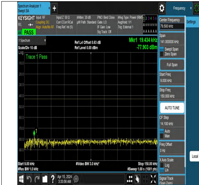
NTNV_N77-3450-3550_PC2_30_80_L_TID2_NS_01_0.009_0.15
