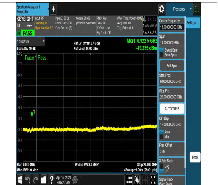
NTNV_N77-3450-3550_PC2_30_80_M_TID2_NS_01_6000_200 00 #1
