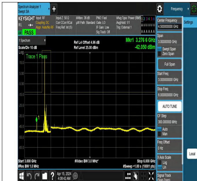
NTNV_N77-3450-3550_PC2_30_80_M_TID2_NS_01_3000_600 0 #1
