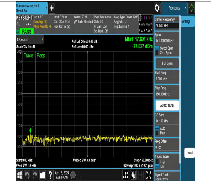
NTNV_N77-3450-3550_PC2_30_60_H_TID6_NS_01_0.009_0.15
