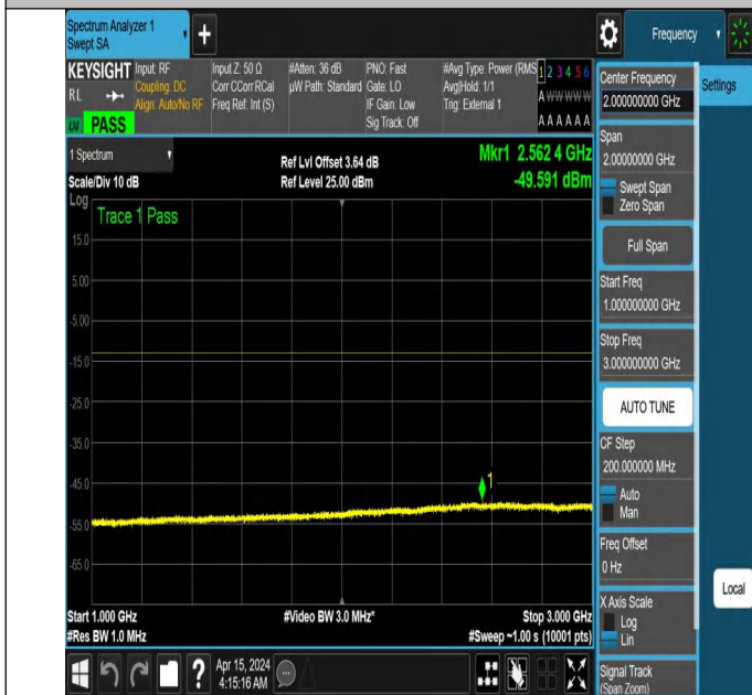
NTNV_N77-3450-3550_PC2_30_80_M_TID3_NS_01_1000_300
