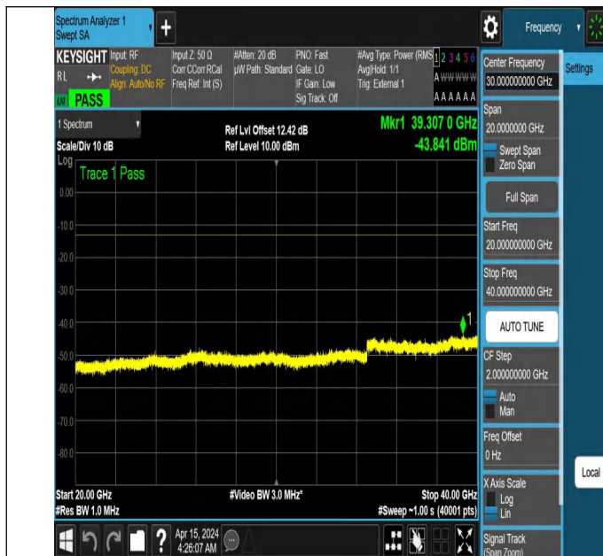
NTNV_N77-3450-3550_PC2_30_80_M_TID5_NS_01_20000_40 000 #1
