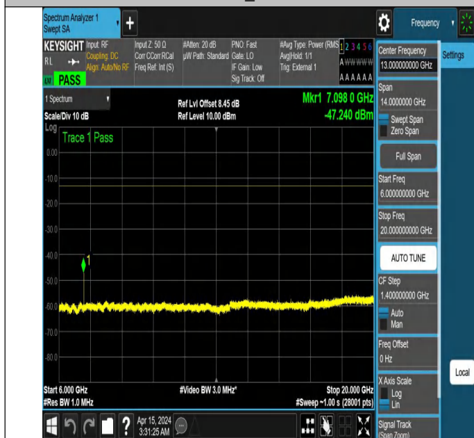
NTNV_N77-3450-3550_PC2_30_60_H_TID6_NS_01_6000_2000
