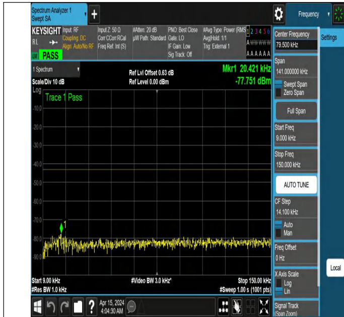
NTNV_N77-3450-3550_PC2_30_80_M_TID2_NS_01_0.009_0.1
