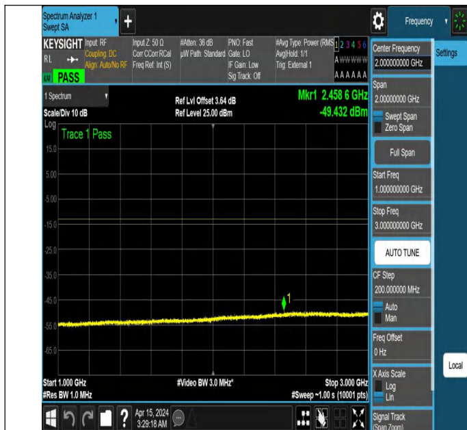
NTNV_N77-3450-3550_PC2_30_60_H_TID6 NS_01_1000_3000
