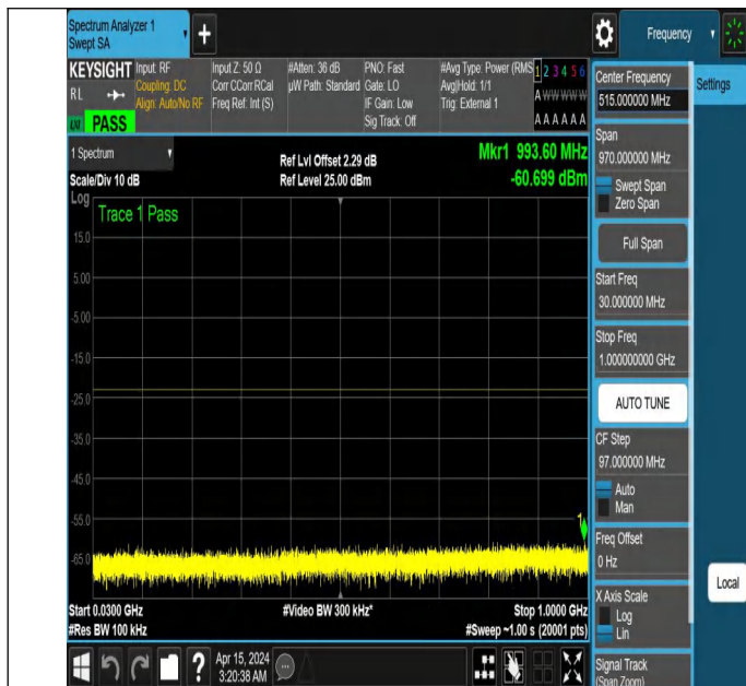
NTNV_N77-3450-3550_PC2_30_60_H_TID5 NS_01_30_1000_#
