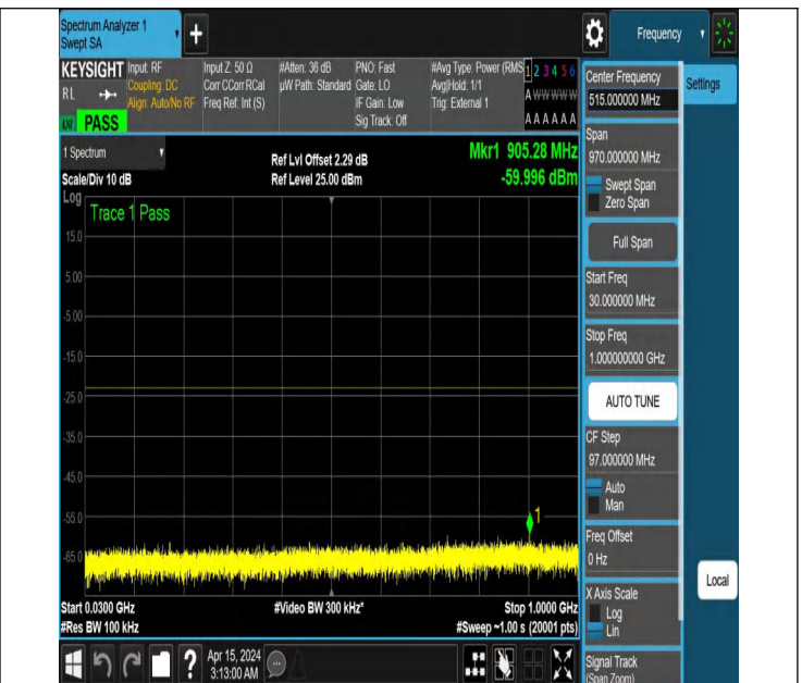
NTNV_N77-3450-3550_PC2_30_60_H_TID3_NS_01_30_1000_#
