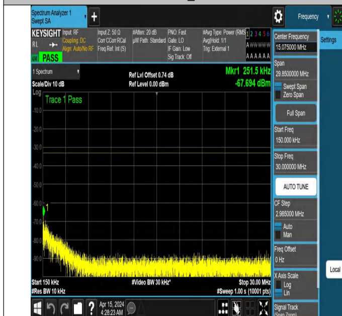
NTNV_N77-3450-3550_PC2_30_80_M_TID6_NS_01_0.15_30_#
