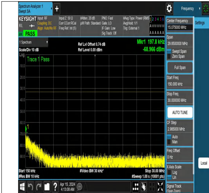
NTNV_N77-3450-3550_PC2_30_80_M_TID3_NS_01_0.15_30_#
