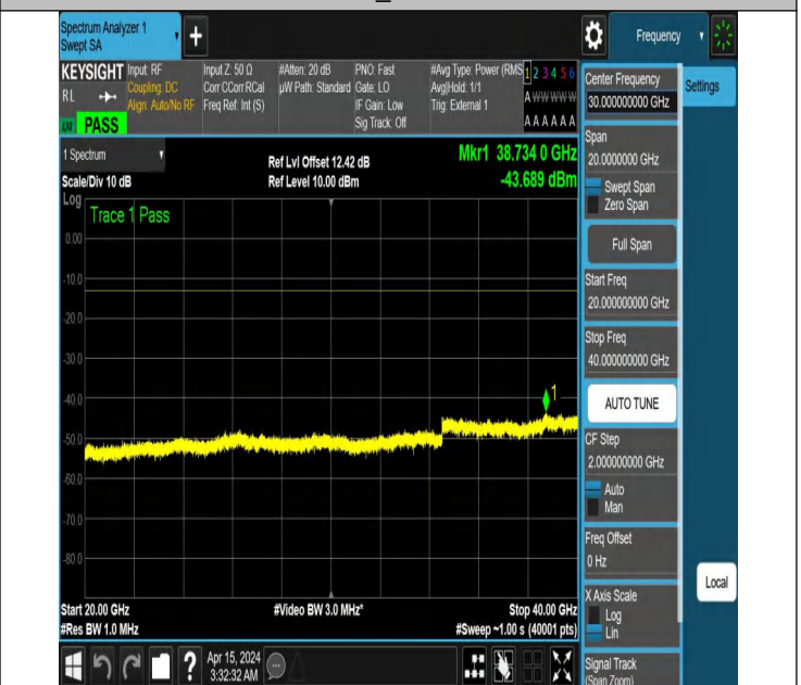
NTNV_N77-3450-3550_PC2_30_60_H_TID6_NS_01_20000_400
