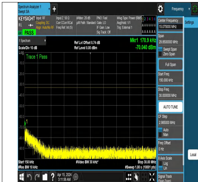
NTNV_N77-3450-3550_PC2_30_60_H_TID3_NS_01_0.15_30_#
