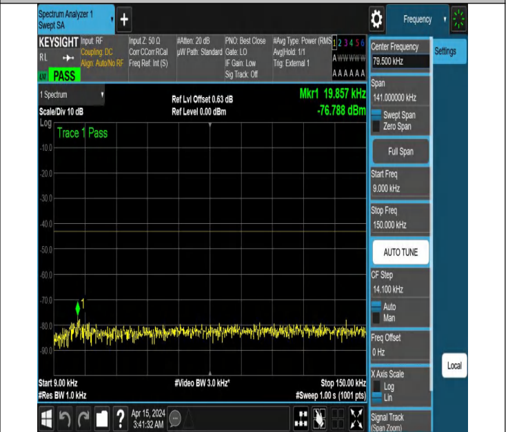
NTNV_N77-3450-3550_PC2_30_80_L_TID3_NS_01_0.009_0.15
