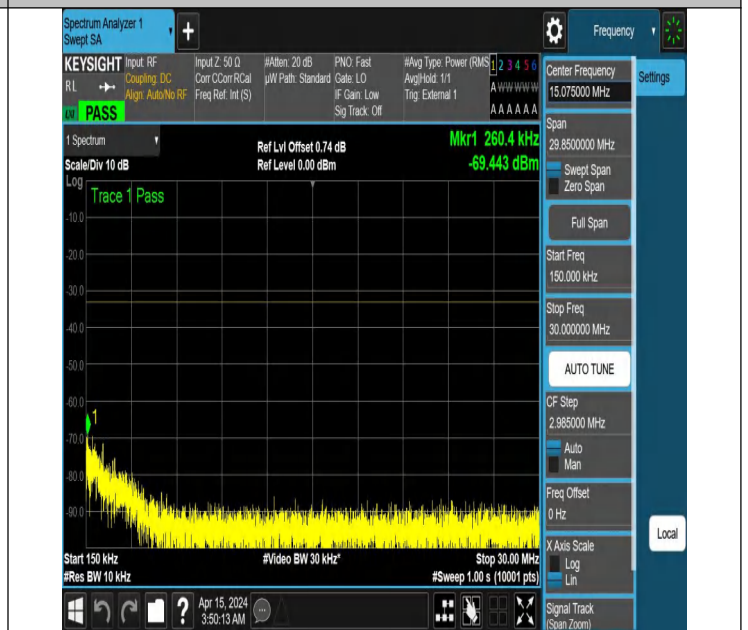
NTNV_N77-3450-3550_PC2_30_80_L_TID5_NS_01_0.15_30_#
