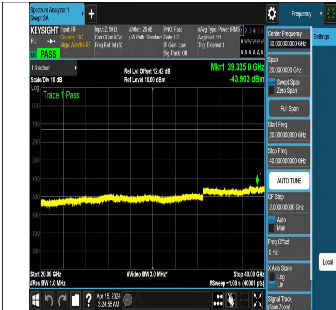
NTNV_N77-3450-3550_PC2_30_60_H_TID5_NS_01_20000_400
