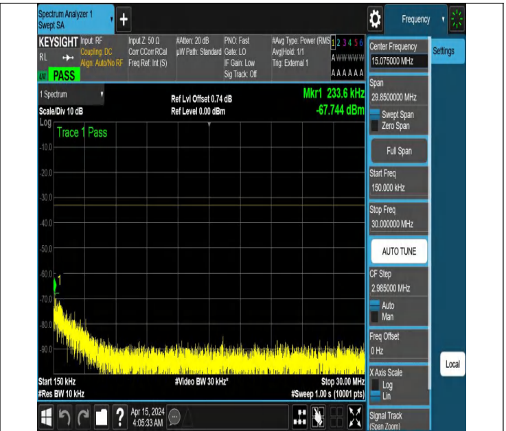
NTNV_N77-3450-3550_PC2_30_80_M_TID2_NS_01_0.15_30_#
