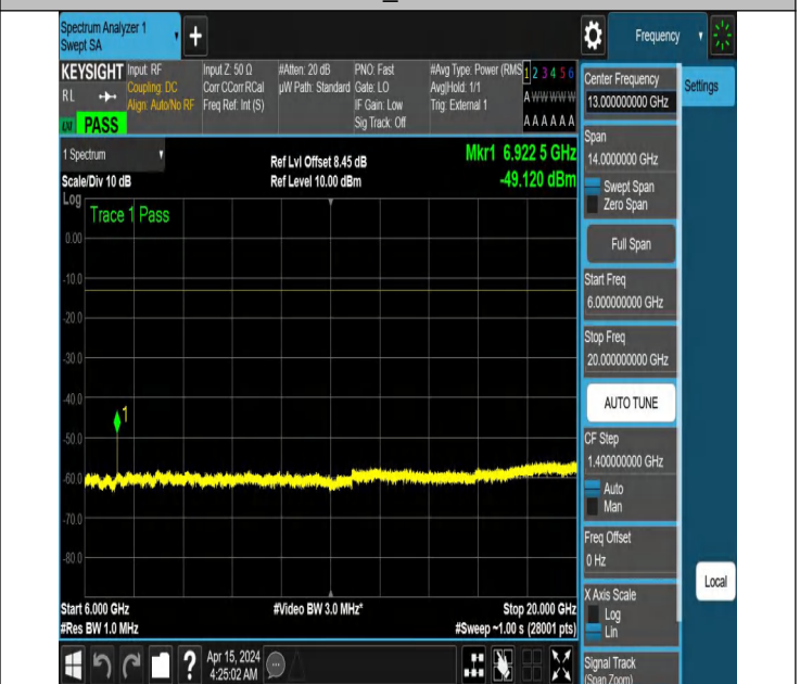
NTNV_N77-3450-3550_PC2_30_80_M_TID5_NS_01_6000_200 00 #1
