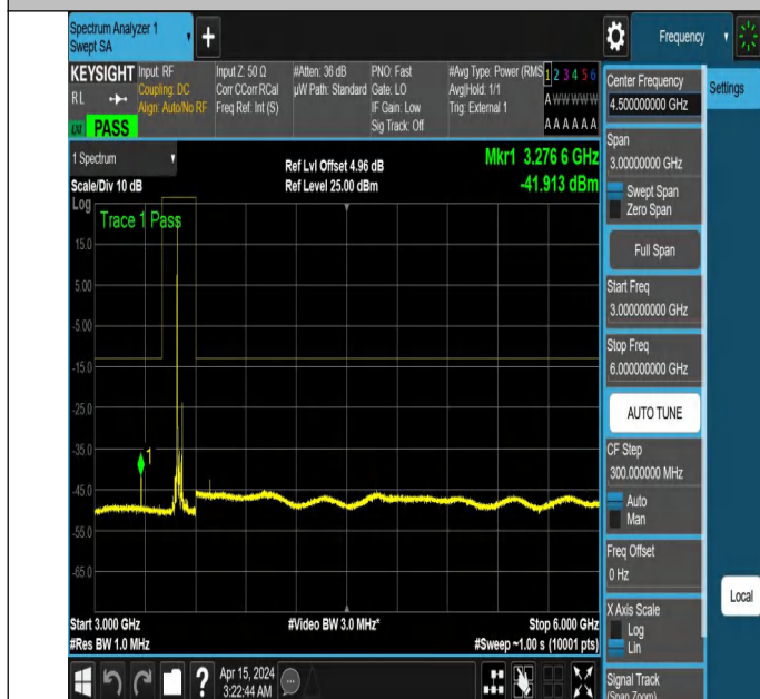
NTNV_N77-3450-3550_PC2_30_60_H_TID5_NS_01_3000_6000
