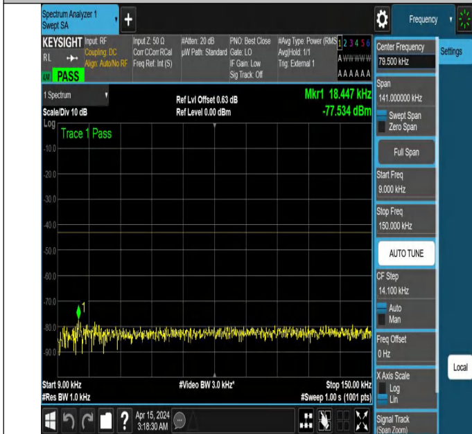
NTNV_N77-3450-3550_PC2_30_60_H_TID5_NS_01_0.009_0.15
