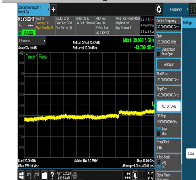
NTNV_N77-3450-3550_PC2_30_80_M_TID2_NS_01_20000_40 000 #1
