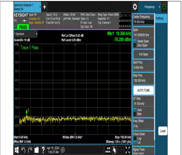
NTNV_N77-3450-3550_PC2_30_50_H_TID6_NS_01_0.009_0.15
