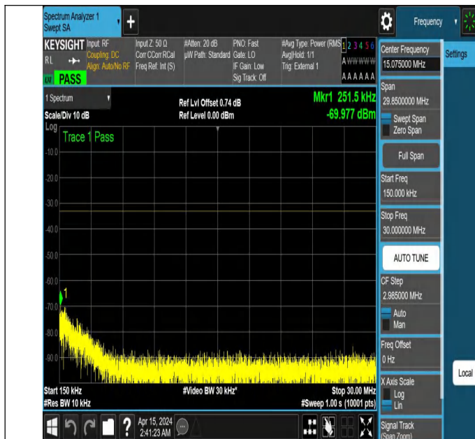
NTNV_N77-3450-3550_PC2_30_60_M_TID3_NS_01_0.15_30_#
