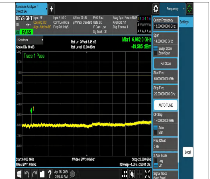
NTNV_N77-3450-3550_PC2_30_60_H_TID2_NS_01_6000_2000
