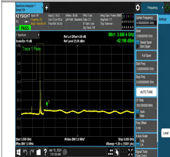
NTNV_N77-3450-3550_PC2_30_50_H_TID5_NS_01_3000_6000
