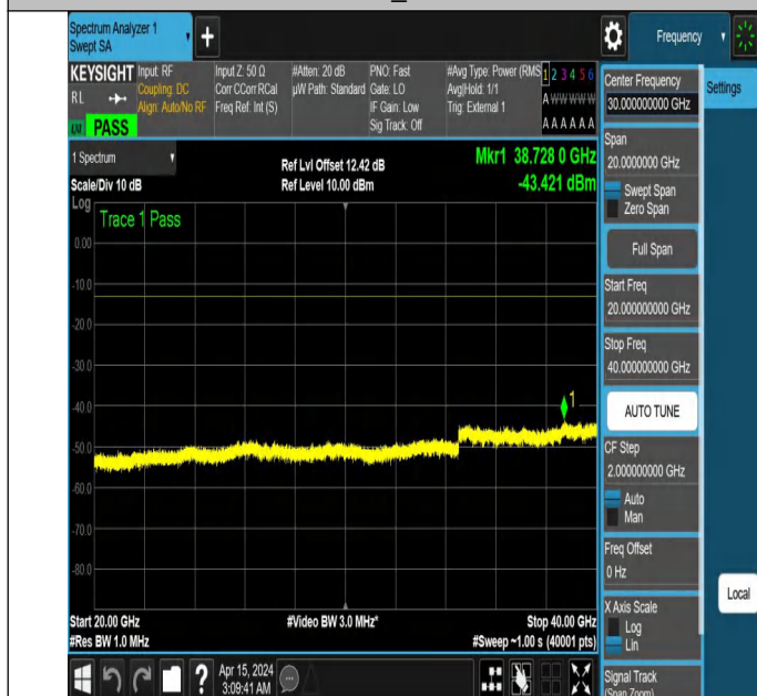
NTNV_N77-3450-3550_PC2_30_60_H_TID2_NS_01_20000_400
