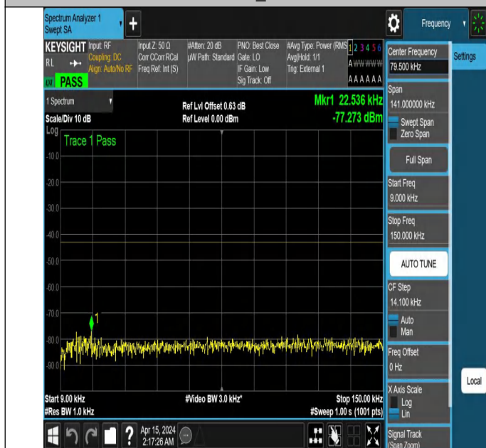
NTNV_N77-3450-3550_PC2_30_60_L_TID5_NS_01_0.009_0.15 #1
