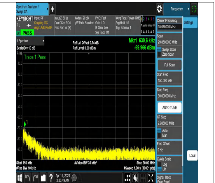
NTNV_N77-3450-3550_PC2_30_60_M_TID2_NS_01_0.15_30_#
