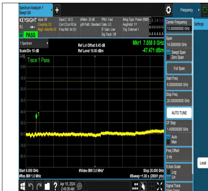
NTNV_N77-3450-3550_PC2_30_60_M_TID3_NS_01_6000_200 00 #1
