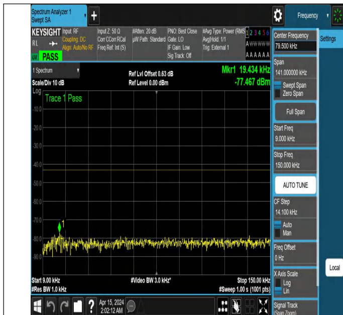
NTNV_N77-3450-3550_PC2_30_60_L_TID2_NS_01_0.009_0.15
