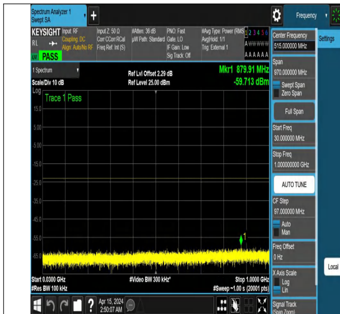
NTNV_N77-3450-3550_PC2_30_60_M_TID5_NS_01_30_1000_#1
