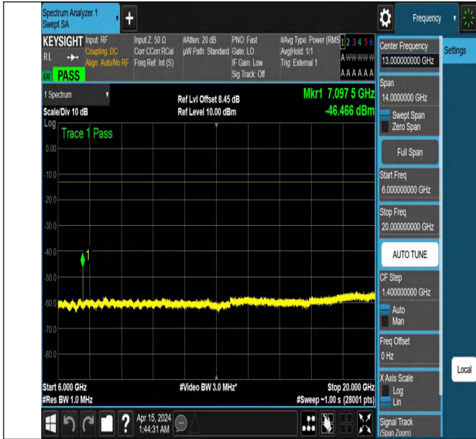
NTNV_N77-3450-3550_PC2_30_50_H_TID3_NS_01_6000_2000
