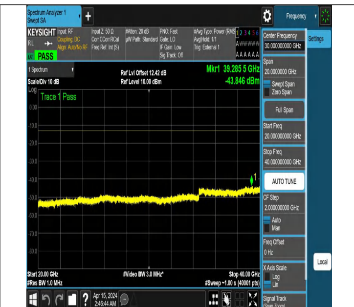
NTNV_N77-3450-3550_PC2_30_60_M_TID3_NS_01_20000_40 000 #1
