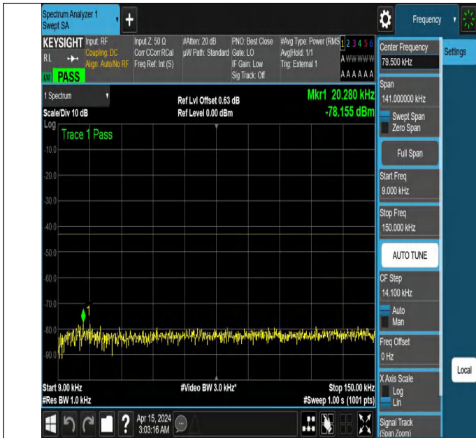
NTNV_N77-3450-3550_PC2_30_60_H_TID2_NS_01_0.009_0.15
