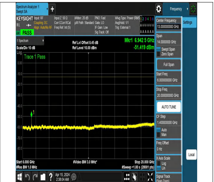
NTNV_N77-3450-3550_PC2_30_60_M_TID2_NS_01_6000_200 00 #1
