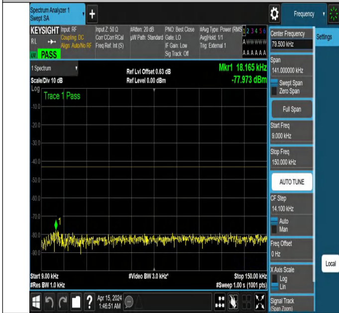
NTNV_N77-3450-3550_PC2_30_50_H_TID5_NS_01_0.009_0.15
