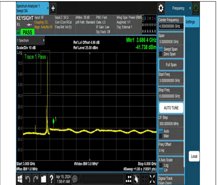
NTNV_N77-3450-3550_PC2_30_50_H_TID6_NS_01_3000_6000
