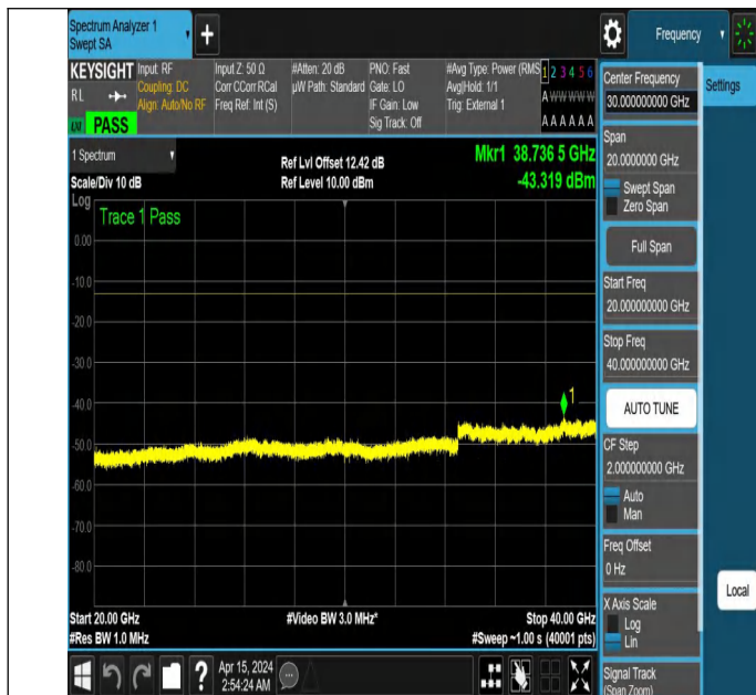
NTNV_N77-3450-3550_PC2_30_60_M_TID5_NS_01_20000_40 000 #1
