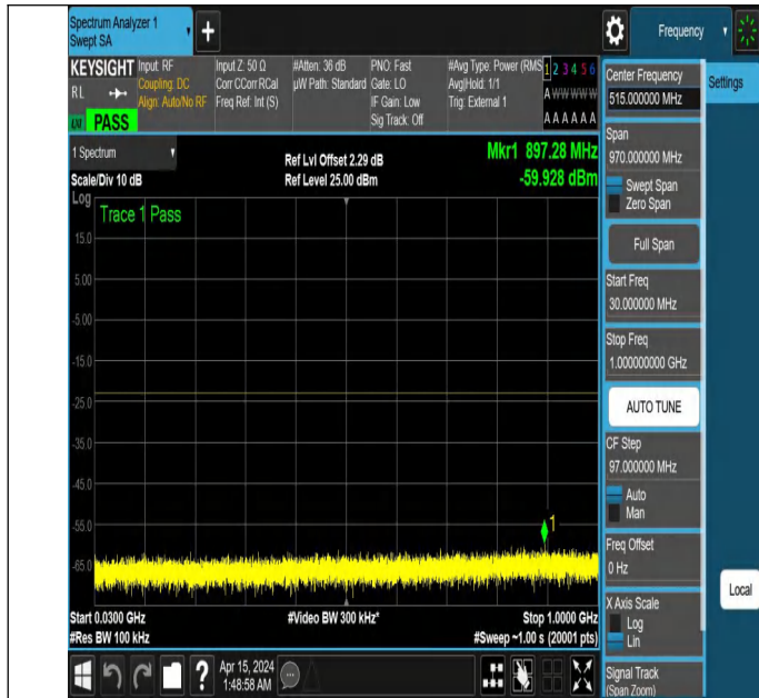
NTNV_N77-3450-3550_PC2_30_50_H_TID5_NS_01_30_1000_#
