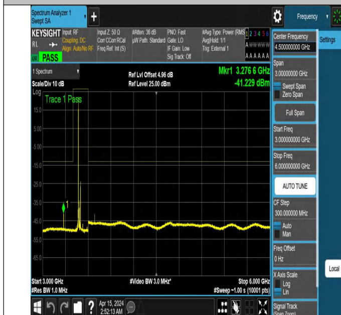
NTNV_N77-3450-3550_PC2_30_60_M_TID5_NS_01_3000_600
