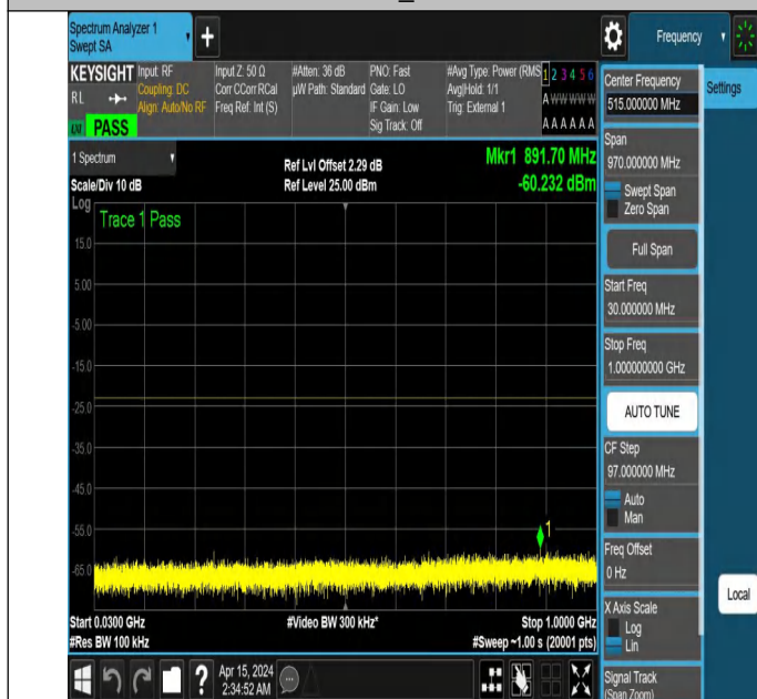
NTNV_N77-3450-3550_PC2_30_60_M_TID2_NS_01_30_1000_#1
