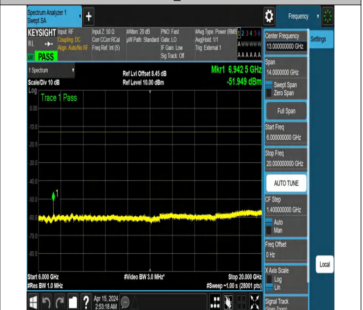
NTNV_N77-3450-3550_PC2_30_60_M_TID5_NS_01_6000_200 00 #1
