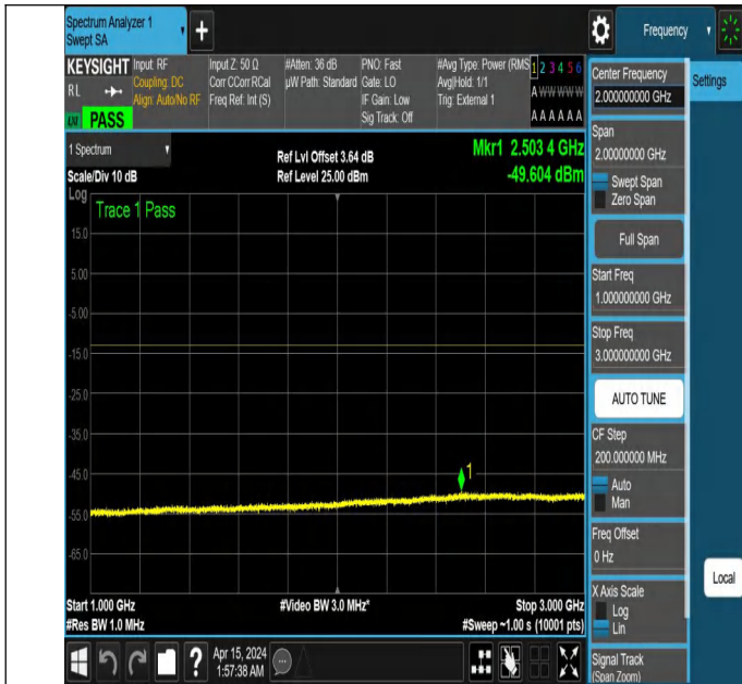
NTNV_N77-3450-3550_PC2_30_50_H_TID6_NS_01_1000_3000
