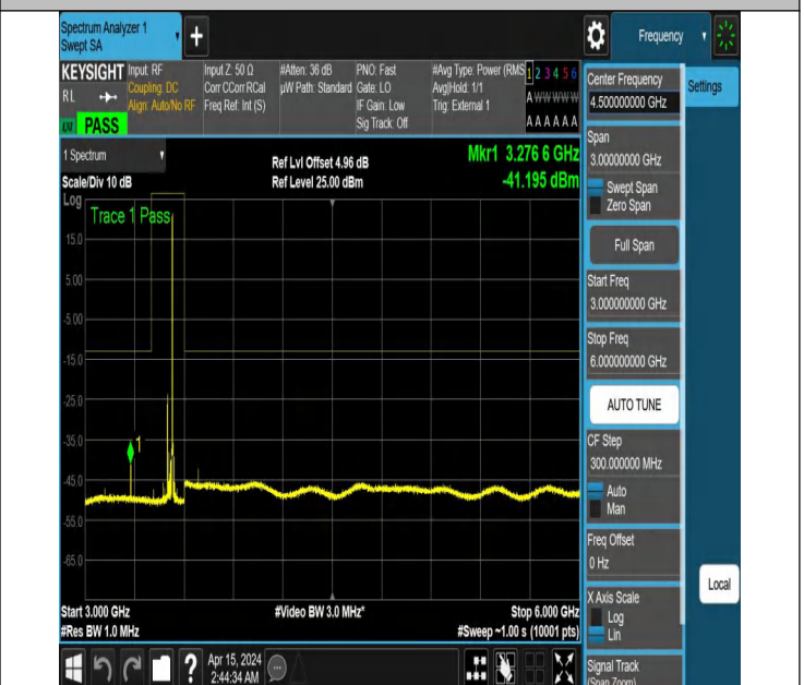
NTNV_N77-3450-3550_PC2_30_60_M_TID3_NS_01_3000_600
