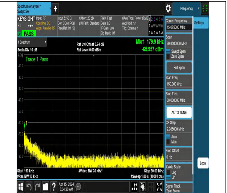
NTNV_N77-3450-3550_PC2_30_60_H_TID2_NS_01_0.15_30_#
