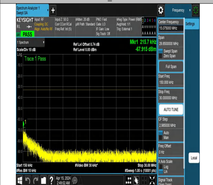
NTNV_N77-3450-3550_PC2_30_60_M_TID5_NS_01_0.15_30_#
