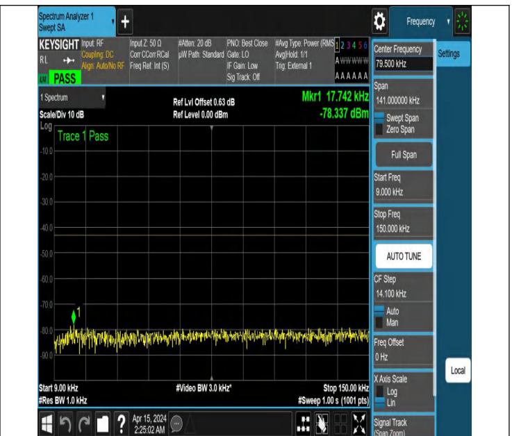
NTNV_N77-3450-3550_PC2_30_60_L_TID6_NS_01_0.009_0.15 #1
