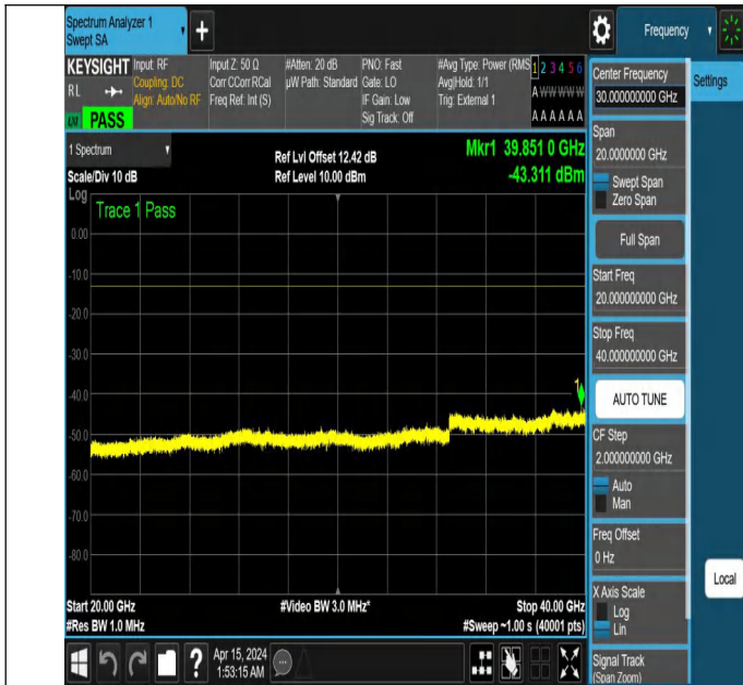
NTNV_N77-3450-3550_PC2_30_50_H_TID5_NS_01_20000_400
