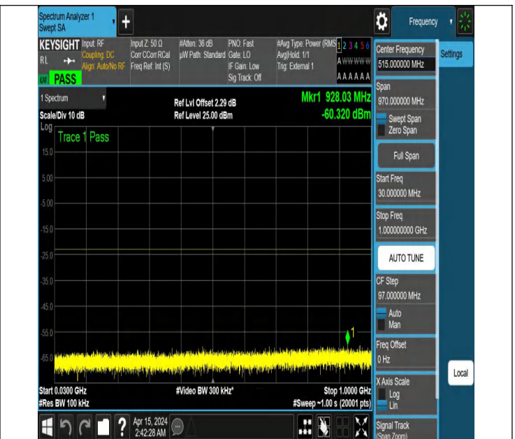
NTNV_N77-3450-3550_PC2_30_60_M_TID3_NS_01_30_1000_
