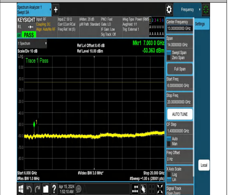
NTNV_N77-3450-3550_PC2_30_50_H_TID5_NS_01_6000_2000
