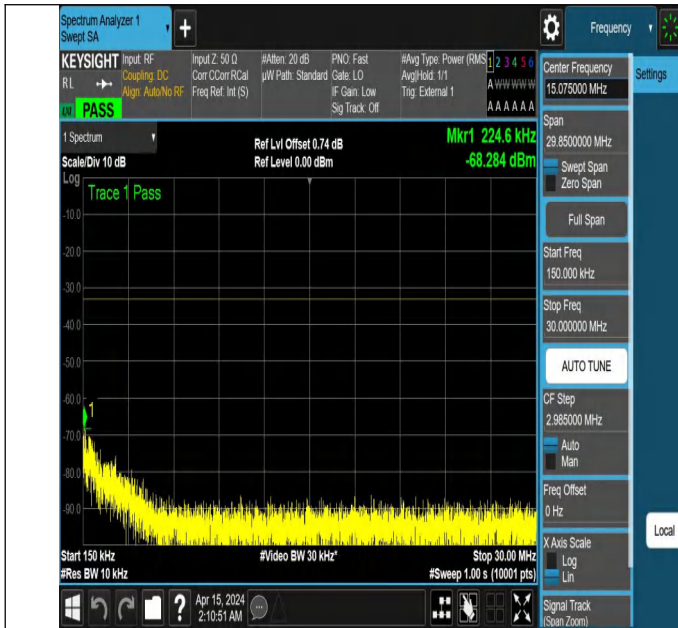
NTNV_N77-3450-3550_PC2_30_60_L_TID3_NS_01_0.15_30_#
