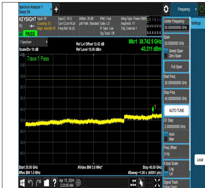
NTNV_N77-3450-3550_PC2_30_60_L_TID5_NS_01_20000_400 00 #1
