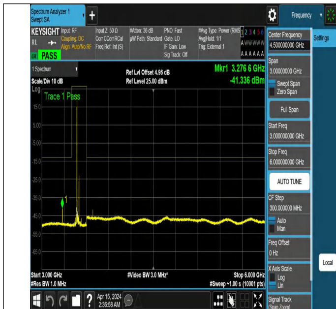
NTNV_N77-3450-3550_PC2_30_60_M_TID2_NS_01_3000_600 0 #1
