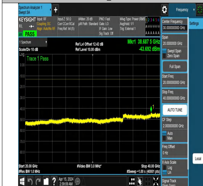
NTNV_N77-3450-3550_PC2_30_60_M_TID2_NS_01_20000_40 000 #1
