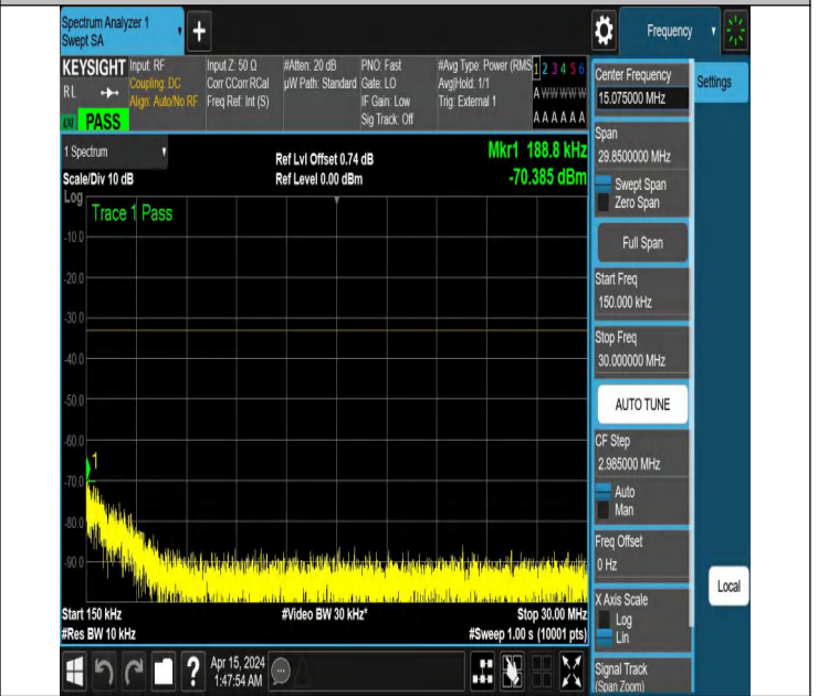
NTNV_N77-3450-3550_PC2_30_50_H_TID5_NS_01_0.15_30_#
