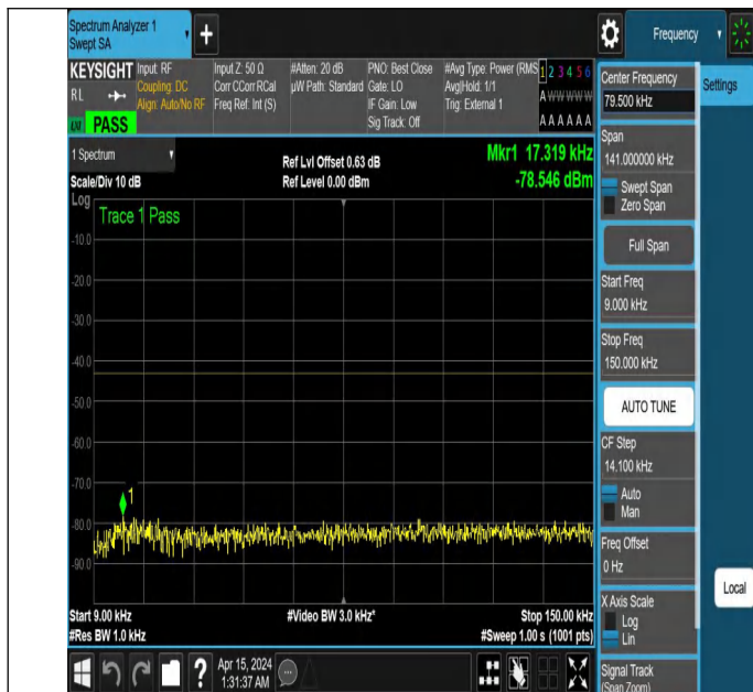
NTNV_N77-3450-3550_PC2_30_50_H_TID2_NS_01_0.009_0.15
