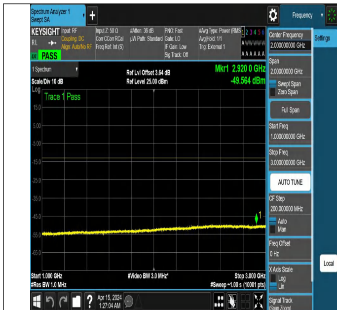
NTNV_N77-3450-3550_PC2_30_50_M_TID6_NS_01_1000_300 0 #1
