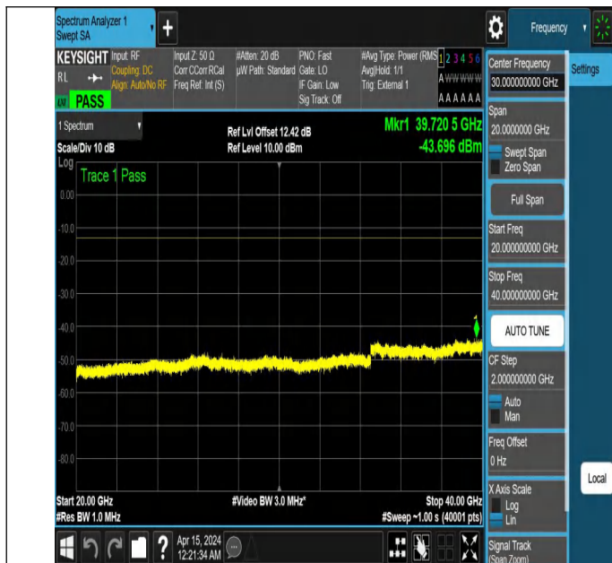
NTNV_N77-3450-3550_PC2_30_40_H_TID5_NS_01_20000_400 00 #1
