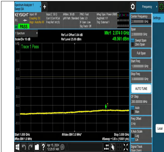
NTNV_N77-3450-3550_PC2_30_40_H_TID6_NS_01_1000_3000
