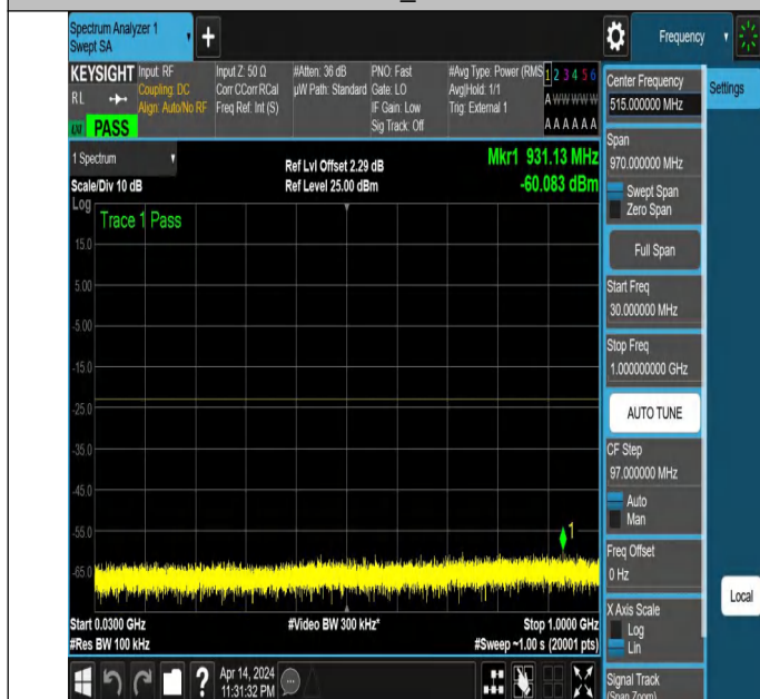
NTNV_N77-3450-3550_PC2_30_40_M_TID2_NS_01_30_1000
