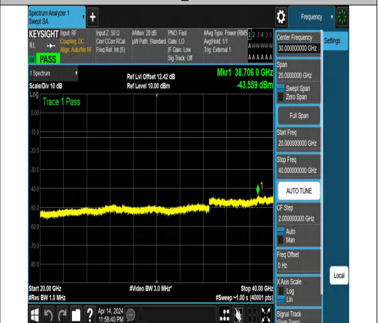
NTNV_N77-3450-3550_PC2_30_40_M_TID6_NS_01_20000_40 000 #1
