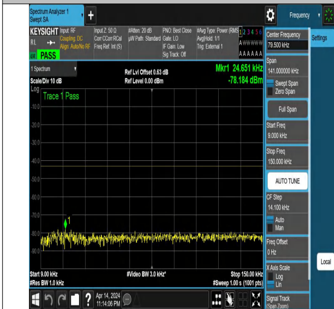
NTNV_N77-3450-3550_PC2_30_40_L_TID5_NS_01_0.009_0.15
