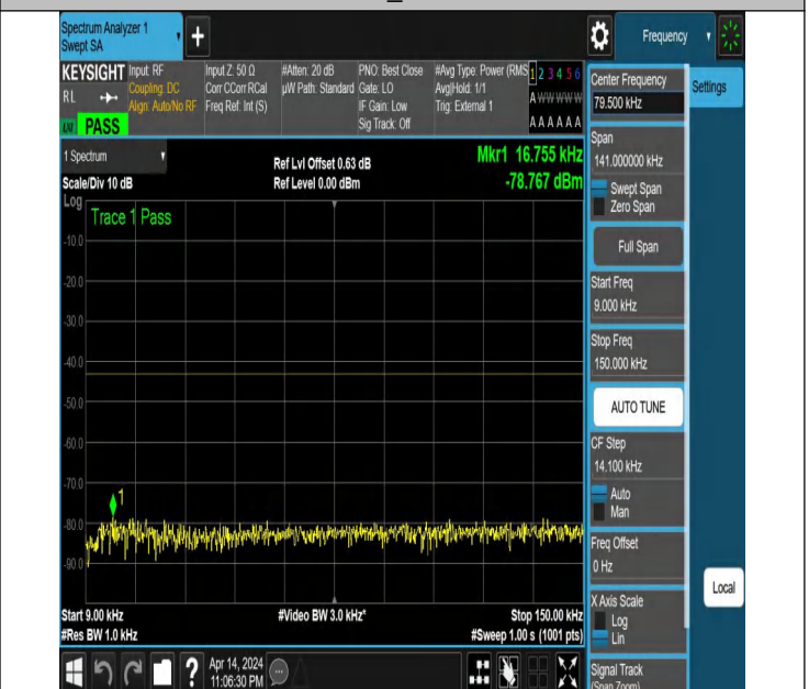
NTNV_N77-3450-3550_PC2_30_40_L_TID3_NS_01_0.009_0.15
