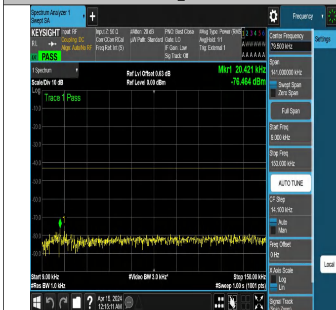
NTNV_N77-3450-3550_PC2_30_40_H_TID5_NS_01_0.009_0.15
