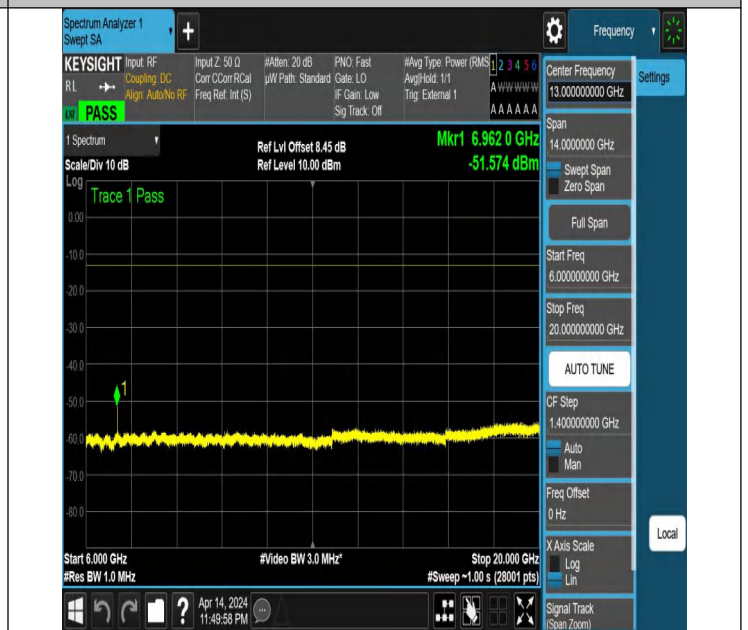
NTNV_N77-3450-3550_PC2_30_40_M_TID5_NS_01_6000_200
