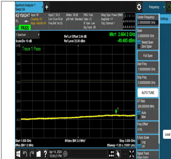
NTNV_N77-3450-3550_PC2_30_30_H_TID6_NS_01_1000_3000
