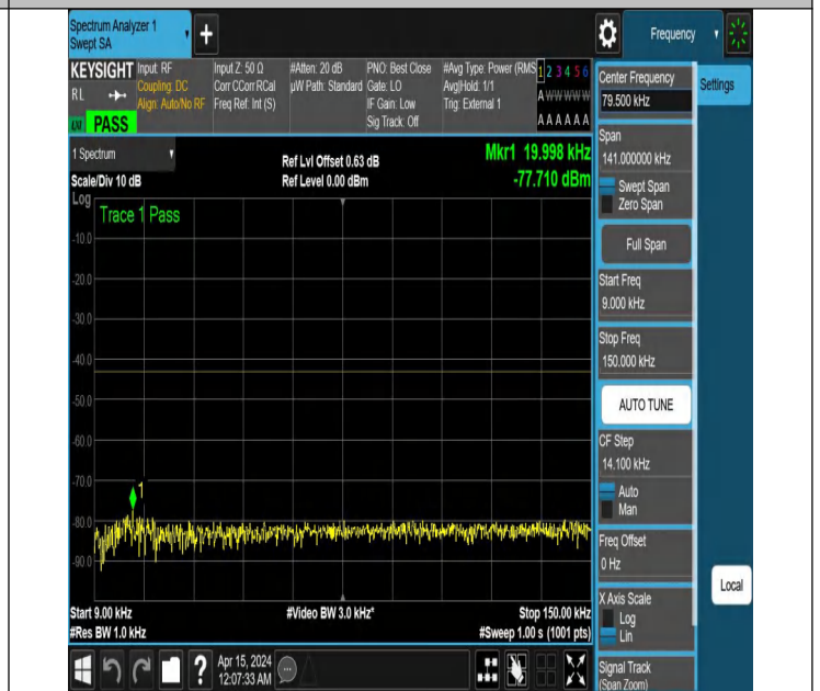
NTNV_N77-3450-3550_PC2_30_40_H_TID3_NS_01_0.009_0.15
