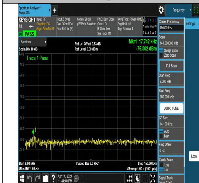
NTNV_N77-3450-3550_PC2_30_40_M_TID5_NS_01_0.009_0.1 5 #1
