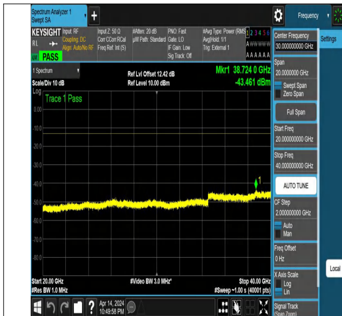
NTNV_N77-3450-3550_PC2_30_30_H_TID5_NS_01_20000_400
