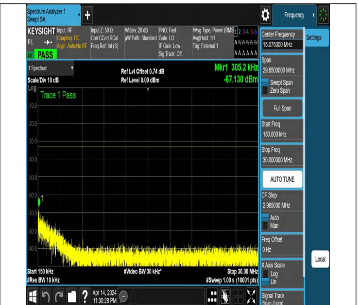
NTNV_N77-3450-3550_PC2_30_40_M_TID2_NS_01_0.15_30_#
