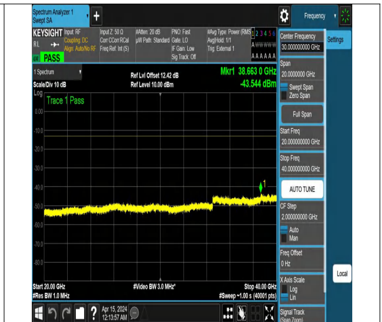
NTNV_N77-3450-3550_PC2_30_40_H_TID3_NS_01_20000_400 00 #1
