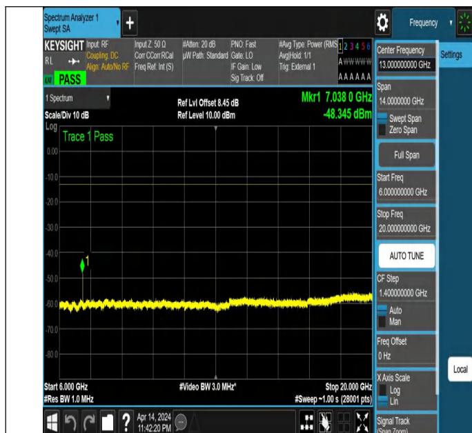
NTNV_N77-3450-3550_PC2_30_40_M_TID3_NS_01_6000_200 00 #1
