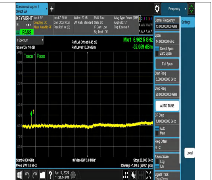
NTNV_N77-3450-3550_PC2_30_40_M_TID2_NS_01_6000_200 00 #1
