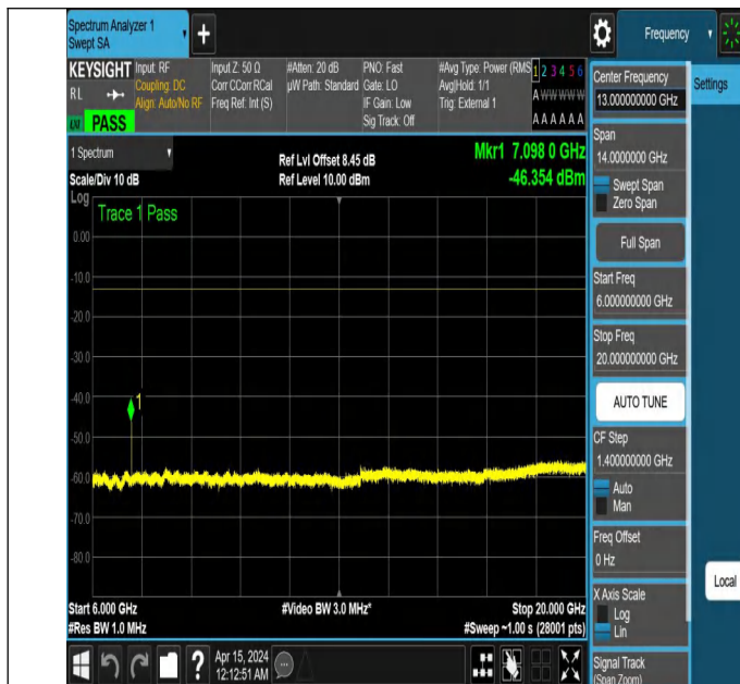
NTNV_N77-3450-3550_PC2_30_40_H_TID3_NS_01_6000_2000
