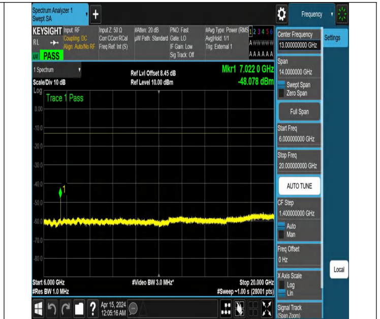
NTNV_N77-3450-3550_PC2_30_40_H_TID2_NS_01_6000_2000
