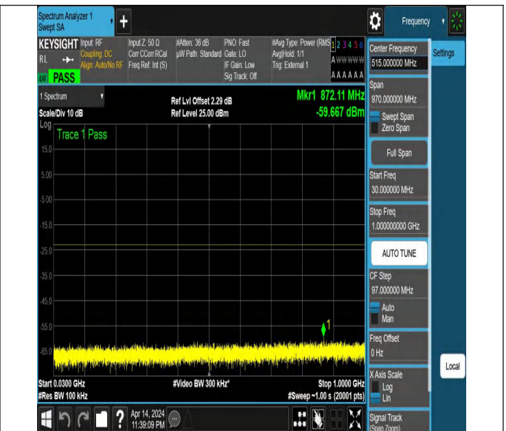
NTNV_N77-3450-3550_PC2_30_40_M_TID3_NS_01_30_1000_
