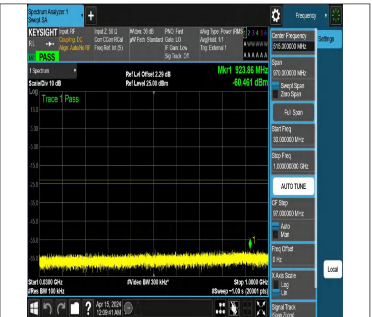
NTNV_N77-3450-3550_PC2_30_40_H_TID3_NS_01_30_1000_#
