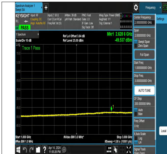
NTNV_N77-3450-3550_PC2_30_40_M_TID6_NS_01_1000_300
