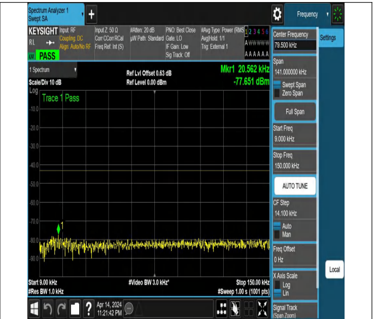
NTNV_N77-3450-3550_PC2_30_40_L_TID6_NS_01_0.009_0.15
