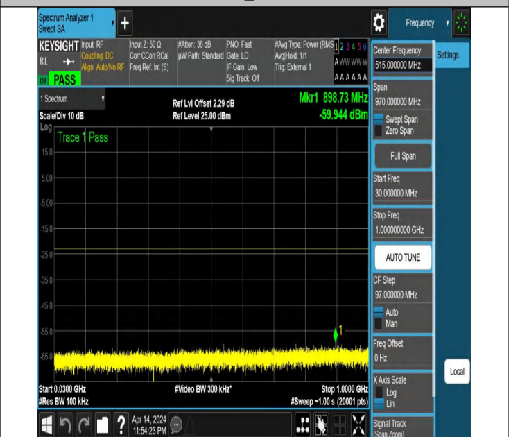
NTNV_N77-3450-3550_PC2_30_40_M_TID6_NS_01_30_1000_ #1
