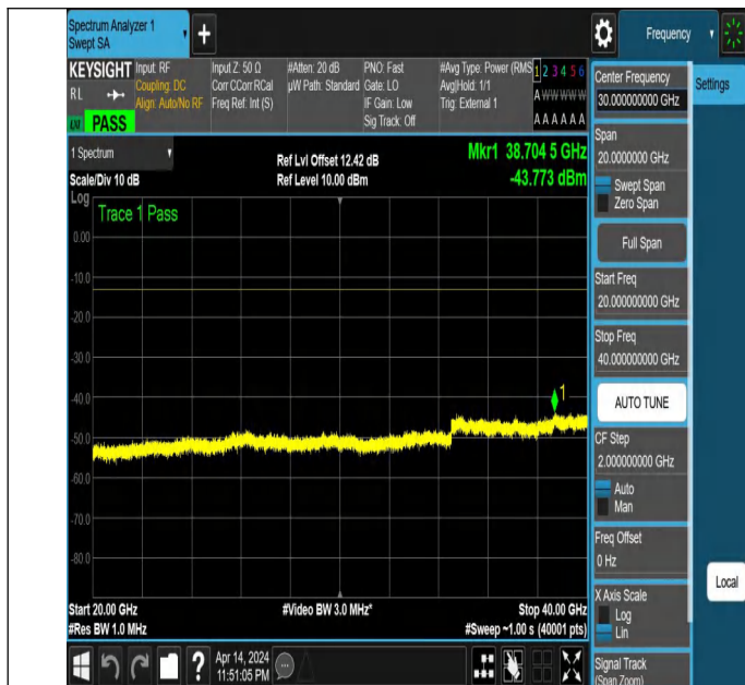
NTNV_N77-3450-3550_PC2_30_40_M_TID5_NS_01_20000_40 000 #1
