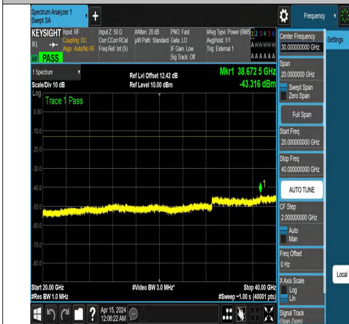
NTNV_N77-3450-3550_PC2_30_40_H_TID2_NS_01_20000_400
