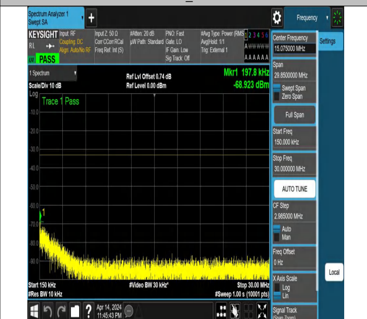
NTNV_N77-3450-3550_PC2_30_40_M_TID5_NS_01_0.15_30_#
