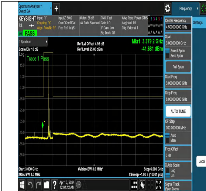
NTNV_N77-3450-3550_PC2_30_40_H_TID2_NS_01_3000_6000
