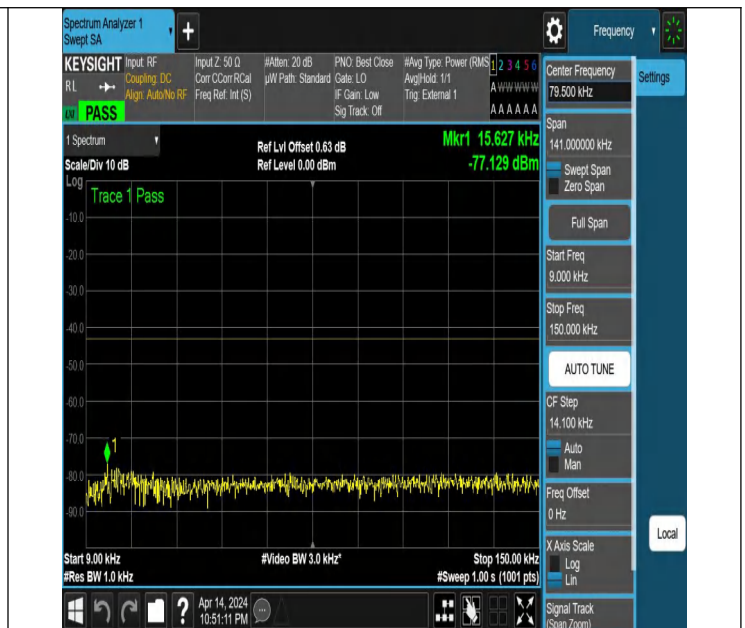
NTNV_N77-3450-3550_PC2_30_30_H_TID6_NS_01_0.009_0.15 #1
