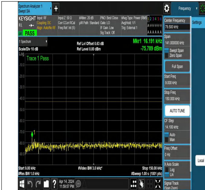
NTNV_N77-3450-3550_PC2_30_40_H_TID2_NS_01_0.009_0.15
