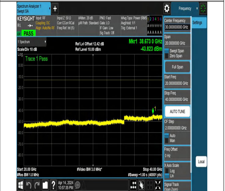
NTNV_N77-3450-3550_PC2_30_30_H_TID6_NS_01_20000_400
