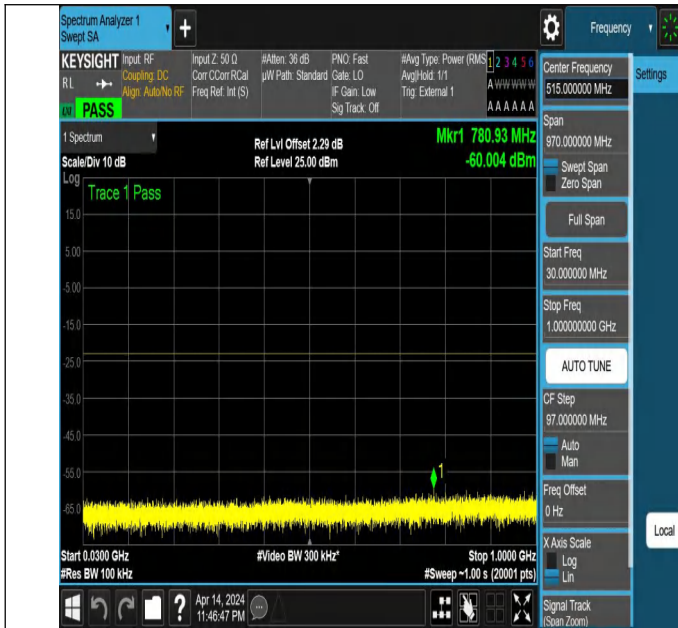
NTNV_N77-3450-3550_PC2_30_40_M_TID5_NS_01_30_1000_
