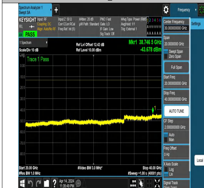
NTNV_N77-3450-3550_PC2_30_40_M_TID2_NS_01_20000_40 000 #1
