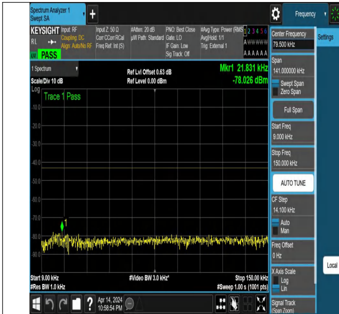
NTNV_N77-3450-3550_PC2_30_40_L_TID2_NS_01_0.009_0.15
