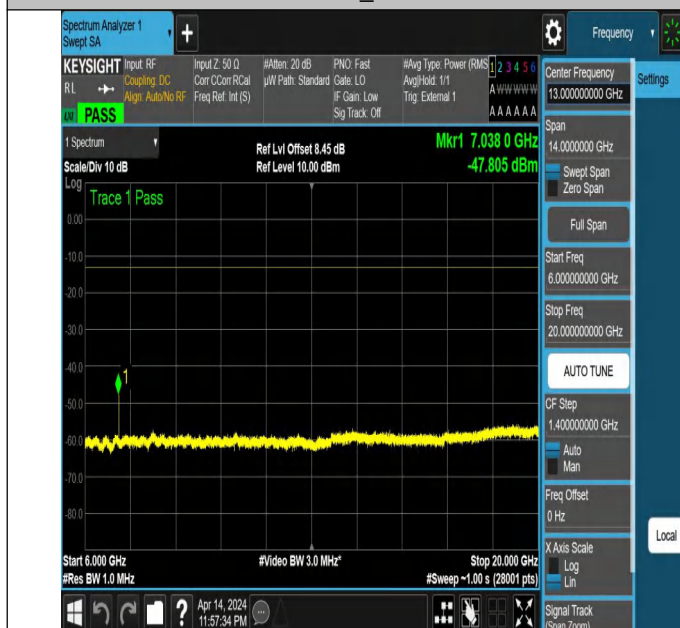
NTNV_N77-3450-3550_PC2_30_40_M_TID6_NS_01_6000_200 00 #1
