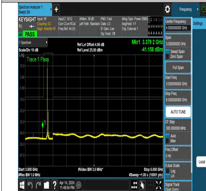
NTNV_N77-3450-3550_PC2_30_40_M_TID5_NS_01_3000_600
