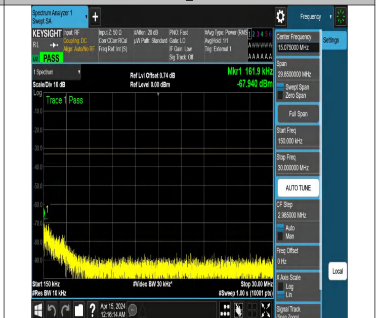
NTNV_N77-3450-3550_PC2_30_40_H_TID5_NS_01_0.15_30_#
