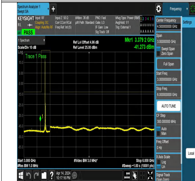
NTNV_N77-3450-3550_PC2_30_30_M_TID5_NS_01_3000_600
