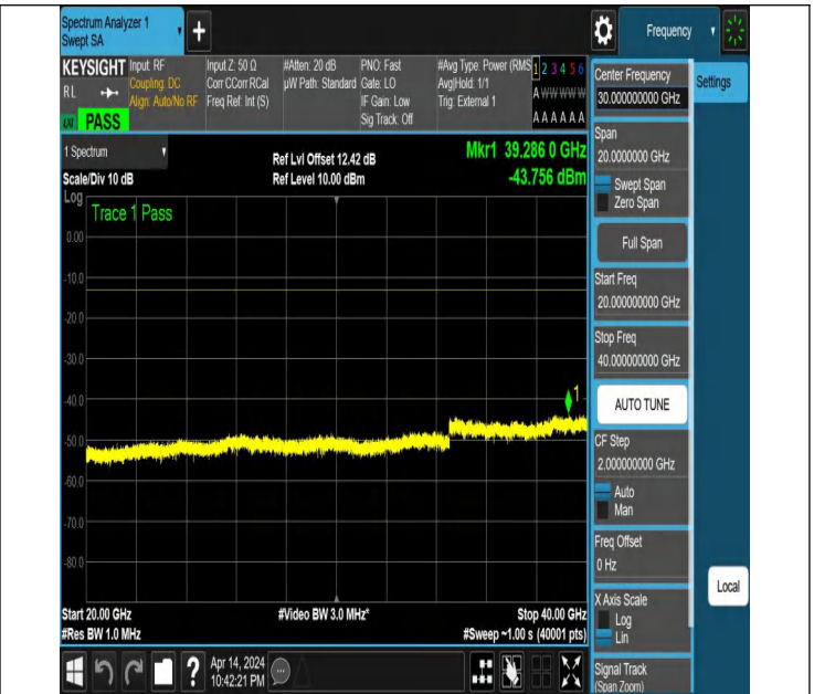
NTNV_N77-3450-3550_PC2_30_30_H_TID3_NS_01_20000_400
