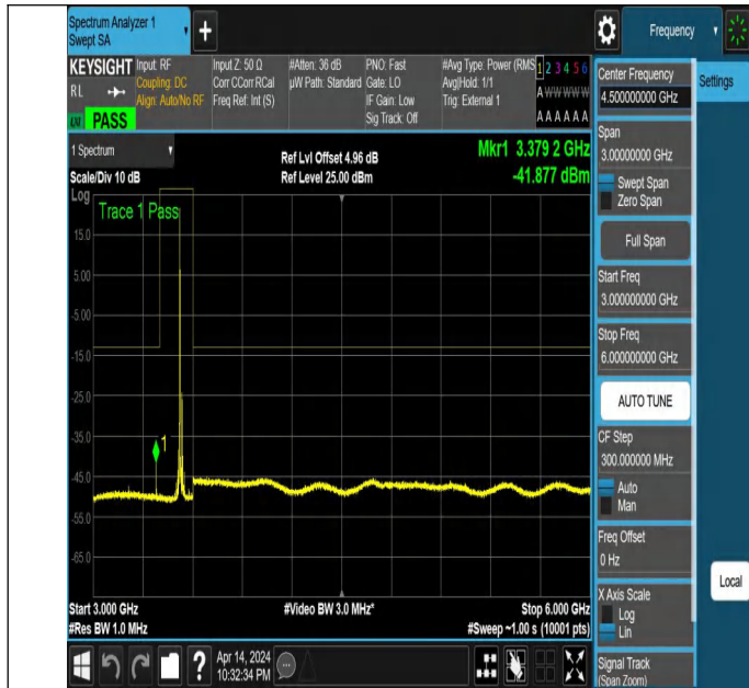
NTNV_N77-3450-3550_PC2_30_30_H_TID2_NS_01_3000_6000
