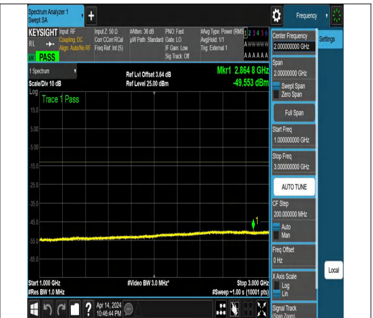
NTNV_N77-3450-3550_PC2_30_30_H_TID5_NS_01_1000_3000
