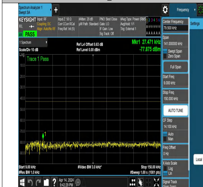
NTNV_N77-3450-3550_PC2_30_30_L_TID5_NS_01_0.009_0.15
