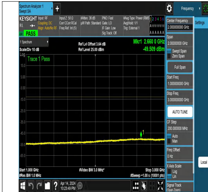
NTNV_N77-3450-3550_PC2_30_30_M_TID6_NS_01_1000_300
