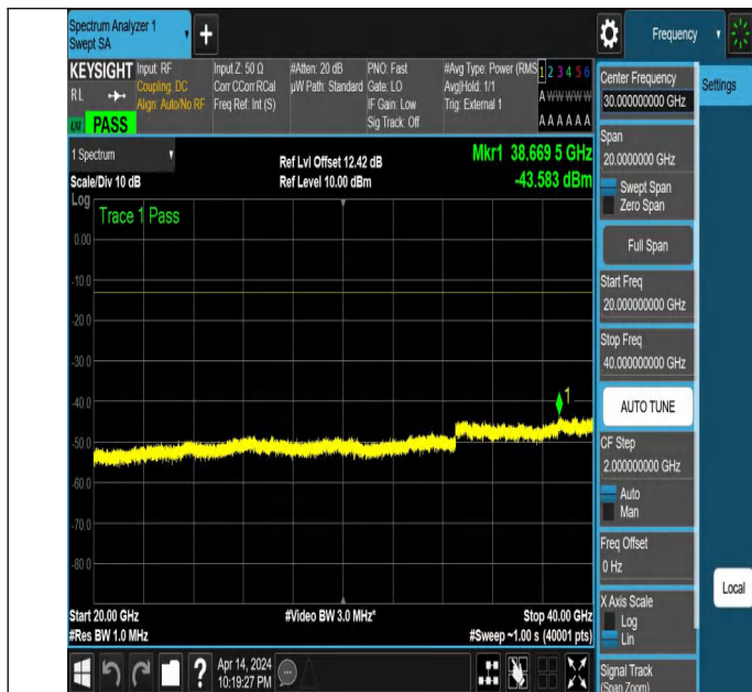
NTNV_N77-3450-3550_PC2_30_30_M_TID5_NS_01_20000_40 000 #1
