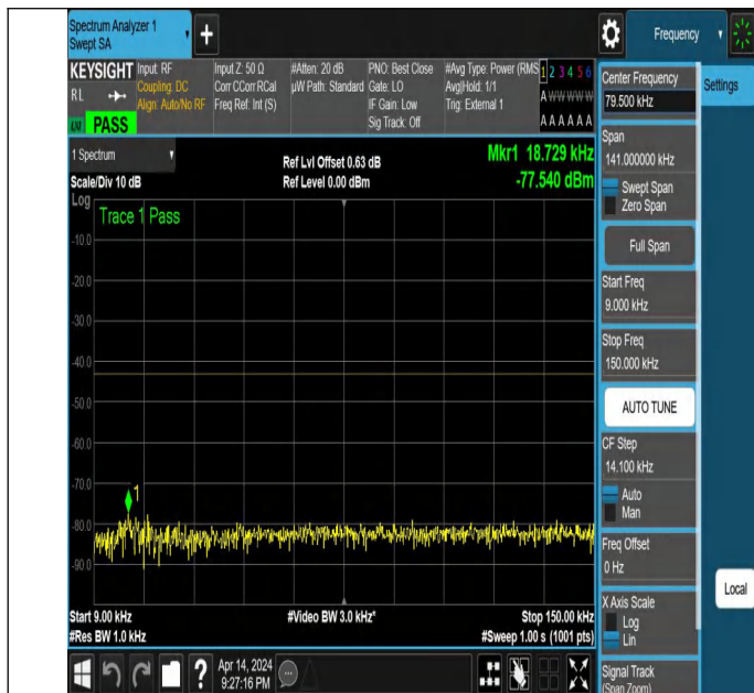
NTNV_N77-3450-3550_PC2_30_30_L_TID2_NS_01_0.009_0.15
