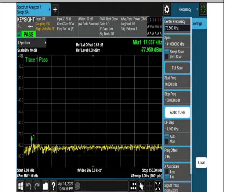
NTNV_N77-3450-3550_PC2_30_30_H_TID3_NS_01_0.009_0.15
