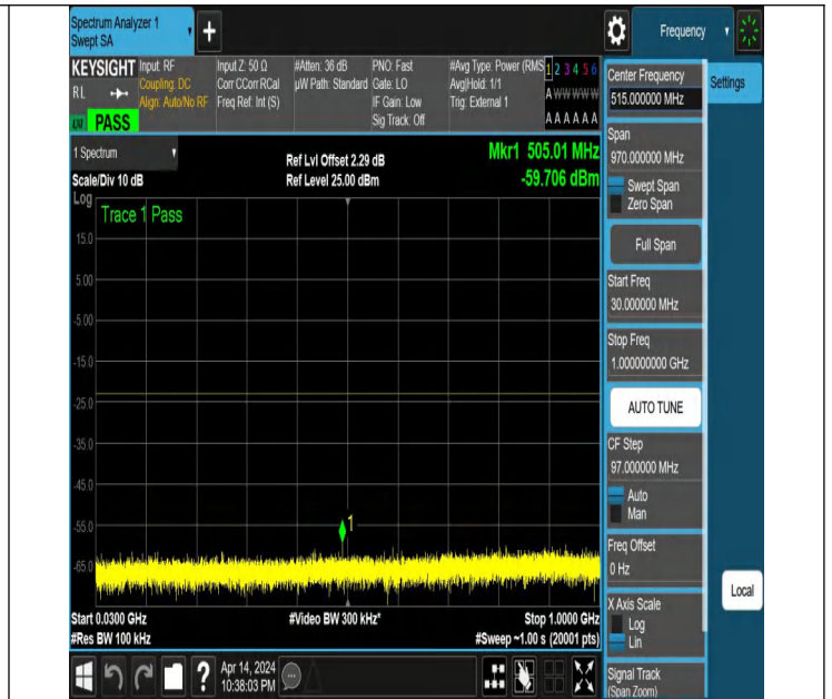
NTNV_N77-3450-3550_PC2_30_30_H_TID3_NS_01_30_1000_#
