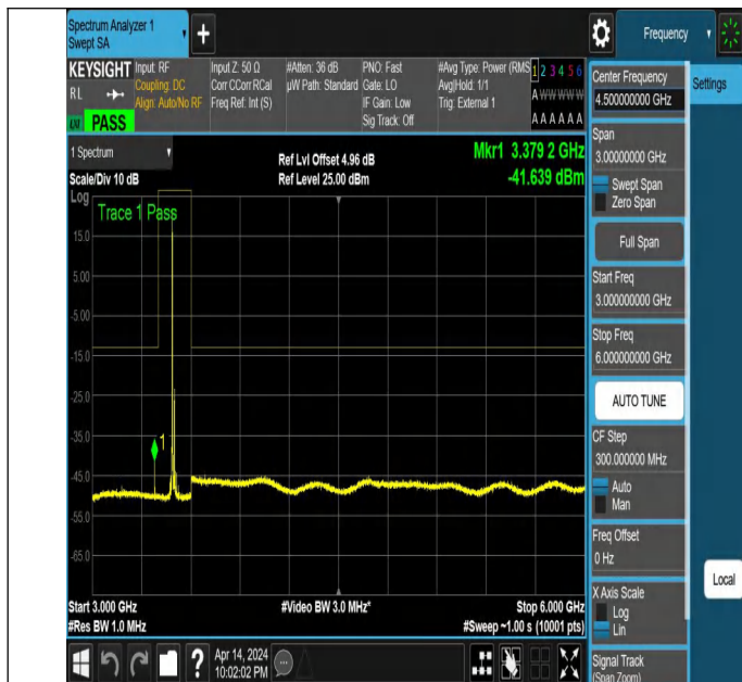
NTNV_N77-3450-3550_PC2_30_30_M_TID2_NS_01_3000_600
