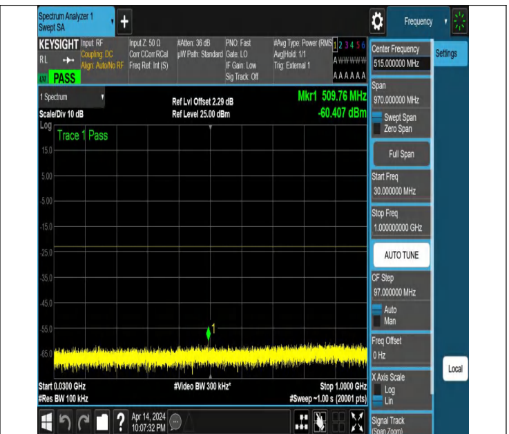
NTNV_N77-3450-3550_PC2_30_30_M_TID3_NS_01_30_1000_
