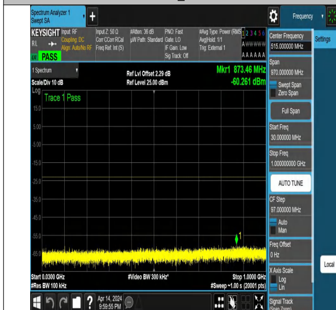
NTNV_N77-3450-3550_PC2_30_30_M_TID2_NS_01_30_1000_#1
