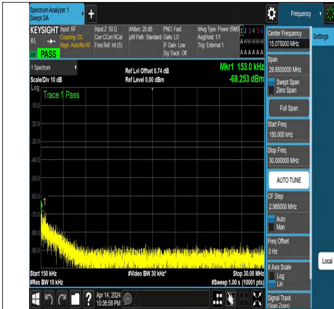
NTNV_N77-3450-3550_PC2_30_30_H_TID3_NS_01_0.15_30_#
