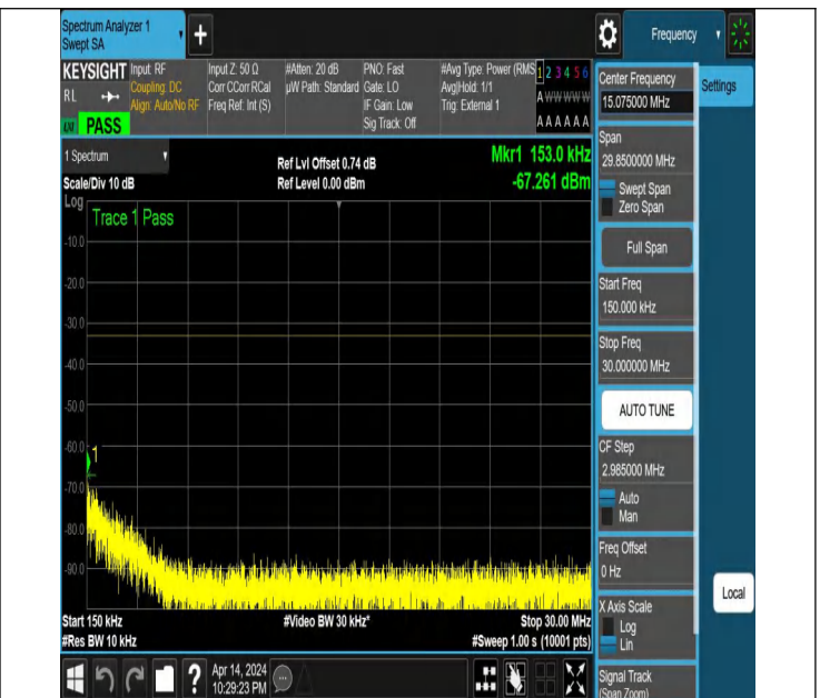
NTNV_N77-3450-3550_PC2_30_30_H_TID2_NS_01_0.15_30_#
