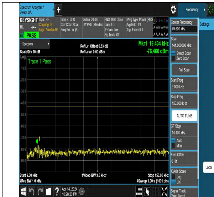
NTNV_N77-3450-3550_PC2_30_30_H_TID2_NS_01_0.009_0.15
