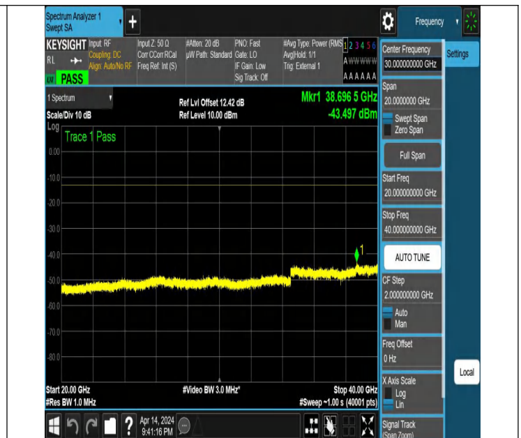
NTNV_N77-3450-3550_PC2_30_30_L_TID3_NS_01_20000_400 00 #1
