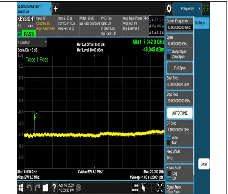
NTNV_N77-3450-3550_PC2_30_30_H_TID2_NS_01_6000_2000
