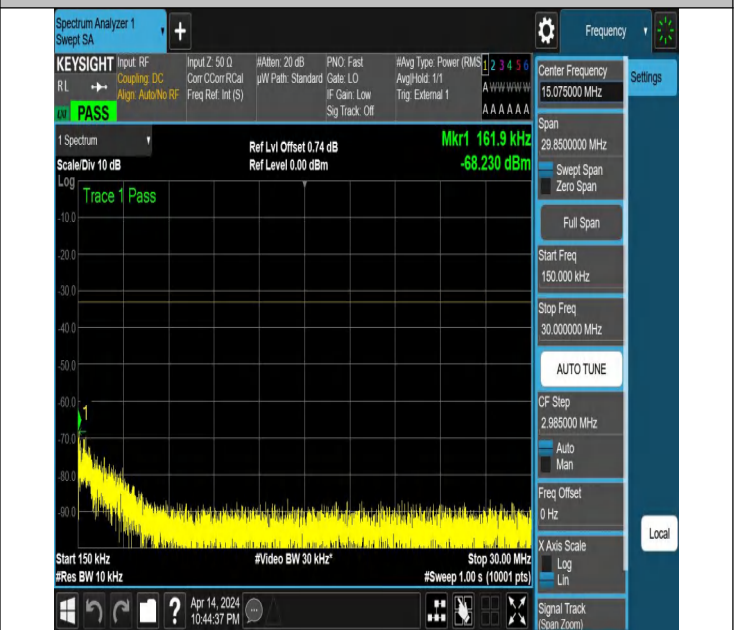
NTNV_N77-3450-3550_PC2_30_30_H_TID5_NS_01_0.15_30_#
