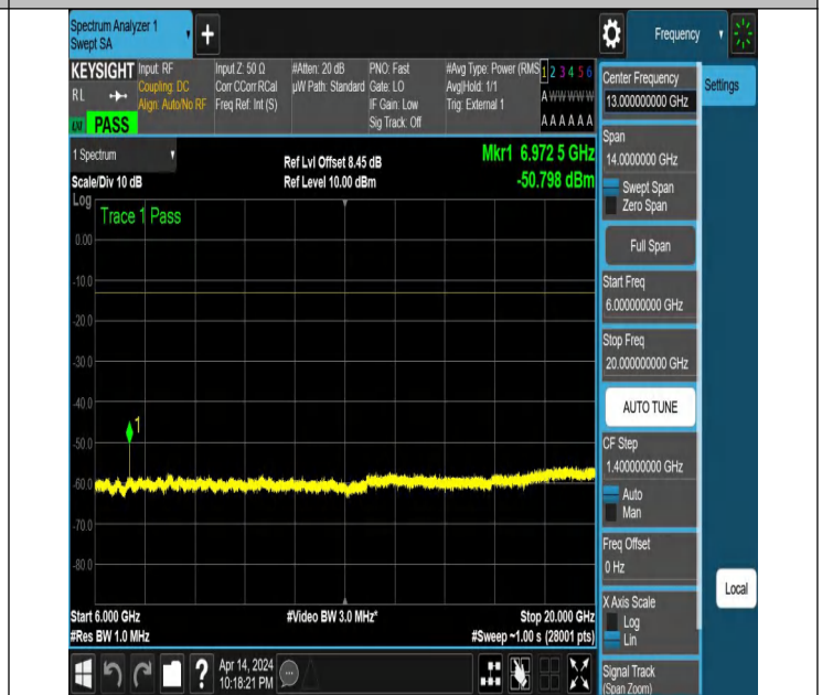
NTNV_N77-3450-3550_PC2_30_30_M_TID5_NS_01_6000_200
