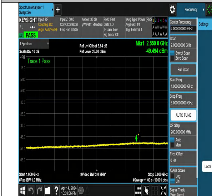
NTNV_N77-3450-3550_PC2_30_30_H_TID3_NS_01_1000_3000
