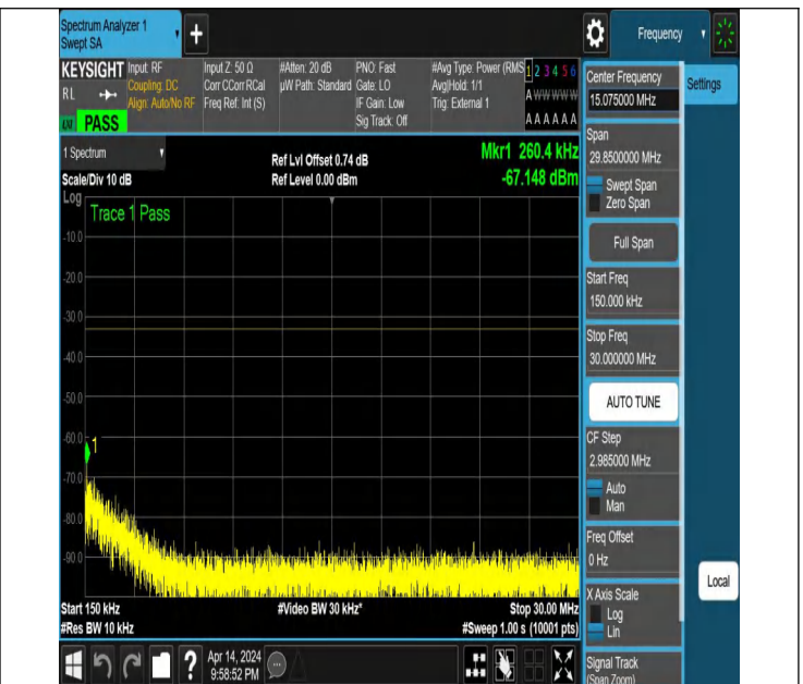
NTNV_N77-3450-3550_PC2_30_30_M_TID2_NS_01_0.15_30_#
