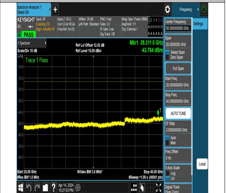
NTNV_N77-3450-3550_PC2_30_30_M_TID6_NS_01_20000_40
