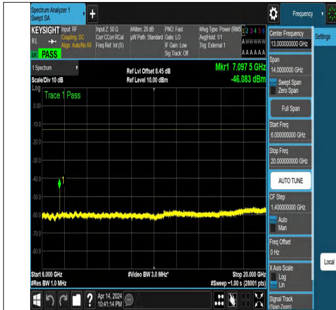
NTNV_N77-3450-3550_PC2_30_30_H_TID3_NS_01_6000_2000
