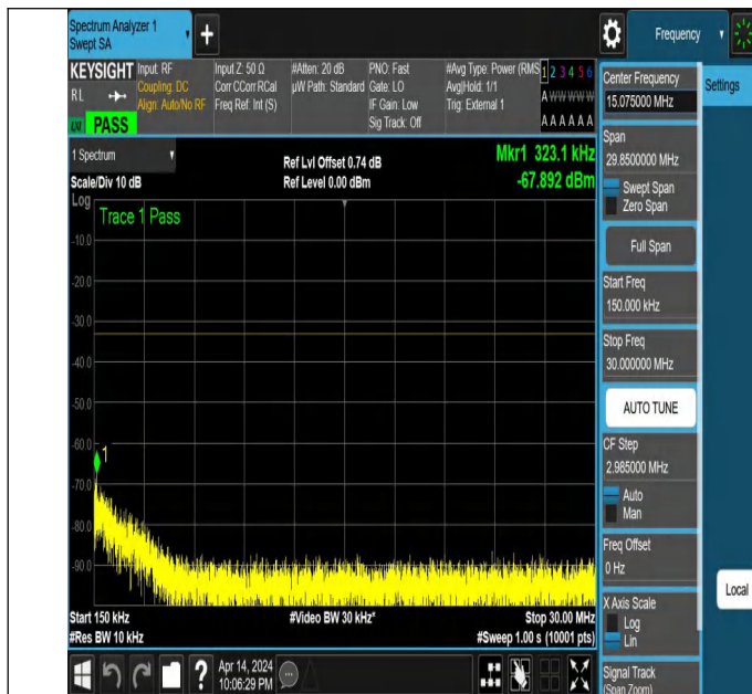
NTNV_N77-3450-3550_PC2_30_30_M_TID3_NS_01_0.15_30_#
