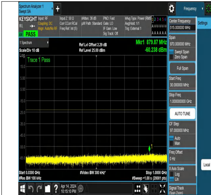
NTNV_N77-3450-3550_PC2_30_30_M_TID5_NS_01_30_1000_
