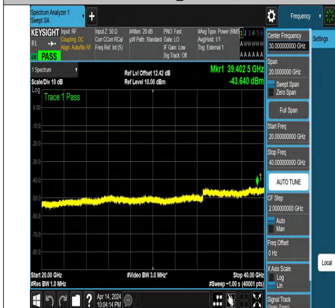
NTNV_N77-3450-3550_PC2_30_30_M_TID2_NS_01_20000_40 000 #1
