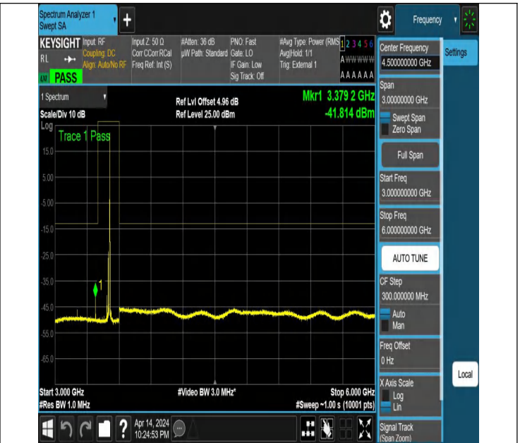
NTNV_N77-3450-3550_PC2_30_30_M_TID6_NS_01_3000_600
