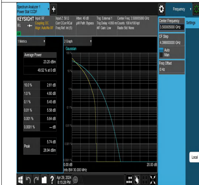
NTNV-N77-3450-3550-PC2-30-30-M-DFT-QPSK-Outter_Full-PAS
