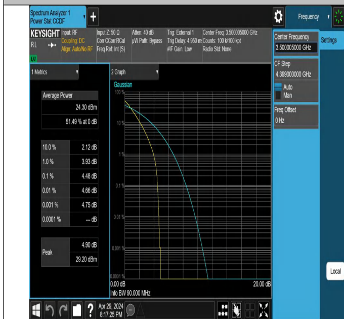
NTNV-N77-3450-3550-PC2-30-90-M-DFT-PI2BPSK-Outer_Full-P ASS
