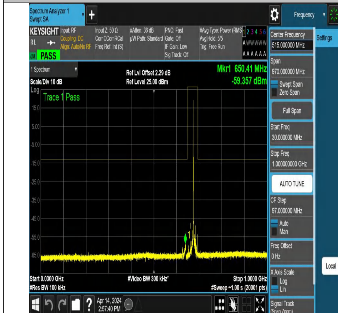
NTNV_N71_PC3_15_15_H_TID2_NS_01_30_1000_#1
