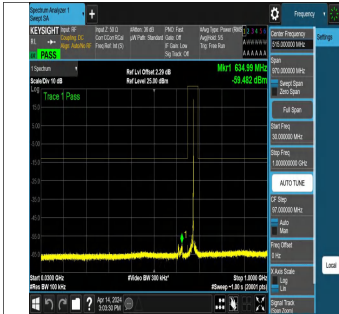
NTNV_N71_PC3_15_20_L_TID3_NS_01_30_1000_#1
