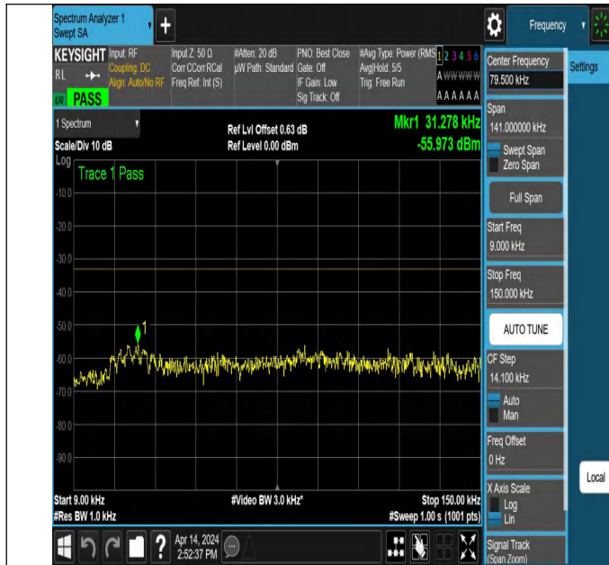
NTNV_N71_PC3_15_15_M_TID2_NS_01_0.009_0.15_#1
