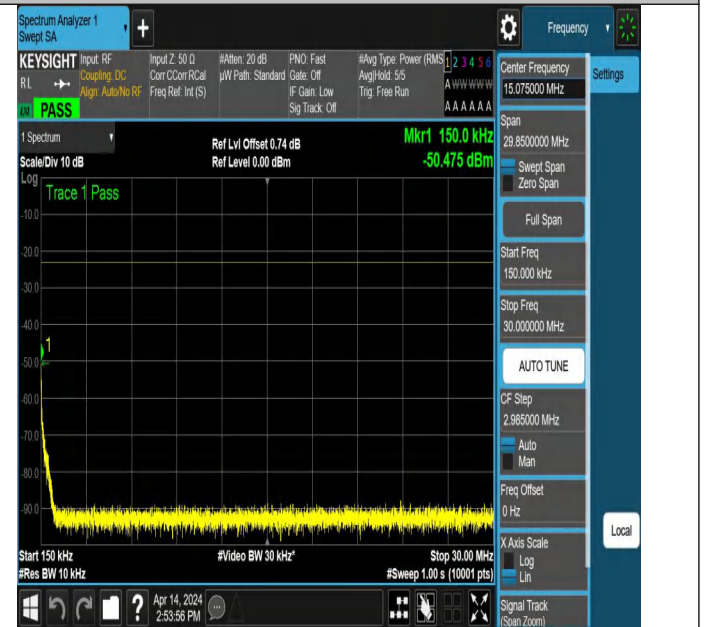
NTNV_N71_PC3_15_15_M_TID3_NS_01_0.15_30_#1
