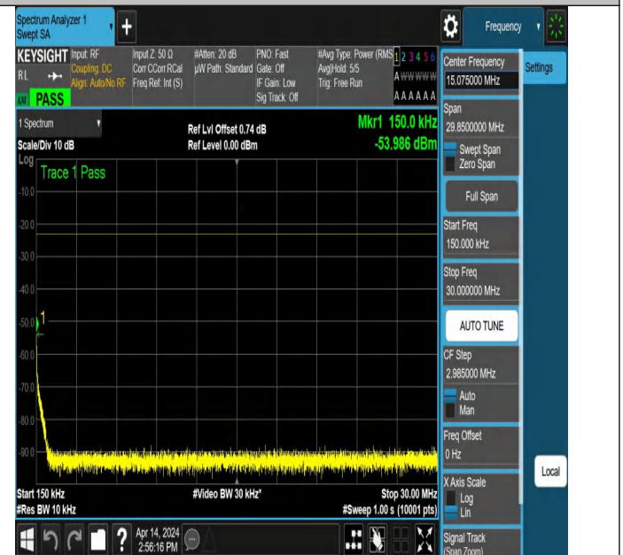
NTNV_N71_PC3_15_15_M_TID6_NS_01_0.15_30_#1
