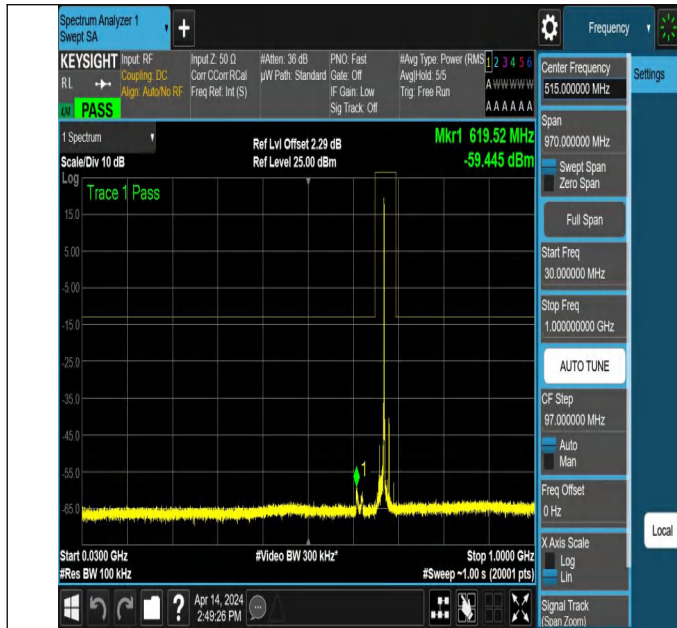
NTNV_N71_PC3_15_15_L_TID3_NS_01_30_1000_#1
