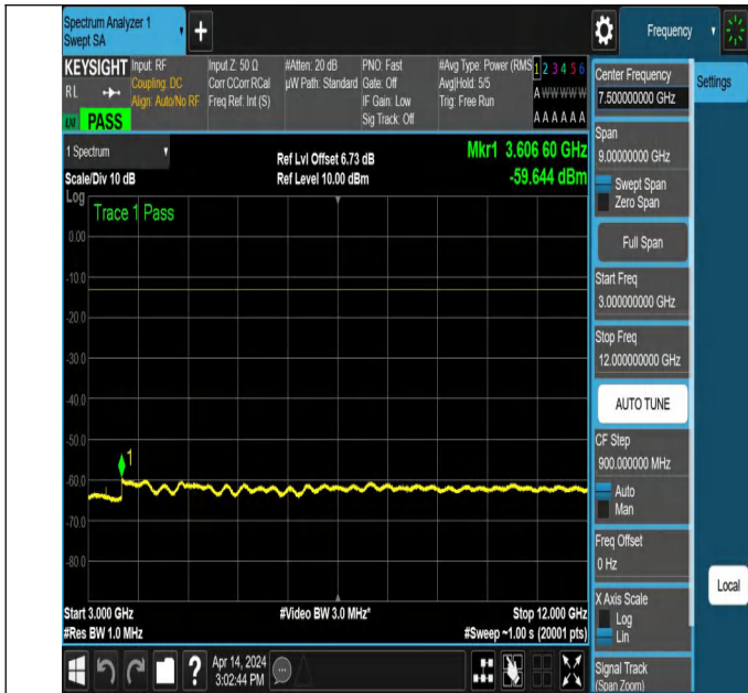
NTNV_N71_PC3_15_20_L_TID2_NS_01_3000_12000_#1
