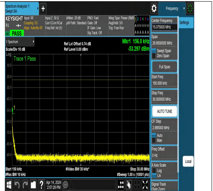
NTNV_N71_PC3_15_15_H_TID2_NS_01_0.15_30_#1
