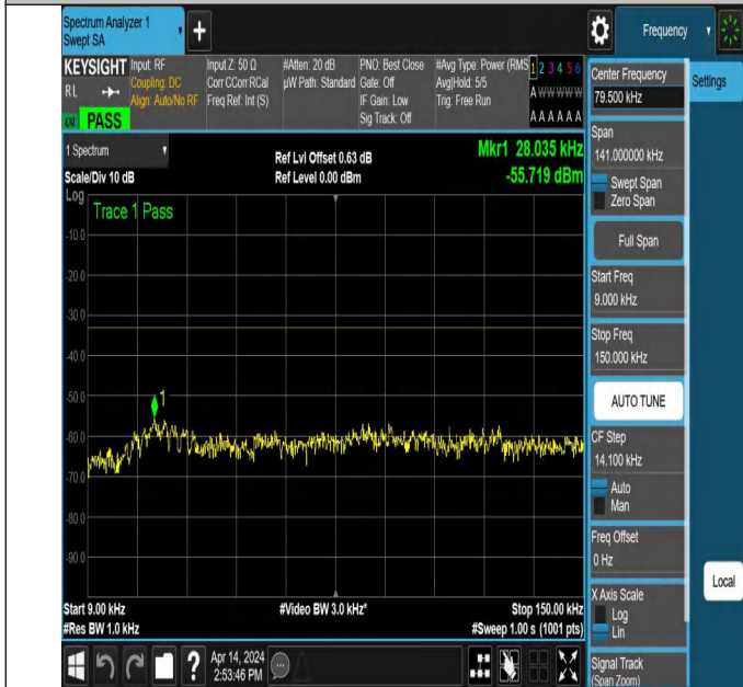
NTNV_N71_PC3_15_15_M_TID3_NS_01_0.009_0.15_#1
