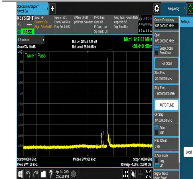
NTNV_N71_PC3_15_15_L_TID5_NS_01_30_1000_#1
