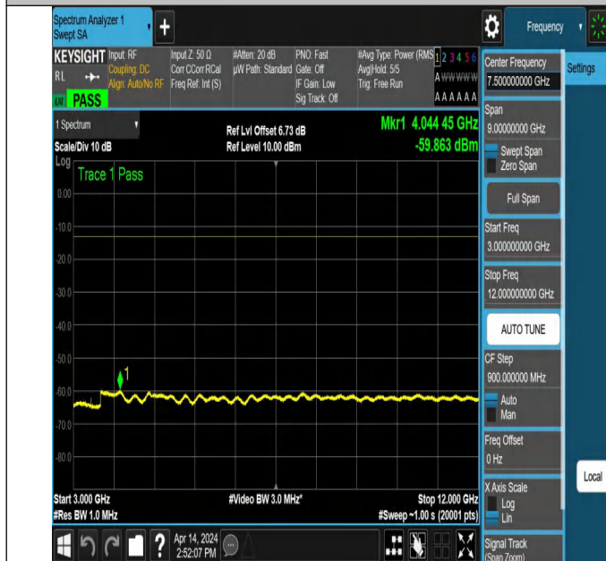
NTNV_N71_PC3_15_15_L_TID6_NS_01_3000_12000_#1
