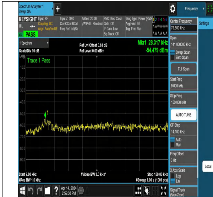
NTNV_N71_PC3_15_15_H_TID5_NS_01_0.009_0.15_#1
