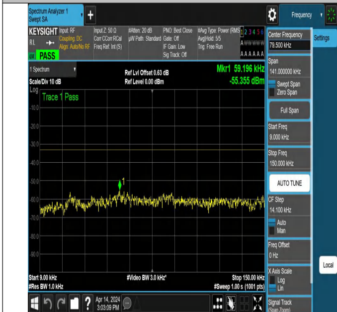
NTNV_N71_PC3_15_20_L_TID3_NS_01_0.009_0.15_#1
