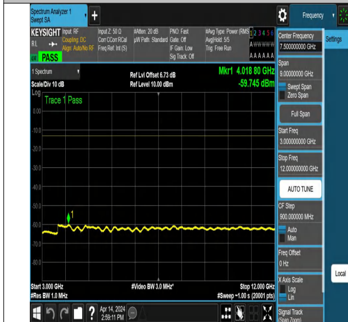
NTNV_N71_PC3_15_15_H_TID3_NS_01_3000_12000_#1
