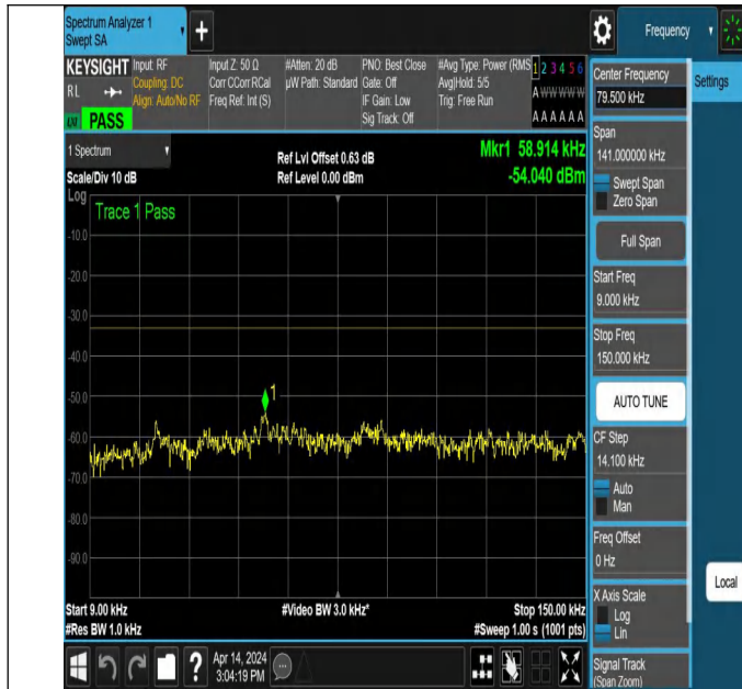
NTNV_N71_PC3_15_20_L_TID5_NS_01_0.009_0.15_#1
