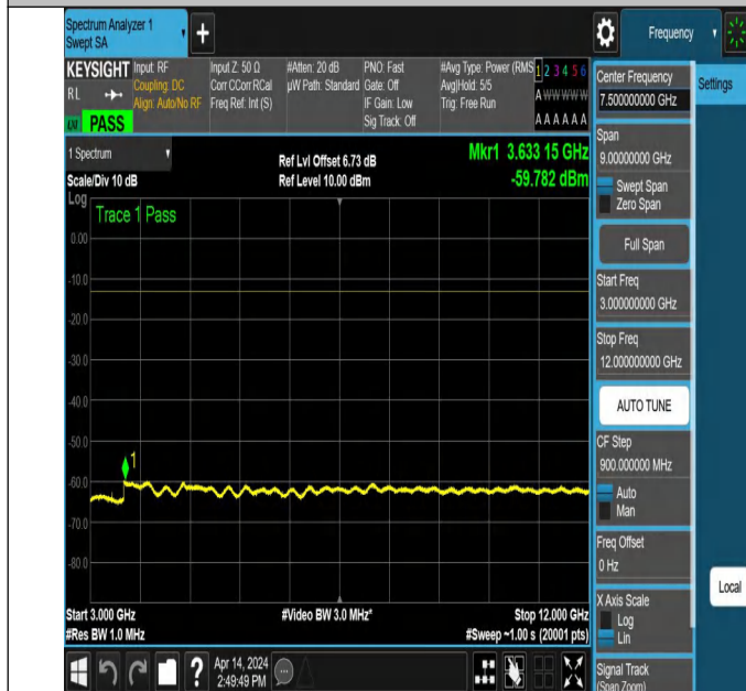
NTNV_N71_PC3_15_15_L_TID3_NS_01_3000_12000_#1
