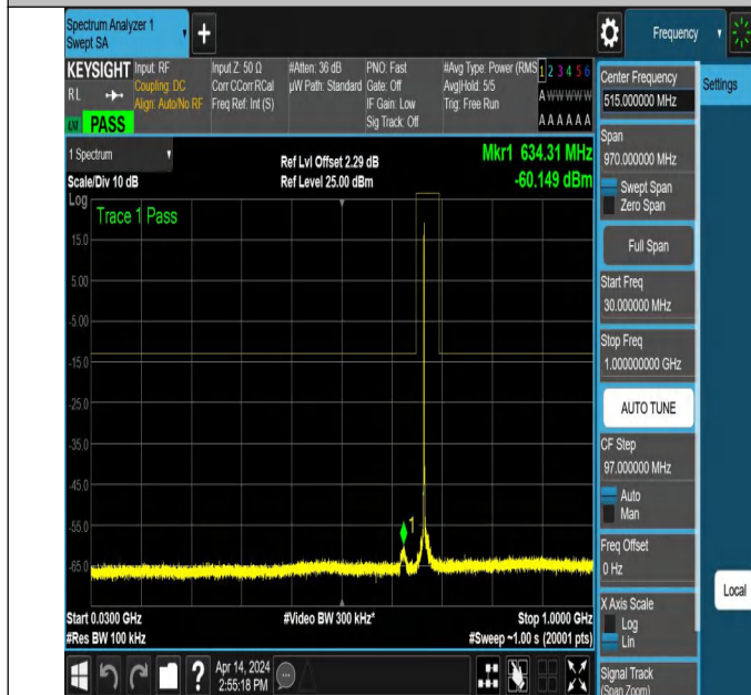
NTNV_N71_PC3_15_15_M_TID5_NS_01_30_1000_#1
