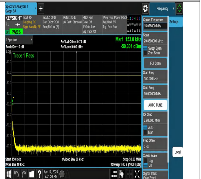
NTNV_N71_PC3_15_15_L_TID6_NS_01_0.15_30_#1
