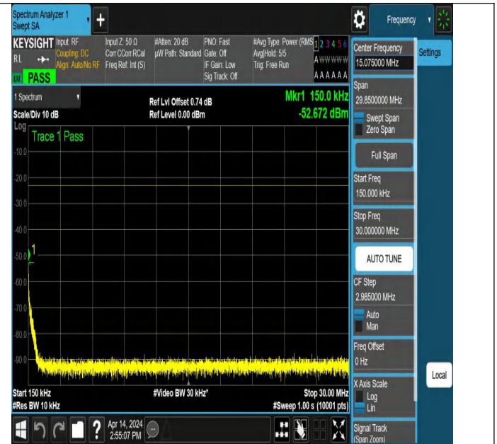
NTNV_N71_PC3_15_15_M_TID5_NS_01_0.15_30_#1
