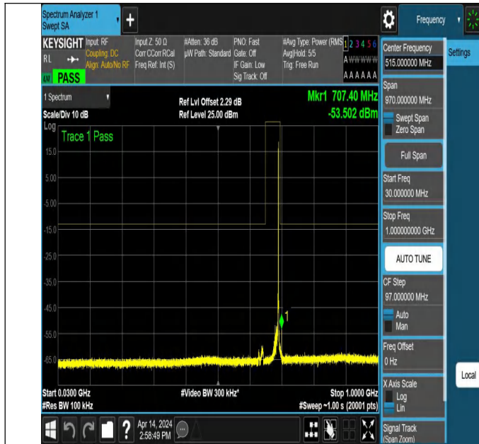
NTNV_N71_PC3_15_15_H_TID3_NS_01_30_1000_#1
