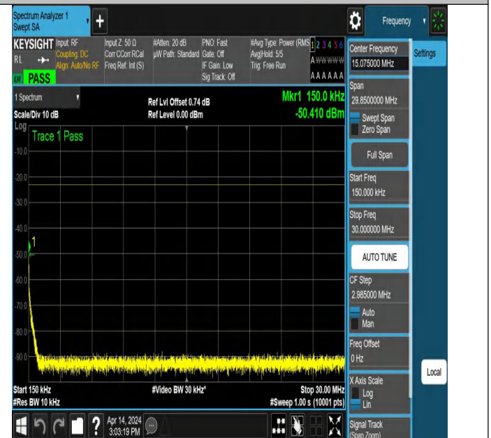
NTNV_N71_PC3_15_20_L_TID3_NS_01_0.15_30_#1
