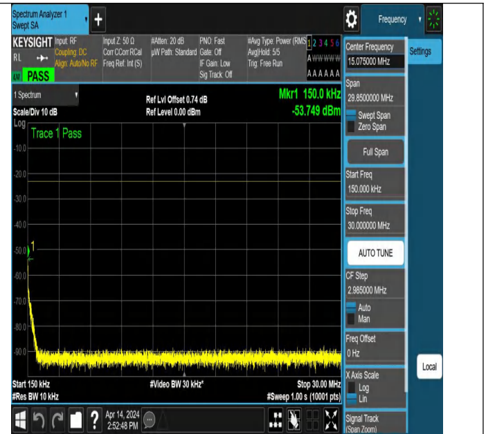
NTNV_N71_PC3_15_15_M_TID2_NS_01_0.15_30_#1
