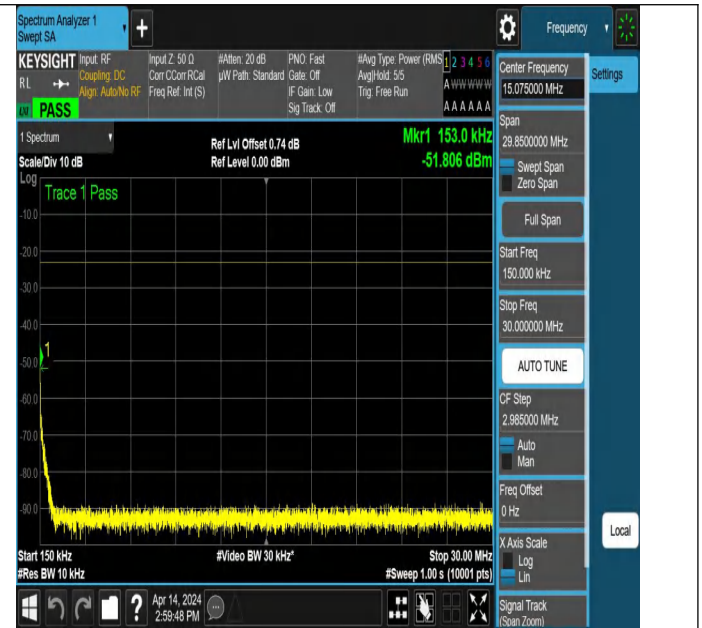
NTNV_N71_PC3_15_15_H_TID5_NS_01_0.15_30_#1
