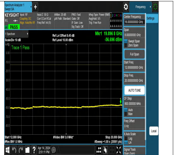
NTNV_N71_PC3_15_15_L_TID5_NS_01_12000_20000_#1
