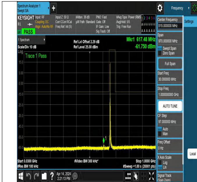
NTNV_N71_PC3_15_5_L_TID3_NS_01_30_1000_#1
