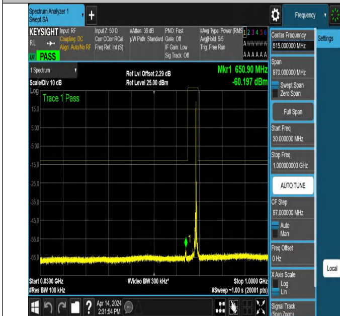
NTNV_N71_PC3_15_5_H_TID5_NS_01_30_1000_#1
