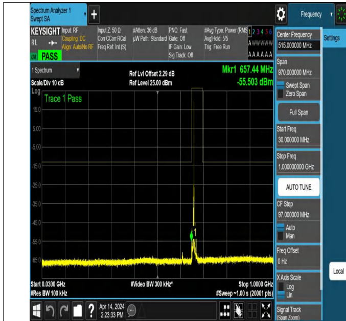
NTNV_N71_PC3_15_5_L_TID6_NS_01_30_1000_#1
