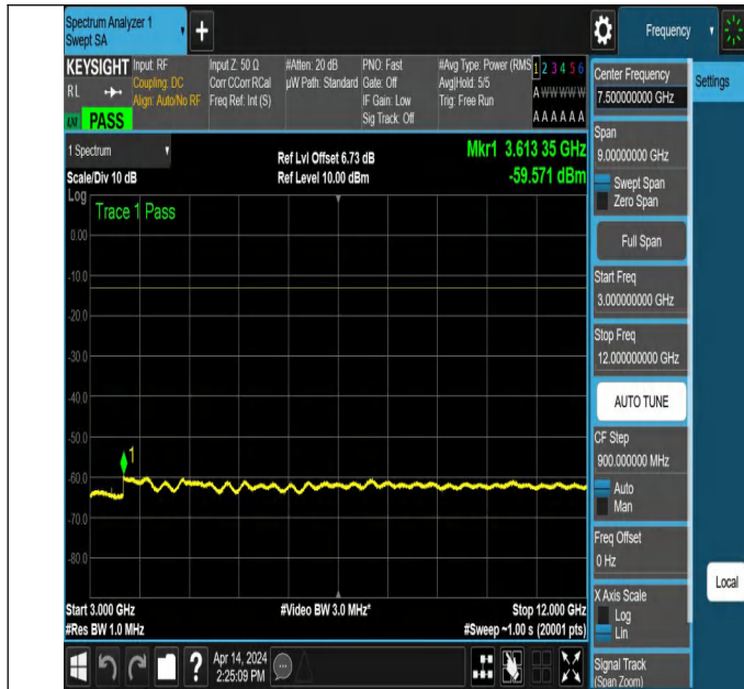
NTNV_N71_PC3_15_5_M_TID2_NS_01_3000_12000_#1
