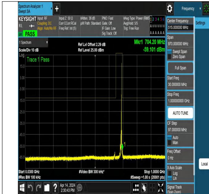
NTNV_N71_PC3_15_5_H_TID3_NS_01_30_1000_#1
