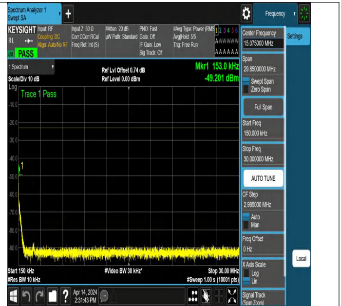
NTNV_N71_PC3_15_5_H_TID5_NS_01_0.15_30_#1
