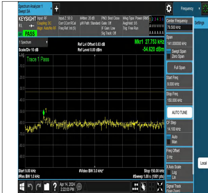
NTNV_N71_PC3_15_5_L_TID5_NS_01_0.009_0.15_#1
