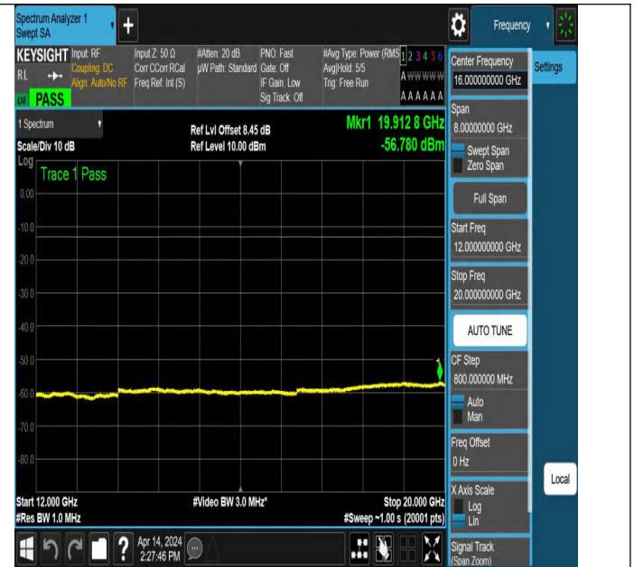
NTNV_N71_PC3_15_5_M_TID5_NS_01_12000_20000_#1
