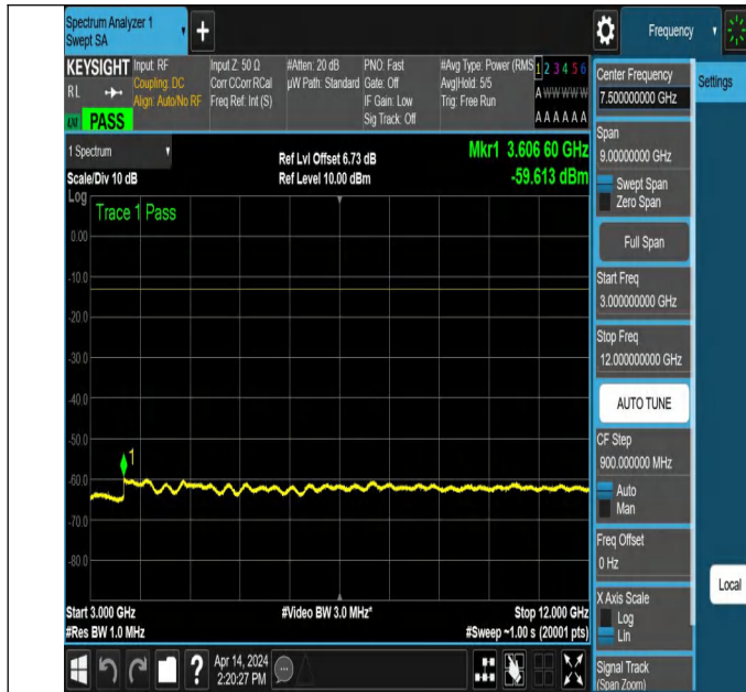
NTNV_N71_PC3_15_5_L_TID2_NS_01_3000_12000_#1
