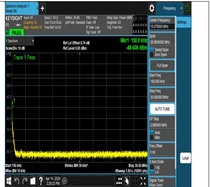
NTNV_N71_PC3_15_5_H_TID2_NS_01_0.15_30_#1
