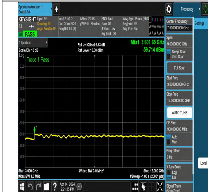
NTNV_N71_PC3_15_5_L_TID3_NS_01_3000_12000_#1
