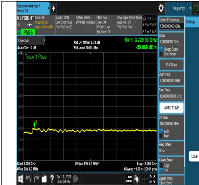
NTNV_N71_PC3_15_5_M_TID5_NS_01_3000_12000_#1
