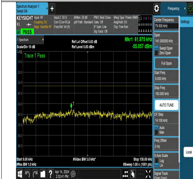
NTNV_N71_PC3_15_5_H_TID6_NS_01_0.009_0.15_#1
