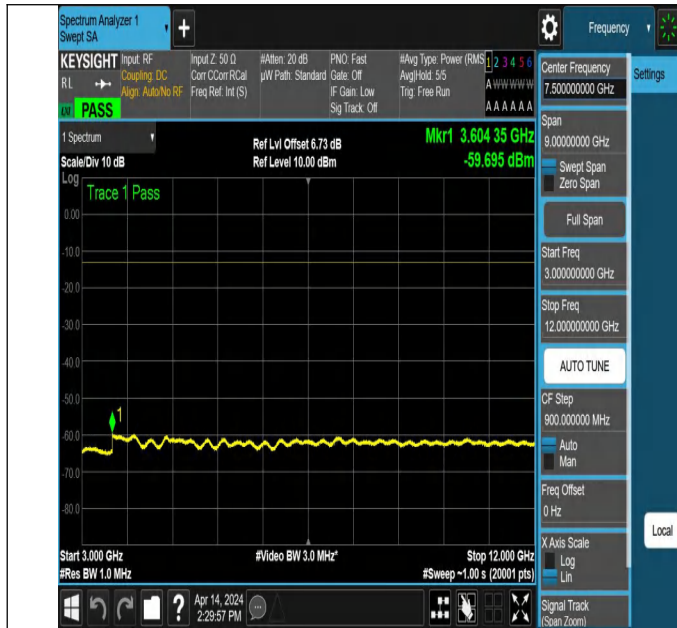
NTNV_N71_PC3_15_5_H_TID2_NS_01_3000_12000_#1
