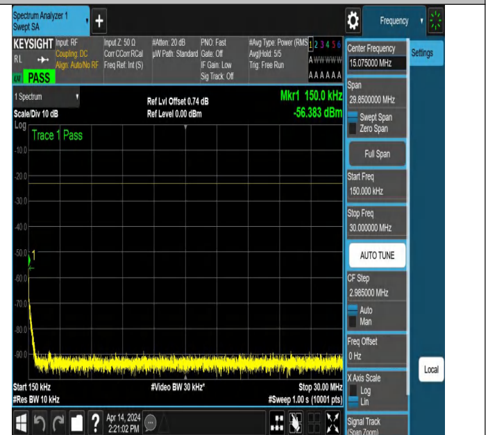
NTNV_N71_PC3_15_5_L_TID3_NS_01_0.15_30_#1
