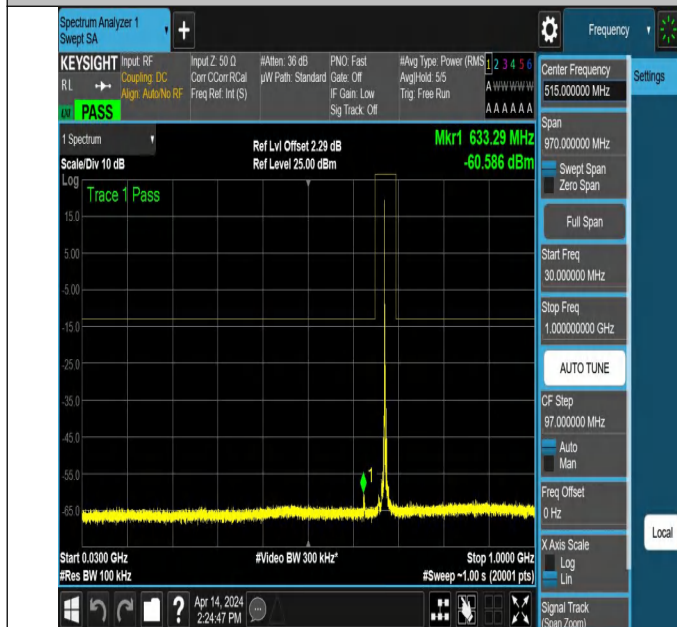
NTNV_N71_PC3_15_5_M_TID2_NS_01_30_1000_#1
