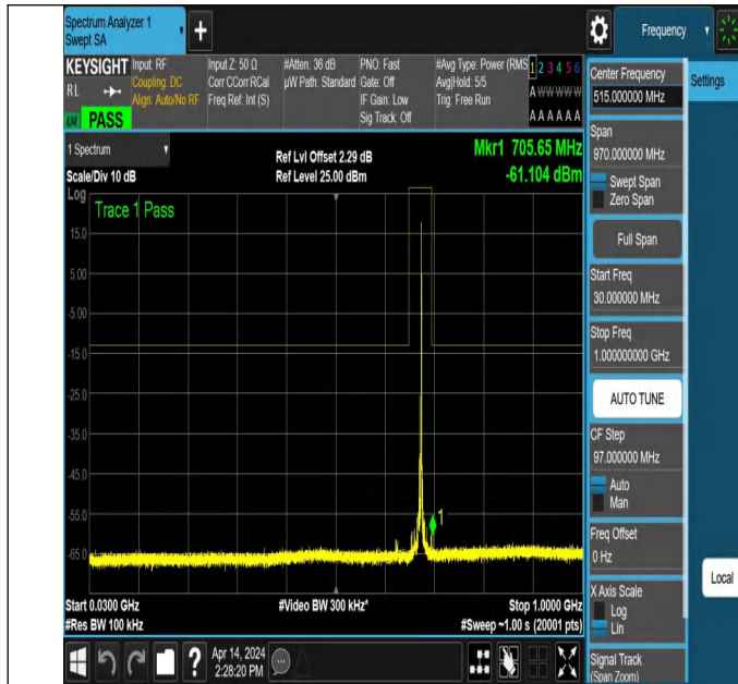
NTNV_N71_PC3_15_5_M_TID6_NS_01_30_1000_#1
