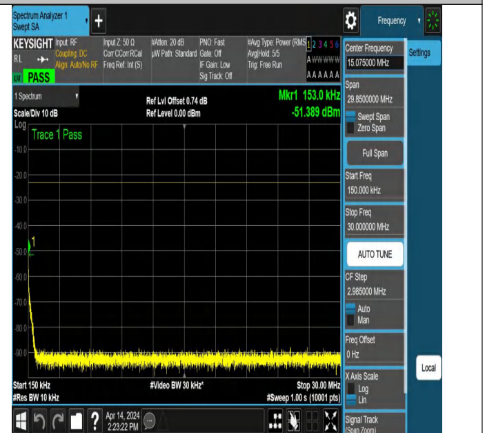
NTNV_N71_PC3_15_5_L_TID6_NS_01_0.15_30_#1
