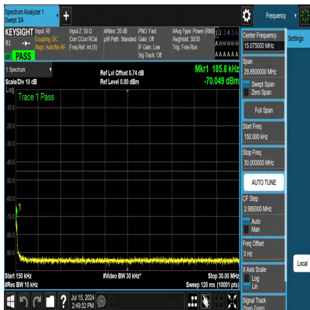
NTNV-N41-PC3-30-100-H-DFT-QPSK-Edge_1RB_Right-0.15-30- Ant1-PASS
