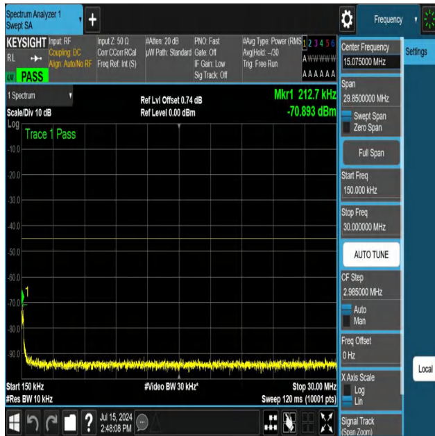
NTNV-N41-PC3-30-100-M-DFT-QPSK-Edge_1RB_Right-0.15-30-Ant1-PASS
