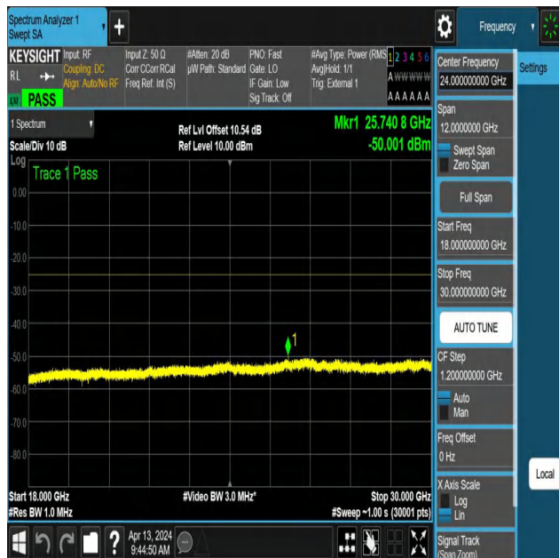
NTNV-N41-PC3-30-100-H-DFT-QPSK-Edge_1RB_Left-18000-300 00-Ant1-PASS
