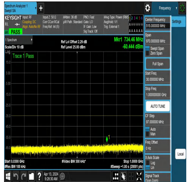
NTNV-N41-PC3-30-100-M-DFT-QPSK-Edge_1RB_Right-30-1000-Ant1-PASS
