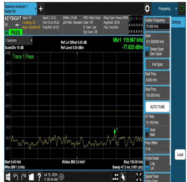
NTNV-N41-PC3-30-100-H-DFT-QPSK-Edge_1RB_Left-0.009-0.1 5-Ant1-PASS
