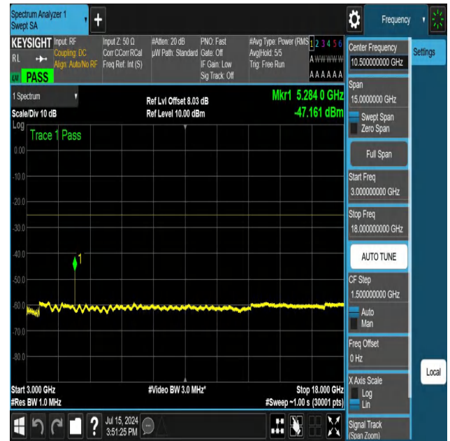
NTNV-N41-PC3-30-100-M-DFT-QPSK-Edge_1RB_Right-3000-1 8000-Ant1-PASS
