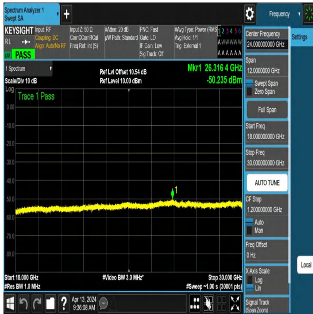
NTNV-N41-PC3-30-100-H-DFT-PI2BPSK-Edge_1RB_Left-18000-30000-Ant1-PASS
