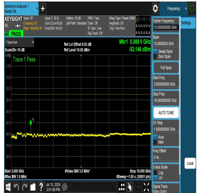
NTNV-N41-PC3-30-100-M-DFT-QPSK-Edge_1RB_Left-3000-180 00-Ant1-PASS
