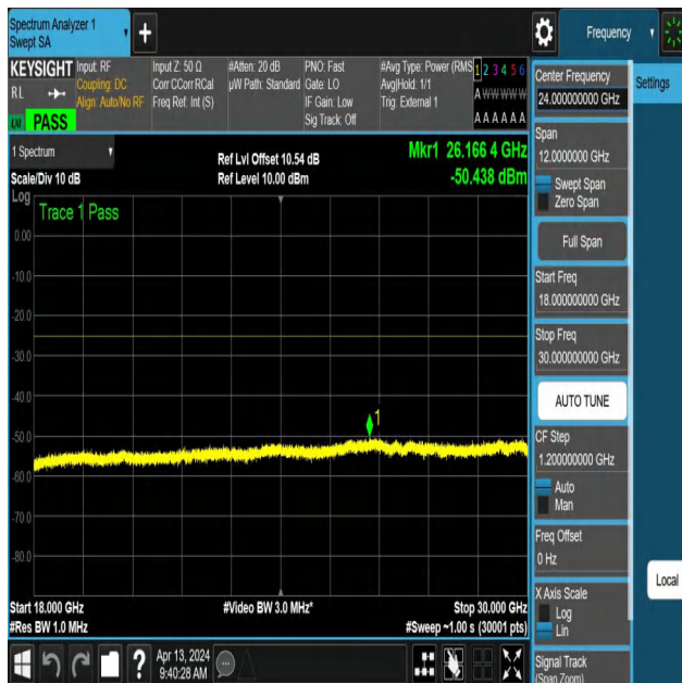
NTNV-N41-PC3-30-100-H-DFT-PI2BPSK-Edge_1RB_Right-18000 -30000-Ant1-PASS
