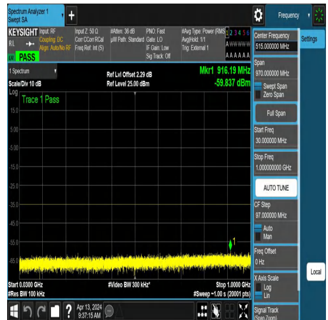
NTNV-N41-PC3-30-100-H-DFT-PI2BPSK-Edge_1RB_Right-30-1 000-Ant1-PASS
