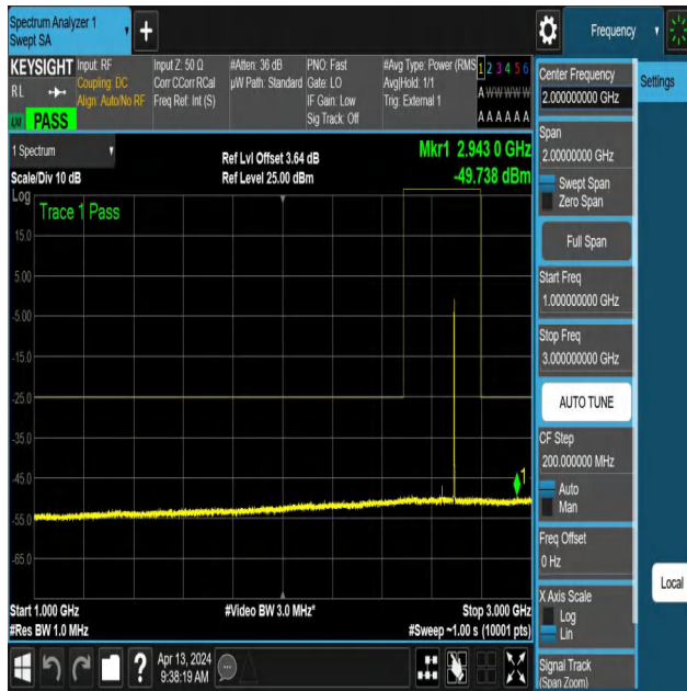
NTNV-N41-PC3-30-100-H-DFT-PI2BPSK-Edge_1RB_Right-1000-3000-Ant1-PASS
