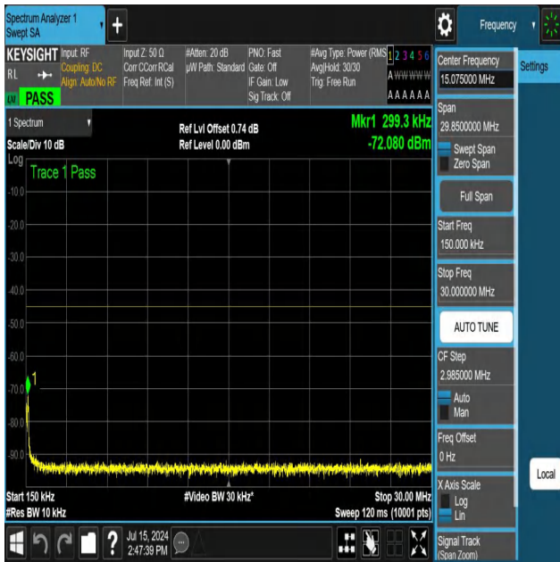
NTNV-N41-PC3-30-100-M-DFT-PI2BPSK-Edge_1RB_Right-0.15-30-Ant1-PASS
