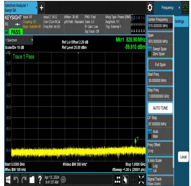
NTNV-N41-PC3-30-100-H-DFT-QPSK-Edge_1RB_Left-30-1000- Ant1-PASS
