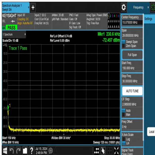
NTNV-N41-PC3-30-100-H-DFT-PI2BPSK-Edge_1RB_Right-0.15-30-Ant1-PASS
