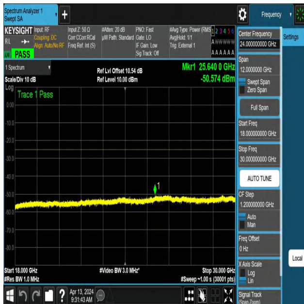
NTNV-N41-PC3-30-100-M-DFT-QPSK-Edge_1RB_Right-18000-3 0000-Ant1-PASS
