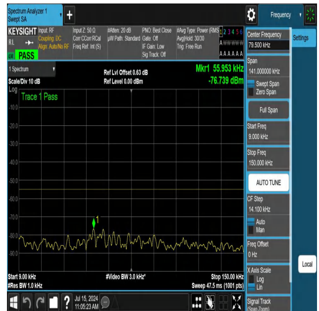
NTNV-N41-PC3-30-100-H-DFT-PI2BPSK-Edge_1RB_Left-0.009- 0.15-Ant1-PASS
