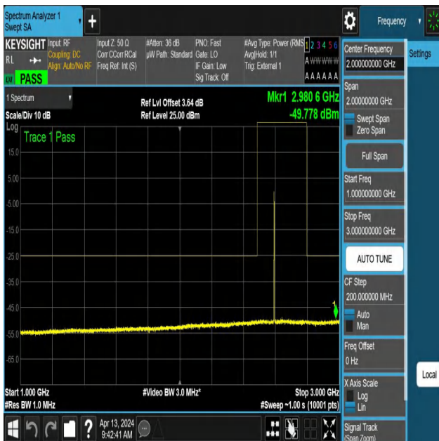
NTNV-N41-PC3-30-100-H-DFT-QPSK-Edge_1RB_Left-1000-3000 -Ant1-PASS
