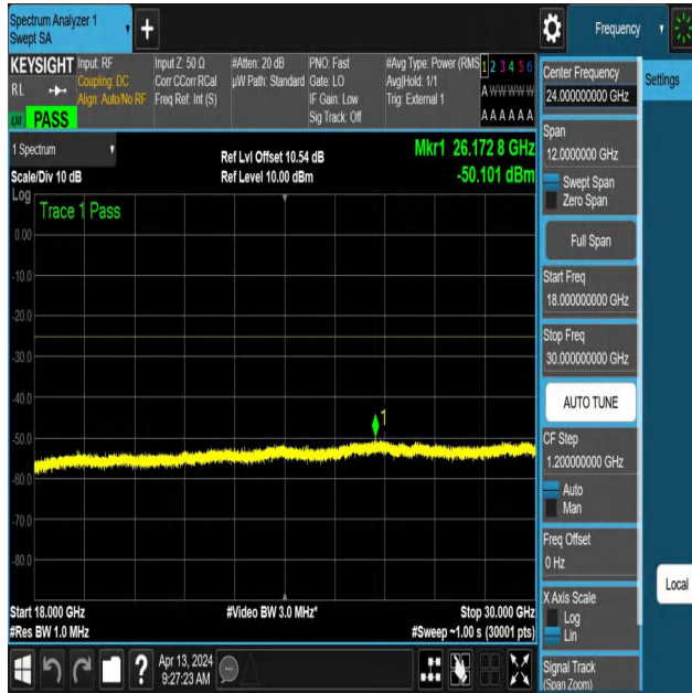
NTNV-N41-PC3-30-100-M-DFT-QPSK-Edge_1RB_Left-18000-30000-Ant1-PASS
