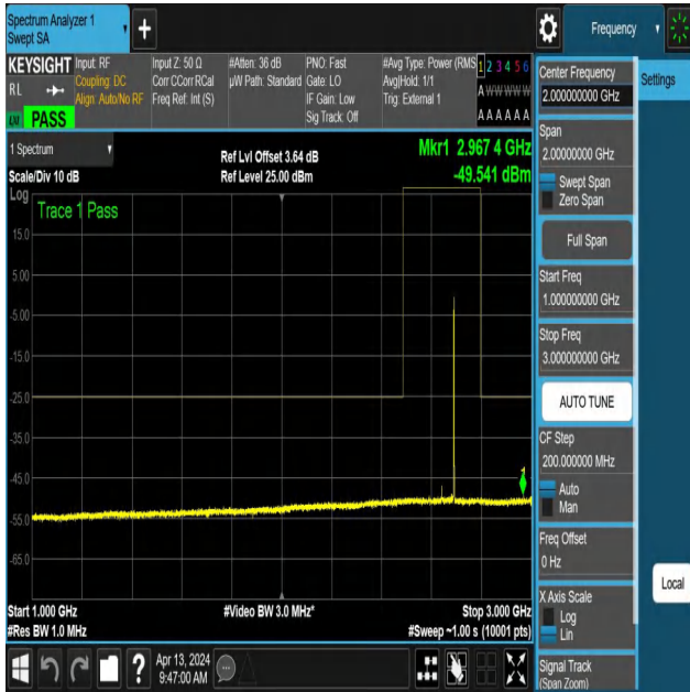
NTNV-N41-PC3-30-100-H-DFT-QPSK-Edge_1RB_Right-1000-30 00-Ant1-PASS
