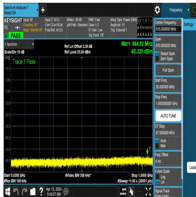
NTNV-N41-PC3-30-100-H-DFT-QPSK-Edge_1RB_Right-30-1000 -Ant1-PASS
