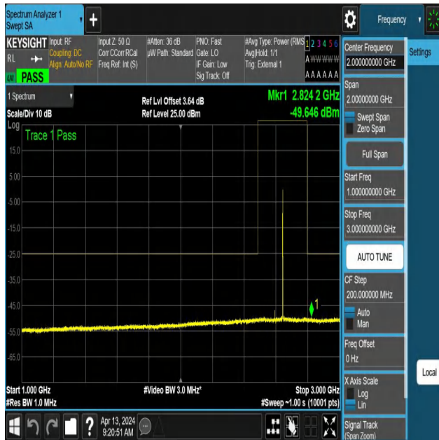
NTNV-N41-PC3-30-100-M-DFT-PI2BPSK-Edge_1RB_Right-1000-3000-Ant1-PASS
