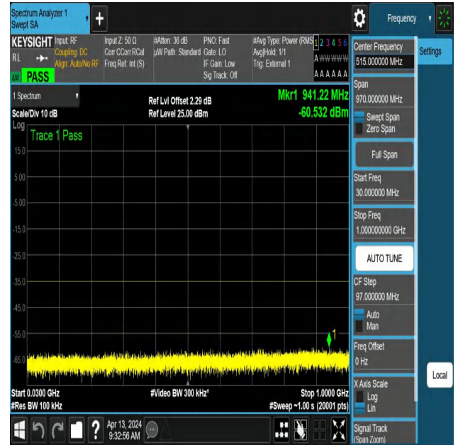
NTNV-N41-PC3-30-100-H-DFT-PI2BPSK-Edge_1RB_Left-30-10 00-Ant1-PASS
