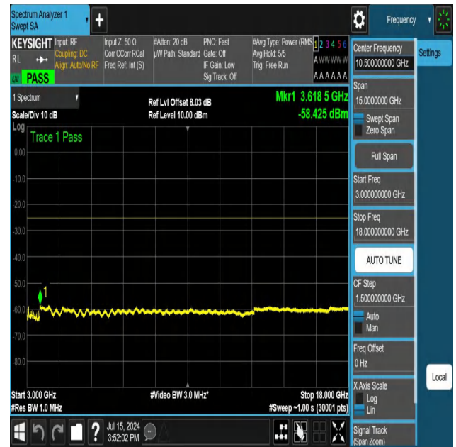
NTNV-N41-PC3-30-100-H-DFT-PI2BPSK-Edge_1RB_Right-3000 -18000-Ant1-PASS
