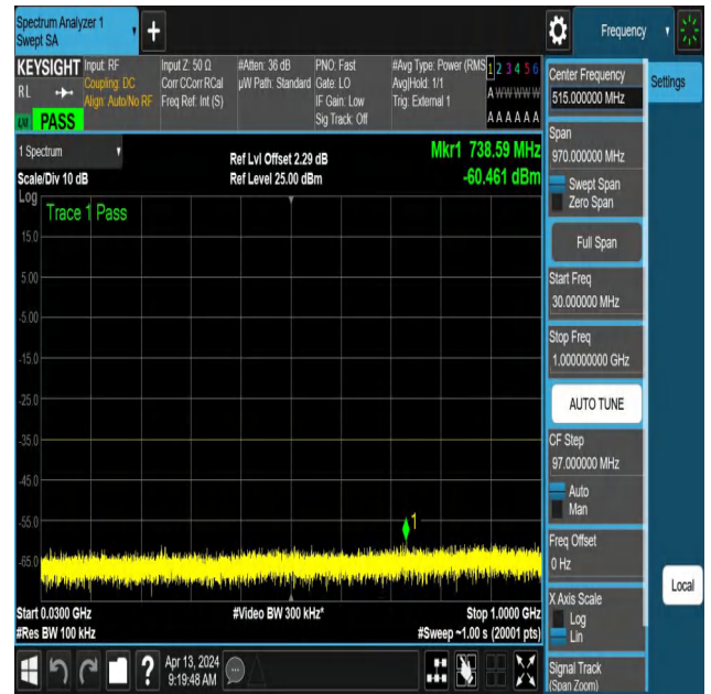
NTNV-N41-PC3-30-100-M-DFT-PI2BPSK-Edge_1RB_Right-30-1 000-Ant1-PASS
