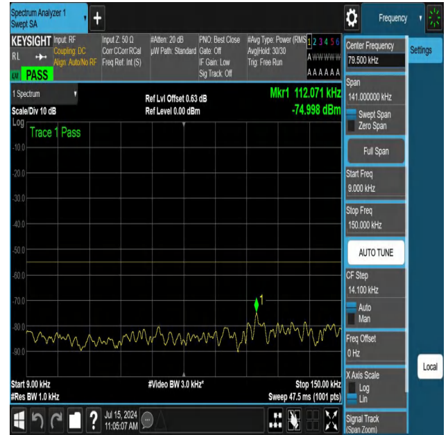
NTNV-N41-PC3-30-100-M-DFT-QPSK-Edge_1RB_Right-0.009-0.15-Ant1-PASS
