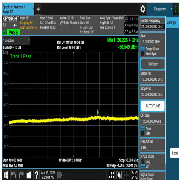
NTNV-N41-PC3-30-100-M-DFT-PI2BPSK-Edge_1RB_Right-1800 0-30000-Ant1-PASS
