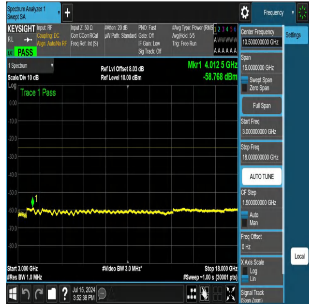
NTNV-N41-PC3-30-100-H-DFT-QPSK-Edge_1RB_Right-3000-18 000-Ant1-PASS
