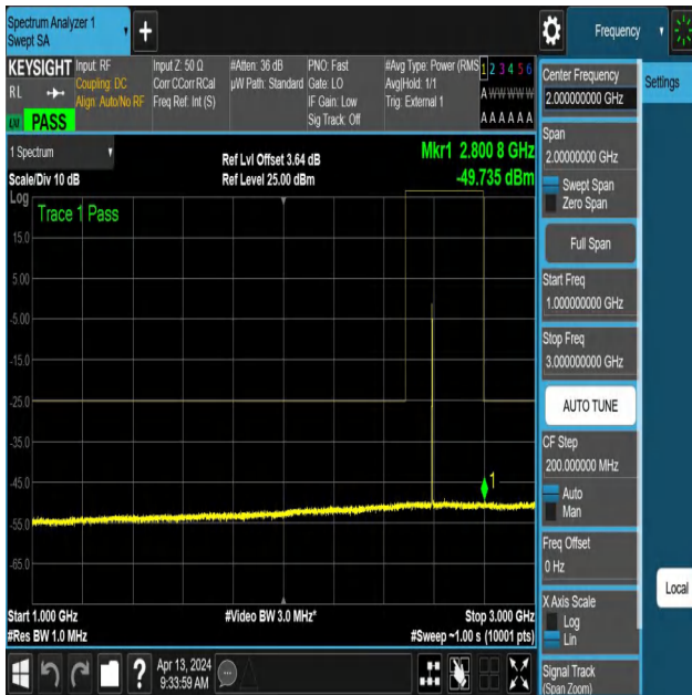
NTNV-N41-PC3-30-100-H-DFT-PI2BPSK-Edge_1RB_Left-1000-3 000-Ant1-PASS
