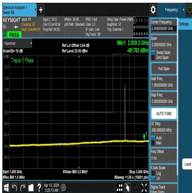
NTNV-N41-PC3-30-30-H-DFT-PI2BPSK-Edge_1RB_Left-1000-30 00-Ant1-PASS
