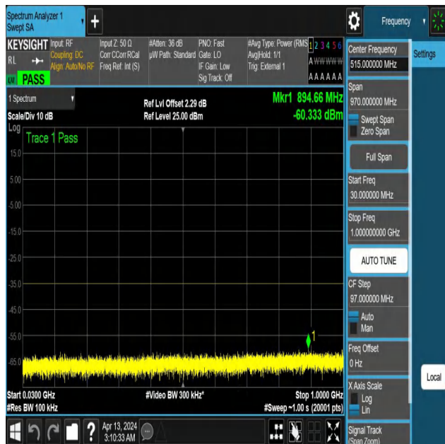
NTNV-N41-PC3-30-30-M-DFT-PI2BPSK-Edge_1RB_Right-30-100 0-Ant1-PASS
