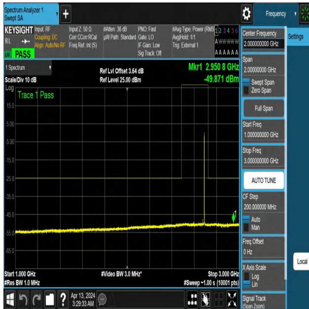
NTNV-N41-PC3-30-30-H-DFT-PI2BPSK-Edge_1RB_Right-1000-3 000-Ant1-PASS
