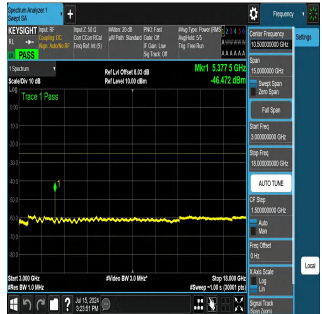
NTNV-N41-PC3-30-30-H-DFT-QPSK-Edge_1RB_Right-3000-180 00-Ant1-PASS
