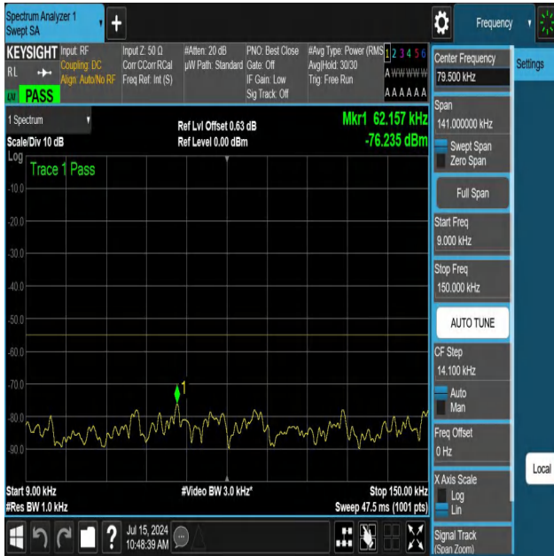
NTNV-N41-PC3-30-30-M-DFT-QPSK-Edge_1RB_Left-0.009-0.15-Ant1-PASS
