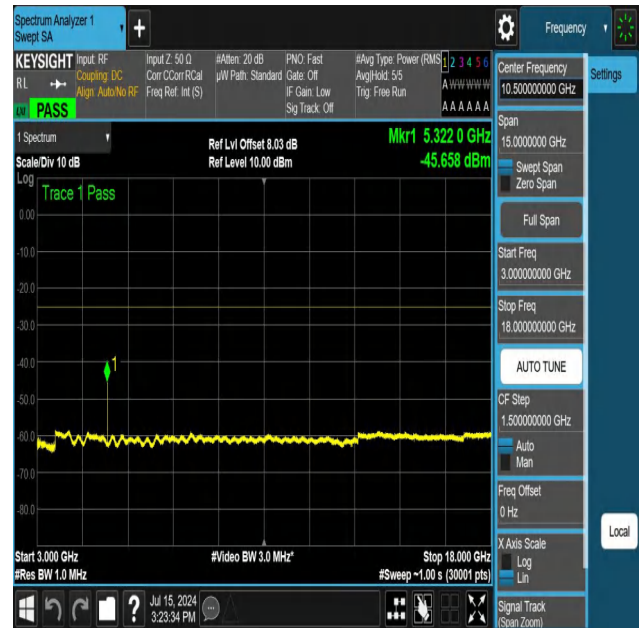
NTNV-N41-PC3-30-30-H-DFT-QPSK-Edge_1RB_Left-3000-1800 0-Ant1-PASS
