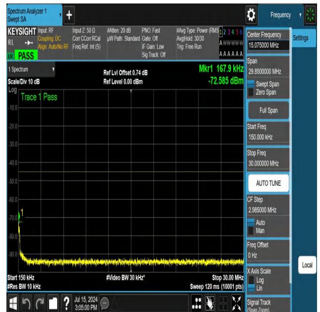
NTNV-N41-PC3-30-20-H-DFT-QPSK-Edge_1RB_Right-0.15-30- Ant1-PASS
