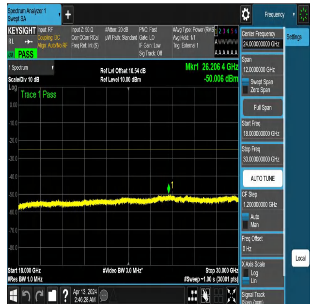
NTNV-N41-PC3-30-20-H-DFT-QPSK-Edge_1RB_Right-18000-30 000-Ant1-PASS
