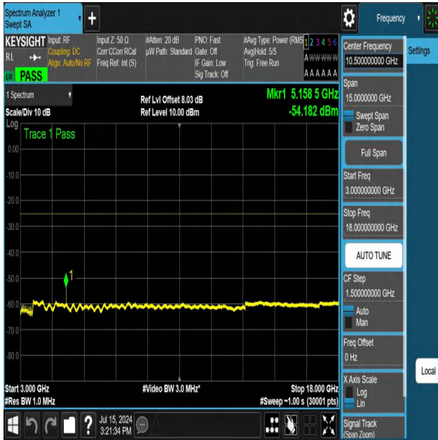
NTNV-N41-PC3-30-30-M-DFT-PI2BPSK-Edge_1RB_Left-3000-18000-Ant1-PASS
