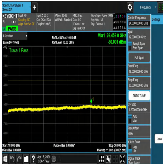
NTNV-N41-PC3-30-30-H-DFT-QPSK-Edge_1RB_Left-18000-3000 0-Ant1-PASS
