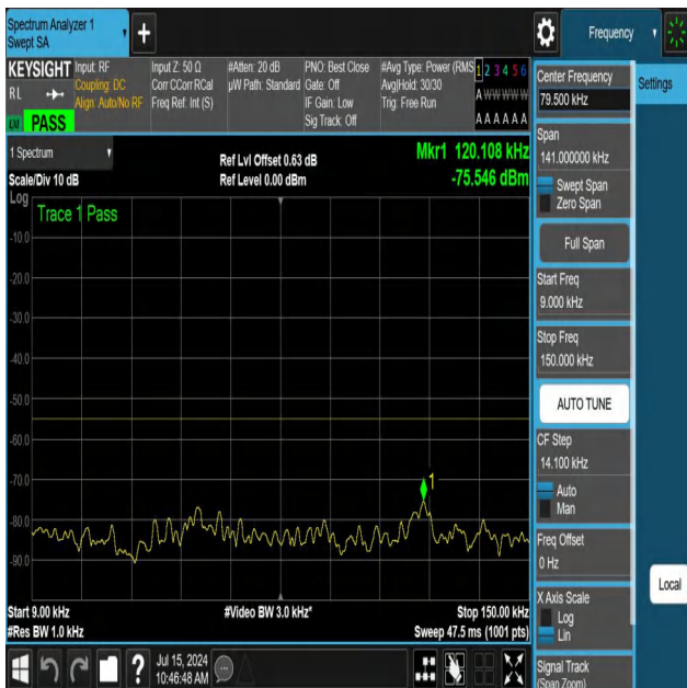
NTNV-N41-PC3-30-20-H-DFT-QPSK-Edge_1RB_Right-0.009-0.1 5-Ant1-PASS
