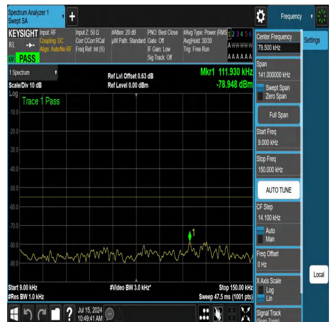
NTNV-N41-PC3-30-40-L-DFT-PI2BPSK-Edge_1RB_Left-0.009-0. 15-Ant1-PASS
