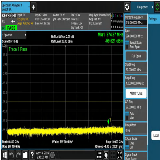
NTNV-N41-PC3-30-30-L-DFT-PI2BPSK-Edge_1RB_Left-30-1000-Ant1-PASS
