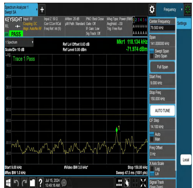
NTNV-N41-PC3-30-30-H-DFT-QPSK-Edge_1RB_Left-0.009-0.15 -Ant1-PASS
