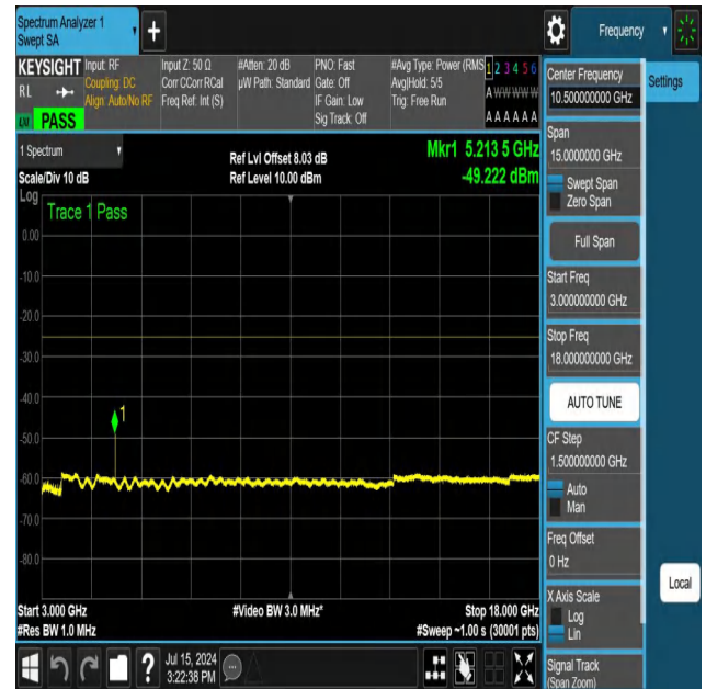
NTNV-N41-PC3-30-30-M-DFT-QPSK-Edge_1RB_Right-3000-18 000-Ant1-PASS
