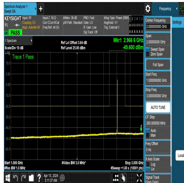
NTNV-N41-PC3-30-30-M-DFT-PI2BPSK-Edge_1RB_Right-1000-3000-Ant1-PASS
