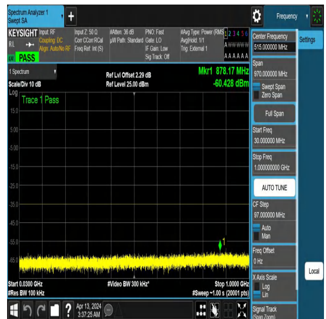
NTNV-N41-PC3-30-30-H-DFT-QPSK-Edge_1RB_Right-30-1000- Ant1-PASS
