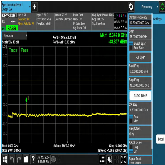
NTNV-N41-PC3-30-20-H-DFT-QPSK-Edge_1RB_Left-3000-18000 -Ant1-PASS
