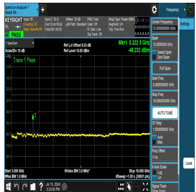
NTNV-N41-PC3-30-30-H-DFT-PI2BPSK-Edge_1RB_Left-3000-1 8000-Ant1-PASS
