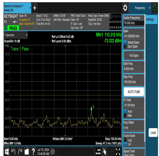
NTNV-N41-PC3-30-30-H-DFT-PI2BPSK-Edge_1RB_Left-0.009-0.15-Ant1-PASS
