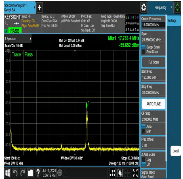
NTNV-N41-PC3-30-30-M-DFT-PI2BPSK-Edge_1RB_Left-0.15-30 -Ant1-PASS
