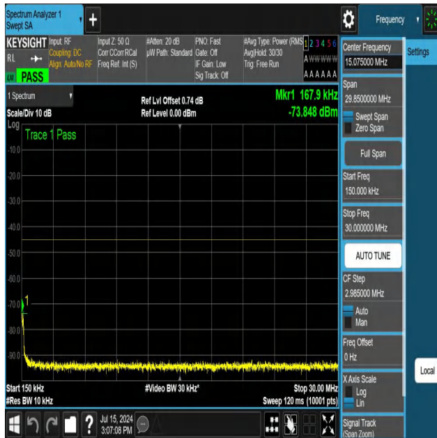
NTNV-N41-PC3-30-30-H-DFT-PI2BPSK-Edge_1RB_Left-0.15-30-Ant1-PASS
