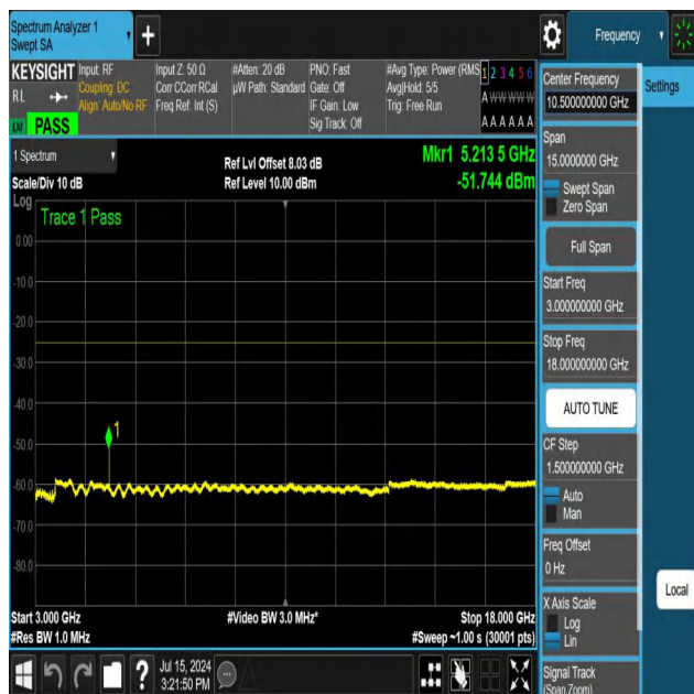
NTNV-N41-PC3-30-30-M-DFT-PI2BPSK-Edge_1RB_Right-3000-1 8000-Ant1-PASS
