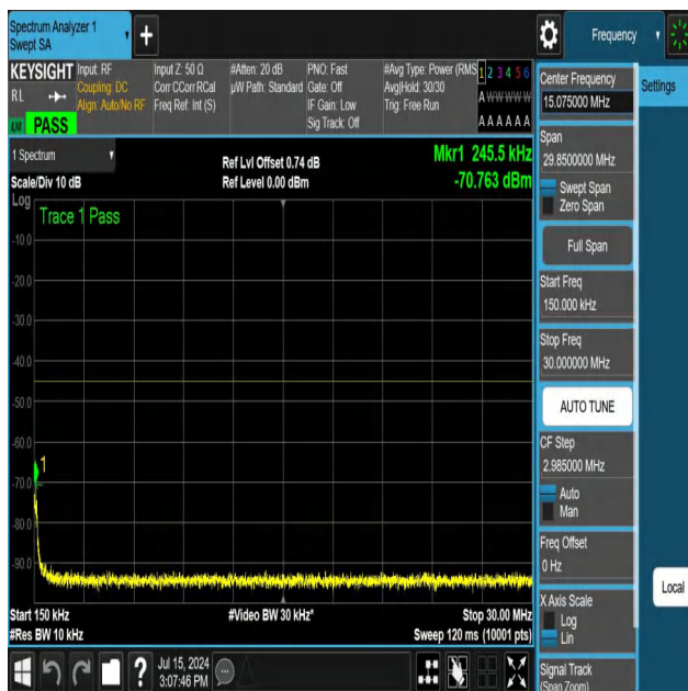
NTNV-N41-PC3-30-30-H-DFT-QPSK-Edge_1RB_Right-0.15-30-A nt1-PASS
