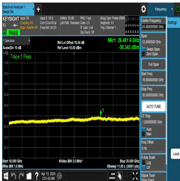
NTNV-N41-PC3-30-30-H-DFT-PI2BPSK-Edge_1RB_Right-18000-30000-Ant1-PASS
