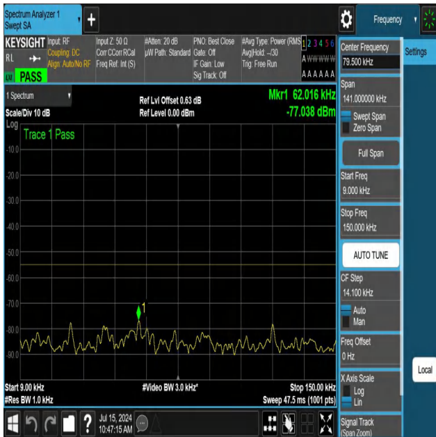
NTNV-N41-PC3-30-30-L-DFT-PI2BPSK-Edge_1RB_Right-0.009-0.15-Ant1-PASS
