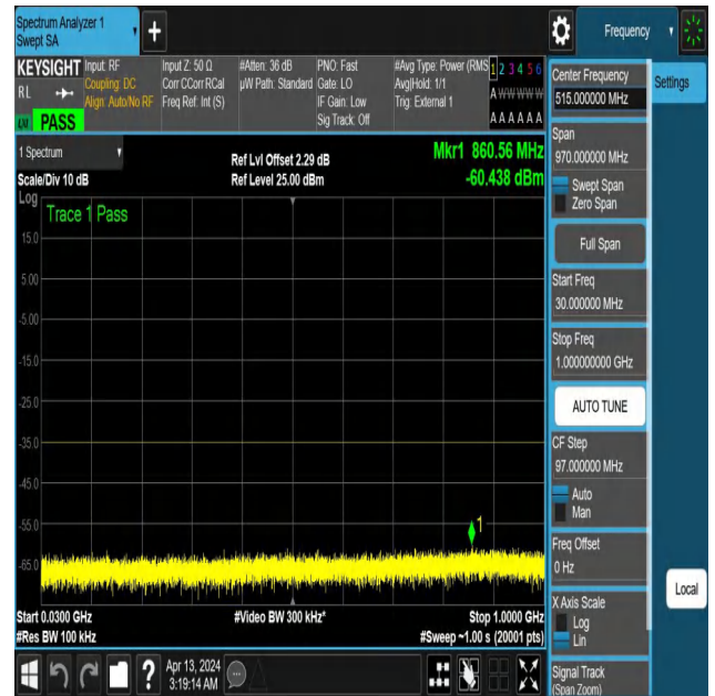
NTNV-N41-PC3-30-30-M-DFT-QPSK-Edge_1RB_Right-30-1000- Ant1-PASS
