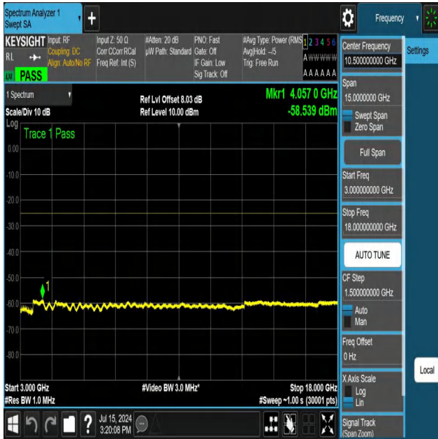
NTNV-N41-PC3-30-30-L-DFT-PI2BPSK-Edge_1RB_Left-3000-18000-Ant1-PASS
