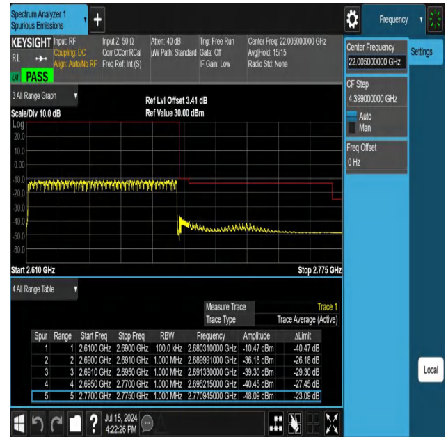
NTNV-N41-PC3-30-80-H-DFT-PI2BPSK-Outer_Full-Ant1-PASS
