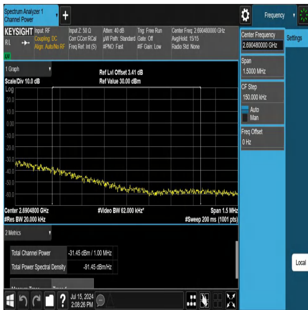
NTNV-N41-PC3-30-90-H-DFT-QPSK-Edge_1RB_Right-Ant1-PASS
