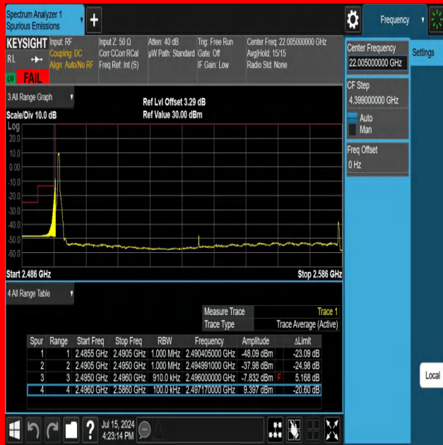
NTNV-N41-PC3-30-90-L-DFT-PI2BPSK-Edge_1RB_Left-Ant1-FA IL
