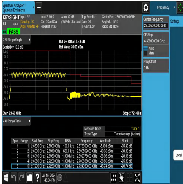
NTNV-N41-PC3-30-30-H-DFT-PI2BPSK-Outter_Full-Ant1-PASS
