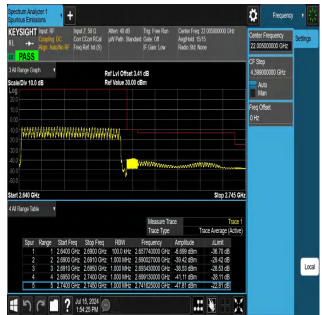
NTNV-N41-PC3-30-50-H-DFT-PI2BPSK-Outer_Full-Ant1-PASS
