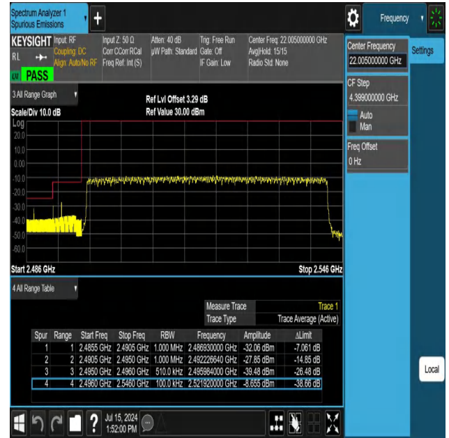
NTNV-N41-PC3-30-50-L-DFT-PI2BPSK-Outer_Full-Ant1-PASS
