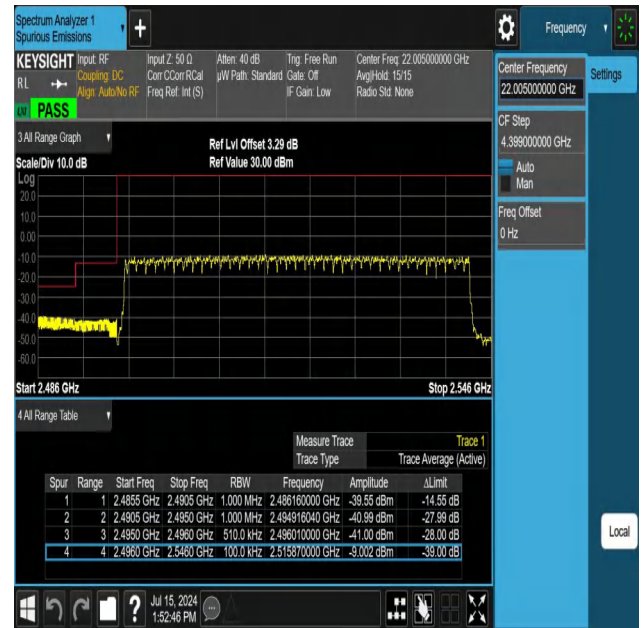
NTNV-N41-PC3-30-50-L-DFT-QPSK-Outer_Full-Ant1-PASS
