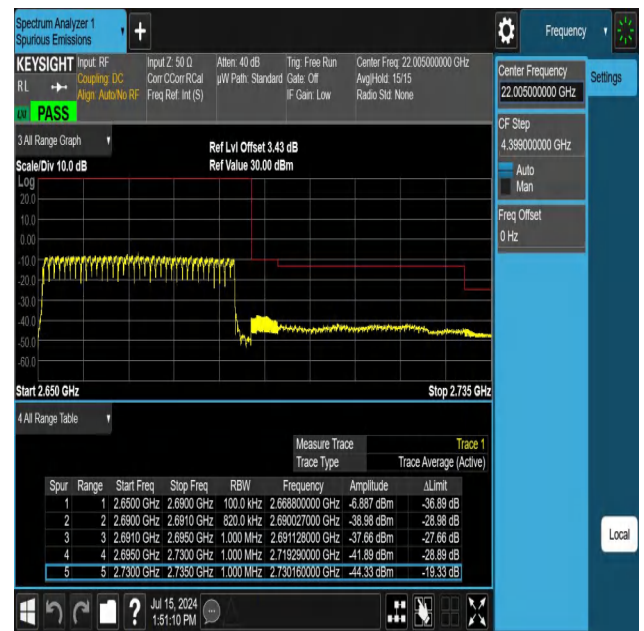
NTNV-N41-PC3-30-40-H-DFT-PI2BPSK-Outer_Full-Ant1-PASS
