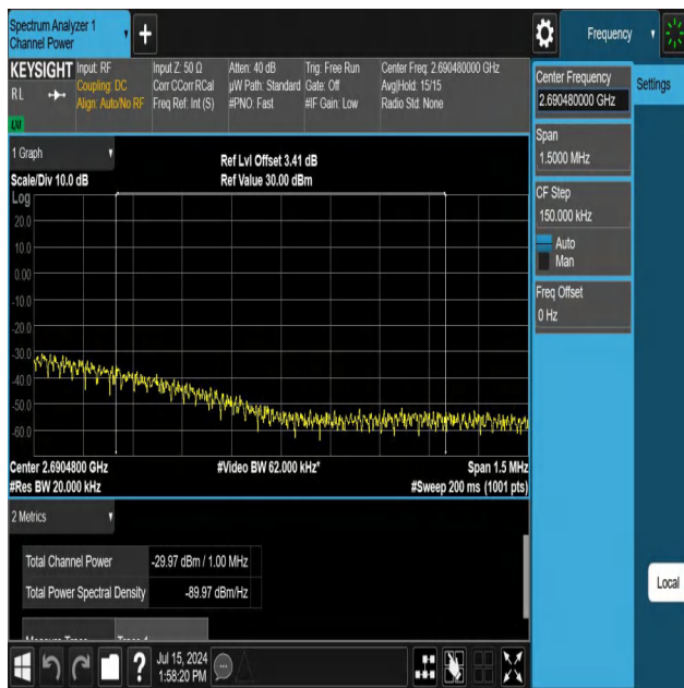
NTNV-N41-PC3-30-60-H-DFT-QPSK-Edge_1RB_Right-Ant1-PASS
