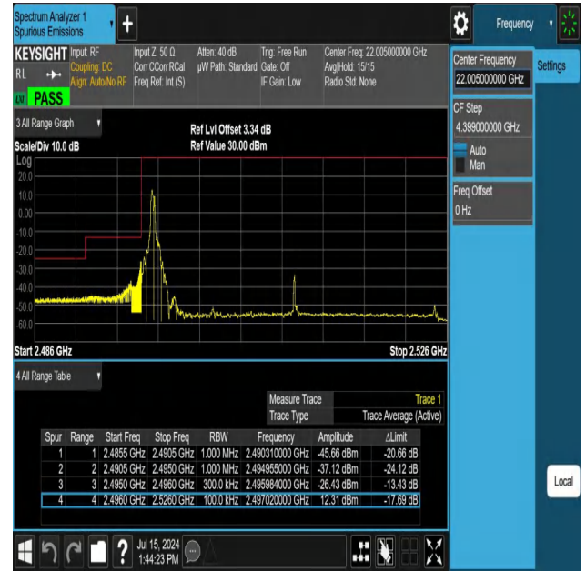
NTNV-N41-PC3-30-30-L-DFT-PI2BPSK-Edge_1RB_Left-Ant1-PASS
