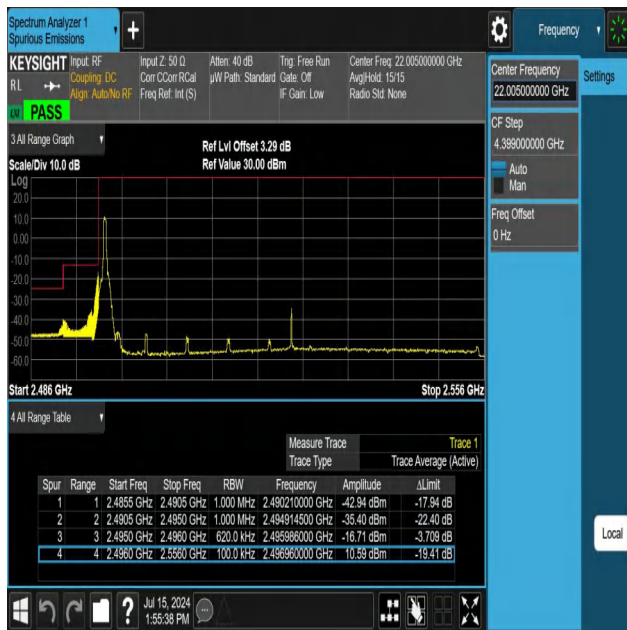
NTNV-N41-PC3-30-60-L-DFT-PI2BPSK-Edge_1RB_Left-Ant1-PA SS
