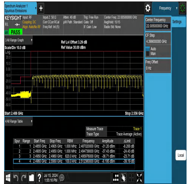
NTNV-N41-PC3-30-60-L-DFT-PI2BPSK-Outer_Full-Ant1-PASS
