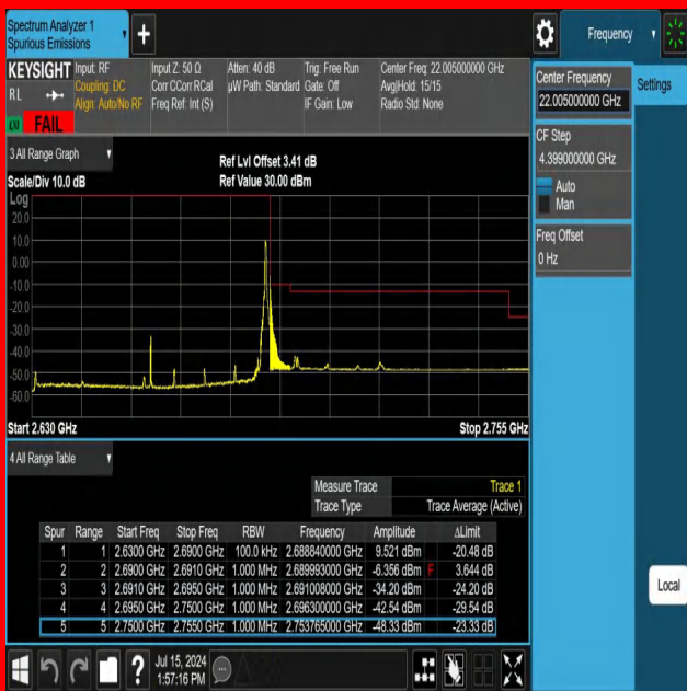
NTNV-N41-PC3-30-60-H-DFT-PI2BPSK-Edge_1RB_Right-Ant1- FAIL
