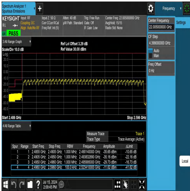
NTNV-N41-PC3-30-100-L-DFT-QPSK-Outer_Full-Ant1-PASS
