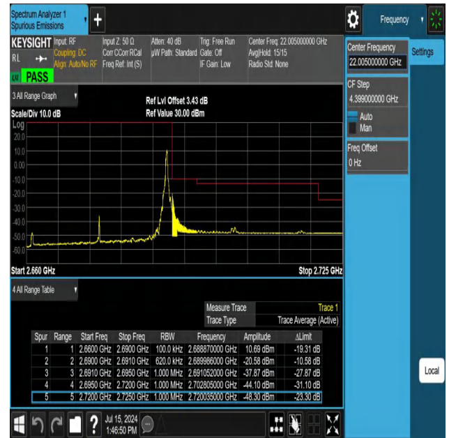
NTNV-N41-PC3-30-30-H-DFT-QPSK-Edge_1RB_Right-Ant1-PASS
