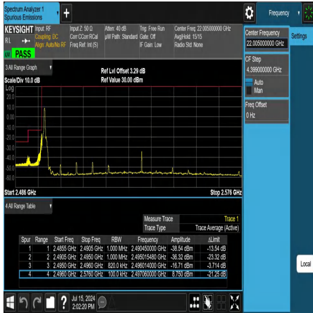
NTNV-N41-PC3-30-80-L-DFT-PI2BPSK-Edge_1RB_Left-Ant1-PA SS
