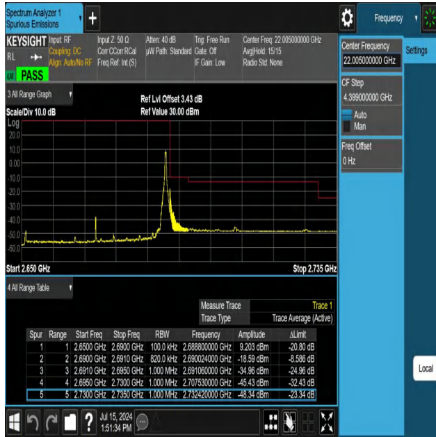
NTNV-N41-PC3-30-40-H-DFT-QPSK-Edge_1RB_Right-Ant1-PA SS
