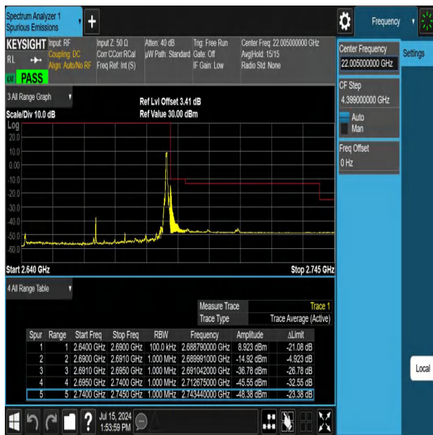
NTNV-N41-PC3-30-50-H-DFT-PI2BPSK-Edge_1RB_Right-Ant1-PASS
