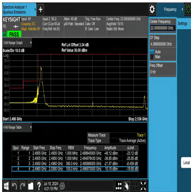
NTNV-N41-PC3-30-40-L-DFT-PI2BPSK-Edge_1RB_Left-Ant1-PASS
