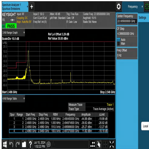
NTNV-N41-PC3-30-50-L-DFT-PI2BPSK-Edge_1RB_Left-Ant1-PA SS
