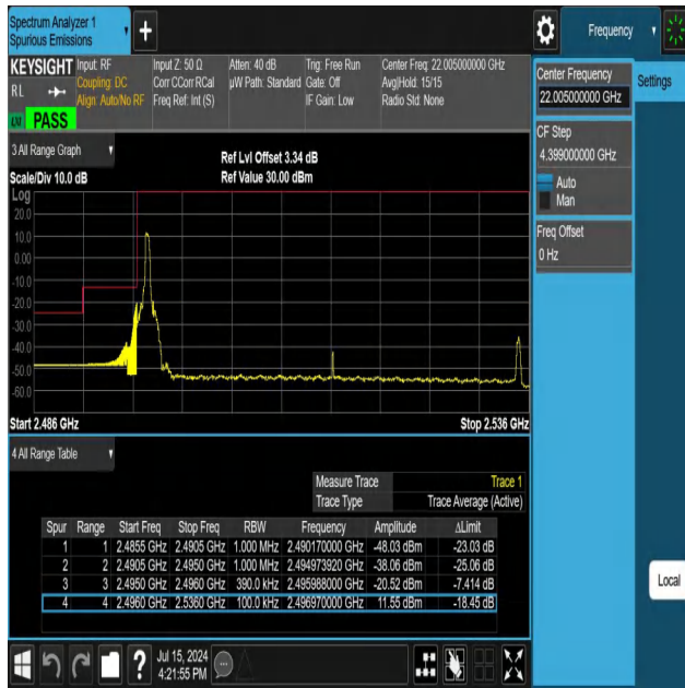
NTNV-N41-PC3-30-40-L-DFT-QPSK-Edge_1RB_Left-Ant1-PASS
