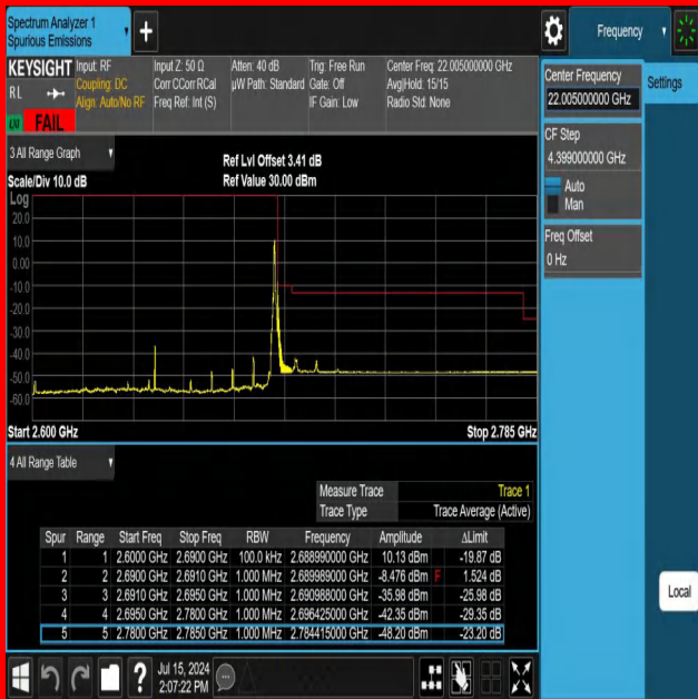
NTNV-N41-PC3-30-90-H-DFT-PI2BPSK-Edge_1RB_Right-Ant1- FAIL
