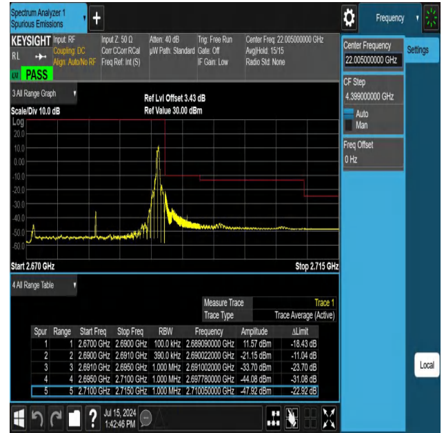
NTNV-N41-PC3-30-20-H-DFT-PI2BPSK-Edge_1RB_Right-Ant1-PASS
