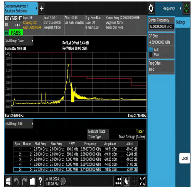
NTNV-N41-PC3-30-20-H-DFT-QPSK-Edge_1RB_Right-Ant1-PASS
