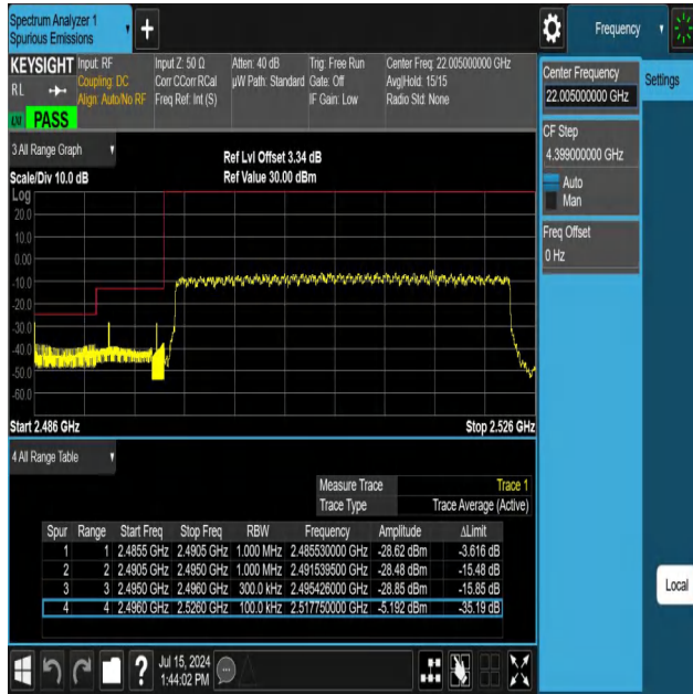
NTNV-N41-PC3-30-30-L-DFT-PI2BPSK-Outer_Full-Ant1-PASS
