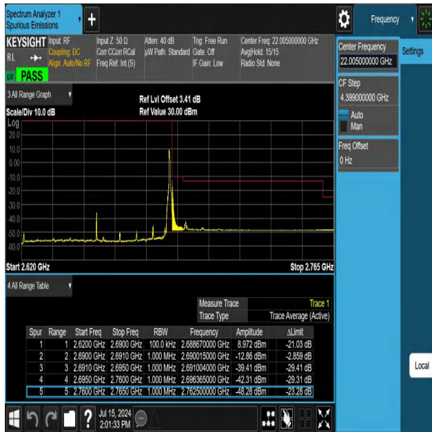
NTNV-N41-PC3-30-70-H-DFT-QPSK-Edge_1RB_Right-Ant1-PASS
