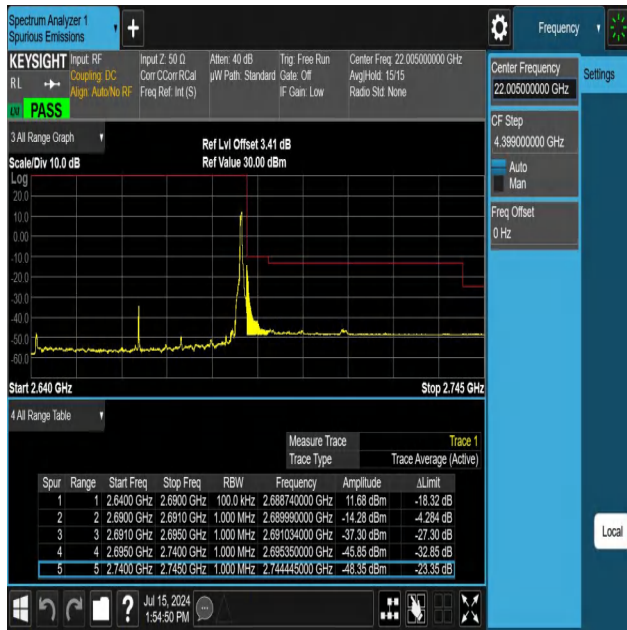
NTNV-N41-PC3-30-50-H-DFT-QPSK-Edge_1RB_Right-Ant1-PA SS
