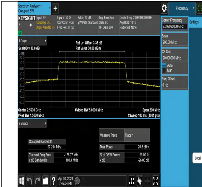
NTNV-N41-PC3-30-100-M-CP-QPSK-Outter_Full-Ant1-PASS
