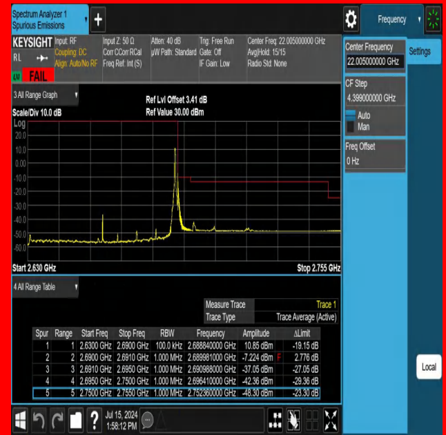
NTNV-N41-PC3-30-60-H-DFT-QPSK-Edge_1RB_Right-Ant1-FAIL
