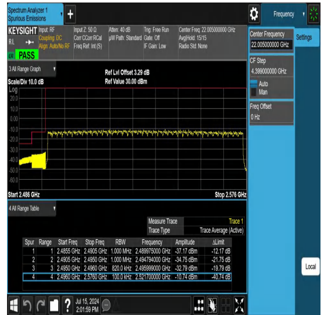
NTNV-N41-PC3-30-80-L-DFT-PI2BPSK-Outer_Full-Ant1-PASS
