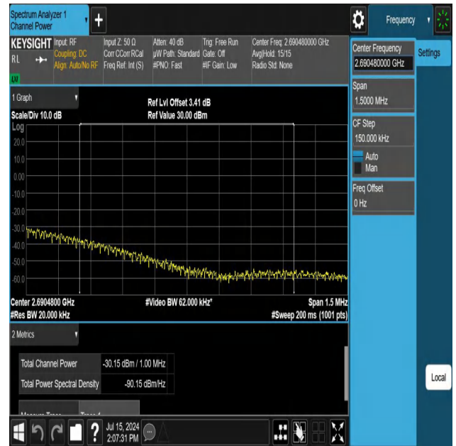
NTNV-N41-PC3-30-90-H-DFT-PI2BPSK-Edge_1RB_Right-Ant1-P ASS
