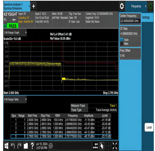
NTNV-N41-PC3-30-90-H-DFT-PI2BPSK-Outer_Full-Ant1-PASS
