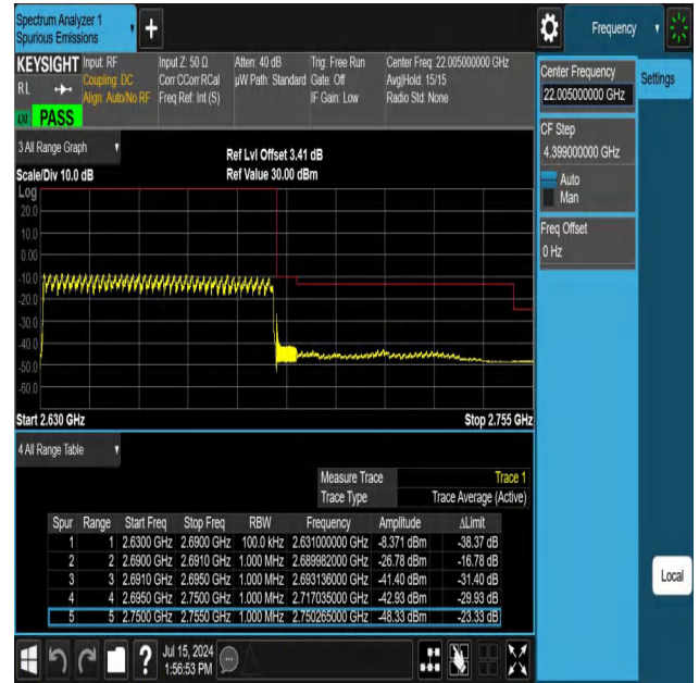
NTNV-N41-PC3-30-60-H-DFT-PI2BPSK-Outer_Full-Ant1-PASS
