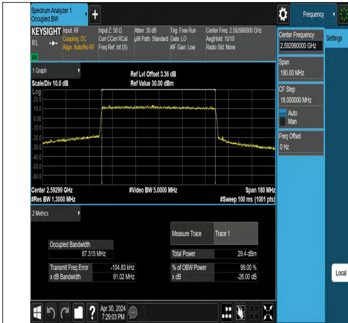
NTNV-N41-PC3-30-90-M-CP-QPSK-Outer_Full-Ant1-PASS
