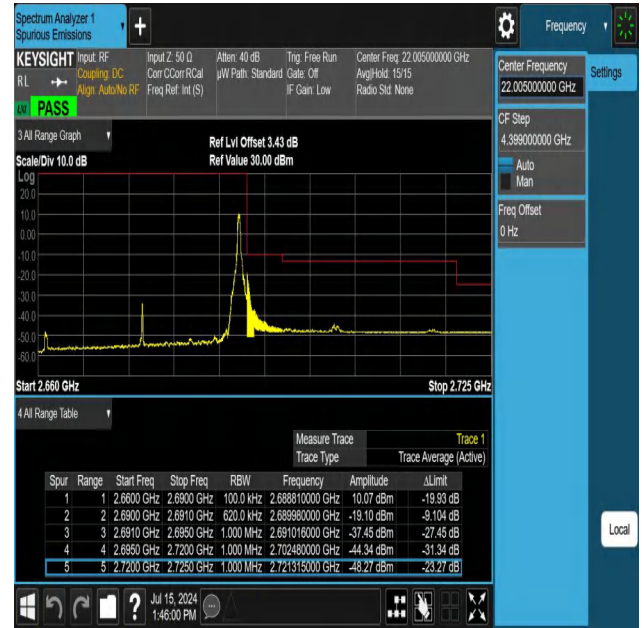
NTNV-N41-PC3-30-30-H-DFT-PI2BPSK-Edge_1RB_Right-Ant1-PASS
