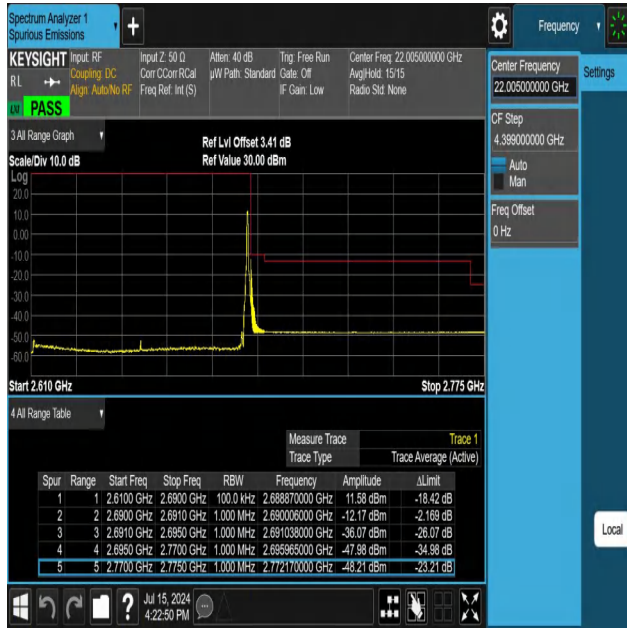
NTNV-N41-PC3-30-80-H-DFT-PI2BPSK-Edge_1RB_Right-Ant1-PASS
