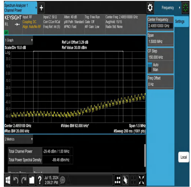
NTNV-N41-PC3-30-100-L-DFT-PI2BPSK-Edge_1RB_Left-Ant1-PA SS
