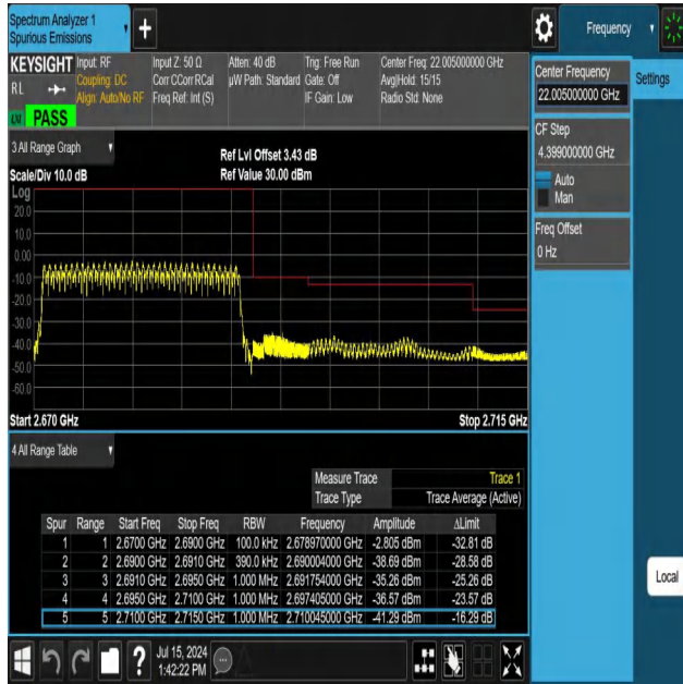
NTNV-N41-PC3-30-20-H-DFT-PI2BPSK-Outter_Full-Ant1-PASS
