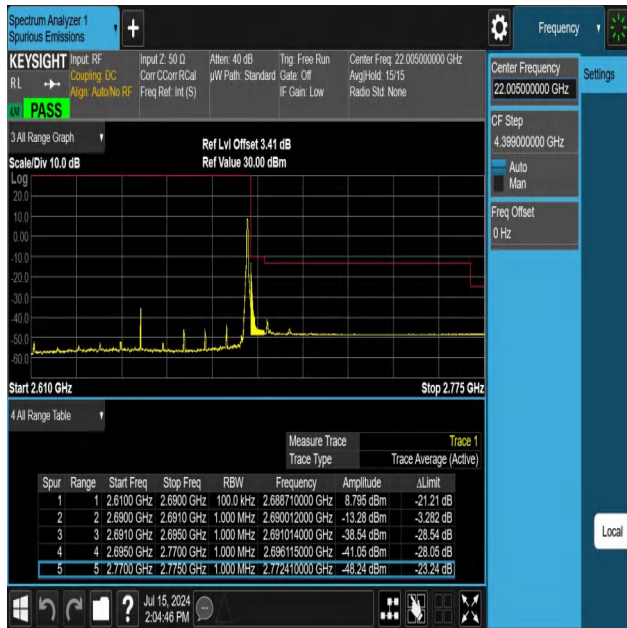
NTNV-N41-PC3-30-80-H-DFT-QPSK-Edge_1RB_Right-Ant1-PASS
