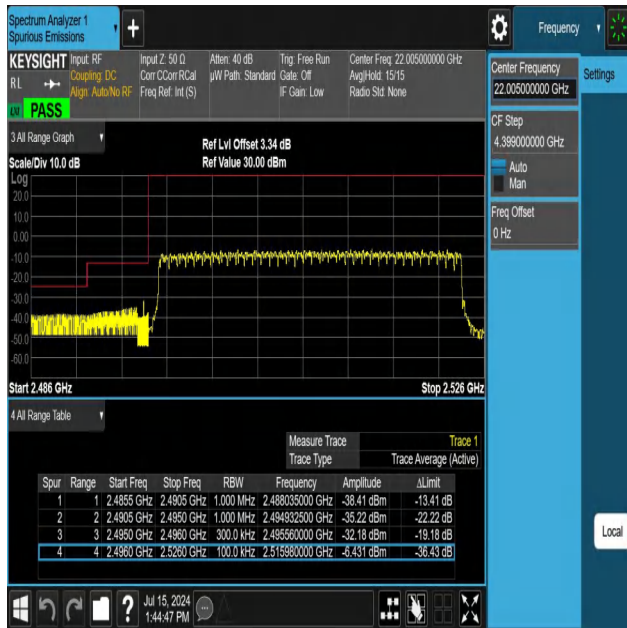
NTNV-N41-PC3-30-30-L-DFT-QPSK-Outer_Full-Ant1-PASS
