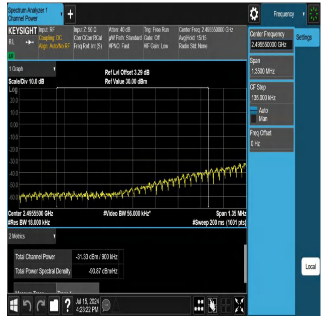
NTNV-N41-PC3-30-90-L-DFT-PI2BPSK-Edge_1RB_Left-Ant1-PA SS
