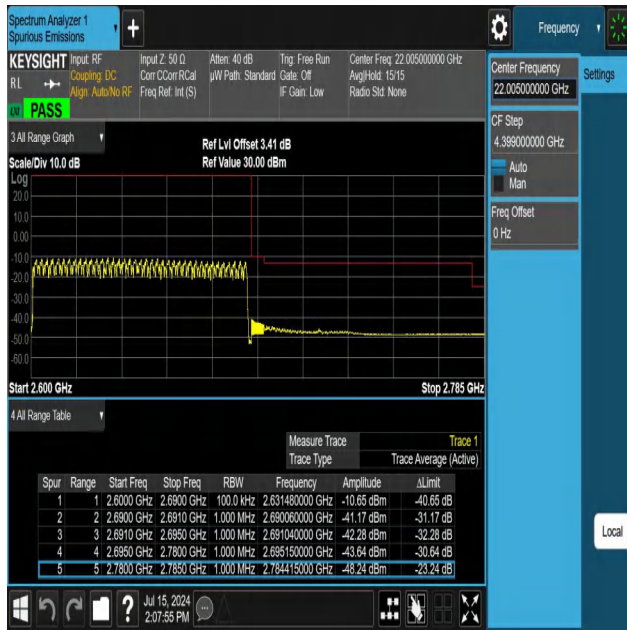
NTNV-N41-PC3-30-90-H-DFT-QPSK-Outer_Full-Ant1-PASS
