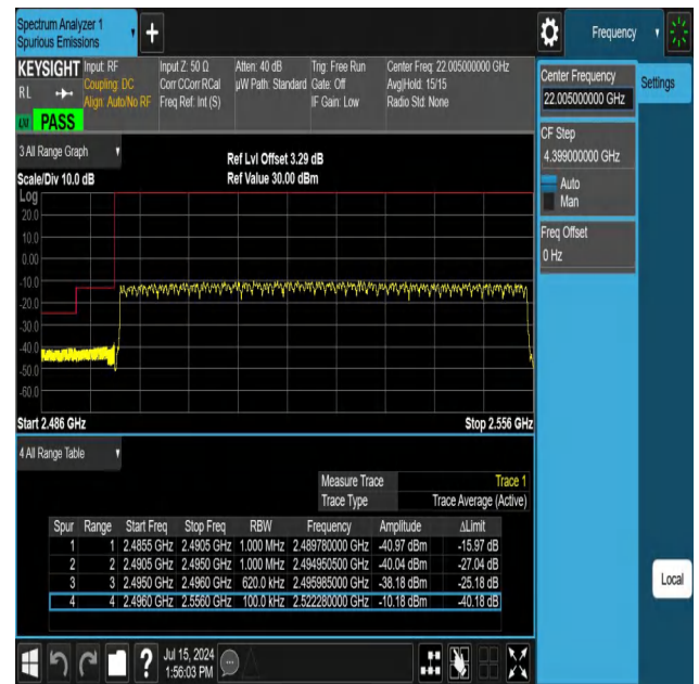
NTNV-N41-PC3-30-60-L-DFT-QPSK-Outer_Full-Ant1-PASS
