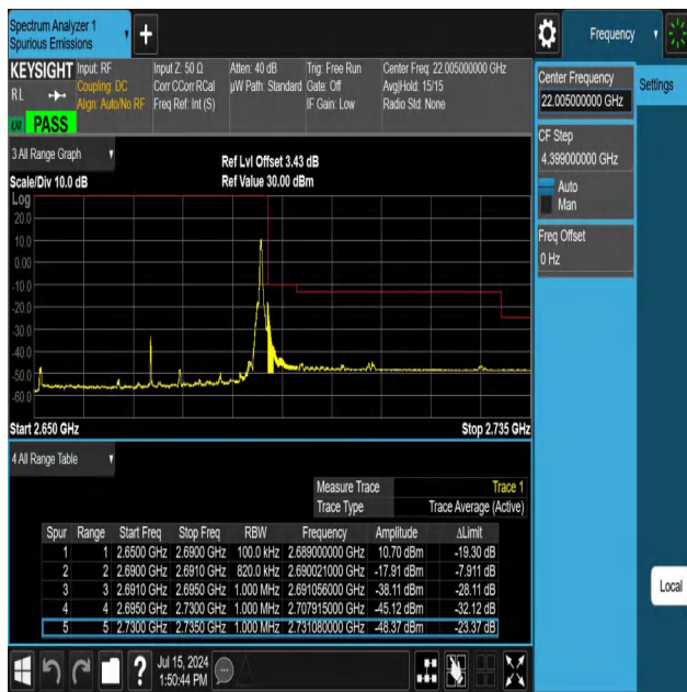
NTNV-N41-PC3-30-40-H-DFT-PI2BPSK-Edge_1RB_Right-Ant1-PASS
