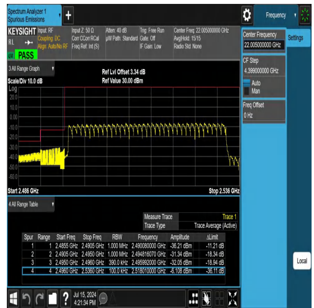
NTNV-N41-PC3-30-40-L-DFT-QPSK-Outer_Full-Ant1-PASS
