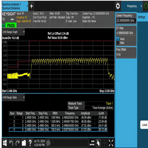
NTNV-N41-PC3-30-40-L-DFT-PI2BPSK-Outer_Full-Ant1-PASS
