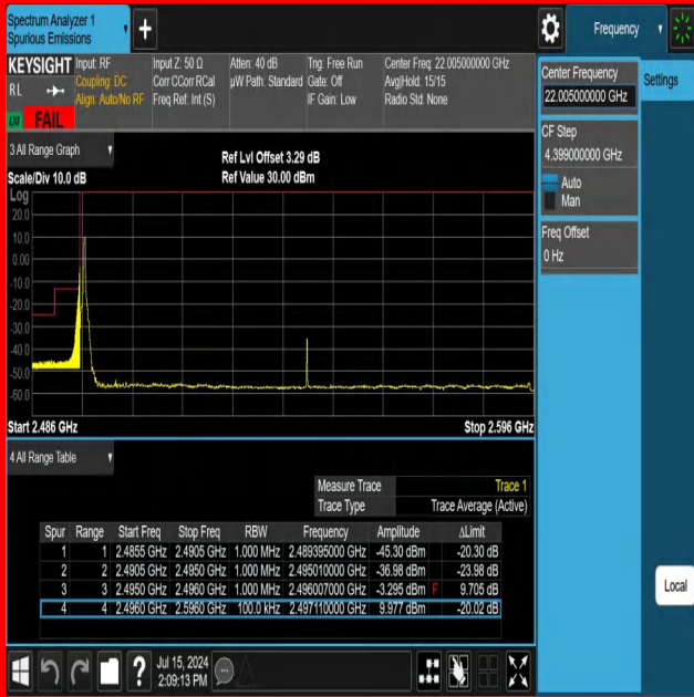
NTNV-N41-PC3-30-100-L-DFT-PI2BPSK-Edge_1RB_Left-Ant1-F AIL
