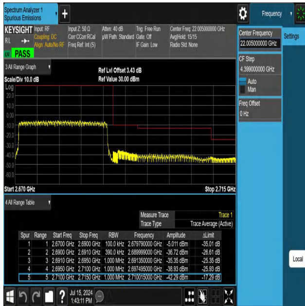
NTNV-N41-PC3-30-20-H-DFT-QPSK-Outter_Full-Ant1-PASS
