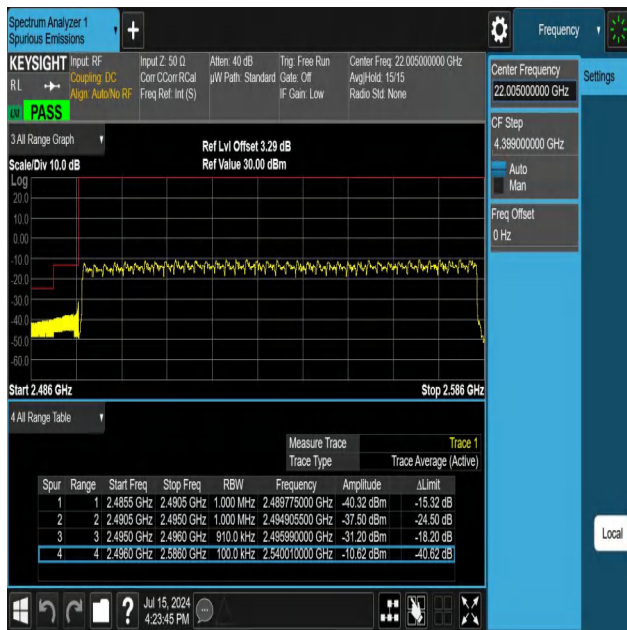
NTNV-N41-PC3-30-90-L-DFT-QPSK-Outer_Full-Ant1-PASS
