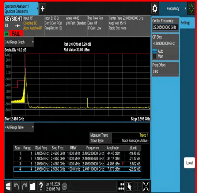
NTNV-N41-PC3-30-100-L-DFT-QPSK-Edge_1RB_Left-Ant1-FAIL
