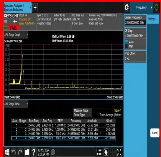
NTNV-N41-PC3-30-90-L-DFT-QPSK-Edge_1RB_Left-Ant1-FAIL
