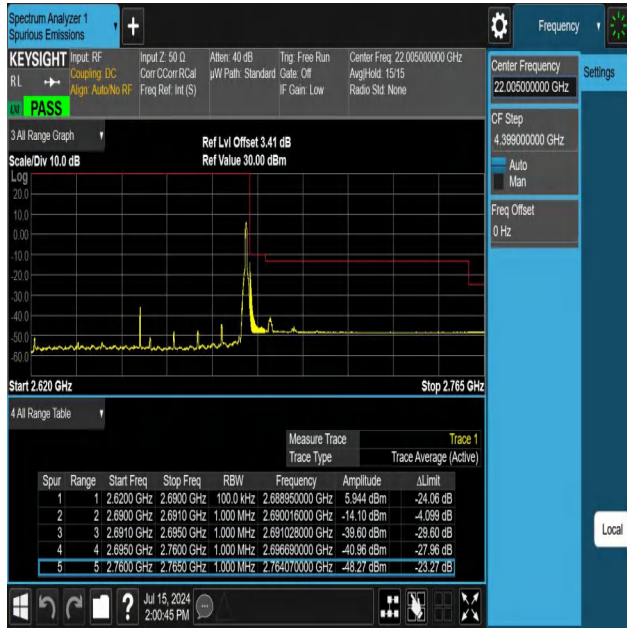
NTNV-N41-PC3-30-70-H-DFT-PI2BPSK-Edge_1RB_Right-Ant1-PASS
