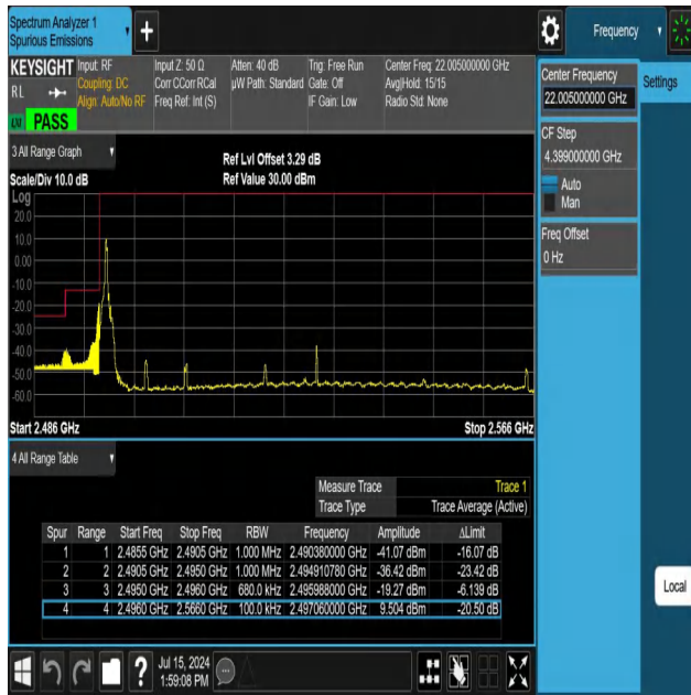
NTNV-N41-PC3-30-70-L-DFT-PI2BPSK-Edge_1RB_Left-Ant1-PA SS
