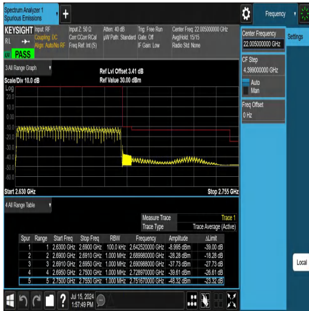
NTNV-N41-PC3-30-60-H-DFT-QPSK-Outer_Full-Ant1-PASS
