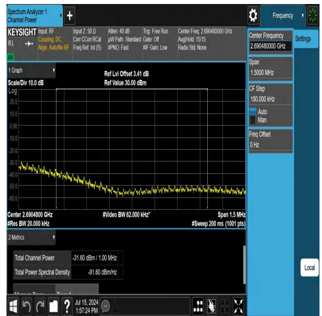
NTNV-N41-PC3-30-60-H-DFT-PI2BPSK-Edge_1RB_Right-Ant1-P ASS
