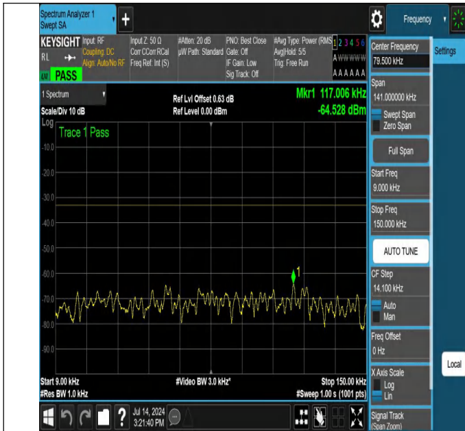
NTNV-N26-824-849-PC3-15-5-H-DFT-QPSK-Edge_1RB_Left-0.0 09-0.15-Ant1-PASS
