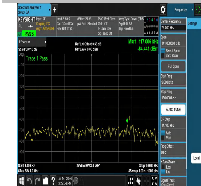
NTNV-N26-824-849-PC3-15-5-H-DFT-QPSK-Edge_1RB_Right-0. 009-0.15-Ant1-PASS
