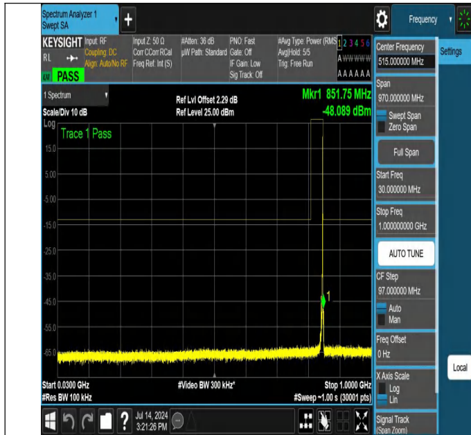
NTNV-N26-824-849-PC3-15-5-H-DFT-PI2BPSK-Edge_1RB_Righ t-30-1000-Ant1-PASS
