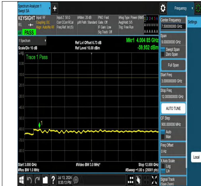
NTNV-N26-824-849-PC3-15-10-M-DFT-PI2BPSK-Edge_1RB_Lef t-3000-12000-Ant1-PASS
