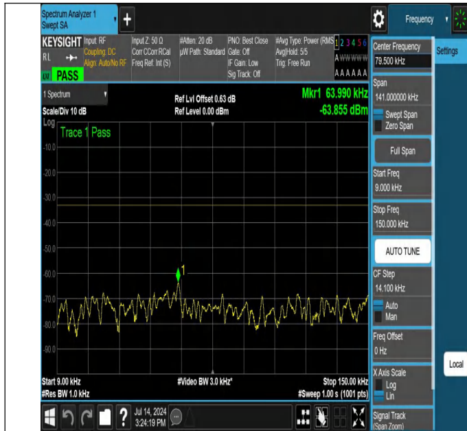
NTNV-N26-824-849-PC3-15-10-M-DFT-PI2BPSK-Edge_1RB_Left t-0.009-0.15-Ant1-PASS
