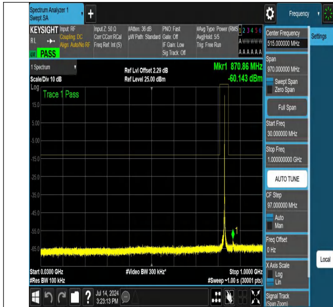
NTNV-N26-824-849-PC3-15-10-L-DFT-PI2BPSK-Edge_1RB_Rig ht-30-1000-Ant1-PASS
