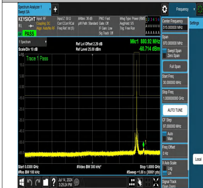
NTNV-N26-824-849-PC3-15-10-M-DFT-QPSK-Edge_1RB_Left-3 0-1000-Ant1-PASS
