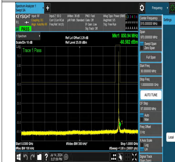
NTNV-N26-824-849-PC3-15-10-H-DFT-QPSK-Edge_1RB_Left-3
