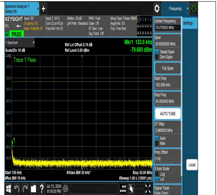
NTNV-N26-824-849-PC3-15-10-L-DFT-PI2BPSK-Edge_1RB_Left 0.15-30-Ant1-PASS
