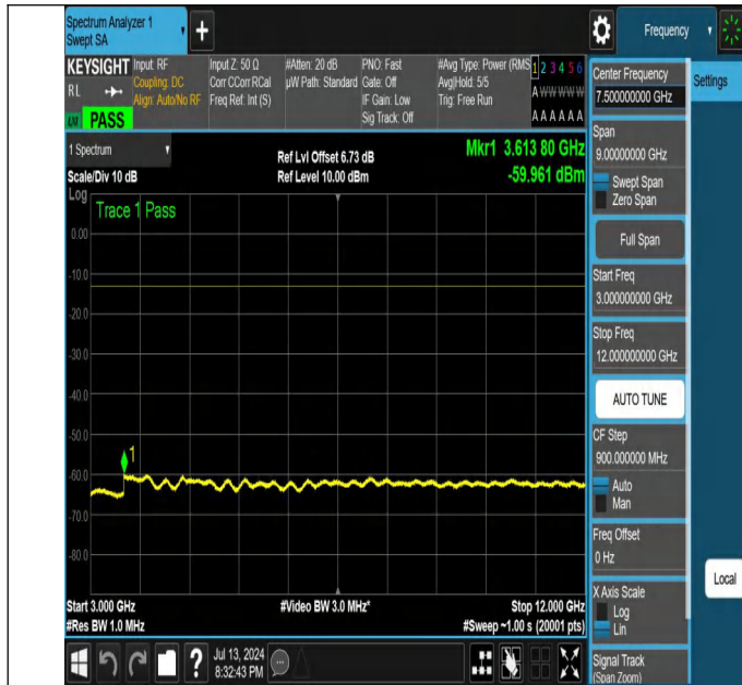
NTNV-N26-824-849-PC3-15-10-L-DFT-QPSK-Edge_1RB_Left-30 00-12000-Ant1-PASS
