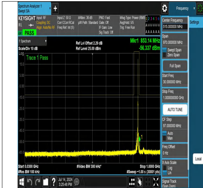
NTNV-N26-824-849-PC3-15-10-M-DFT-QPSK-Edge_1RB_Right-30-1000-Ant1-PASS
