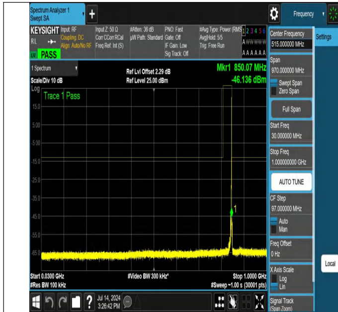
NTNV-N26-824-849-PC3-15-10-H-DFT-PI2BPSK-Edge_1RB_Rig ht-30-1000-Ant1-PASS
