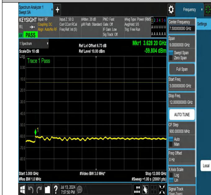
NTNV-N26-824-849-PC3-15-5-H-DFT-QPSK-Edge_1RB_Right-3 000-12000-Ant1-PASS
