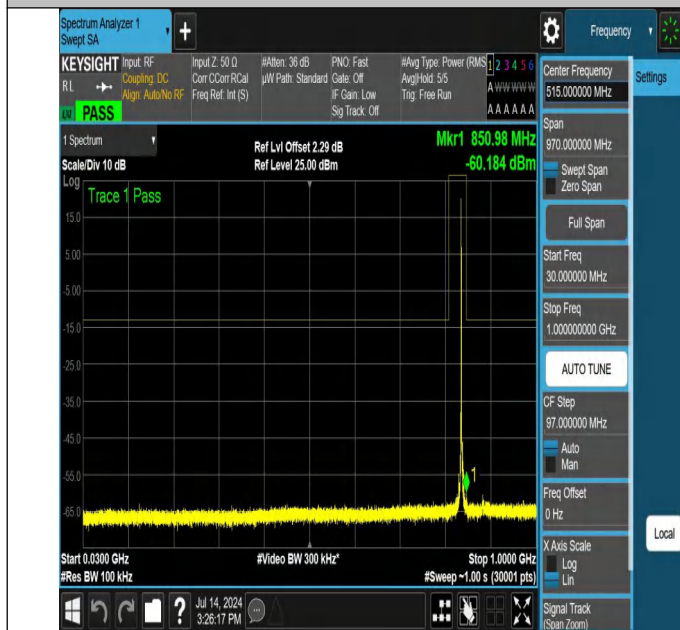
NTNV-N26-824-849-PC3-15-10-H-DFT-PI2BPSK-Edge_1RB_Lef t-30-1000-Ant1-PASS
