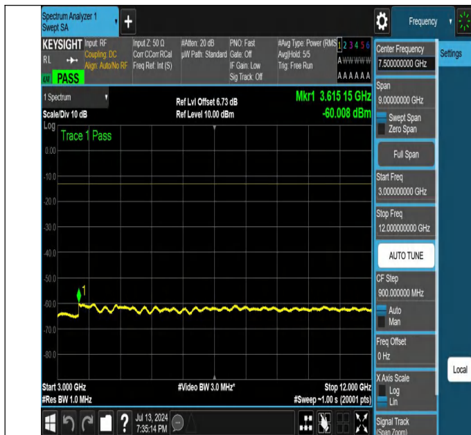
NTNV-N26-824-849-PC3-15-5-H-DFT-QPSK-Edge_1RB_Left-30 00-12000-Ant1-PASS
