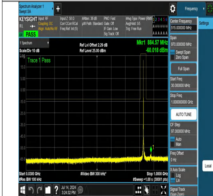
NTNV-N26-824-849-PC3-15-10-M-DFT-PI2BPSK-Edge_1RB_Left t-30-1000-Ant1-PASS
