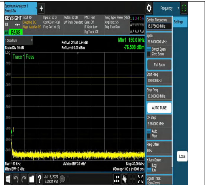
NTNV-N26-824-849-PC3-15-10-H-DFT-PI2BPSK-Edge_1RB_Left- 0.15-30-Ant1-PASS
