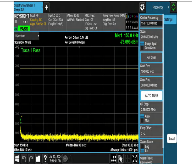
NTNV-N26-824-849-PC3-15-5-H-DFT-QPSK-Edge_1RB_Left-0.15 -30-Ant1-PASS
