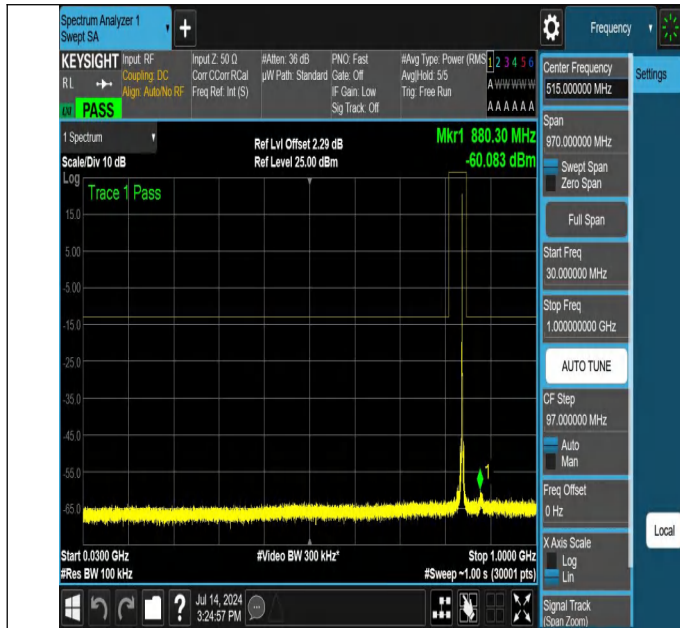
NTNV-N26-824-849-PC3-15-10-M-DFT-PI2BPSK-Edge_1RB_Rig ht-30-1000-Ant1-PASS
