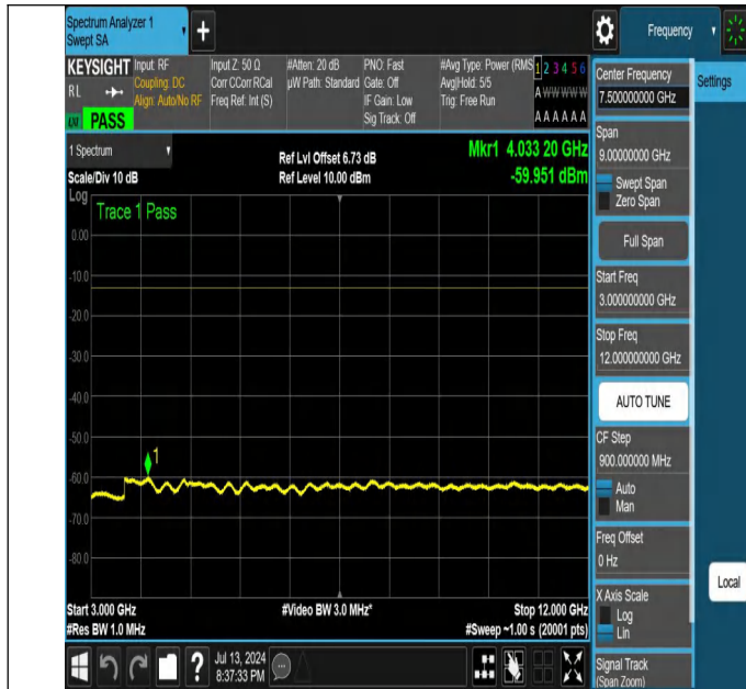
NTNV-N26-824-849-PC3-15-10-M-DFT-QPSK-Edge_1RB_Left-3 000-12000-Ant1-PASS
