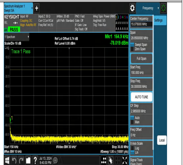
NTNV-N26-824-849-PC3-15-10-H-DFT-PI2BPSK-Edge_1RB_Rig ht-0.15-30-Ant1-PASS
