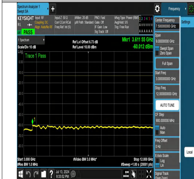
NTNV-N26-824-849-PC3-15-10-L-DFT-QPSK-Edge_1RB_Right-3000-12000-Ant1-PASS
