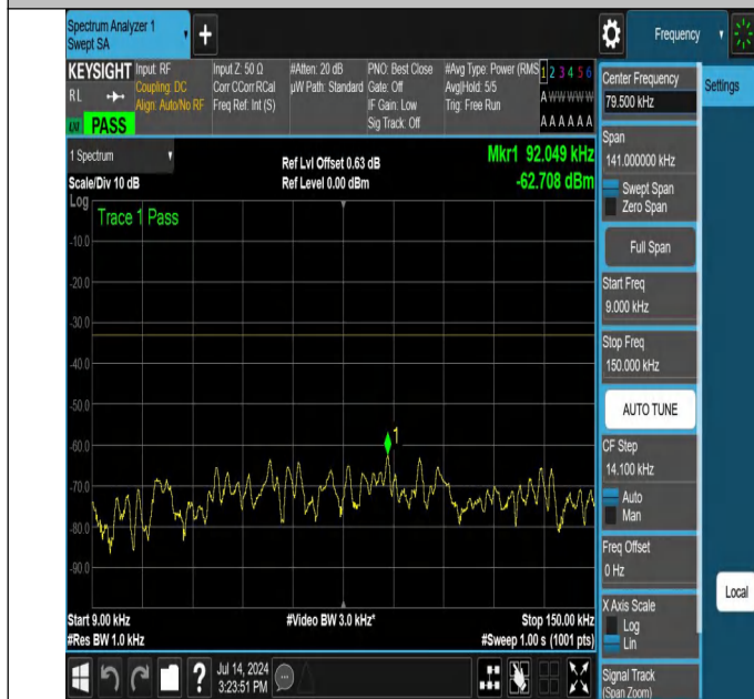
NTNV-N26-824-849-PC3-15-10-L-DFT-QPSK-Edge_1RB_Right- 0.009-0.15-Ant1-PASS
