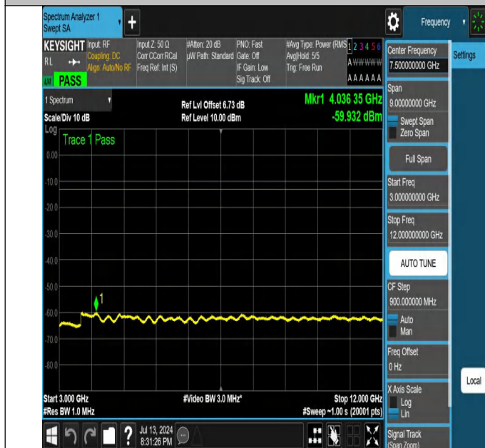
NTNV-N26-824-849-PC3-15-10-L-DFT-PI2BPSK-Edge_1RB_Rig ht-3000-12000-Ant1-PASS
