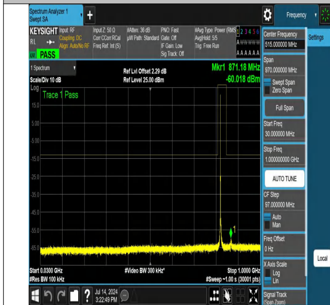
NTNV-N26-824-849-PC3-15-10-L-DFT-PI2BPSK-Edge_1RB_Left -30-1000-Ant1-PASS
