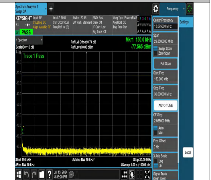
NTNV-N26-824-849-PC3-15-10-L-DFT-QPSK-Edge_1RB_Right-0. 15-30-Ant1-PASS
