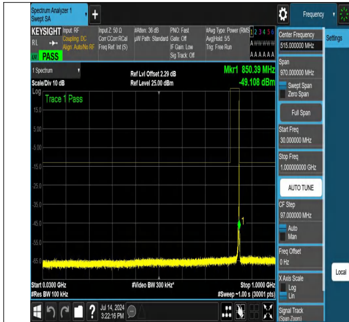
NTNV-N26-824-849-PC3-15-5-H-DFT-QPSK-Edge_1RB_Right-3 0-1000-Ant1-PASS
