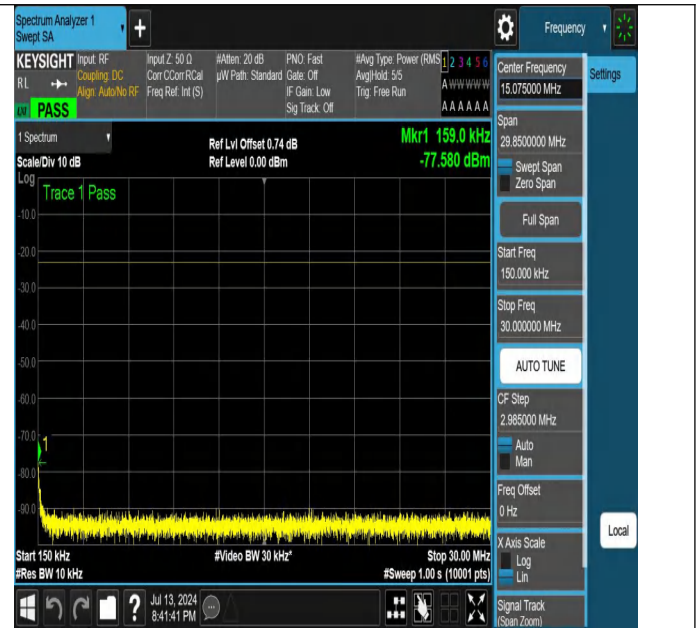
NTNV-N26-824-849-PC3-15-10-H-DFT-QPSK-Edge_1RB_Left-0.1
