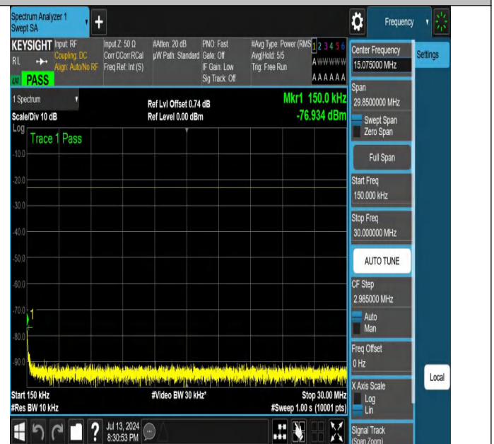
NTNV-N26-824-849-PC3-15-10-L-DFT-PI2BPSK-Edge_1RB_Righ t-0.15-30-Ant1-PASS
