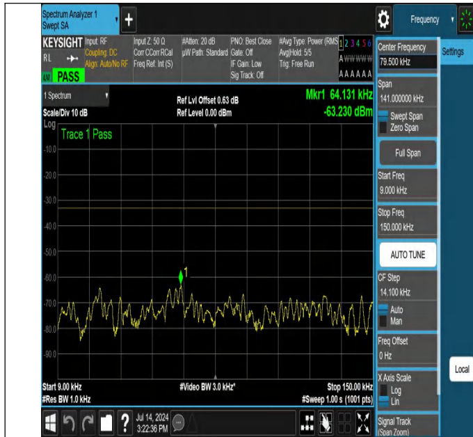
NTNV-N26-824-849-PC3-15-10-L-DFT-PI2BPSK-Edge_1RB_Left -0.009-0.15-Ant1-PASS
