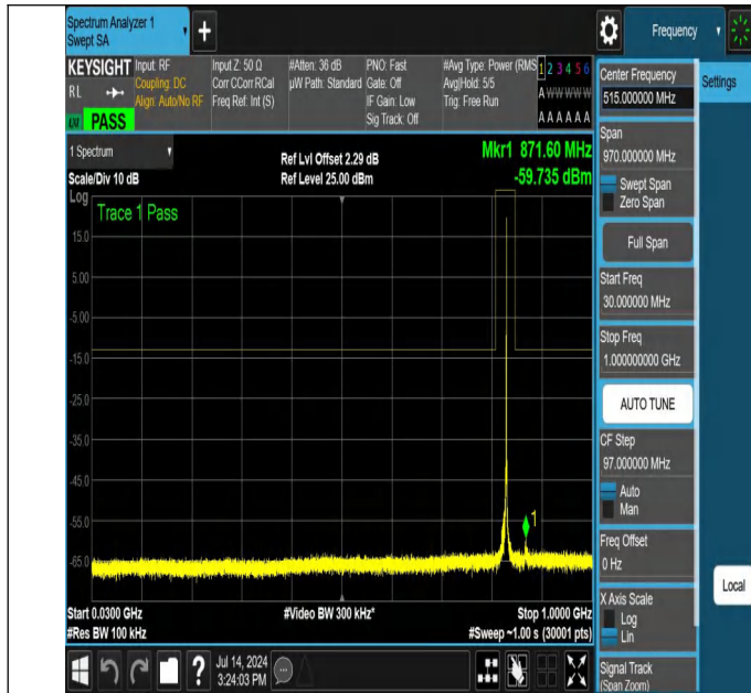
NTNV-N26-824-849-PC3-15-10-L-DFT-QPSK-Edge_1RB_Right-30-1000-Ant1-PASS
