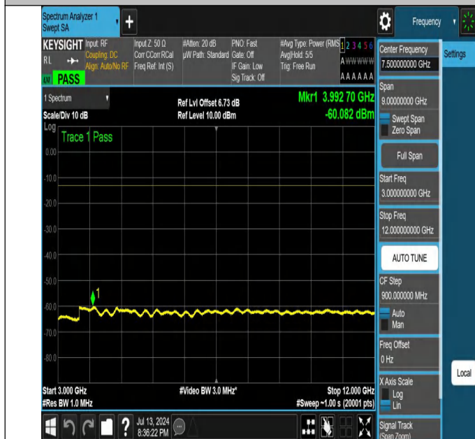
NTNV-N26-824-849-PC3-15-10-M-DFT-PI2BPSK-Edge_1RB_Rig ht-3000-12000-Ant1-PASS
