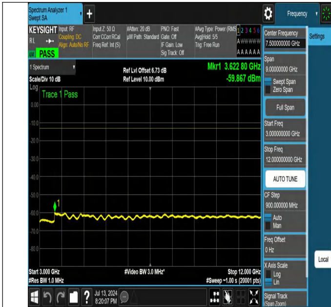
NTNV-N26-824-849-PC3-15-10-L-DFT-PI2BPSK-Edge_1RB_Left -3000-12000-Ant1-PASS
