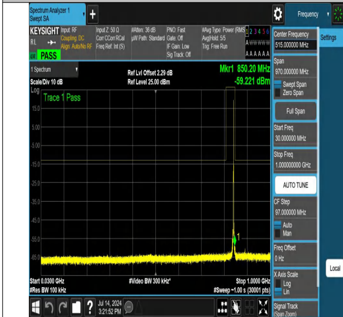
NTNV-N26-824-849-PC3-15-5-H-DFT-QPSK-Edge_1RB_Left-30- 1000-Ant1-PASS
