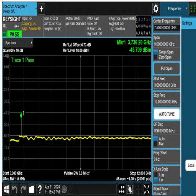
NTNV-N25-PC3-15-30-M-DFT-PI2BPSK-Edge_1RB_Left-3000-1 2000-Ant1-PASS
