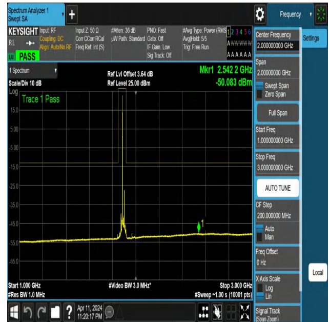
NTNV-N25-PC3-15-30-H-DFT-PI2BPSK-Edge_1RB_Left-1000-3000-Ant1-PASS
