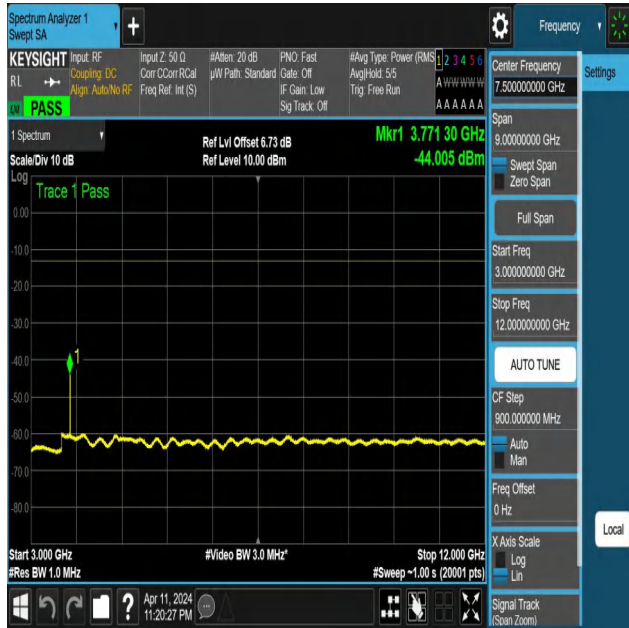
NTNV-N25-PC3-15-30-H-DFT-PI2BPSK-Edge_1RB_Left-3000-1 2000-Ant1-PASS
