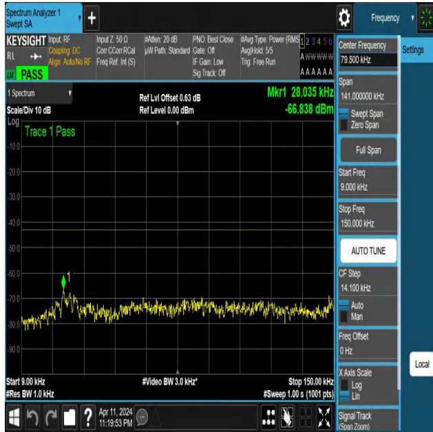
NTNV-N25-PC3-15-30-H-DFT-PI2BPSK-Edge_1RB_Left-0.009-0.15-Ant1-PASS
