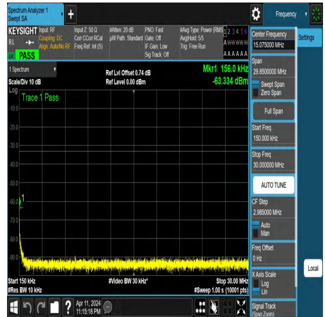
NTNV-N25-PC3-15-30-L-DFT-QPSK-Edge_1RB_Right-0.15-30-A nt1-PASS
