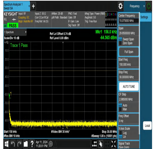
NTNV-N25-PC3-15-30-H-DFT-PI2BPSK-Edge_1RB_Left-0.15-30-Ant1-PASS
