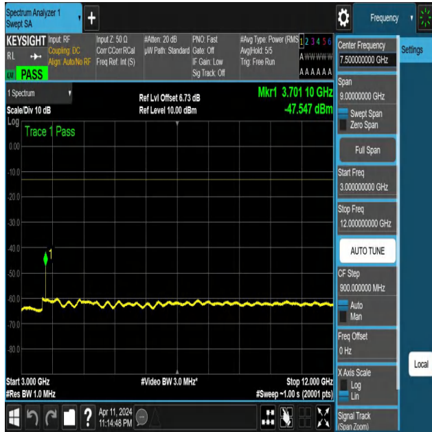
NTNV-N25-PC3-15-30-L-DFT-QPSK-Edge_1RB_Left-3000-1200 0-Ant1-PASS
