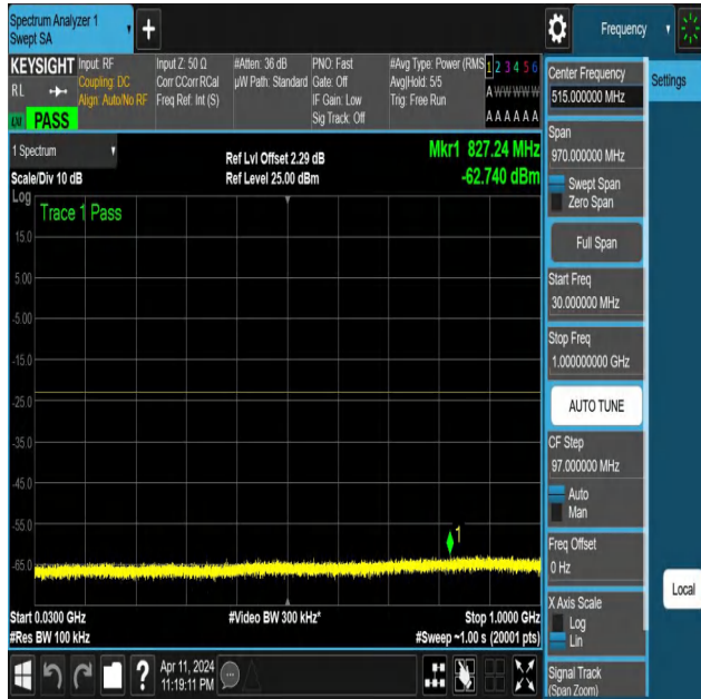
NTNV-N25-PC3-15-30-M-DFT-QPSK-Edge_1RB_Right-30-1000- Ant1-PASS
