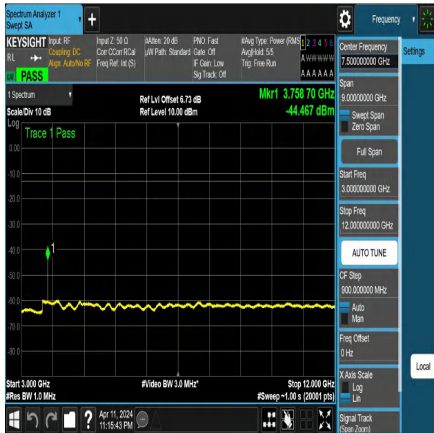
NTNV-N25-PC3-15-30-L-DFT-QPSK-Edge_1RB_Right-3000-12000-Ant1-PASS
