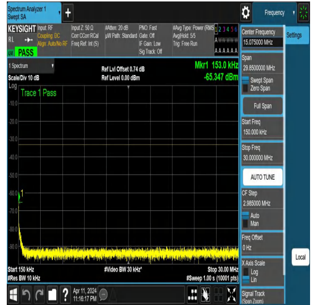
NTNV-N25-PC3-15-30-M-DFT-PI2BPSK-Edge_1RB_Left-0.15-30- Ant1-PASS
