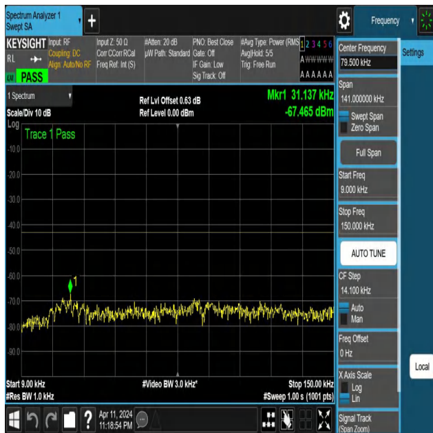
NTNV-N25-PC3-15-30-M-DFT-QPSK-Edge_1RB_Right-0.009-0. 15-Ant1-PASS
