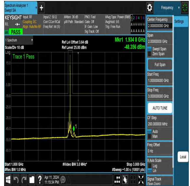
NTNV-N25-PC3-15-30-L-DFT-QPSK-Edge_1RB_Right-1000-3000-Ant1-PASS
