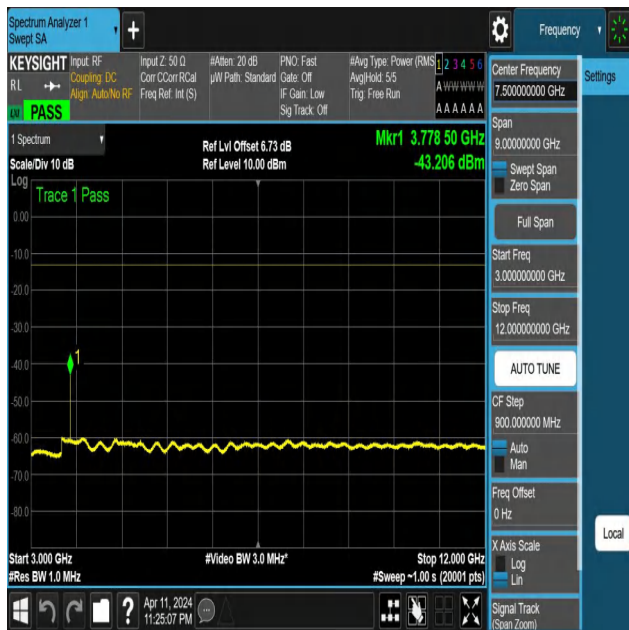
NTNV-N25-PC3-15-40-L-DFT-PI2BPSK-Edge_1RB_Right-3000- 12000-Ant1-PASS
