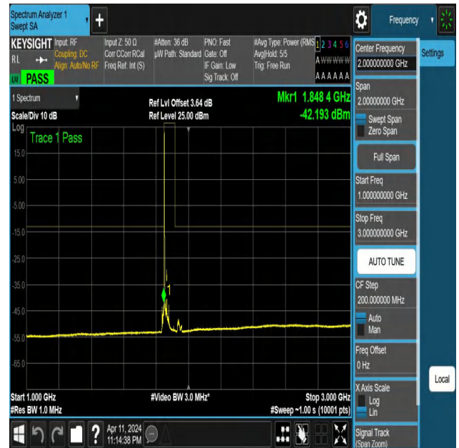
NTNV-N25-PC3-15-30-L-DFT-QPSK-Edge_1RB_Left-1000-3000-Ant1-PASS
