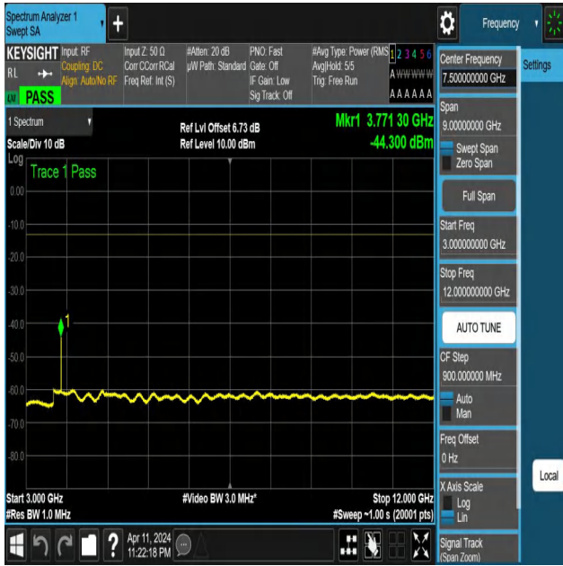
NTNV-N25-PC3-15-30-H-DFT-QPSK-Edge_1RB_Left-3000-1200 0-Ant1-PASS
