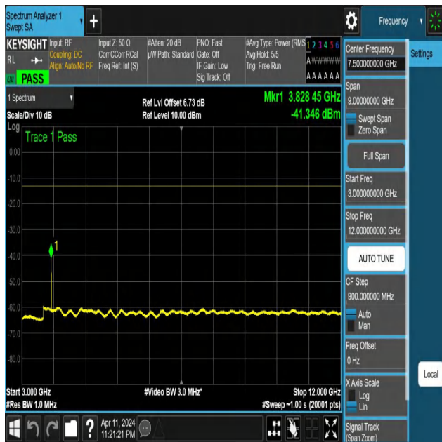
NTNV-N25-PC3-15-30-H-DFT-PI2BPSK-Edge_1RB_Right-3000- 12000-Ant1-PASS
