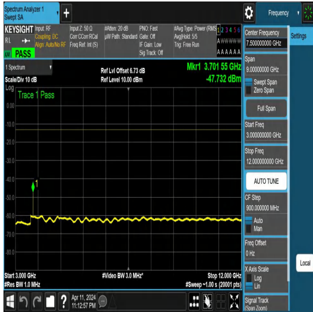
NTNV-N25-PC3-15-30-L-DFT-PI2BPSK-Edge_1RB_Left-3000-12000-Ant1-PASS
