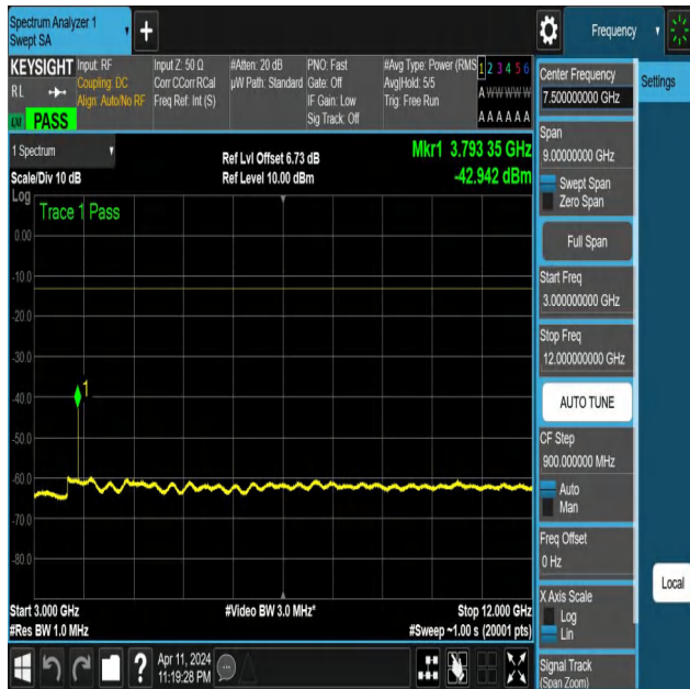
NTNV-N25-PC3-15-30-M-DFT-QPSK-Edge_1RB_Right-3000-12 000-Ant1-PASS
