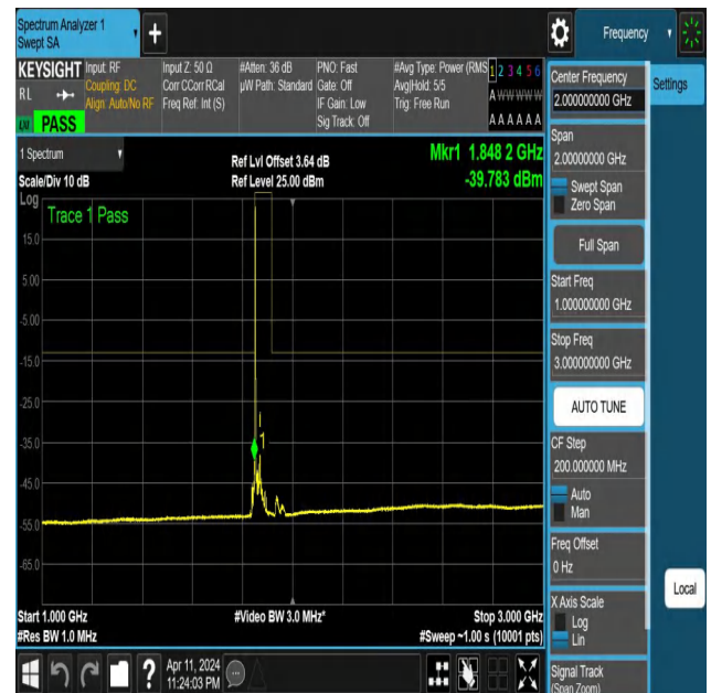
NTNV-N25-PC3-15-40-L-DFT-PI2BPSK-Edge_1RB_Left-1000-3000-Ant1-PASS
