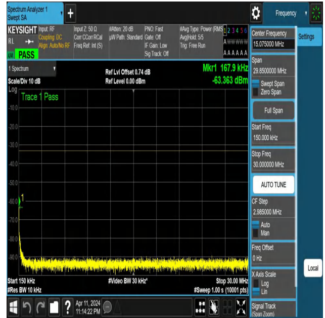
NTNV-N25-PC3-15-30-L-DFT-QPSK-Edge_1RB_Left-0.15-30-Ant 1-PASS
