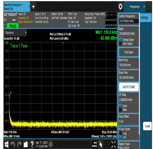
NTNV-N25-PC3-15-30-L-DFT-PI2BPSK-Edge_1RB_Right-0.15-30-Ant1-PASS
