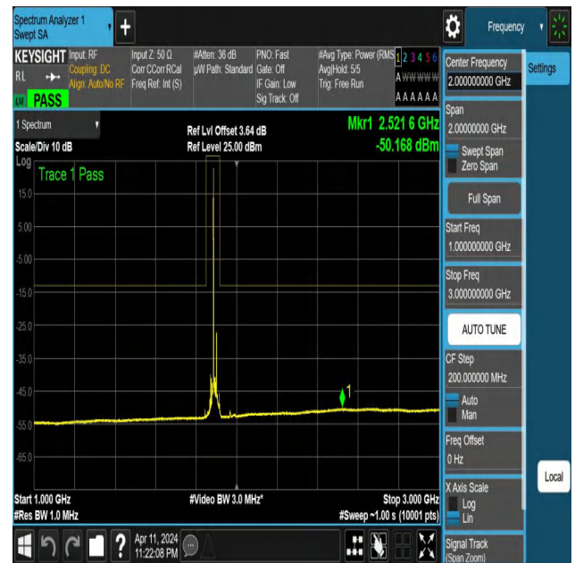
NTNV-N25-PC3-15-30-H-DFT-QPSK-Edge_1RB_Left-1000-3000- Ant1-PASS
