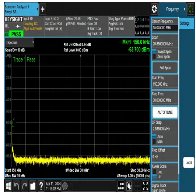
NTNV-N25-PC3-15-30-M-DFT-QPSK-Edge_1RB_Right-0.15-30-A nt1-PASS
