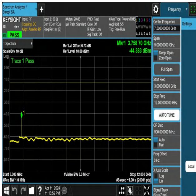
NTNV-N25-PC3-15-30-L-DFT-PI2BPSK-Edge_1RB_Right-3000-12000-Ant1-PASS
