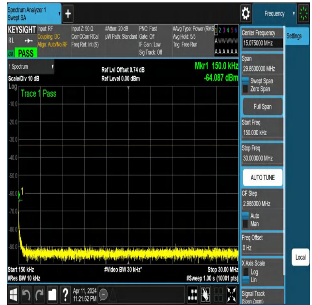
NTNV-N25-PC3-15-30-H-DFT-QPSK-Edge_1RB_Left-0.15-30-Ant 1-PASS
