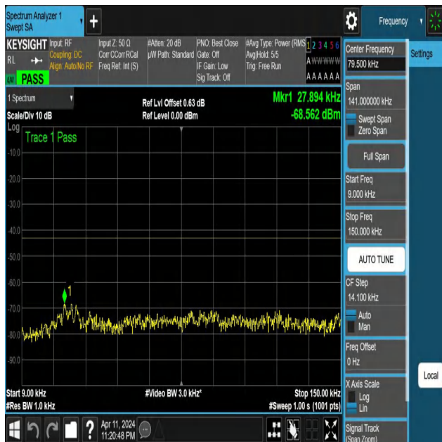
NTNV-N25-PC3-15-30-H-DFT-PI2BPSK-Edge_1RB_Right-0.009- 0.15-Ant1-PASS
