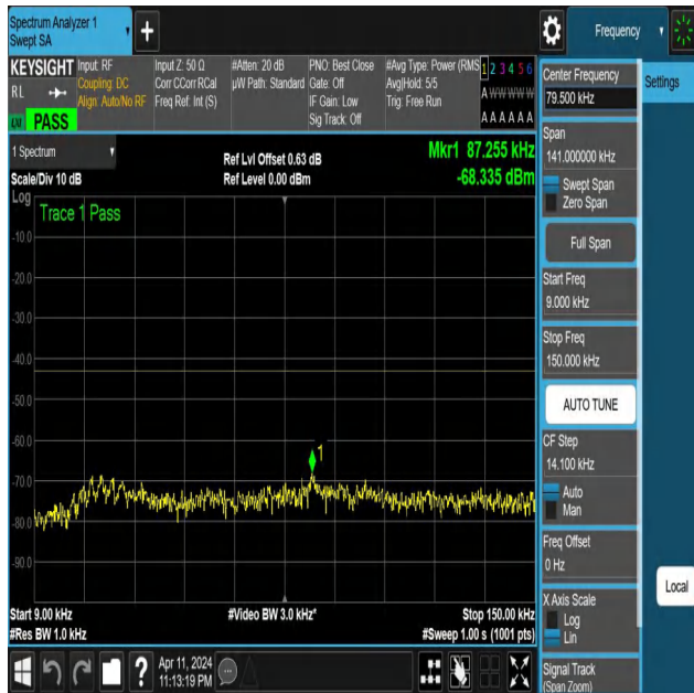
NTNV-N25-PC3-15-30-L-DFT-PI2BPSK-Edge_1RB_Right-0.009-0.15-Ant1-PASS
