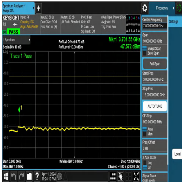
NTNV-N25-PC3-15-40-L-DFT-PI2BPSK-Edge_1RB_Left-3000-12 000-Ant1-PASS
