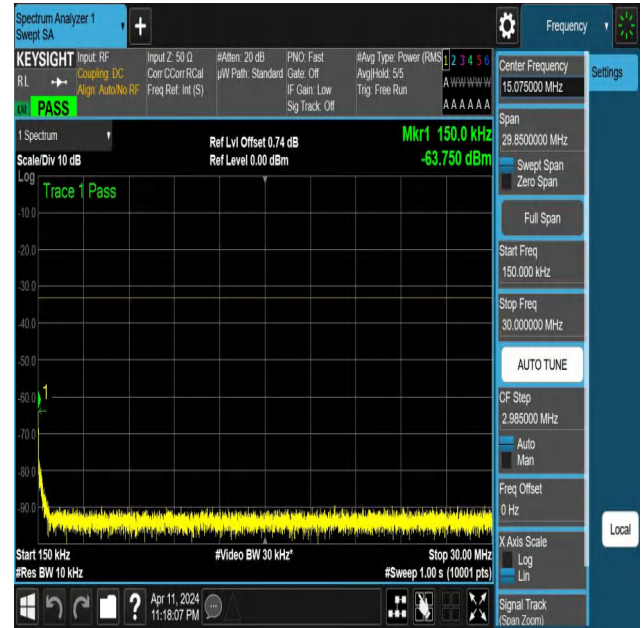
NTNV-N25-PC3-15-30-M-DFT-QPSK-Edge_1RB_Left-0.15-30-Ant 1-PASS
