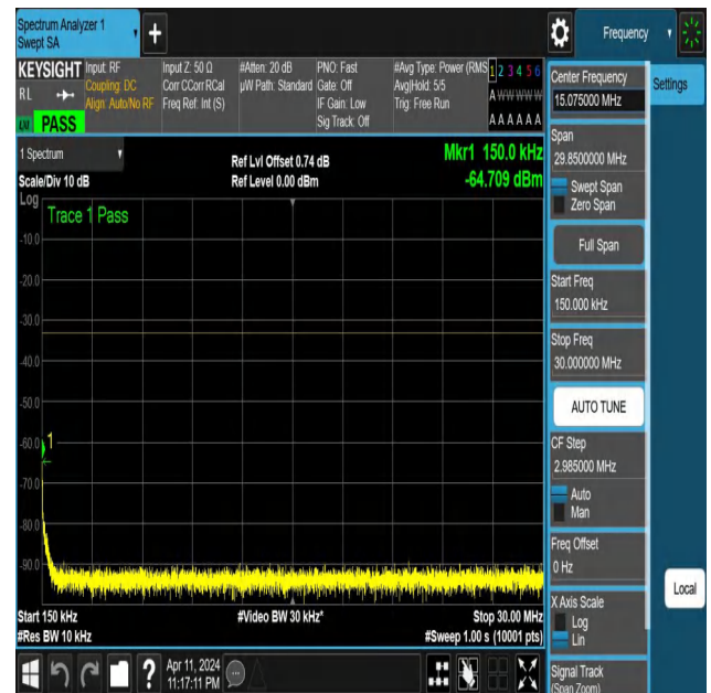
NTNV-N25-PC3-15-30-M-DFT-PI2BPSK-Edge_1RB_Right-0.15-3 0-Ant1-PASS
