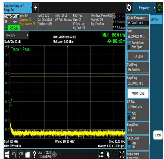
NTNV-N25-PC3-15-30-H-DFT-PI2BPSK-Edge_1RB_Right-0.15-3 0-Ant1-PASS
