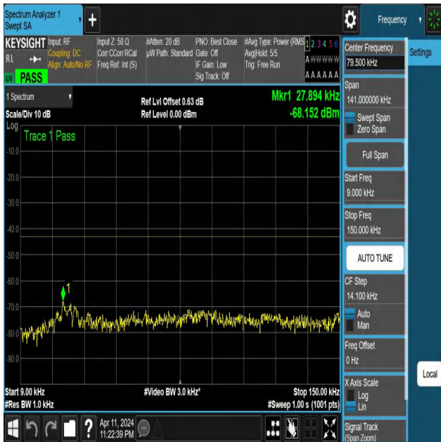
NTNV-N25-PC3-15-30-H-DFT-QPSK-Edge_1RB_Right-0.009-0.1 5-Ant1-PASS
