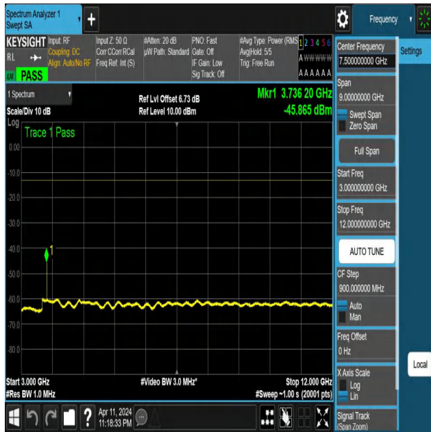
NTNV-N25-PC3-15-30-M-DFT-QPSK-Edge_1RB_Left-3000-1200 0-Ant1-PASS
