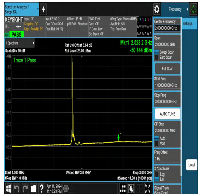
NTNV-N25-PC3-15-30-M-DFT-QPSK-Edge_1RB_Left-1000-3000- Ant1-PASS
