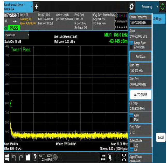
NTNV-N25-PC3-15-40-L-DFT-PI2BPSK-Edge_1RB_Left-0.15-30-Ant1-PASS
