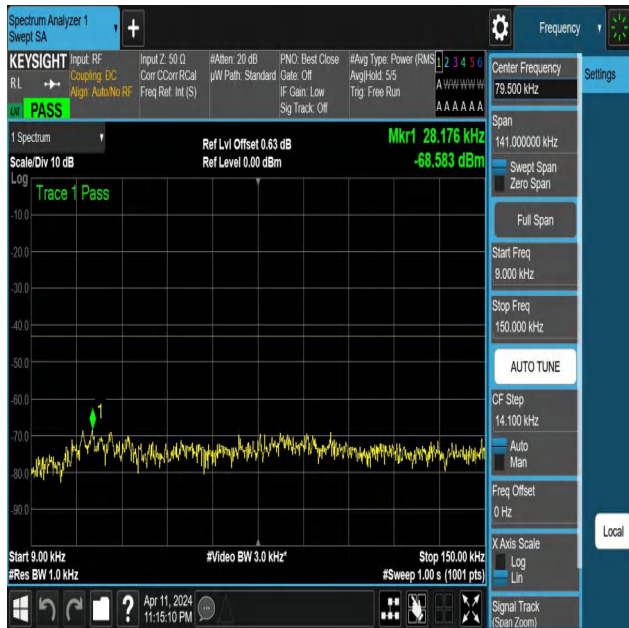
NTNV-N25-PC3-15-30-L-DFT-QPSK-Edge_1RB_Right-0.009-0.1 5-Ant1-PASS
