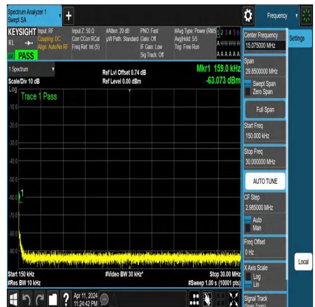
NTNV-N25-PC3-15-40-L-DFT-PI2BPSK-Edge_1RB_Right-0.15-30 -Ant1-PASS
