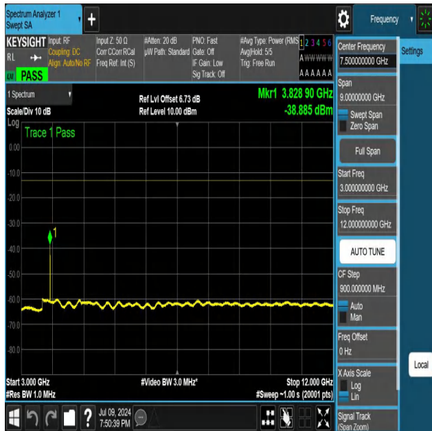
NTNV-N25-PC3-15-25-H-DFT-PI2BPSK-Edge_1RB_Right-3000- 12000-Ant1-PASS
