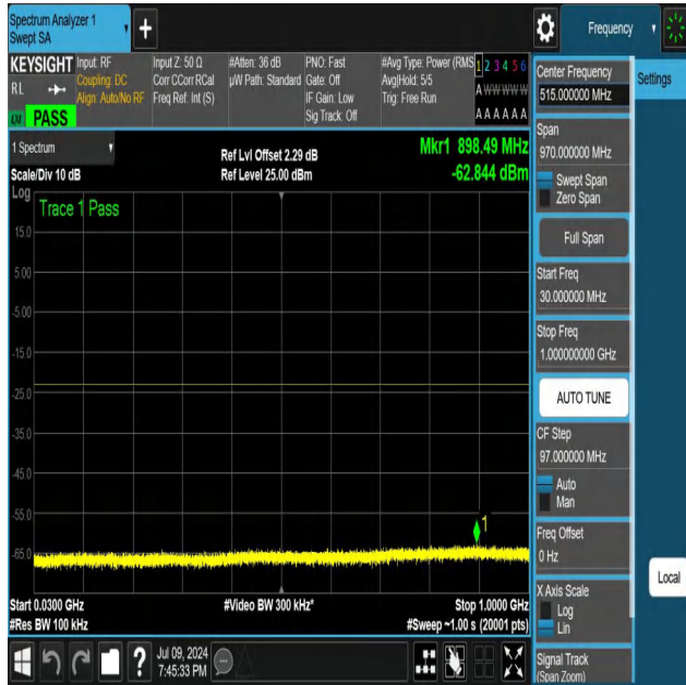
NTNV-N25-PC3-15-25-M-DFT-PI2BPSK-Edge_1RB_Right-30-10 00-Ant1-PASS
