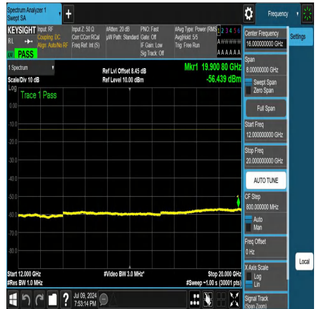
NTNV-N25-PC3-15-25-H-DFT-QPSK-Edge_1RB_Right-12000-20 000-Ant1-PASS
