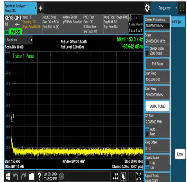
NTNV-N25-PC3-15-25-M-DFT-PI2BPSK-Edge_1RB_Right-0.15-3 0-Ant1-PASS
