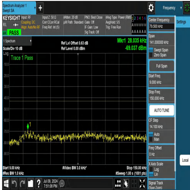
NTNV-N25-PC3-15-25-H-DFT-QPSK-Edge_1RB_Left-0.009-0.15 -Ant1-PASS
