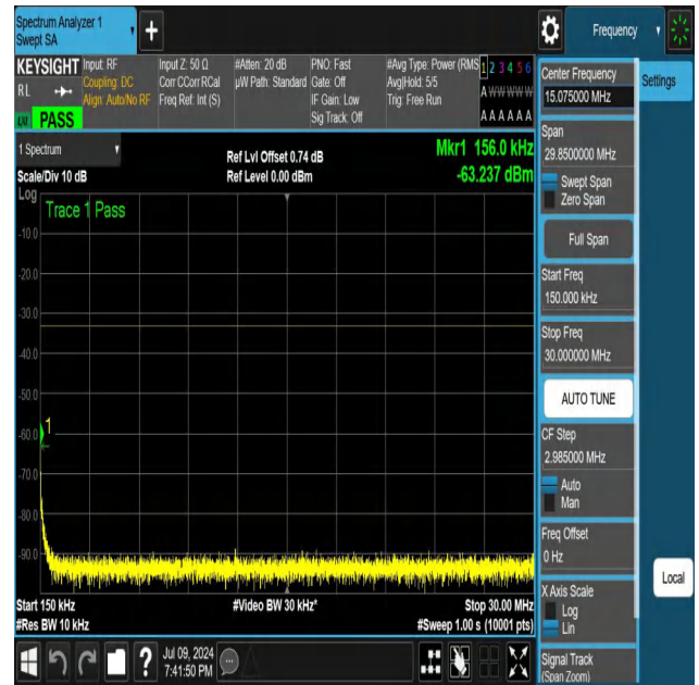
NTNV-N25-PC3-15-25-L-DFT-QPSK-Edge_1RB_Left-0.15-30-Ant 1-PASS
