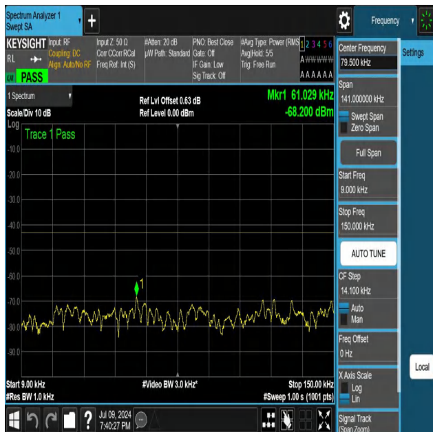
NTNV-N25-PC3-15-25-L-DFT-PI2BPSK-Edge_1RB_Right-0.009-0.15-Ant1-PASS
