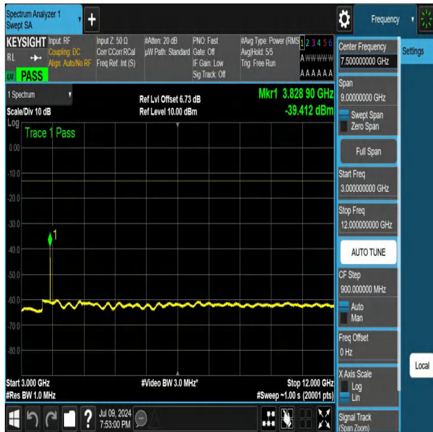
NTNV-N25-PC3-15-25-H-DFT-QPSK-Edge_1RB_Right-3000-120 00-Ant1-PASS
