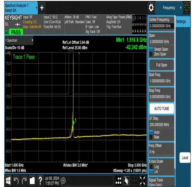
NTNV-N25-PC3-15-25-H-DFT-PI2BPSK-Edge_1RB_Right-1000-3 000-Ant1-PASS
