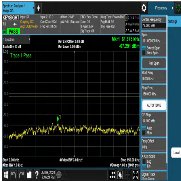
NTNV-N25-PC3-15-25-M-DFT-QPSK-Edge_1RB_Left-0.009-0.15 -Ant1-PASS
