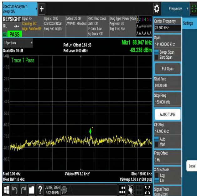
NTNV-N25-PC3-15-25-L-DFT-QPSK-Edge_1RB_Right-0.009-0.1 5-Ant1-PASS
