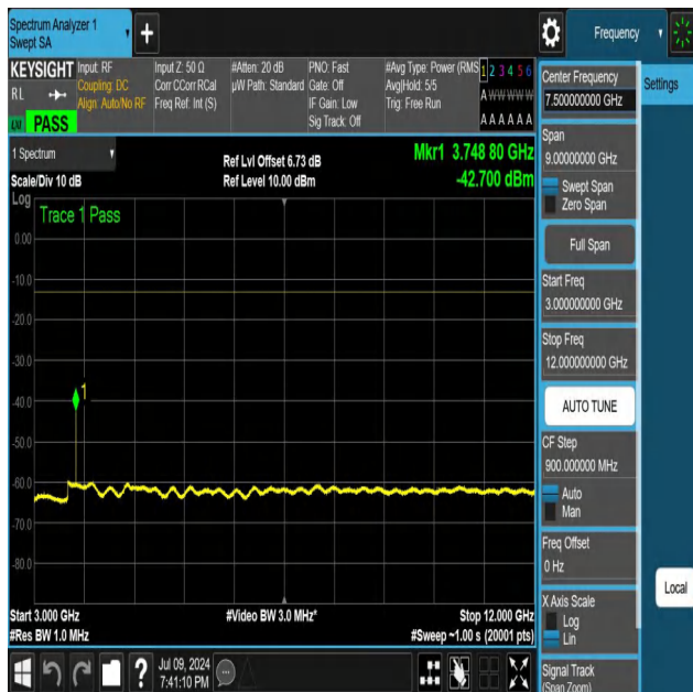
NTNV-N25-PC3-15-25-L-DFT-PI2BPSK-Edge_1RB_Right-3000-12000-Ant1-PASS
