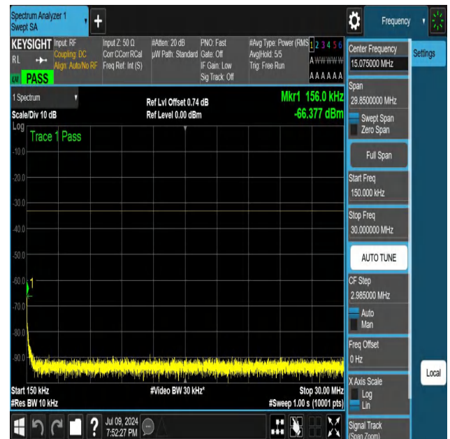
NTNV-N25-PC3-15-25-H-DFT-QPSK-Edge_1RB_Right-0.15-30-A nt1-PASS
