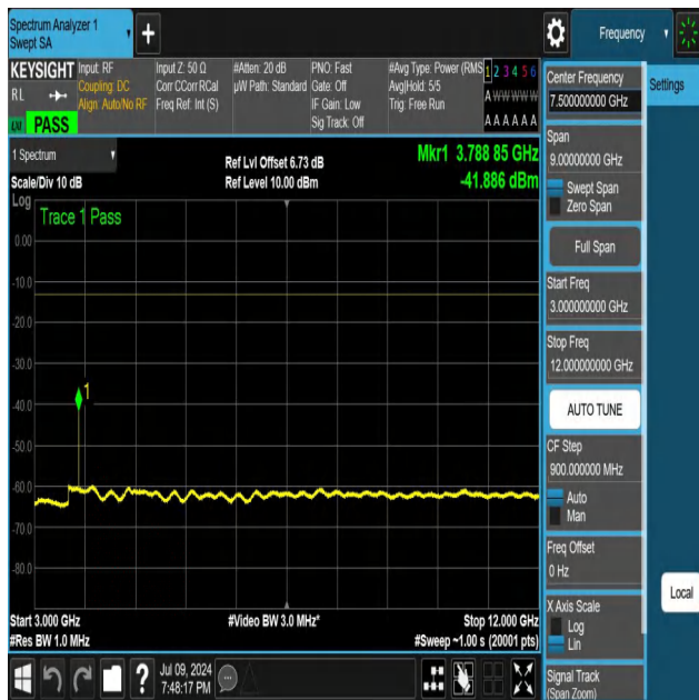
NTNV-N25-PC3-15-25-M-DFT-QPSK-Edge_1RB_Right-3000-12 000-Ant1-PASS
