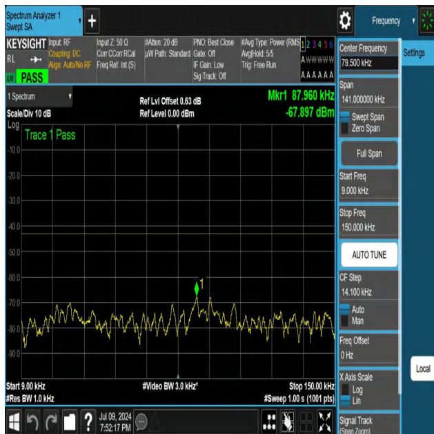
NTNV-N25-PC3-15-25-H-DFT-QPSK-Edge_1RB_Right-0.009-0.1 5-Ant1-PASS
