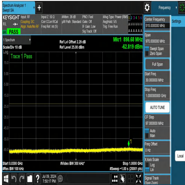
NTNV-N25-PC3-15-25-H-DFT-PI2BPSK-Edge_1RB_Right-30-10 00-Ant1-PASS
