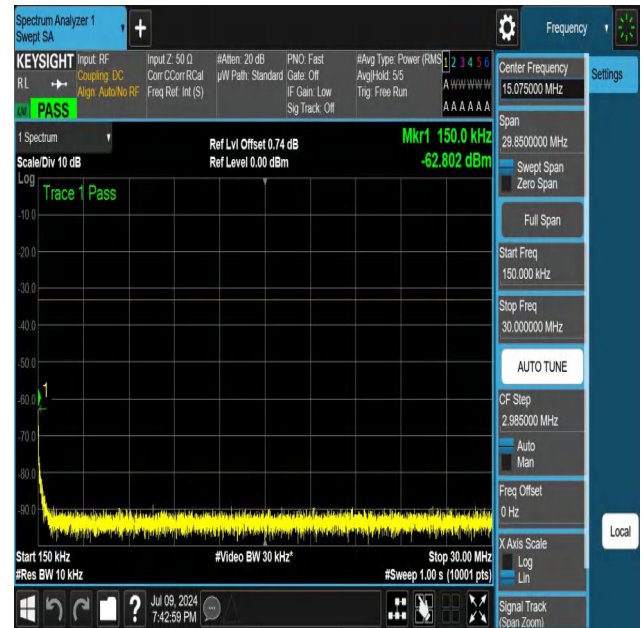
NTNV-N25-PC3-15-25-L-DFT-QPSK-Edge_1RB_Right-0.15-30-A nt1-PASS
