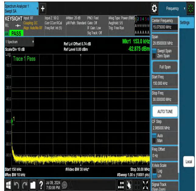
NTNV-N25-PC3-15-25-H-DFT-PI2BPSK-Edge_1RB_Right-0.15-3 0-Ant1-PASS
