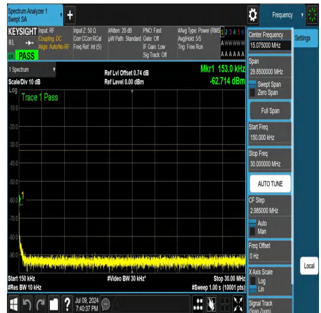
NTNV-N25-PC3-15-25-L-DFT-PI2BPSK-Edge_1RB_Right-0.15-30-Ant1-PASS
