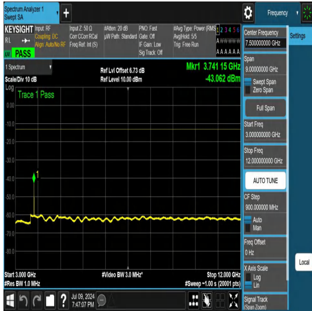
NTNV-N25-PC3-15-25-M-DFT-QPSK-Edge_1RB_Left-3000-1200 0-Ant1-PASS
