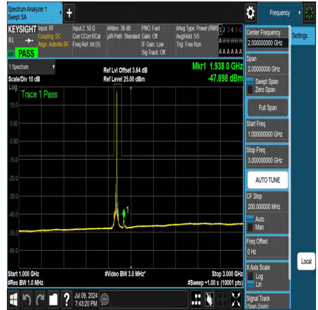
NTNV-N25-PC3-15-25-L-DFT-QPSK-Edge_1RB_Right-1000-3000-Ant1-PASS
