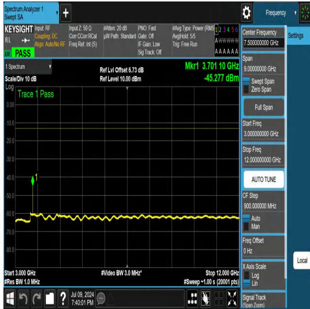
NTNV-N25-PC3-15-25-L-DFT-PI2BPSK-Edge_1RB_Left-3000-12000-Ant1-PASS
