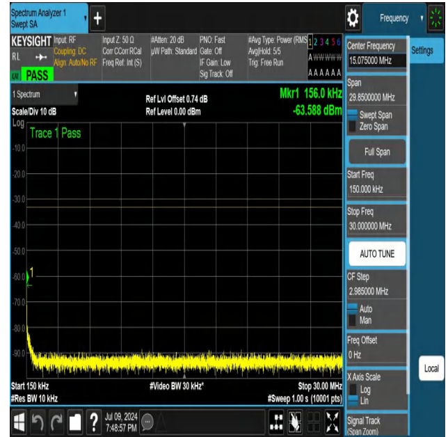
NTNV-N25-PC3-15-25-H-DFT-PI2BPSK-Edge_1RB_Left-0.15-30-Ant1-PASS
