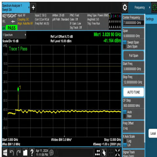
NTNV-N25-PC3-15-20-H-DFT-QPSK-Edge_1RB_Right-3000-120 00-Ant1-PASS
