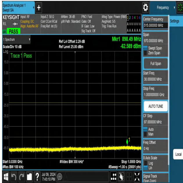
NTNV-N25-PC3-15-25-L-DFT-QPSK-Edge_1RB_Right-30-1000-Ant1-PASS
