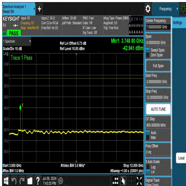
NTNV-N25-PC3-15-25-L-DFT-QPSK-Edge_1RB_Right-3000-12000-Ant1-PASS
