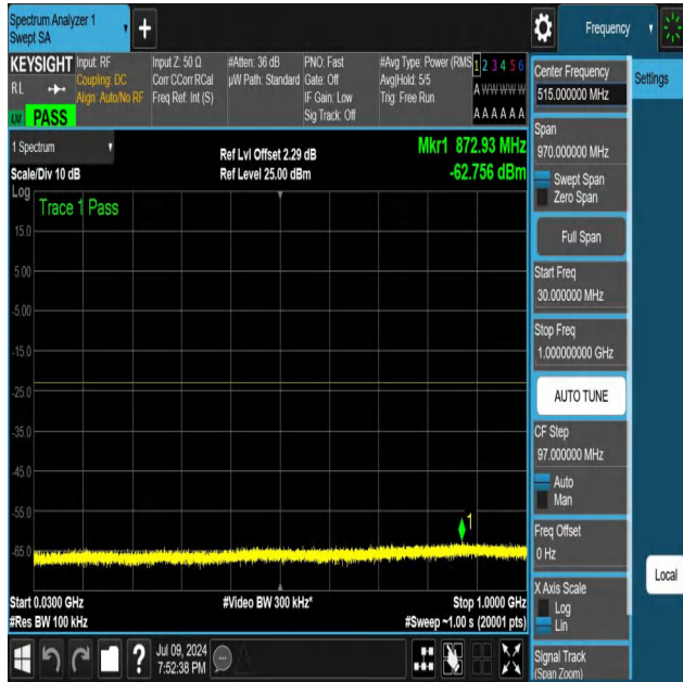
NTNV-N25-PC3-15-25-H-DFT-QPSK-Edge_1RB_Right-30-1000- Ant1-PASS
