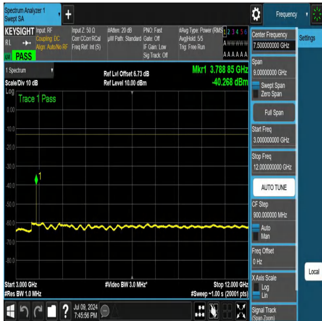
NTNV-N25-PC3-15-25-M-DFT-PI2BPSK-Edge_1RB_Right-3000- 12000-Ant1-PASS
