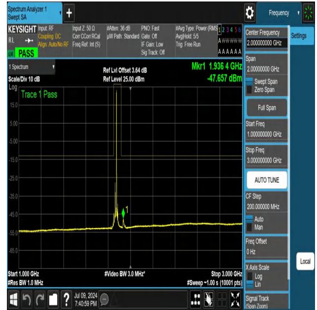
NTNV-N25-PC3-15-25-L-DFT-PI2BPSK-Edge_1RB_Right-1000-3000-Ant1-PASS
