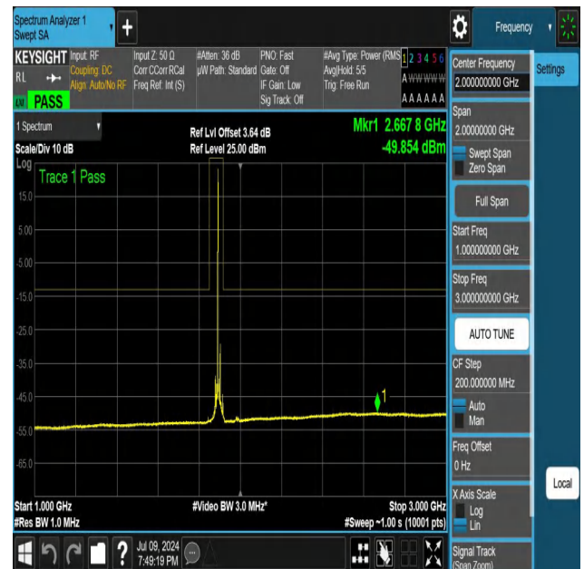
NTNV-N25-PC3-15-25-H-DFT-PI2BPSK-Edge_1RB_Left-1000-3000-Ant1-PASS
