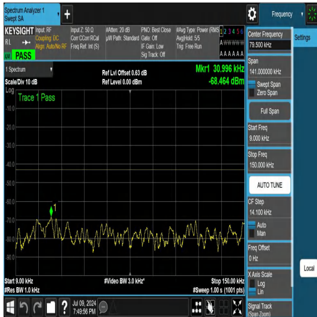
NTNV-N25-PC3-15-25-H-DFT-PI2BPSK-Edge_1RB_Right-0.009- 0.15-Ant1-PASS
