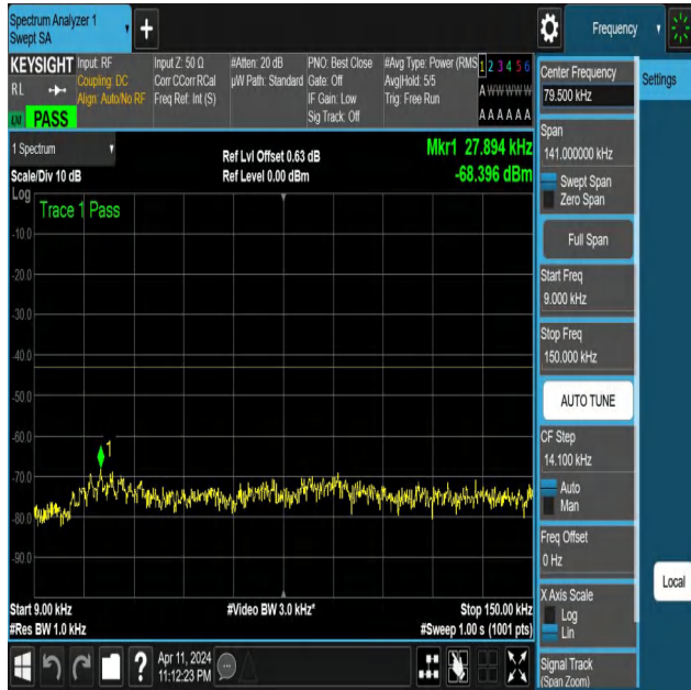
NTNV-N25-PC3-15-30-L-DFT-PI2BPSK-Edge_1RB_Left-0.009-0. 15-Ant1-PASS
