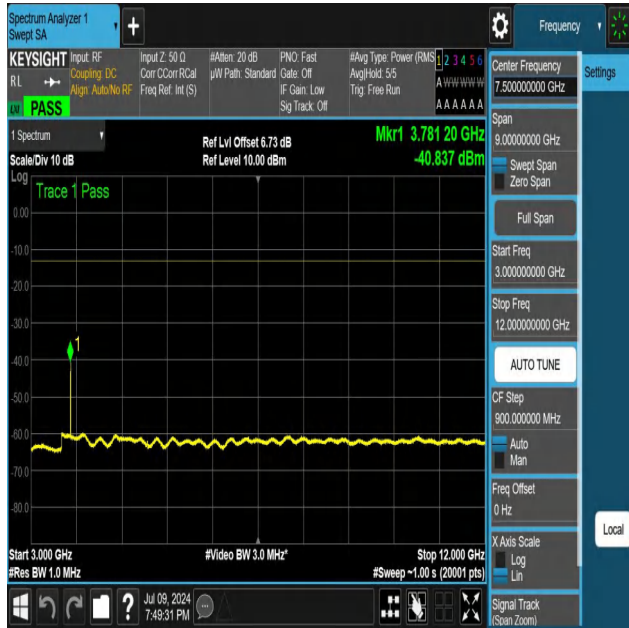
NTNV-N25-PC3-15-25-H-DFT-PI2BPSK-Edge_1RB_Left-3000-1 2000-Ant1-PASS
