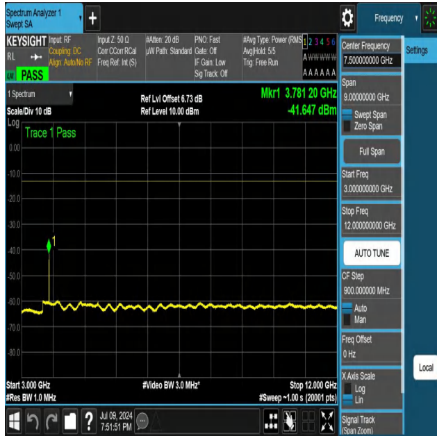
NTNV-N25-PC3-15-25-H-DFT-QPSK-Edge_1RB_Left-3000-1200 0-Ant1-PASS
