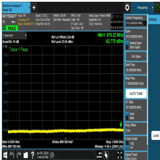
NTNV-N25-PC3-15-25-M-DFT-QPSK-Edge_1RB_Left-30-1000-A nt1-PASS
