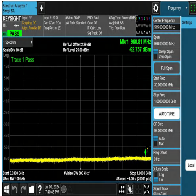
NTNV-N25-PC3-15-25-L-DFT-PI2BPSK-Edge_1RB_Right-30-1000-Ant1-PASS
