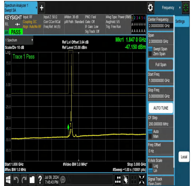
NTNV-N25-PC3-15-25-M-DFT-PI2BPSK-Edge_1RB_Right-1000-3 000-Ant1-PASS
