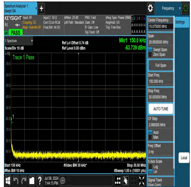
NTNV-N25-PC3-15-25-M-DFT-PI2BPSK-Edge_1RB_Left-0.15-30-Ant1-PASS
