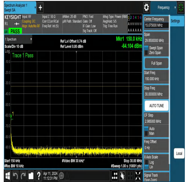
NTNV-N25-PC3-15-30-L-DFT-PI2BPSK-Edge_1RB_Left-0.15-30- Ant1-PASS
