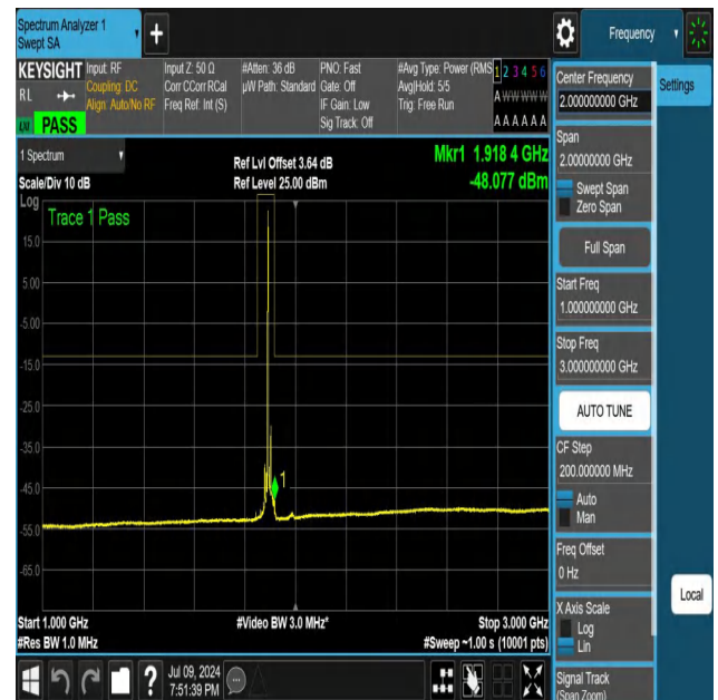
NTNV-N25-PC3-15-25-H-DFT-QPSK-Edge_1RB_Left-1000-3000- Ant1-PASS
