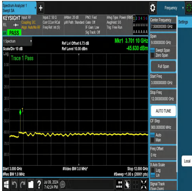
NTNV-N25-PC3-15-25-L-DFT-QPSK-Edge_1RB_Left-3000-1200 0-Ant1-PASS
