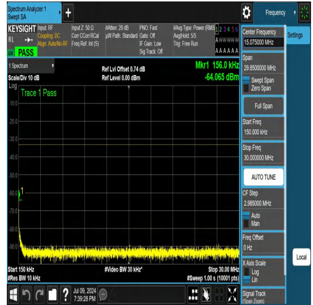
NTNV-N25-PC3-15-25-L-DFT-PI2BPSK-Edge_1RB_Left-0.15-30- Ant1-PASS
