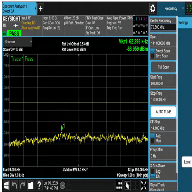
NTNV-N25-PC3-15-25-L-DFT-QPSK-Edge_1RB_Left-0.009-0.15-Ant1-PASS
