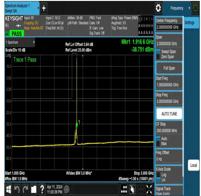
NTNV-N25-PC3-15-15-H-DFT-QPSK-Edge_1RB_Right-1000-300 0-Ant1-PASS
