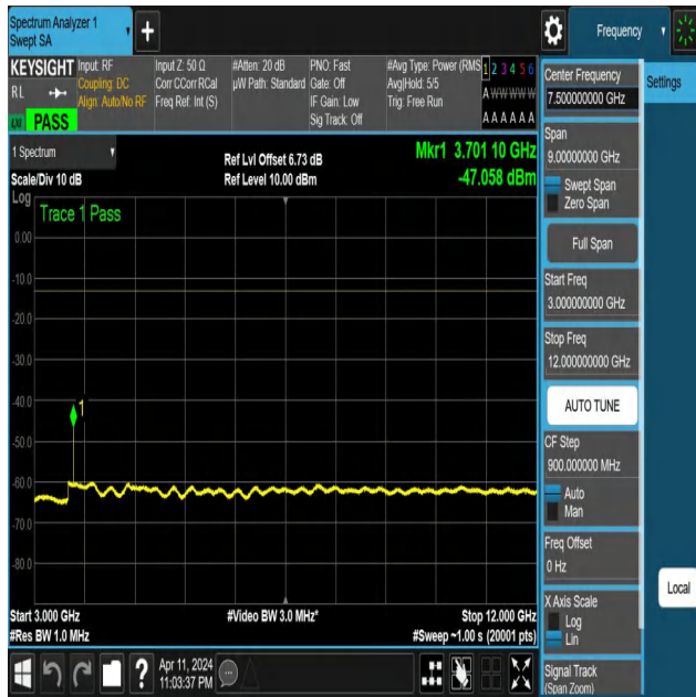
NTNV-N25-PC3-15-20-L-DFT-QPSK-Edge_1RB_Left-3000-1200 0-Ant1-PASS
