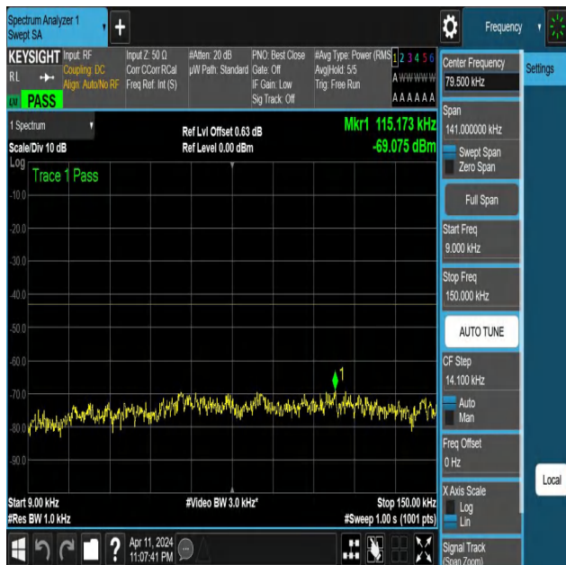
NTNV-N25-PC3-15-20-M-DFT-QPSK-Edge_1RB_Right-0.009-0. 15-Ant1-PASS
