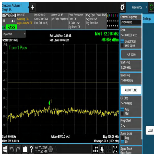
NTNV-N25-PC3-15-20-H-DFT-QPSK-Edge_1RB_Right-0.009-0.1 5-Ant1-PASS
