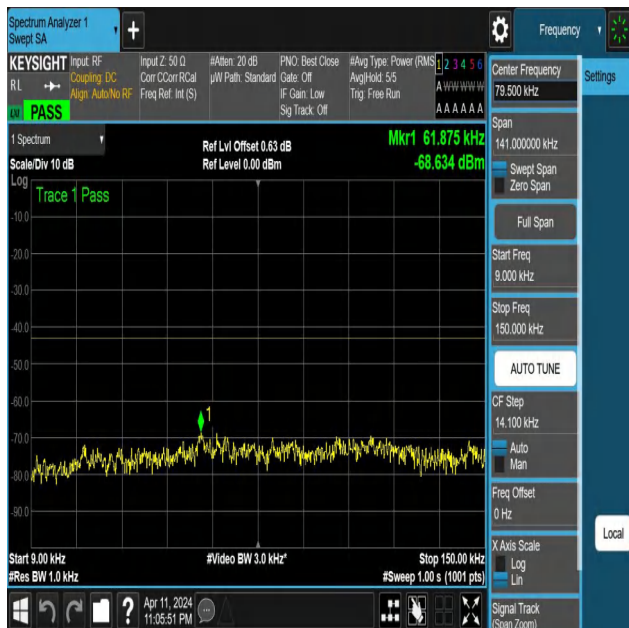
NTNV-N25-PC3-15-20-M-DFT-PI2BPSK-Edge_1RB_Right-0.009 -0.15-Ant1-PASS
