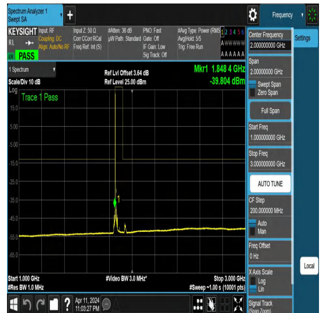
NTNV-N25-PC3-15-20-L-DFT-QPSK-Edge_1RB_Left-1000-3000-Ant1-PASS
