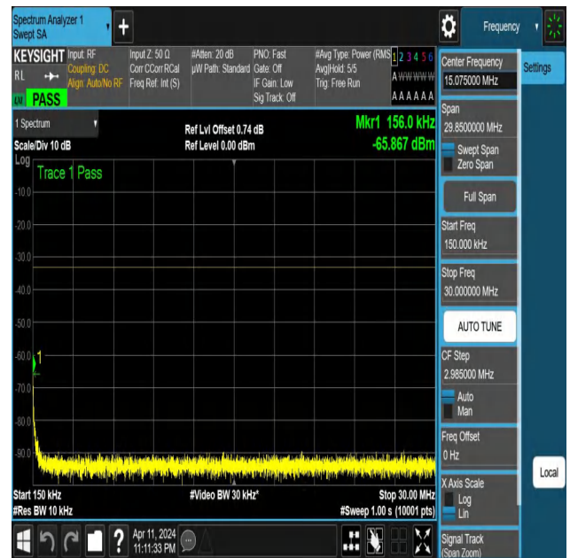
NTNV-N25-PC3-15-20-H-DFT-QPSK-Edge_1RB_Right-0.15-30-A nt1-PASS
