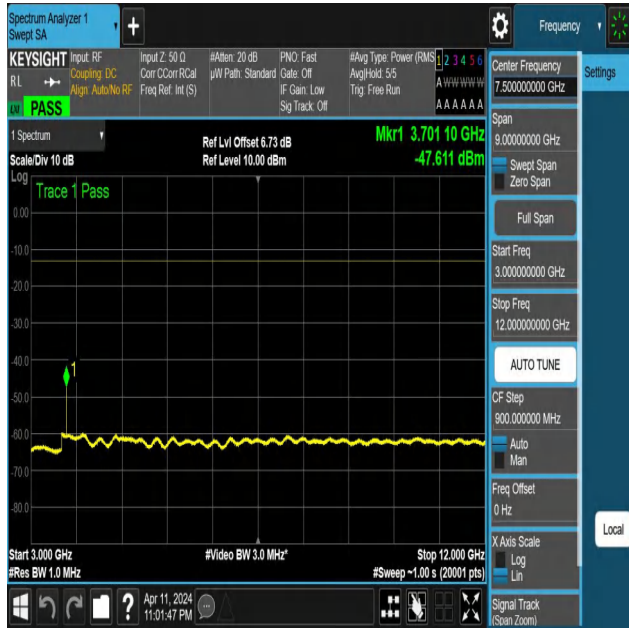
NTNV-N25-PC3-15-20-L-DFT-PI2BPSK-Edge_1RB_Left-3000-12000-Ant1-PASS
