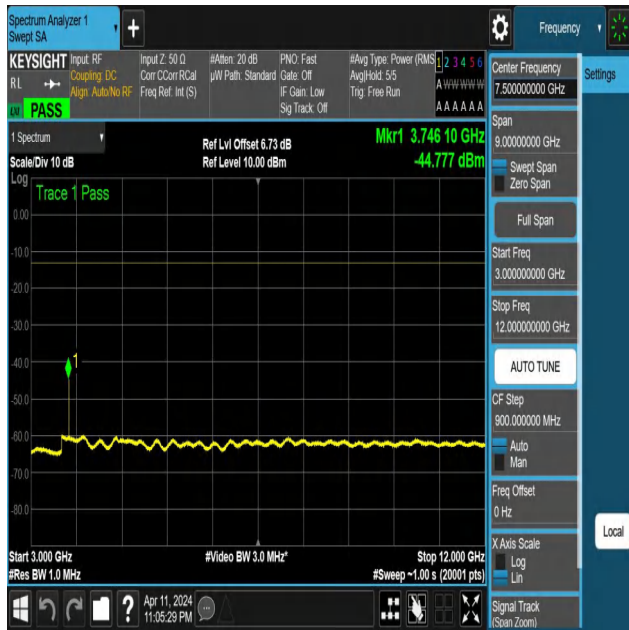
NTNV-N25-PC3-15-20-M-DFT-PI2BPSK-Edge_1RB_Left-3000-1 2000-Ant1-PASS
