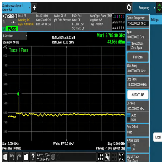
NTNV-N25-PC3-15-20-M-DFT-PI2BPSK-Edge_1RB_Right-3000- 12000-Ant1-PASS
