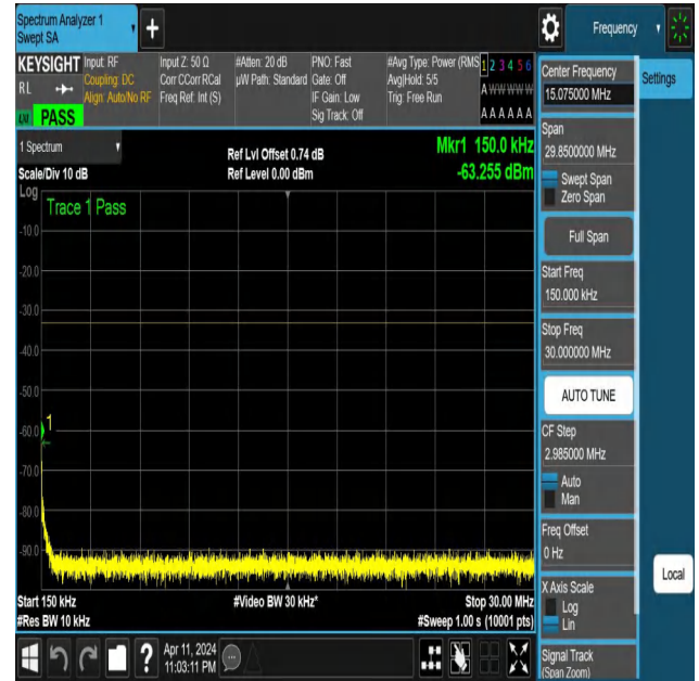
NTNV-N25-PC3-15-20-L-DFT-QPSK-Edge_1RB_Left-0.15-30-Ant 1-PASS
