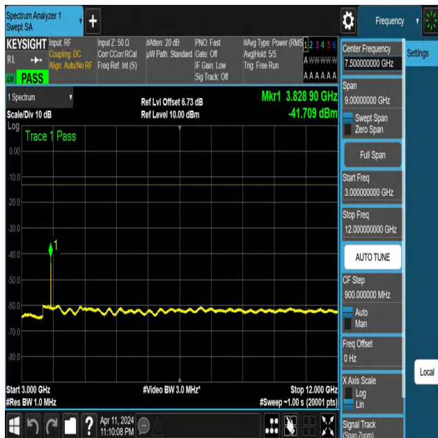
NTNV-N25-PC3-15-20-H-DFT-PI2BPSK-Edge_1RB_Right-3000-12000-Ant1-PASS
