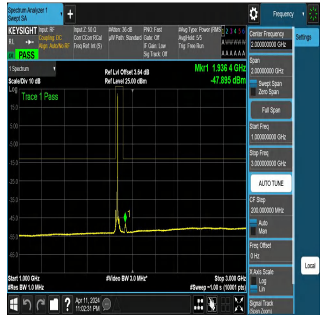
NTNV-N25-PC3-15-20-L-DFT-PI2BPSK-Edge_1RB_Right-1000-3 000-Ant1-PASS
