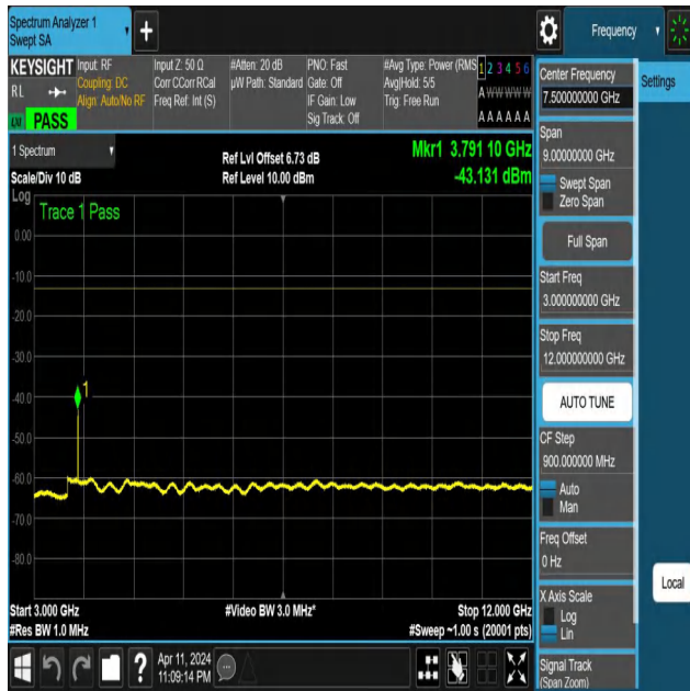
NTNV-N25-PC3-15-20-H-DFT-PI2BPSK-Edge_1RB_Left-3000-1 2000-Ant1-PASS
