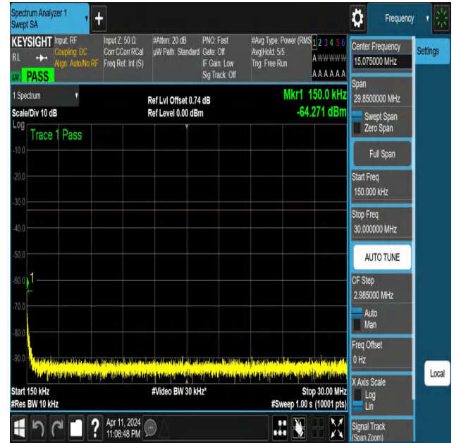
NTNV-N25-PC3-15-20-H-DFT-PI2BPSK-Edge_1RB_Left-0.15-30-Ant1-PASS
