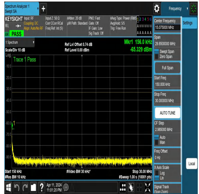
NTNV-N25-PC3-15-20-L-DFT-PI2BPSK-Edge_1RB_Left-0.15-30-Ant1-PASS
