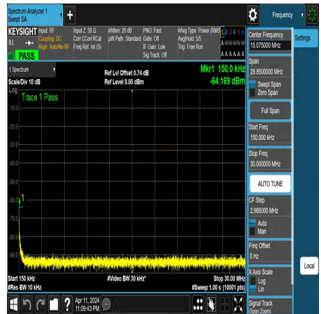
NTNV-N25-PC3-15-20-H-DFT-PI2BPSK-Edge_1RB_Right-0.15-3 0-Ant1-PASS
