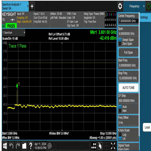
NTNV-N25-PC3-15-15-H-DFT-QPSK-Edge_1RB_Left-3000-1200 0-Ant1-PASS
