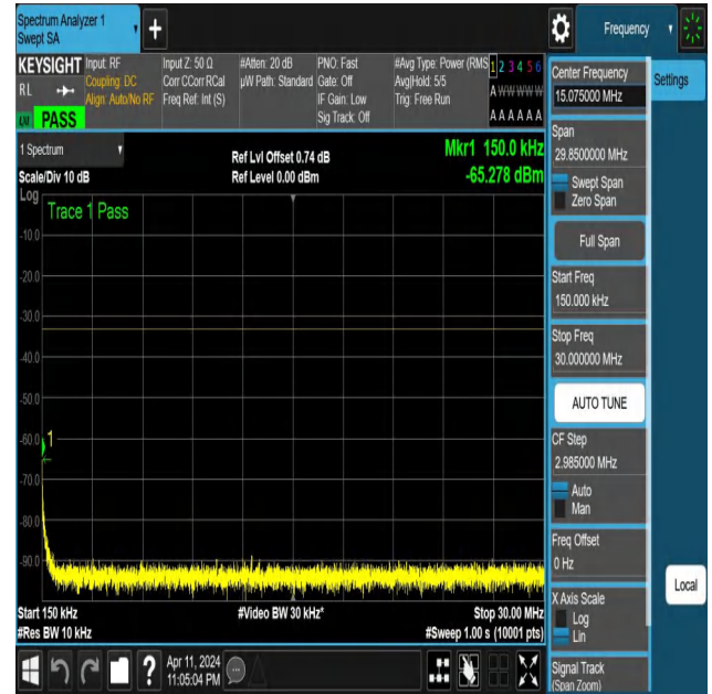
NTNV-N25-PC3-15-20-M-DFT-PI2BPSK-Edge_1RB_Left-0.15-30-Ant1-PASS
