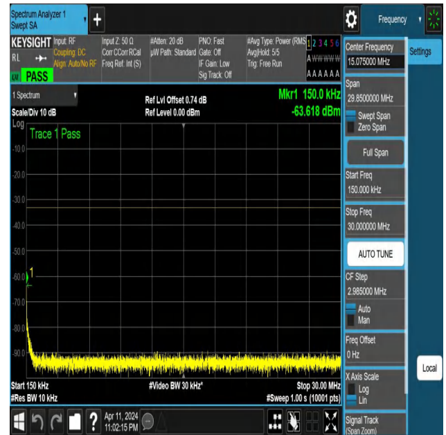
NTNV-N25-PC3-15-20-L-DFT-PI2BPSK-Edge_1RB_Right-0.15-30-Ant1-PASS
