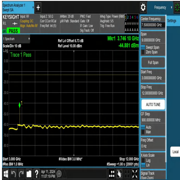
NTNV-N25-PC3-15-20-M-DFT-QPSK-Edge_1RB_Left-3000-1200 0-Ant1-PASS
