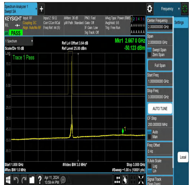
NTNV-N25-PC3-15-15-H-DFT-QPSK-Edge_1RB_Left-1000-3000- Ant1-PASS
