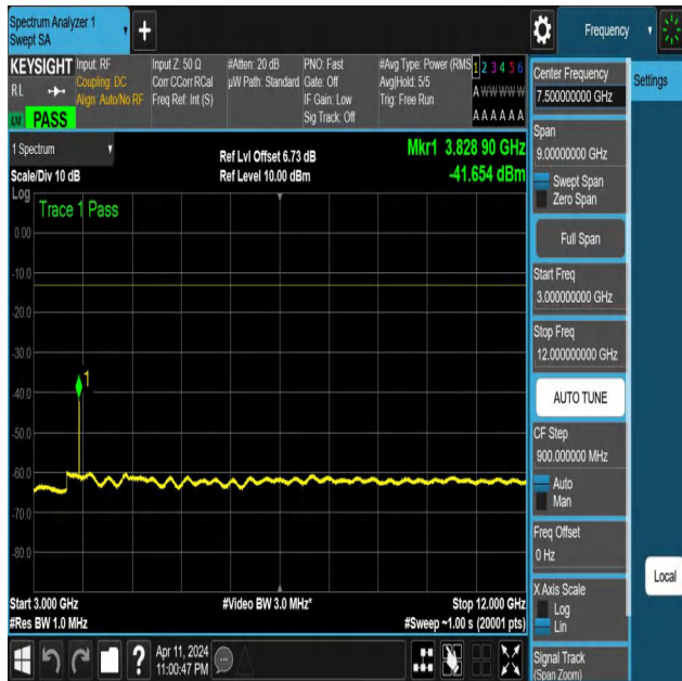
NTNV-N25-PC3-15-15-H-DFT-QPSK-Edge_1RB_Right-3000-120 00-Ant1-PASS
