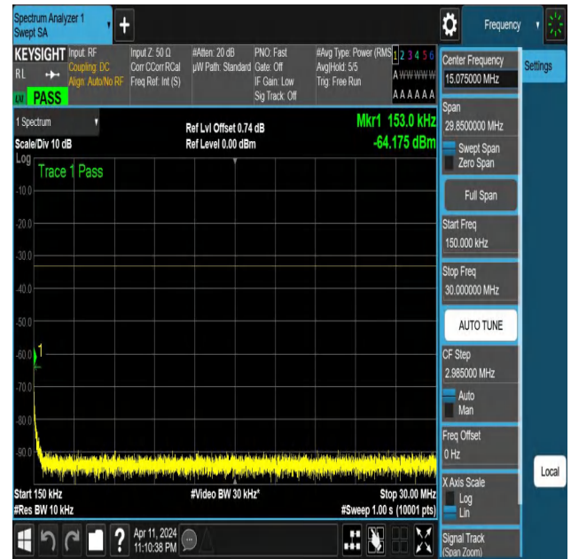
NTNV-N25-PC3-15-20-H-DFT-QPSK-Edge_1RB_Left-0.15-30-Ant 1-PASS
