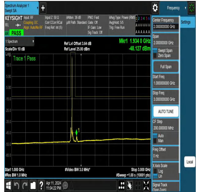
NTNV-N25-PC3-15-20-L-DFT-QPSK-Edge_1RB_Right-1000-3000-Ant1-PASS
