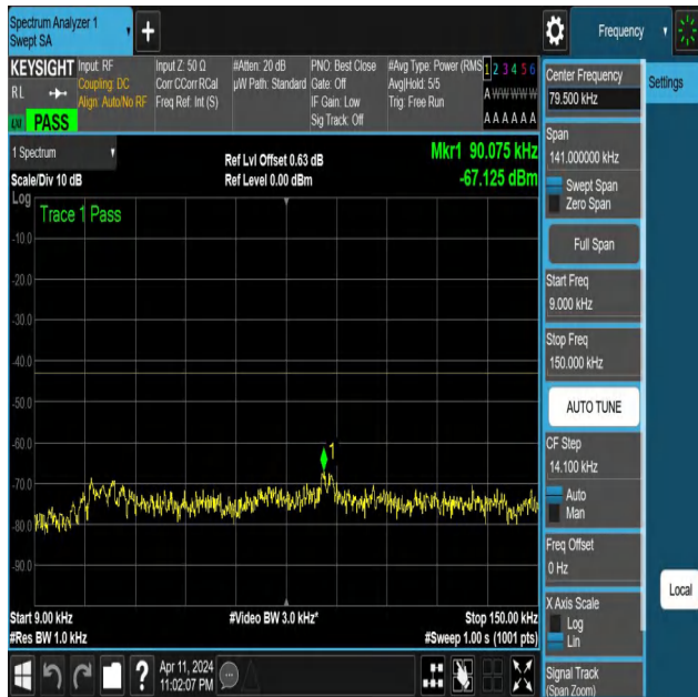
NTNV-N25-PC3-15-20-L-DFT-PI2BPSK-Edge_1RB_Right-0.009-0.15-Ant1-PASS
