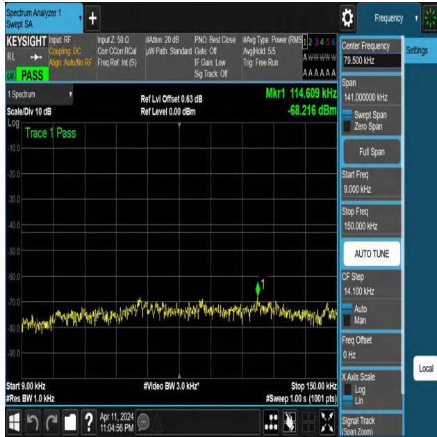
NTNV-N25-PC3-15-20-M-DFT-PI2BPSK-Edge_1RB_Left-0.009-0.15-Ant1-PASS
