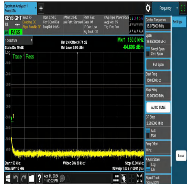
NTNV-N25-PC3-15-15-H-DFT-QPSK-Edge_1RB_Right-0.15-30-A nt1-PASS
