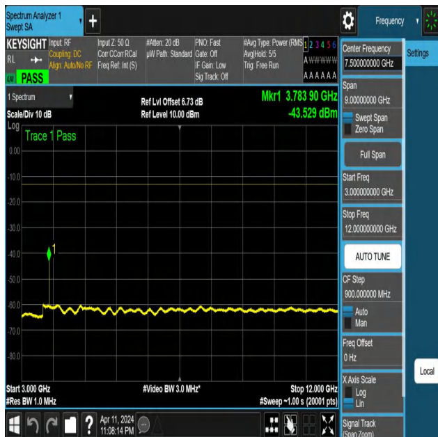
NTNV-N25-PC3-15-20-M-DFT-QPSK-Edge_1RB_Right-3000-12 000-Ant1-PASS
