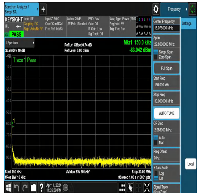
NTNV-N25-PC3-15-20-M-DFT-PI2BPSK-Edge_1RB_Right-0.15-3 0-Ant1-PASS
