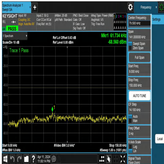
NTNV-N25-PC3-15-15-H-DFT-QPSK-Edge_1RB_Right-0.009-0.1 5-Ant1-PASS
