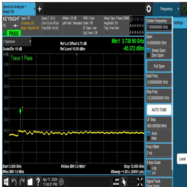
NTNV-N25-PC3-15-20-L-DFT-QPSK-Edge_1RB_Right-3000-12000-Ant1-PASS
