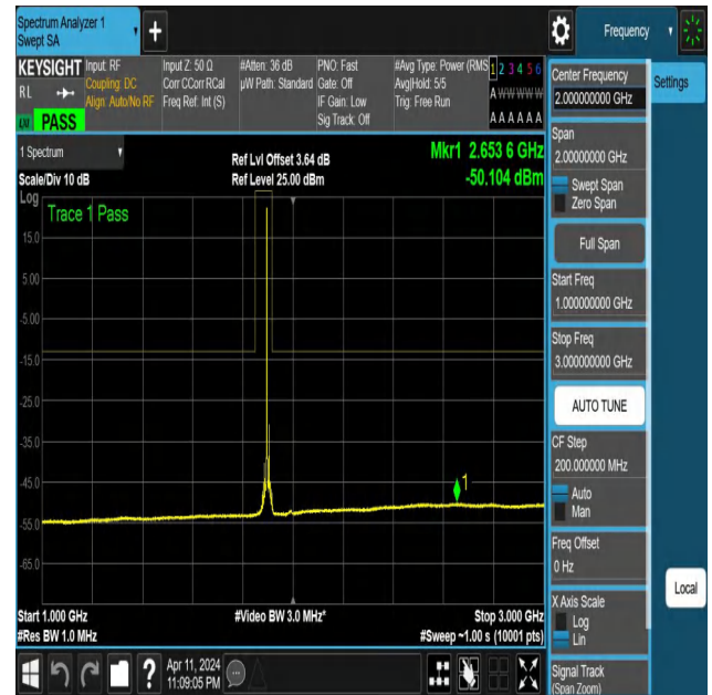
NTNV-N25-PC3-15-20-H-DFT-PI2BPSK-Edge_1RB_Left-1000-3000-Ant1-PASS
