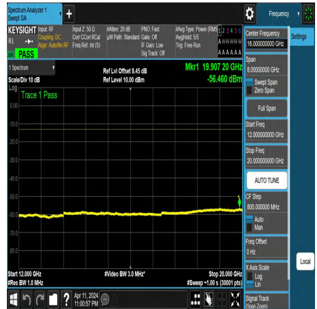
NTNV-N25-PC3-15-15-H-DFT-QPSK-Edge_1RB_Right-12000-20 000-Ant1-PASS
