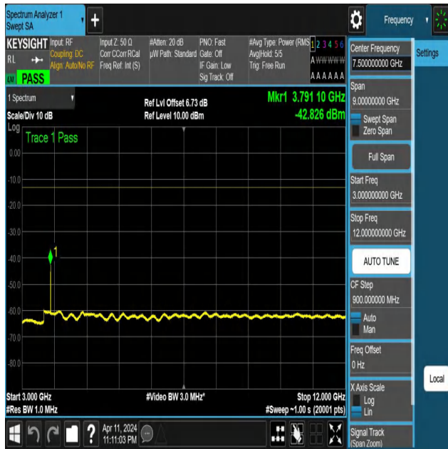
NTNV-N25-PC3-15-20-H-DFT-QPSK-Edge_1RB_Left-3000-1200 0-Ant1-PASS
