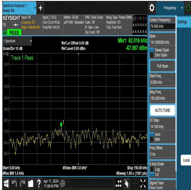
NTNV-N25-PC3-15-20-H-DFT-PI2BPSK-Edge_1RB_Left-0.009-0.15-Ant1-PASS
