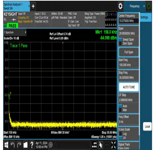
NTNV-N25-PC3-15-15-M-DFT-QPSK-Edge_1RB_Left-0.15-30-Ant 1-PASS
