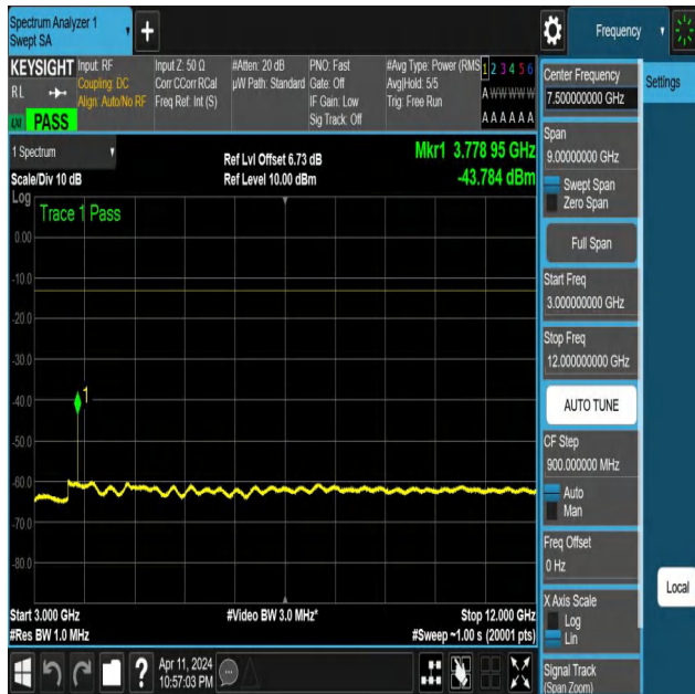
NTNV-N25-PC3-15-15-M-DFT-QPSK-Edge_1RB_Right-3000-12 000-Ant1-PASS
