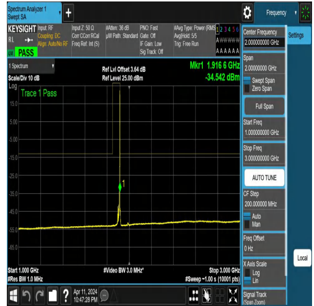
NTNV-N25-PC3-15-10-H-DFT-PI2BPSK-Edge_1RB_Right-1000-3 000-Ant1-PASS
