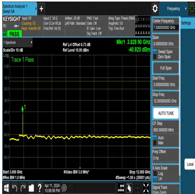
NTNV-N25-PC3-15-15-H-DFT-PI2BPSK-Edge_1RB_Right-3000- 12000-Ant1-PASS
