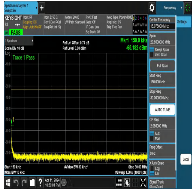
NTNV-N25-PC3-15-15-L-DFT-PI2BPSK-Edge_1RB_Left-0.15-30-Ant1-PASS
