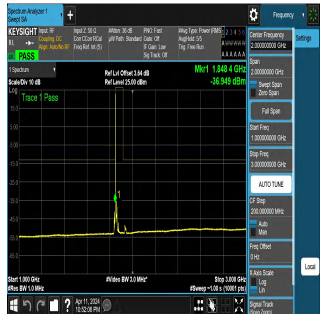
NTNV-N25-PC3-15-15-L-DFT-QPSK-Edge_1RB_Left-1000-3000-Ant1-PASS
