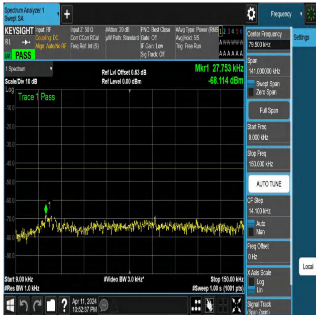
NTNV-N25-PC3-15-15-L-DFT-QPSK-Edge_1RB_Right-0.009-0.1 5-Ant1-PASS
