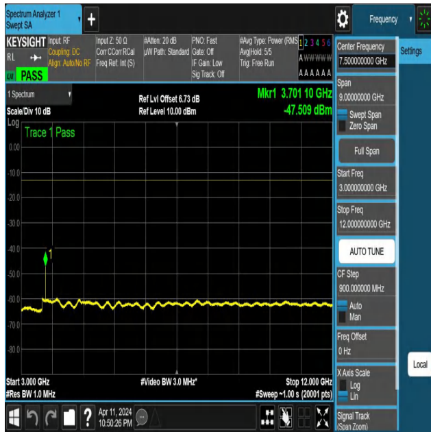
NTNV-N25-PC3-15-15-L-DFT-PI2BPSK-Edge_1RB_Left-3000-12000-Ant1-PASS
