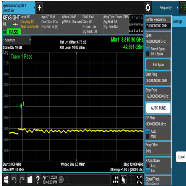
NTNV-N25-PC3-15-10-H-DFT-QPSK-Edge_1RB_Left-3000-1200 0-Ant1-PASS
