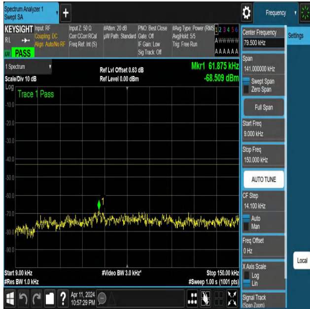
NTNV-N25-PC3-15-15-H-DFT-PI2BPSK-Edge_1RB_Left-0.009-0.15-Ant1-PASS
