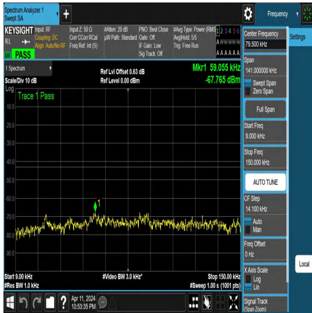
NTNV-N25-PC3-15-15-M-DFT-PI2BPSK-Edge_1RB_Left-0.009-0.15-Ant1-PASS
