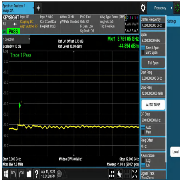
NTNV-N25-PC3-15-15-M-DFT-PI2BPSK-Edge_1RB_Left-3000-1 2000-Ant1-PASS
