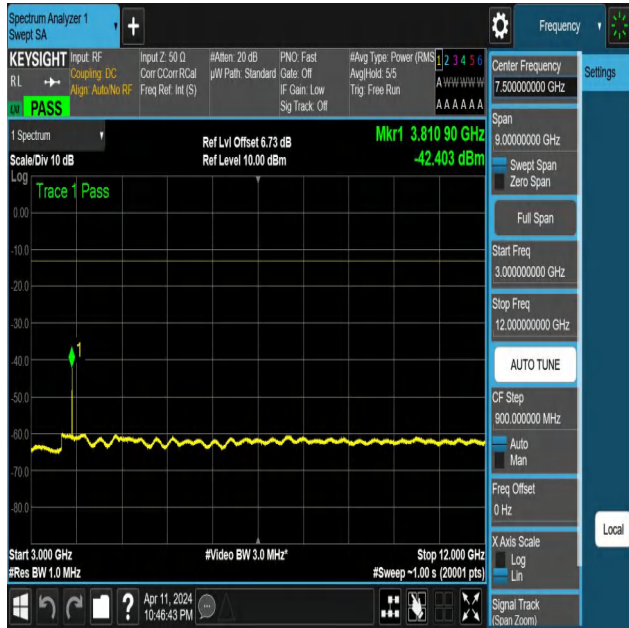
NTNV-N25-PC3-15-10-H-DFT-PI2BPSK-Edge_1RB_Left-3000-1 2000-Ant1-PASS
