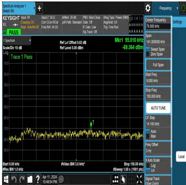
NTNV-N25-PC3-15-10-H-DFT-QPSK-Edge_1RB_Right-0.009-0.1 5-Ant1-PASS
