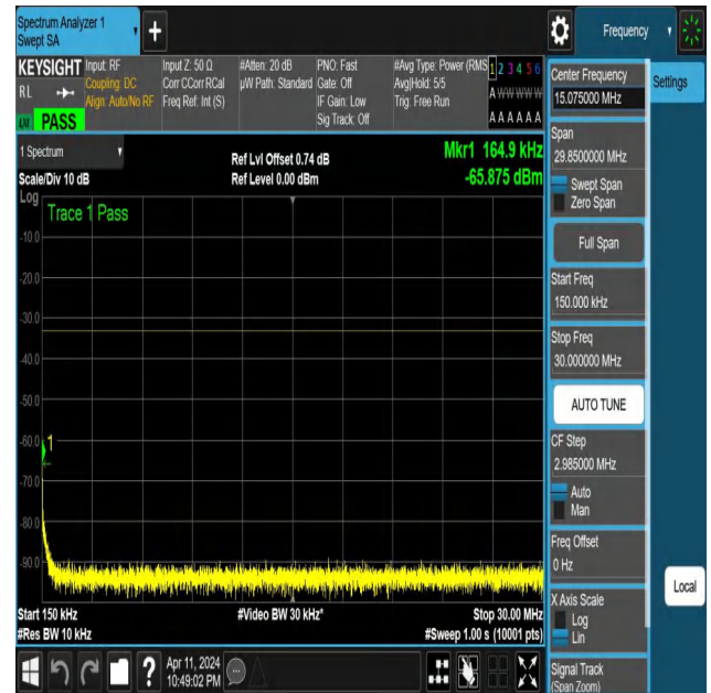
NTNV-N25-PC3-15-10-H-DFT-QPSK-Edge_1RB_Right-0.15-30-A nt1-PASS
