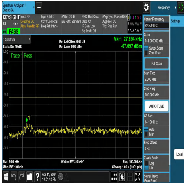
NTNV-N25-PC3-15-15-L-DFT-QPSK-Edge_1RB_Left-0.009-0.15-Ant1-PASS
