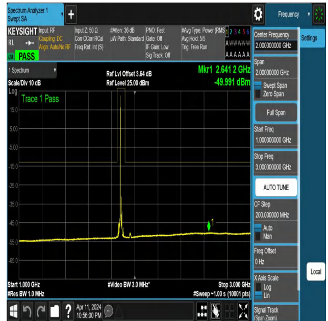
NTNV-N25-PC3-15-15-M-DFT-QPSK-Edge_1RB_Left-1000-3000-A Ant1-PASS
