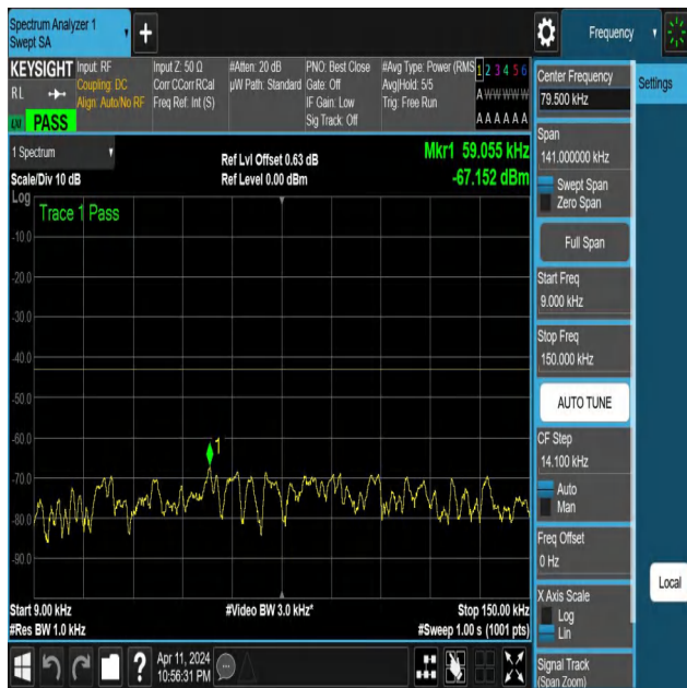
NTNV-N25-PC3-15-15-M-DFT-QPSK-Edge_1RB_Right-0.009-0. 15-Ant1-PASS
