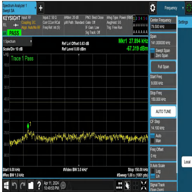
NTNV-N25-PC3-15-15-L-DFT-PI2BPSK-Edge_1RB_Left-0.009-0.15-Ant1-PASS
