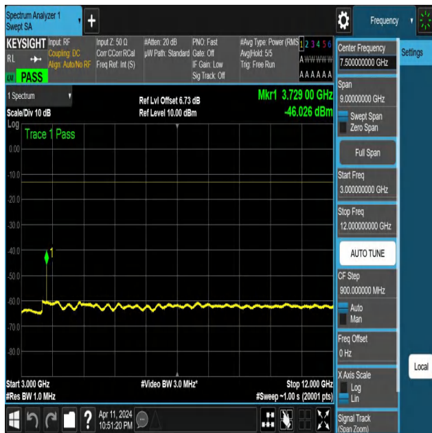
NTNV-N25-PC3-15-15-L-DFT-PI2BPSK-Edge_1RB_Right-3000- 12000-Ant1-PASS
