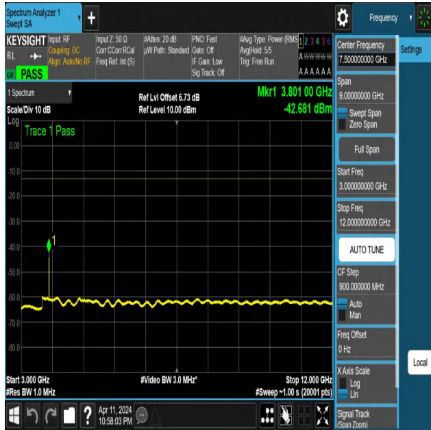
NTNV-N25-PC3-15-15-H-DFT-PI2BPSK-Edge_1RB_Left-3000-1 2000-Ant1-PASS
