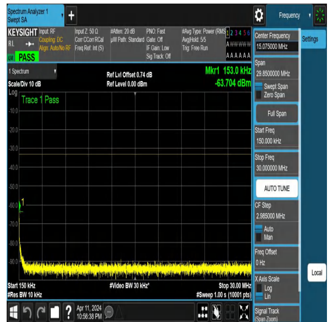
NTNV-N25-PC3-15-15-M-DFT-QPSK-Edge_1RB_Right-0.15-30-A nt1-PASS
