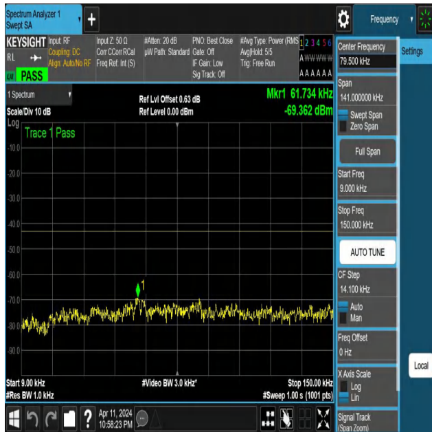
NTNV-N25-PC3-15-15-H-DFT-PI2BPSK-Edge_1RB_Right-0.009- 0.15-Ant1-PASS
