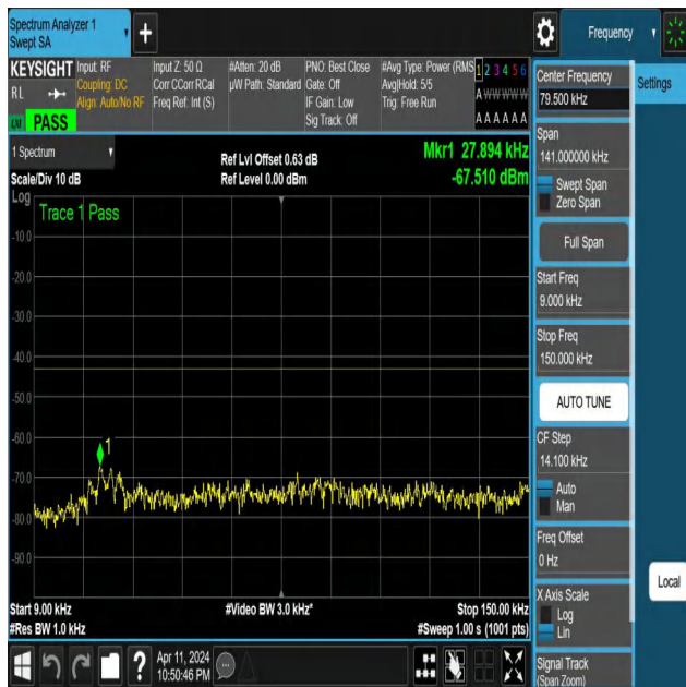
NTNV-N25-PC3-15-15-L-DFT-PI2BPSK-Edge_1RB_Right-0.009-0.15-Ant1-PASS
