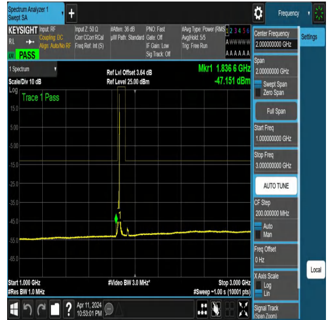
NTNV-N25-PC3-15-15-L-DFT-QPSK-Edge_1RB_Right-1000-3000-Ant1-PASS
