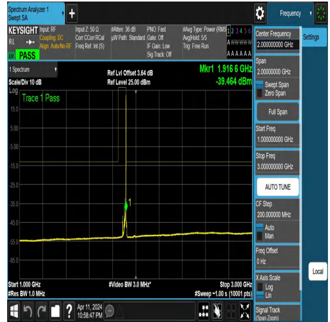
NTNV-N25-PC3-15-15-H-DFT-PI2BPSK-Edge_1RB_Right-1000-3 000-Ant1-PASS
