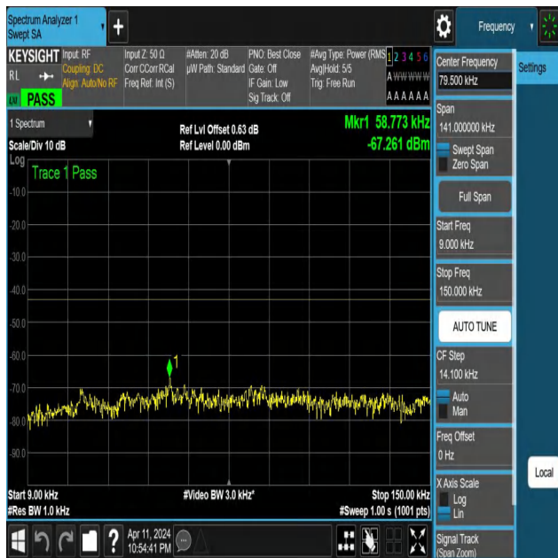
NTNV-N25-PC3-15-15-M-DFT-PI2BPSK-Edge_1RB_Right-0.009 -0.15-Ant1-PASS
