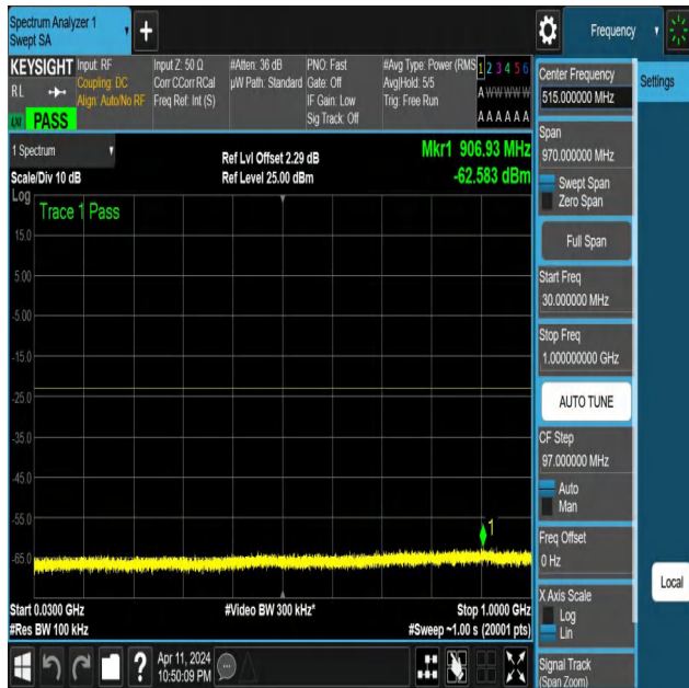
NTNV-N25-PC3-15-15-L-DFT-PI2BPSK-Edge_1RB_Left-30-1000-Ant1-PASS
