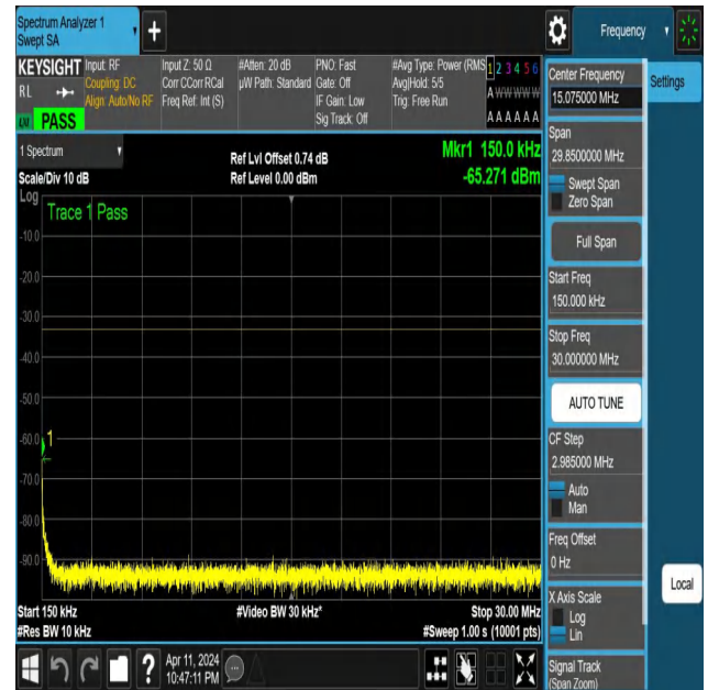
NTNV-N25-PC3-15-10-H-DFT-PI2BPSK-Edge_1RB_Right-0.15-3 0-Ant1-PASS
