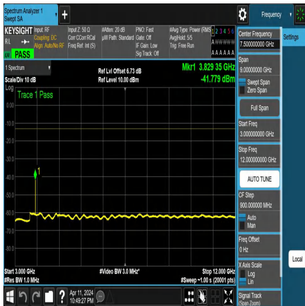
NTNV-N25-PC3-15-10-H-DFT-QPSK-Edge_1RB_Right-3000-120 00-Ant1-PASS
