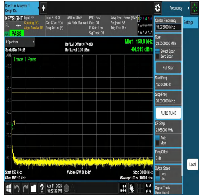
NTNV-N25-PC3-15-15-H-DFT-PI2BPSK-Edge_1RB_Left-0.15-30-Ant1-PASS
