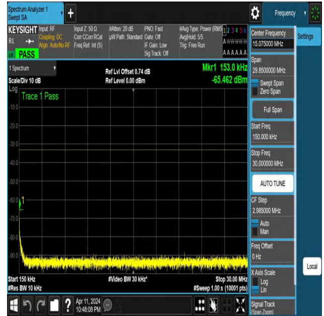
NTNV-N25-PC3-15-10-H-DFT-QPSK-Edge_1RB_Left-0.15-30-Ant 1-PASS
