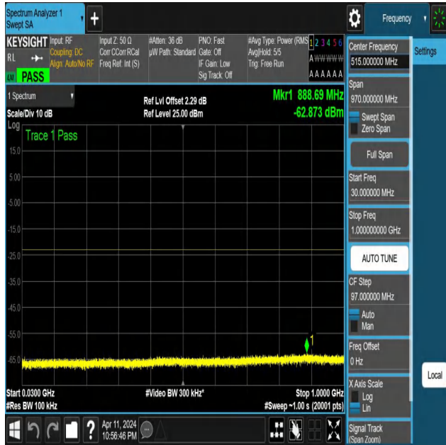
NTNV-N25-PC3-15-15-M-DFT-QPSK-Edge_1RB_Right-30-1000- Ant1-PASS
