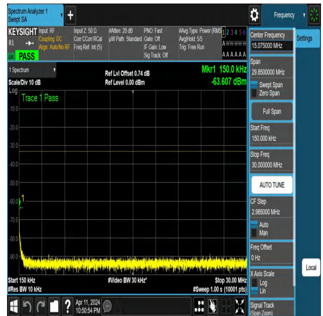
NTNV-N25-PC3-15-15-L-DFT-PI2BPSK-Edge_1RB_Right-0.15-30-Ant1-PASS
