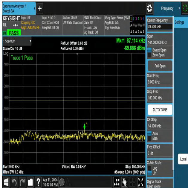
NTNV-N25-PC3-15-10-H-DFT-PI2BPSK-Edge_1RB_Right-0.009- 0.15-Ant1-PASS
