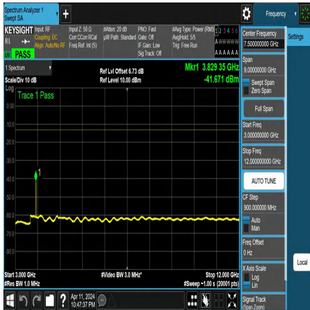
NTNV-N25-PC3-15-10-H-DFT-PI2BPSK-Edge_1RB_Right-3000- 12000-Ant1-PASS
