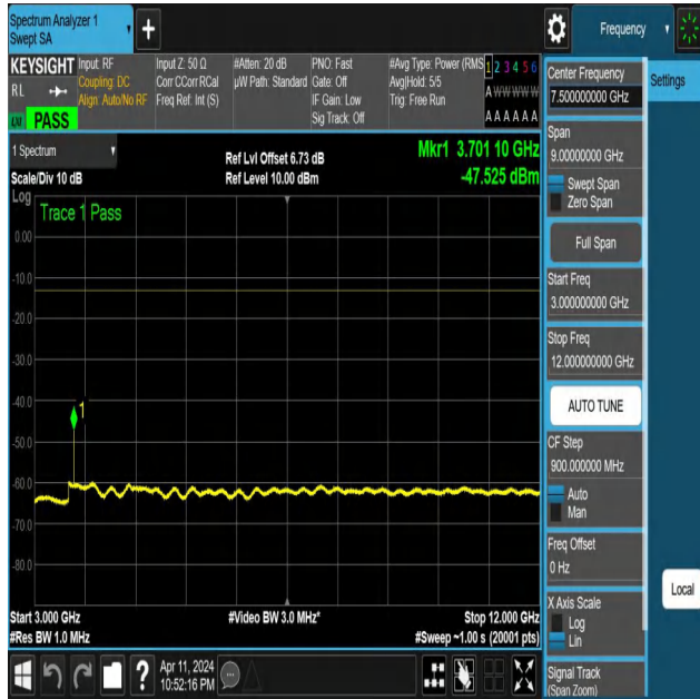
NTNV-N25-PC3-15-15-L-DFT-QPSK-Edge_1RB_Left-3000-1200 0-Ant1-PASS
