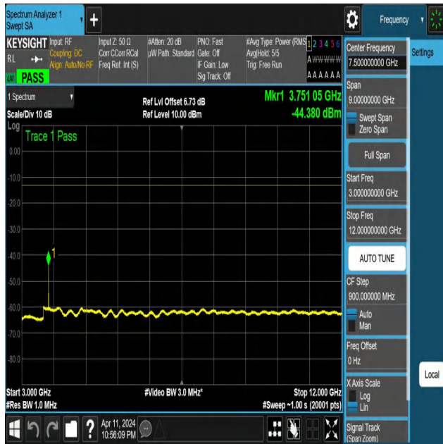
NTNV-N25-PC3-15-15-M-DFT-QPSK-Edge_1RB_Left-3000-1200 0-Ant1-PASS
