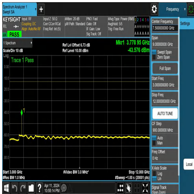
NTNV-N25-PC3-15-15-M-DFT-PI2BPSK-Edge_1RB_Right-3000- 12000-Ant1-PASS
