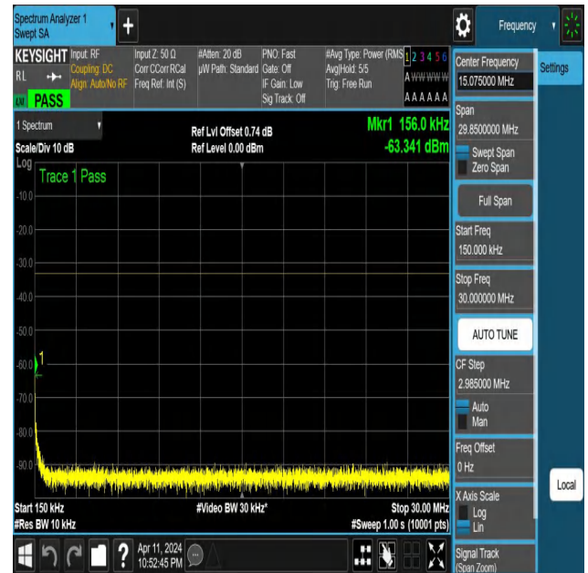
NTNV-N25-PC3-15-15-L-DFT-QPSK-Edge_1RB_Right-0.15-30-A nt1-PASS
