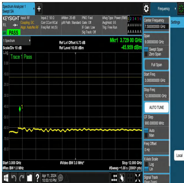
NTNV-N25-PC3-15-15-L-DFT-QPSK-Edge_1RB_Right-3000-12000-Ant1-PASS
