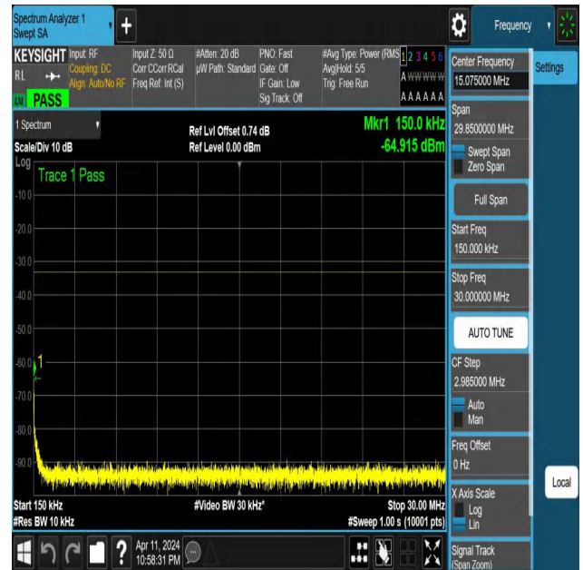
NTNV-N25-PC3-15-15-H-DFT-PI2BPSK-Edge_1RB_Right-0.15-3 0-Ant1-PASS
