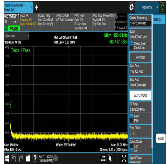
NTNV-N25-PC3-15-15-M-DFT-PI2BPSK-Edge_1RB_Left-0.15-30-Ant1-PASS
