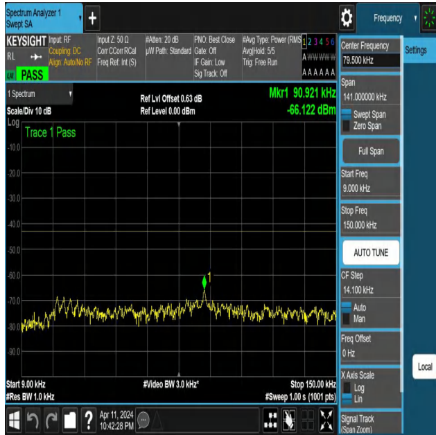
NTNV-N25-PC3-15-10-M-DFT-PI2BPSK-Edge_1RB_Left-0.009-0.15-Ant1-PASS
