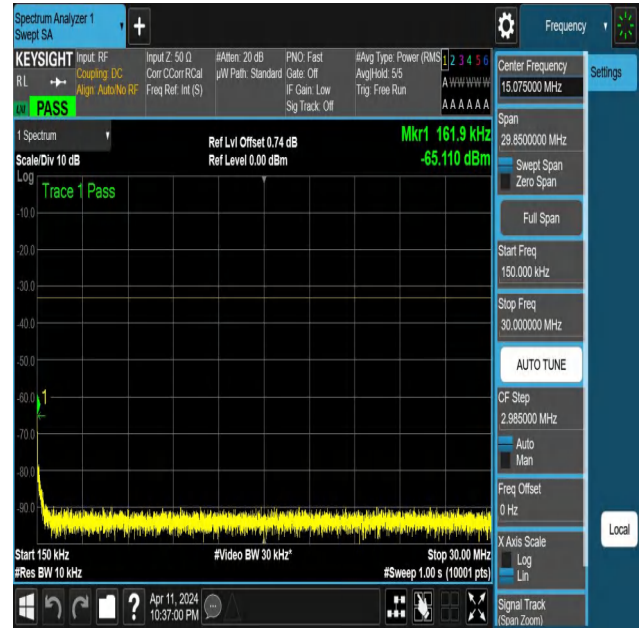
NTNV-N25-PC3-15-5-H-DFT-QPSK-Edge_1RB_Left-0.15-30-Ant1-PASS
