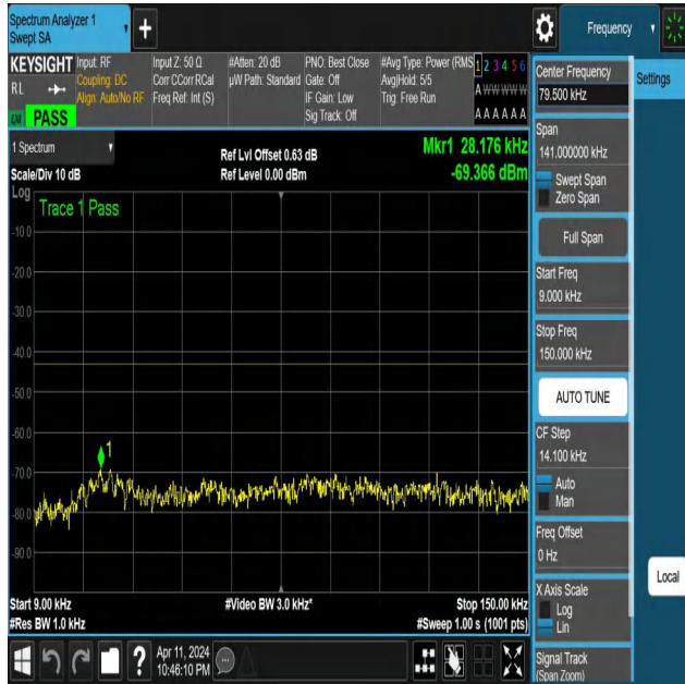
NTNV-N25-PC3-15-10-H-DFT-PI2BPSK-Edge_1RB_Left-0.009-0.15-Ant1-PASS
