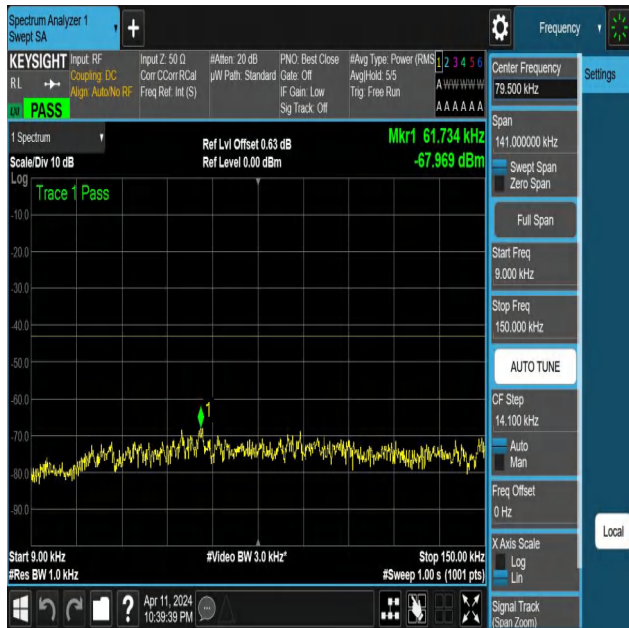
NTNV-N25-PC3-15-10-L-DFT-PI2BPSK-Edge_1RB_Right-0.009-0.15-Ant1-PASS
