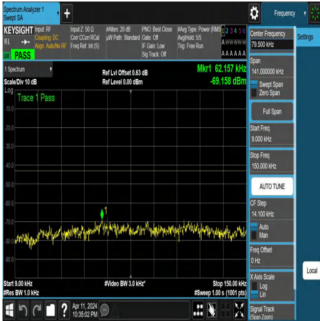
NTNV-N25-PC3-15-5-H-DFT-PI2BPSK-Edge_1RB_Left-0.009-0. 15-Ant1-PASS
