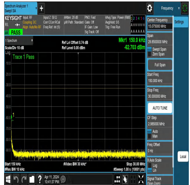
NTNV-N25-PC3-15-10-L-DFT-QPSK-Edge_1RB_Right-0.15-30-A nt1-PASS
