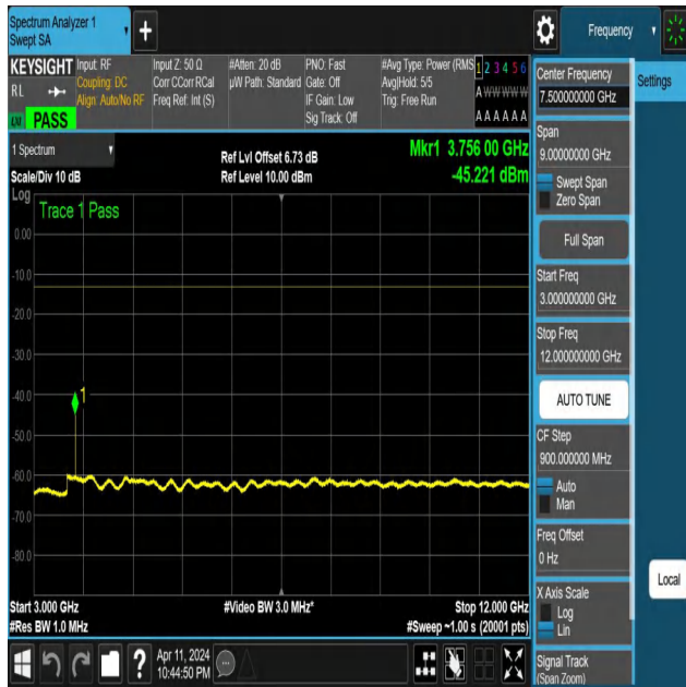
NTNV-N25-PC3-15-10-M-DFT-QPSK-Edge_1RB_Left-3000-1200 0-Ant1-PASS
