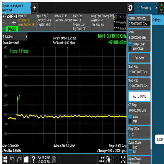
NTNV-N25-PC3-15-10-L-DFT-QPSK-Edge_1RB_Right-3000-12000-Ant1-PASS
