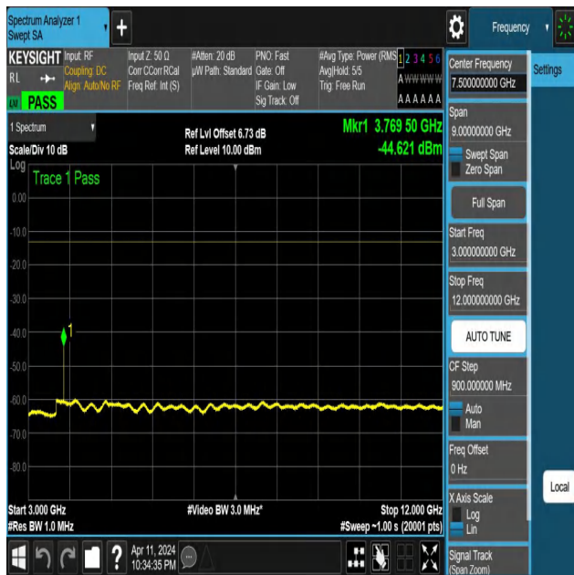
NTNV-N25-PC3-15-5-M-DFT-QPSK-Edge_1RB_Right-3000-120 00-Ant1-PASS
