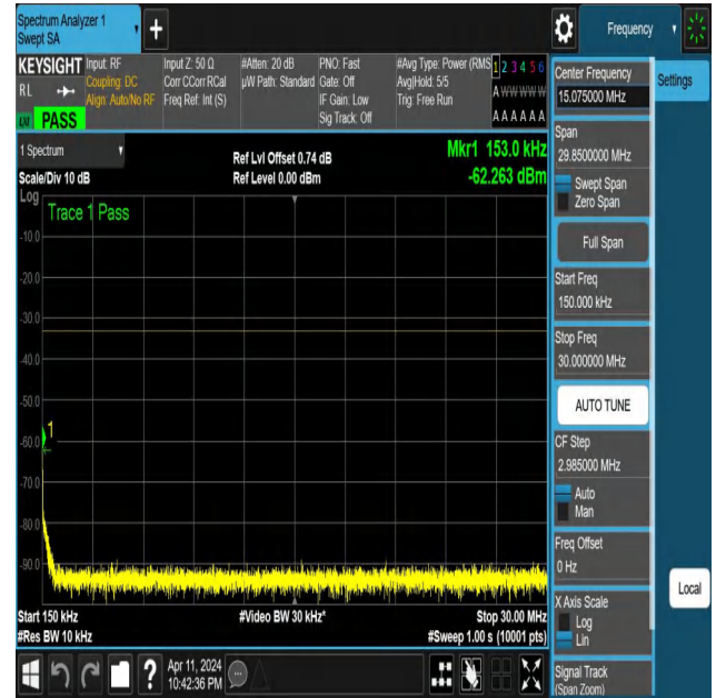
NTNV-N25-PC3-15-10-M-DFT-PI2BPSK-Edge_1RB_Left-0.15-30-Ant1-PASS
