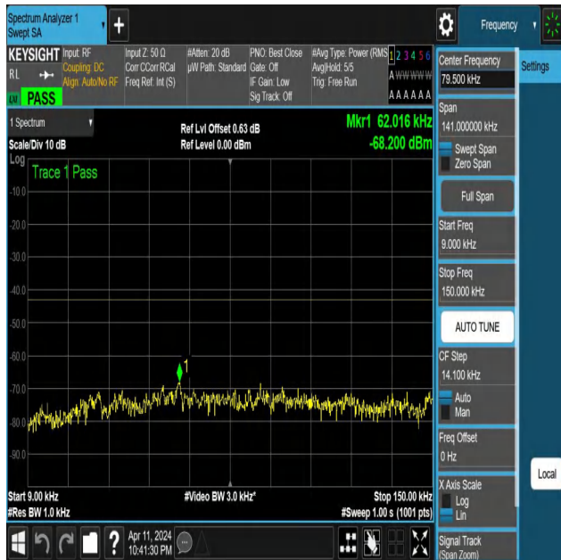
NTNV-N25-PC3-15-10-L-DFT-QPSK-Edge_1RB_Right-0.009-0.1 5-Ant1-PASS
