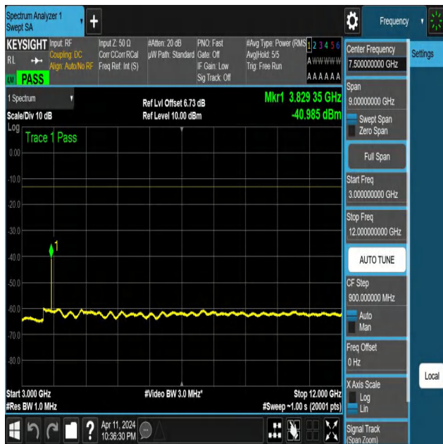
NTNV-N25-PC3-15-5-H-DFT-PI2BPSK-Edge_1RB_Right-3000-1 2000-Ant1-PASS
