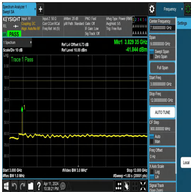
NTNV-N25-PC3-15-5-H-DFT-QPSK-Edge_1RB_Right-3000-1200 0-Ant1-PASS
