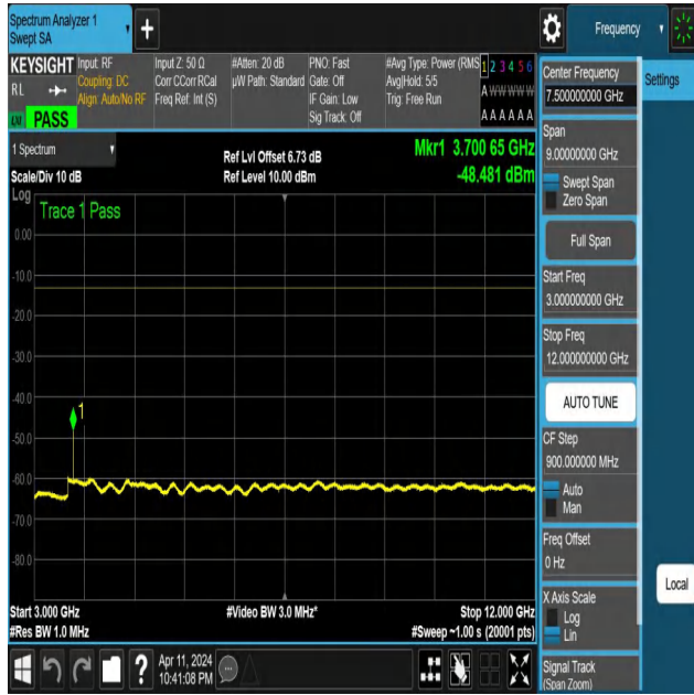
NTNV-N25-PC3-15-10-L-DFT-QPSK-Edge_1RB_Left-3000-1200 0-Ant1-PASS
