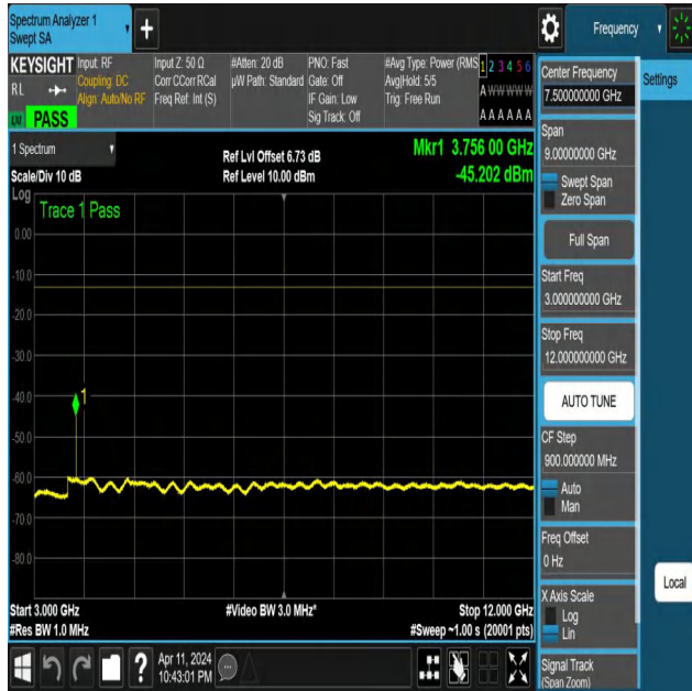
NTNV-N25-PC3-15-10-M-DFT-PI2BPSK-Edge_1RB_Left-3000-1 2000-Ant1-PASS
