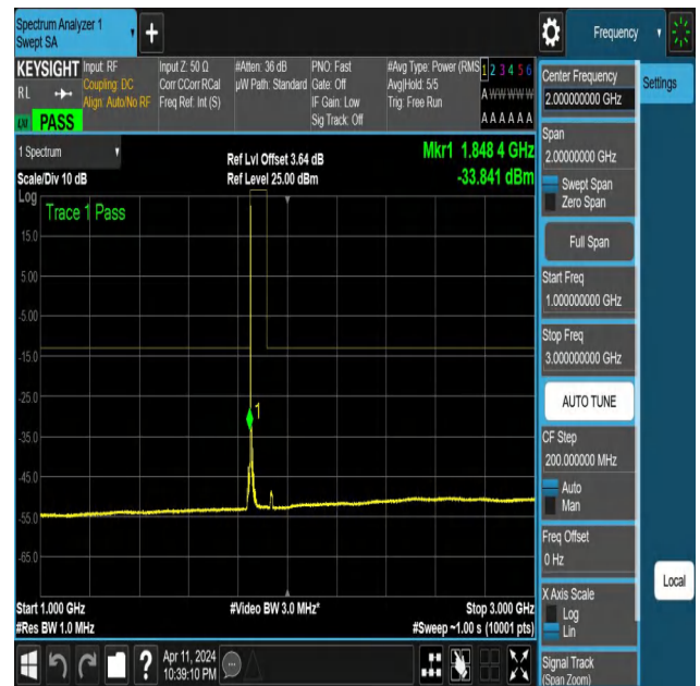
NTNV-N25-PC3-15-10-L-DFT-PI2BPSK-Edge_1RB_Left-1000-3000-Ant1-PASS
