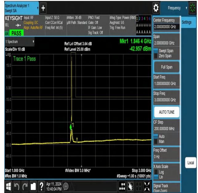
NTNV-N25-PC3-15-10-L-DFT-PI2BPSK-Edge_1RB_Right-1000-3000-Ant1-PASS
