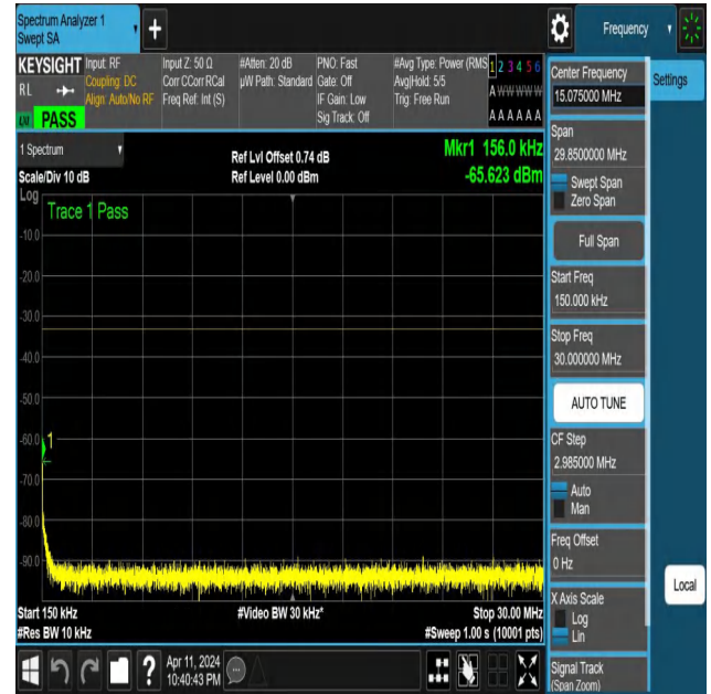
NTNV-N25-PC3-15-10-L-DFT-QPSK-Edge_1RB_Left-0.15-30-Ant 1-PASS
