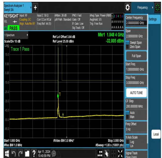
NTNV-N25-PC3-15-10-L-DFT-QPSK-Edge_1RB_Left-1000-3000-Ant1-PASS
