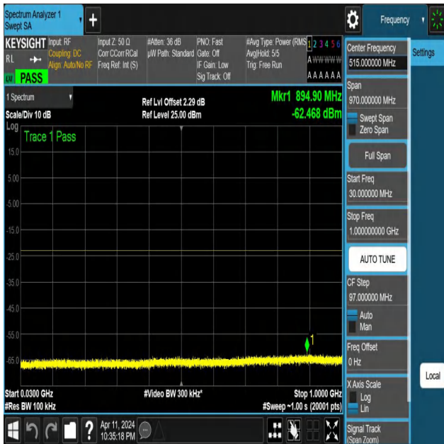
NTNV-N25-PC3-15-5-H-DFT-PI2BPSK-Edge_1RB_Left-30-1000- Ant1-PASS
