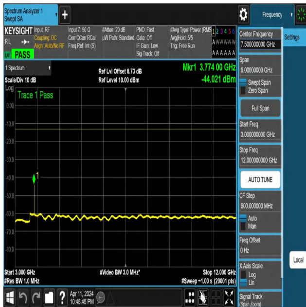
NTNV-N25-PC3-15-10-M-DFT-QPSK-Edge_1RB_Right-3000-12 000-Ant1-PASS
