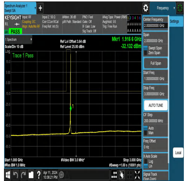
NTNV-N25-PC3-15-5-H-DFT-PI2BPSK-Edge_1RB_Right-1000-30 00-Ant1-PASS
