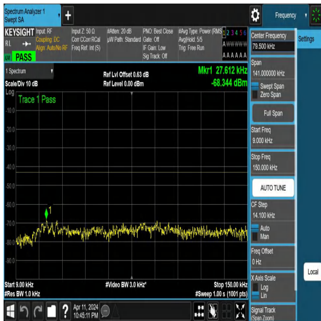
NTNV-N25-PC3-15-10-M-DFT-QPSK-Edge_1RB_Right-0.009-0. 15-Ant1-PASS
