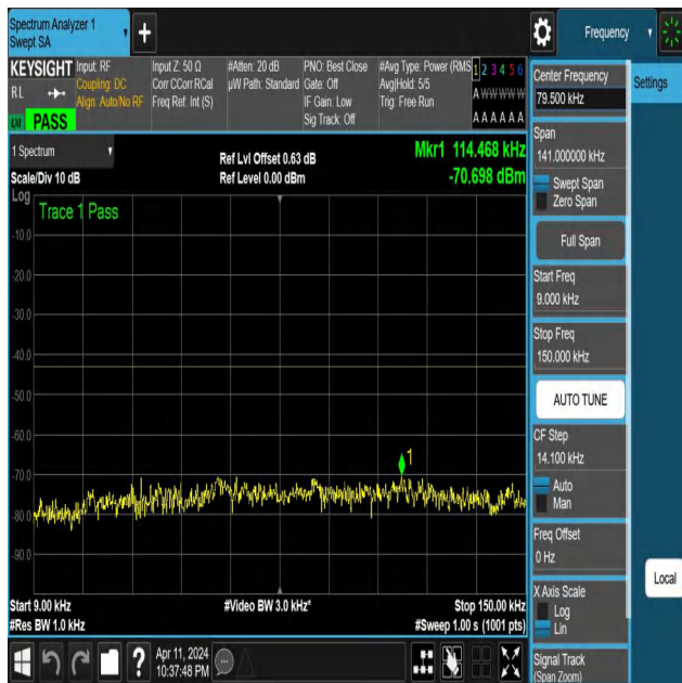
NTNV-N25-PC3-15-5-H-DFT-QPSK-Edge_1RB_Right-0.009-0.15 -Ant1-PASS
