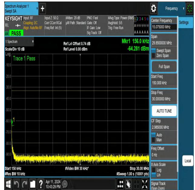
NTNV-N25-PC3-15-10-M-DFT-PI2BPSK-Edge_1RB_Right-0.15-3 0-Ant1-PASS
