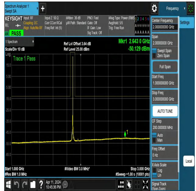
NTNV-N25-PC3-15-10-M-DFT-QPSK-Edge_1RB_Right-1000-300 0-Ant1-PASS
