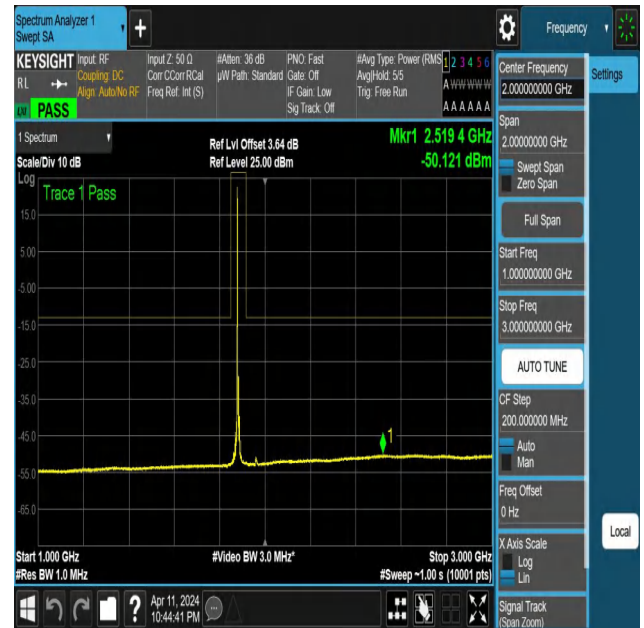
NTNV-N25-PC3-15-10-M-DFT-QPSK-Edge_1RB_Left-1000-3000- Ant1-PASS
