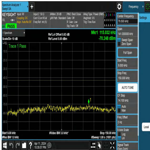
NTNV-N25-PC3-15-5-H-DFT-PI2BPSK-Edge_1RB_Right-0.009-0.15-Ant1-PASS
