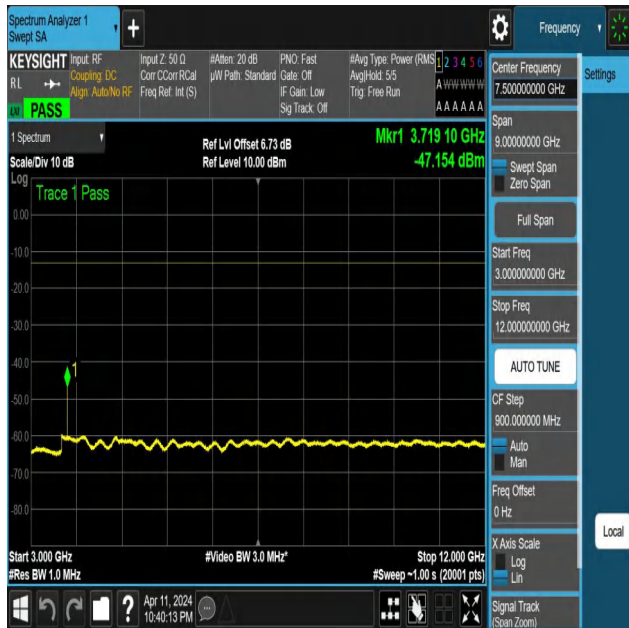
NTNV-N25-PC3-15-10-L-DFT-PI2BPSK-Edge_1RB_Right-3000-12000-Ant1-PASS
