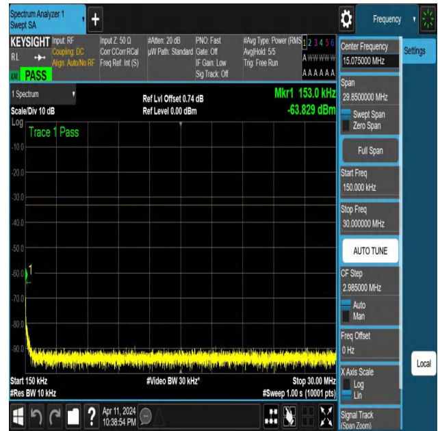
NTNV-N25-PC3-15-10-L-DFT-PI2BPSK-Edge_1RB_Left-0.15-30-Ant1-PASS
