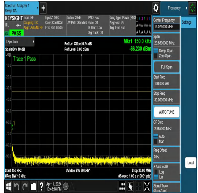
NTNV-N25-PC3-15-10-H-DFT-PI2BPSK-Edge_1RB_Left-0.15-30-Ant1-PASS
