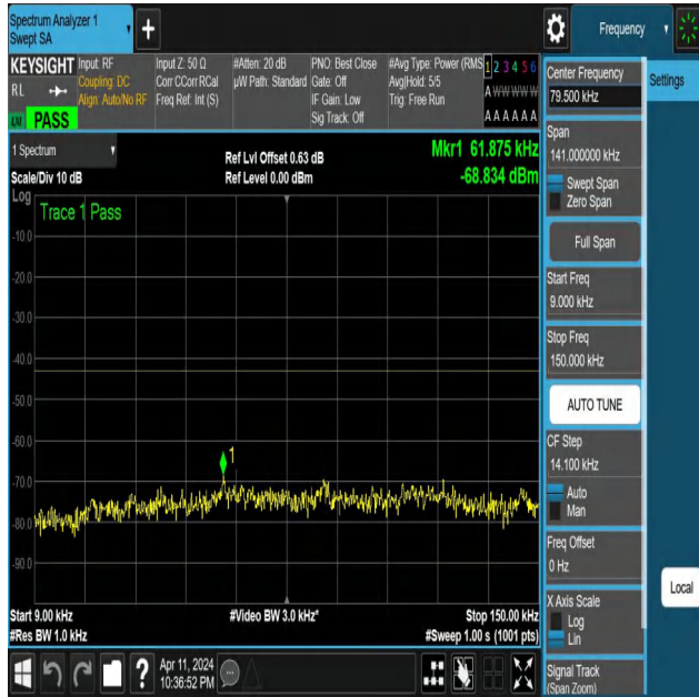
NTNV-N25-PC3-15-5-H-DFT-QPSK-Edge_1RB_Left-0.009-0.15-Ant1-PASS
