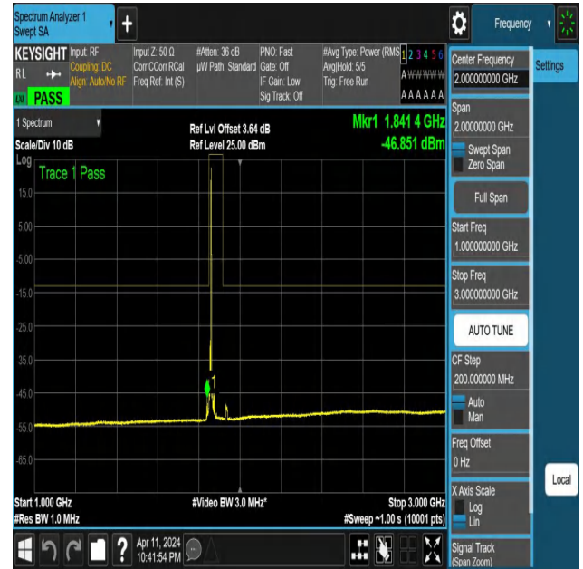
NTNV-N25-PC3-15-10-L-DFT-QPSK-Edge_1RB_Right-1000-3000-Ant1-PASS
