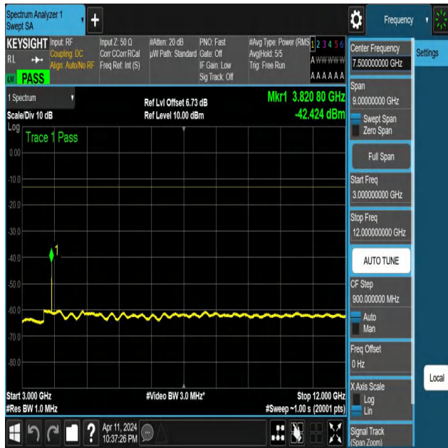
NTNV-N25-PC3-15-5-H-DFT-QPSK-Edge_1RB_Left-3000-12000 -Ant1-PASS
