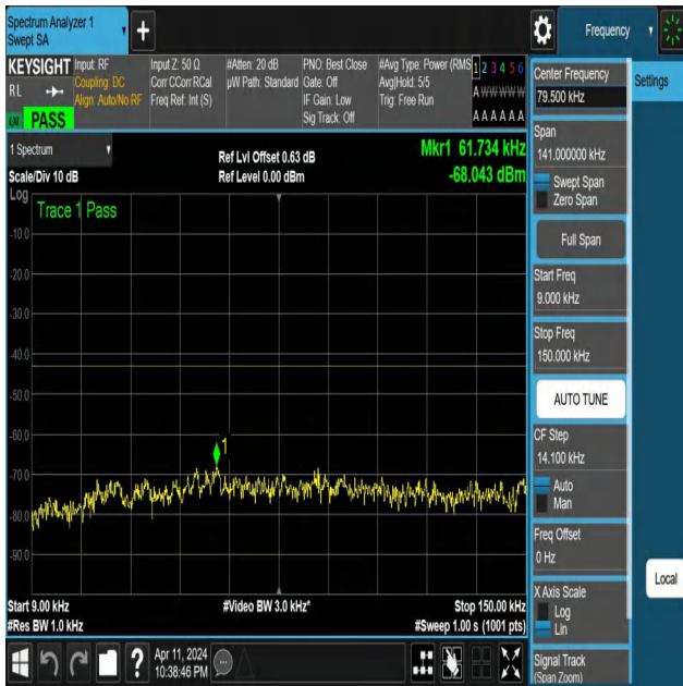
NTNV-N25-PC3-15-10-L-DFT-PI2BPSK-Edge_1RB_Left-0.009-0.15-Ant1-PASS
