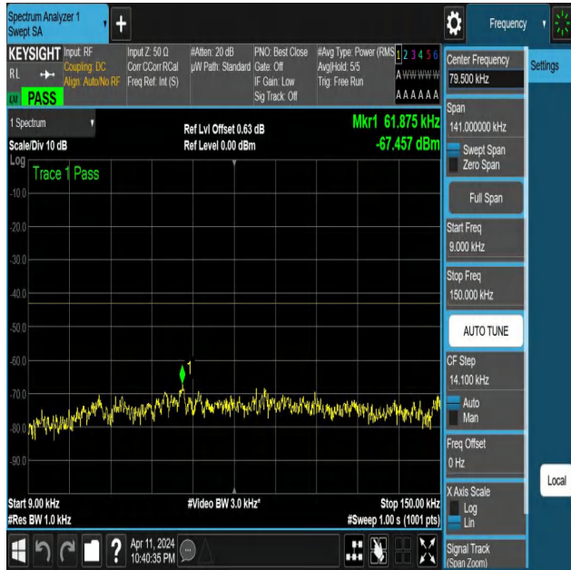
NTNV-N25-PC3-15-10-L-DFT-QPSK-Edge_1RB_Left-0.009-0.15-Ant1-PASS
