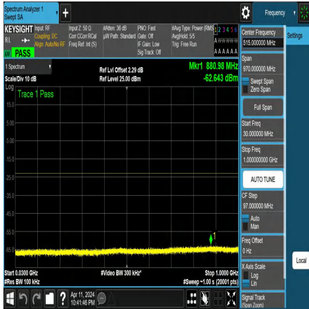
NTNV-N25-PC3-15-10-L-DFT-QPSK-Edge_1RB_Right-30-1000-Ant1-PASS
