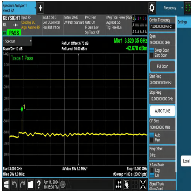
NTNV-N25-PC3-15-5-H-DFT-PI2BPSK-Edge_1RB_Left-3000-12000-Ant1-PASS
