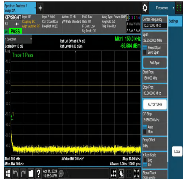
NTNV-N25-PC3-15-5-H-DFT-PI2BPSK-Edge_1RB_Right-0.15-30-Ant1-PASS
