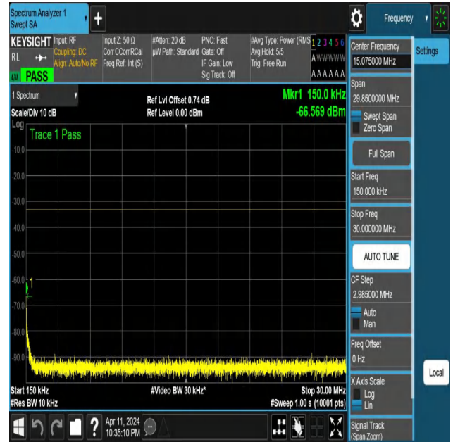
NTNV-N25-PC3-15-5-H-DFT-PI2BPSK-Edge_1RB_Left-0.15-30-A nt1-PASS
