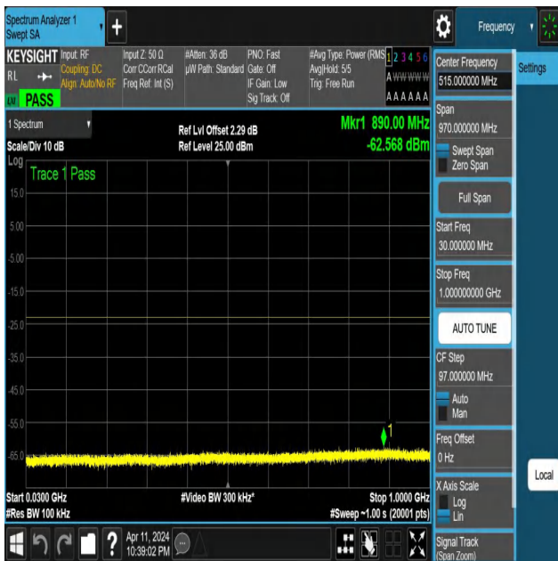
NTNV-N25-PC3-15-10-L-DFT-PI2BPSK-Edge_1RB_Left-30-1000-Ant1-PASS
