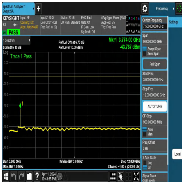
NTNV-N25-PC3-15-10-M-DFT-PI2BPSK-Edge_1RB_Right-3000- 12000-Ant1-PASS
