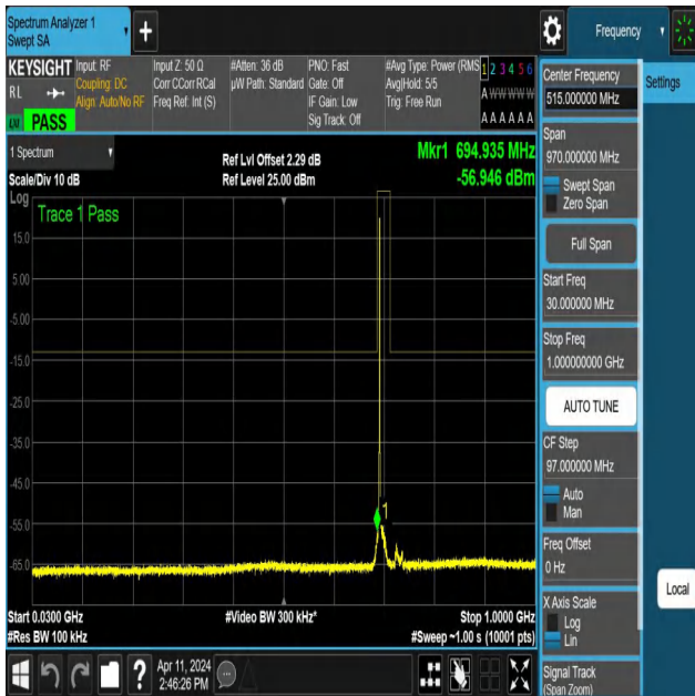
NTNV-N12-PC3-15-15-L-DFT-QPSK-Edge_1RB_Left-30-1000-Ant1-PASS
