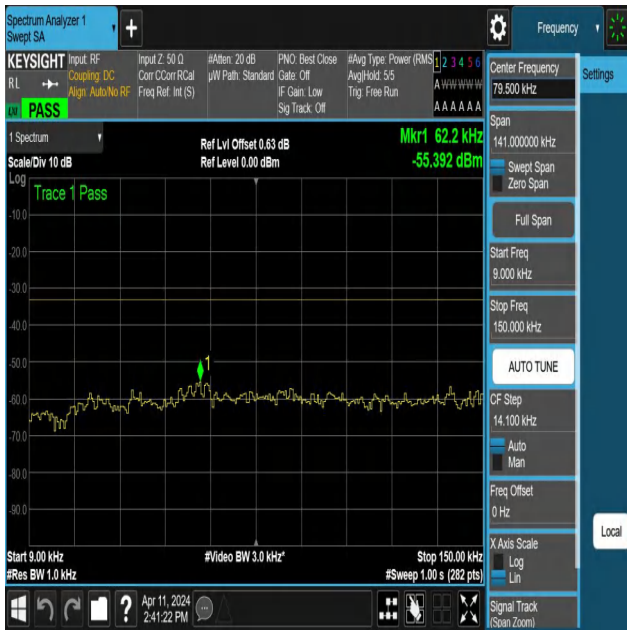
NTNV-N12-PC3-15-10-H-DFT-PI2BPSK-Edge_1RB_Right-0.009- 0.15-Ant1-PASS
