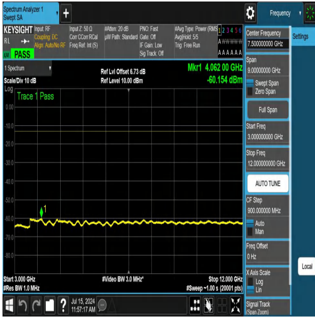
NTNV-N12-PC3-15-10-H-DFT-QPSK-Edge_1RB_Left-3000-1200 0-Ant1-PASS
