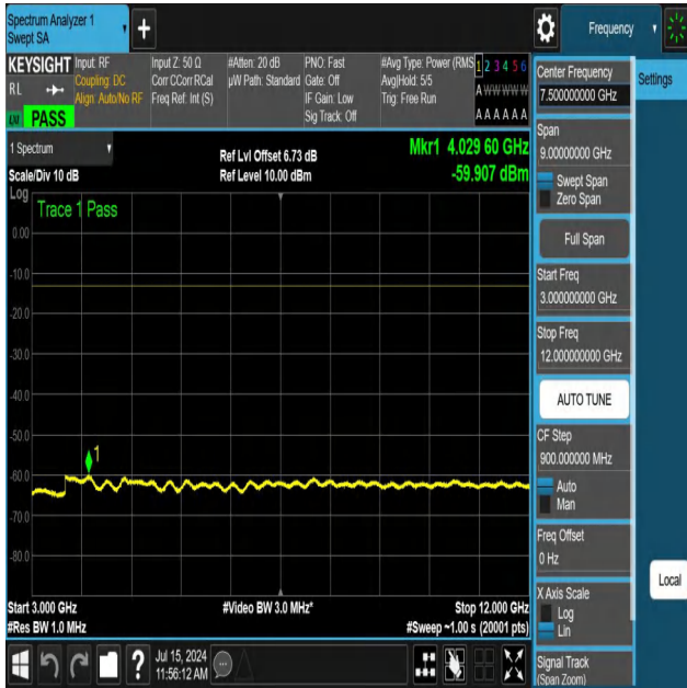
NTNV-N12-PC3-15-10-M-DFT-QPSK-Edge_1RB_Left-3000-1200 0-Ant1-PASS
