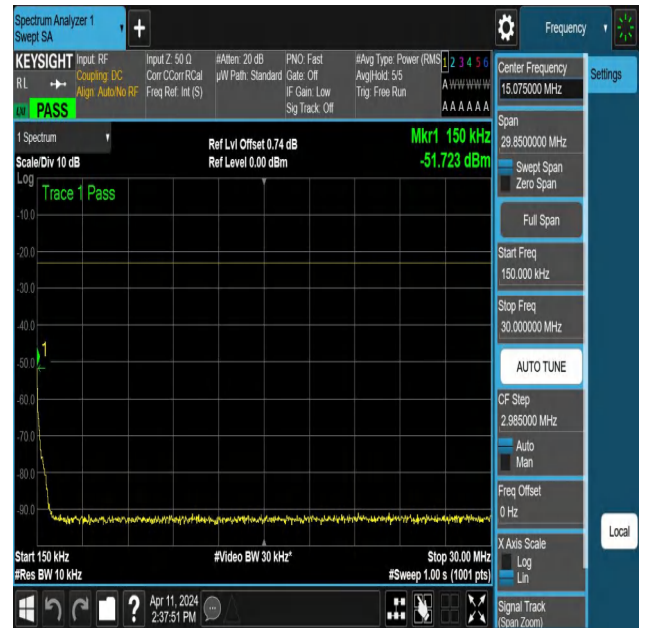
NTNV-N12-PC3-15-10-M-DFT-PI2BPSK-Edge_1RB_Right-0.15-3 0-Ant1-PASS
