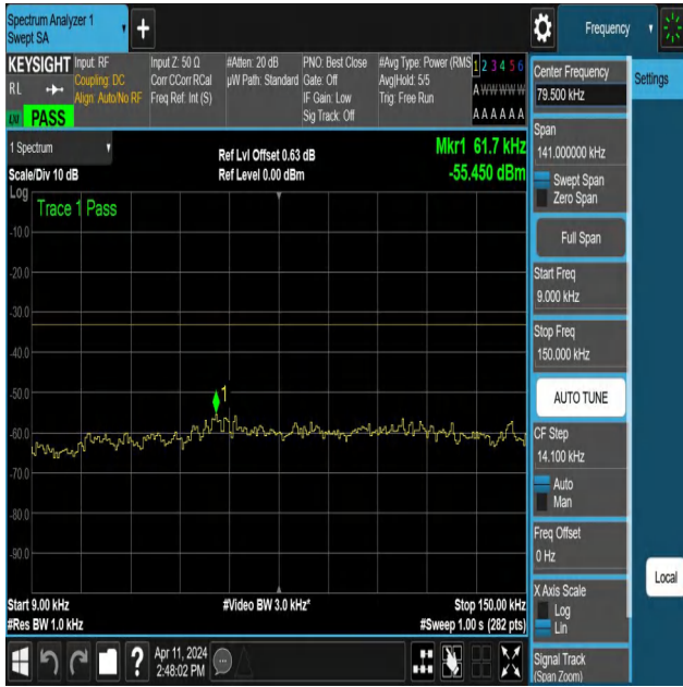
NTNV-N12-PC3-15-15-M-DFT-PI2BPSK-Edge_1RB_Left-0.009-0.15-Ant1-PASS
