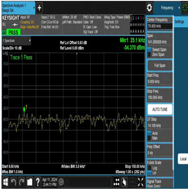
NTNV-N12-PC3-15-15-L-DFT-PI2BPSK-Edge_1RB_Left-0.009-0.15-Ant1-PASS
