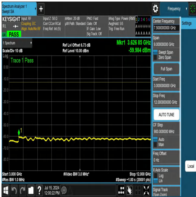
NTNV-N12-PC3-15-15-L-DFT-QPSK-Edge_1RB_Right-3000-12000-Ant1-PASS
