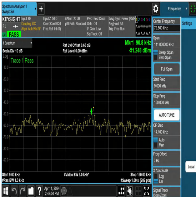
NTNV-N12-PC3-15-15-L-DFT-QPSK-Edge_1RB_Right-0.009-0.1 5-Ant1-PASS
