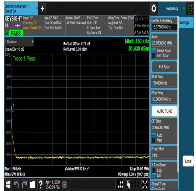
NTNV-N12-PC3-15-15-M-DFT-PI2BPSK-Edge_1RB_Right-0.15-3 0-Ant1-PASS
