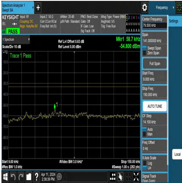
NTNV-N12-PC3-15-10-M-DFT-QPSK-Edge_1RB_Left-0.009-0.15 -Ant1-PASS
