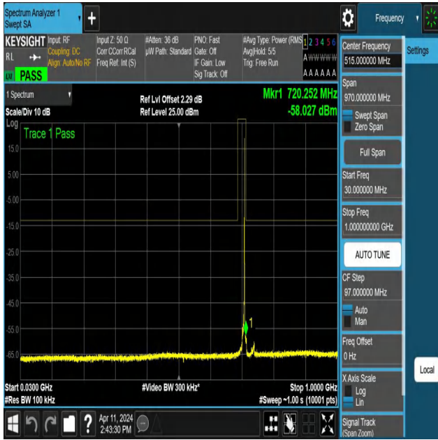
NTNV-N12-PC3-15-10-H-DFT-QPSK-Edge_1RB_Right-30-1000-Ant1-PASS
