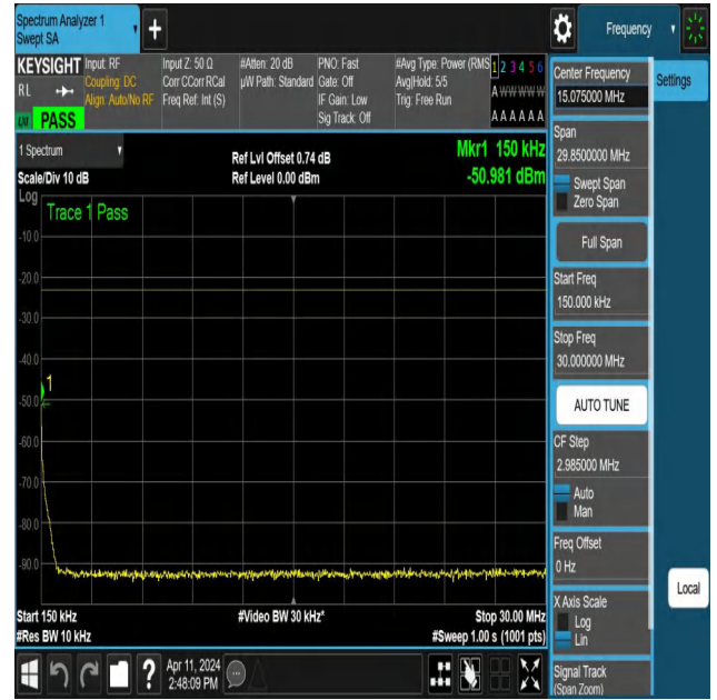
NTNV-N12-PC3-15-15-M-DFT-PI2BPSK-Edge_1RB_Left-0.15-30-Ant1-PASS
