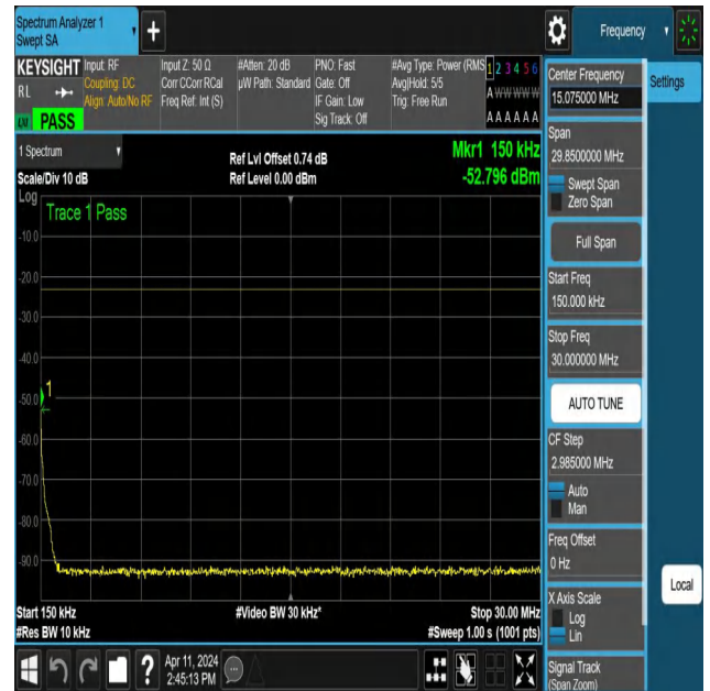
NTNV-N12-PC3-15-15-L-DFT-PI2BPSK-Edge_1RB_Right-0.15-30-Ant1-PASS
