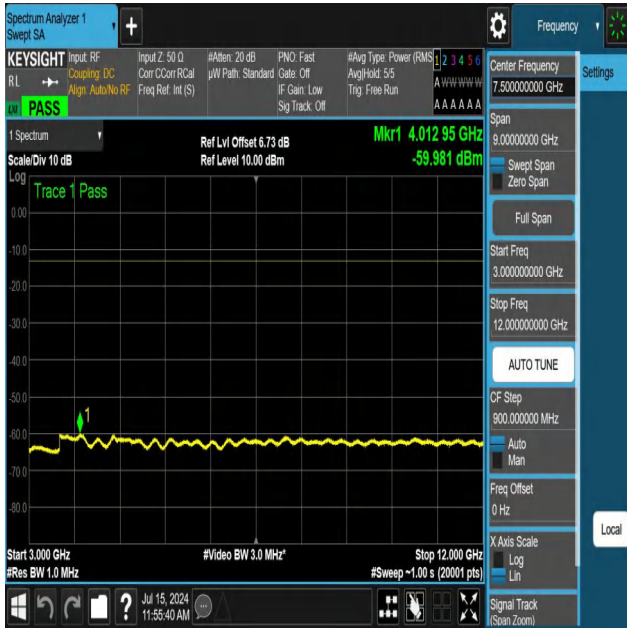
NTNV-N12-PC3-15-10-M-DFT-PI2BPSK-Edge_1RB_Left-3000-1 2000-Ant1-PASS
