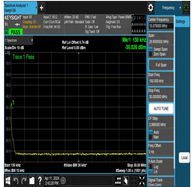
NTNV-N12-PC3-15-10-H-DFT-QPSK-Edge_1RB_Left-0.15-30-Ant 1-PASS
