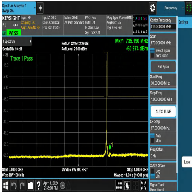
NTNV-N12-PC3-15-10-M-DFT-PI2BPSK-Edge_1RB_Right-30-10 00-Ant1-PASS
