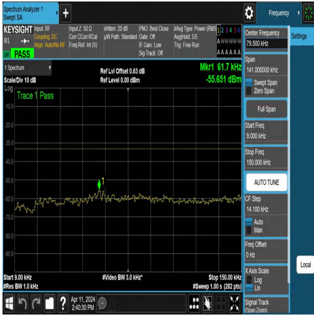
NTNV-N12-PC3-15-10-H-DFT-PI2BPSK-Edge_1RB_Left-0.009-0.15-Ant1-PASS
