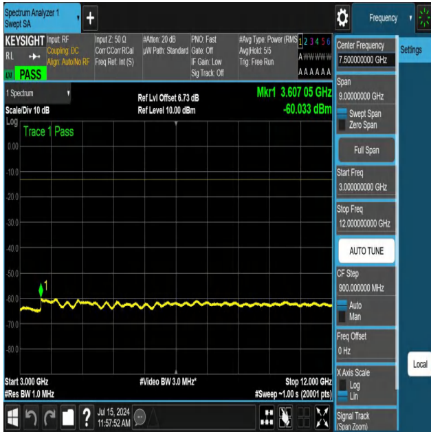
NTNV-N12-PC3-15-15-L-DFT-PI2BPSK-Edge_1RB_Left-3000-12000-Ant1-PASS
