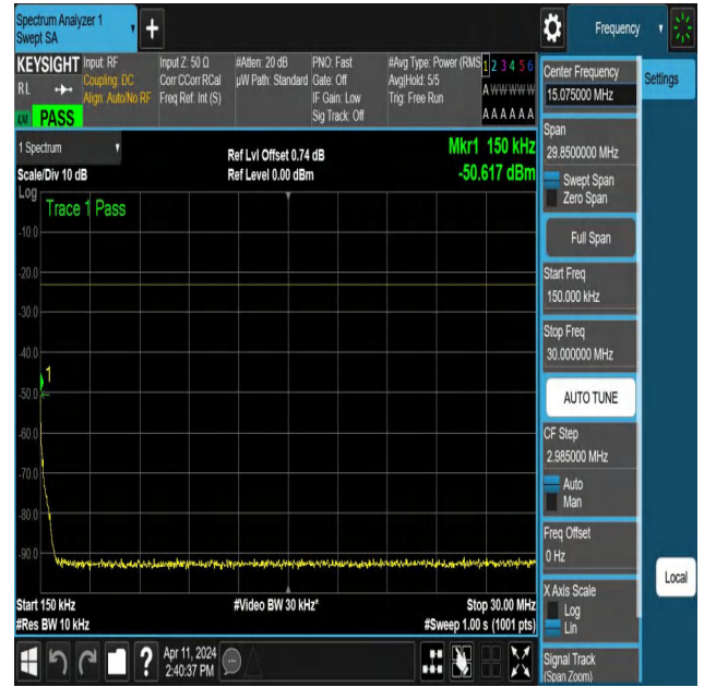
NTNV-N12-PC3-15-10-H-DFT-PI2BPSK-Edge_1RB_Left-0.15-30-Ant1-PASS
