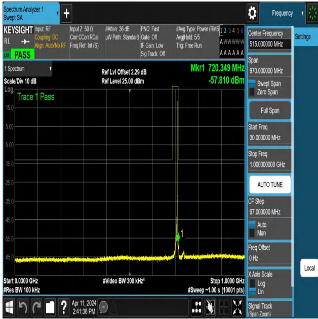
NTNV-N12-PC3-15-10-H-DFT-PI2BPSK-Edge_1RB_Right-30-10 00-Ant1-PASS
