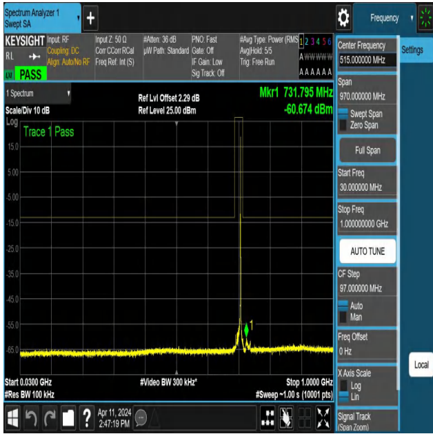
NTNV-N12-PC3-15-15-L-DFT-QPSK-Edge_1RB_Right-30-1000-Ant1-PASS
