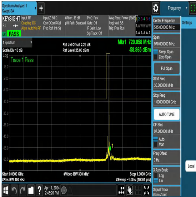
NTNV-N12-PC3-15-15-L-DFT-PI2BPSK-Edge_1RB_Right-30-1000-Ant1-PASS
