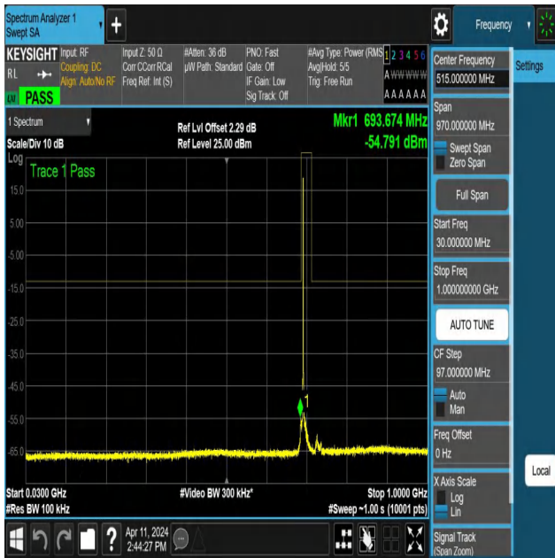
NTNV-N12-PC3-15-15-L-DFT-PI2BPSK-Edge_1RB_Left-30-1000-Ant1-PASS
