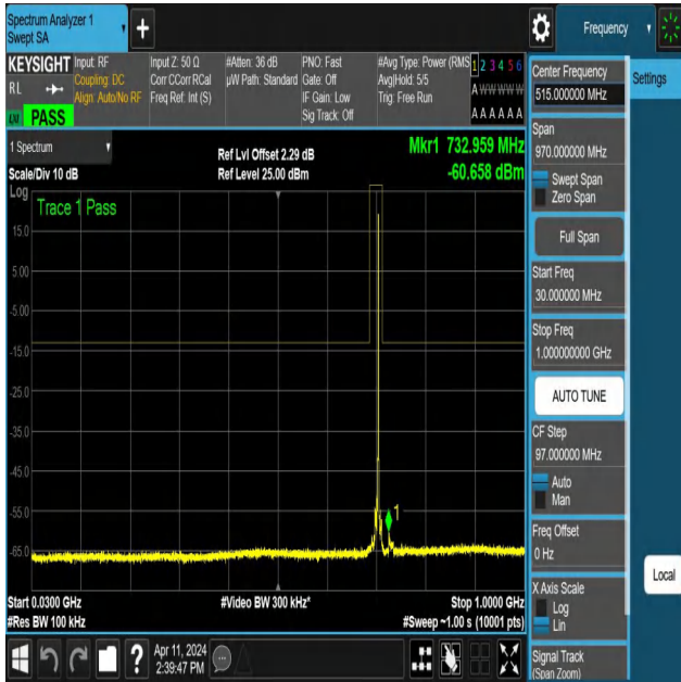
NTNV-N12-PC3-15-10-M-DFT-QPSK-Edge_1RB_Right-30-1000-Ant1-PASS
