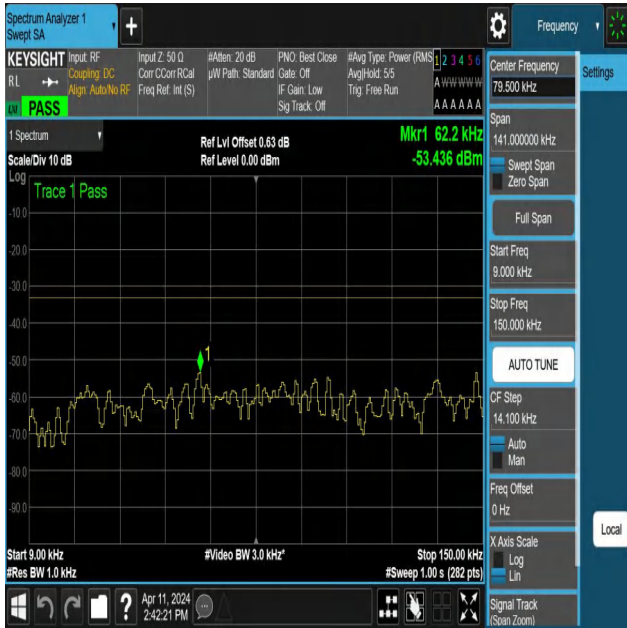
NTNV-N12-PC3-15-10-H-DFT-QPSK-Edge_1RB_Left-0.009-0.15 -Ant1-PASS
