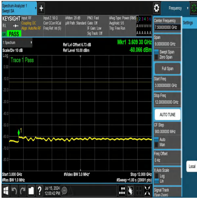
NTNV-N12-PC3-15-15-M-DFT-PI2BPSK-Edge_1RB_Left-3000-1 2000-Ant1-PASS
