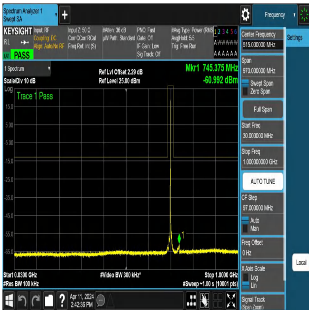
NTNV-N12-PC3-15-10-H-DFT-QPSK-Edge_1RB_Left-30-1000-A nt1-PASS
