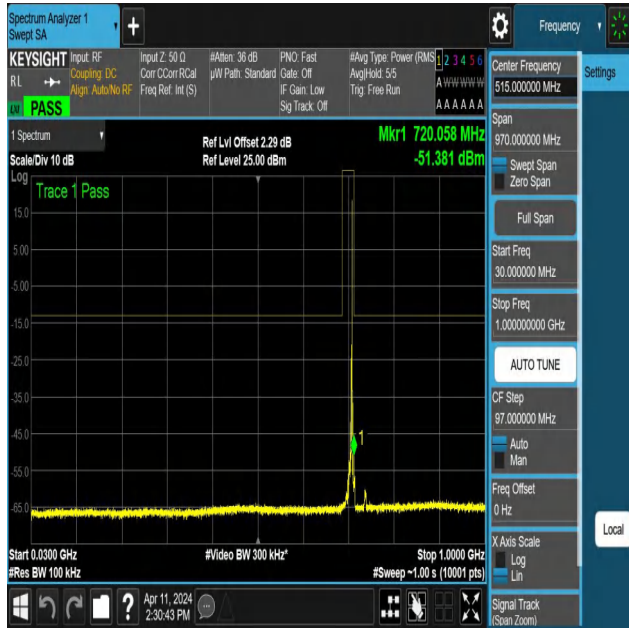
NTNV-N12-PC3-15-5-H-DFT-PI2BPSK-Edge_1RB_Right-30-100 0-Ant1-PASS
