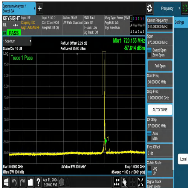
NTNV-N12-PC3-15-5-H-DFT-PI2BPSK-Edge_1RB_Left-30-1000-Ant1-PASS
