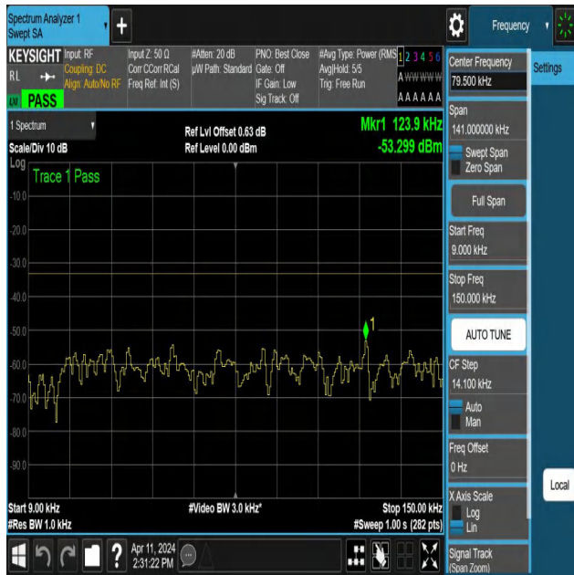
NTNV-N12-PC3-15-5-H-DFT-QPSK-Edge_1RB_Left-0.009-0.15-Ant1-PASS
