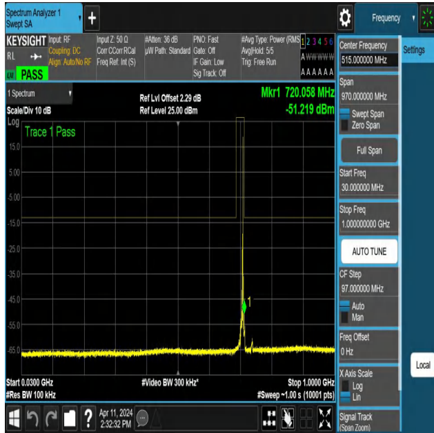
NTNV-N12-PC3-15-5-H-DFT-QPSK-Edge_1RB_Right-30-1000-A nt1-PASS
