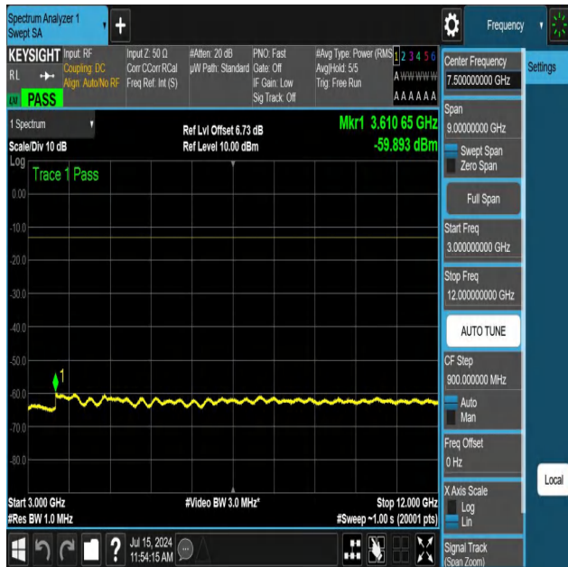
NTNV-N12-PC3-15-5-H-DFT-QPSK-Edge_1RB_Right-3000-1200 0-Ant1-PASS
