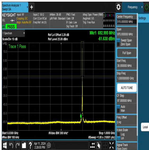
NTNV-N12-PC3-15-5-M-DFT-QPSK-Edge_1RB_Left-30-1000-An t1-PASS
