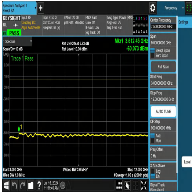
NTNV-N12-PC3-15-5-L-DFT-QPSK-Edge_1RB_Left-3000-12000- Ant1-PASS
