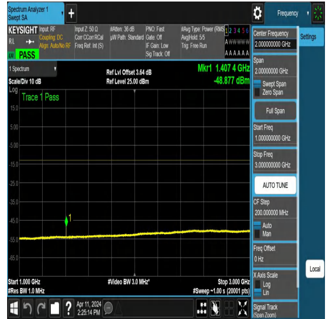
NTNV-N12-PC3-15-5-L-DFT-QPSK-Edge_1RB_Right-1000-3000- Ant1-PASS
