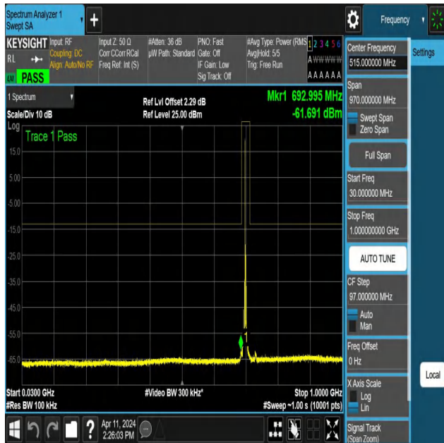
NTNV-N12-PC3-15-5-M-DFT-PI2BPSK-Edge_1RB_Left-30-1000-Ant1-PASS
