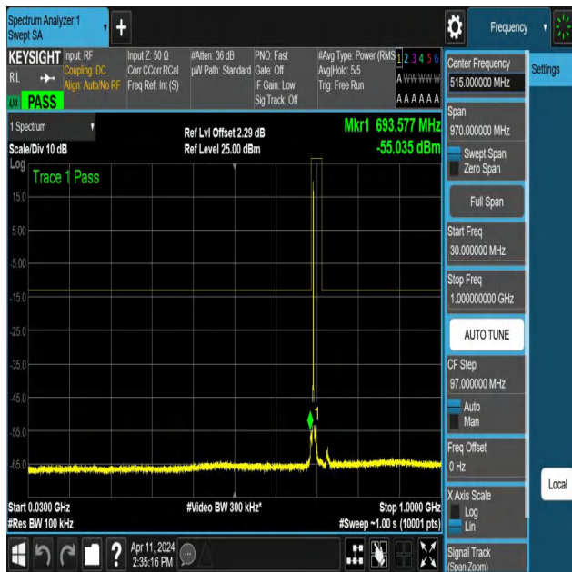
NTNV-N12-PC3-15-10-L-DFT-QPSK-Edge_1RB_Left-30-1000-Ant1-PASS
