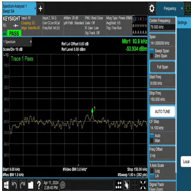
NTNV-N12-PC3-15-5-M-DFT-PI2BPSK-Edge_1RB_Right-0.009-0.15-Ant1-PASS
