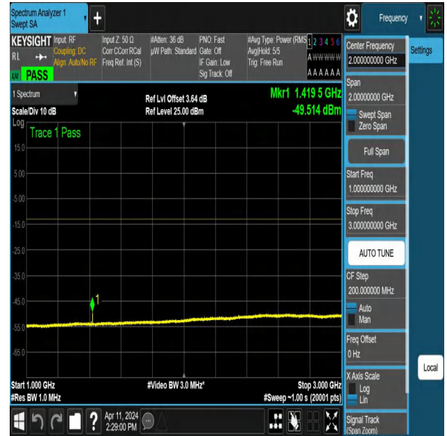
NTNV-N12-PC3-15-5-M-DFT-QPSK-Edge_1RB_Right-1000-3000- Ant1-PASS
