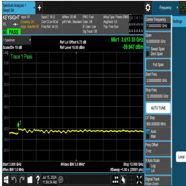
NTNV-N12-PC3-15-10-L-DFT-PI2BPSK-Edge_1RB_Left-3000-12000-Ant1-PASS
