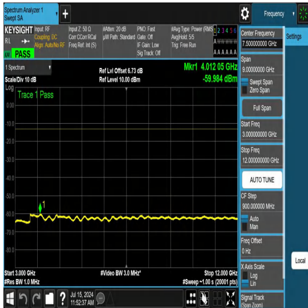
NTNV-N12-PC3-15-5-M-DFT-PI2BPSK-Edge_1RB_Right-3000-1 2000-Ant1-PASS
