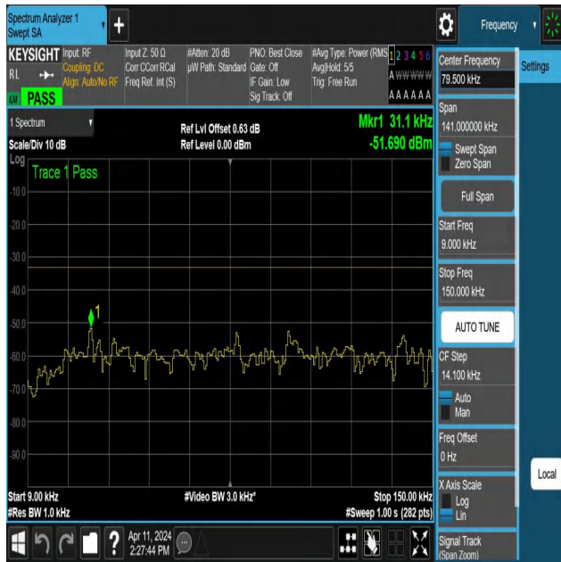
NTNV-N12-PC3-15-5-M-DFT-QPSK-Edge_1RB_Left-0.009-0.15- Ant1-PASS
