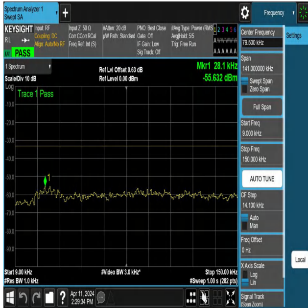
NTNV-N12-PC3-15-5-H-DFT-PI2BPSK-Edge_1RB_Left-0.009-0.15-Ant1-PASS
