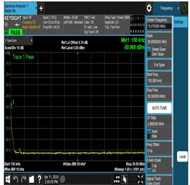
NTNV-N12-PC3-15-5-H-DFT-PI2BPSK-Edge_1RB_Right-0.15-30-Ant1-PASS
