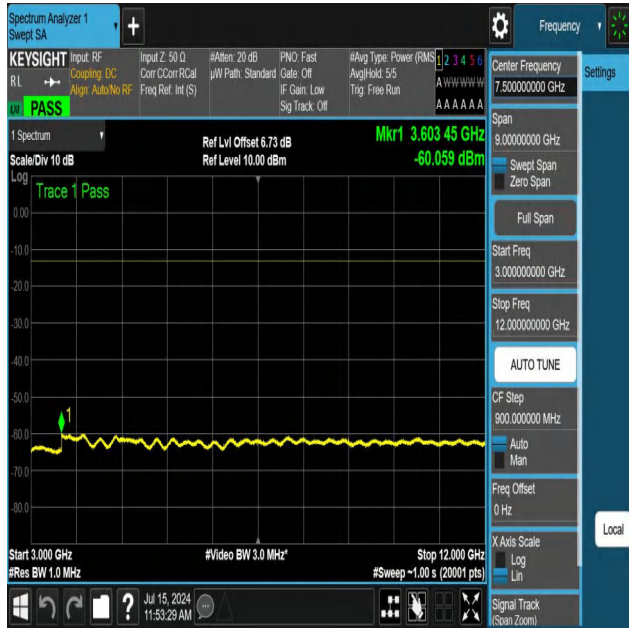
NTNV-N12-PC3-15-5-H-DFT-PI2BPSK-Edge_1RB_Left-3000-12000-Ant1-PASS
