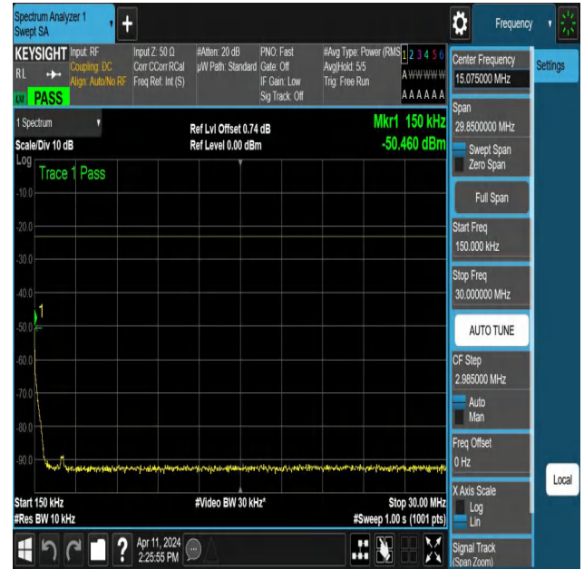
NTNV-N12-PC3-15-5-M-DFT-PI2BPSK-Edge_1RB_Left-0.15-30-Ant1-PASS
