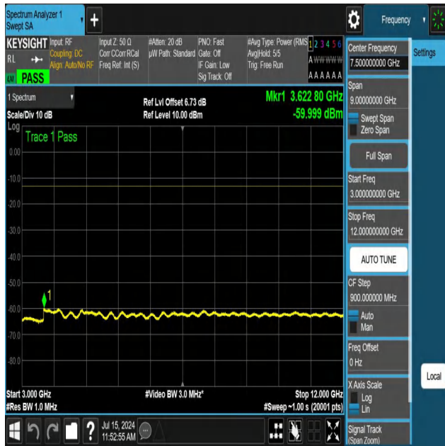
NTNV-N12-PC3-15-5-M-DFT-QPSK-Edge_1RB_Left-3000-12000 -Ant1-PASS
