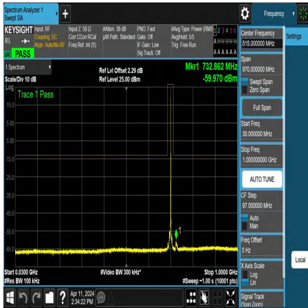
NTNV-N12-PC3-15-10-L-DFT-PI2BPSK-Edge_1RB_Right-30-10 00-Ant1-PASS
