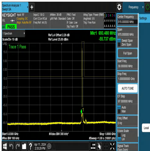
NTNV-N12-PC3-15-10-L-DFT-PI2BPSK-Edge_1RB_Left-30-1000-Ant1-PASS
