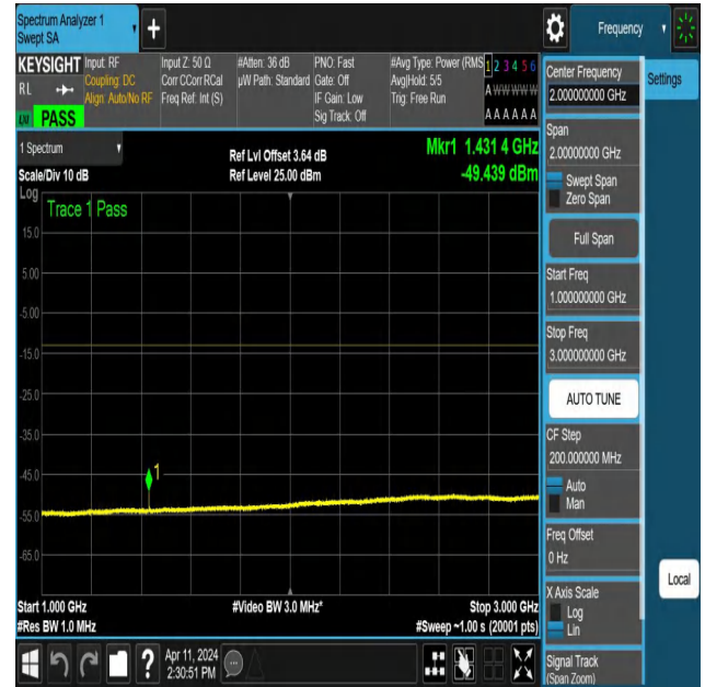
NTNV-N12-PC3-15-5-H-DFT-PI2BPSK-Edge_1RB_Right-1000-30 00-Ant1-PASS
