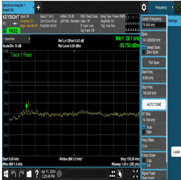
NTNV-N12-PC3-15-5-M-DFT-PI2BPSK-Edge_1RB_Left-0.009-0.15-Ant1-PASS
