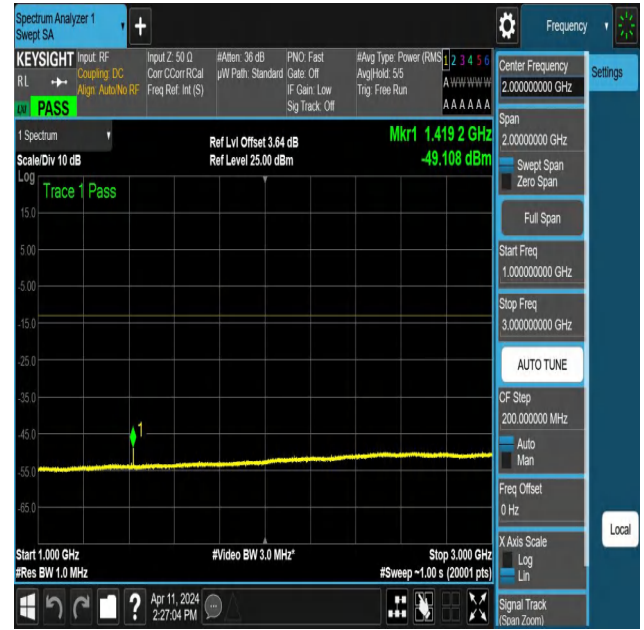
NTNV-N12-PC3-15-5-M-DFT-PI2BPSK-Edge_1RB_Right-1000-30 00-Ant1-PASS
