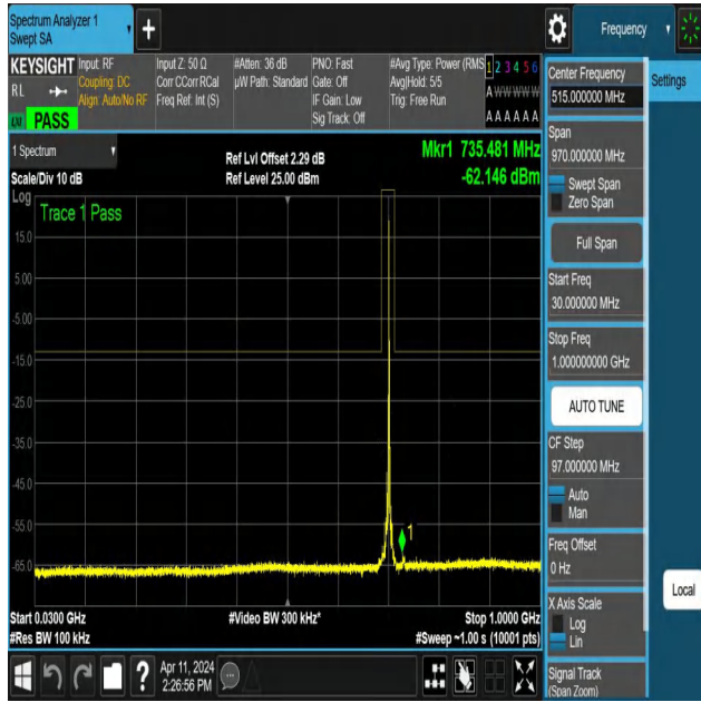
NTNV-N12-PC3-15-5-M-DFT-PI2BPSK-Edge_1RB_Right-30-100 0-Ant1-PASS
