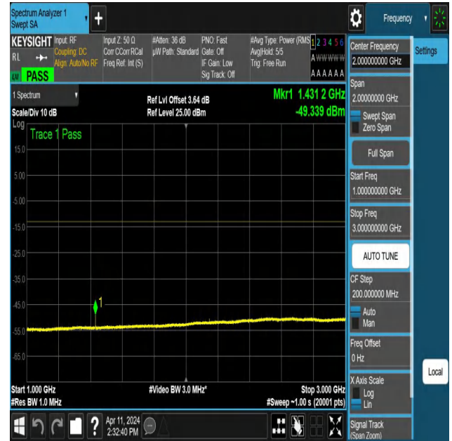
NTNV-N12-PC3-15-5-H-DFT-QPSK-Edge_1RB_Right-1000-3000- Ant1-PASS
