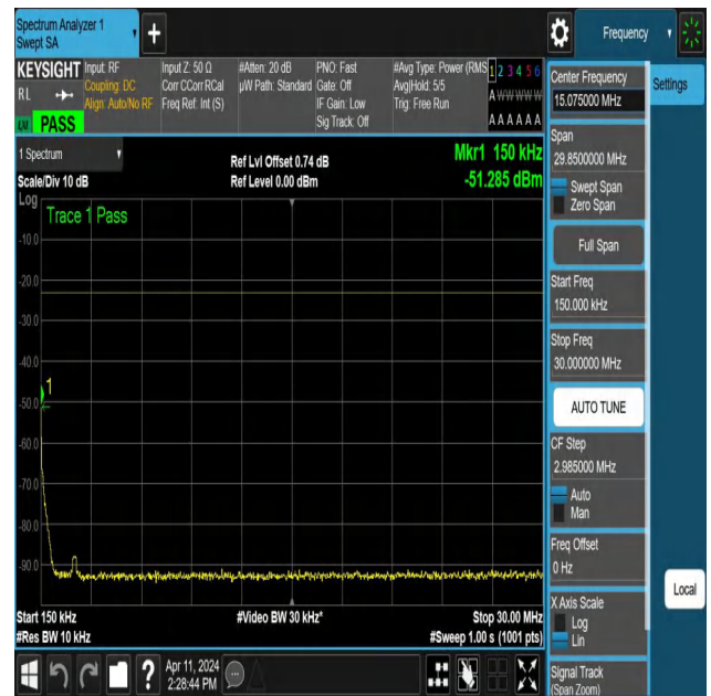
NTNV-N12-PC3-15-5-M-DFT-QPSK-Edge_1RB_Right-0.15-30-An t1-PASS
