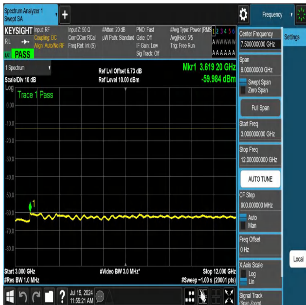
NTNV-N12-PC3-15-10-L-DFT-QPSK-Edge_1RB_Right-3000-12000-Ant1-PASS
