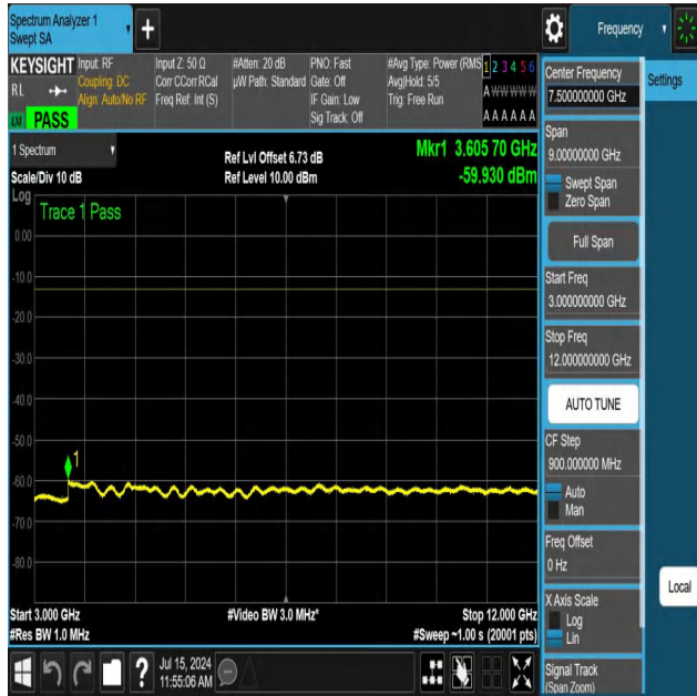
NTNV-N12-PC3-15-10-L-DFT-QPSK-Edge_1RB_Left-3000-1200 0-Ant1-PASS
