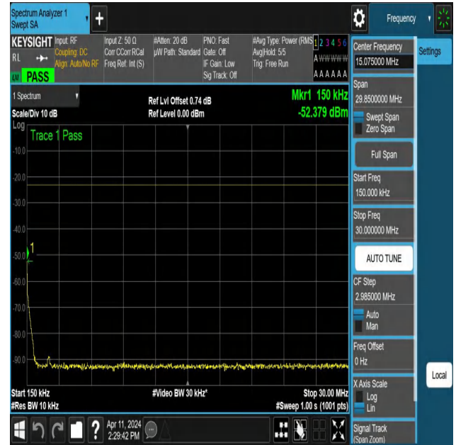
NTNV-N12-PC3-15-5-H-DFT-PI2BPSK-Edge_1RB_Left-0.15-30-Ant1-PASS
