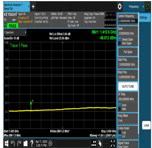
NTNV-N12-PC3-15-5-M-DFT-PI2BPSK-Edge_1RB_Left-1000-3000-Ant1-PASS
