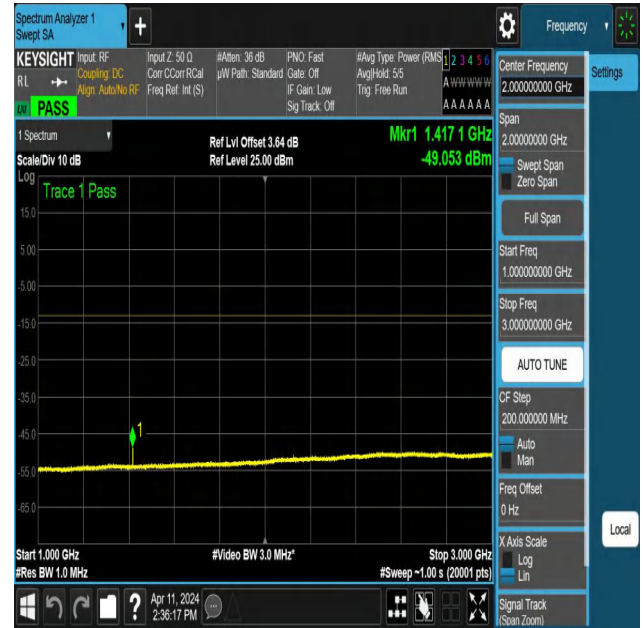
NTNV-N12-PC3-15-10-L-DFT-QPSK-Edge_1RB_Right-1000-3000-Ant1-PASS
