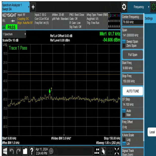
NTNV-N12-PC3-15-5-L-DFT-QPSK-Edge_1RB_Right-0.009-0.15 -Ant1-PASS
