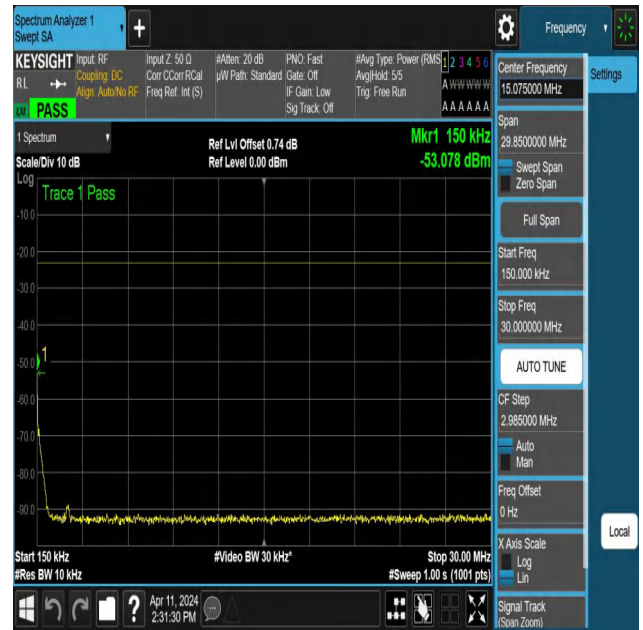
NTNV-N12-PC3-15-5-H-DFT-QPSK-Edge_1RB_Left-0.15-30-Ant1-PASS
