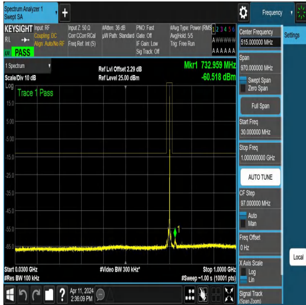
NTNV-N12-PC3-15-10-L-DFT-QPSK-Edge_1RB_Right-30-1000-Ant1-PASS
