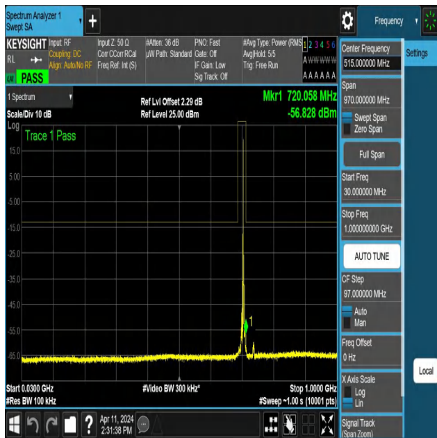
NTNV-N12-PC3-15-5-H-DFT-QPSK-Edge_1RB_Left-30-1000-Ant1-PASS
