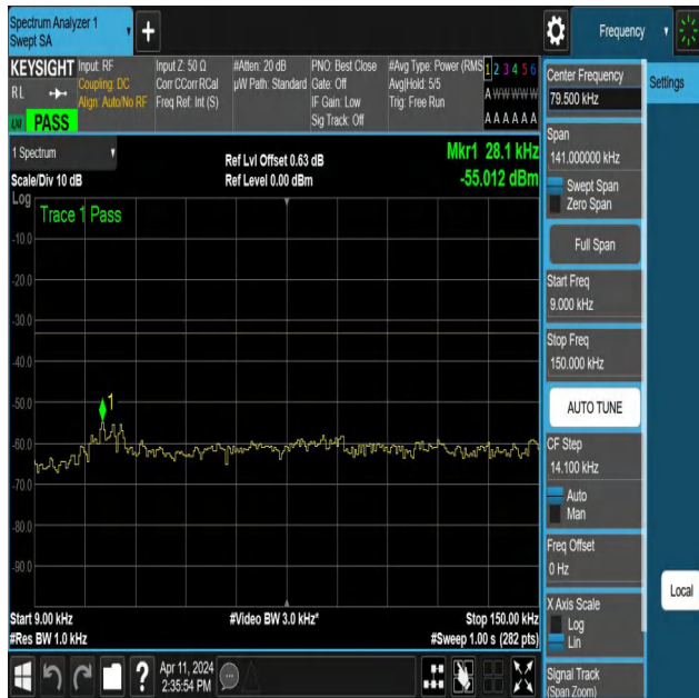
NTNV-N12-PC3-15-10-L-DFT-QPSK-Edge_1RB_Right-0.009-0.1 5-Ant1-PASS
