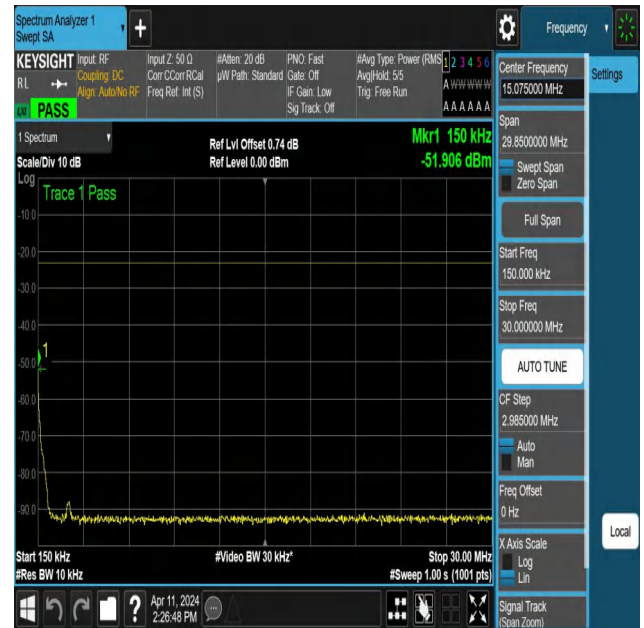
NTNV-N12-PC3-15-5-M-DFT-PI2BPSK-Edge_1RB_Right-0.15-30-Ant1-PASS
