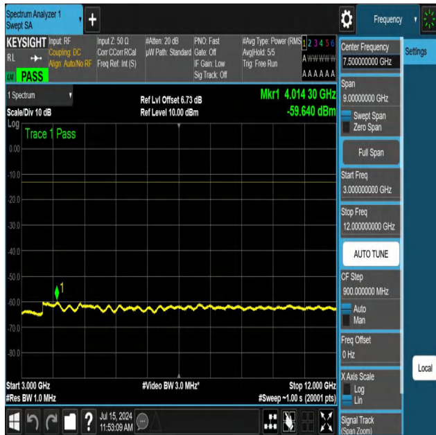
NTNV-N12-PC3-15-5-M-DFT-QPSK-Edge_1RB_Right-3000-120 00-Ant1-PASS
