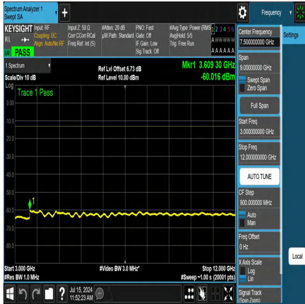
NTNV-N12-PC3-15-5-M-DFT-PI2BPSK-Edge_1RB_Left-3000-12000-Ant1-PASS
