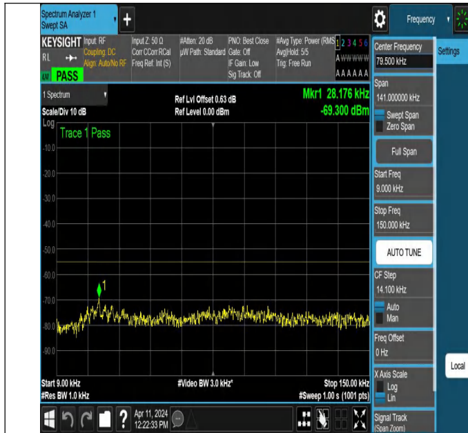
NTNV-N7-PC3-15-40-L-DFT-PI2BPSK-Edge_1RB_Left-0.009-0.1 5-Ant1-PASS
