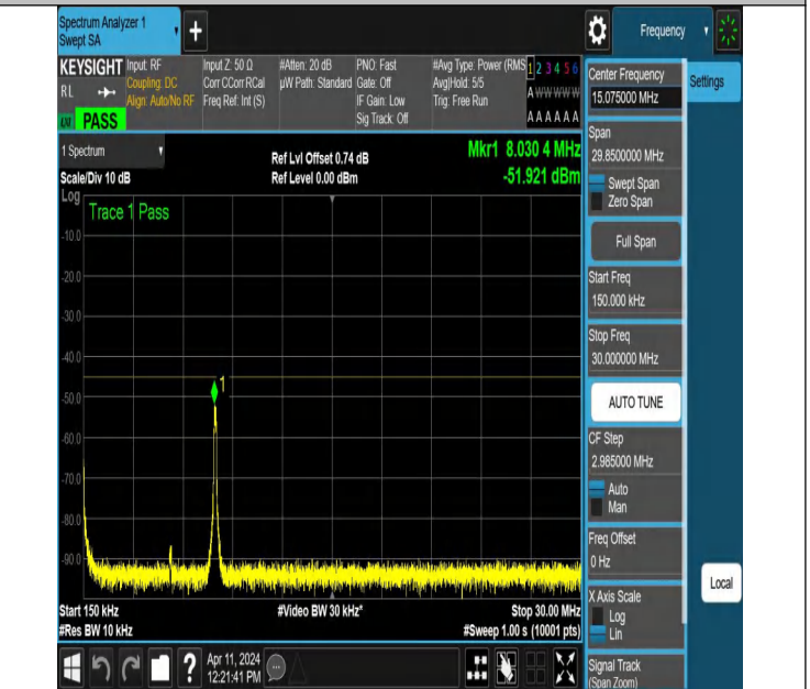
NTNV-N7-PC3-15-30-H-DFT-QPSK-Edge_1RB_Right-0.15-30-Ant 1-PASS
