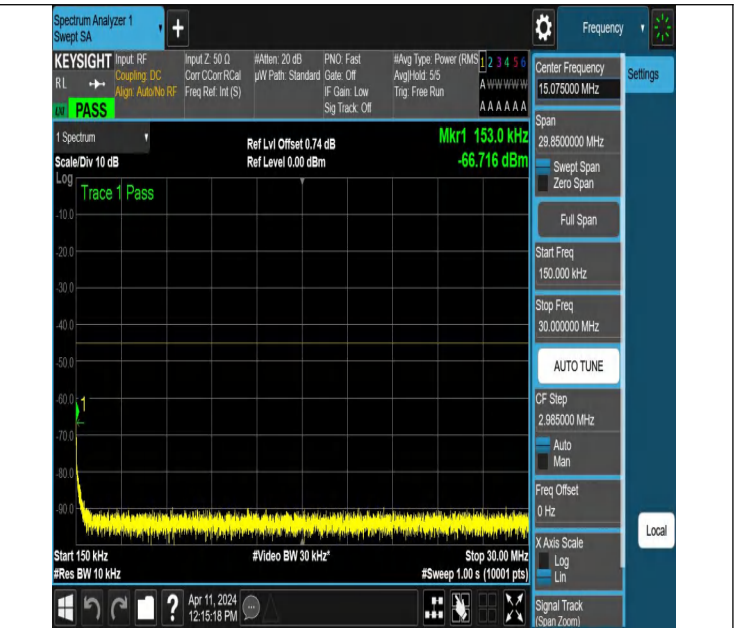
NTNV-N7-PC3-15-30-M-DFT-PI2BPSK-Edge_1RB_Left-0.15-30-Ant1-PASS
