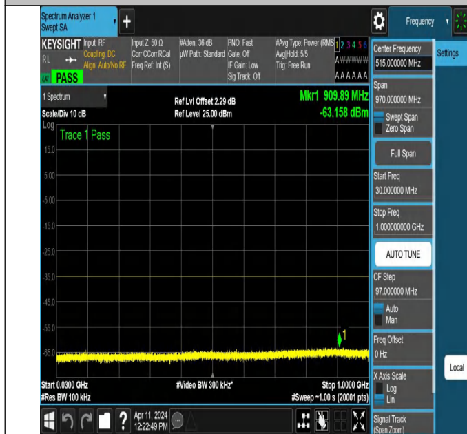
NTNV-N7-PC3-15-40-L-DFT-PI2BPSK-Edge_1RB_Left-30-1000- Ant1-PASS
