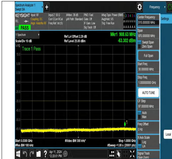
NTNV-N7-PC3-15-30-H-DFT-PI2BPSK-Edge_1RB_Right-30-100 0-Ant1-PASS
