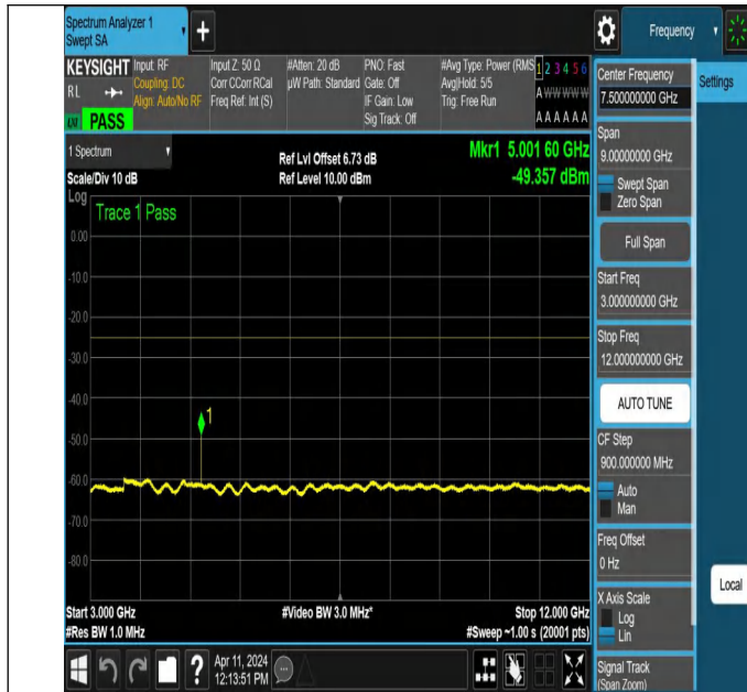
NTNV-N7-PC3-15-30-L-DFT-QPSK-Edge_1RB_Left-3000-12000-Ant1-PASS
