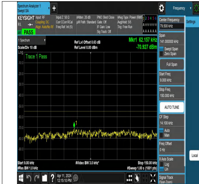
NTNV-N7-PC3-15-30-M-DFT-PI2BPSK-Edge_1RB_Left-0.009-0.15-Ant1-PASS
