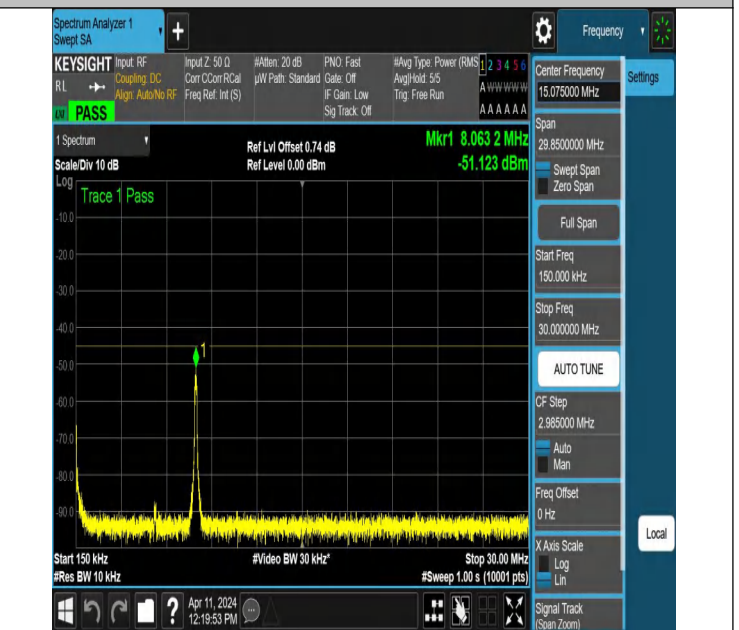
NTNV-N7-PC3-15-30-H-DFT-PI2BPSK-Edge_1RB_Right-0.15-30-Ant1-PASS
