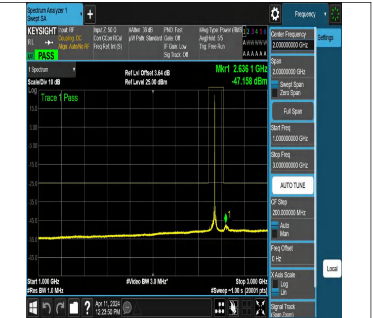
NTNV-N7-PC3-15-40-L-DFT-PI2BPSK-Edge_1RB_Right-1000-30 00-Ant1-PASS
