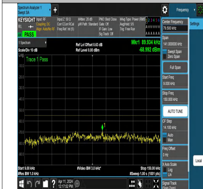
NTNV-N7-PC3-15-30-M-DFT-QPSK-Edge_1RB_Right-0.009-0.1 5-Ant1-PASS
