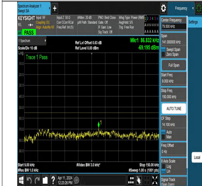
NTNV-N7-PC3-15-40-L-DFT-PI2BPSK-Edge_1RB_Right-0.009-0.15-Ant1-PASS
