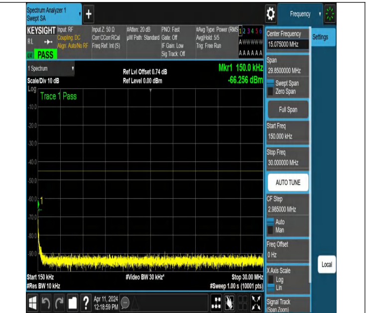
NTNV-N7-PC3-15-30-H-DFT-PI2BPSK-Edge_1RB_Left-0.15-30-Ant1-PASS
