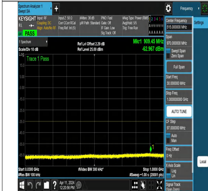
NTNV-N7-PC3-15-30-H-DFT-QPSK-Edge_1RB_Left-30-1000-Ant1-PASS
