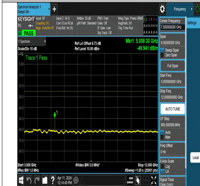
NTNV-N7-PC3-15-30-L-DFT-QPSK-Edge_1RB_Right-3000-1200 0-Ant1-PASS
