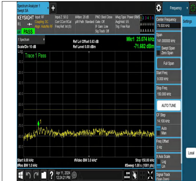
NTNV-N7-PC3-15-40-L-DFT-QPSK-Edge_1RB_Left-0.009-0.15-Ant1-PASS
