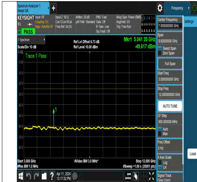
NTNV-N7-PC3-15-30-M-DFT-QPSK-Edge_1RB_Left-3000-12000 -Ant1-PASS
