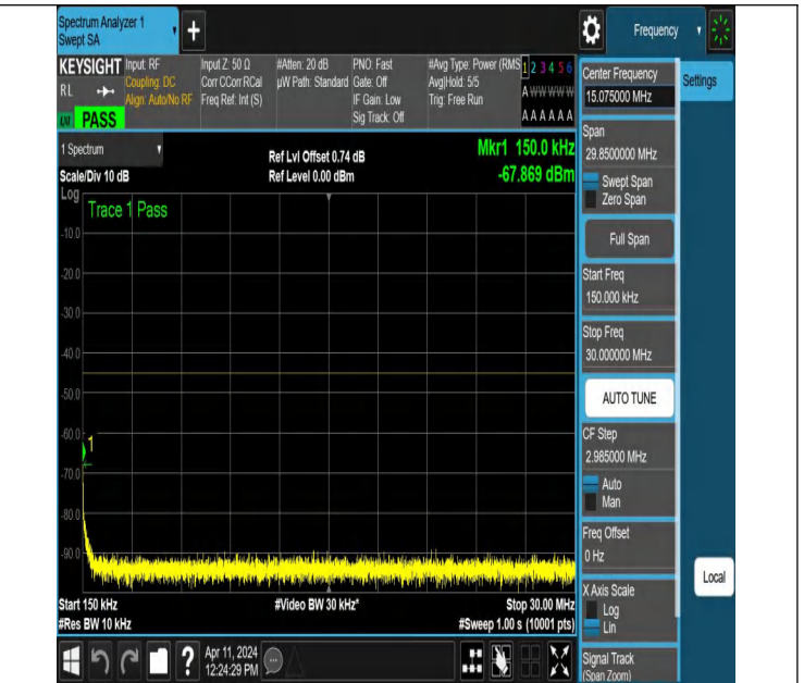
NTNV-N7-PC3-15-40-L-DFT-QPSK-Edge_1RB_Left-0.15-30-Ant1-PASS
