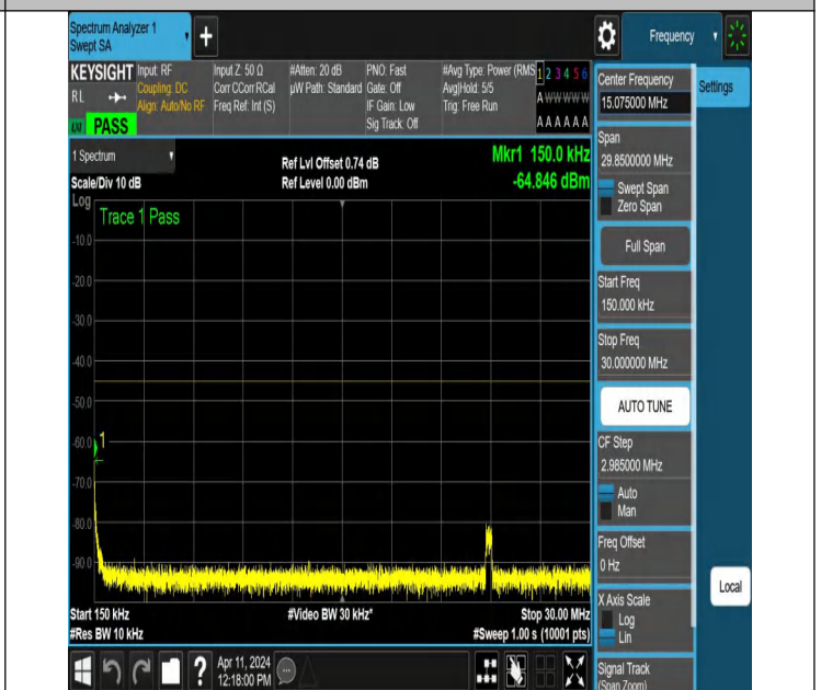
NTNV-N7-PC3-15-30-M-DFT-QPSK-Edge_1RB_Right-0.15-30-An t1-PASS
