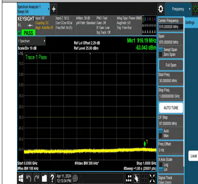
NTNV-N7-PC3-15-30-L-DFT-QPSK-Edge_1RB_Left-30-1000-Ant1-PASS
