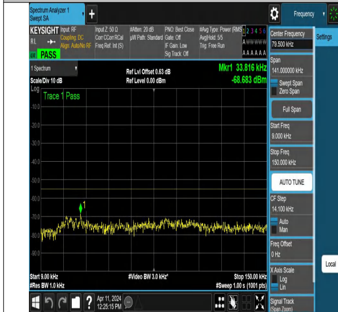
NTNV-N7-PC3-15-40-L-DFT-QPSK-Edge_1RB_Right-0.009-0.15 -Ant1-PASS
