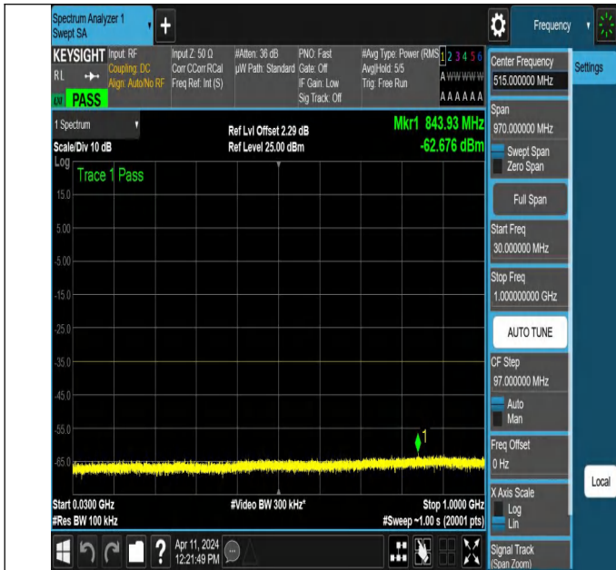
NTNV-N7-PC3-15-30-H-DFT-QPSK-Edge_1RB_Right-30-1000-A nt1-PASS
