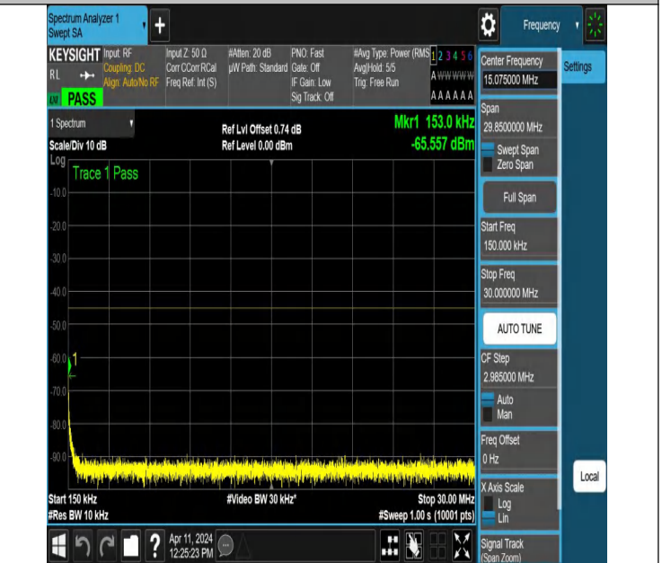
NTNV-N7-PC3-15-40-L-DFT-QPSK-Edge_1RB_Right-0.15-30-Ant 1-PASS
