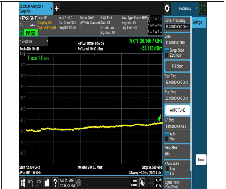
NTNV-N7-PC3-15-30-M-DFT-QPSK-Edge_1RB_Left-12000-2650 0-Ant1-PASS
