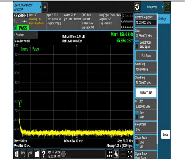
NTNV-N7-PC3-15-40-L-DFT-PI2BPSK-Edge_1RB_Right-0.15-30-Ant1-PASS
