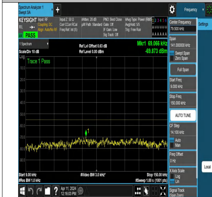
NTNV-N7-PC3-15-30-M-DFT-PI2BPSK-Edge_1RB_Right-0.009-0.15-Ant1-PASS
