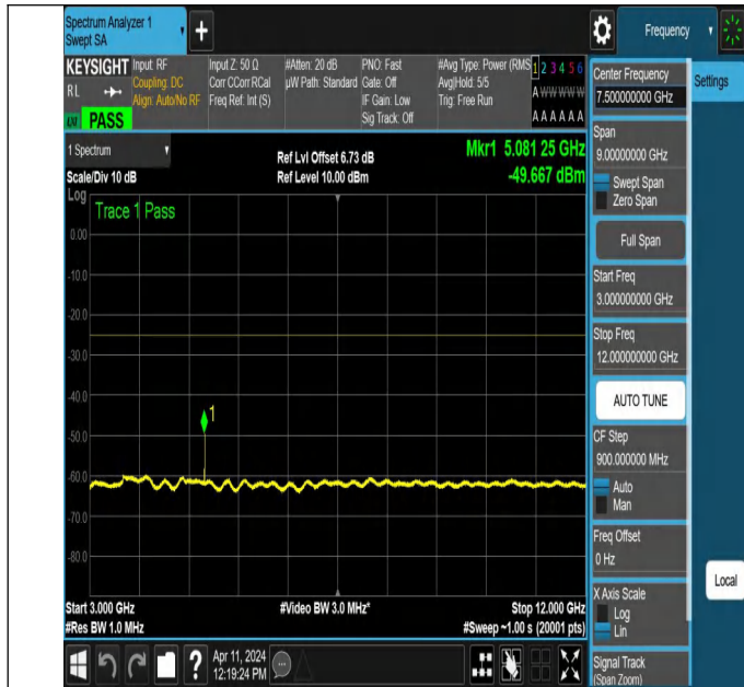
NTNV-N7-PC3-15-30-H-DFT-PI2BPSK-Edge_1RB_Left-3000-12000-Ant1-PASS
