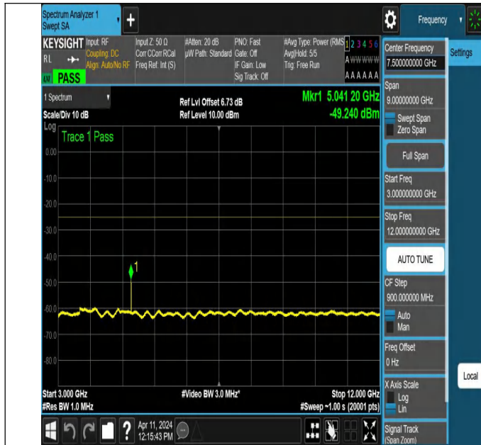
NTNV-N7-PC3-15-30-M-DFT-PI2BPSK-Edge_1RB_Left-3000-12000-Ant1-PASS
