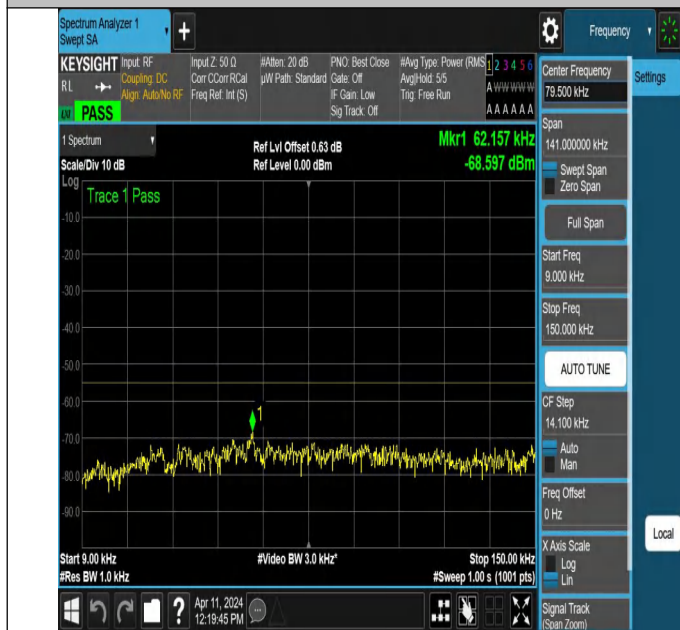
NTNV-N7-PC3-15-30-H-DFT-PI2BPSK-Edge_1RB_Right-0.009-0.15-Ant1-PASS
