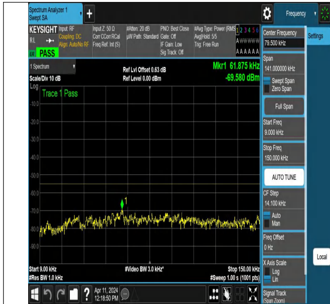
NTNV-N7-PC3-15-30-H-DFT-PI2BPSK-Edge_1RB_Left-0.009-0.15-Ant1-PASS
