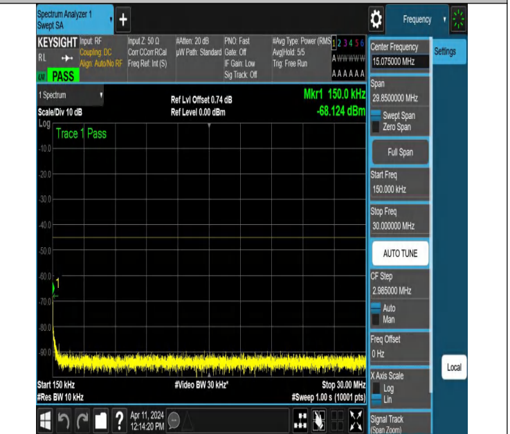
NTNV-N7-PC3-15-30-L-DFT-QPSK-Edge_1RB_Right-0.15-30-Ant1-PASS
