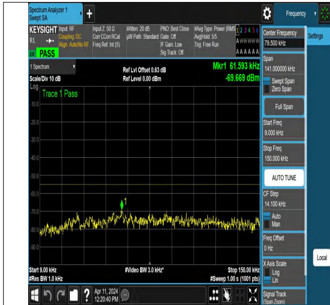
NTNV-N7-PC3-15-30-H-DFT-QPSK-Edge_1RB_Left-0.009-0.15-Ant1-PASS
