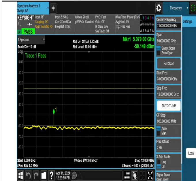
NTNV-N7-PC3-15-40-L-DFT-PI2BPSK-Edge_1RB_Right-3000-1 2000-Ant1-PASS
