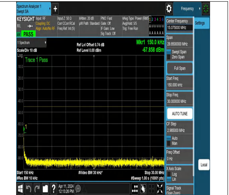
NTNV-N7-PC3-15-30-L-DFT-QPSK-Edge_1RB_Left-0.15-30-Ant1-PASS
