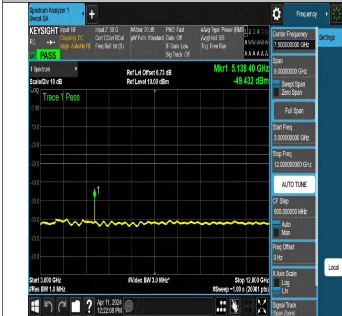
NTNV-N7-PC3-15-30-H-DFT-QPSK-Edge_1RB_Right-3000-1200 0-Ant1-PASS
