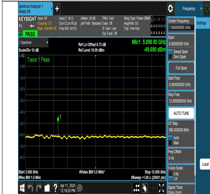
NTNV-N7-PC3-15-30-M-DFT-QPSK-Edge_1RB_Right-3000-120 00-Ant1-PASS
