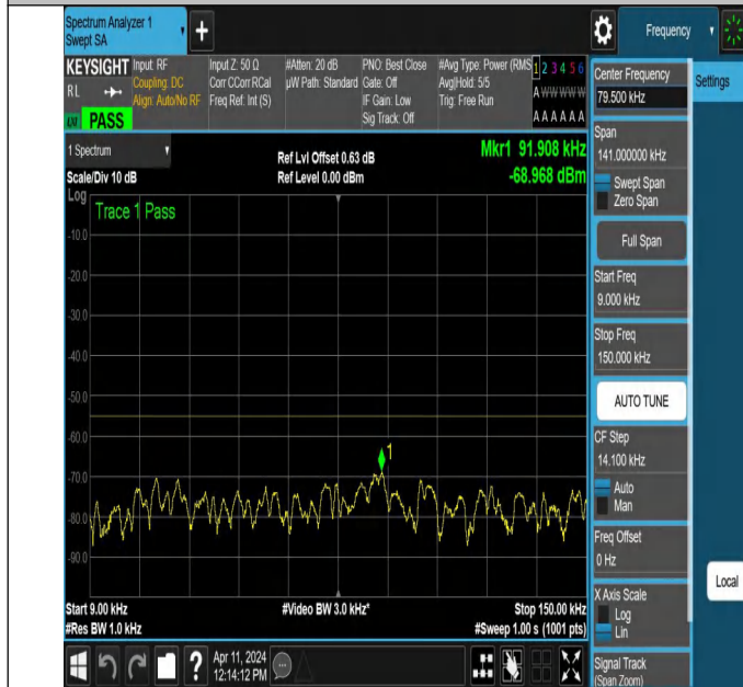
NTNV-N7-PC3-15-30-L-DFT-QPSK-Edge_1RB_Right-0.009-0.15-Ant1-PASS
