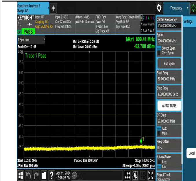
NTNV-N7-PC3-15-30-M-DFT-PI2BPSK-Edge_1RB_Left-30-1000-Ant1-PASS
