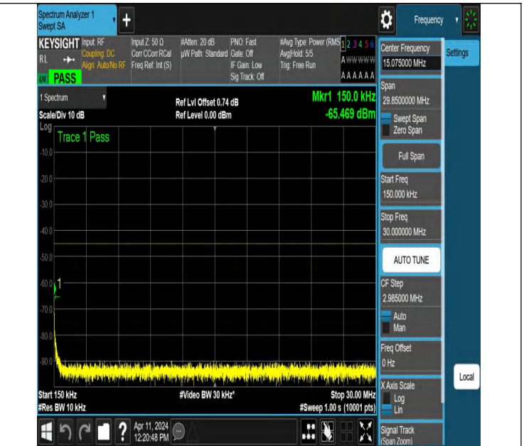
NTNV-N7-PC3-15-30-H-DFT-QPSK-Edge_1RB_Left-0.15-30-Ant1-PASS
