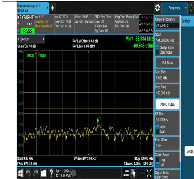
NTNV-N7-PC3-15-30-L-DFT-QPSK-Edge_1RB_Left-0.009-0.15-Ant1-PASS
