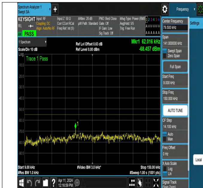
NTNV-N7-PC3-15-30-M-DFT-QPSK-Edge_1RB_Left-0.009-0.15- Ant1-PASS
