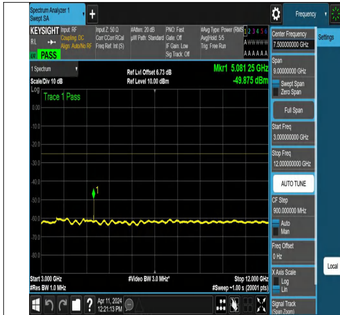
NTNV-N7-PC3-15-30-H-DFT-QPSK-Edge_1RB_Left-3000-12000 -Ant1-PASS
