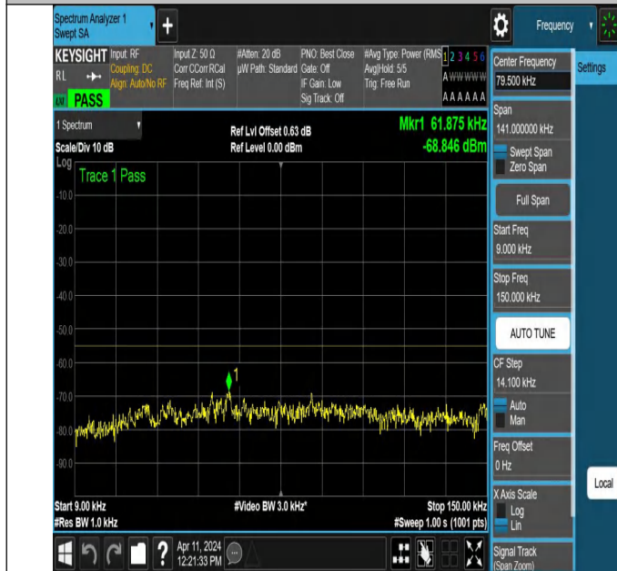
NTNV-N7-PC3-15-30-H-DFT-QPSK-Edge_1RB_Right-0.009-0.15 -Ant1-PASS
