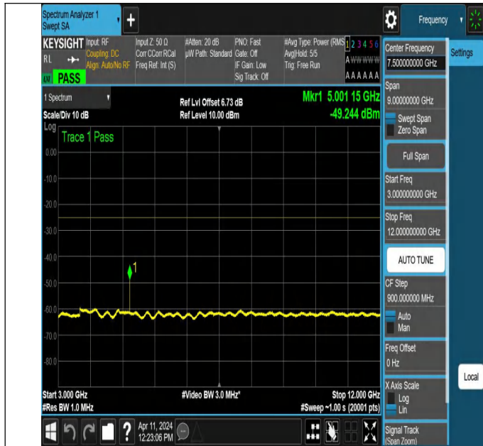
NTNV-N7-PC3-15-40-L-DFT-PI2BPSK-Edge_1RB_Left-3000-12000-Ant1-PASS
