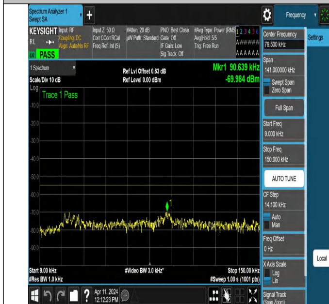
NTNV-N7-PC3-15-30-L-DFT-PI2BPSK-Edge_1RB_Right-0.009-0 .15-Ant1-PASS
