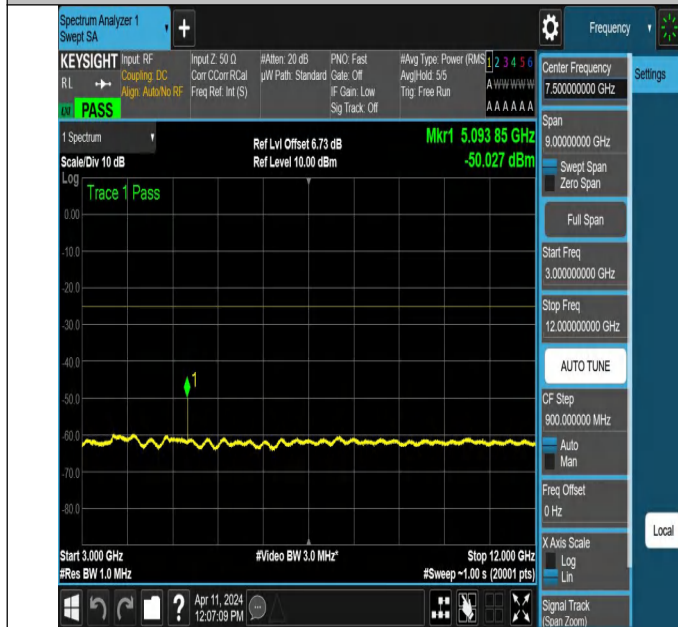
NTNV-N7-PC3-15-25-M-DFT-QPSK-Edge_1RB_Right-3000-120 00-Ant1-PASS
