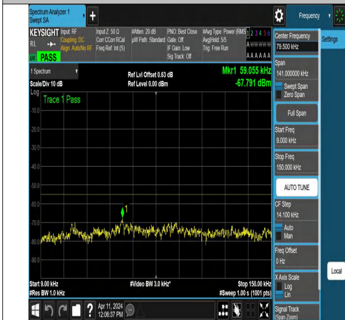
NTNV-N7-PC3-15-25-M-DFT-QPSK-Edge_1RB_Right-0.009-0.1 5-Ant1-PASS
