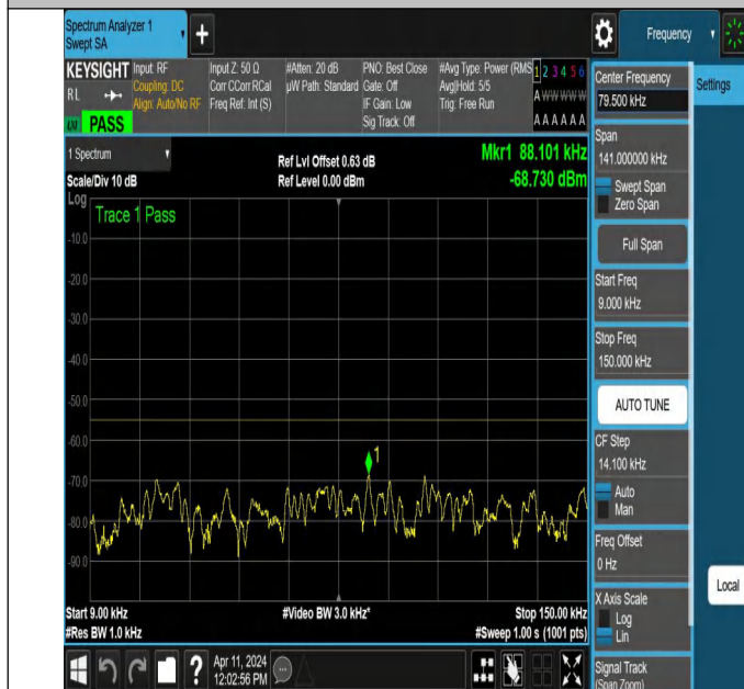
NTNV-N7-PC3-15-25-L-DFT-QPSK-Edge_1RB_Right-0.009-0.15-Ant1-PASS
