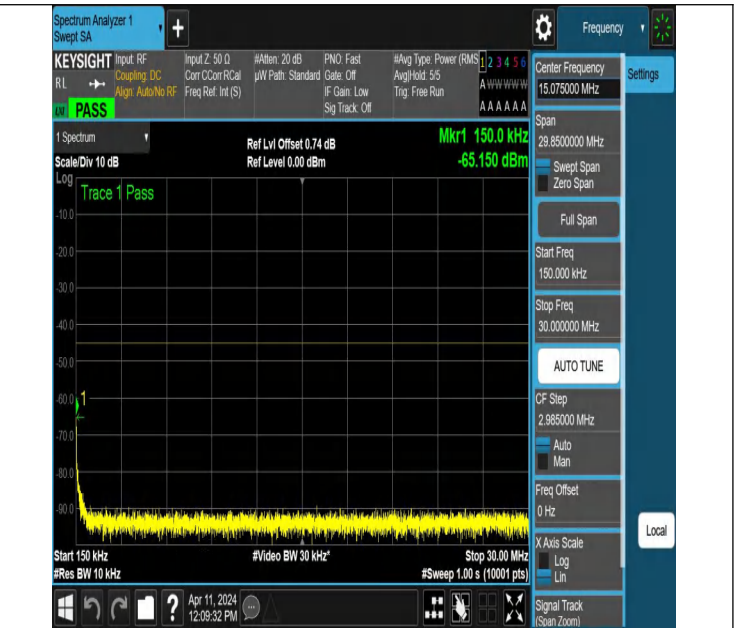
NTNV-N7-PC3-15-25-H-DFT-QPSK-Edge_1RB_Left-0.15-30-Ant1-PASS
