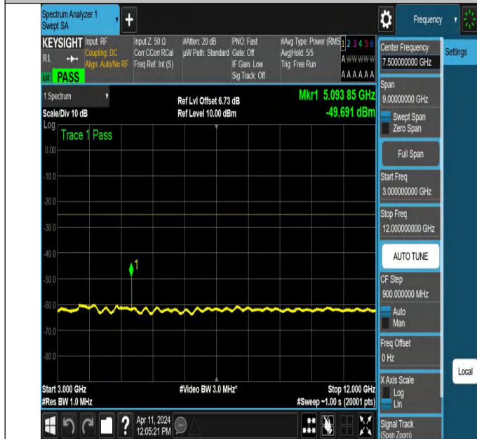
NTNV-N7-PC3-15-25-M-DFT-PI2BPSK-Edge_1RB_Right-3000-1 2000-Ant1-PASS
