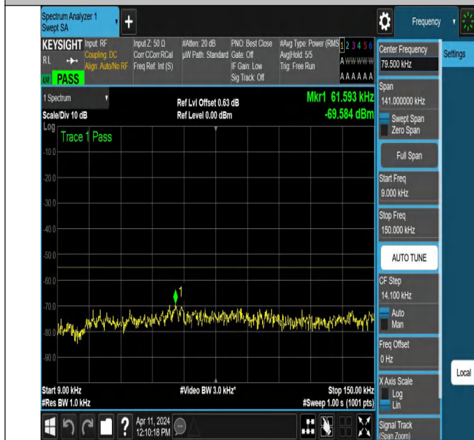
NTNV-N7-PC3-15-25-H-DFT-QPSK-Edge_1RB_Right-0.009-0.15 -Ant1-PASS
