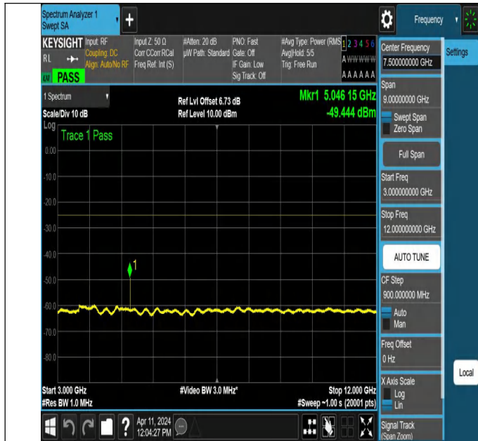
NTNV-N7-PC3-15-25-M-DFT-PI2BPSK-Edge_1RB_Left-3000-12000-Ant1-PASS
