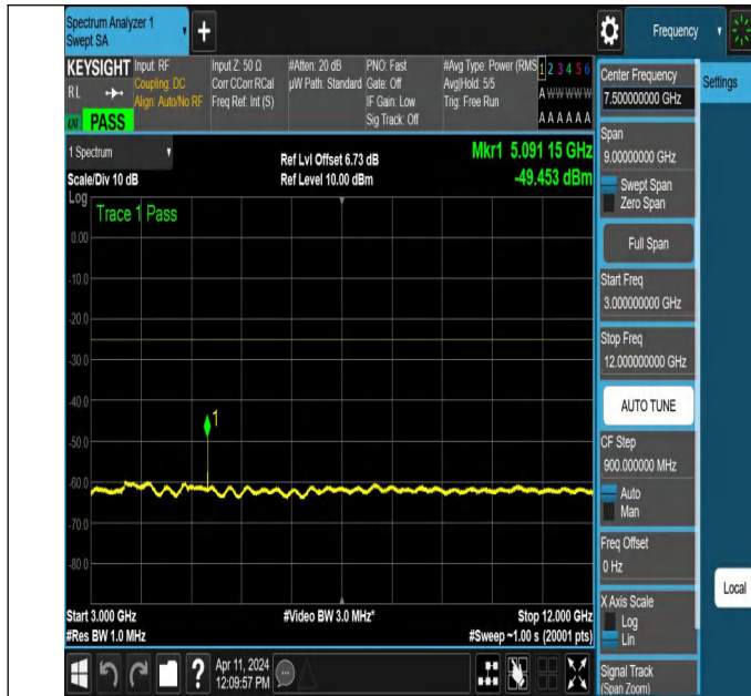
NTNV-N7-PC3-15-25-H-DFT-QPSK-Edge_1RB_Left-3000-12000 -Ant1-PASS
