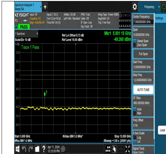
NTNV-N7-PC3-15-30-L-DFT-PI2BPSK-Edge_1RB_Left-3000-120 00-Ant1-PASS
