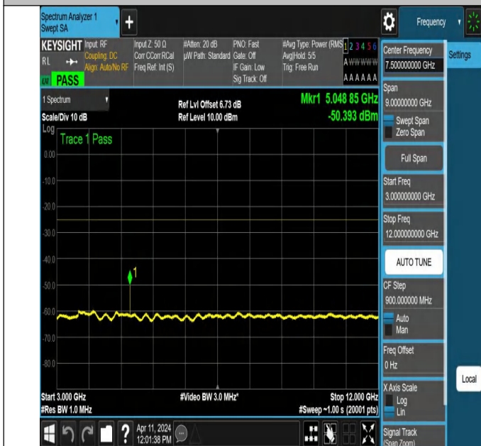
NTNV-N7-PC3-15-25-L-DFT-PI2BPSK-Edge_1RB_Right-3000-1 2000-Ant1-PASS
