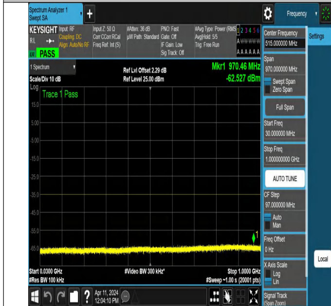
NTNV-N7-PC3-15-25-M-DFT-PI2BPSK-Edge_1RB_Left-30-1000-Ant1-PASS
