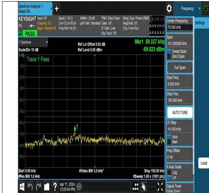
NTNV-N7-PC3-15-25-M-DFT-PI2BPSK-Edge_1RB_Left-0.009-0.15-Ant1-PASS
