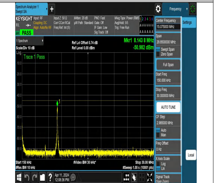
NTNV-N7-PC3-15-25-H-DFT-PI2BPSK-Edge_1RB_Right-0.15-30-Ant1-PASS
