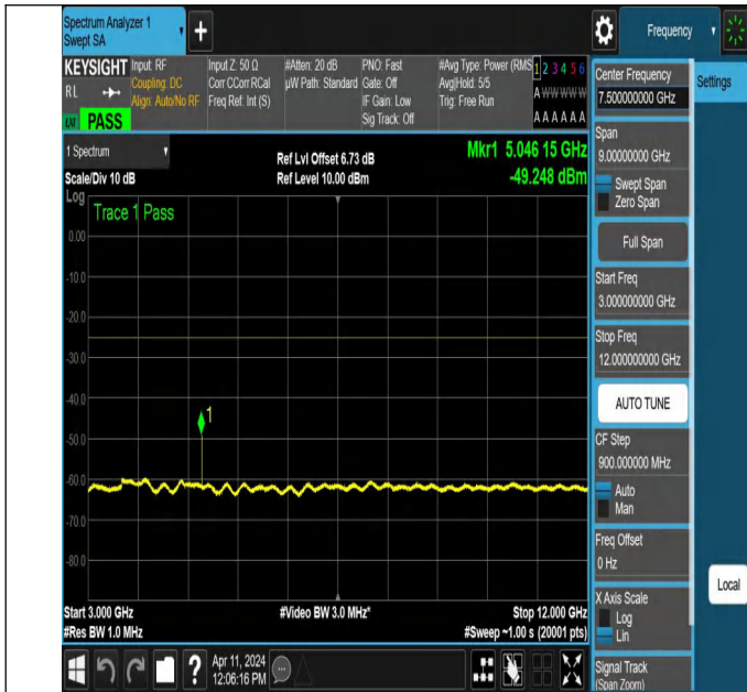
NTNV-N7-PC3-15-25-M-DFT-QPSK-Edge_1RB_Left-3000-12000 -Ant1-PASS
