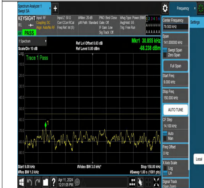
NTNV-N7-PC3-15-25-L-DFT-PI2BPSK-Edge_1RB_Right-0.009-0.15-Ant1-PASS
