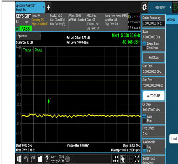
NTNV-N7-PC3-15-30-L-DFT-PI2BPSK-Edge_1RB_Right-3000-1 2000-Ant1-PASS
