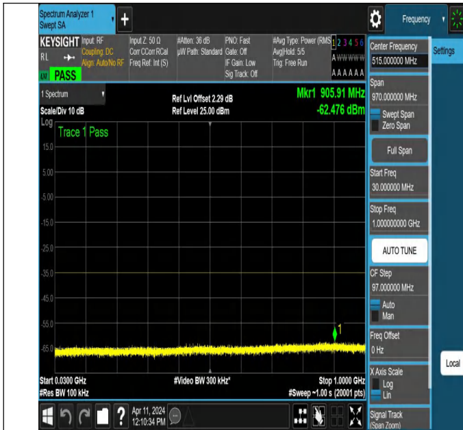
NTNV-N7-PC3-15-25-H-DFT-QPSK-Edge_1RB_Right-30-1000-A nt1-PASS
