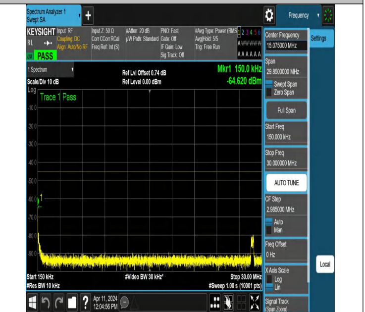
NTNV-N7-PC3-15-25-M-DFT-PI2BPSK-Edge_1RB_Right-0.15-30-Ant1-PASS
