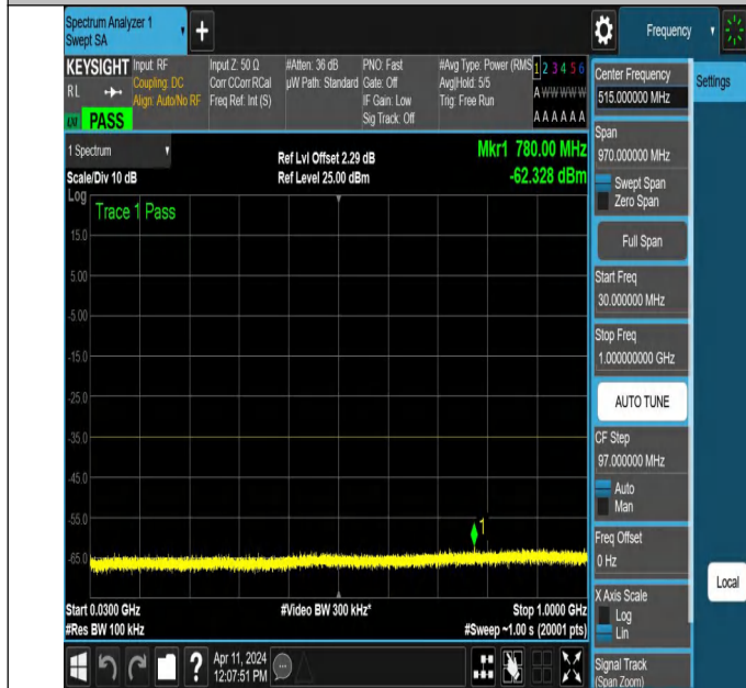
NTNV-N7-PC3-15-25-H-DFT-PI2BPSK-Edge_1RB_Left-30-1000-Ant1-PASS
