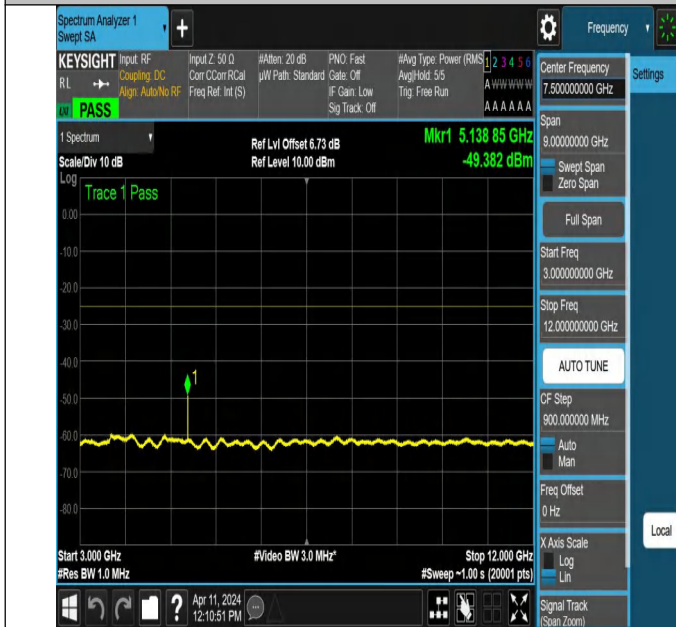
NTNV-N7-PC3-15-25-H-DFT-QPSK-Edge_1RB_Right-3000-1200 0-Ant1-PASS
