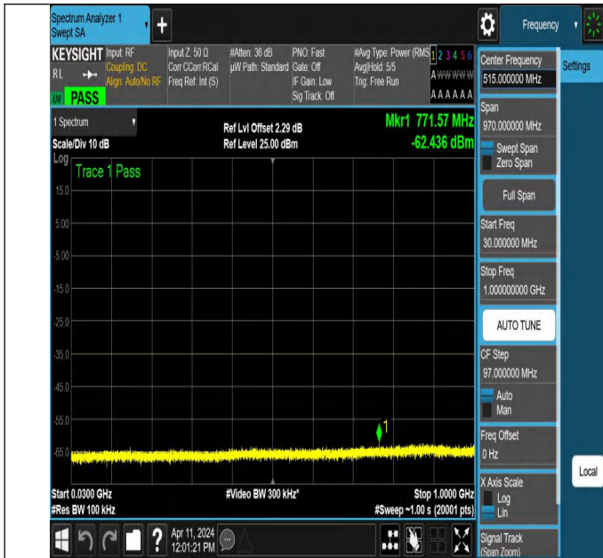
NTNV-N7-PC3-15-25-L-DFT-PI2BPSK-Edge_1RB_Right-30-100 0-Ant1-PASS
