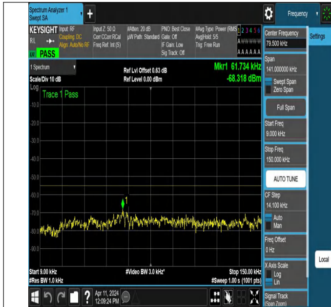
NTNV-N7-PC3-15-25-H-DFT-QPSK-Edge_1RB_Left-0.009-0.15-Ant1-PASS
