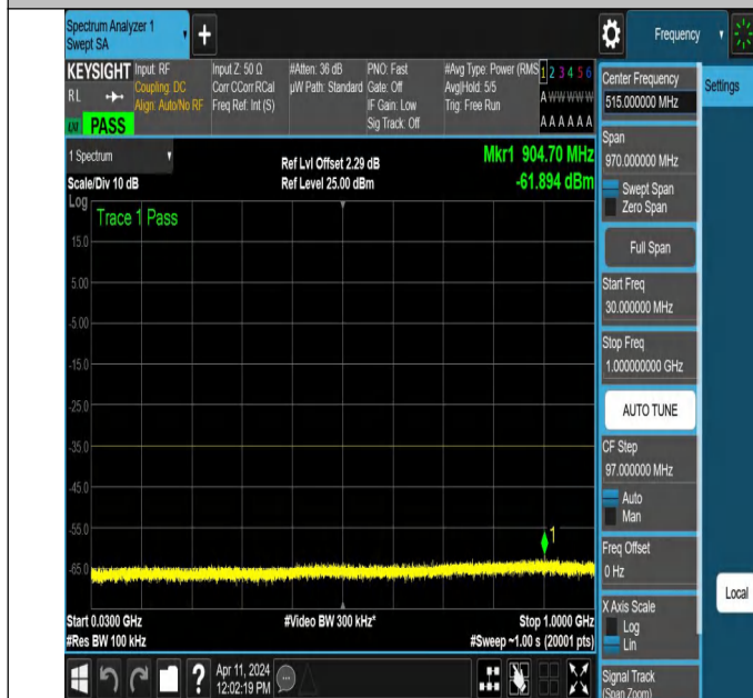
NTNV-N7-PC3-15-25-L-DFT-QPSK-Edge_1RB_Left-30-1000-Ant1-PASS
