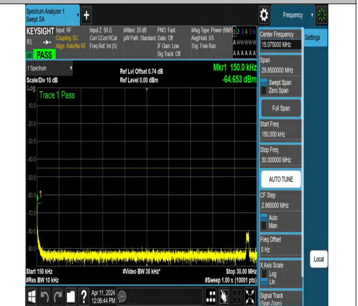
NTNV-N7-PC3-15-25-M-DFT-QPSK-Edge_1RB_Right-0.15-30-An t1-PASS
