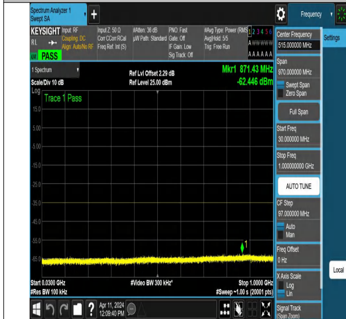
NTNV-N7-PC3-15-25-H-DFT-QPSK-Edge_1RB_Left-30-1000-Ant1-PASS
