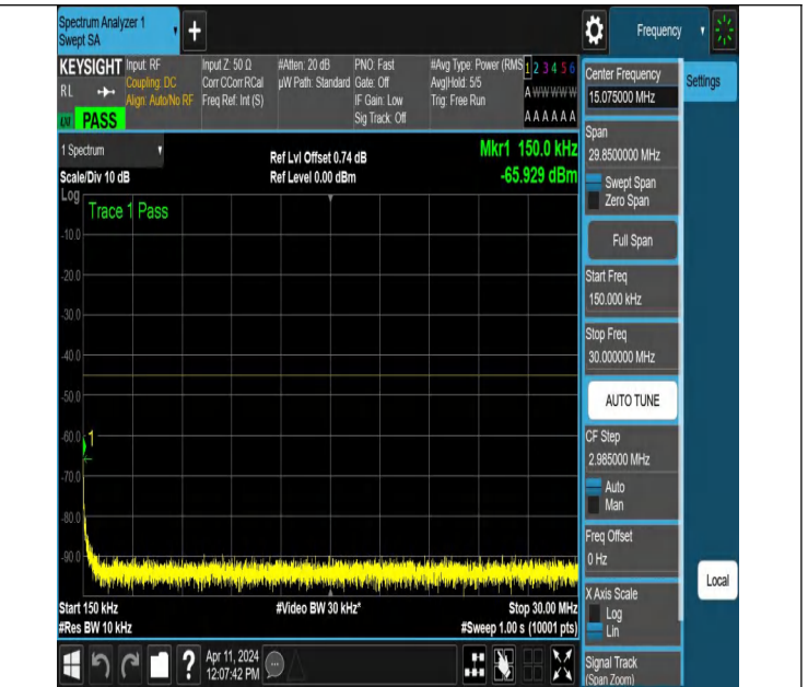
NTNV-N7-PC3-15-25-H-DFT-PI2BPSK-Edge_1RB_Left-0.15-30-Ant1-PASS
