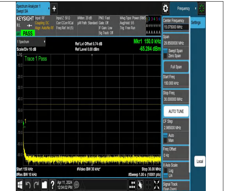
NTNV-N7-PC3-15-25-M-DFT-PI2BPSK-Edge_1RB_Left-0.15-30-Ant1-PASS
