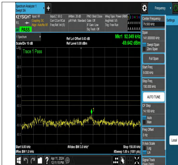
NTNV-N7-PC3-15-30-L-DFT-PI2BPSK-Edge_1RB_Left-0.009-0.1 5-Ant1-PASS
