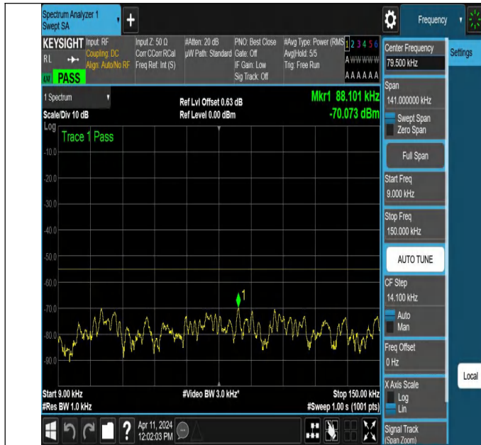
NTNV-N7-PC3-15-25-L-DFT-QPSK-Edge_1RB_Left-0.009-0.15-Ant1-PASS
