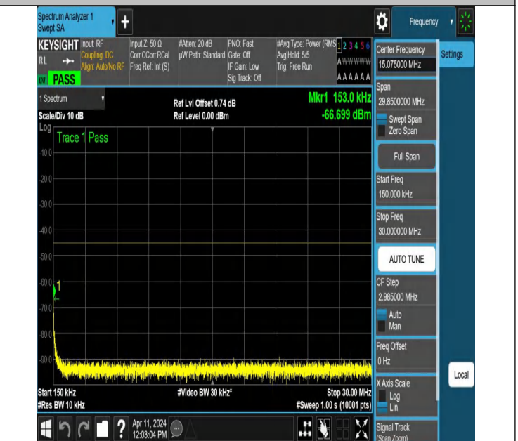
NTNV-N7-PC3-15-25-L-DFT-QPSK-Edge_1RB_Right-0.15-30-Ant1-PASS
