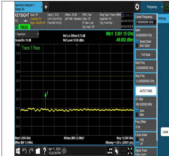
NTNV-N7-PC3-15-25-L-DFT-QPSK-Edge_1RB_Left-3000-12000-Ant1-PASS
