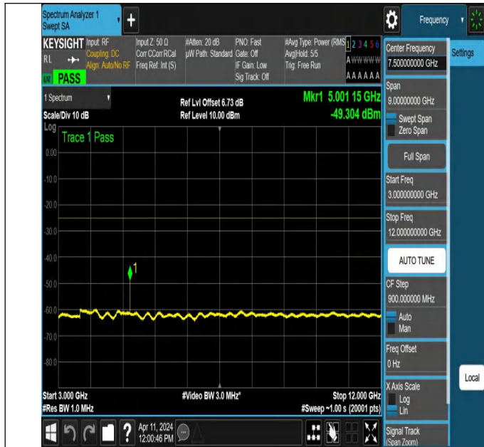
NTNV-N7-PC3-15-25-L-DFT-PI2BPSK-Edge_1RB_Left-3000-12000-Ant1-PASS
