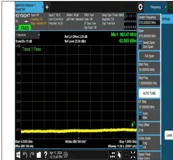
NTNV-N7-PC3-15-30-L-DFT-PI2BPSK-Edge_1RB_Right-30-100 0-Ant1-PASS
