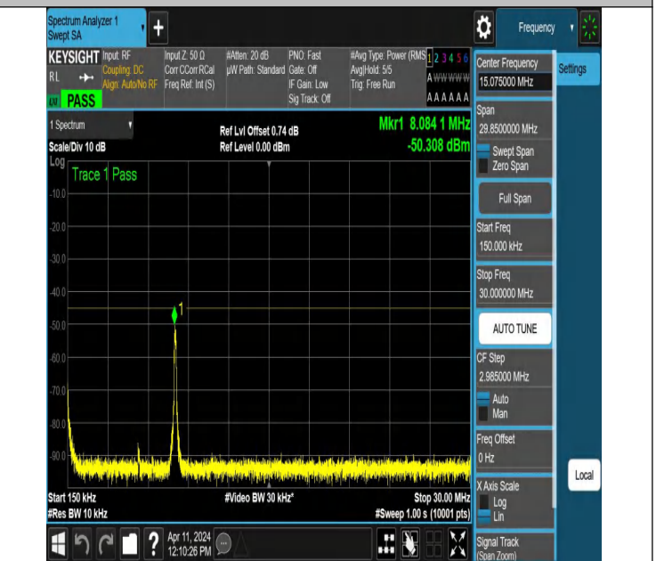
NTNV-N7-PC3-15-25-H-DFT-QPSK-Edge_1RB_Right-0.15-30-Ant 1-PASS
