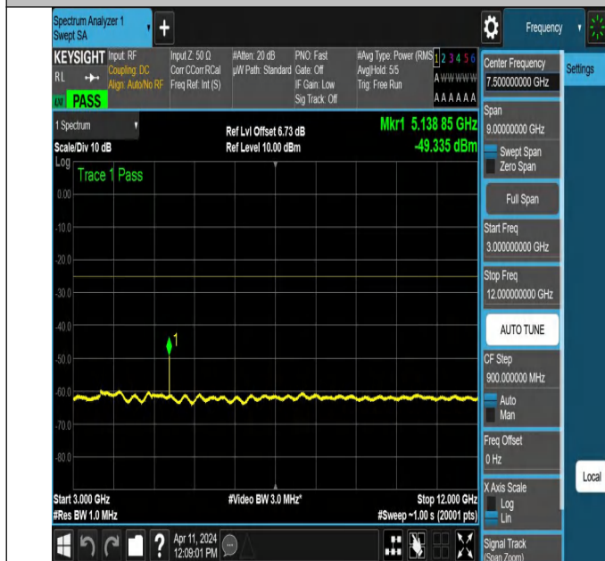
NTNV-N7-PC3-15-25-H-DFT-PI2BPSK-Edge_1RB_Right-3000-1 2000-Ant1-PASS
