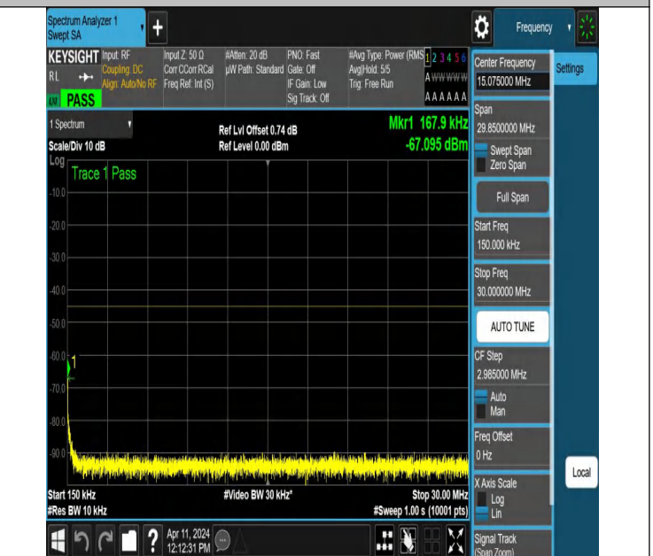
NTNV-N7-PC3-15-30-L-DFT-PI2BPSK-Edge_1RB_Right-0.15-30- Ant1-PASS
