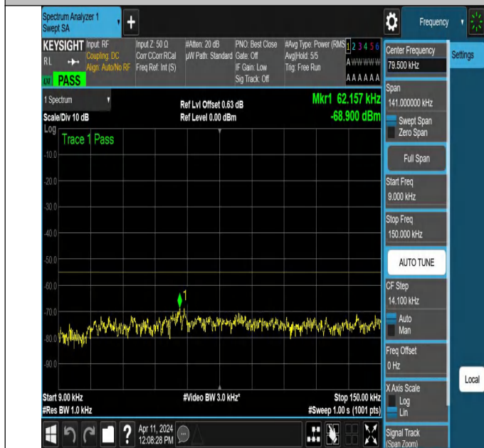
NTNV-N7-PC3-15-25-H-DFT-PI2BPSK-Edge_1RB_Right-0.009-0.15-Ant1-PASS
