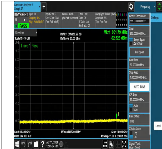
NTNV-N7-PC3-15-25-M-DFT-PI2BPSK-Edge_1RB_Right-30-100 0-Ant1-PASS
