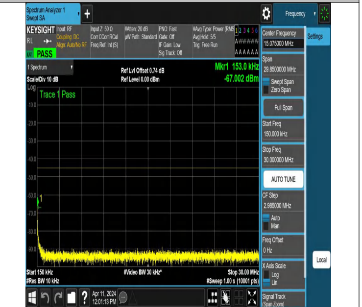
NTNV-N7-PC3-15-25-L-DFT-PI2BPSK-Edge_1RB_Right-0.15-30-Ant1-PASS
