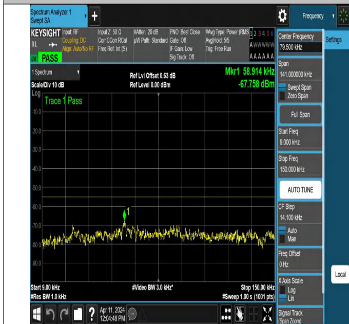
NTNV-N7-PC3-15-25-M-DFT-PI2BPSK-Edge_1RB_Right-0.009-0.15-Ant1-PASS
