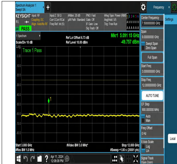
NTNV-N7-PC3-15-25-H-DFT-PI2BPSK-Edge_1RB_Left-3000-12000-Ant1-PASS
