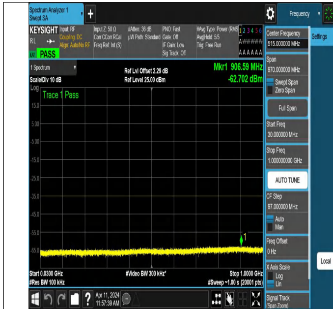
NTNV-N7-PC3-15-20-H-DFT-PI2BPSK-Edge_1RB_Right-30-100 0-Ant1-PASS
