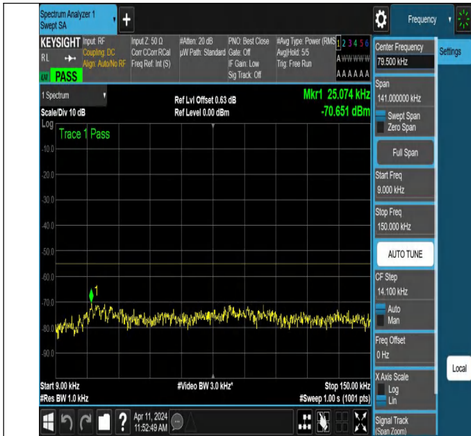
NTNV-N7-PC3-15-20-M-DFT-PI2BPSK-Edge_1RB_Left-0.009-0.15-Ant1-PASS
