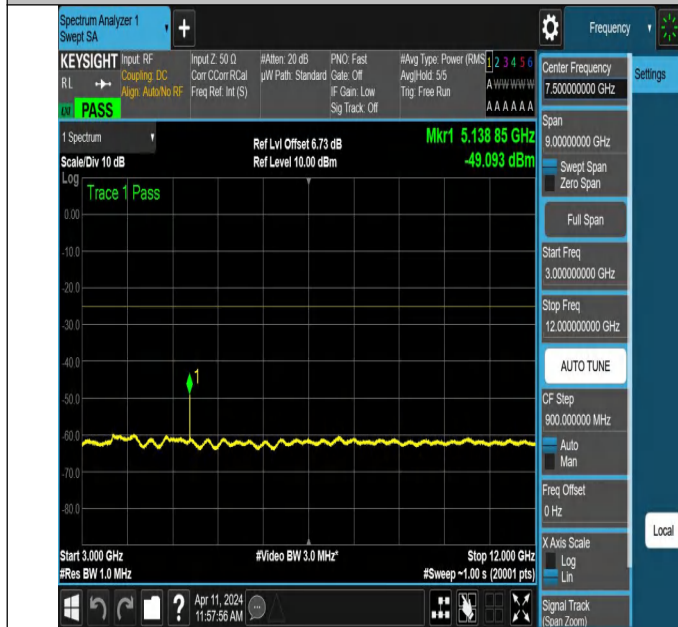
NTNV-N7-PC3-15-20-H-DFT-PI2BPSK-Edge_1RB_Right-3000-1 2000-Ant1-PASS
