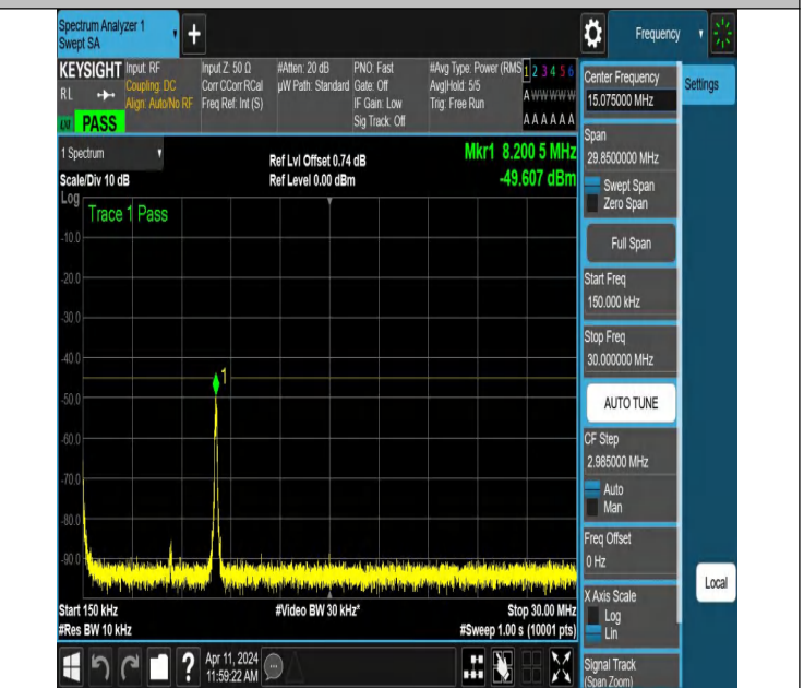
NTNV-N7-PC3-15-20-H-DFT-QPSK-Edge_1RB_Right-0.15-30-Ant 1-PASS
