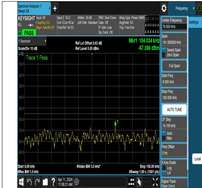
NTNV-N7-PC3-15-20-H-DFT-QPSK-Edge_1RB_Left-0.009-0.15-Ant1-PASS
