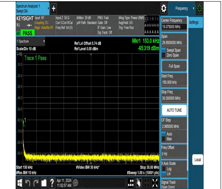
NTNV-N7-PC3-15-20-M-DFT-PI2BPSK-Edge_1RB_Left-0.15-30-Ant1-PASS
