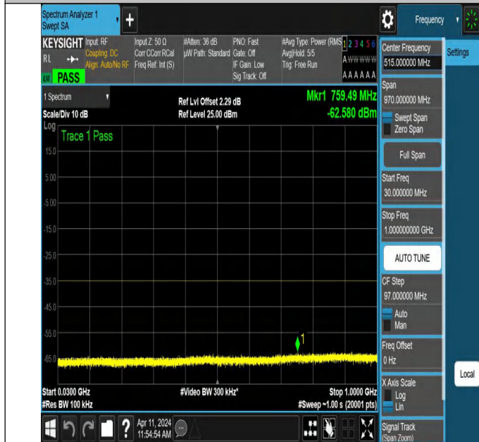
NTNV-N7-PC3-15-20-M-DFT-QPSK-Edge_1RB_Left-30-1000-Ant1-PASS
