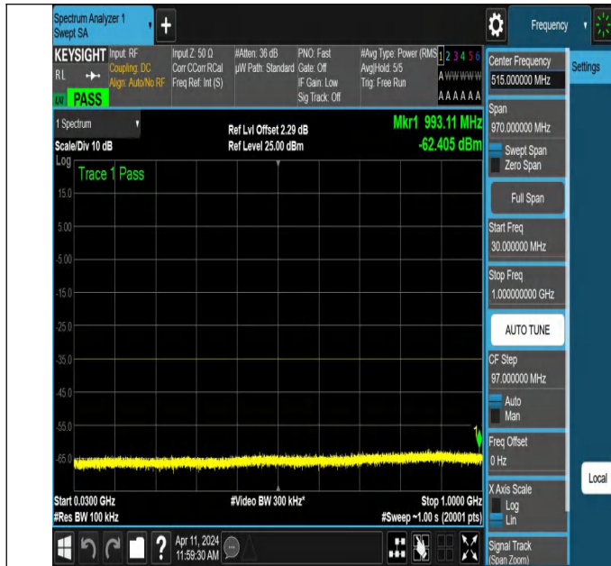
NTNV-N7-PC3-15-20-H-DFT-QPSK-Edge_1RB_Right-30-1000-A nt1-PASS
