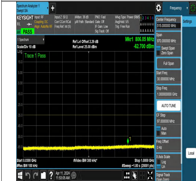
NTNV-N7-PC3-15-20-M-DFT-PI2BPSK-Edge_1RB_Left-30-1000-Ant1-PASS
