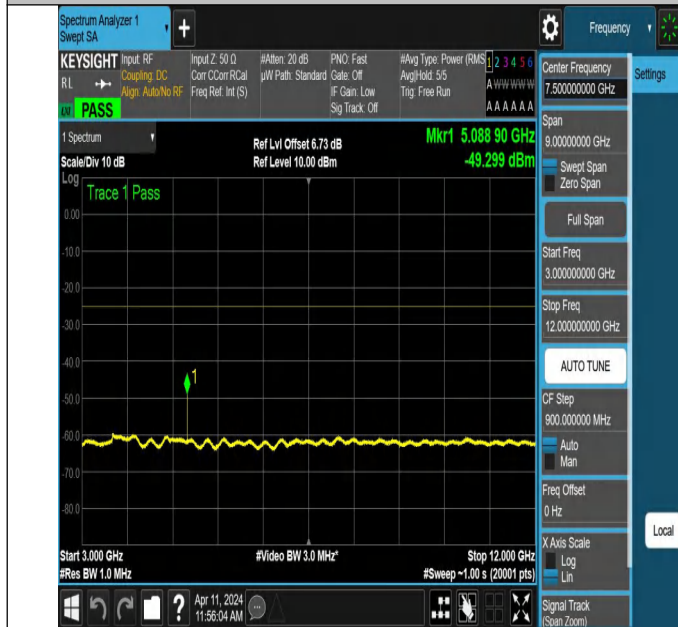
NTNV-N7-PC3-15-20-M-DFT-QPSK-Edge_1RB_Right-3000-12000-Ant1-PASS
