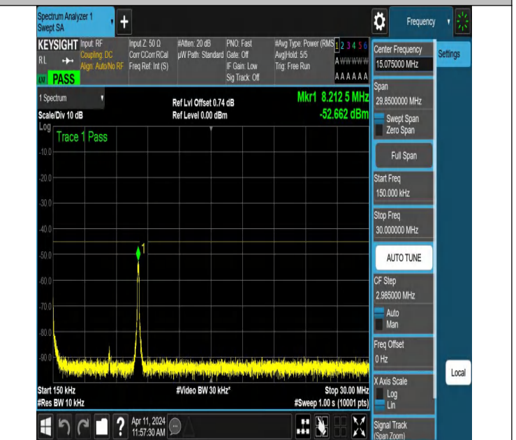
NTNV-N7-PC3-15-20-H-DFT-PI2BPSK-Edge_1RB_Right-0.15-30-Ant1-PASS
