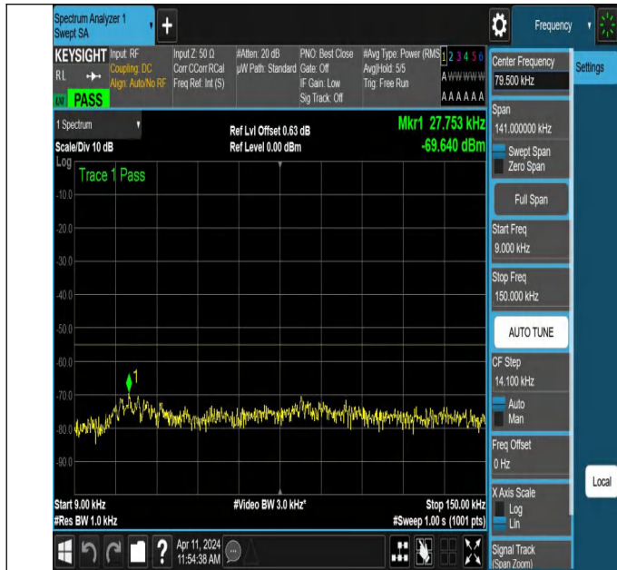
NTNV-N7-PC3-15-20-M-DFT-QPSK-Edge_1RB_Left-0.009-0.15-Ant1-PASS
