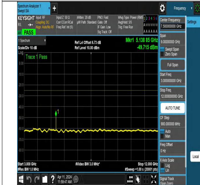
NTNV-N7-PC3-15-20-H-DFT-QPSK-Edge_1RB_Right-3000-12000 0-Ant1-PASS
