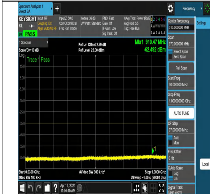
NTNV-N7-PC3-15-20-H-DFT-PI2BPSK-Edge_1RB_Left-30-1000-Ant1-PASS
