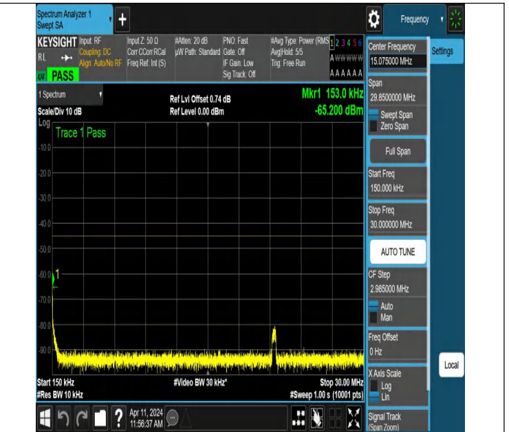
NTNV-N7-PC3-15-20-H-DFT-PI2BPSK-Edge_1RB_Left-0.15-30-Ant1-PASS
