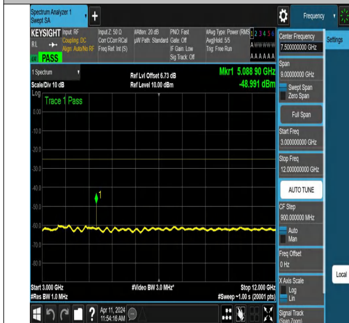
NTNV-N7-PC3-15-20-M-DFT-PI2BPSK-Edge_1RB_Right-3000-1 2000-Ant1-PASS
