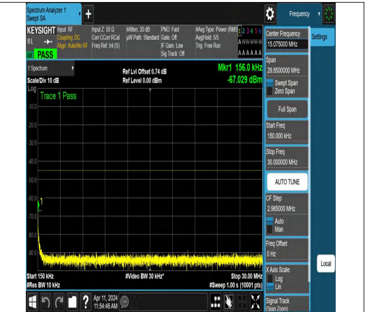
NTNV-N7-PC3-15-20-M-DFT-QPSK-Edge_1RB_Left-0.15-30-Ant1-PASS
