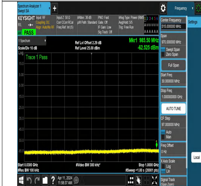
NTNV-N7-PC3-15-20-H-DFT-QPSK-Edge_1RB_Left-30-1000-Ant1-PASS
