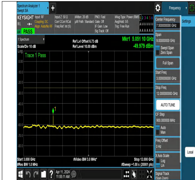
NTNV-N7-PC3-15-20-M-DFT-QPSK-Edge_1RB_Left-3000-12000 -Ant1-PASS
