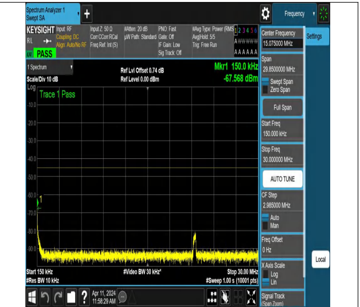
NTNV-N7-PC3-15-20-H-DFT-QPSK-Edge_1RB_Left-0.15-30-Ant1-PASS
