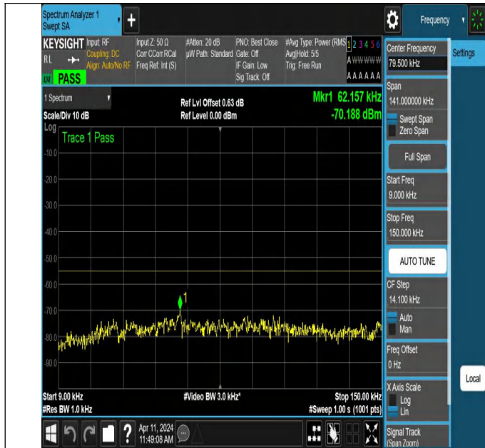
NTNV-N7-PC3-15-20-L-DFT-PI2BPSK-Edge_1RB_Left-0.009-0.1 5-Ant1-PASS
