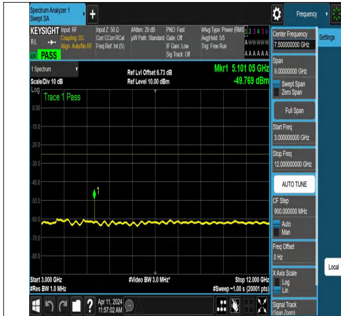
NTNV-N7-PC3-15-20-H-DFT-PI2BPSK-Edge_1RB_Left-3000-12000-Ant1-PASS
