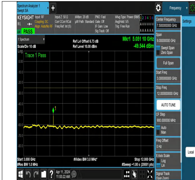
NTNV-N7-PC3-15-20-M-DFT-PI2BPSK-Edge_1RB_Left-3000-12000-Ant1-PASS
