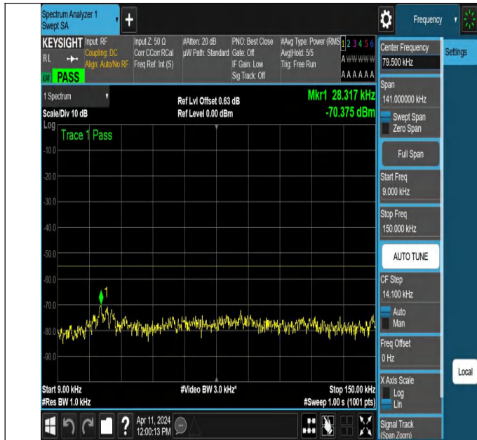
NTNV-N7-PC3-15-25-L-DFT-PI2BPSK-Edge_1RB_Left-0.009-0.1 5-Ant1-PASS
