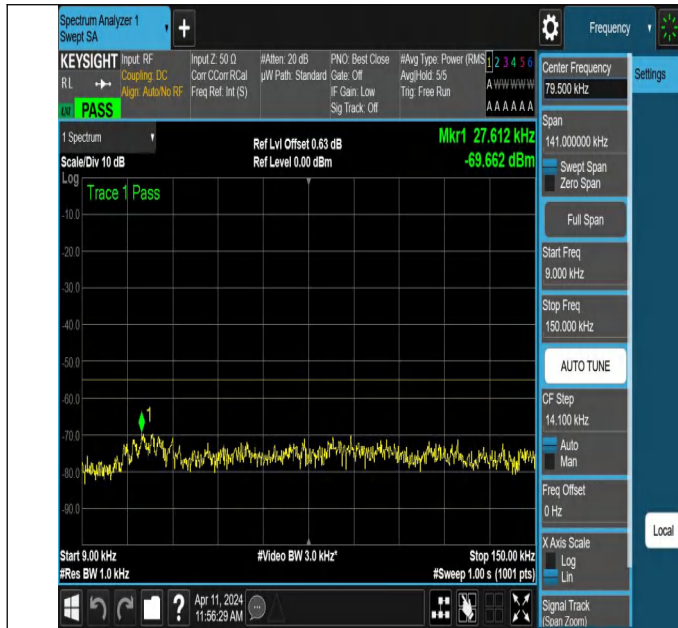
NTNV-N7-PC3-15-20-H-DFT-PI2BPSK-Edge_1RB_Left-0.009-0.15-Ant1-PASS
