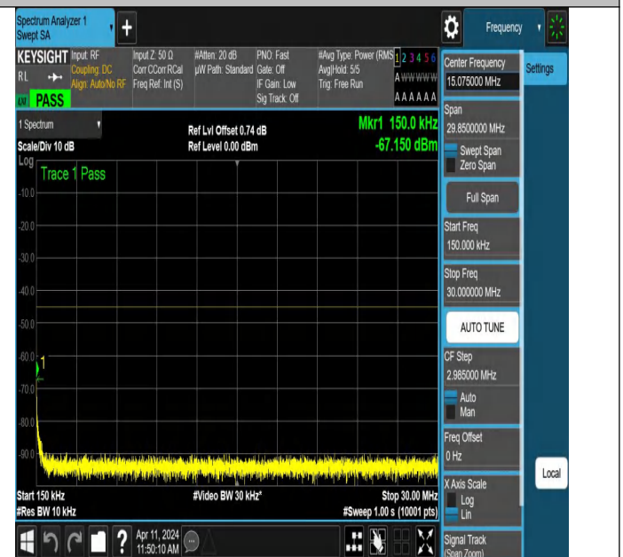
NTNV-N7-PC3-15-20-L-DFT-PI2BPSK-Edge_1RB_Right-0.15-30- Ant1-PASS
