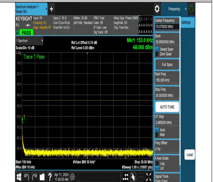
NTNV-N7-PC3-15-20-M-DFT-PI2BPSK-Edge_1RB_Right-0.15-30-Ant1-PASS
