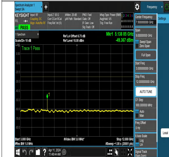
NTNV-N7-PC3-15-15-H-DFT-QPSK-Edge_1RB_Right-3000-1200 0-Ant1-PASS
