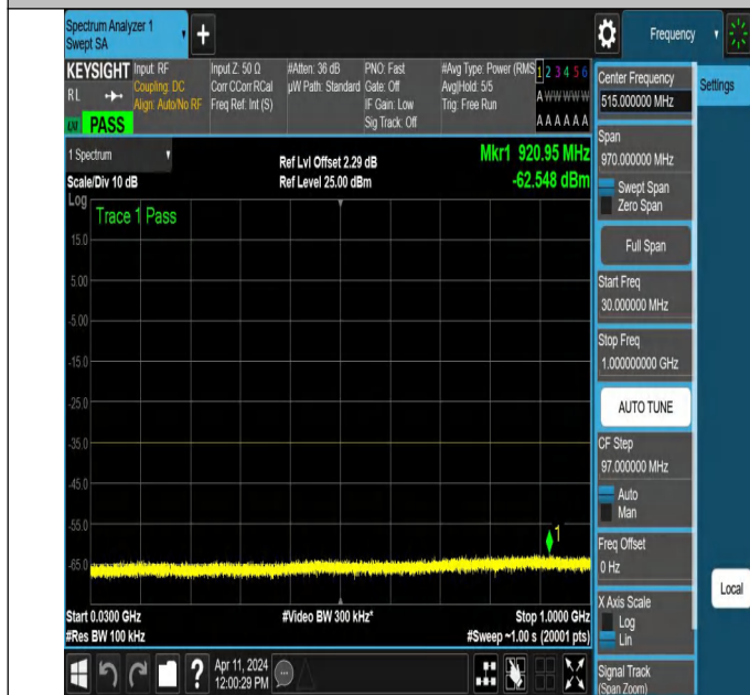
NTNV-N7-PC3-15-25-L-DFT-PI2BPSK-Edge_1RB_Left-30-1000- Ant1-PASS
