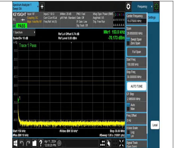
NTNV-N7-PC3-15-25-L-DFT-PI2BPSK-Edge_1RB_Left-0.15-30-A nt1-PASS
