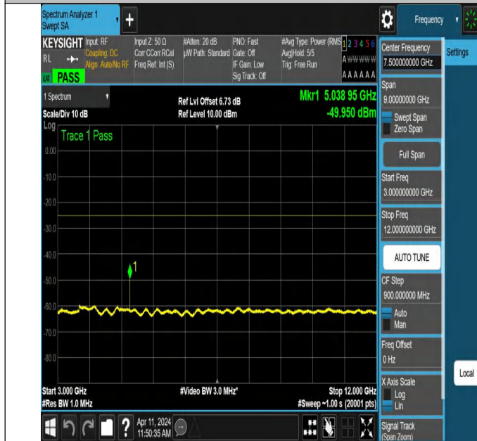
NTNV-N7-PC3-15-20-L-DFT-PI2BPSK-Edge_1RB_Right-3000-1 2000-Ant1-PASS
