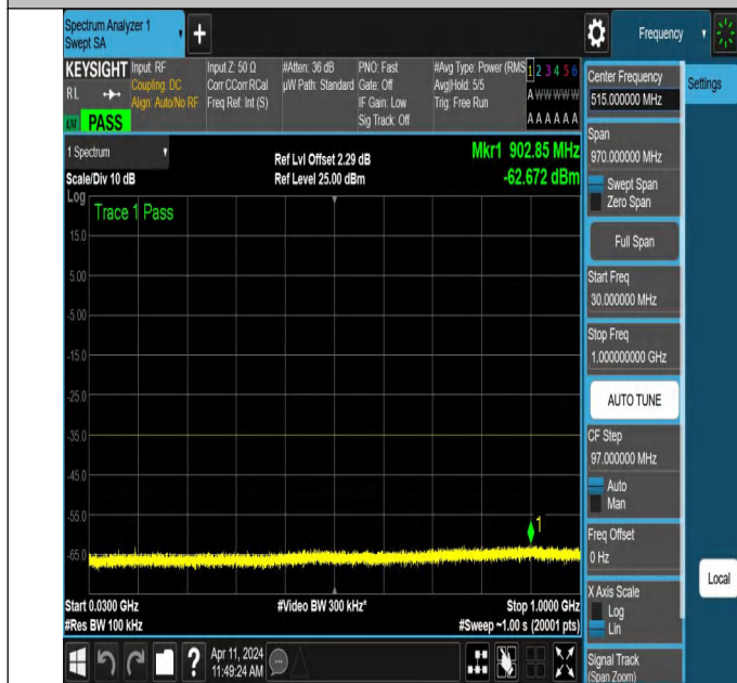
NTNV-N7-PC3-15-20-L-DFT-PI2BPSK-Edge_1RB_Left-30-1000- Ant1-PASS
