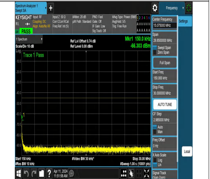
NTNV-N7-PC3-15-20-L-DFT-QPSK-Edge_1RB_Right-0.15-30-Ant 1-PASS
