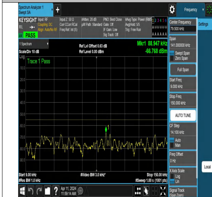
NTNV-N7-PC3-15-20-H-DFT-QPSK-Edge_1RB_Right-0.009-0.15 -Ant1-PASS
