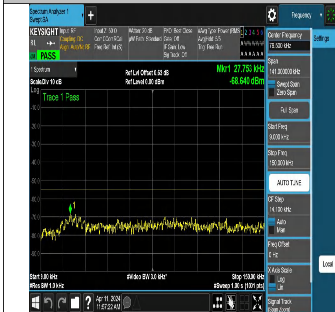
NTNV-N7-PC3-15-20-H-DFT-PI2BPSK-Edge_1RB_Right-0.009-0.15-Ant1-PASS
