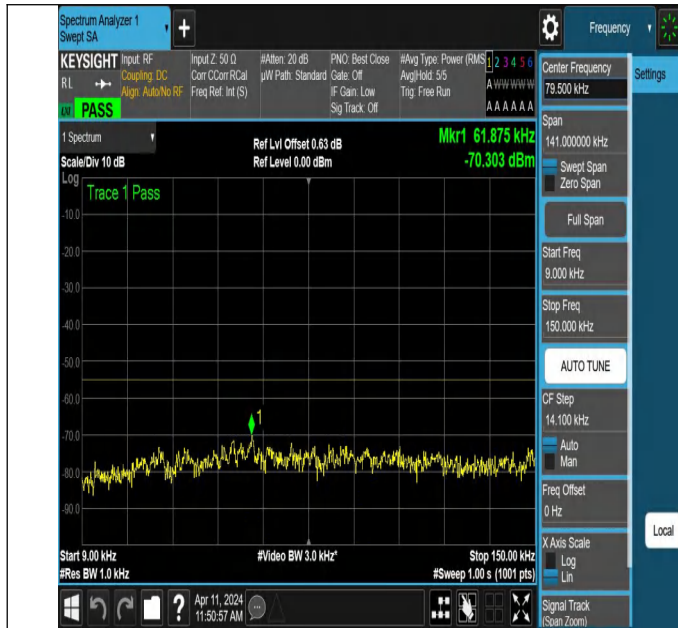
NTNV-N7-PC3-15-20-L-DFT-QPSK-Edge_1RB_Left-0.009-0.15-Ant1-PASS
