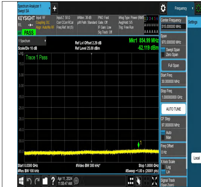
NTNV-N7-PC3-15-20-M-DFT-QPSK-Edge_1RB_Right-30-1000-Ant1-PASS
