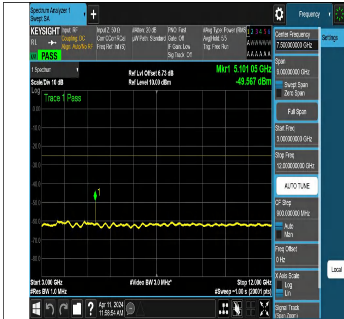
NTNV-N7-PC3-15-20-H-DFT-QPSK-Edge_1RB_Left-3000-12000 -Ant1-PASS
