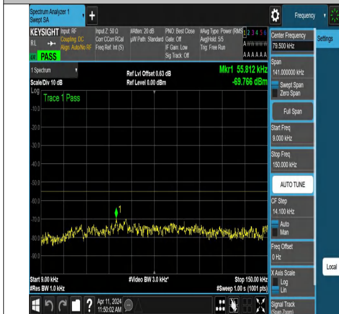
NTNV-N7-PC3-15-20-L-DFT-PI2BPSK-Edge_1RB_Right-0.009-0 .15-Ant1-PASS
