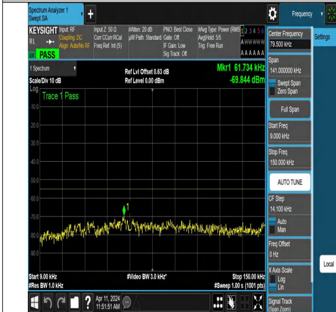
NTNV-N7-PC3-15-20-L-DFT-QPSK-Edge_1RB_Right-0.009-0.15 -Ant1-PASS
