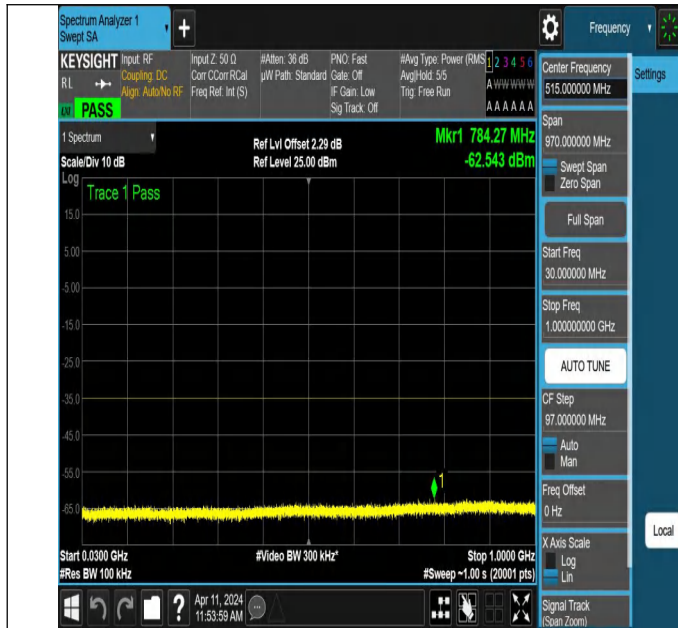
NTNV-N7-PC3-15-20-M-DFT-PI2BPSK-Edge_1RB_Right-30-100 0-Ant1-PASS
