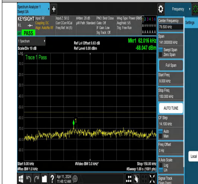
NTNV-N7-PC3-15-15-H-DFT-QPSK-Edge_1RB_Right-0.009-0.15 -Ant1-PASS
