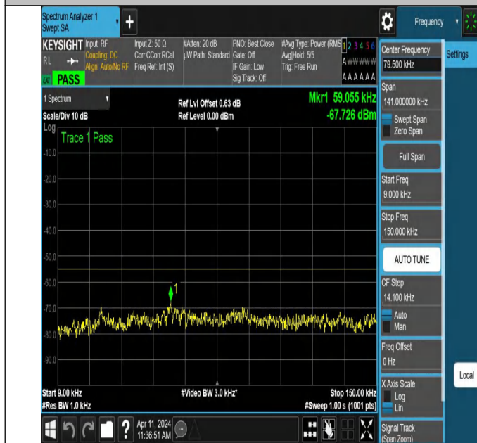
NTNV-N7-PC3-15-10-H-DFT-QPSK-Edge_1RB_Right-0.009-0.15 -Ant1-PASS
