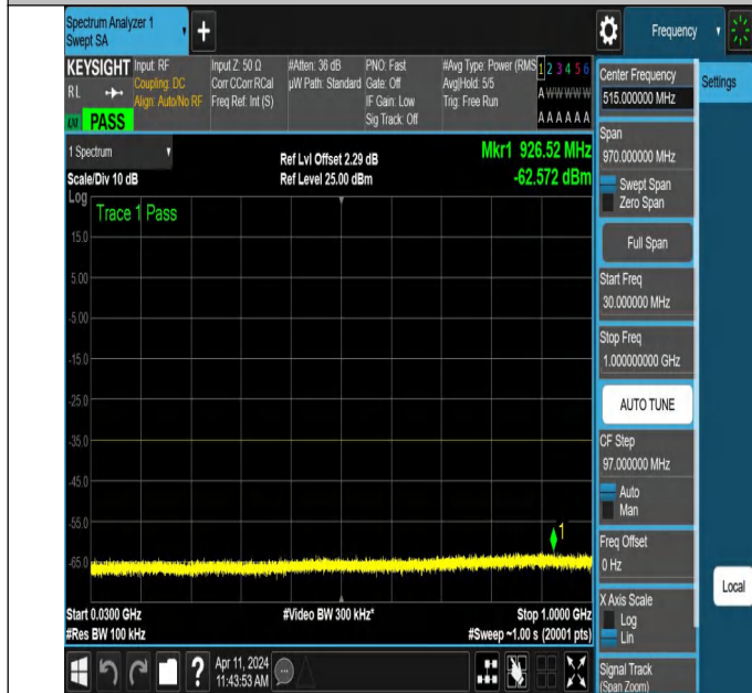
NTNV-N7-PC3-15-15-M-DFT-QPSK-Edge_1RB_Left-30-1000-Ant1-PASS
