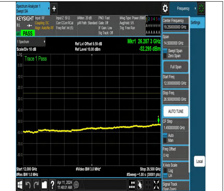
NTNV-N7-PC3-15-15-H-DFT-QPSK-Edge_1RB_Left-12000-26500 -Ant1-PASS
