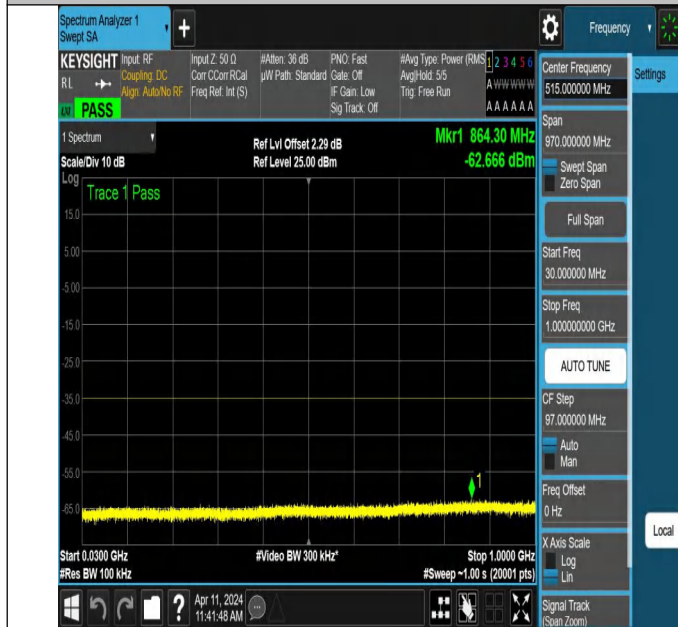
NTNV-N7-PC3-15-15-M-DFT-PI2BPSK-Edge_1RB_Left-30-1000- Ant1-PASS
