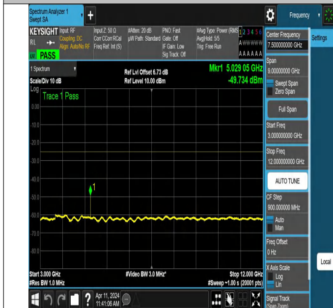
NTNV-N7-PC3-15-15-L-DFT-QPSK-Edge_1RB_Right-3000-1200 0-Ant1-PASS
