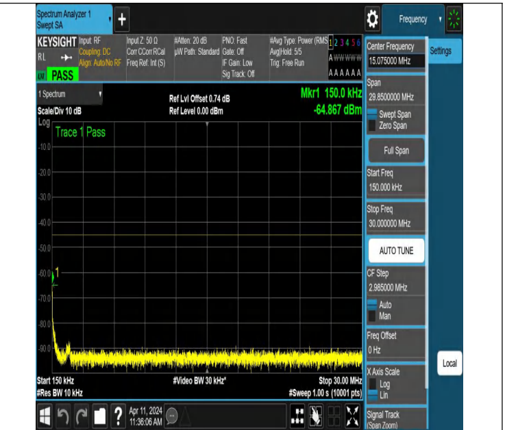
NTNV-N7-PC3-15-10-H-DFT-QPSK-Edge_1RB_Left-0.15-30-Ant1-PASS
