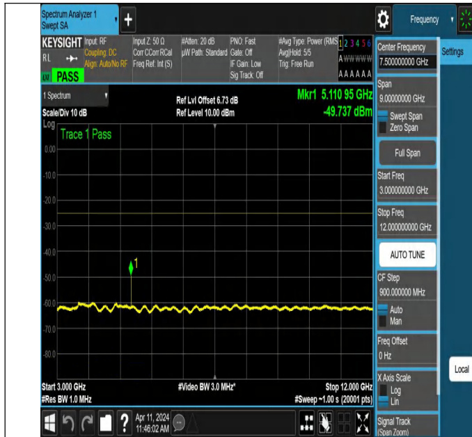
NTNV-N7-PC3-15-15-H-DFT-PI2BPSK-Edge_1RB_Left-3000-12000-Ant1-PASS
