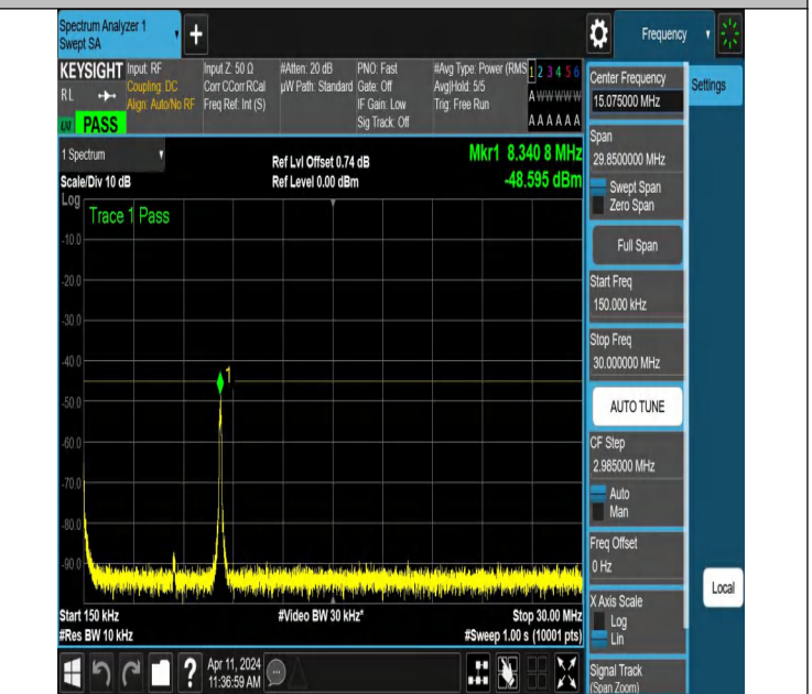
NTNV-N7-PC3-15-10-H-DFT-QPSK-Edge_1RB_Right-0.15-30-Ant 1-PASS
