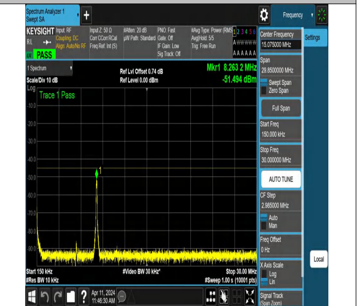
NTNV-N7-PC3-15-15-H-DFT-PI2BPSK-Edge_1RB_Right-0.15-30-Ant1-PASS
