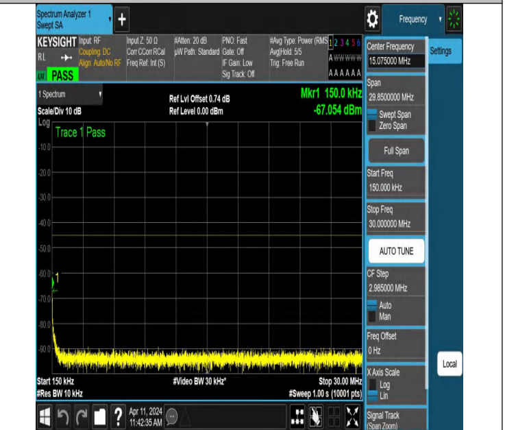
NTNV-N7-PC3-15-15-M-DFT-PI2BPSK-Edge_1RB_Right-0.15-30-Ant1-PASS
