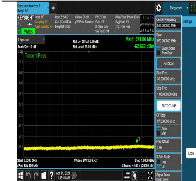
NTNV-N7-PC3-15-15-H-DFT-PI2BPSK-Edge_1RB_Left-30-1000-Ant1-PASS
