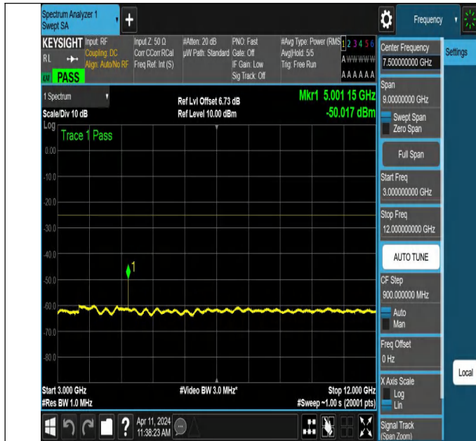
NTNV-N7-PC3-15-15-L-DFT-PI2BPSK-Edge_1RB_Left-3000-120 00-Ant1-PASS
