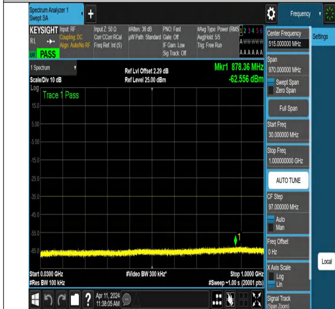
NTNV-N7-PC3-15-15-L-DFT-PI2BPSK-Edge_1RB_Left-30-1000- Ant1-PASS
