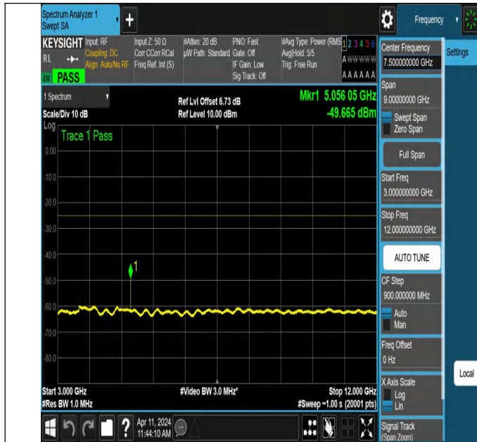
NTNV-N7-PC3-15-15-M-DFT-QPSK-Edge_1RB_Left-3000-12000 -Ant1-PASS
