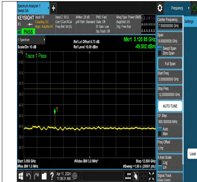
NTNV-N7-PC3-15-10-H-DFT-QPSK-Edge_1RB_Left-3000-12000 -Ant1-PASS
