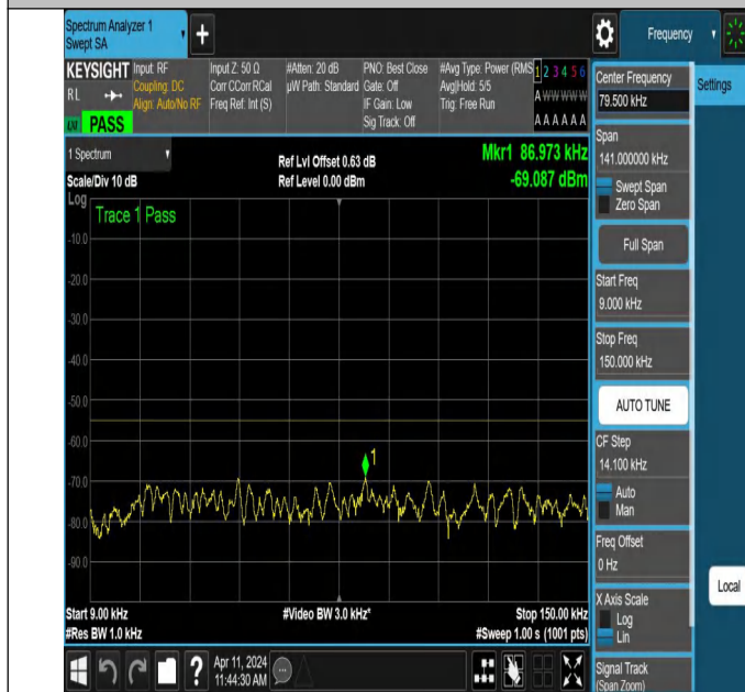
NTNV-N7-PC3-15-15-M-DFT-QPSK-Edge_1RB_Right-0.009-0.1 5-Ant1-PASS
