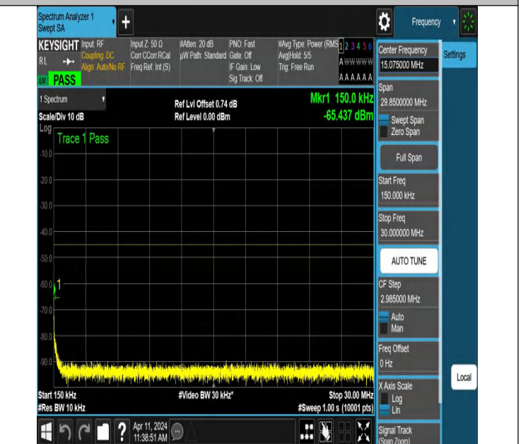
NTNV-N7-PC3-15-15-L-DFT-PI2BPSK-Edge_1RB_Right-0.15-30- Ant1-PASS
