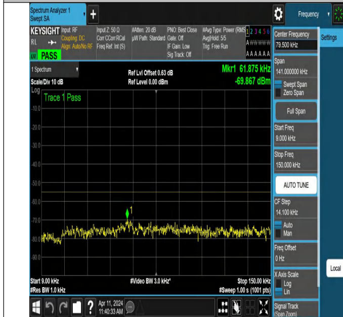
NTNV-N7-PC3-15-15-L-DFT-QPSK-Edge_1RB_Right-0.009-0.15 -Ant1-PASS
