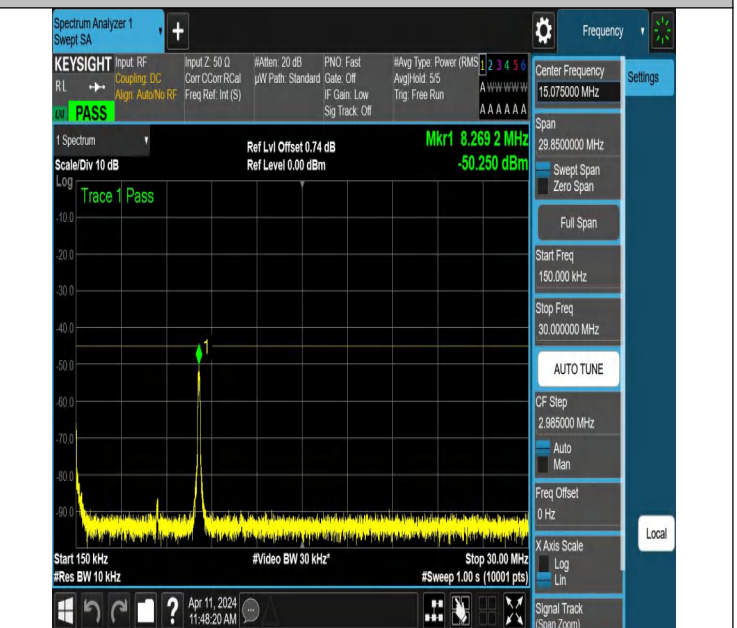
NTNV-N7-PC3-15-15-H-DFT-QPSK-Edge_1RB_Right-0.15-30-Ant 1-PASS
