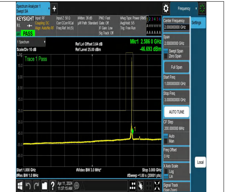
NTNV-N7-PC3-15-10-H-DFT-QPSK-Edge_1RB_Right-1000-3000- Ant1-PASS
