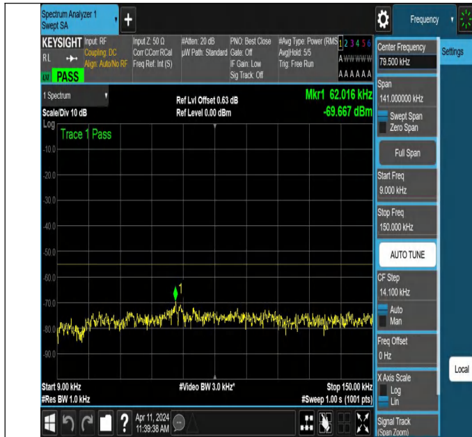
NTNV-N7-PC3-15-15-L-DFT-QPSK-Edge_1RB_Left-0.009-0.15-Ant1-PASS
