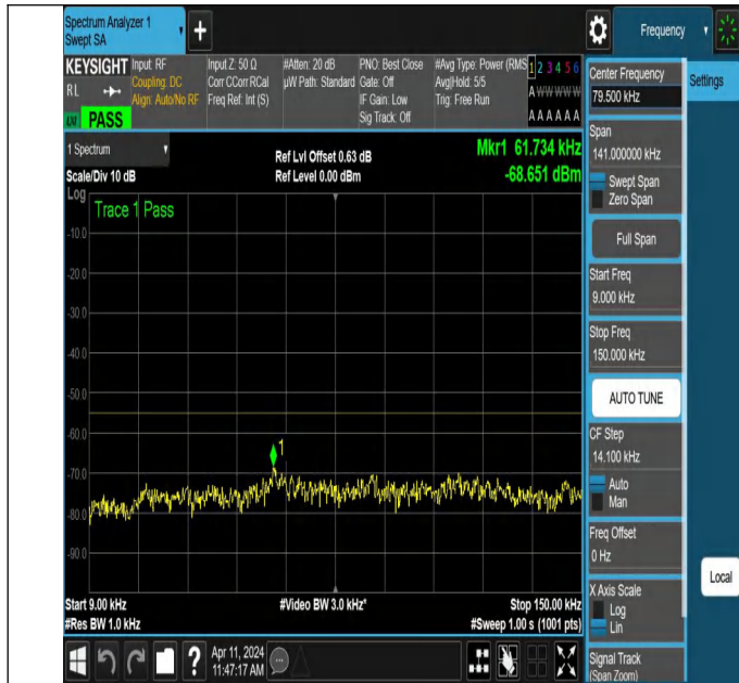
NTNV-N7-PC3-15-15-H-DFT-QPSK-Edge_1RB_Left-0.009-0.15-Ant1-PASS
