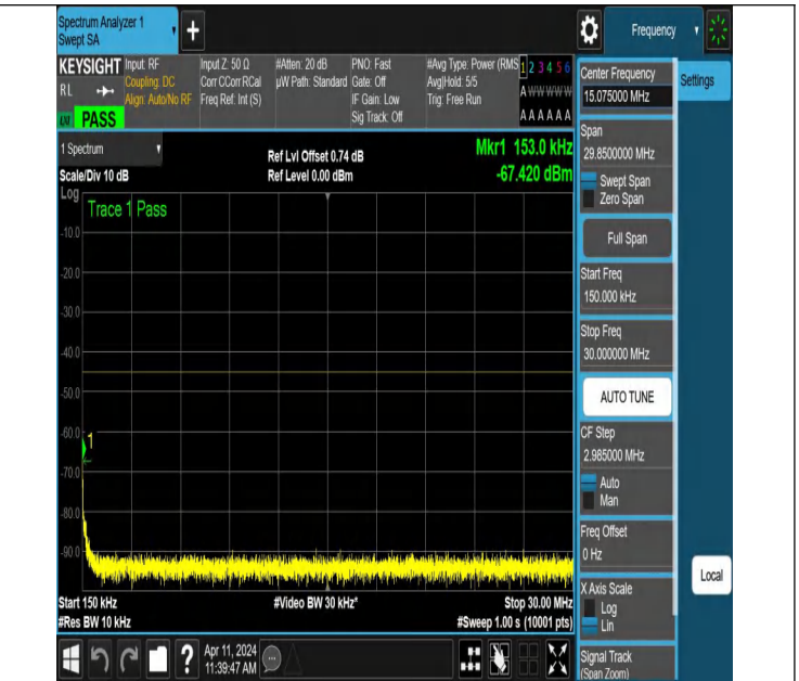
NTNV-N7-PC3-15-15-L-DFT-QPSK-Edge_1RB_Left-0.15-30-Ant1-PASS
