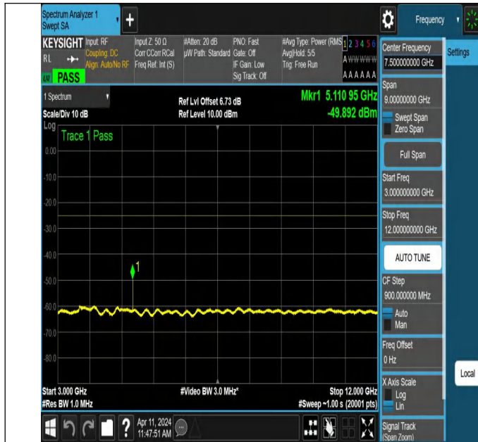
NTNV-N7-PC3-15-15-H-DFT-QPSK-Edge_1RB_Left-3000-12000 -Ant1-PASS
