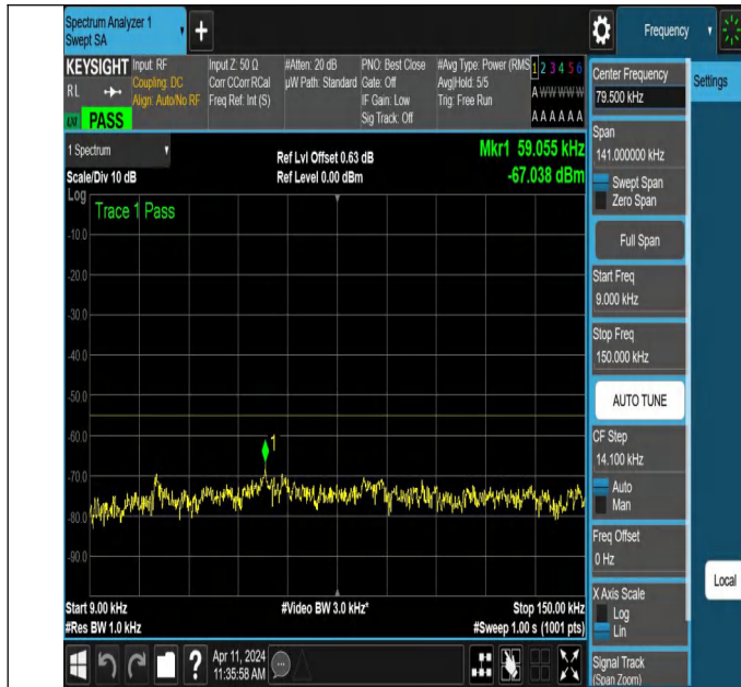
NTNV-N7-PC3-15-10-H-DFT-QPSK-Edge_1RB_Left-0.009-0.15-Ant1-PASS
