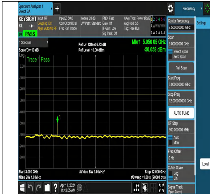
NTNV-N7-PC3-15-15-M-DFT-PI2BPSK-Edge_1RB_Left-3000-12000-Ant1-PASS
