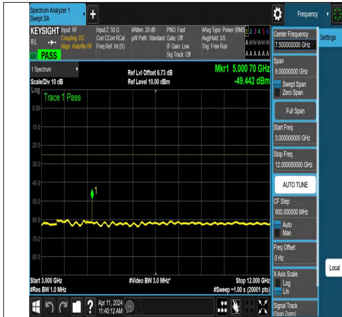
NTNV-N7-PC3-15-15-L-DFT-QPSK-Edge_1RB_Left-3000-12000- Ant1-PASS
