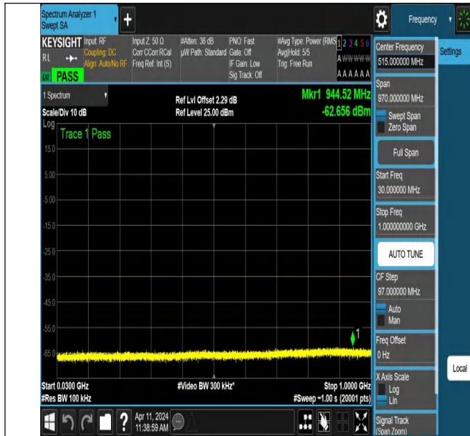
NTNV-N7-PC3-15-15-L-DFT-PI2BPSK-Edge_1RB_Right-30-100 0-Ant1-PASS
