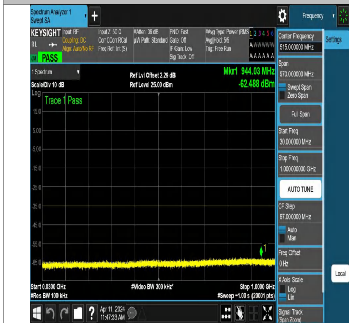
NTNV-N7-PC3-15-15-H-DFT-QPSK-Edge_1RB_Left-30-1000-Ant1-PASS
