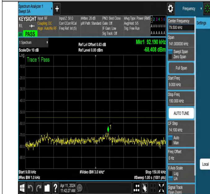
NTNV-N7-PC3-15-15-M-DFT-PI2BPSK-Edge_1RB_Right-0.009-0.15-Ant1-PASS
