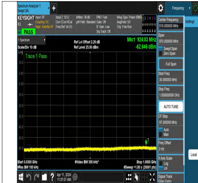
NTNV-N7-PC3-15-10-H-DFT-QPSK-Edge_1RB_Right-30-1000-A nt1-PASS
