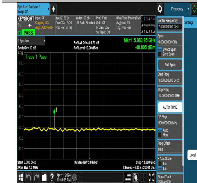
NTNV-N7-PC3-15-15-M-DFT-QPSK-Edge_1RB_Right-3000-120 00-Ant1-PASS
