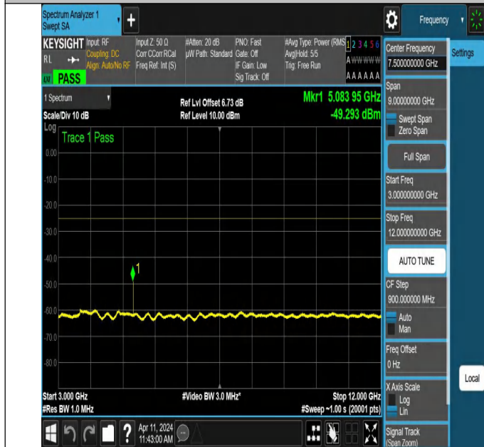
NTNV-N7-PC3-15-15-M-DFT-PI2BPSK-Edge_1RB_Right-3000-1 2000-Ant1-PASS
