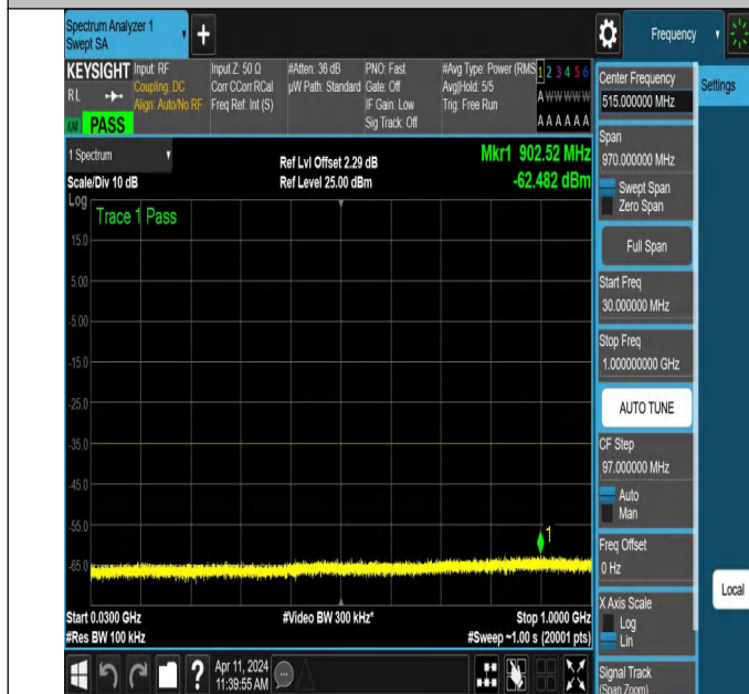
NTNV-N7-PC3-15-15-L-DFT-QPSK-Edge_1RB_Left-30-1000-Ant1-PASS
