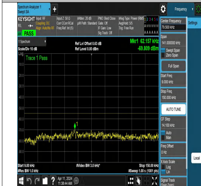
NTNV-N7-PC3-15-15-L-DFT-PI2BPSK-Edge_1RB_Right-0.009-0 .15-Ant1-PASS
