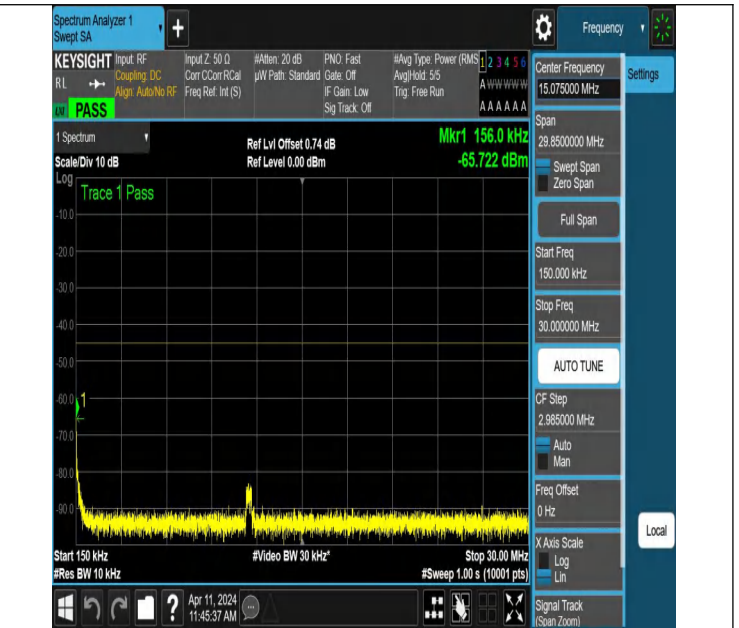
NTNV-N7-PC3-15-15-H-DFT-PI2BPSK-Edge_1RB_Left-0.15-30-Ant1-PASS
