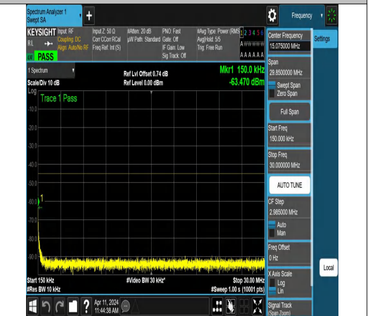
NTNV-N7-PC3-15-15-M-DFT-QPSK-Edge_1RB_Right-0.15-30-An t1-PASS
