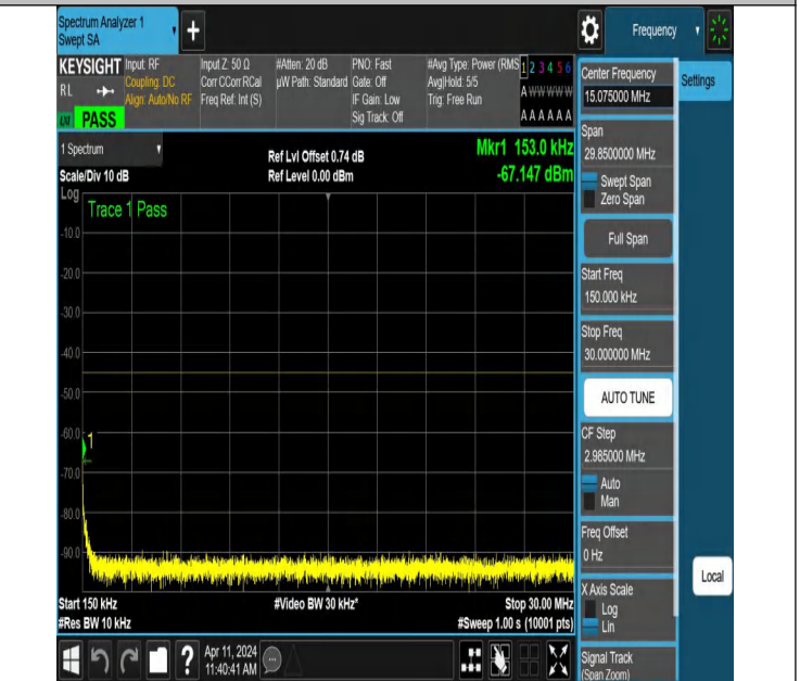
NTNV-N7-PC3-15-15-L-DFT-QPSK-Edge_1RB_Right-0.15-30-Ant 1-PASS
