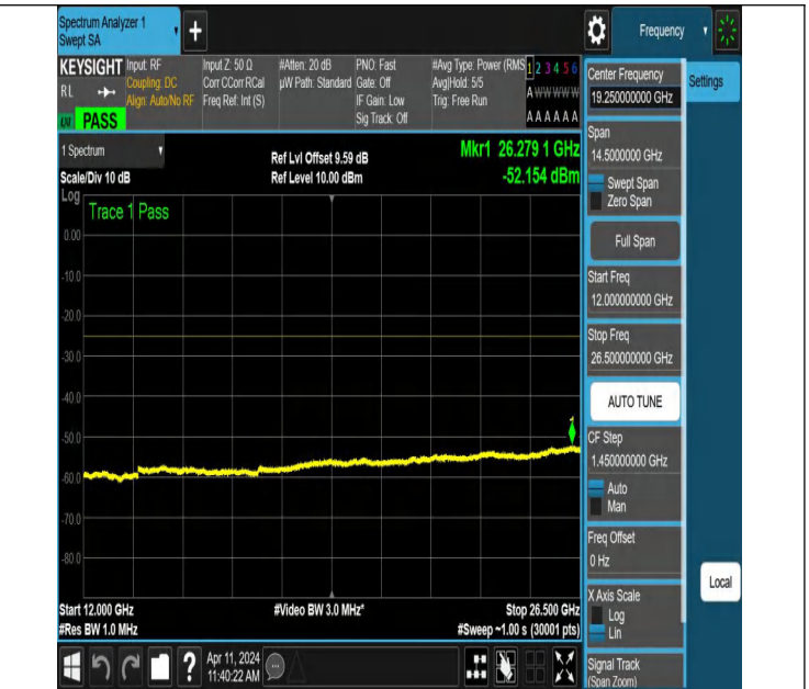
NTNV-N7-PC3-15-15-L-DFT-QPSK-Edge_1RB_Left-12000-26500 -Ant1-PASS
