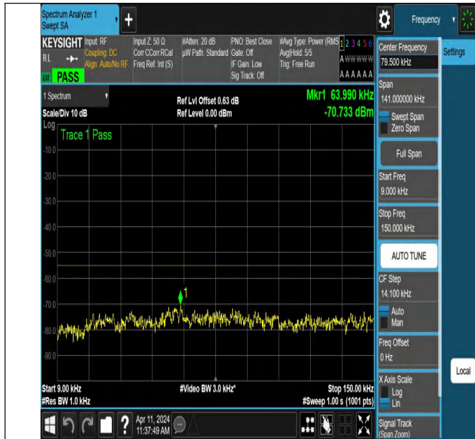
NTNV-N7-PC3-15-15-L-DFT-PI2BPSK-Edge_1RB_Left-0.009-0.1 5-Ant1-PASS
