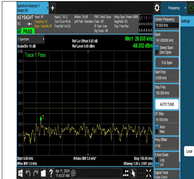
NTNV-N7-PC3-15-15-M-DFT-QPSK-Edge_1RB_Left-0.009-0.15-Ant1-PASS
