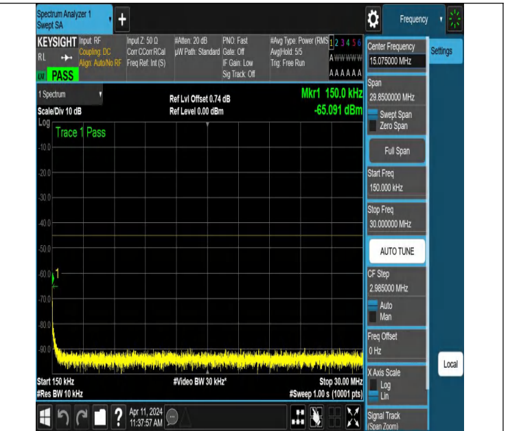
NTNV-N7-PC3-15-15-L-DFT-PI2BPSK-Edge_1RB_Left-0.15-30-A nt1-PASS
