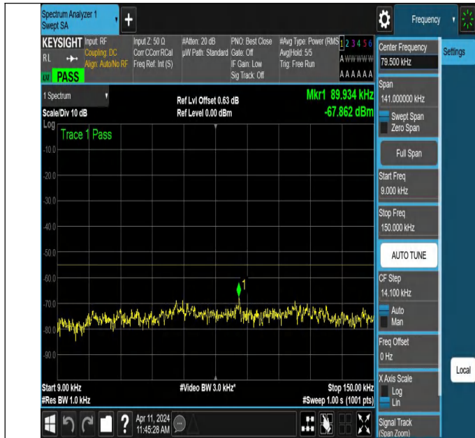
NTNV-N7-PC3-15-15-H-DFT-PI2BPSK-Edge_1RB_Left-0.009-0.15-Ant1-PASS
