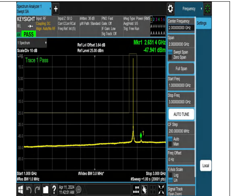
NTNV-N7-PC3-15-15-M-DFT-PI2BPSK-Edge_1RB_Right-1000-30 00-Ant1-PASS
