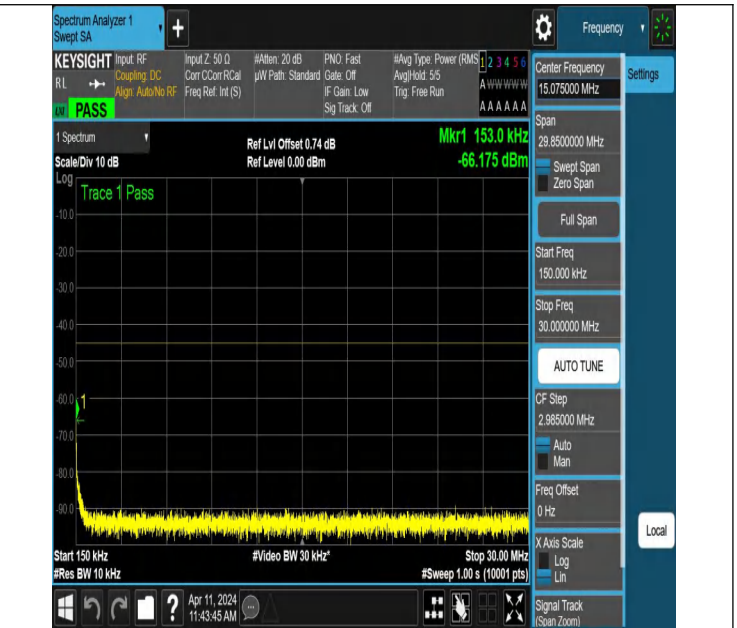
NTNV-N7-PC3-15-15-M-DFT-QPSK-Edge_1RB_Left-0.15-30-Ant1-PASS
