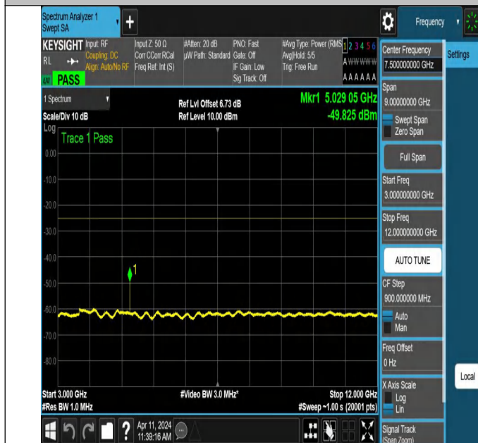
NTNV-N7-PC3-15-15-L-DFT-PI2BPSK-Edge_1RB_Right-3000-1 2000-Ant1-PASS
