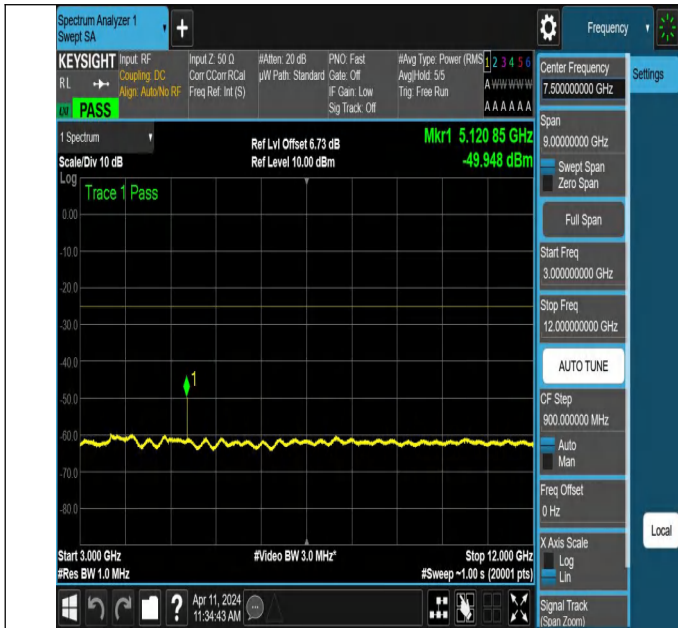
NTNV-N7-PC3-15-10-H-DFT-PI2BPSK-Edge_1RB_Left-3000-12000-Ant1-PASS
