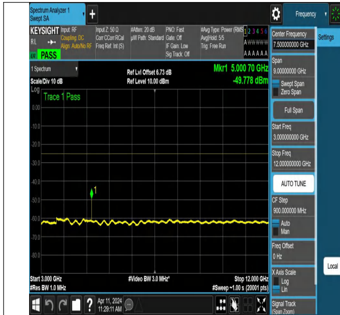
NTNV-N7-PC3-15-10-L-DFT-QPSK-Edge_1RB_Left-3000-12000- Ant1-PASS
