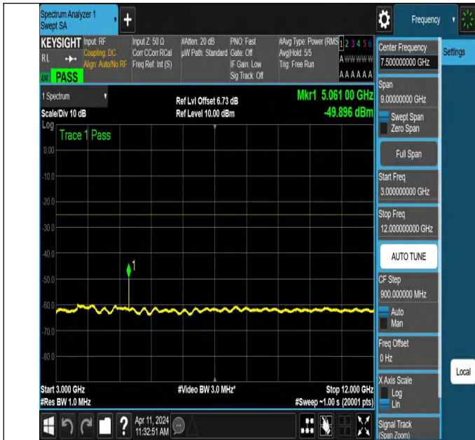
NTNV-N7-PC3-15-10-M-DFT-QPSK-Edge_1RB_Left-3000-12000 -Ant1-PASS
