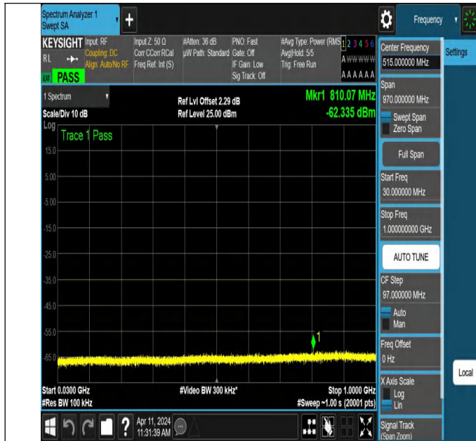
NTNV-N7-PC3-15-10-M-DFT-PI2BPSK-Edge_1RB_Right-30-100 0-Ant1-PASS
