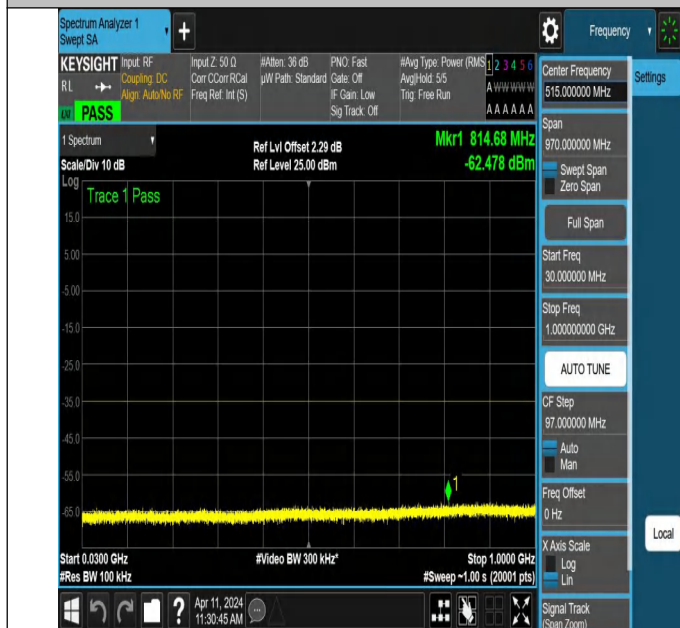
NTNV-N7-PC3-15-10-M-DFT-PI2BPSK-Edge_1RB_Left-30-1000-Ant1-PASS
