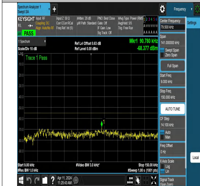
NTNV-N7-PC3-15-5-H-DFT-QPSK-Edge_1RB_Right-0.009-0.15-Ant1-PASS
