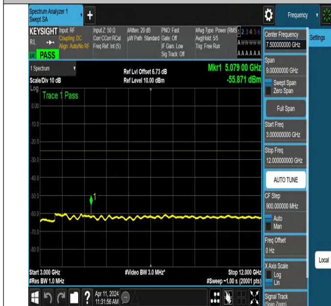
NTNV-N7-PC3-15-10-M-DFT-PI2BPSK-Edge_1RB_Right-3000-1 2000-Ant1-PASS
