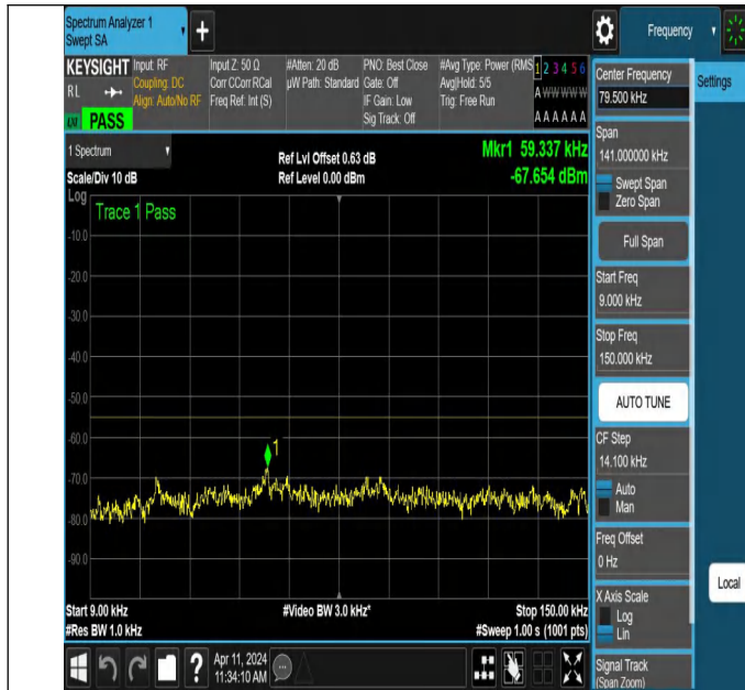
NTNV-N7-PC3-15-10-H-DFT-PI2BPSK-Edge_1RB_Left-0.009-0.15-Ant1-PASS
