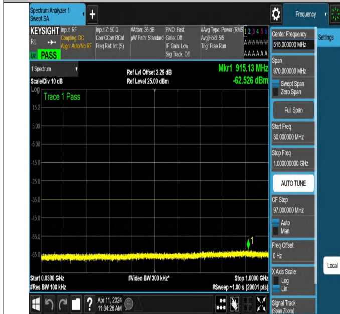
NTNV-N7-PC3-15-10-H-DFT-PI2BPSK-Edge_1RB_Left-30-1000-Ant1-PASS
