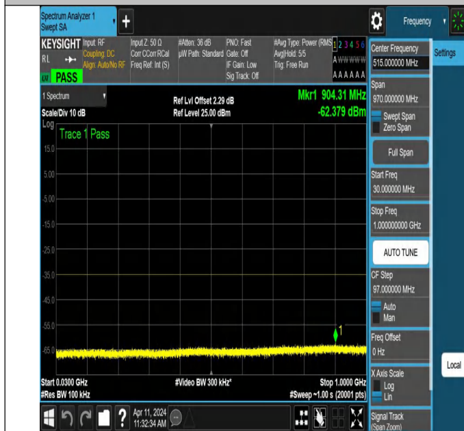
NTNV-N7-PC3-15-10-M-DFT-QPSK-Edge_1RB_Left-30-1000-Ant1-PASS
