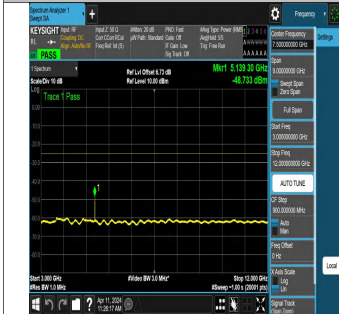
NTNV-N7-PC3-15-5-H-DFT-QPSK-Edge_1RB_Right-3000-12000 -Ant1-PASS
