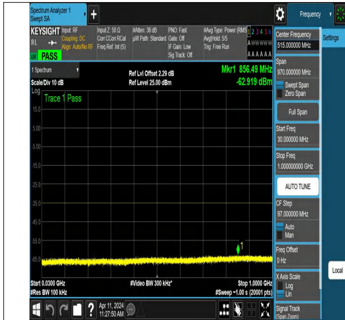
NTNV-N7-PC3-15-10-L-DFT-PI2BPSK-Edge_1RB_Right-30-100 0-Ant1-PASS
