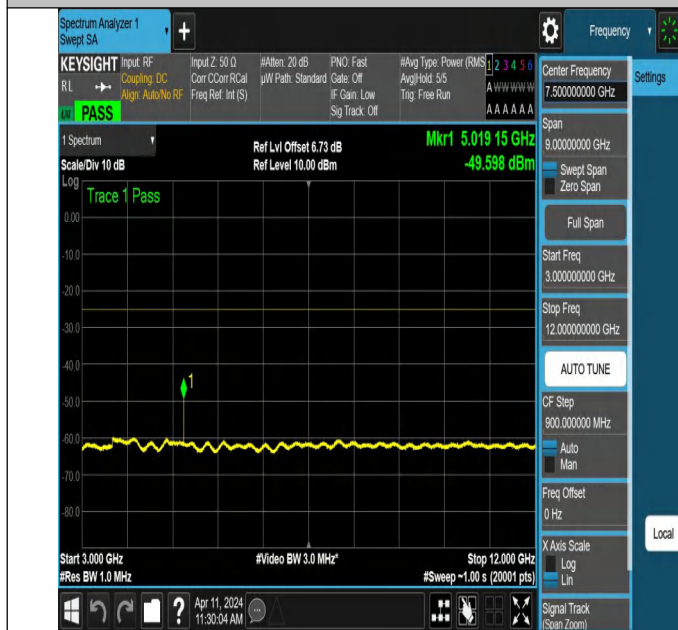
NTNV-N7-PC3-15-10-L-DFT-QPSK-Edge_1RB_Right-3000-1200 0-Ant1-PASS
