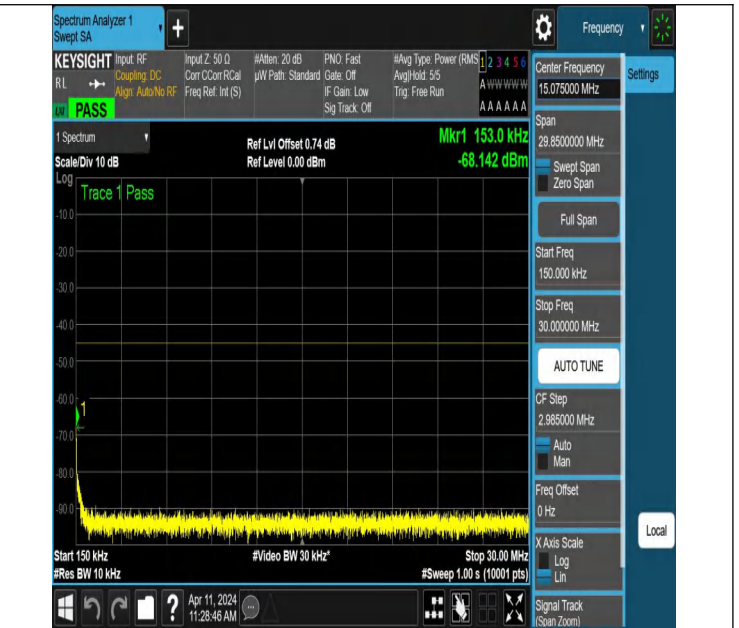
NTNV-N7-PC3-15-10-L-DFT-QPSK-Edge_1RB_Left-0.15-30-Ant1-PASS
