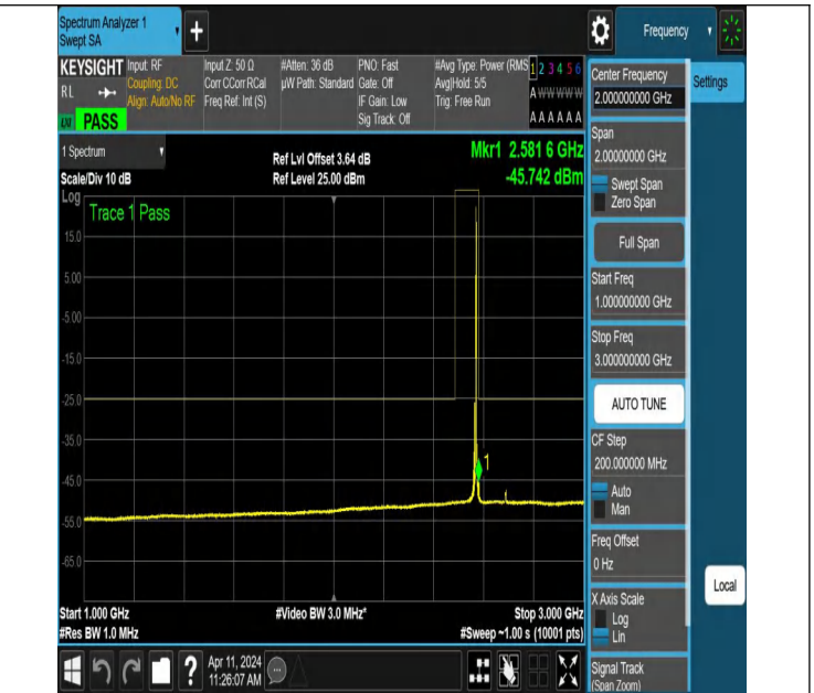
NTNV-N7-PC3-15-5-H-DFT-QPSK-Edge_1RB_Right-1000-3000-A nt1-PASS
