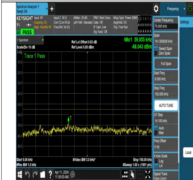
NTNV-N7-PC3-15-10-H-DFT-PI2BPSK-Edge_1RB_Right-0.009-0.15-Ant1-PASS
