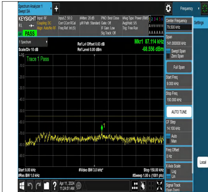
NTNV-N7-PC3-15-5-H-DFT-QPSK-Edge_1RB_Left-0.009-0.15-A nt1-PASS
