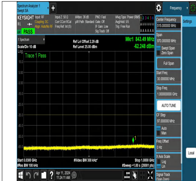
NTNV-N7-PC3-15-5-H-DFT-PI2BPSK-Edge_1RB_Right-30-1000-Ant1-PASS
