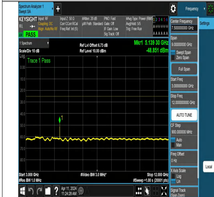
NTNV-N7-PC3-15-5-H-DFT-PI2BPSK-Edge_1RB_Right-3000-12000-Ant1-PASS
