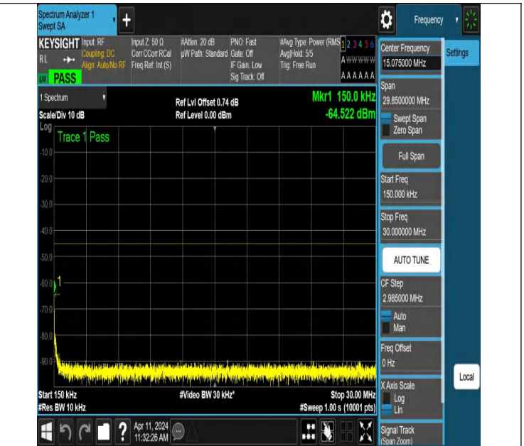
NTNV-N7-PC3-15-10-M-DFT-QPSK-Edge_1RB_Left-0.15-30-Ant1-PASS
