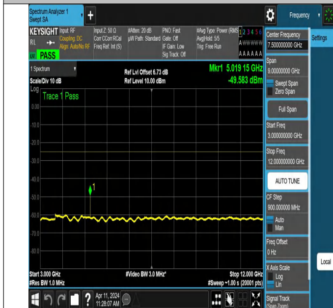
NTNV-N7-PC3-15-10-L-DFT-PI2BPSK-Edge_1RB_Right-3000-1 2000-Ant1-PASS
