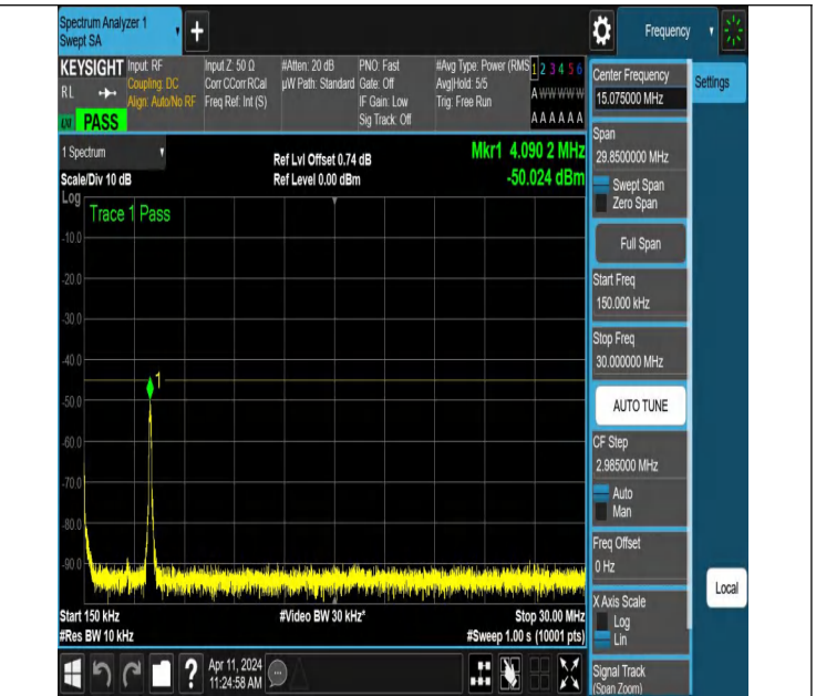
NTNV-N7-PC3-15-5-H-DFT-QPSK-Edge_1RB_Left-0.15-30-Ant1- PASS
