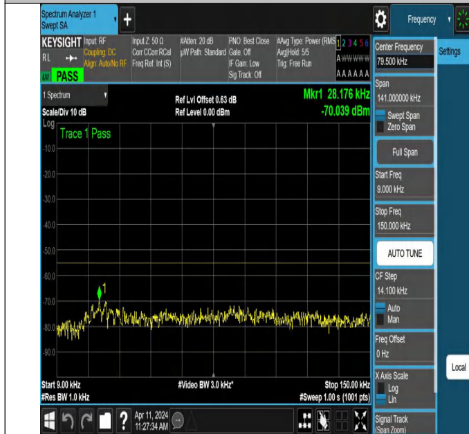
NTNV-N7-PC3-15-10-L-DFT-PI2BPSK-Edge_1RB_Right-0.009-0 .15-Ant1-PASS
