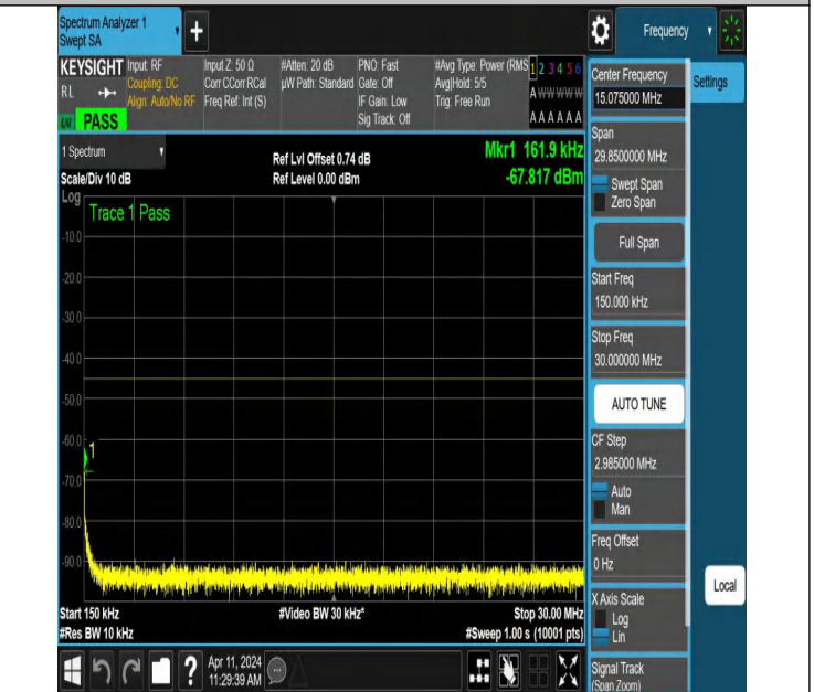
NTNV-N7-PC3-15-10-L-DFT-QPSK-Edge_1RB_Right-0.15-30-Ant 1-PASS
