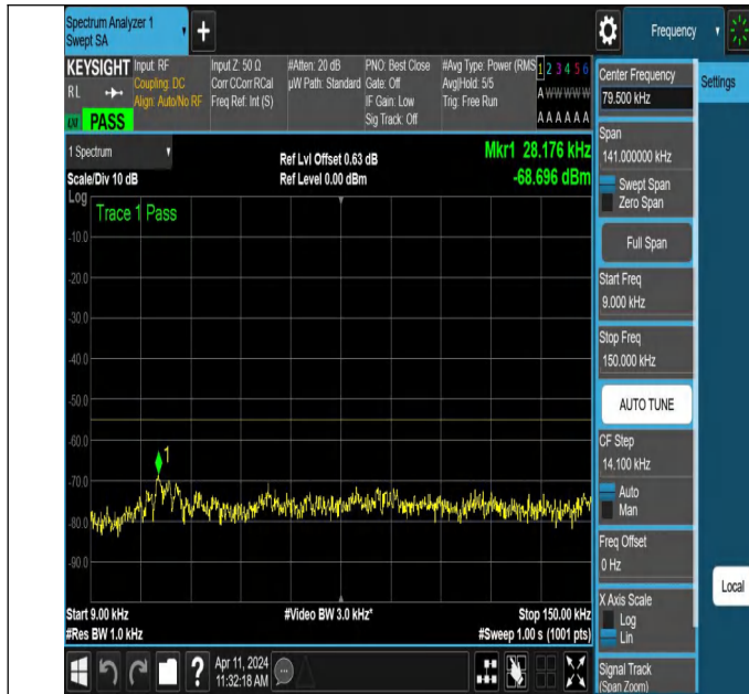
NTNV-N7-PC3-15-10-M-DFT-QPSK-Edge_1RB_Left-0.009-0.15-Ant1-PASS
