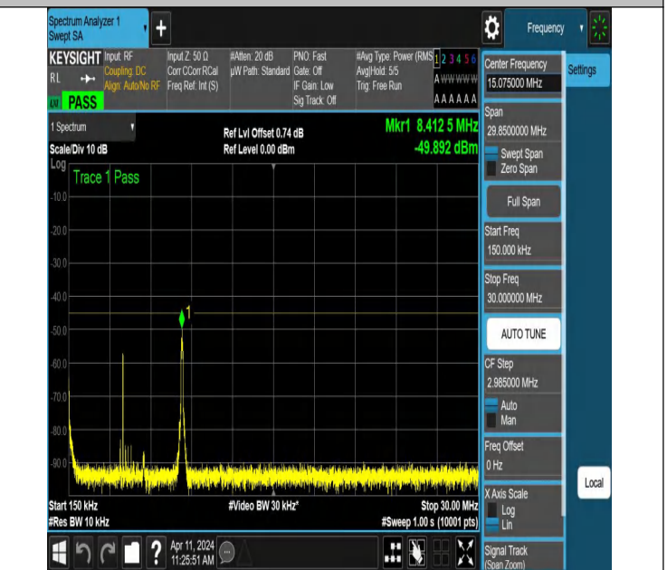
NTNV-N7-PC3-15-5-H-DFT-QPSK-Edge_1RB_Right-0.15-30-Ant1-PASS
