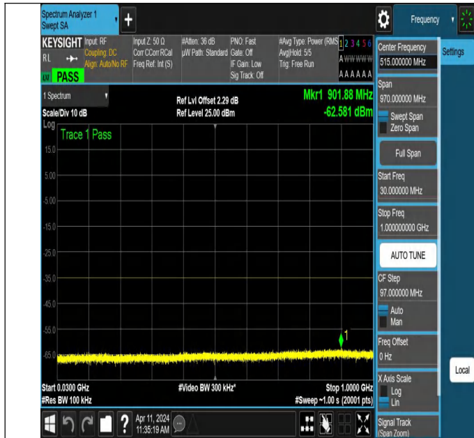
NTNV-N7-PC3-15-10-H-DFT-PI2BPSK-Edge_1RB_Right-30-100 0-Ant1-PASS
