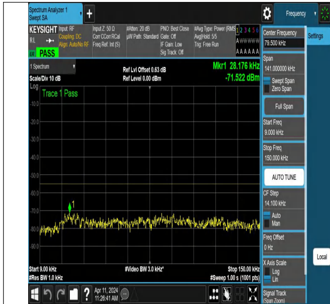
NTNV-N7-PC3-15-10-L-DFT-PI2BPSK-Edge_1RB_Left-0.009-0.1 5-Ant1-PASS
