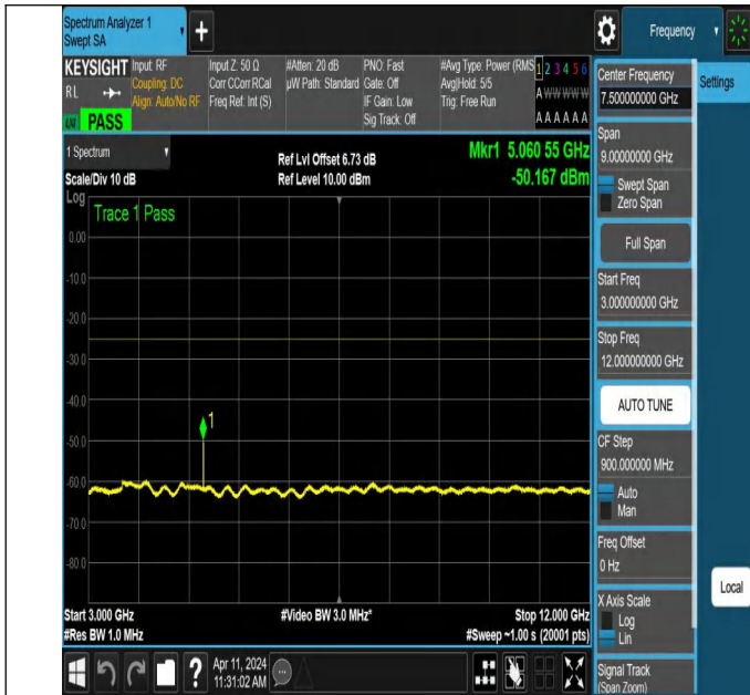
NTNV-N7-PC3-15-10-M-DFT-PI2BPSK-Edge_1RB_Left-3000-12000-Ant1-PASS
