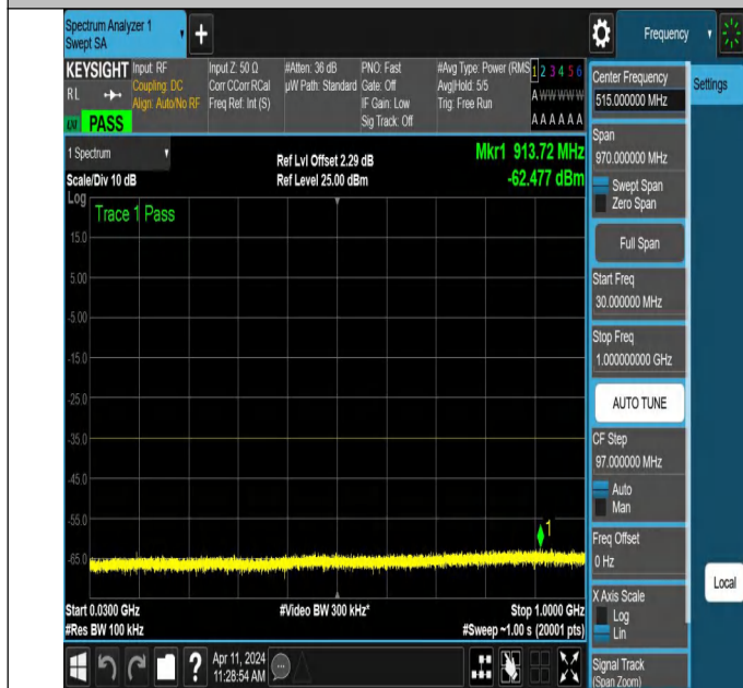
NTNV-N7-PC3-15-10-L-DFT-QPSK-Edge_1RB_Left-30-1000-Ant1-PASS
