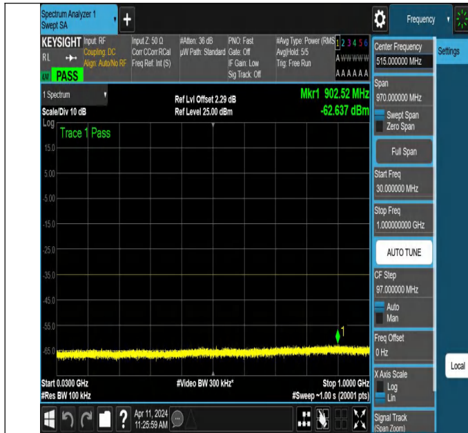
NTNV-N7-PC3-15-5-H-DFT-QPSK-Edge_1RB_Right-30-1000-An t1-PASS
