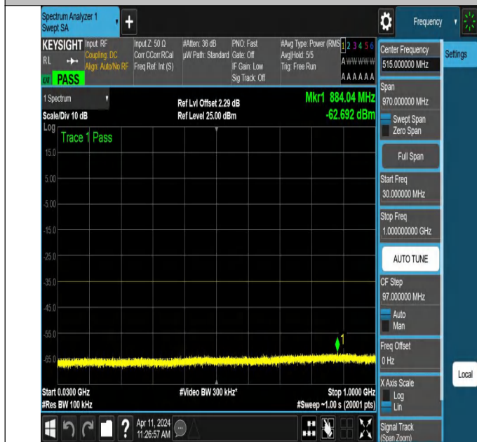
NTNV-N7-PC3-15-10-L-DFT-PI2BPSK-Edge_1RB_Left-30-1000- Ant1-PASS
