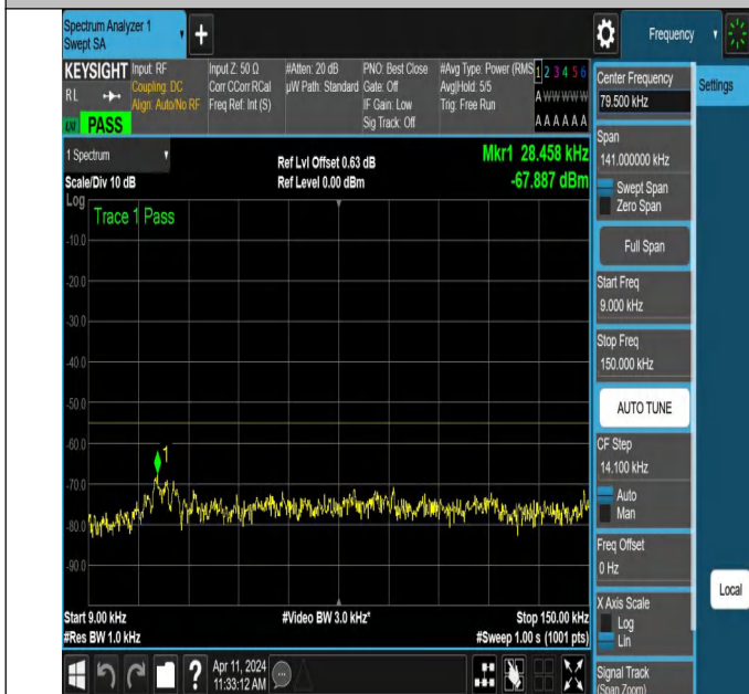
NTNV-N7-PC3-15-10-M-DFT-QPSK-Edge_1RB_Right-0.009-0.1 5-Ant1-PASS
