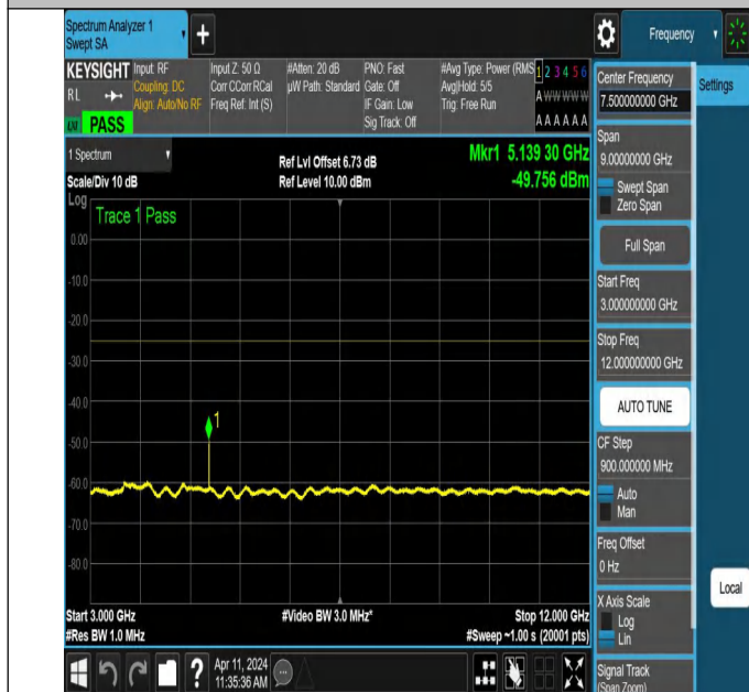
NTNV-N7-PC3-15-10-H-DFT-PI2BPSK-Edge_1RB_Right-3000-1 2000-Ant1-PASS
