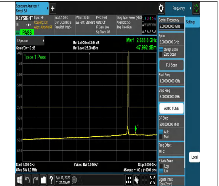
NTNV-N7-PC3-15-5-H-DFT-PI2BPSK-Edge_1RB_Right-1000-300-0-Ant1-PASS
