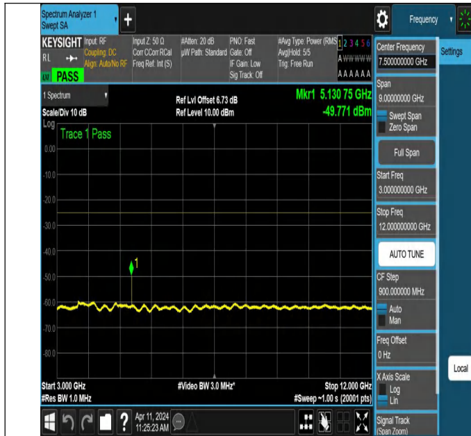
NTNV-N7-PC3-15-5-H-DFT-QPSK-Edge_1RB_Left-3000-12000-Ant1-PASS
