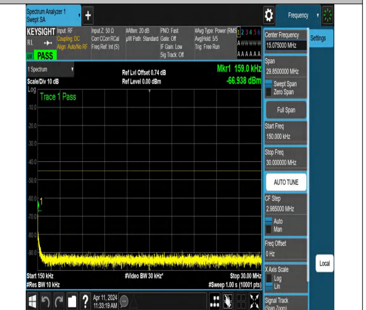
NTNV-N7-PC3-15-10-M-DFT-QPSK-Edge_1RB_Right-0.15-30-An t1-PASS
