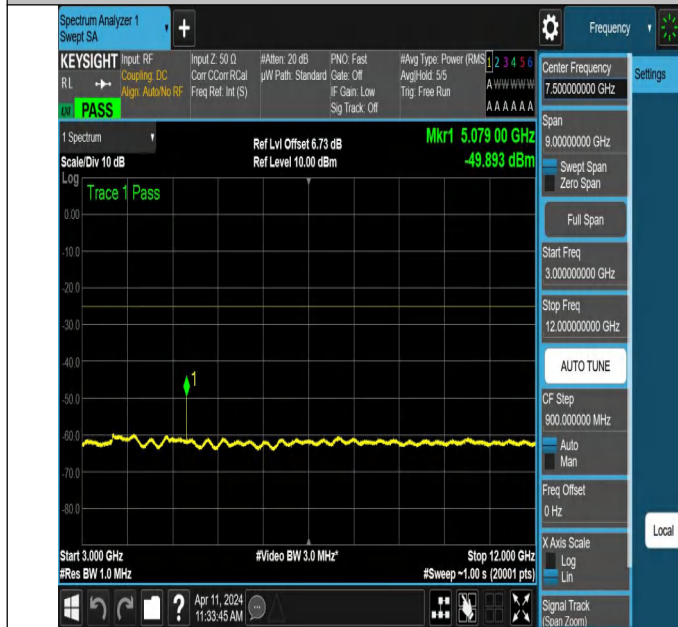
NTNV-N7-PC3-15-10-M-DFT-QPSK-Edge_1RB_Right-3000-120 00-Ant1-PASS
