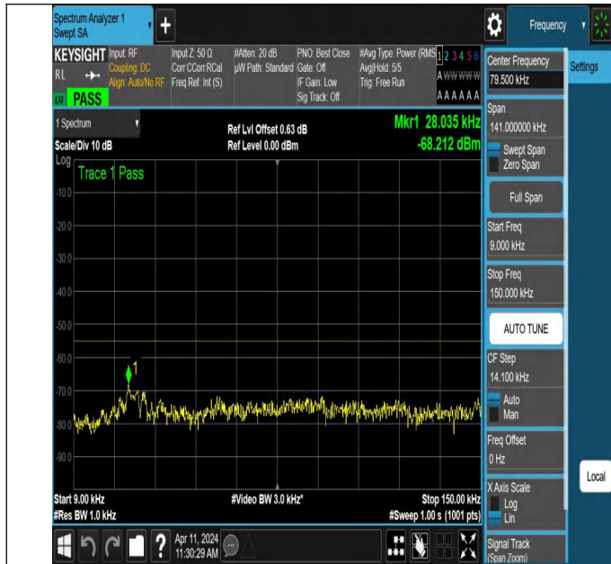
NTNV-N7-PC3-15-10-M-DFT-PI2BPSK-Edge_1RB_Left-0.009-0.15-Ant1-PASS
