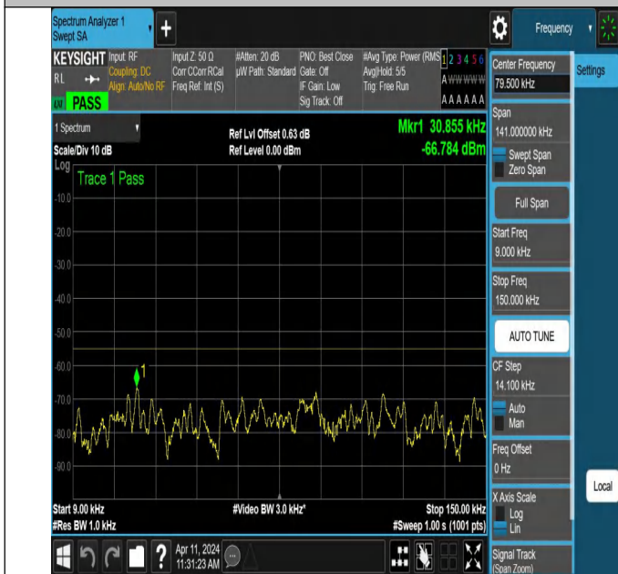
NTNV-N7-PC3-15-10-M-DFT-PI2BPSK-Edge_1RB_Right-0.009-0.15-Ant1-PASS
