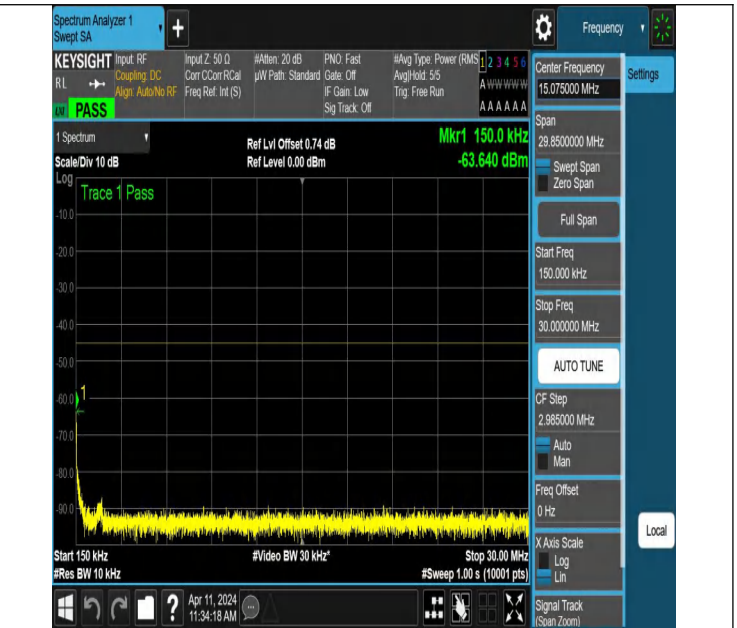
NTNV-N7-PC3-15-10-H-DFT-PI2BPSK-Edge_1RB_Left-0.15-30-Ant1-PASS
