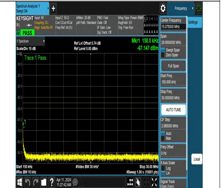
NTNV-N7-PC3-15-10-L-DFT-PI2BPSK-Edge_1RB_Right-0.15-30- Ant1-PASS
