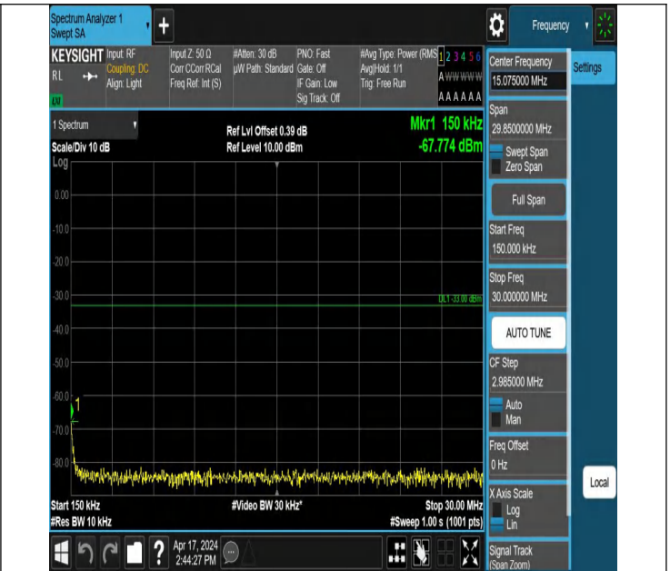
66-66-20MHz-15MHz-QPSK-QPSK-132423-132594-1RB#99-0RB B#0-0.15~30MHz-PASS
