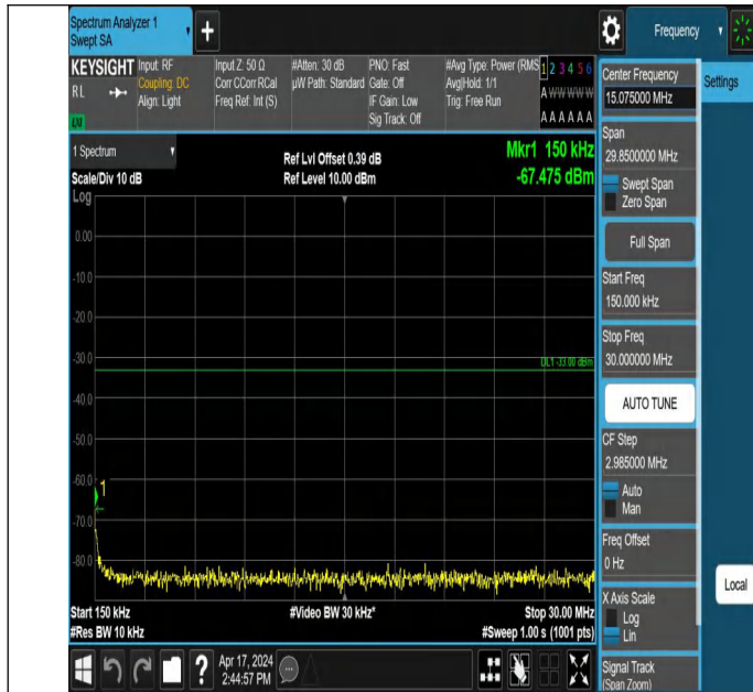
66-66-20MHz-15MHz-QPSK-QPSK-132423-132594-1RB#0-1RB# 74-0.15~30MHz-PASS
