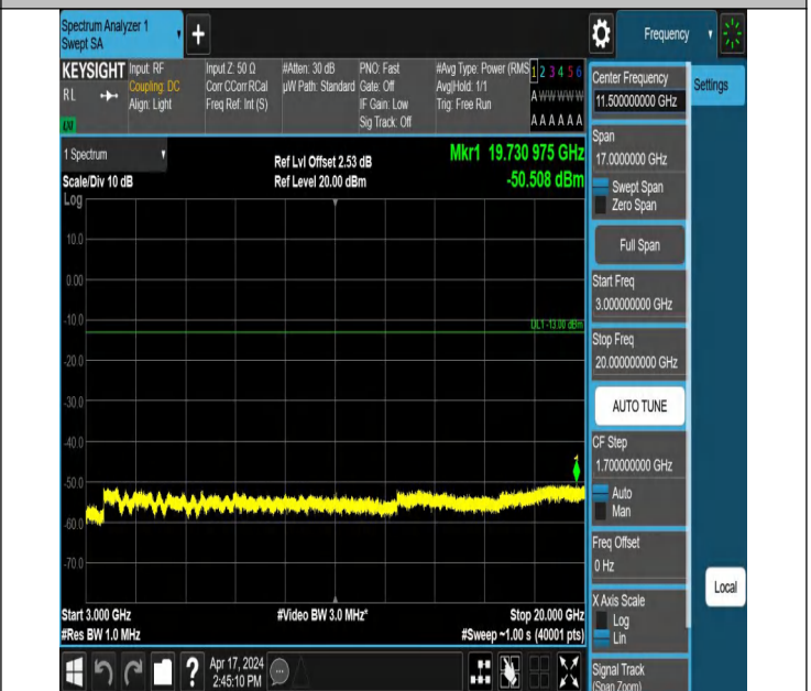
66-66-20MHz-15MHz-QPSK-QPSK-132423-132594-1RB#0-1RB #74-3000~20000MHz-PASS
