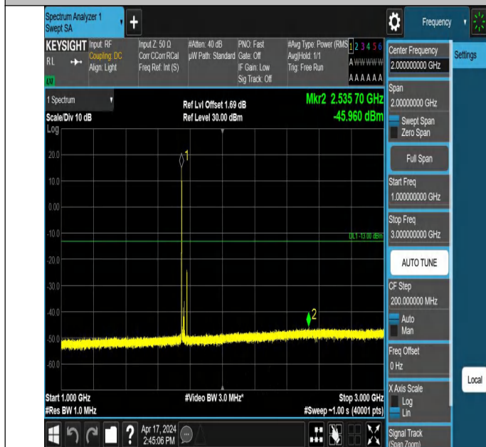
66-66-20MHz-15MHz-QPSK-QPSK-132423-132594-1RB#0-1RB# 74-1000~3000MHz-PASS
